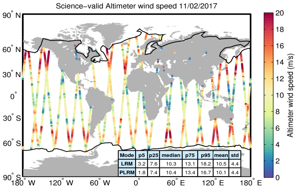
Figure 34. Geographical distribution of science-valid wind data over oceans and lakes for 11/02/2017. The statistical values shown in the table refer to the wind in m/s and are calculated separately for LRM and PLRM regions. The black lines mark the outer limit of the Arctic and Antarctic polar polygons. Gray circles denote records that have been rejected based on the editing criteria described in Table 5.
