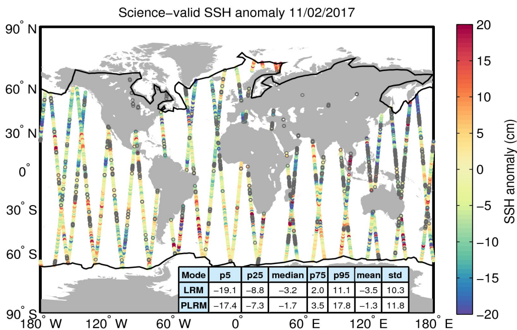
Figure 10. Geographical distribution of science-valid SSH anomaly data over oceans and lakes for 11/02/2017. The statistical values shown in the table refer to the SSH anomaly in cm and are calculated separately for LRM and PLRM regions. The black lines mark the outer limit of the Arctic and Antarctic polar polygons. Gray circles denote records that have been rejected based on the editing criteria described in Table 2.
