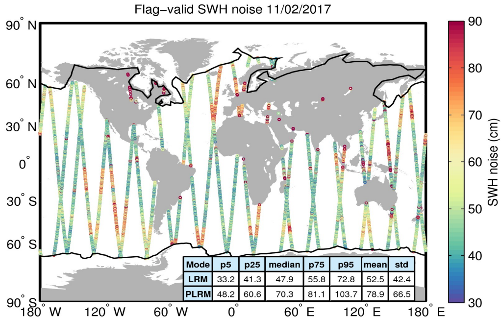
Figure 18. Geographical distribution of flag-valid 20-Hz SWH measurement noise over oceans and lakes for 11/02/2017. The statistical values shown in the table refer to the SWH noise and are calculated separately for LRM and PLRM regions. Measurements taken over polar polygons have been excluded from the computation of the statistical values. The black lines mark the outer limit of the Arctic and Antarctic polar polygons.
