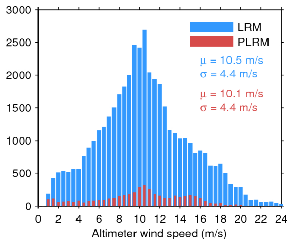
Figure 35. Histogram of science-valid wind over oceans and lakes for LRM (blue) and PLRM (red) for 11/02/2017. The mean ( \mu ) and standard deviation ( \sigma ) are also shown. Note that values larger than 24 m/s are excluded from the histogram for the sake of readability but not from the computation of \mu and \sigma .
