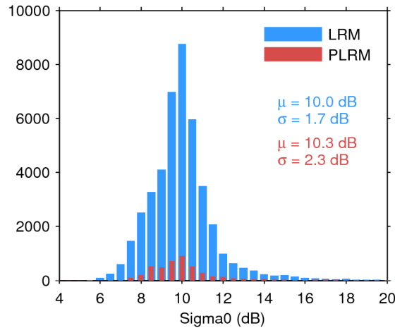
Figure 25. Histogram of flag-valid sigma0 over oceans and lakes for LRM (blue) and PLRM (red) for 11/02/2017. The mean ( \mu ) and standard deviation ( \sigma ) are also shown. Note that values outside [4 20] dB are excluded from the histogram for the sake of readability but not from the computation of \mu and \sigma .
