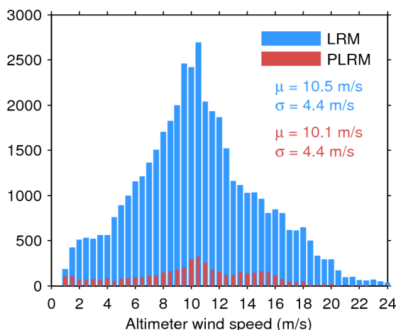
Figure 33. Histogram of flag-valid wind over oceans and lakes for LRM (blue) and PLRM (red) for 11/02/2017. The mean ( \mu ) and standard deviation ( \sigma ) are also shown. Note that values larger than 24 m/s are excluded from the histogram for the sake of readability but not from the computation of \mu and \sigma .
