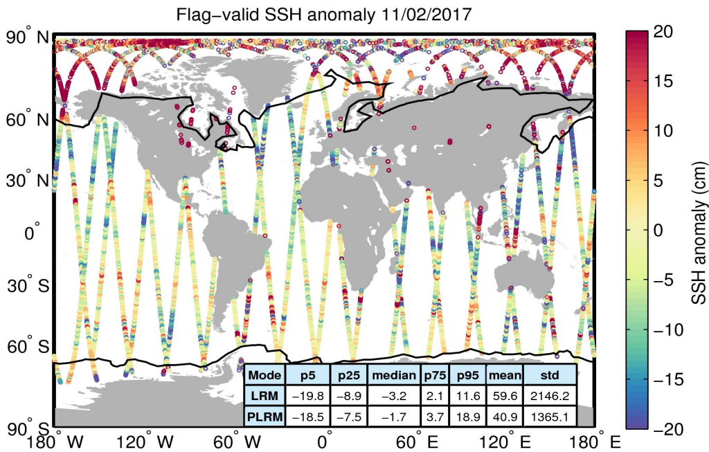
Figure 5. Geographical distribution of flag-valid 1-Hz SSH anomaly data over oceans and lakes for 11/02/2017. The statistical values shown in the table refer to the SSH anomaly in cm and are calculated separately for LRM and PLRM regions. Measurements taken over polar polygons have been excluded from the computation of the statistical values. The black lines mark the outer limit of the Arctic and Antarctic polar polygons.
