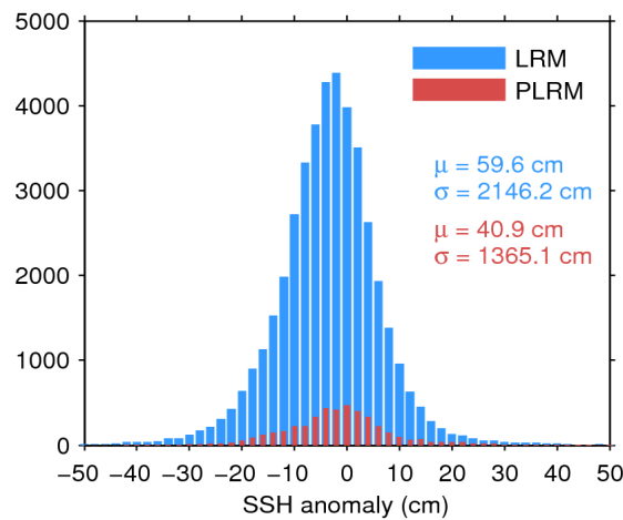
Figure 7. Histogram of flag-valid SSH anomaly over oceans and lakes for LRM (blue) and PLRM (red) for 11/02/2017. The mean ( \mu ) and standard deviation ( \sigma ) are also shown. Note that values outside [-50 50] cm are excluded from the histogram for the sake of readability but not from the computation of \mu and \sigma .
