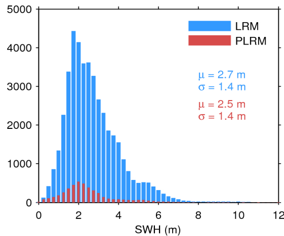
Figure 17. Histogram of flag-valid SWH over oceans and lakes for LRM (blue) and PLRM (red) for 11/02/2017. The mean ( \mu ) and standard deviation ( \sigma ) are also shown. Note that values larger than 12 m are excluded from the histogram for the sake of readability but not from the computation of \mu and \sigma .
