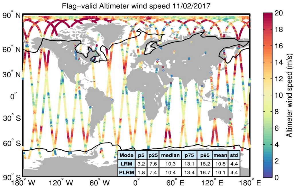
Figure 31. Geographical distribution of flag-valid wind data over oceans and lakes for 11/02/2017. The statistical values shown in the table refer to the wind in m/s and are calculated separately for LRM and PLRM regions. Measurements taken over polar polygons have been excluded from the computation of the statistical values. The black lines mark the outer limit of the Arctic and Antarctic polar polygons.
