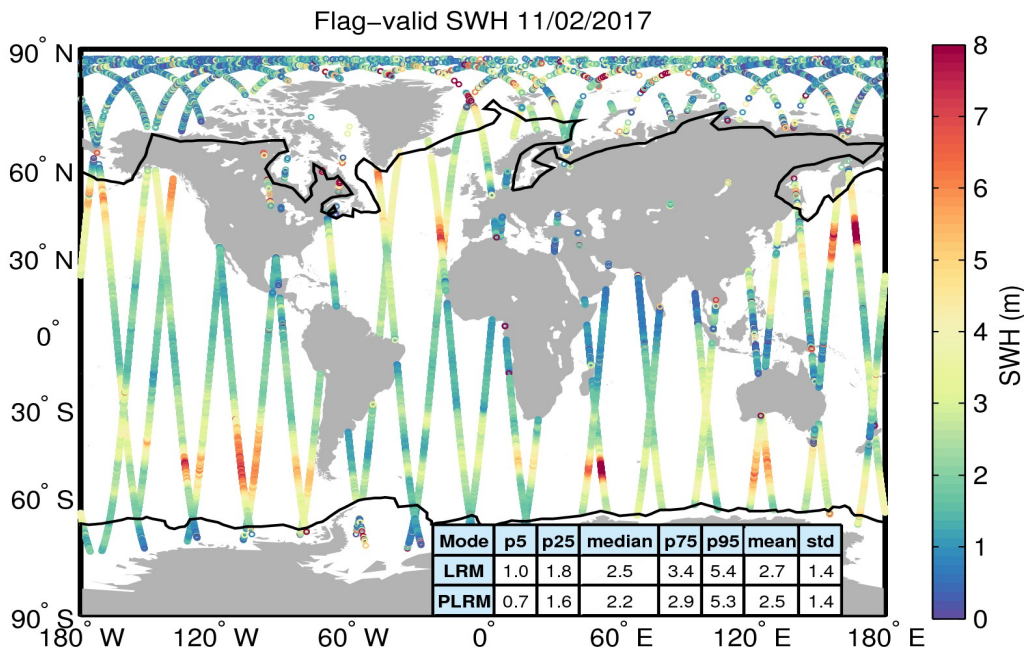
Figure 15. Geographical distribution of flag-valid SWH data over oceans and lakes for 11/02/2017. The statistical values shown in the table refer to the SWH in m and are calculated separately for LRM and PLRM regions. Measurements taken over polar polygons have been excluded from the computation of the statistical values. The black lines mark the outer limit of the Arctic and Antarctic polar polygons.
