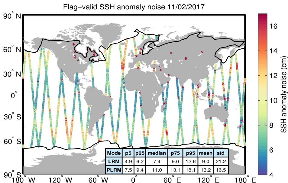
Figure 8. Geographical distribution of flag-valid 20-Hz SSH anomaly measurement noise over oceans and lakes for 11/02/2017. The statistical values shown in the table refer to the SSH anomaly noise and are calculated separately for LRM and PLRM regions. Measurements taken over polar polygons have been excluded from the computation of the statistical values. The black lines mark the outer limit of the Arctic and Antarctic polar polygons.
