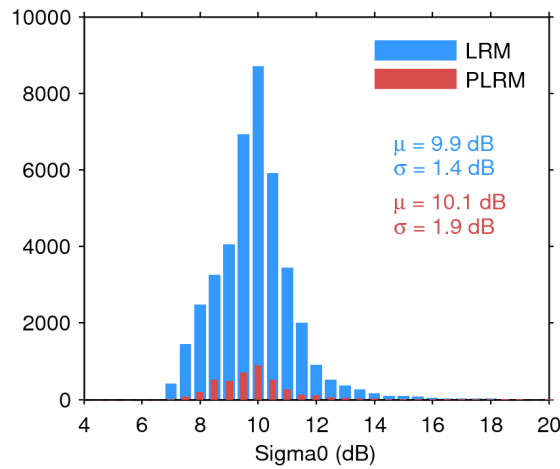
Figure 28. Histogram of science-valid sigma0 over oceans and lakes for LRM (blue) and PLRM (red) for 11/02/2017. The mean ( \mu ) and standard deviation ( \sigma ) are also shown. Note that values outside [4 20] dB are excluded from the histogram for the sake of readability but not from the computation of \mu and \sigma .
