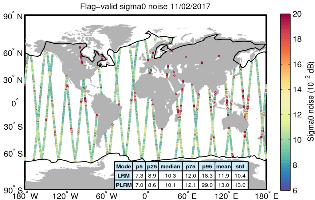
Figure 26. Geographical distribution of flag-valid 20-Hz sigma0 measurement noise over oceans and lakes for 11/02/2017. The statistical values shown in the table refer to the sigma0 noise and are calculated separately for LRM and PLRM regions. Measurements taken over polar polygons have been excluded from the computation of the statistical values. The black lines mark the outer limit of the Arctic and Antarctic polar polygons.
