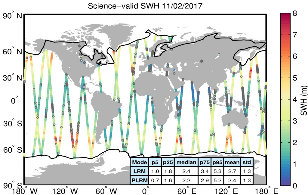
Figure 19. Geographical distribution of science-valid SWH data over oceans and lakes for 11/02/2017. The statistical values shown in the table refer to the SWH in m and are calculated separately for LRM and PLRM regions. The black lines mark the outer limit of the Arctic and Antarctic polar polygons. Gray circles denote records that have been rejected based on the editing criteria described in Table 3.
