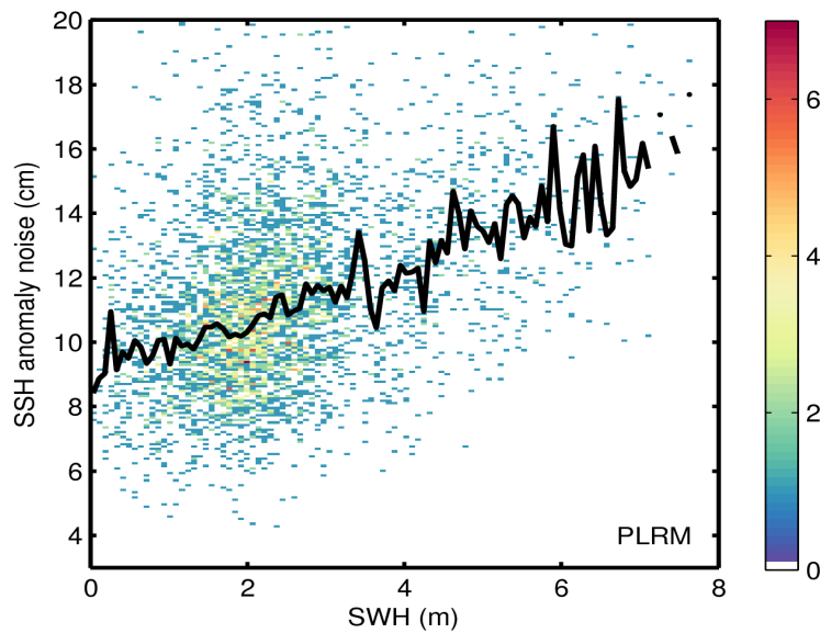
Figure 9. 2D histogram showing flag-valid SSH anomaly noise as a function of SWH for LRM (top) and PLRM (bottom) for 11/02/2017. The black line denotes the median SSH anomaly noise as a function of SWH.
