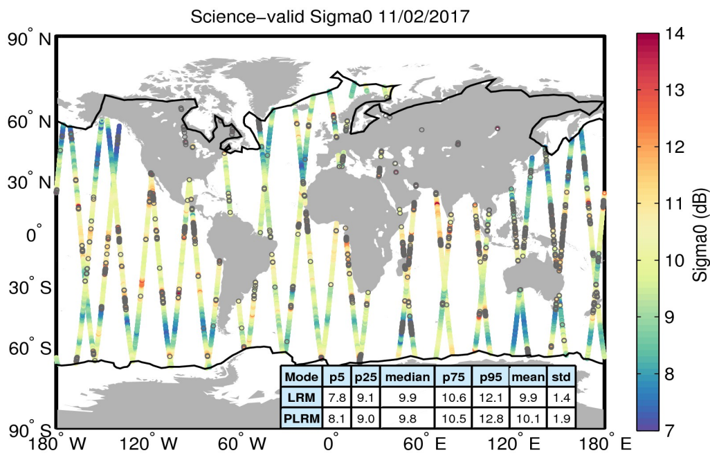
Figure 27. Geographical distribution of science-valid sigma0 data over oceans and lakes for 11/02/2017. The statistical values shown in the table refer to the sigma0 in dB and are calculated separately for LRM and PLRM regions. The black lines mark the outer limit of the Arctic and Antarctic polar polygons. Gray circles denote records that have been rejected based on the editing criteria described in Table 4.
