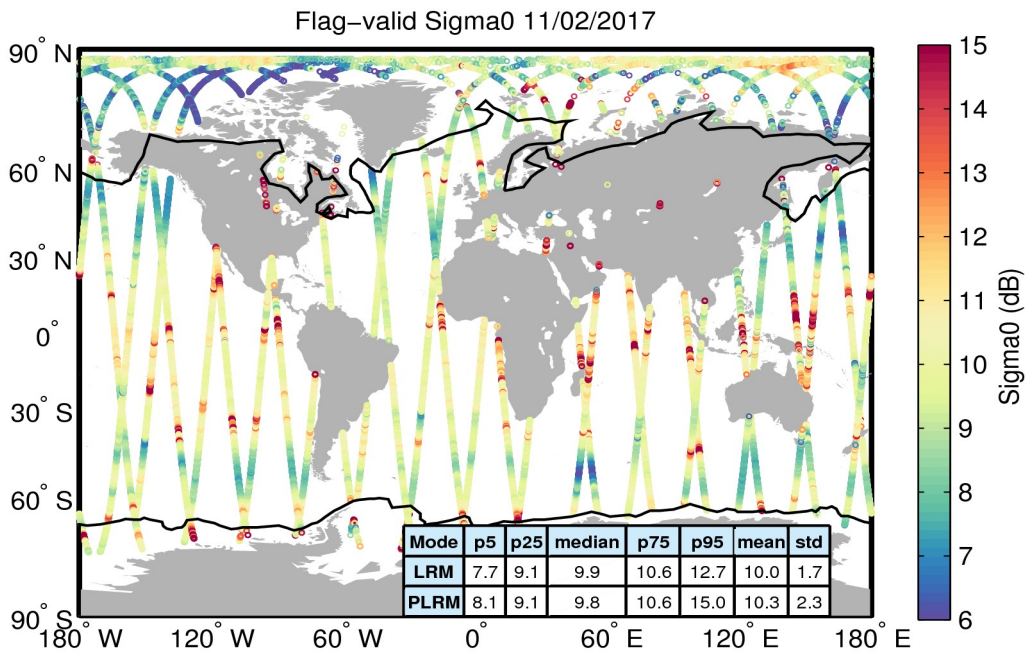
Figure 23. Geographical distribution of flag-valid sigma0 data over oceans and lakes for 11/02/2017. The statistical values shown in the table refer to the sigma0 in dB and are calculated separately for LRM and PLRM regions. Measurements taken over polar polygons have been excluded from the computation of the statistical values. The black lines mark the outer limit of the Arctic and Antarctic polar polygons.
