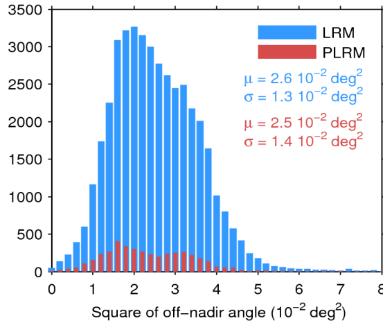
Figure 39. Histogram of flag-valid mispointing over oceans and lakes for LRM (blue) and PLRM (red) for 11/02/2017. Only positive values have been considered. The mean ( \mu ) and standard deviation ( \sigma ) are also shown. Note that values larger than 8 \cdot 10^{-2} \text{ deg}^2 are excluded from the histogram for the sake of readability but not from the computation of \mu and \sigma .
