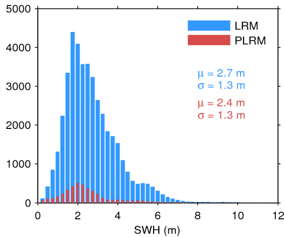
Figure 20. Histogram of science-valid SWH over oceans and lakes for LRM (blue) and PLRM (red) for 11/02/2017. The mean ( \mu ) and standard deviation ( \sigma ) are also shown. Note that values larger than 12 m are excluded from the histogram for the sake of readability but not from the computation of \mu and \sigma .
