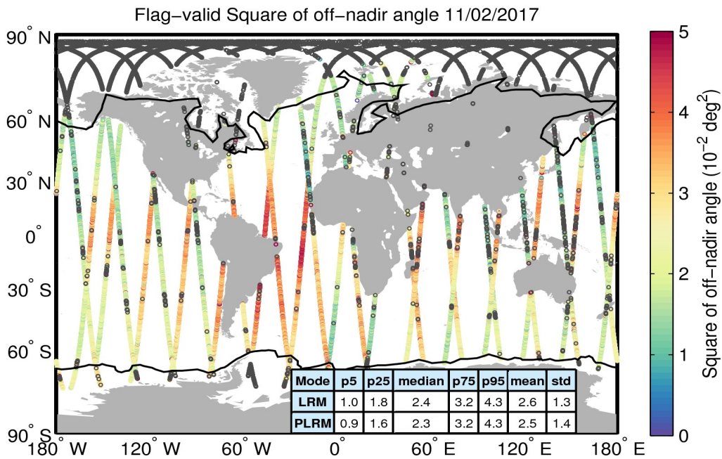
Figure 37. Geographical distribution of flag-valid mispointing data over oceans and lakes for 11/02/2017. The statistical values shown in the table refer to the mispointing in 10^{-2} \text{ deg}^2 and are calculated separately for LRM and PLRM regions. Measurements taken over polar polygons have been excluded from the computation of the statistical values. The black lines mark the outer limit of the Arctic and Antarctic polar polygons. Gray circles denote negative values.
