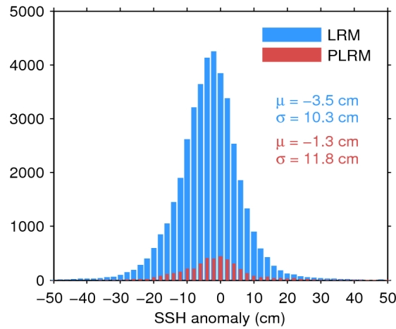
Figure 11. Histogram of science-valid SSH anomaly over oceans and lakes for LRM (blue) and PLRM (red) for 11/02/2017. The mean ( \mu ) and standard deviation ( \sigma ) are also shown. Note that values outside [-50 50] cm are excluded from the histogram for the sake of readability but not from the computation of \mu and \sigma .
