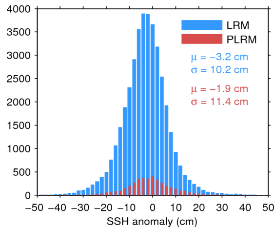
Figure 11. Histogram of science-valid SSH anomaly over oceans and lakes for LRM (blue) and PLRM (red) for 10/02/2017. The mean ( \mu ) and standard deviation ( \sigma ) are also shown. Note that values outside [-50 50] cm are excluded from the histogram for the sake of readability but not from the computation of \mu and \sigma .
