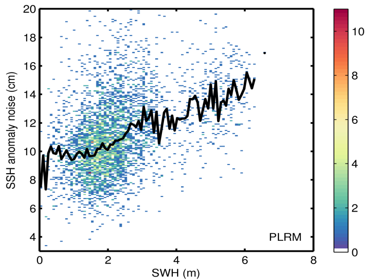
Figure 9. 2D histogram showing flag-valid SSH anomaly noise as a function of SWH for LRM (top) and PLRM (bottom) for 10/02/2017. The black line denotes the median SSH anomaly noise as a function of SWH.
