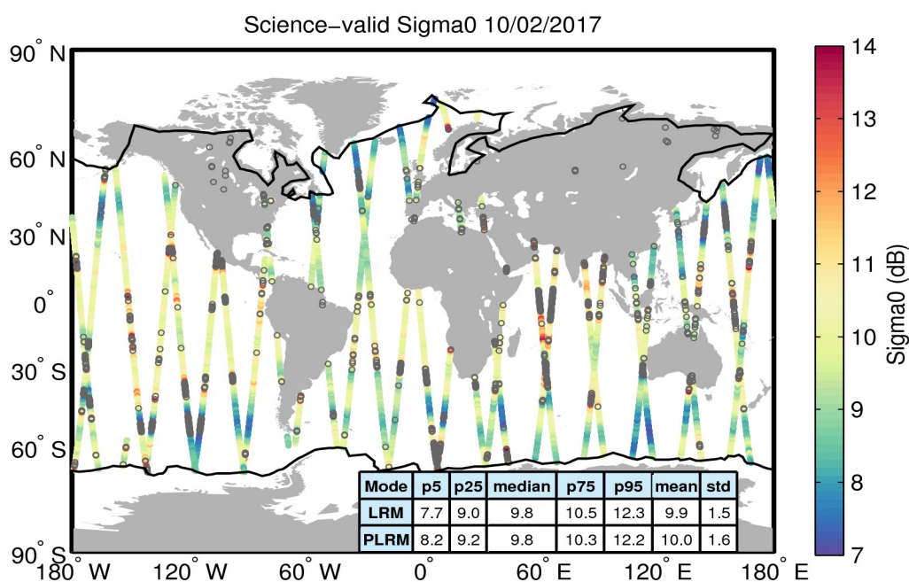
Figure 27. Geographical distribution of science-valid sigma0 data over oceans and lakes for 10/02/2017. The statistical values shown in the table refer to the sigma0 in dB and are calculated separately for LRM and PLRM regions. The black lines mark the outer limit of the Arctic and Antarctic polar polygons. Gray circles denote records that have been rejected based on the editing criteria described in Table 4.
