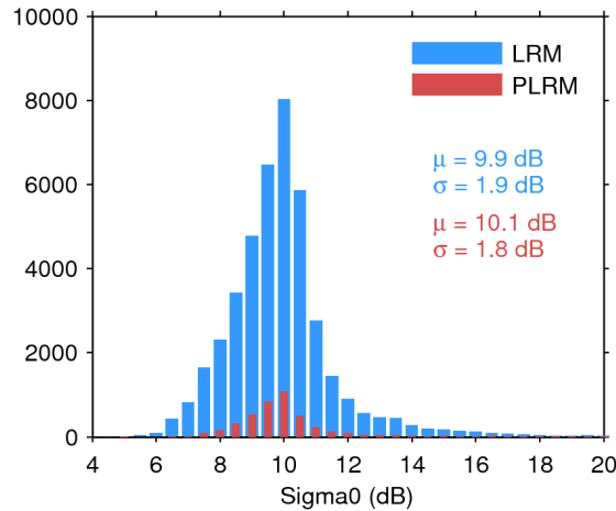
Figure 25. Histogram of flag-valid sigma0 over oceans and lakes for LRM (blue) and PLRM (red) for 10/02/2017. The mean ( \mu ) and standard deviation ( \sigma ) are also shown. Note that values outside [4 20] dB are excluded from the histogram for the sake of readability but not from the computation of \mu and \sigma .
