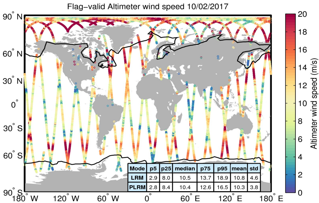
Figure 31. Geographical distribution of flag-valid wind data over oceans and lakes for 10/02/2017. The statistical values shown in the table refer to the wind in m/s and are calculated separately for LRM and PLRM regions. Measurements taken over polar polygons have been excluded from the computation of the statistical values. The black lines mark the outer limit of the Arctic and Antarctic polar polygons.
