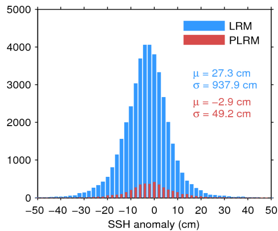
Figure 7. Histogram of flag-valid SSH anomaly over oceans and lakes for LRM (blue) and PLRM (red) for 10/02/2017. The mean ( \mu ) and standard deviation ( \sigma ) are also shown. Note that values outside [-50\ 50] cm are excluded from the histogram for the sake of readability but not from the computation of \mu and \sigma .
