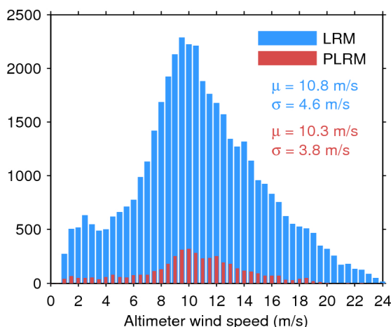
Figure 33. Histogram of flag-valid wind over oceans and lakes for LRM (blue) and PLRM (red) for 10/02/2017. The mean ( \mu ) and standard deviation ( \sigma ) are also shown. Note that values larger than 24 m/s are excluded from the histogram for the sake of readability but not from the computation of \mu and \sigma .
