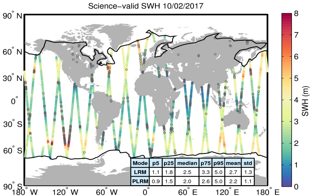
Figure 19. Geographical distribution of science-valid SWH data over oceans and lakes for 10/02/2017. The statistical values shown in the table refer to the SWH in m and are calculated separately for LRM and PLRM regions. The black lines mark the outer limit of the Arctic and Antarctic polar polygons. Gray circles denote records that have been rejected based on the editing criteria described in Table 3.
