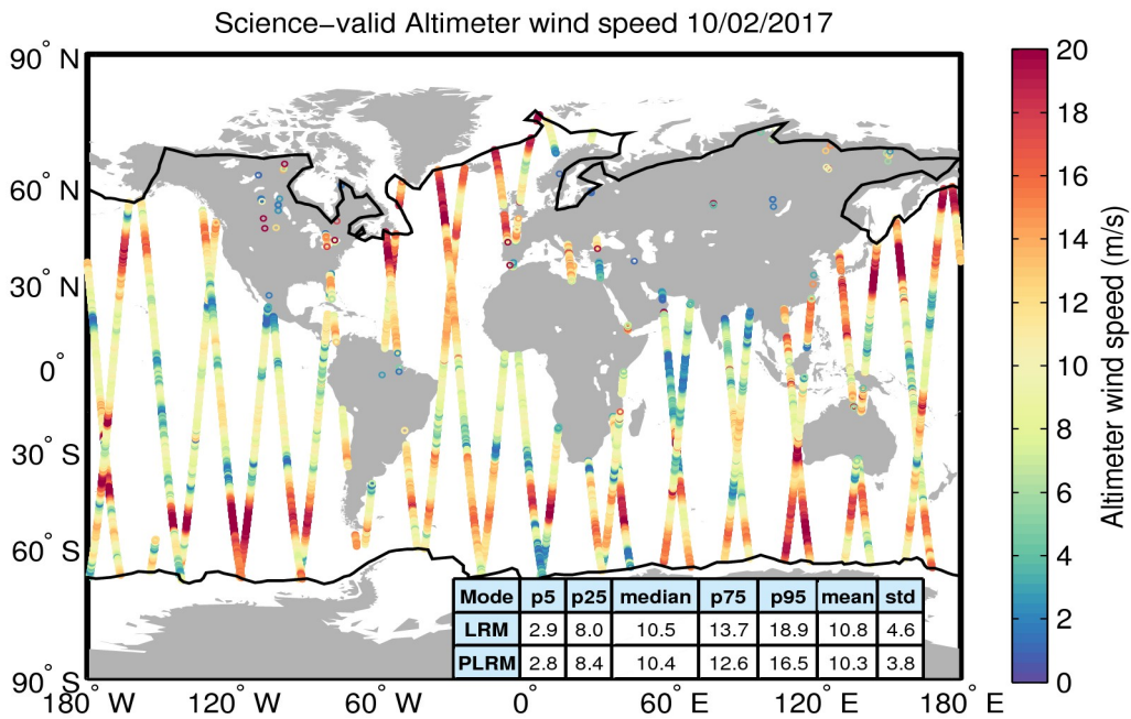
Figure 34. Geographical distribution of science-valid wind data over oceans and lakes for 10/02/2017. The statistical values shown in the table refer to the wind in m/s and are calculated separately for LRM and PLRM regions. The black lines mark the outer limit of the Arctic and Antarctic polar polygons. Gray circles denote records that have been rejected based on the editing criteria described in Table 5.
