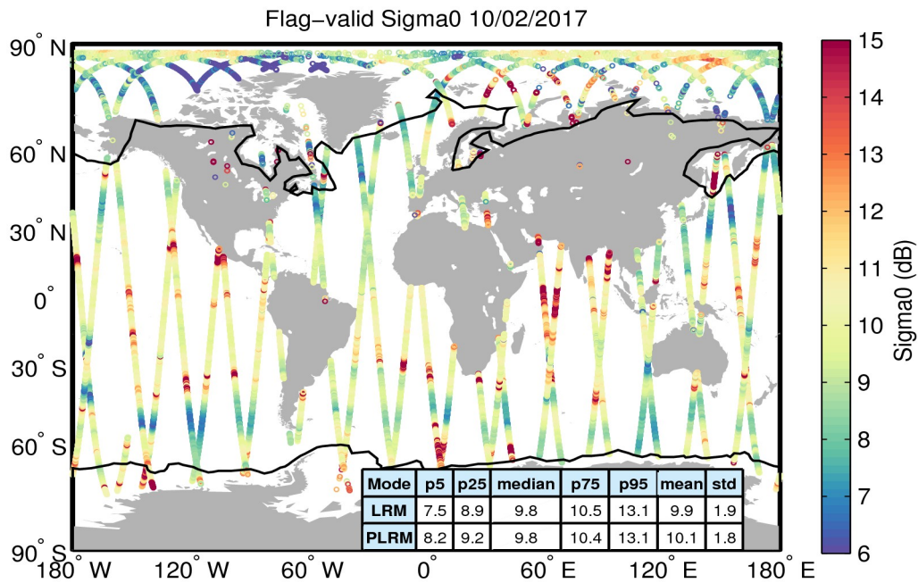
Figure 23. Geographical distribution of flag-valid sigma0 data over oceans and lakes for 10/02/2017. The statistical values shown in the table refer to the sigma0 in dB and are calculated separately for LRM and PLRM regions. Measurements taken over polar polygons have been excluded from the computation of the statistical values. The black lines mark the outer limit of the Arctic and Antarctic polar polygons.
