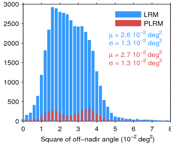
Figure 39. Histogram of flag-valid mispointing over oceans and lakes for LRM (blue) and PLRM (red) for 10/02/2017. Only positive values have been considered. The mean ( \mu ) and standard deviation ( \sigma ) are also shown. Note that values larger than 8 \cdot 10^{-2} \text{ deg}^2 are excluded from the histogram for the sake of readability but not from the computation of \mu and \sigma .
