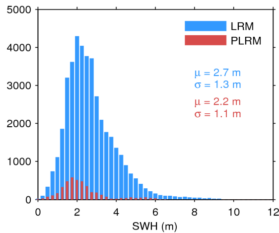
Figure 20. Histogram of science-valid SWH over oceans and lakes for LRM (blue) and PLRM (red) for 10/02/2017. The mean ( \mu ) and standard deviation ( \sigma ) are also shown. Note that values larger than 12 m are excluded from the histogram for the sake of readability but not from the computation of \mu and \sigma .
