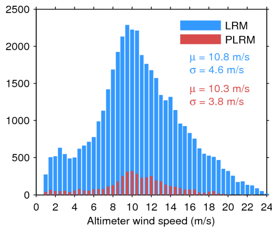
Figure 35. Histogram of science-valid wind over oceans and lakes for LRM (blue) and PLRM (red) for 10/02/2017. The mean ( \mu ) and standard deviation ( \sigma ) are also shown. Note that values larger than 24 m/s are excluded from the histogram for the sake of readability but not from the computation of \mu and \sigma .
