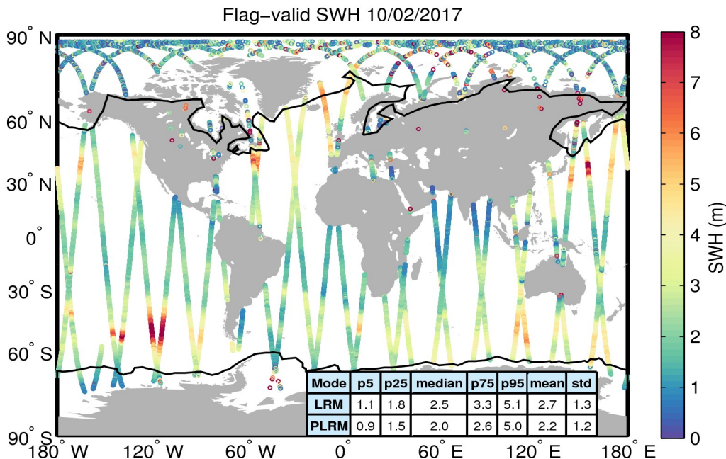
Figure 15. Geographical distribution of flag-valid SWH data over oceans and lakes for 10/02/2017. The statistical values shown in the table refer to the SWH in m and are calculated separately for LRM and PLRM regions. Measurements taken over polar polygons have been excluded from the computation of the statistical values. The black lines mark the outer limit of the Arctic and Antarctic polar polygons.
