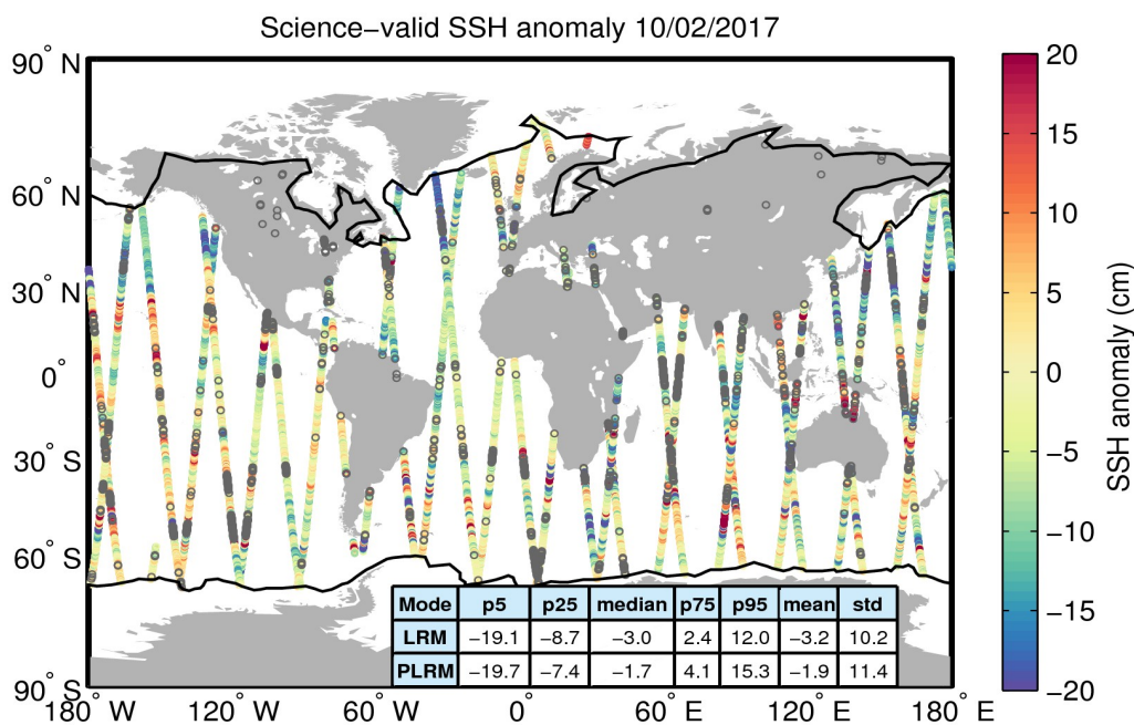
Figure 10. Geographical distribution of science-valid SSH anomaly data over oceans and lakes for 10/02/2017. The statistical values shown in the table refer to the SSH anomaly in cm and are calculated separately for LRM and PLRM regions. The black lines mark the outer limit of the Arctic and Antarctic polar polygons. Gray circles denote records that have been rejected based on the editing criteria described in Table 2.
