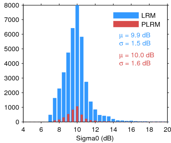
Figure 28. Histogram of science-valid sigma0 over oceans and lakes for LRM (blue) and PLRM (red) for 10/02/2017. The mean ( \mu ) and standard deviation ( \sigma ) are also shown. Note that values outside [4 20] dB are excluded from the histogram for the sake of readability but not from the computation of \mu and \sigma .
