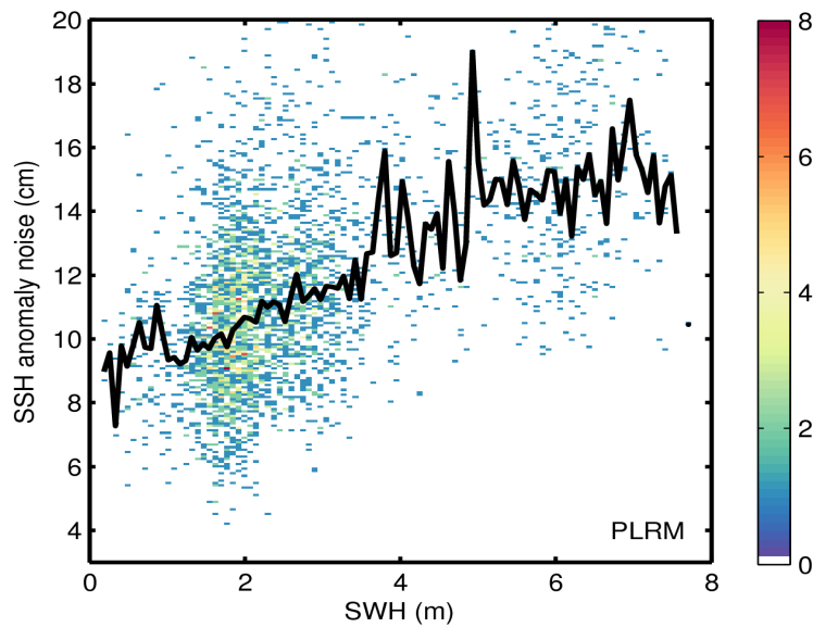
Figure 9. 2D histogram showing flag-valid SSH anomaly noise as a function of SWH for LRM (top) and PLRM (bottom) for 08/02/2017. The black line denotes the median SSH anomaly noise as a function of SWH.
