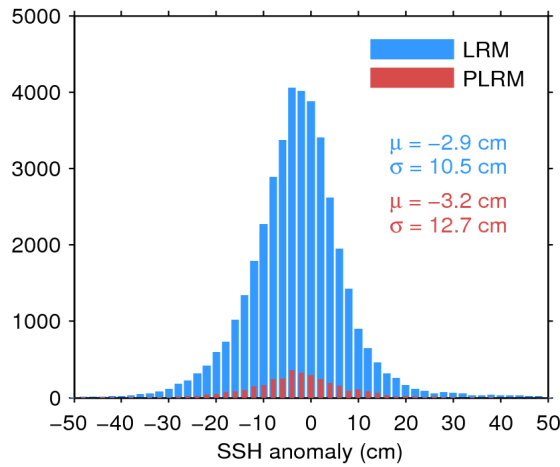
Figure 11. Histogram of science-valid SSH anomaly over oceans and lakes for LRM (blue) and PLRM (red) for 08/02/2017. The mean ( \mu ) and standard deviation ( \sigma ) are also shown. Note that values outside [-50\ 50] cm are excluded from the histogram for the sake of readability but not from the computation of \mu and \sigma .
