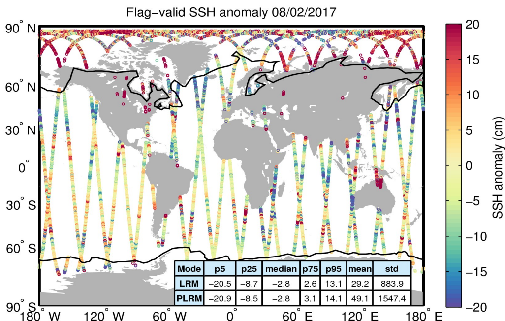
Figure 5. Geographical distribution of flag-valid 1-Hz SSH anomaly data over oceans and lakes for 08/02/2017. The statistical values shown in the table refer to the SSH anomaly in cm and are calculated separately for LRM and PLRM regions. Measurements taken over polar polygons have been excluded from the computation of the statistical values. The black lines mark the outer limit of the Arctic and Antarctic polar polygons.
