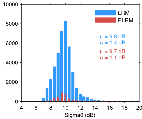
Figure 28. Histogram of science-valid sigma0 over oceans and lakes for LRM (blue) and PLRM (red) for 08/02/2017. The mean ( \mu ) and standard deviation ( \sigma ) are also shown. Note that values outside [4 20] dB are excluded from the histogram for the sake of readability but not from the computation of \mu and \sigma .
