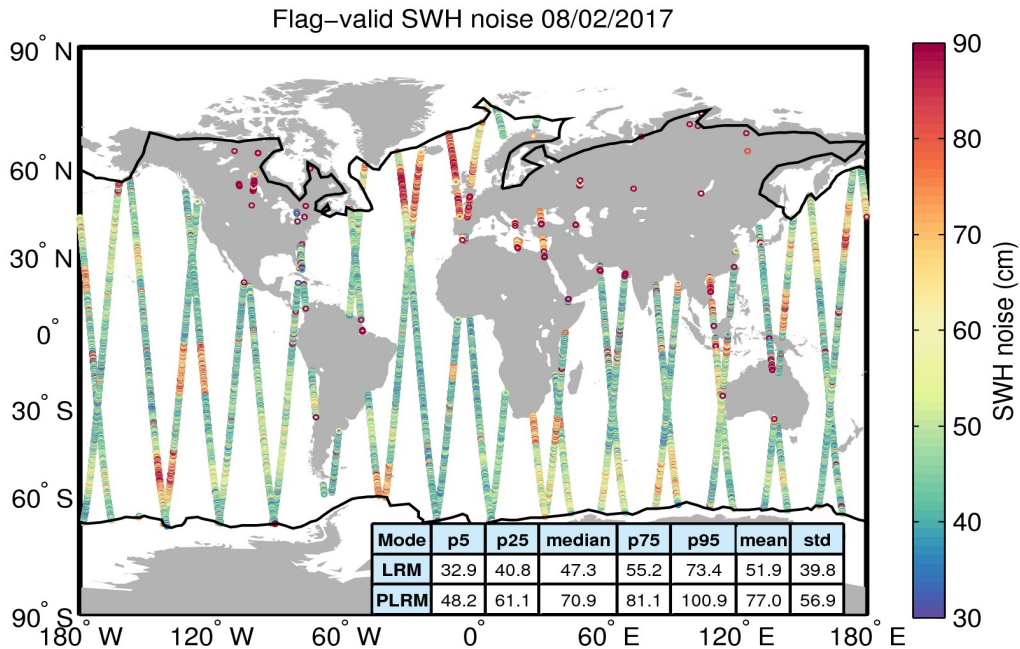
Figure 18. Geographical distribution of flag-valid 20-Hz SWH measurement noise over oceans and lakes for 08/02/2017. The statistical values shown in the table refer to the SWH noise and are calculated separately for LRM and PLRM regions. Measurements taken over polar polygons have been excluded from the computation of the statistical values. The black lines mark the outer limit of the Arctic and Antarctic polar polygons.
