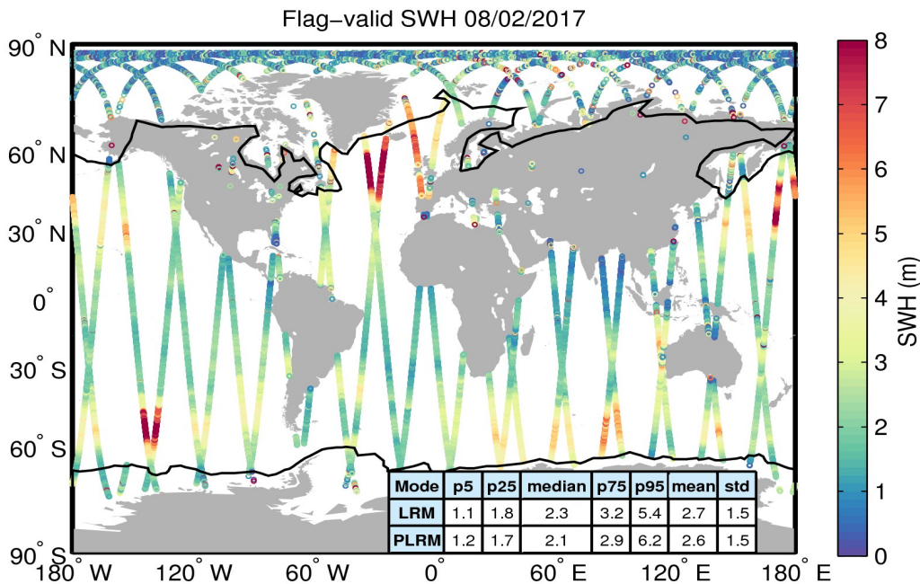
Figure 15. Geographical distribution of flag-valid SWH data over oceans and lakes for 08/02/2017. The statistical values shown in the table refer to the SWH in m and are calculated separately for LRM and PLRM regions. Measurements taken over polar polygons have been excluded from the computation of the statistical values. The black lines mark the outer limit of the Arctic and Antarctic polar polygons.
