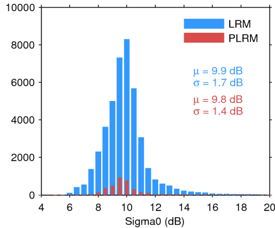
Figure 25. Histogram of flag-valid sigma0 over oceans and lakes for LRM (blue) and PLRM (red) for 08/02/2017. The mean ( \mu ) and standard deviation ( \sigma ) are also shown. Note that values outside [4 20] dB are excluded from the histogram for the sake of readability but not from the computation of \mu and \sigma .
