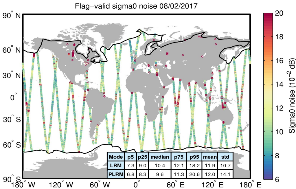
Figure 26. Geographical distribution of flag-valid 20-Hz sigma0 measurement noise over oceans and lakes for 08/02/2017. The statistical values shown in the table refer to the sigma0 noise and are calculated separately for LRM and PLRM regions. Measurements taken over polar polygons have been excluded from the computation of the statistical values. The black lines mark the outer limit of the Arctic and Antarctic polar polygons.
