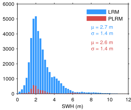
Figure 20. Histogram of science-valid SWH over oceans and lakes for LRM (blue) and PLRM (red) for 08/02/2017. The mean ( \mu ) and standard deviation ( \sigma ) are also shown. Note that values larger than 12 m are excluded from the histogram for the sake of readability but not from the computation of \mu and \sigma .
