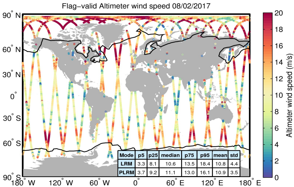
Figure 31. Geographical distribution of flag-valid wind data over oceans and lakes for 08/02/2017. The statistical values shown in the table refer to the wind in m/s and are calculated separately for LRM and PLRM regions. Measurements taken over polar polygons have been excluded from the computation of the statistical values. The black lines mark the outer limit of the Arctic and Antarctic polar polygons.
