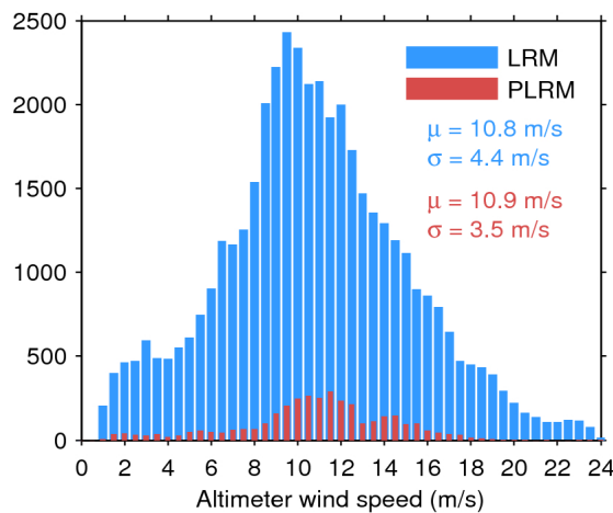
Figure 35. Histogram of science-valid wind over oceans and lakes for LRM (blue) and PLRM (red) for 08/02/2017. The mean ( \mu ) and standard deviation ( \sigma ) are also shown. Note that values larger than 24 m/s are excluded from the histogram for the sake of readability but not from the computation of \mu and \sigma .
