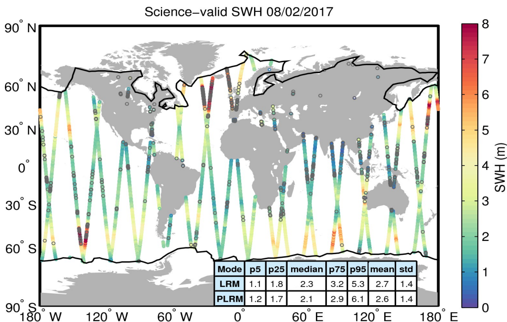
Figure 19. Geographical distribution of science-valid SWH data over oceans and lakes for 08/02/2017. The statistical values shown in the table refer to the SWH in m and are calculated separately for LRM and PLRM regions. The black lines mark the outer limit of the Arctic and Antarctic polar polygons. Gray circles denote records that have been rejected based on the editing criteria described in Table 3.
