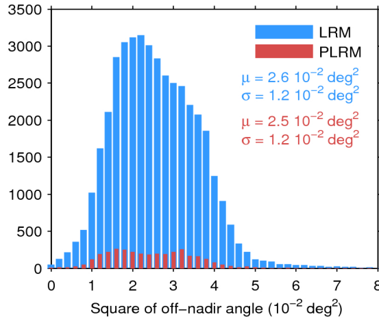
Figure 39. Histogram of flag-valid mispointing over oceans and lakes for LRM (blue) and PLRM (red) for 08/02/2017. Only positive values have been considered. The mean ( \mu ) and standard deviation ( \sigma ) are also shown. Note that values larger than 8 \cdot 10^{-2} \text{ deg}^2 are excluded from the histogram for the sake of readability but not from the computation of \mu and \sigma .
