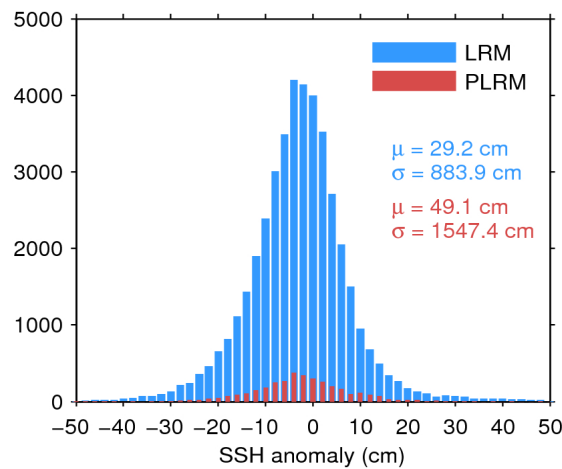
Figure 7. Histogram of flag-valid SSH anomaly over oceans and lakes for LRM (blue) and PLRM (red) for 08/02/2017. The mean ( \mu ) and standard deviation ( \sigma ) are also shown. Note that values outside [-50\ 50] cm are excluded from the histogram for the sake of readability but not from the computation of \mu and \sigma .
