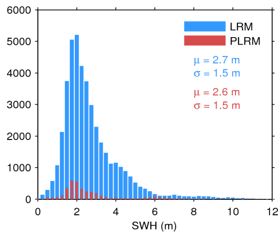
Figure 17. Histogram of flag-valid SWH over oceans and lakes for LRM (blue) and PLRM (red) for 08/02/2017. The mean ( \mu ) and standard deviation ( \sigma ) are also shown. Note that values larger than 12 m are excluded from the histogram for the sake of readability but not from the computation of \mu and \sigma .
