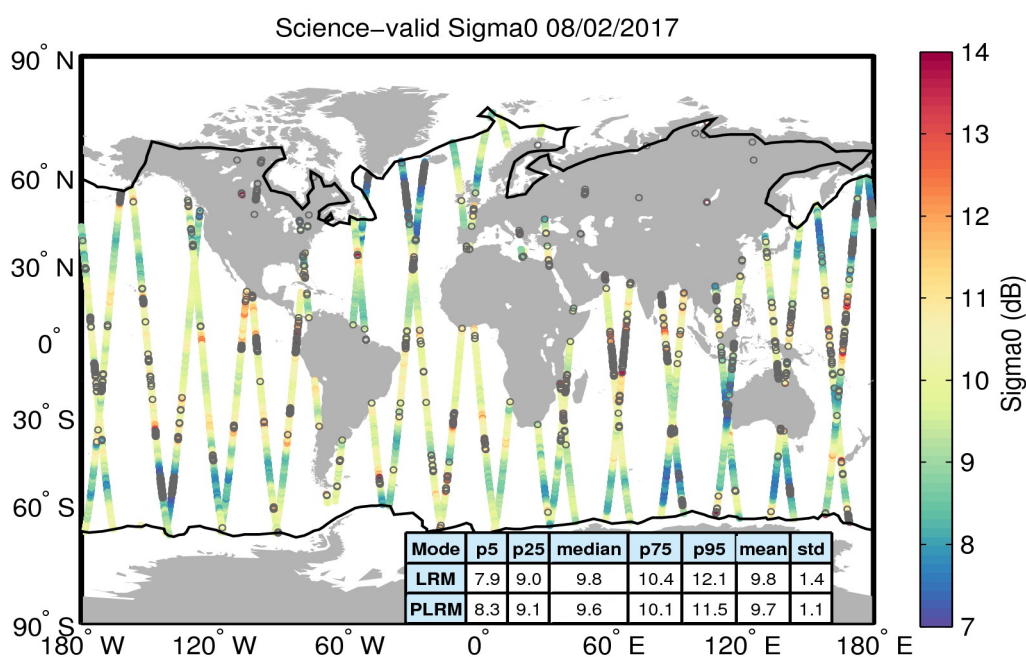
Figure 27. Geographical distribution of science-valid sigma0 data over oceans and lakes for 08/02/2017. The statistical values shown in the table refer to the sigma0 in dB and are calculated separately for LRM and PLRM regions. The black lines mark the outer limit of the Arctic and Antarctic polar polygons. Gray circles denote records that have been rejected based on the editing criteria described in Table 4.
