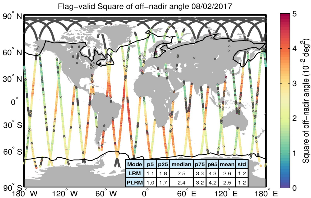
Figure 37. Geographical distribution of flag-valid mispointing data over oceans and lakes for 08/02/2017. The statistical values shown in the table refer to the mispointing in 10^{-2} deg 2 and are calculated separately for LRM and PLRM regions. Measurements taken over polar polygons have been excluded from the computation of the statistical values. The black lines mark the outer limit of the Arctic and Antarctic polar polygons. Gray circles denote negative values.
