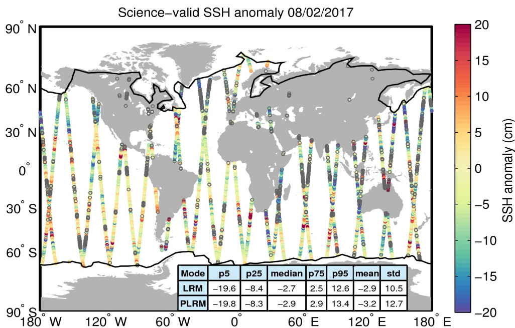
Figure 10. Geographical distribution of science-valid SSH anomaly data over oceans and lakes for 08/02/2017. The statistical values shown in the table refer to the SSH anomaly in cm and are calculated separately for LRM and PLRM regions. The black lines mark the outer limit of the Arctic and Antarctic polar polygons. Gray circles denote records that have been rejected based on the editing criteria described in Table 2.
