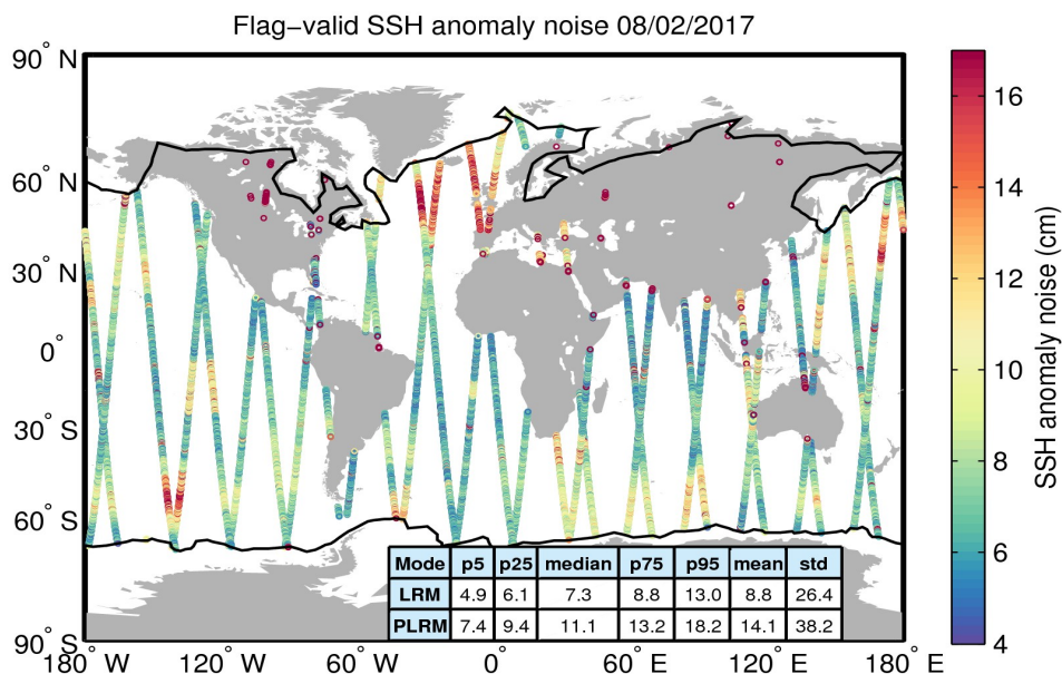
Figure 8. Geographical distribution of flag-valid 20-Hz SSH anomaly measurement noise over oceans and lakes for 08/02/2017. The statistical values shown in the table refer to the SSH anomaly noise and are calculated separately for LRM and PLRM regions. Measurements taken over polar polygons have been excluded from the computation of the statistical values. The black lines mark the outer limit of the Arctic and Antarctic polar polygons.
