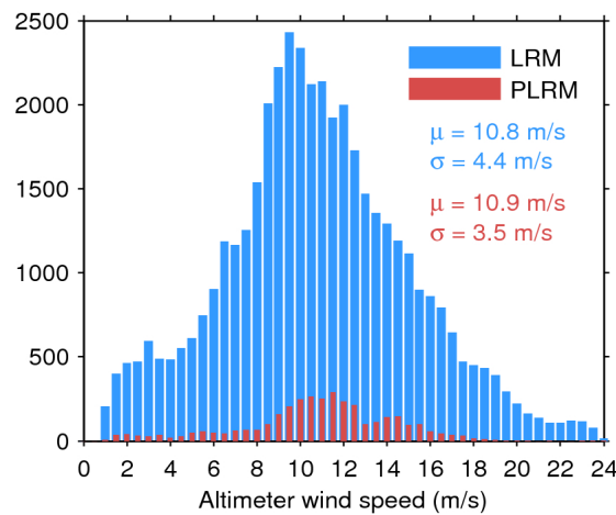
Figure 33. Histogram of flag-valid wind over oceans and lakes for LRM (blue) and PLRM (red) for 08/02/2017. The mean ( \mu ) and standard deviation ( \sigma ) are also shown. Note that values larger than 24 m/s are excluded from the histogram for the sake of readability but not from the computation of \mu and \sigma .
