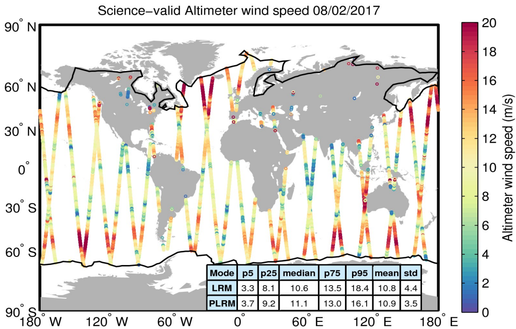
Figure 34. Geographical distribution of science-valid wind data over oceans and lakes for 08/02/2017. The statistical values shown in the table refer to the wind in m/s and are calculated separately for LRM and PLRM regions. The black lines mark the outer limit of the Arctic and Antarctic polar polygons. Gray circles denote records that have been rejected based on the editing criteria described in Table 5.
