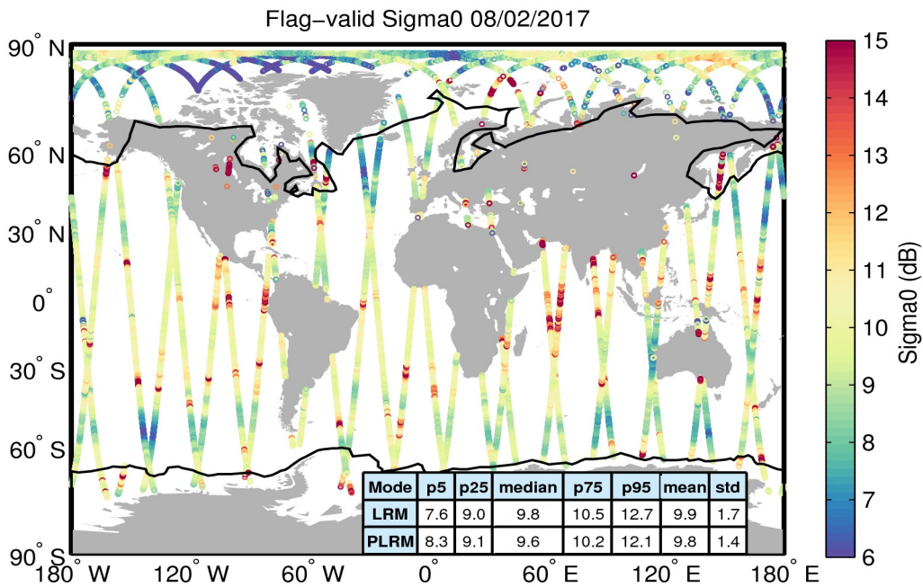
Figure 23. Geographical distribution of flag-valid sigma0 data over oceans and lakes for 08/02/2017. The statistical values shown in the table refer to the sigma0 in dB and are calculated separately for LRM and PLRM regions. Measurements taken over polar polygons have been excluded from the computation of the statistical values. The black lines mark the outer limit of the Arctic and Antarctic polar polygons.
