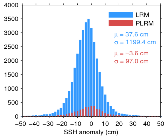
Figure 7. Histogram of flag-valid SSH anomaly over oceans and lakes for LRM (blue) and PLRM (red) for 07/02/2017. The mean ( \mu ) and standard deviation ( \sigma ) are also shown. Note that values outside [-50 \ 50] cm are excluded from the histogram for the sake of readability but not from the computation of \mu and \sigma .
