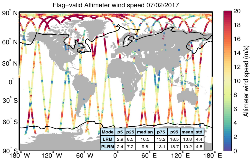
Figure 31. Geographical distribution of flag-valid wind data over oceans and lakes for 07/02/2017. The statistical values shown in the table refer to the wind in m/s and are calculated separately for LRM and PLRM regions. Measurements taken over polar polygons have been excluded from the computation of the statistical values. The black lines mark the outer limit of the Arctic and Antarctic polar polygons.
