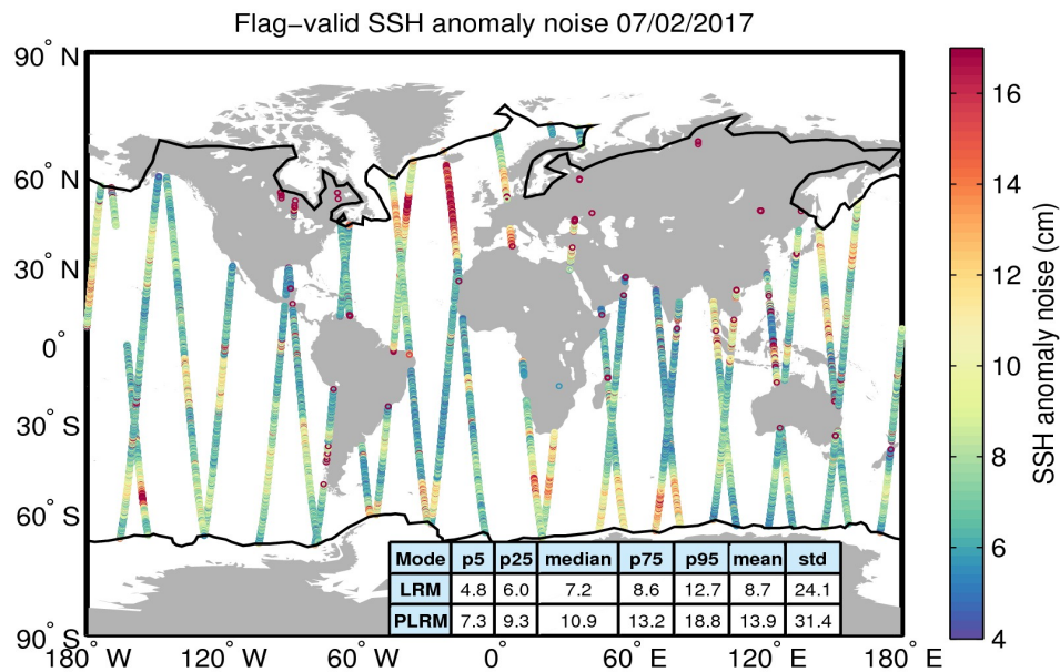
Figure 8. Geographical distribution of flag-valid 20-Hz SSH anomaly measurement noise over oceans and lakes for 07/02/2017. The statistical values shown in the table refer to the SSH anomaly noise and are calculated separately for LRM and PLRM regions. Measurements taken over polar polygons have been excluded from the computation of the statistical values. The black lines mark the outer limit of the Arctic and Antarctic polar polygons.
