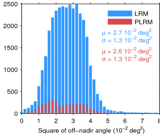
Figure 39. Histogram of flag-valid mispointing over oceans and lakes for LRM (blue) and PLRM (red) for 07/02/2017. Only positive values have been considered. The mean ( \mu ) and standard deviation ( \sigma ) are also shown. Note that values larger than 8 \cdot 10^{-2} \text{ deg}^2 are excluded from the histogram for the sake of readability but not from the computation of \mu and \sigma .
