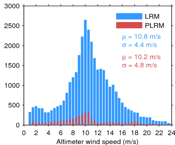
Figure 35. Histogram of science-valid wind over oceans and lakes for LRM (blue) and PLRM (red) for 07/02/2017. The mean ( \mu ) and standard deviation ( \sigma ) are also shown. Note that values larger than 24 m/s are excluded from the histogram for the sake of readability but not from the computation of \mu and \sigma .
