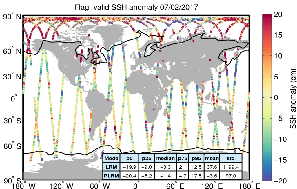
Figure 5. Geographical distribution of flag-valid 1-Hz SSH anomaly data over oceans and lakes for 07/02/2017. The statistical values shown in the table refer to the SSH anomaly in cm and are calculated separately for LRM and PLRM regions. Measurements taken over polar polygons have been excluded from the computation of the statistical values. The black lines mark the outer limit of the Arctic and Antarctic polar polygons.
