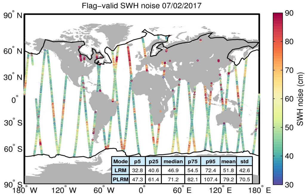
Figure 18. Geographical distribution of flag-valid 20-Hz SWH measurement noise over oceans and lakes for 07/02/2017. The statistical values shown in the table refer to the SWH noise and are calculated separately for LRM and PLRM regions. Measurements taken over polar polygons have been excluded from the computation of the statistical values. The black lines mark the outer limit of the Arctic and Antarctic polar polygons.
