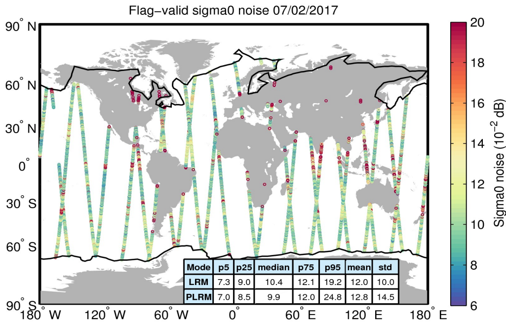
Figure 26. Geographical distribution of flag-valid 20-Hz sigma0 measurement noise over oceans and lakes for 07/02/2017. The statistical values shown in the table refer to the sigma0 noise and are calculated separately for LRM and PLRM regions. Measurements taken over polar polygons have been excluded from the computation of the statistical values. The black lines mark the outer limit of the Arctic and Antarctic polar polygons.
