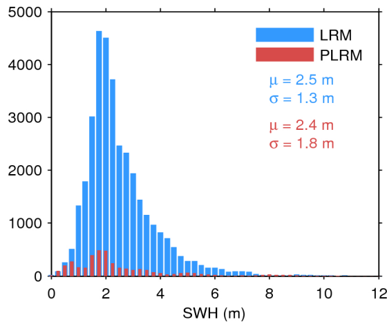
Figure 20. Histogram of science-valid SWH over oceans and lakes for LRM (blue) and PLRM (red) for 07/02/2017. The mean ( \mu ) and standard deviation ( \sigma ) are also shown. Note that values larger than 12 m are excluded from the histogram for the sake of readability but not from the computation of \mu and \sigma .
