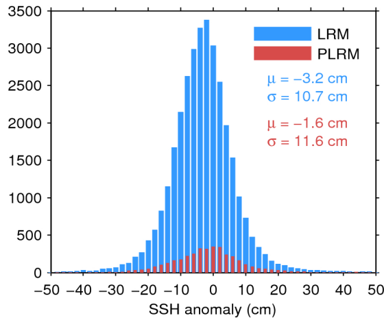
Figure 11. Histogram of science-valid SSH anomaly over oceans and lakes for LRM (blue) and PLRM (red) for 07/02/2017. The mean ( \mu ) and standard deviation ( \sigma ) are also shown. Note that values outside [-50 50] cm are excluded from the histogram for the sake of readability but not from the computation of \mu and \sigma .
