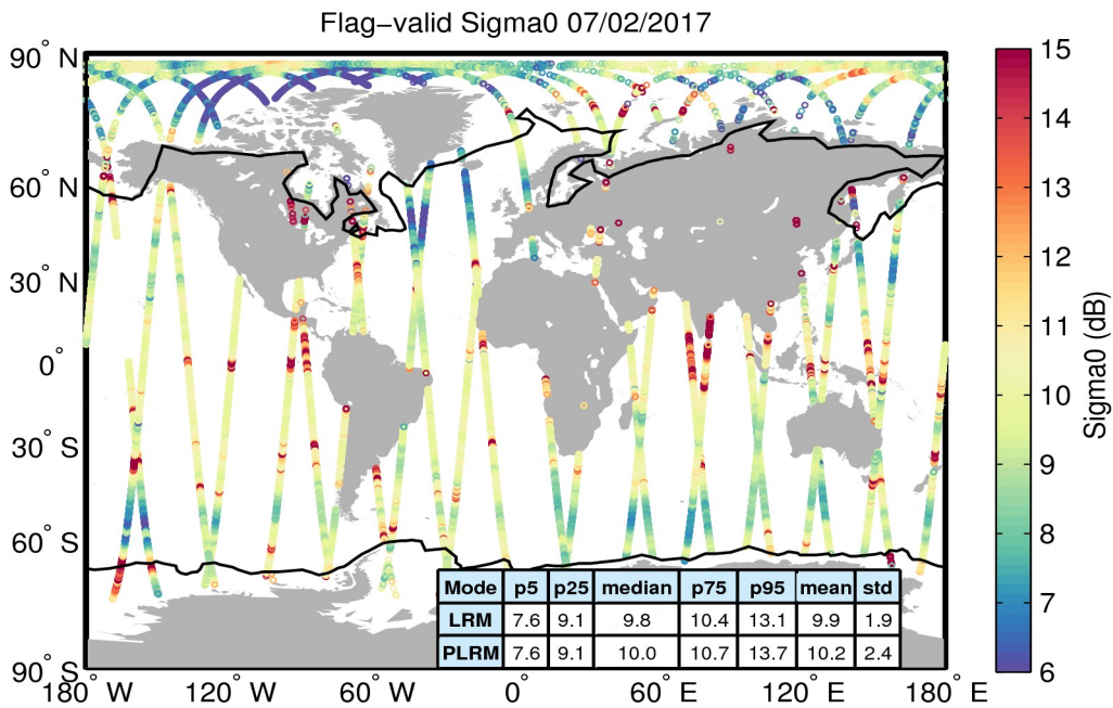
Figure 23. Geographical distribution of flag-valid sigma0 data over oceans and lakes for 07/02/2017. The statistical values shown in the table refer to the sigma0 in dB and are calculated separately for LRM and PLRM regions. Measurements taken over polar polygons have been excluded from the computation of the statistical values. The black lines mark the outer limit of the Arctic and Antarctic polar polygons.
