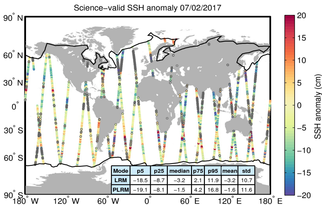
Figure 10. Geographical distribution of science-valid SSH anomaly data over oceans and lakes for 07/02/2017. The statistical values shown in the table refer to the SSH anomaly in cm and are calculated separately for LRM and PLRM regions. The black lines mark the outer limit of the Arctic and Antarctic polar polygons. Gray circles denote records that have been rejected based on the editing criteria described in Table 2.
