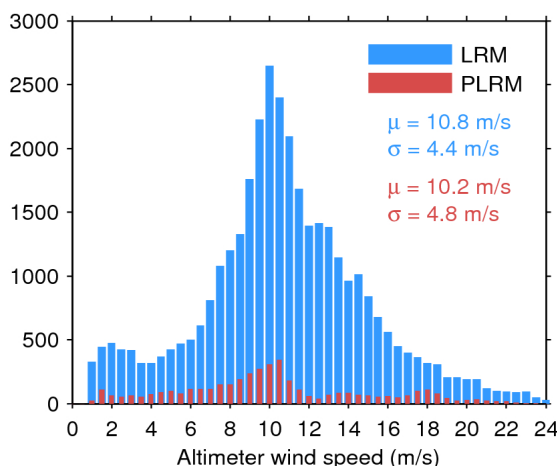
Figure 33. Histogram of flag-valid wind over oceans and lakes for LRM (blue) and PLRM (red) for 07/02/2017. The mean ( \mu ) and standard deviation ( \sigma ) are also shown. Note that values larger than 24 m/s are excluded from the histogram for the sake of readability but not from the computation of \mu and \sigma .
