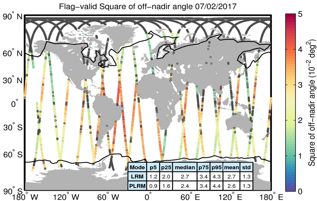
Figure 37. Geographical distribution of flag-valid mispointing data over oceans and lakes for 07/02/2017. The statistical values shown in the table refer to the mispointing in 10^{-2} deg 2 and are calculated separately for LRM and PLRM regions. Measurements taken over polar polygons have been excluded from the computation of the statistical values. The black lines mark the outer limit of the Arctic and Antarctic polar polygons. Gray circles denote negative values.
