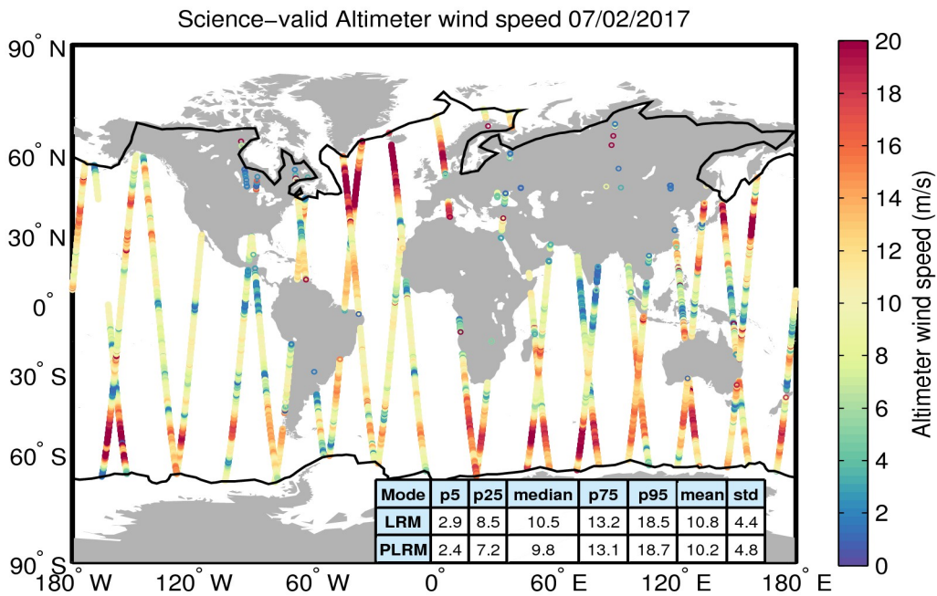
Figure 34. Geographical distribution of science-valid wind data over oceans and lakes for 07/02/2017. The statistical values shown in the table refer to the wind in m/s and are calculated separately for LRM and PLRM regions. The black lines mark the outer limit of the Arctic and Antarctic polar polygons. Gray circles denote records that have been rejected based on the editing criteria described in Table 5.
