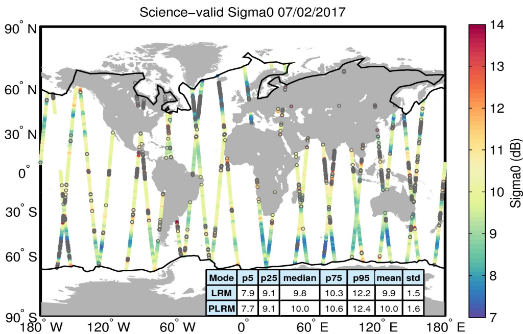
Figure 27. Geographical distribution of science-valid sigma0 data over oceans and lakes for 07/02/2017. The statistical values shown in the table refer to the sigma0 in dB and are calculated separately for LRM and PLRM regions. The black lines mark the outer limit of the Arctic and Antarctic polar polygons. Gray circles denote records that have been rejected based on the editing criteria described in Table 4.
