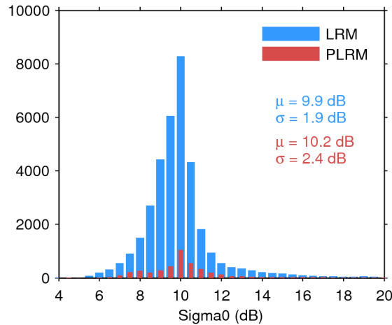
Figure 25. Histogram of flag-valid sigma0 over oceans and lakes for LRM (blue) and PLRM (red) for 07/02/2017. The mean ( \mu ) and standard deviation ( \sigma ) are also shown. Note that values outside [4 20] dB are excluded from the histogram for the sake of readability but not from the computation of \mu and \sigma .
