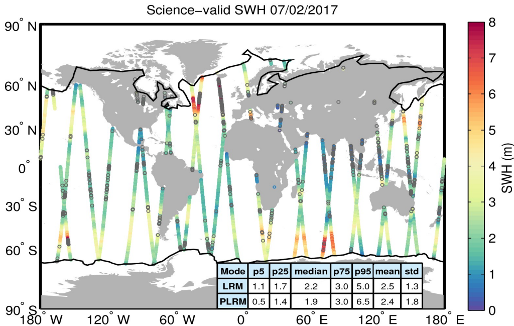
Figure 19. Geographical distribution of science-valid SWH data over oceans and lakes for 07/02/2017. The statistical values shown in the table refer to the SWH in m and are calculated separately for LRM and PLRM regions. The black lines mark the outer limit of the Arctic and Antarctic polar polygons. Gray circles denote records that have been rejected based on the editing criteria described in Table 3.
