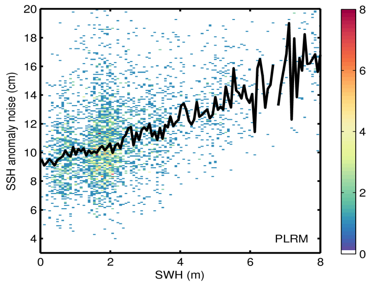
Figure 9. 2D histogram showing flag-valid SSH anomaly noise as a function of SWH for LRM (top) and PLRM (bottom) for 07/02/2017. The black line denotes the median SSH anomaly noise as a function of SWH.
