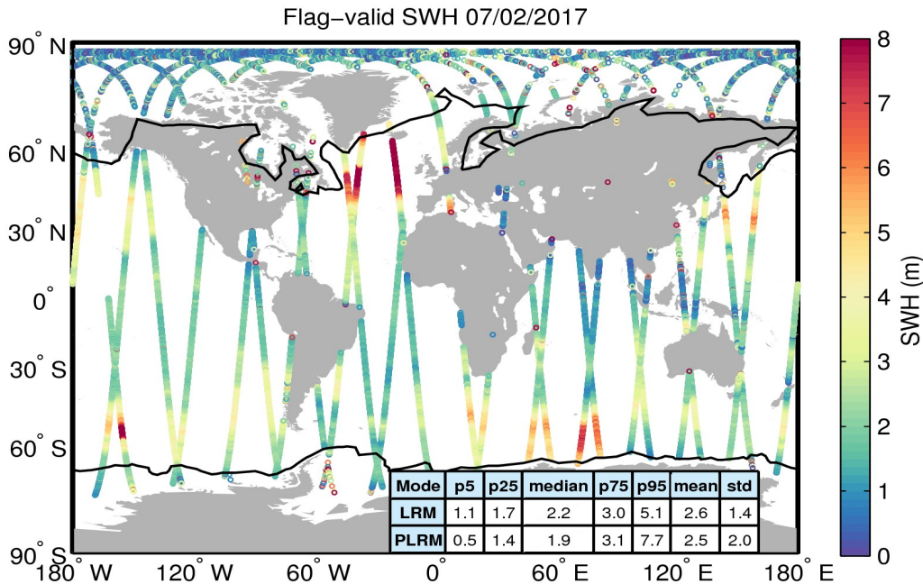
Figure 15. Geographical distribution of flag-valid SWH data over oceans and lakes for 07/02/2017. The statistical values shown in the table refer to the SWH in m and are calculated separately for LRM and PLRM regions. Measurements taken over polar polygons have been excluded from the computation of the statistical values. The black lines mark the outer limit of the Arctic and Antarctic polar polygons.
