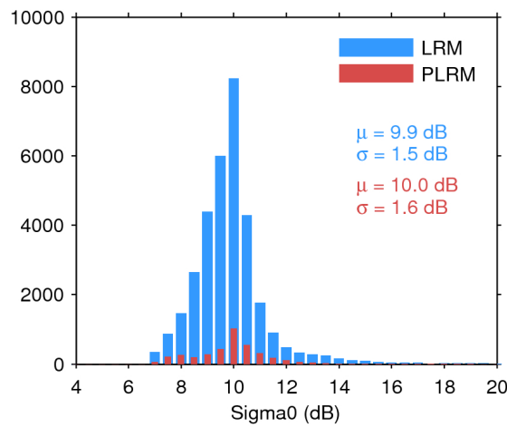
Figure 28. Histogram of science-valid sigma0 over oceans and lakes for LRM (blue) and PLRM (red) for 07/02/2017. The mean ( \mu ) and standard deviation ( \sigma ) are also shown. Note that values outside [4 20] dB are excluded from the histogram for the sake of readability but not from the computation of \mu and \sigma .
