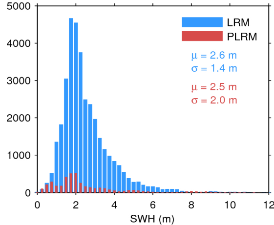
Figure 17. Histogram of flag-valid SWH over oceans and lakes for LRM (blue) and PLRM (red) for 07/02/2017. The mean ( \mu ) and standard deviation ( \sigma ) are also shown. Note that values larger than 12 m are excluded from the histogram for the sake of readability but not from the computation of \mu and \sigma .
