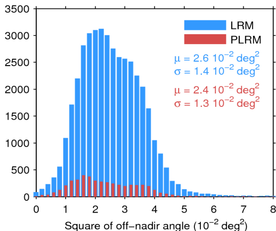
Figure 39. Histogram of flag-valid mispointing over oceans and lakes for LRM (blue) and PLRM (red) for 05/02/2017. Only positive values have been considered. The mean ( \mu ) and standard deviation ( \sigma ) are also shown. Note that values larger than 8 \cdot 10^{-2} \text{ deg}^2 are excluded from the histogram for the sake of readability but not from the computation of \mu and \sigma .
