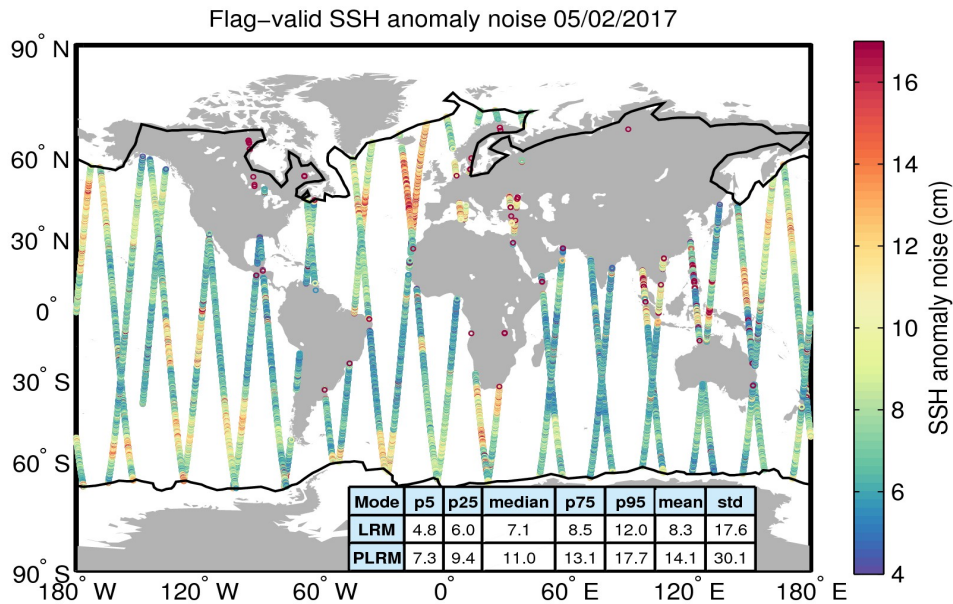
Figure 8. Geographical distribution of flag-valid 20-Hz SSH anomaly measurement noise over oceans and lakes for 05/02/2017. The statistical values shown in the table refer to the SSH anomaly noise and are calculated separately for LRM and PLRM regions. Measurements taken over polar polygons have been excluded from the computation of the statistical values. The black lines mark the outer limit of the Arctic and Antarctic polar polygons.
