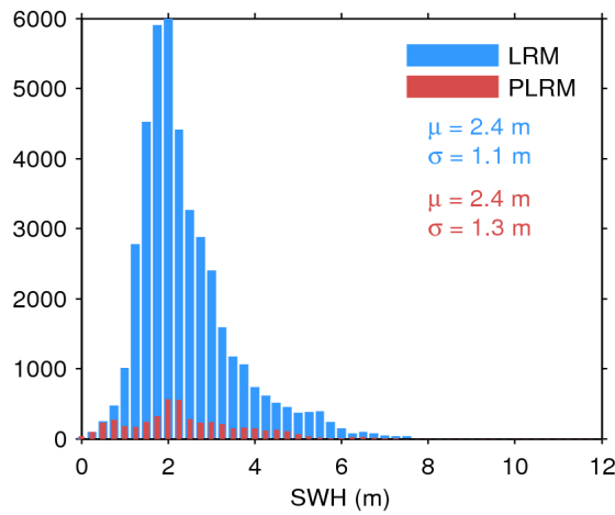
Figure 20. Histogram of science-valid SWH over oceans and lakes for LRM (blue) and PLRM (red) for 05/02/2017. The mean ( \mu ) and standard deviation ( \sigma ) are also shown. Note that values larger than 12 m are excluded from the histogram for the sake of readability but not from the computation of \mu and \sigma .
