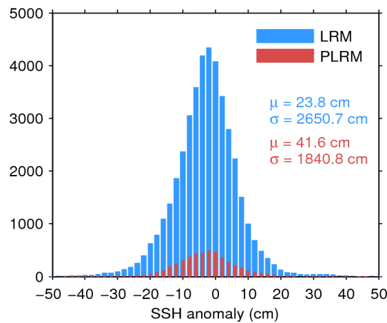
Figure 7. Histogram of flag-valid SSH anomaly over oceans and lakes for LRM (blue) and PLRM (red) for 05/02/2017. The mean ( \mu ) and standard deviation ( \sigma ) are also shown. Note that values outside [-50\ 50] cm are excluded from the histogram for the sake of readability but not from the computation of \mu and \sigma .
