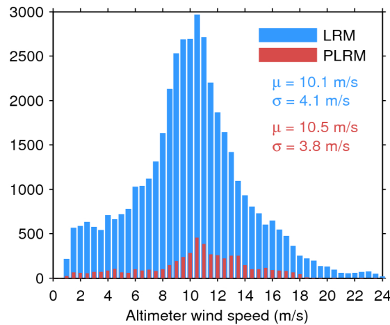
Figure 33. Histogram of flag-valid wind over oceans and lakes for LRM (blue) and PLRM (red) for 05/02/2017. The mean ( \mu ) and standard deviation ( \sigma ) are also shown. Note that values larger than 24 m/s are excluded from the histogram for the sake of readability but not from the computation of \mu and \sigma .
