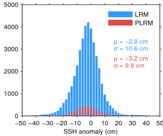
Figure 11. Histogram of science-valid SSH anomaly over oceans and lakes for LRM (blue) and PLRM (red) for 05/02/2017. The mean ( \mu ) and standard deviation ( \sigma ) are also shown. Note that values outside [-50 50] cm are excluded from the histogram for the sake of readability but not from the computation of \mu and \sigma .
