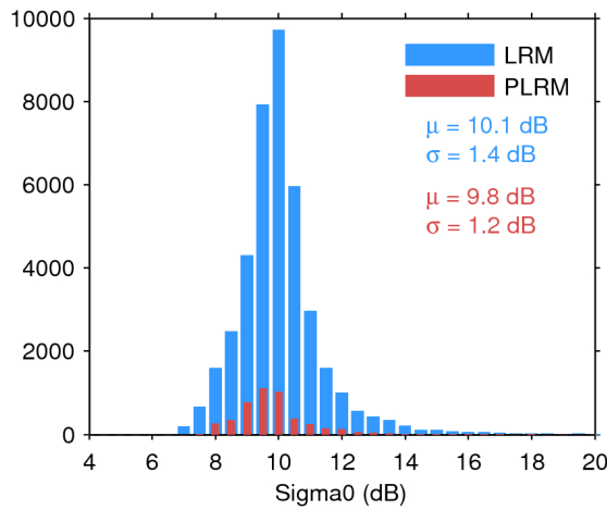
Figure 28. Histogram of science-valid sigma0 over oceans and lakes for LRM (blue) and PLRM (red) for 05/02/2017. The mean ( \mu ) and standard deviation ( \sigma ) are also shown. Note that values outside [4 20] dB are excluded from the histogram for the sake of readability but not from the computation of \mu and \sigma .
