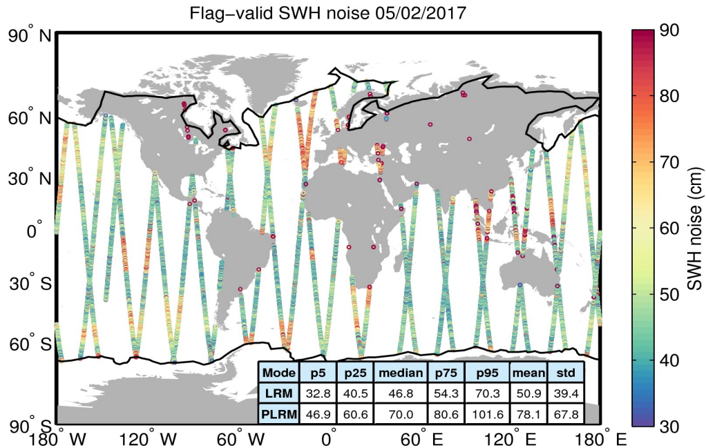
Figure 18. Geographical distribution of flag-valid 20-Hz SWH measurement noise over oceans and lakes for 05/02/2017. The statistical values shown in the table refer to the SWH noise and are calculated separately for LRM and PLRM regions. Measurements taken over polar polygons have been excluded from the computation of the statistical values. The black lines mark the outer limit of the Arctic and Antarctic polar polygons.
