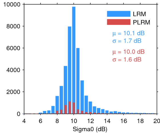
Figure 25. Histogram of flag-valid sigma0 over oceans and lakes for LRM (blue) and PLRM (red) for 05/02/2017. The mean ( \mu ) and standard deviation ( \sigma ) are also shown. Note that values outside [4 20] dB are excluded from the histogram for the sake of readability but not from the computation of \mu and \sigma .
