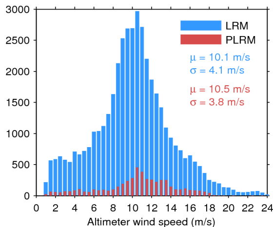
Figure 35. Histogram of science-valid wind over oceans and lakes for LRM (blue) and PLRM (red) for 05/02/2017. The mean ( \mu ) and standard deviation ( \sigma ) are also shown. Note that values larger than 24 m/s are excluded from the histogram for the sake of readability but not from the computation of \mu and \sigma .
