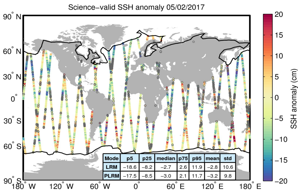
Figure 10. Geographical distribution of science-valid SSH anomaly data over oceans and lakes for 05/02/2017. The statistical values shown in the table refer to the SSH anomaly in cm and are calculated separately for LRM and PLRM regions. The black lines mark the outer limit of the Arctic and Antarctic polar polygons. Gray circles denote records that have been rejected based on the editing criteria described in Table 2.
