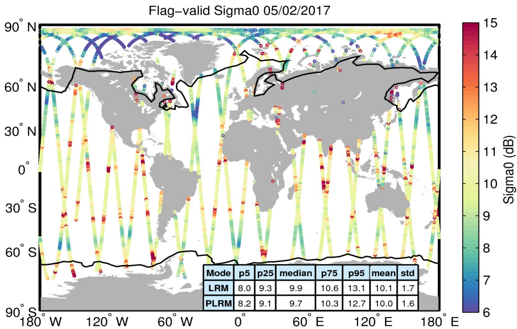
Figure 23. Geographical distribution of flag-valid sigma0 data over oceans and lakes for 05/02/2017. The statistical values shown in the table refer to the sigma0 in dB and are calculated separately for LRM and PLRM regions. Measurements taken over polar polygons have been excluded from the computation of the statistical values. The black lines mark the outer limit of the Arctic and Antarctic polar polygons.
