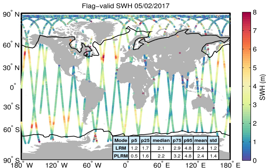
Figure 15. Geographical distribution of flag-valid SWH data over oceans and lakes for 05/02/2017. The statistical values shown in the table refer to the SWH in m and are calculated separately for LRM and PLRM regions. Measurements taken over polar polygons have been excluded from the computation of the statistical values. The black lines mark the outer limit of the Arctic and Antarctic polar polygons.
