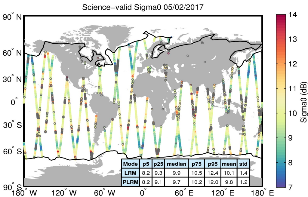
Figure 27. Geographical distribution of science-valid sigma0 data over oceans and lakes for 05/02/2017. The statistical values shown in the table refer to the sigma0 in dB and are calculated separately for LRM and PLRM regions. The black lines mark the outer limit of the Arctic and Antarctic polar polygons. Gray circles denote records that have been rejected based on the editing criteria described in Table 4.
