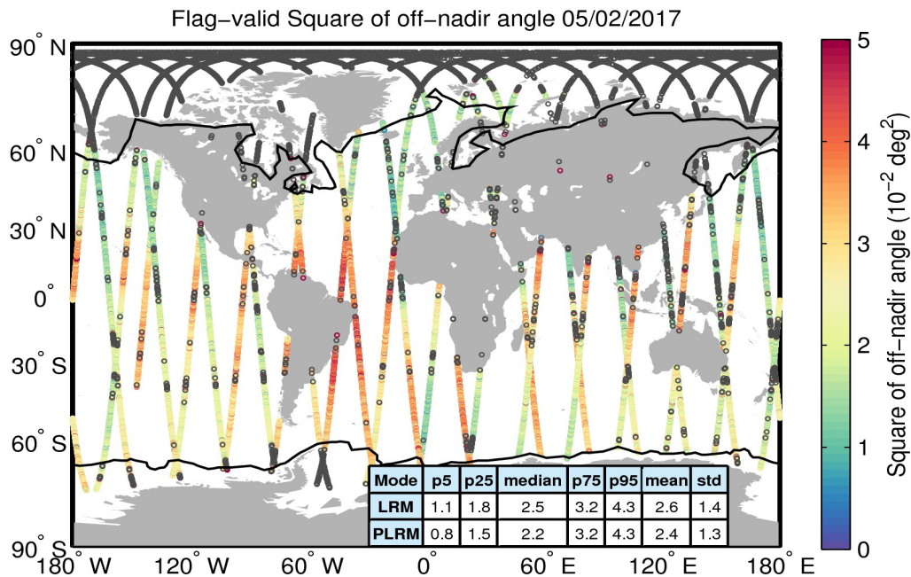
Figure 37. Geographical distribution of flag-valid mispointing data over oceans and lakes for 05/02/2017. The statistical values shown in the table refer to the mispointing in 10^{-2} deg 2 and are calculated separately for LRM and PLRM regions. Measurements taken over polar polygons have been excluded from the computation of the statistical values. The black lines mark the outer limit of the Arctic and Antarctic polar polygons. Gray circles denote negative values.
