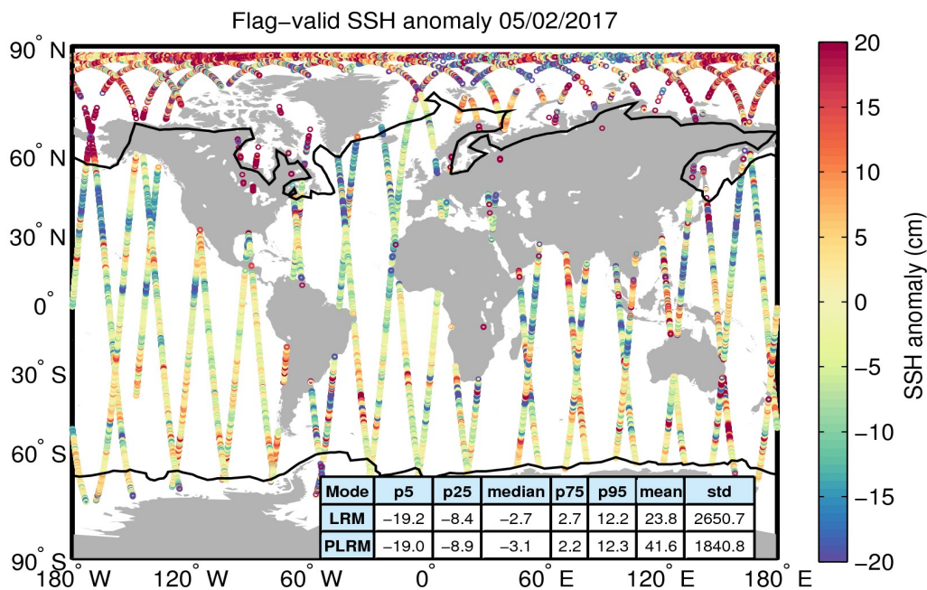
Figure 5. Geographical distribution of flag-valid 1-Hz SSH anomaly data over oceans and lakes for 05/02/2017. The statistical values shown in the table refer to the SSH anomaly in cm and are calculated separately for LRM and PLRM regions. Measurements taken over polar polygons have been excluded from the computation of the statistical values. The black lines mark the outer limit of the Arctic and Antarctic polar polygons.
