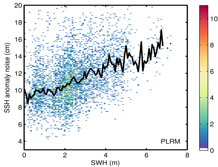
Figure 9. 2D histogram showing flag-valid SSH anomaly noise as a function of SWH for LRM (top) and PLRM (bottom) for 05/02/2017. The black line denotes the median SSH anomaly noise as a function of SWH.
