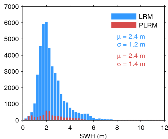
Figure 17. Histogram of flag-valid SWH over oceans and lakes for LRM (blue) and PLRM (red) for 05/02/2017. The mean ( \mu ) and standard deviation ( \sigma ) are also shown. Note that values larger than 12 m are excluded from the histogram for the sake of readability but not from the computation of \mu and \sigma .
