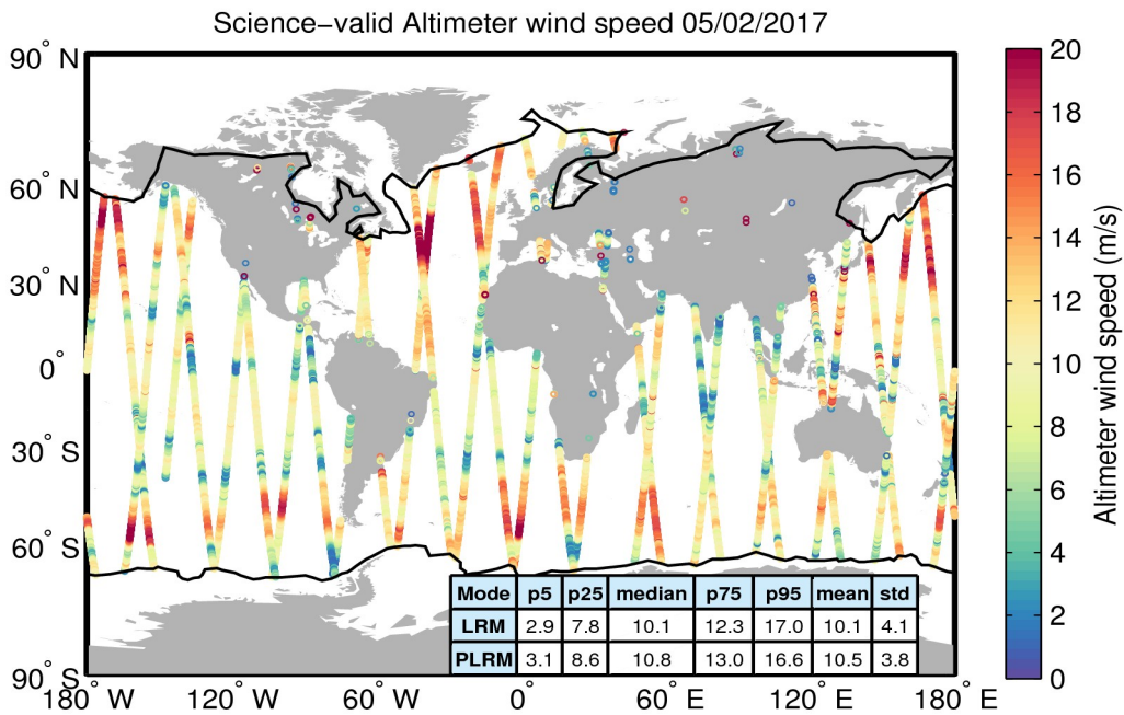
Figure 34. Geographical distribution of science-valid wind data over oceans and lakes for 05/02/2017. The statistical values shown in the table refer to the wind in m/s and are calculated separately for LRM and PLRM regions. The black lines mark the outer limit of the Arctic and Antarctic polar polygons. Gray circles denote records that have been rejected based on the editing criteria described in Table 5.
