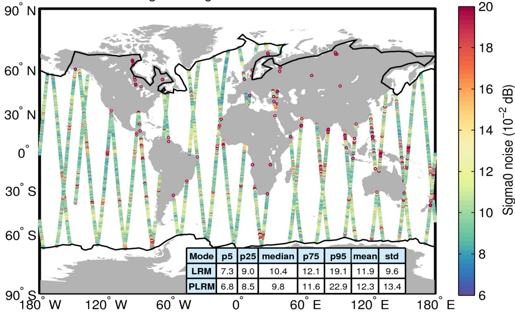
Flag-valid sigma0 noise 05/02/2017
