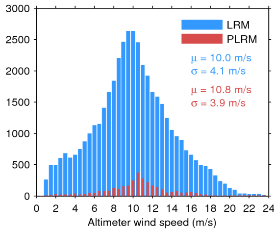
Figure 33. Histogram of flag-valid wind over oceans and lakes for LRM (blue) and PLRM (red) for 04/02/2017. The mean ( \mu ) and standard deviation ( \sigma ) are also shown. Note that values larger than 24 m/s are excluded from the histogram for the sake of readability but not from the computation of \mu and \sigma .
