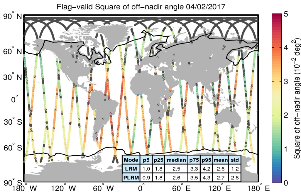
Figure 37. Geographical distribution of flag-valid mispointing data over oceans and lakes for 04/02/2017. The statistical values shown in the table refer to the mispointing in 10^{-2} deg 2 and are calculated separately for LRM and PLRM regions. Measurements taken over polar polygons have been excluded from the computation of the statistical values. The black lines mark the outer limit of the Arctic and Antarctic polar polygons. Gray circles denote negative values.
