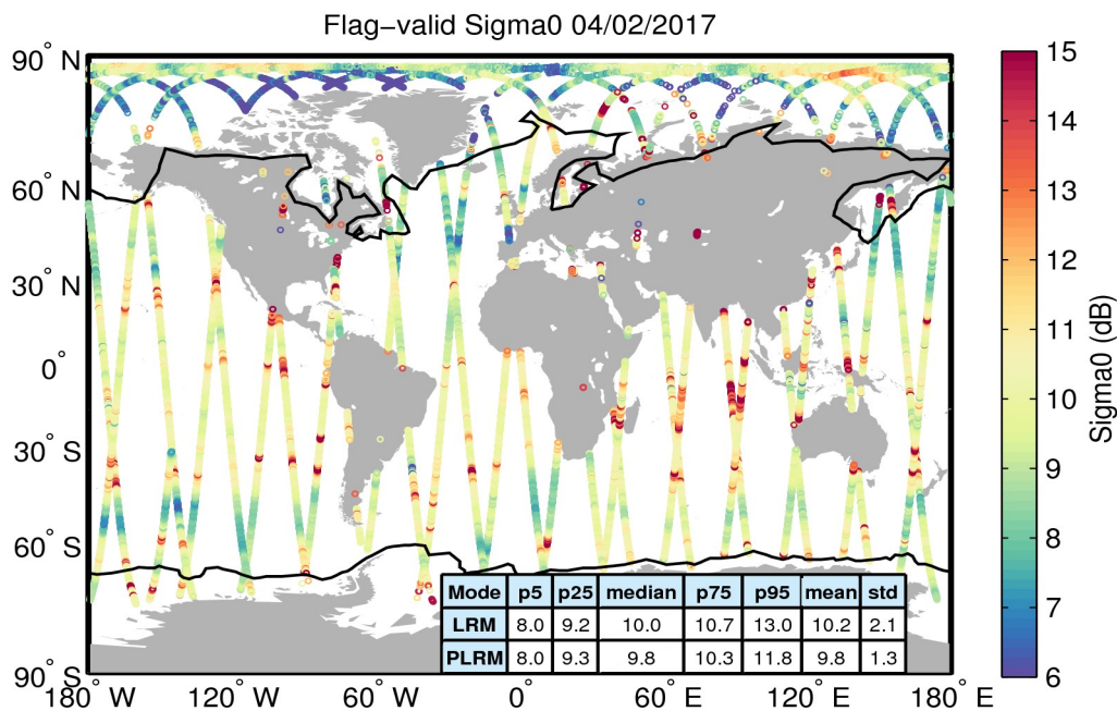
Figure 23. Geographical distribution of flag-valid sigma0 data over oceans and lakes for 04/02/2017. The statistical values shown in the table refer to the sigma0 in dB and are calculated separately for LRM and PLRM regions. Measurements taken over polar polygons have been excluded from the computation of the statistical values. The black lines mark the outer limit of the Arctic and Antarctic polar polygons.
