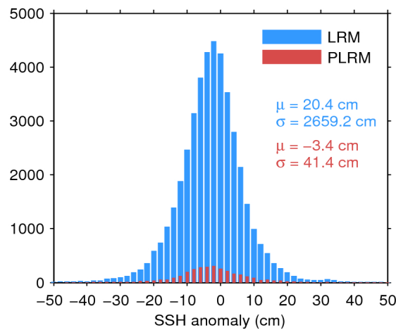
Figure 7. Histogram of flag-valid SSH anomaly over oceans and lakes for LRM (blue) and PLRM (red) for 04/02/2017. The mean ( \mu ) and standard deviation ( \sigma ) are also shown. Note that values outside [-50 50] cm are excluded from the histogram for the sake of readability but not from the computation of \mu and \sigma .
