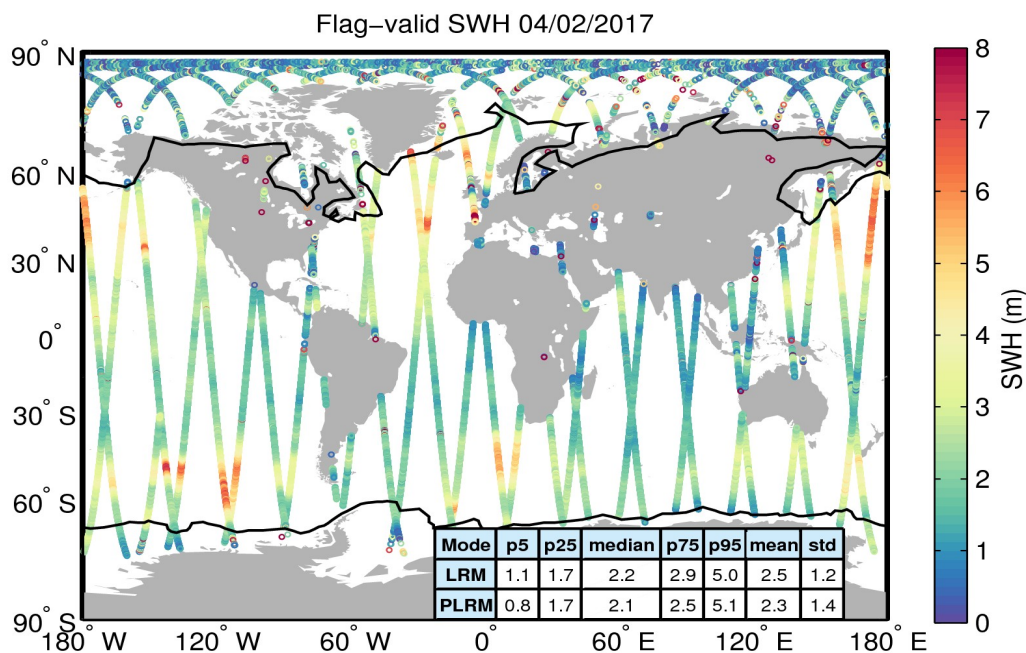
Figure 15. Geographical distribution of flag-valid SWH data over oceans and lakes for 04/02/2017. The statistical values shown in the table refer to the SWH in m and are calculated separately for LRM and PLRM regions. Measurements taken over polar polygons have been excluded from the computation of the statistical values. The black lines mark the outer limit of the Arctic and Antarctic polar polygons.
