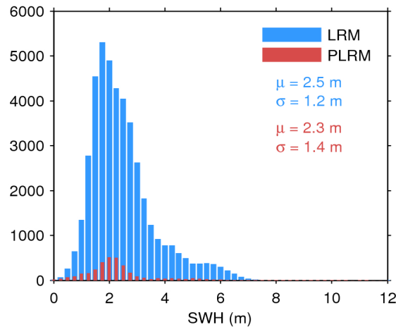
Figure 17. Histogram of flag-valid SWH over oceans and lakes for LRM (blue) and PLRM (red) for 04/02/2017. The mean ( \mu ) and standard deviation ( \sigma ) are also shown. Note that values larger than 12 m are excluded from the histogram for the sake of readability but not from the computation of \mu and \sigma .
