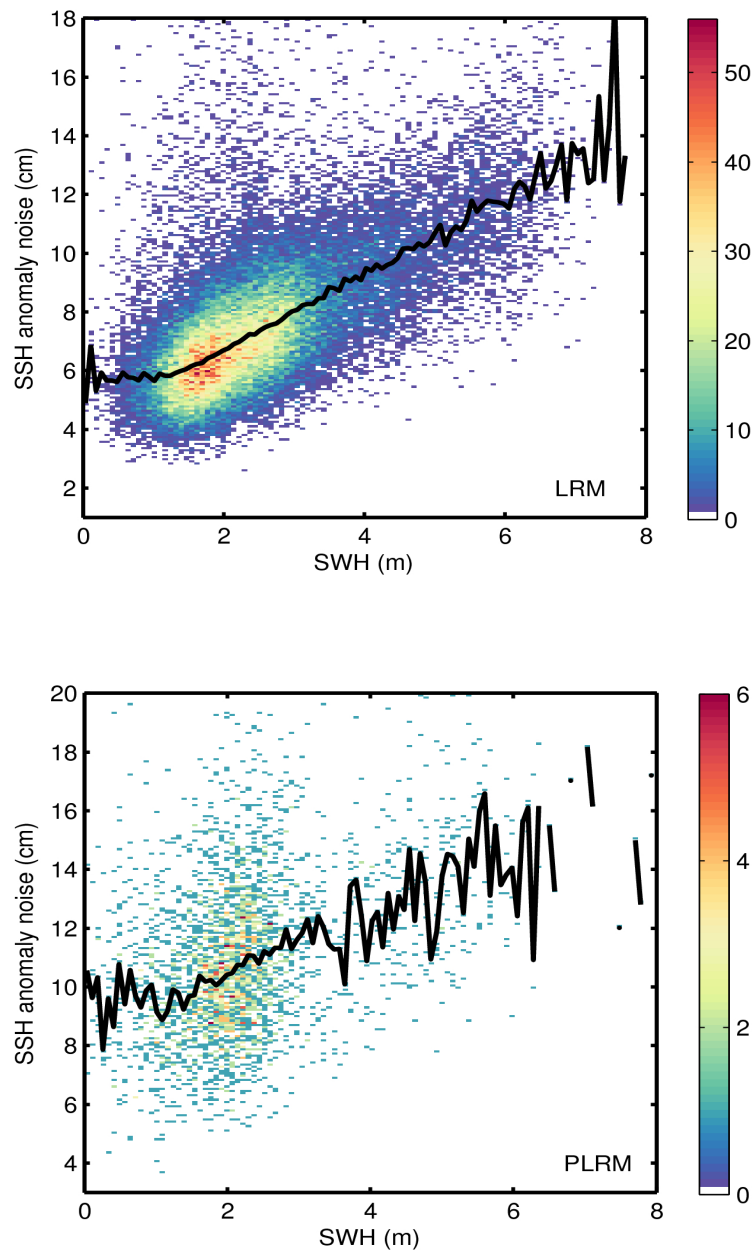
Figure 9. 2D histogram showing flag-valid SSH anomaly noise as a function of SWH for LRM (top) and PLRM (bottom) for 04/02/2017. The black line denotes the median SSH anomaly noise as a function of SWH.
