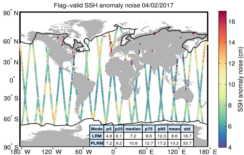
Figure 8. Geographical distribution of flag-valid 20-Hz SSH anomaly measurement noise over oceans and lakes for 04/02/2017. The statistical values shown in the table refer to the SSH anomaly noise and are calculated separately for LRM and PLRM regions. Measurements taken over polar polygons have been excluded from the computation of the statistical values. The black lines mark the outer limit of the Arctic and Antarctic polar polygons.
