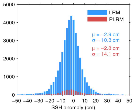
Figure 11. Histogram of science-valid SSH anomaly over oceans and lakes for LRM (blue) and PLRM (red) for 04/02/2017. The mean ( \mu ) and standard deviation ( \sigma ) are also shown. Note that values outside [-50 50] cm are excluded from the histogram for the sake of readability but not from the computation of \mu and \sigma .
