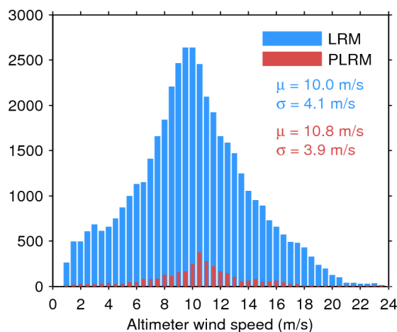
Figure 35. Histogram of science-valid wind over oceans and lakes for LRM (blue) and PLRM (red) for 04/02/2017. The mean ( \mu ) and standard deviation ( \sigma ) are also shown. Note that values larger than 24 m/s are excluded from the histogram for the sake of readability but not from the computation of \mu and \sigma .
