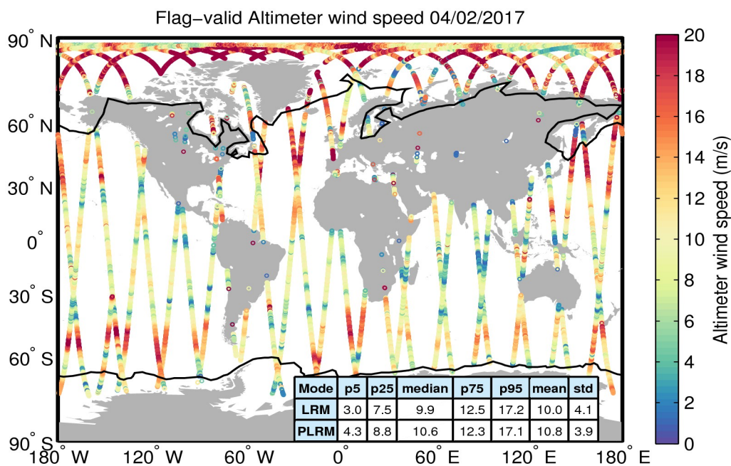
Figure 31. Geographical distribution of flag-valid wind data over oceans and lakes for 04/02/2017. The statistical values shown in the table refer to the wind in m/s and are calculated separately for LRM and PLRM regions. Measurements taken over polar polygons have been excluded from the computation of the statistical values. The black lines mark the outer limit of the Arctic and Antarctic polar polygons.
