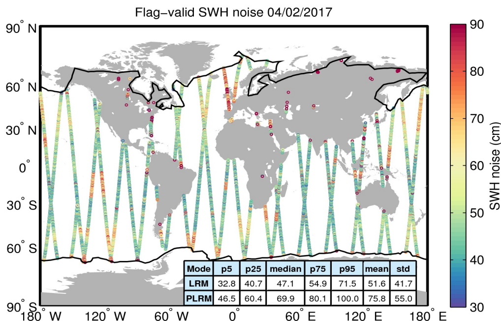
Figure 18. Geographical distribution of flag-valid 20-Hz SWH measurement noise over oceans and lakes for 04/02/2017. The statistical values shown in the table refer to the SWH noise and are calculated separately for LRM and PLRM regions. Measurements taken over polar polygons have been excluded from the computation of the statistical values. The black lines mark the outer limit of the Arctic and Antarctic polar polygons.
