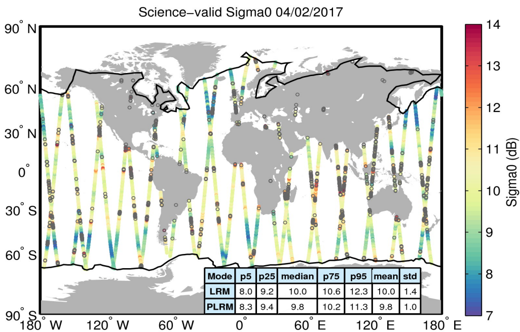
Figure 27. Geographical distribution of science-valid sigma0 data over oceans and lakes for 04/02/2017. The statistical values shown in the table refer to the sigma0 in dB and are calculated separately for LRM and PLRM regions. The black lines mark the outer limit of the Arctic and Antarctic polar polygons. Gray circles denote records that have been rejected based on the editing criteria described in Table 4.
