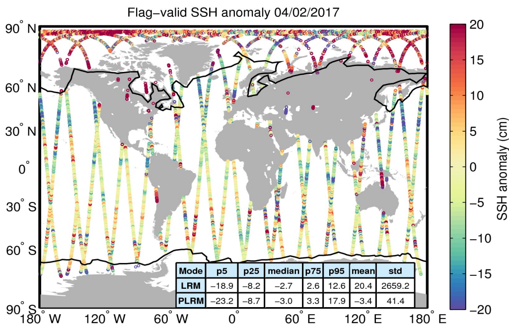
Figure 5. Geographical distribution of flag-valid 1-Hz SSH anomaly data over oceans and lakes for 04/02/2017. The statistical values shown in the table refer to the SSH anomaly in cm and are calculated separately for LRM and PLRM regions. Measurements taken over polar polygons have been excluded from the computation of the statistical values. The black lines mark the outer limit of the Arctic and Antarctic polar polygons.
