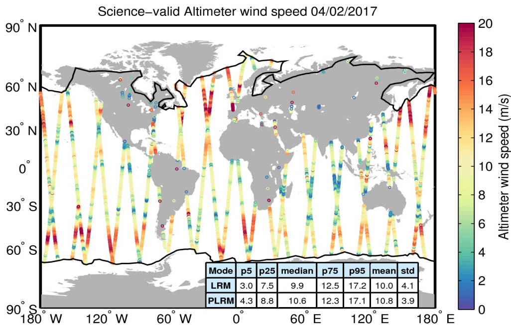
Figure 34. Geographical distribution of science-valid wind data over oceans and lakes for 04/02/2017. The statistical values shown in the table refer to the wind in m/s and are calculated separately for LRM and PLRM regions. The black lines mark the outer limit of the Arctic and Antarctic polar polygons. Gray circles denote records that have been rejected based on the editing criteria described in Table 5.
