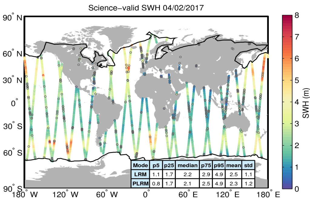
Figure 19. Geographical distribution of science-valid SWH data over oceans and lakes for 04/02/2017. The statistical values shown in the table refer to the SWH in m and are calculated separately for LRM and PLRM regions. The black lines mark the outer limit of the Arctic and Antarctic polar polygons. Gray circles denote records that have been rejected based on the editing criteria described in Table 3.
