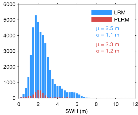
Figure 20. Histogram of science-valid SWH over oceans and lakes for LRM (blue) and PLRM (red) for 04/02/2017. The mean ( \mu ) and standard deviation ( \sigma ) are also shown. Note that values larger than 12 m are excluded from the histogram for the sake of readability but not from the computation of \mu and \sigma .
