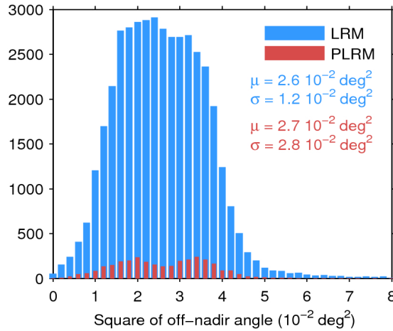
Figure 39. Histogram of flag-valid mispointing over oceans and lakes for LRM (blue) and PLRM (red) for 04/02/2017. Only positive values have been considered. The mean ( \mu ) and standard deviation ( \sigma ) are also shown. Note that values larger than 8 \cdot 10^{-2} \text{ deg}^2 are excluded from the histogram for the sake of readability but not from the computation of \mu and \sigma .
