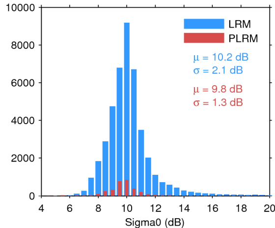
Figure 25. Histogram of flag-valid sigma0 over oceans and lakes for LRM (blue) and PLRM (red) for 04/02/2017. The mean ( \mu ) and standard deviation ( \sigma ) are also shown. Note that values outside [4 20] dB are excluded from the histogram for the sake of readability but not from the computation of \mu and \sigma .
