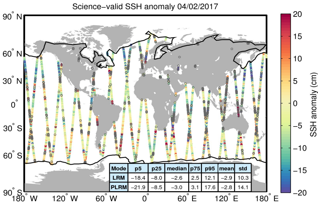
Figure 10. Geographical distribution of science-valid SSH anomaly data over oceans and lakes for 04/02/2017. The statistical values shown in the table refer to the SSH anomaly in cm and are calculated separately for LRM and PLRM regions. The black lines mark the outer limit of the Arctic and Antarctic polar polygons. Gray circles denote records that have been rejected based on the editing criteria described in Table 2.
