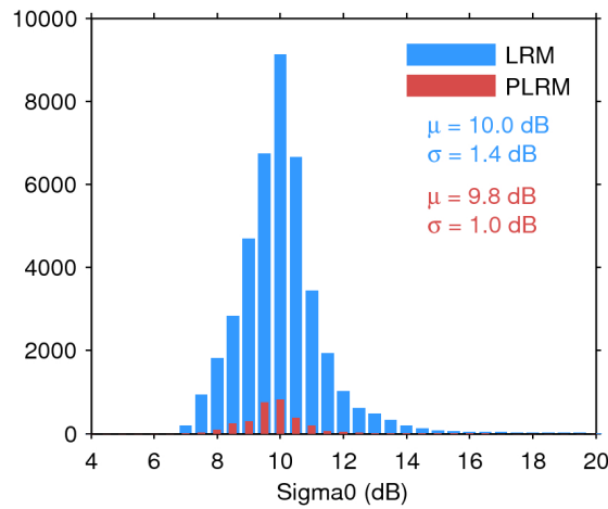
Figure 28. Histogram of science-valid sigma0 over oceans and lakes for LRM (blue) and PLRM (red) for 04/02/2017. The mean ( \mu ) and standard deviation ( \sigma ) are also shown. Note that values outside [4 20] dB are excluded from the histogram for the sake of readability but not from the computation of \mu and \sigma .
