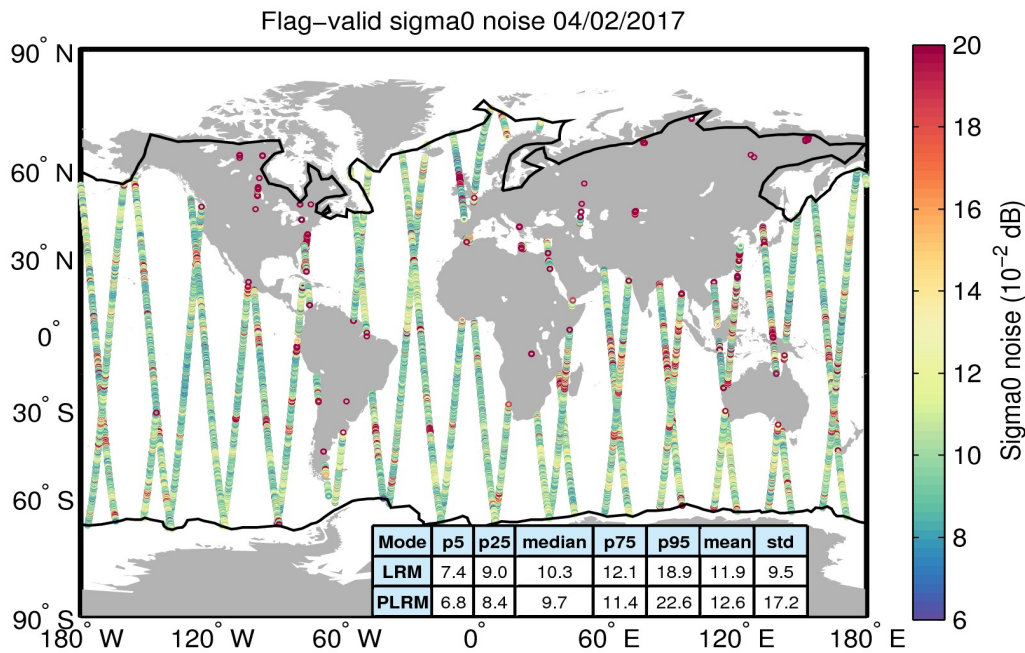
Figure 26. Geographical distribution of flag-valid 20-Hz sigma0 measurement noise over oceans and lakes for 04/02/2017. The statistical values shown in the table refer to the sigma0 noise and are calculated separately for LRM and PLRM regions. Measurements taken over polar polygons have been excluded from the computation of the statistical values. The black lines mark the outer limit of the Arctic and Antarctic polar polygons.
