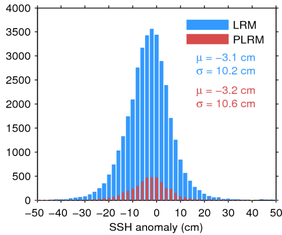
Figure 11. Histogram of science-valid SSH anomaly over oceans and lakes for LRM (blue) and PLRM (red) for 03/02/2017. The mean ( \mu ) and standard deviation ( \sigma ) are also shown. Note that values outside [-50 50] cm are excluded from the histogram for the sake of readability but not from the computation of \mu and \sigma .
