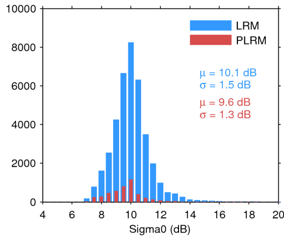
Figure 28. Histogram of science-valid sigma0 over oceans and lakes for LRM (blue) and PLRM (red) for 03/02/2017. The mean ( \mu ) and standard deviation ( \sigma ) are also shown. Note that values outside [4 20] dB are excluded from the histogram for the sake of readability but not from the computation of \mu and \sigma .
