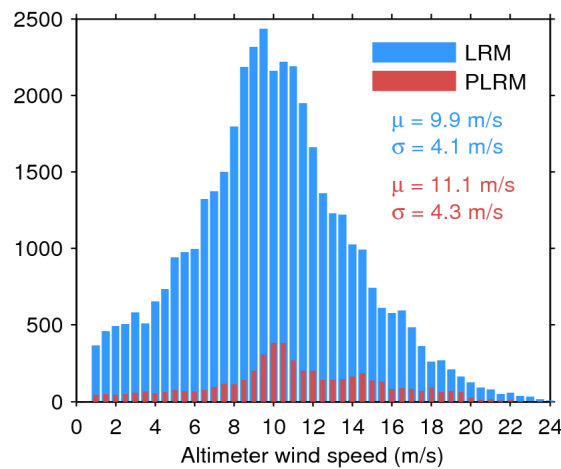
Figure 33. Histogram of flag-valid wind over oceans and lakes for LRM (blue) and PLRM (red) for 03/02/2017. The mean ( \mu ) and standard deviation ( \sigma ) are also shown. Note that values larger than 24 m/s are excluded from the histogram for the sake of readability but not from the computation of \mu and \sigma .
