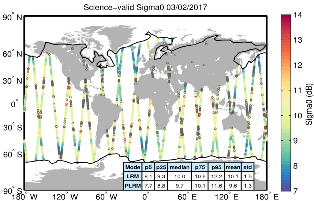
Figure 27. Geographical distribution of science-valid sigma0 data over oceans and lakes for 03/02/2017. The statistical values shown in the table refer to the sigma0 in dB and are calculated separately for LRM and PLRM regions. The black lines mark the outer limit of the Arctic and Antarctic polar polygons. Gray circles denote records that have been rejected based on the editing criteria described in Table 4.
