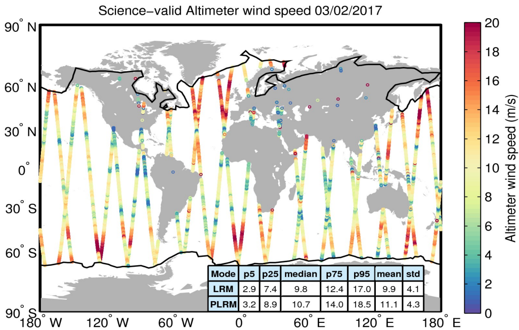
Figure 34. Geographical distribution of science-valid wind data over oceans and lakes for 03/02/2017. The statistical values shown in the table refer to the wind in m/s and are calculated separately for LRM and PLRM regions. The black lines mark the outer limit of the Arctic and Antarctic polar polygons. Gray circles denote records that have been rejected based on the editing criteria described in Table 5.
