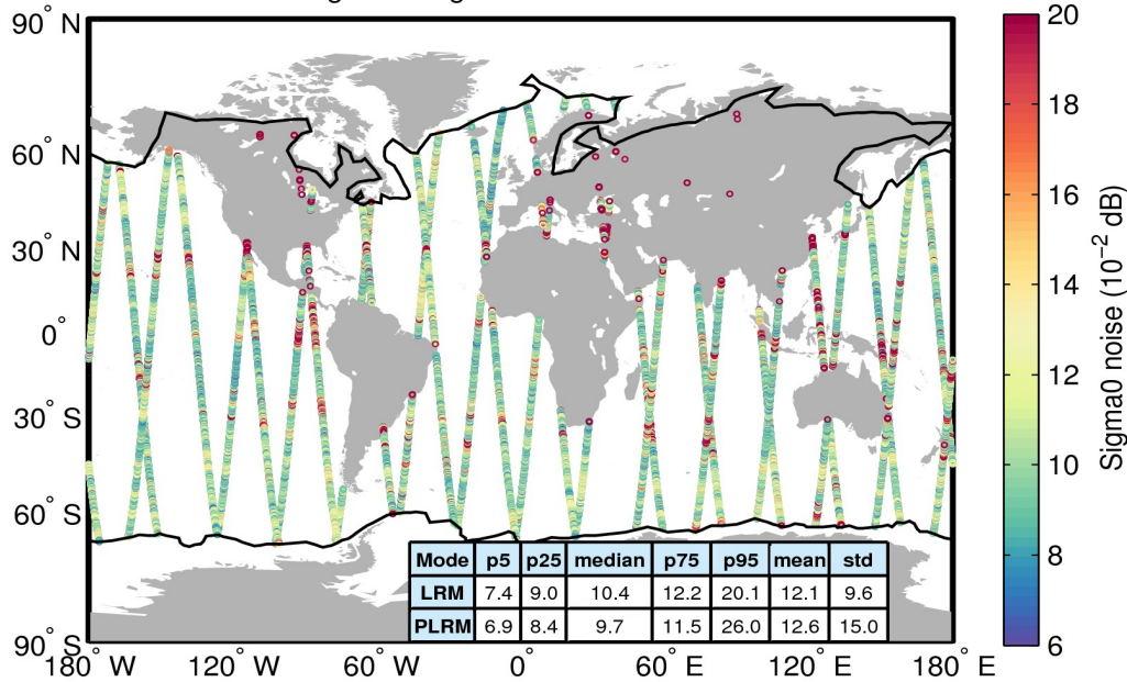
Flag-valid sigma0 noise 03/02/2017
