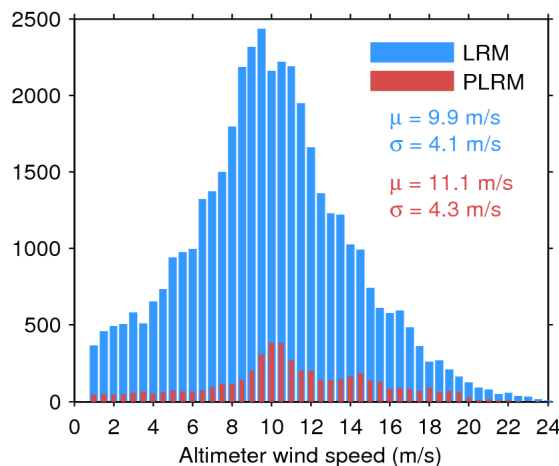
Figure 35. Histogram of science-valid wind over oceans and lakes for LRM (blue) and PLRM (red) for 03/02/2017. The mean ( \mu ) and standard deviation ( \sigma ) are also shown. Note that values larger than 24 m/s are excluded from the histogram for the sake of readability but not from the computation of \mu and \sigma .
