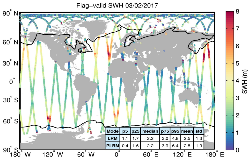
Figure 15. Geographical distribution of flag-valid SWH data over oceans and lakes for 03/02/2017. The statistical values shown in the table refer to the SWH in m and are calculated separately for LRM and PLRM regions. Measurements taken over polar polygons have been excluded from the computation of the statistical values. The black lines mark the outer limit of the Arctic and Antarctic polar polygons.
