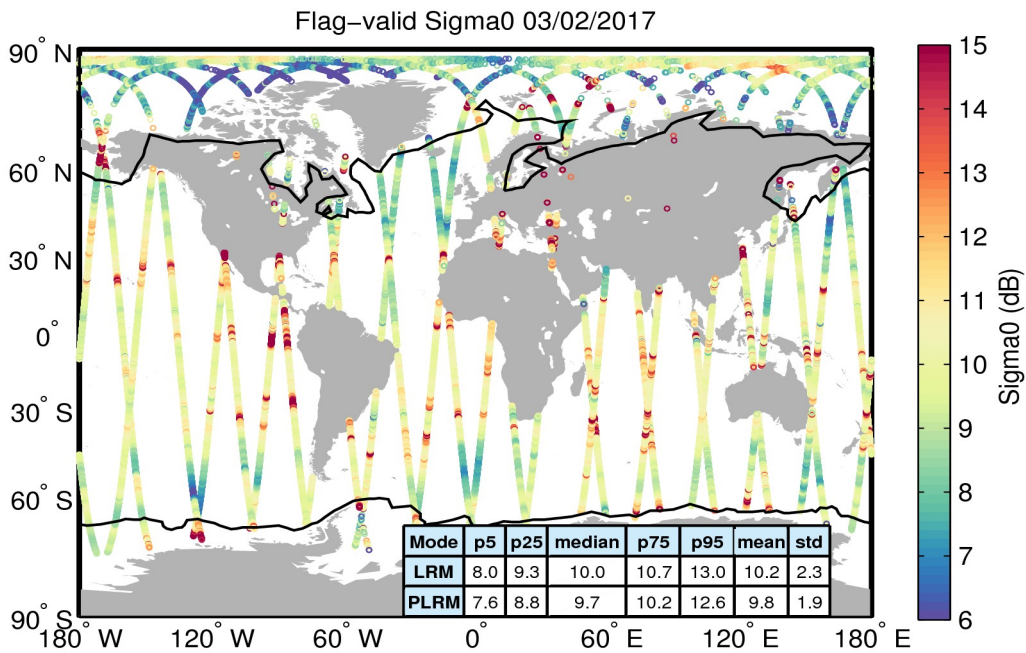
Figure 23. Geographical distribution of flag-valid sigma0 data over oceans and lakes for 03/02/2017. The statistical values shown in the table refer to the sigma0 in dB and are calculated separately for LRM and PLRM regions. Measurements taken over polar polygons have been excluded from the computation of the statistical values. The black lines mark the outer limit of the Arctic and Antarctic polar polygons.
