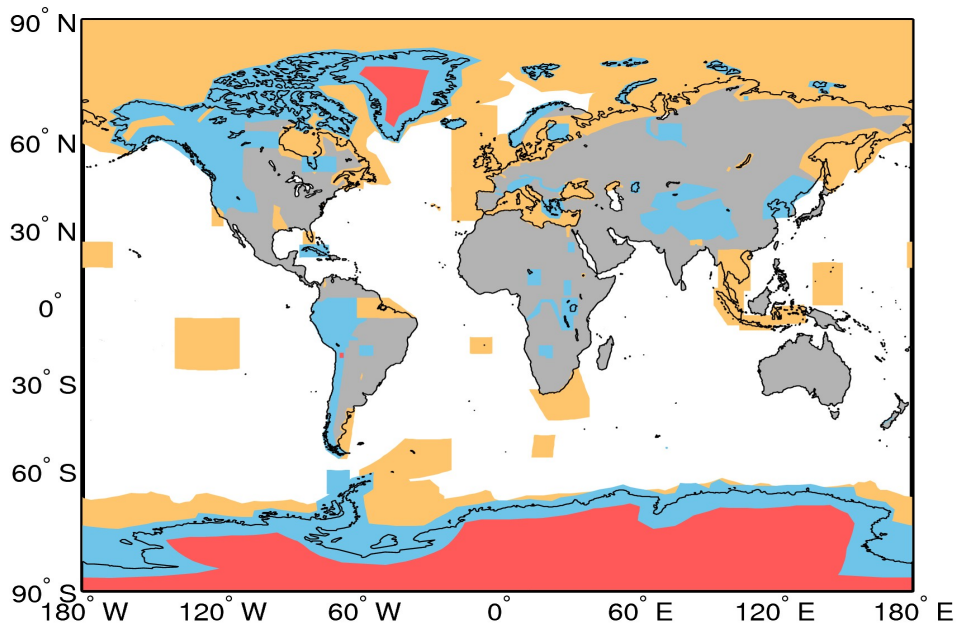
Figure A1. Extent of the regions defining the geographical mode mask for 03/02/2017. The regions where SAR, and SARIn are operated are denoted by the orange and blue polygons, respectively. LRM is operated over areas of the continental ice sheets (red polygons) and over oceans and land not covered by other modes.
