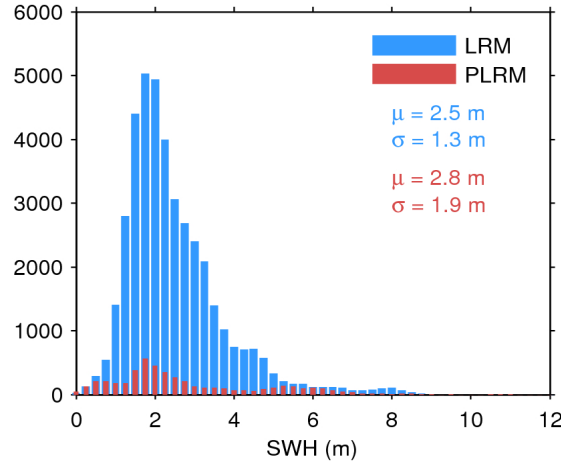
Figure 17. Histogram of flag-valid SWH over oceans and lakes for LRM (blue) and PLRM (red) for 03/02/2017. The mean ( \mu ) and standard deviation ( \sigma ) are also shown. Note that values larger than 12 m are excluded from the histogram for the sake of readability but not from the computation of \mu and \sigma .
