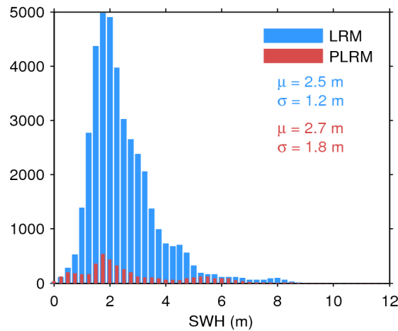
Figure 20. Histogram of science-valid SWH over oceans and lakes for LRM (blue) and PLRM (red) for 03/02/2017. The mean ( \mu ) and standard deviation ( \sigma ) are also shown. Note that values larger than 12 m are excluded from the histogram for the sake of readability but not from the computation of \mu and \sigma .
