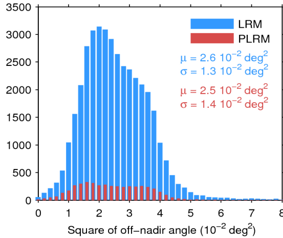
Figure 39. Histogram of flag-valid mispointing over oceans and lakes for LRM (blue) and PLRM (red) for 03/02/2017. Only positive values have been considered. The mean ( \mu ) and standard deviation ( \sigma ) are also shown. Note that values larger than 8 \cdot 10^{-2} \text{ deg}^2 are excluded from the histogram for the sake of readability but not from the computation of \mu and \sigma .
