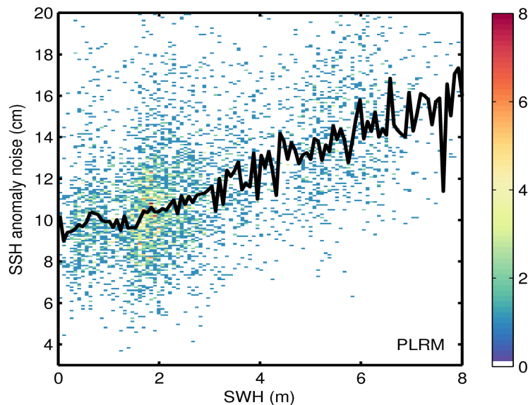
Figure 9. 2D histogram showing flag-valid SSH anomaly noise as a function of SWH for LRM (top) and PLRM (bottom) for 03/02/2017. The black line denotes the median SSH anomaly noise as a function of SWH.
