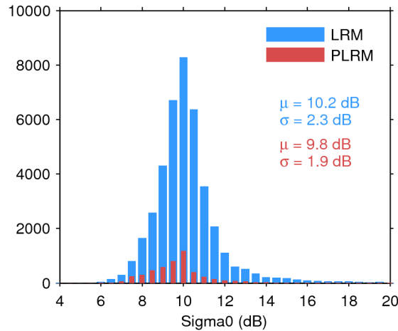
Figure 25. Histogram of flag-valid sigma0 over oceans and lakes for LRM (blue) and PLRM (red) for 03/02/2017. The mean ( \mu ) and standard deviation ( \sigma ) are also shown. Note that values outside [4 20] dB are excluded from the histogram for the sake of readability but not from the computation of \mu and \sigma .
