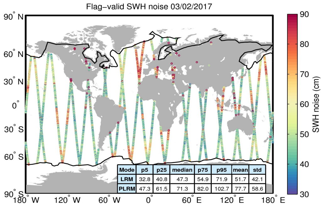
Figure 18. Geographical distribution of flag-valid 20-Hz SWH measurement noise over oceans and lakes for 03/02/2017. The statistical values shown in the table refer to the SWH noise and are calculated separately for LRM and PLRM regions. Measurements taken over polar polygons have been excluded from the computation of the statistical values. The black lines mark the outer limit of the Arctic and Antarctic polar polygons.
