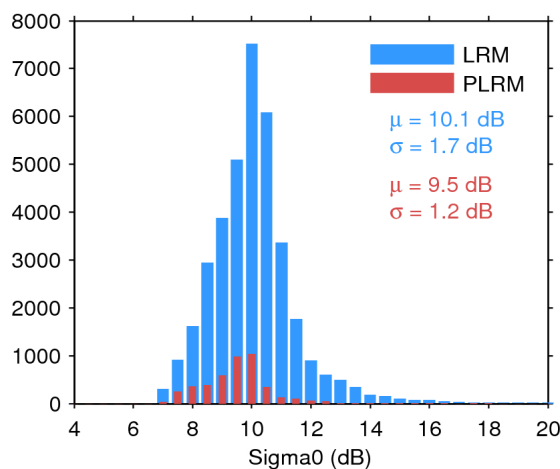
Figure 28. Histogram of science-valid sigma0 over oceans and lakes for LRM (blue) and PLRM (red) for 01/02/2017. The mean ( \mu ) and standard deviation ( \sigma ) are also shown. Note that values outside [4 20] dB are excluded from the histogram for the sake of readability but not from the computation of \mu and \sigma .
