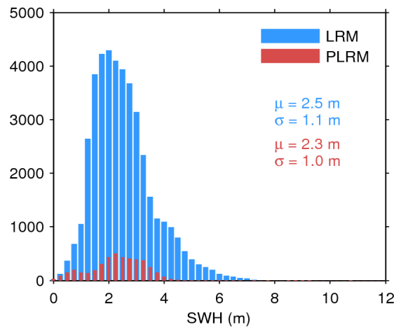
Figure 17. Histogram of flag-valid SWH over oceans and lakes for LRM (blue) and PLRM (red) for 30/01/2017. The mean ( \mu ) and standard deviation ( \sigma ) are also shown. Note that values larger than 12 m are excluded from the histogram for the sake of readability but not from the computation of \mu and \sigma .
