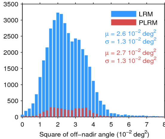
Figure 39. Histogram of flag-valid mispointing over oceans and lakes for LRM (blue) and PLRM (red) for 30/01/2017. Only positive values have been considered. The mean ( \mu ) and standard deviation ( \sigma ) are also shown. Note that values larger than 8 \cdot 10^{-2} \text{ deg}^2 are excluded from the histogram for the sake of readability but not from the computation of \mu and \sigma .
