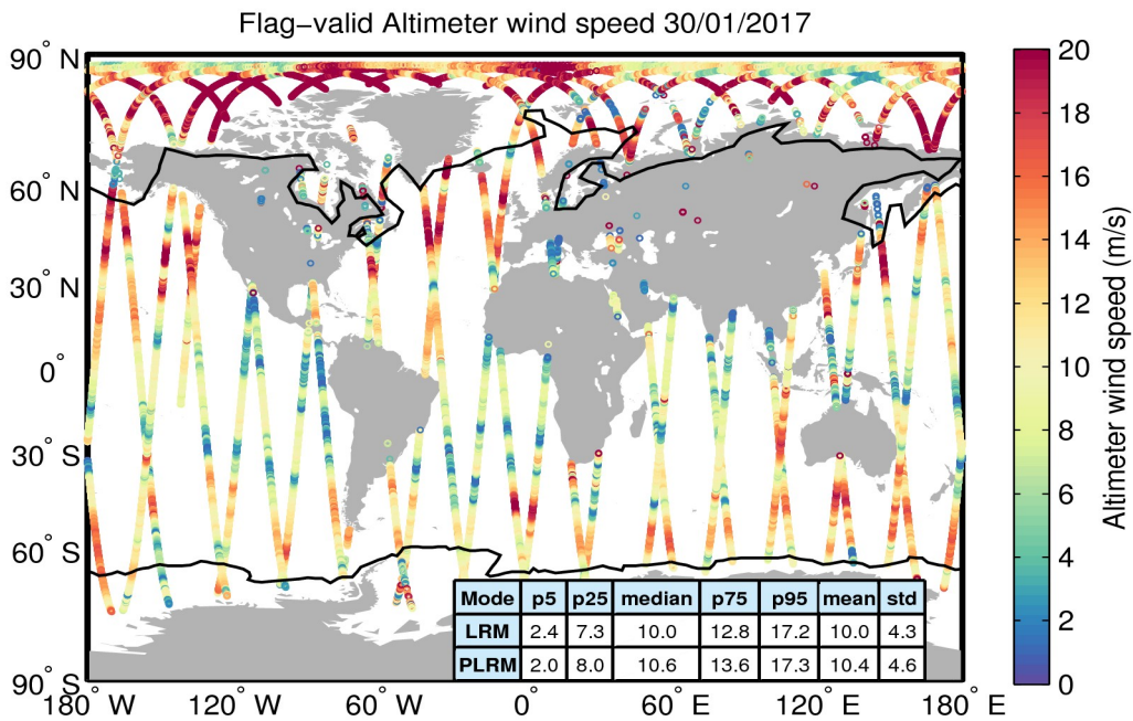
Figure 31. Geographical distribution of flag-valid wind data over oceans and lakes for 30/01/2017. The statistical values shown in the table refer to the wind in m/s and are calculated separately for LRM and PLRM regions. Measurements taken over polar polygons have been excluded from the computation of the statistical values. The black lines mark the outer limit of the Arctic and Antarctic polar polygons.
