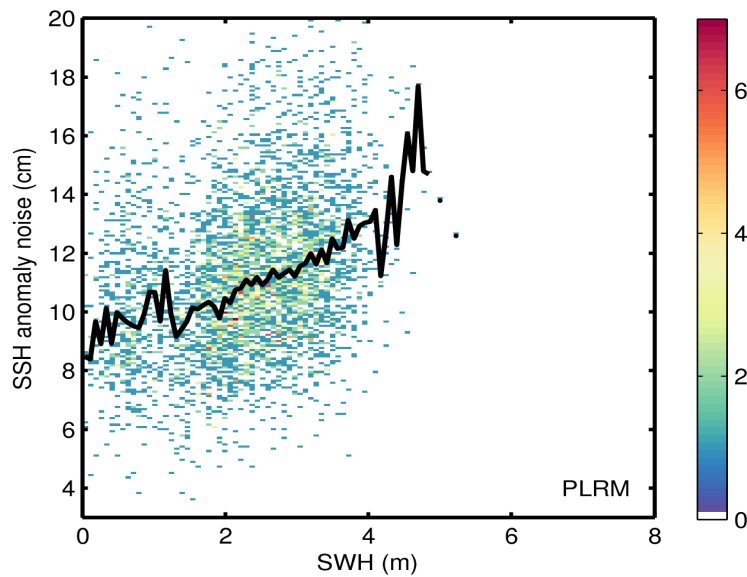
Figure 9. 2D histogram showing flag-valid SSH anomaly noise as a function of SWH for LRM (top) and PLRM (bottom) for 30/01/2017. The black line denotes the median SSH anomaly noise as a function of SWH.
