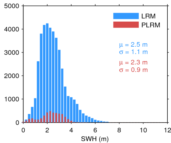
Figure 20. Histogram of science-valid SWH over oceans and lakes for LRM (blue) and PLRM (red) for 30/01/2017. The mean ( \mu ) and standard deviation ( \sigma ) are also shown. Note that values larger than 12 m are excluded from the histogram for the sake of readability but not from the computation of \mu and \sigma .
