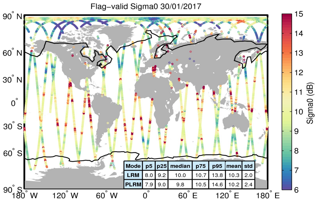
Figure 23. Geographical distribution of flag-valid sigma0 data over oceans and lakes for 30/01/2017. The statistical values shown in the table refer to the sigma0 in dB and are calculated separately for LRM and PLRM regions. Measurements taken over polar polygons have been excluded from the computation of the statistical values. The black lines mark the outer limit of the Arctic and Antarctic polar polygons.
