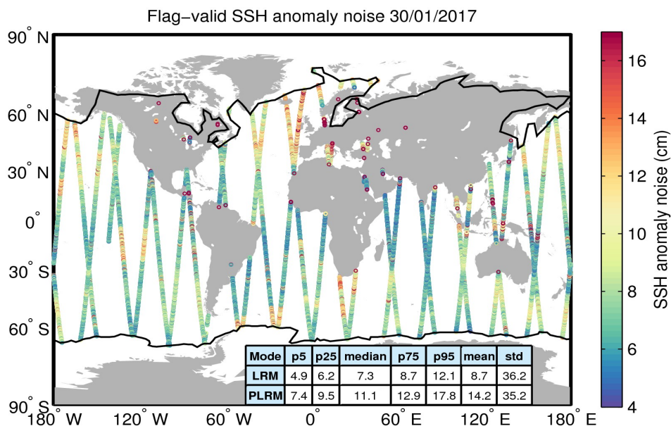
Figure 8. Geographical distribution of flag-valid 20-Hz SSH anomaly measurement noise over oceans and lakes for 30/01/2017. The statistical values shown in the table refer to the SSH anomaly noise and are calculated separately for LRM and PLRM regions. Measurements taken over polar polygons have been excluded from the computation of the statistical values. The black lines mark the outer limit of the Arctic and Antarctic polar polygons.
