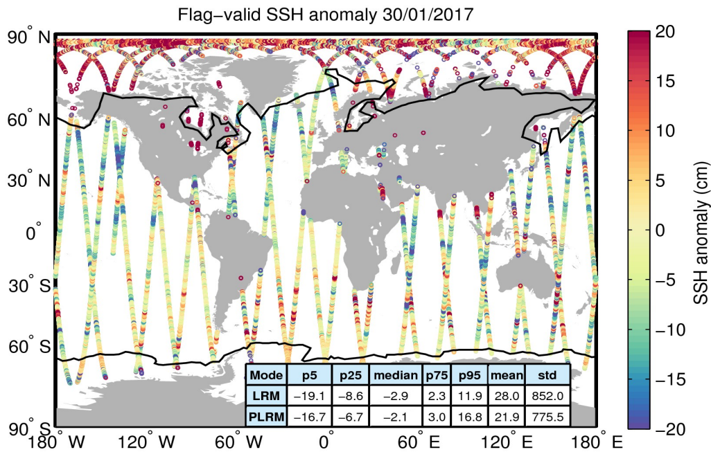
Figure 5. Geographical distribution of flag-valid 1-Hz SSH anomaly data over oceans and lakes for 30/01/2017. The statistical values shown in the table refer to the SSH anomaly in cm and are calculated separately for LRM and PLRM regions. Measurements taken over polar polygons have been excluded from the computation of the statistical values. The black lines mark the outer limit of the Arctic and Antarctic polar polygons.
