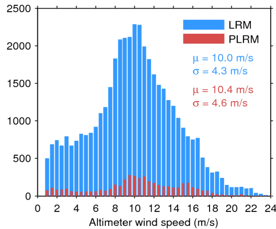
Figure 33. Histogram of flag-valid wind over oceans and lakes for LRM (blue) and PLRM (red) for 30/01/2017. The mean ( \mu ) and standard deviation ( \sigma ) are also shown. Note that values larger than 24 m/s are excluded from the histogram for the sake of readability but not from the computation of \mu and \sigma .
