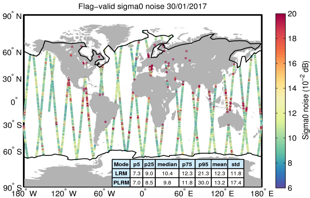
Figure 26. Geographical distribution of flag-valid 20-Hz sigma0 measurement noise over oceans and lakes for 30/01/2017. The statistical values shown in the table refer to the sigma0 noise and are calculated separately for LRM and PLRM regions. Measurements taken over polar polygons have been excluded from the computation of the statistical values. The black lines mark the outer limit of the Arctic and Antarctic polar polygons.
