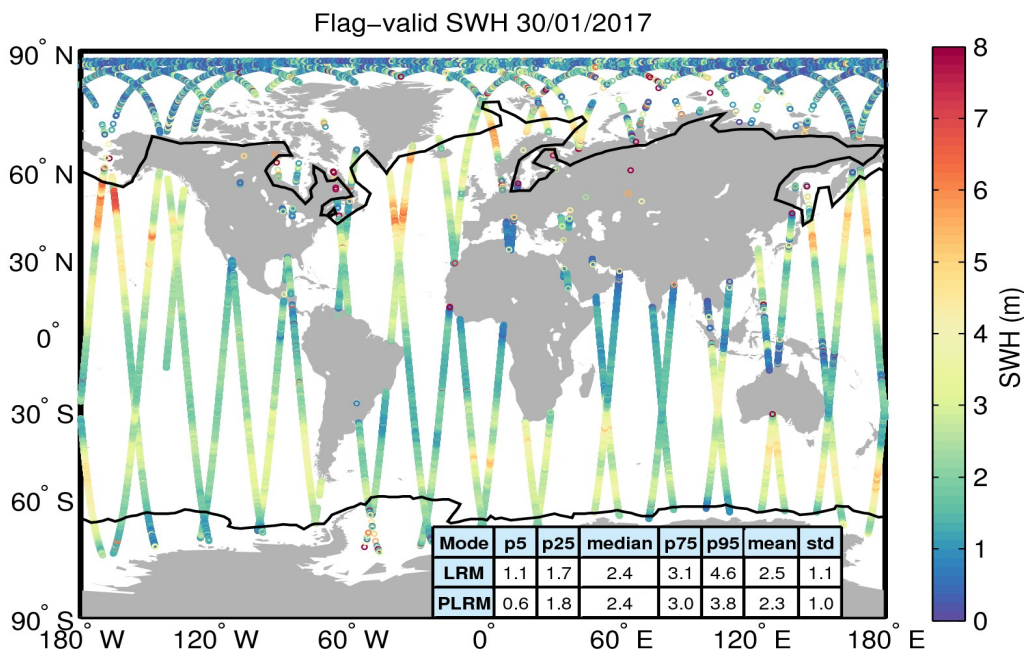
Figure 15. Geographical distribution of flag-valid SWH data over oceans and lakes for 30/01/2017. The statistical values shown in the table refer to the SWH in m and are calculated separately for LRM and PLRM regions. Measurements taken over polar polygons have been excluded from the computation of the statistical values. The black lines mark the outer limit of the Arctic and Antarctic polar polygons.
