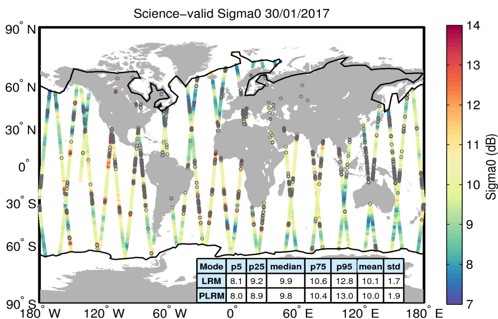
Figure 27. Geographical distribution of science-valid sigma0 data over oceans and lakes for 30/01/2017. The statistical values shown in the table refer to the sigma0 in dB and are calculated separately for LRM and PLRM regions. The black lines mark the outer limit of the Arctic and Antarctic polar polygons. Gray circles denote records that have been rejected based on the editing criteria described in Table 4.
