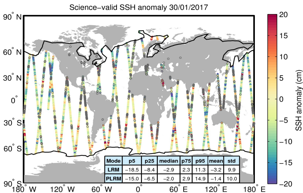
Figure 10. Geographical distribution of science-valid SSH anomaly data over oceans and lakes for 30/01/2017. The statistical values shown in the table refer to the SSH anomaly in cm and are calculated separately for LRM and PLRM regions. The black lines mark the outer limit of the Arctic and Antarctic polar polygons. Gray circles denote records that have been rejected based on the editing criteria described in Table 2.
