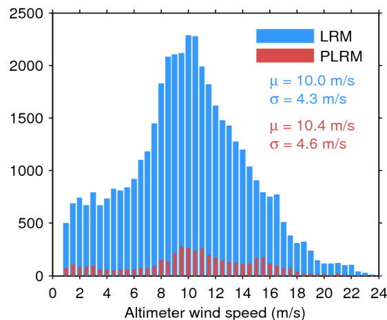
Figure 35. Histogram of science-valid wind over oceans and lakes for LRM (blue) and PLRM (red) for 30/01/2017. The mean ( \mu ) and standard deviation ( \sigma ) are also shown. Note that values larger than 24 m/s are excluded from the histogram for the sake of readability but not from the computation of \mu and \sigma .
