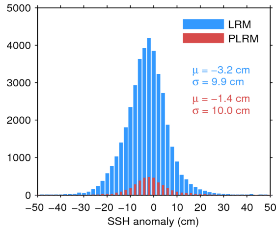
Figure 11. Histogram of science-valid SSH anomaly over oceans and lakes for LRM (blue) and PLRM (red) for 30/01/2017. The mean ( \mu ) and standard deviation ( \sigma ) are also shown. Note that values outside [-50 50] cm are excluded from the histogram for the sake of readability but not from the computation of \mu and \sigma .
