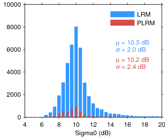
Figure 25. Histogram of flag-valid sigma0 over oceans and lakes for LRM (blue) and PLRM (red) for 30/01/2017. The mean ( \mu ) and standard deviation ( \sigma ) are also shown. Note that values outside [4 20] dB are excluded from the histogram for the sake of readability but not from the computation of \mu and \sigma .
