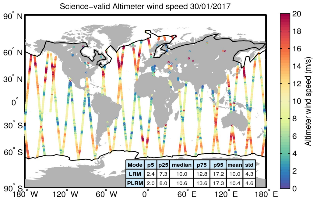
Figure 34. Geographical distribution of science-valid wind data over oceans and lakes for 30/01/2017. The statistical values shown in the table refer to the wind in m/s and are calculated separately for LRM and PLRM regions. The black lines mark the outer limit of the Arctic and Antarctic polar polygons. Gray circles denote records that have been rejected based on the editing criteria described in Table 5.
