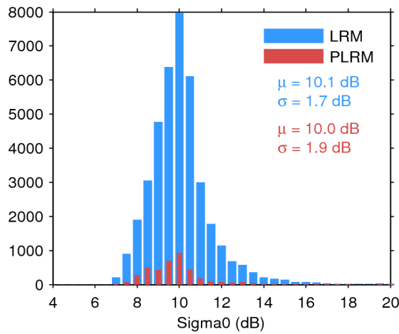
Figure 28. Histogram of science-valid sigma0 over oceans and lakes for LRM (blue) and PLRM (red) for 30/01/2017. The mean ( \mu ) and standard deviation ( \sigma ) are also shown. Note that values outside [4 20] dB are excluded from the histogram for the sake of readability but not from the computation of \mu and \sigma .
