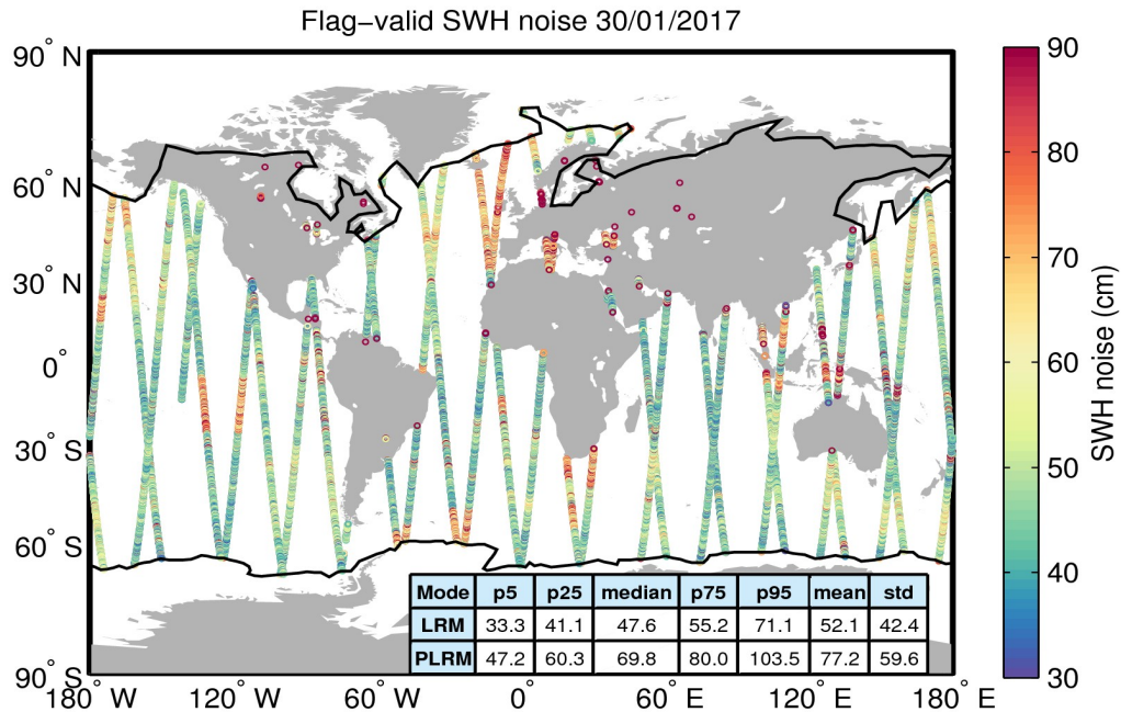
Figure 18. Geographical distribution of flag-valid 20-Hz SWH measurement noise over oceans and lakes for 30/01/2017. The statistical values shown in the table refer to the SWH noise and are calculated separately for LRM and PLRM regions. Measurements taken over polar polygons have been excluded from the computation of the statistical values. The black lines mark the outer limit of the Arctic and Antarctic polar polygons.
