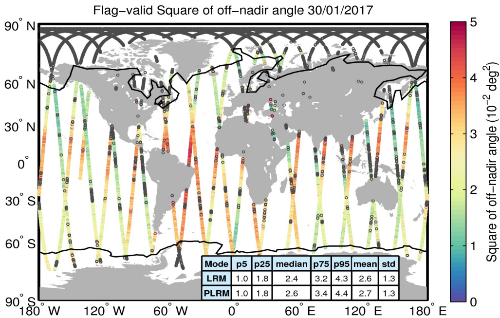
Figure 37. Geographical distribution of flag-valid mispointing data over oceans and lakes for 30/01/2017. The statistical values shown in the table refer to the mispointing in 10^{-2} deg 2 and are calculated separately for LRM and PLRM regions. Measurements taken over polar polygons have been excluded from the computation of the statistical values. The black lines mark the outer limit of the Arctic and Antarctic polar polygons. Gray circles denote negative values.
