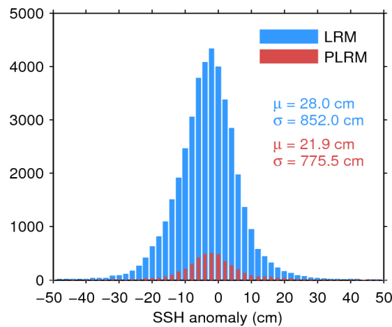
Figure 7. Histogram of flag-valid SSH anomaly over oceans and lakes for LRM (blue) and PLRM (red) for 30/01/2017. The mean ( \mu ) and standard deviation ( \sigma ) are also shown. Note that values outside [-50\ 50] cm are excluded from the histogram for the sake of readability but not from the computation of \mu and \sigma .
