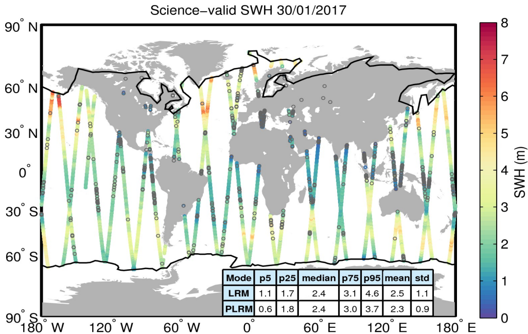
Figure 19. Geographical distribution of science-valid SWH data over oceans and lakes for 30/01/2017. The statistical values shown in the table refer to the SWH in m and are calculated separately for LRM and PLRM regions. The black lines mark the outer limit of the Arctic and Antarctic polar polygons. Gray circles denote records that have been rejected based on the editing criteria described in Table 3.
