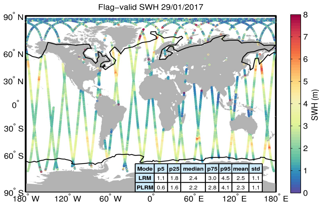
Figure 15. Geographical distribution of flag-valid SWH data over oceans and lakes for 29/01/2017. The statistical values shown in the table refer to the SWH in m and are calculated separately for LRM and PLRM regions. Measurements taken over polar polygons have been excluded from the computation of the statistical values. The black lines mark the outer limit of the Arctic and Antarctic polar polygons.
