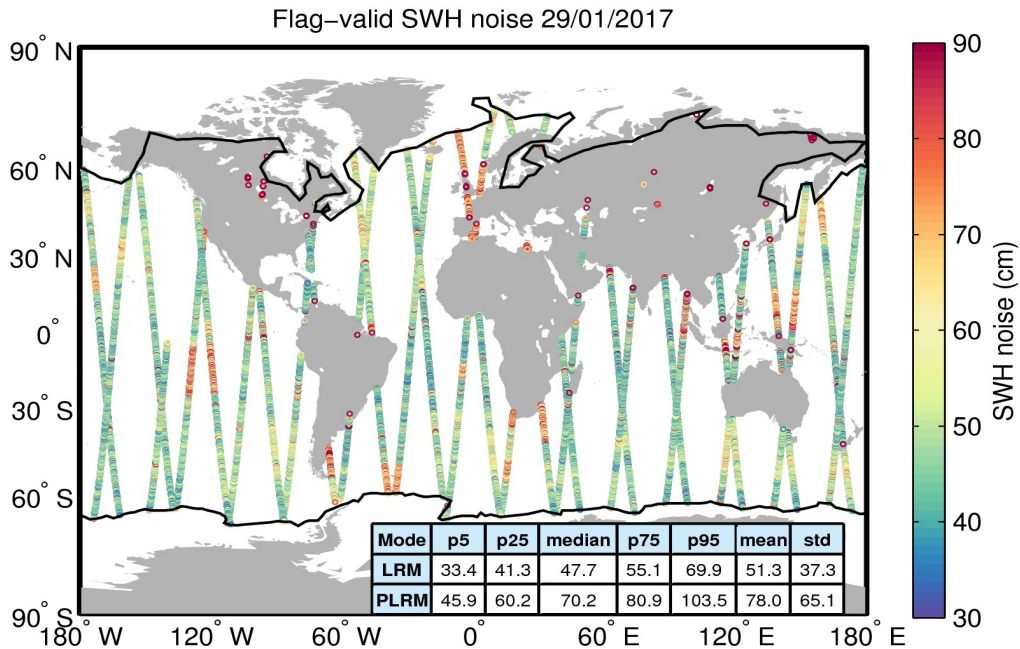
Figure 18. Geographical distribution of flag-valid 20-Hz SWH measurement noise over oceans and lakes for 29/01/2017. The statistical values shown in the table refer to the SWH noise and are calculated separately for LRM and PLRM regions. Measurements taken over polar polygons have been excluded from the computation of the statistical values. The black lines mark the outer limit of the Arctic and Antarctic polar polygons.
