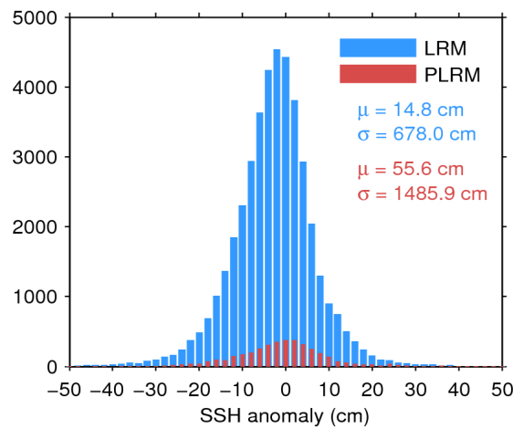
Figure 7. Histogram of flag-valid SSH anomaly over oceans and lakes for LRM (blue) and PLRM (red) for 29/01/2017. The mean ( \mu ) and standard deviation ( \sigma ) are also shown. Note that values outside [-50 50] cm are excluded from the histogram for the sake of readability but not from the computation of \mu and \sigma .
