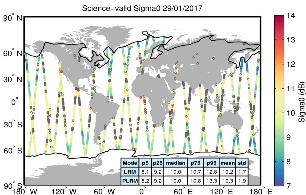
Figure 27. Geographical distribution of science-valid sigma0 data over oceans and lakes for 29/01/2017. The statistical values shown in the table refer to the sigma0 in dB and are calculated separately for LRM and PLRM regions. The black lines mark the outer limit of the Arctic and Antarctic polar polygons. Gray circles denote records that have been rejected based on the editing criteria described in Table 4.
