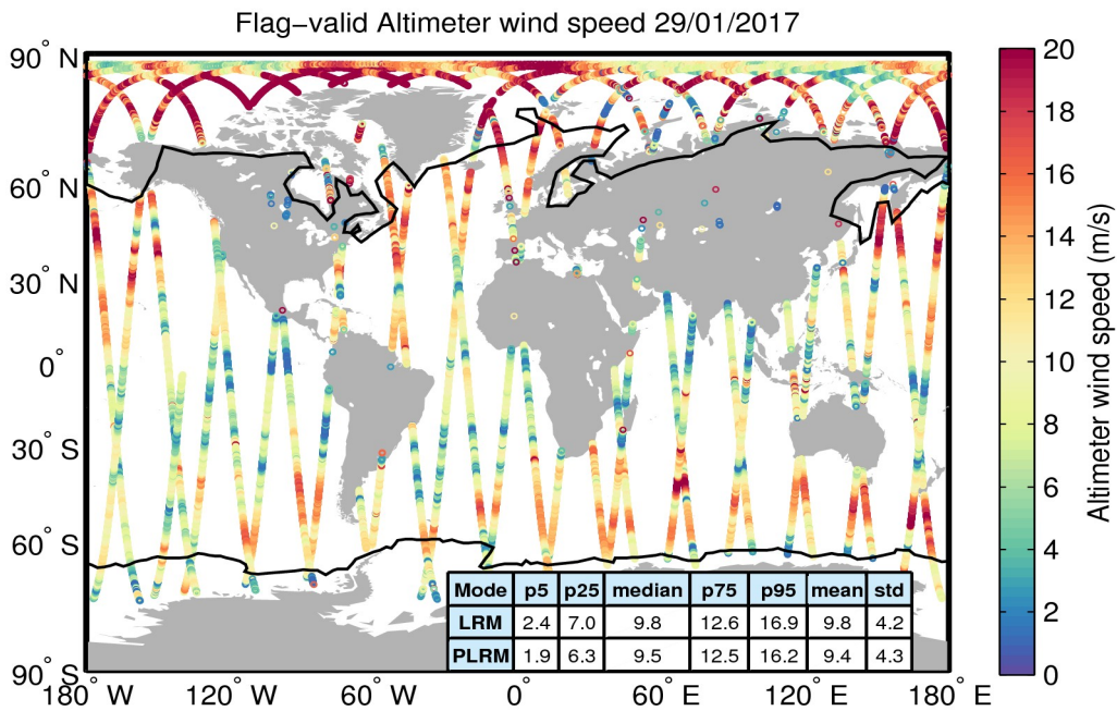
Figure 31. Geographical distribution of flag-valid wind data over oceans and lakes for 29/01/2017. The statistical values shown in the table refer to the wind in m/s and are calculated separately for LRM and PLRM regions. Measurements taken over polar polygons have been excluded from the computation of the statistical values. The black lines mark the outer limit of the Arctic and Antarctic polar polygons.
