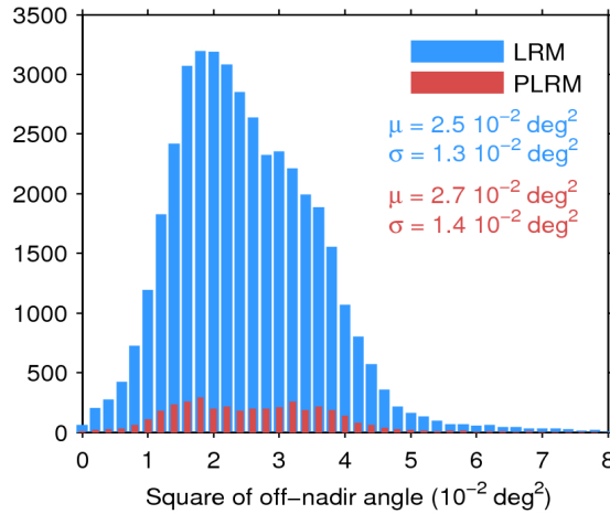
Figure 39. Histogram of flag-valid mispointing over oceans and lakes for LRM (blue) and PLRM (red) for 29/01/2017. Only positive values have been considered. The mean ( \mu ) and standard deviation ( \sigma ) are also shown. Note that values larger than 8 \cdot 10^{-2} \text{ deg}^2 are excluded from the histogram for the sake of readability but not from the computation of \mu and \sigma .
