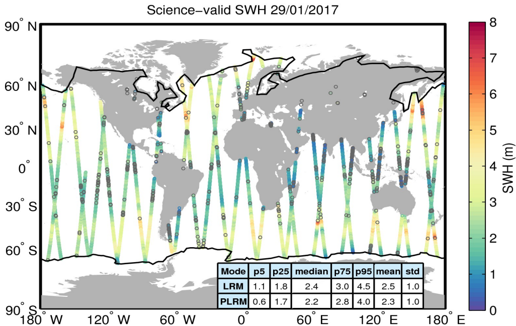
Figure 19. Geographical distribution of science-valid SWH data over oceans and lakes for 29/01/2017. The statistical values shown in the table refer to the SWH in m and are calculated separately for LRM and PLRM regions. The black lines mark the outer limit of the Arctic and Antarctic polar polygons. Gray circles denote records that have been rejected based on the editing criteria described in Table 3.
