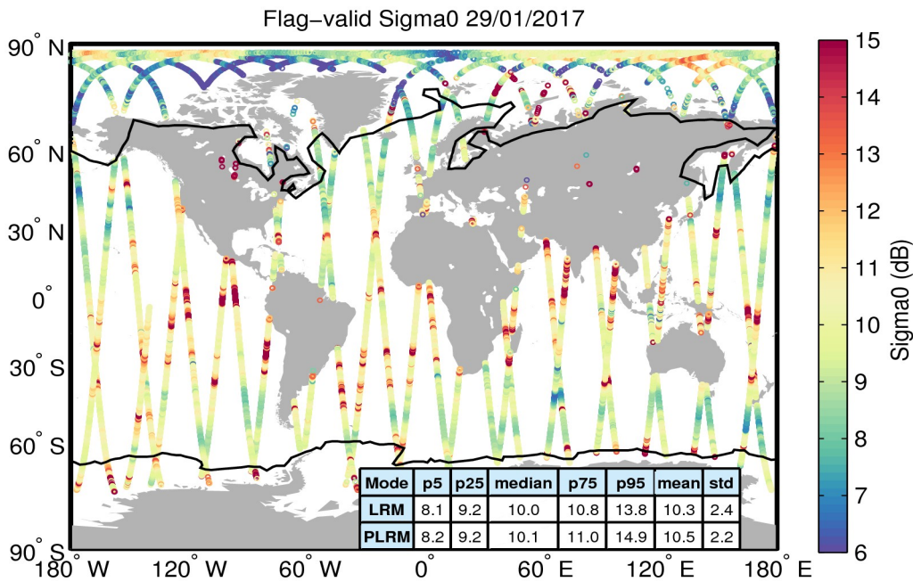
Figure 23. Geographical distribution of flag-valid sigma0 data over oceans and lakes for 29/01/2017. The statistical values shown in the table refer to the sigma0 in dB and are calculated separately for LRM and PLRM regions. Measurements taken over polar polygons have been excluded from the computation of the statistical values. The black lines mark the outer limit of the Arctic and Antarctic polar polygons.
