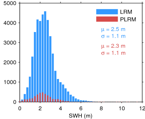
Figure 17. Histogram of flag-valid SWH over oceans and lakes for LRM (blue) and PLRM (red) for 29/01/2017. The mean ( \mu ) and standard deviation ( \sigma ) are also shown. Note that values larger than 12 m are excluded from the histogram for the sake of readability but not from the computation of \mu and \sigma .
