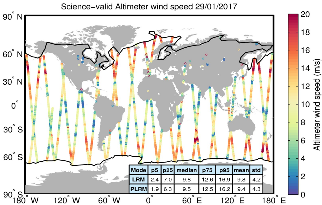
Figure 34. Geographical distribution of science-valid wind data over oceans and lakes for 29/01/2017. The statistical values shown in the table refer to the wind in m/s and are calculated separately for LRM and PLRM regions. The black lines mark the outer limit of the Arctic and Antarctic polar polygons. Gray circles denote records that have been rejected based on the editing criteria described in Table 5.
