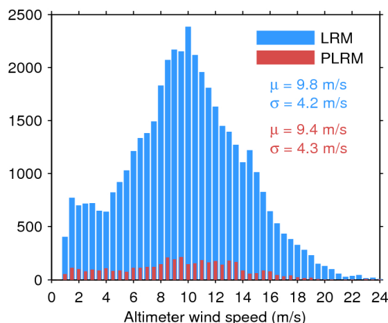
Figure 33. Histogram of flag-valid wind over oceans and lakes for LRM (blue) and PLRM (red) for 29/01/2017. The mean ( \mu ) and standard deviation ( \sigma ) are also shown. Note that values larger than 24 m/s are excluded from the histogram for the sake of readability but not from the computation of \mu and \sigma .
