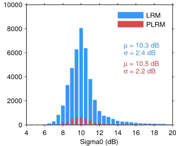
Figure 25. Histogram of flag-valid sigma0 over oceans and lakes for LRM (blue) and PLRM (red) for 29/01/2017. The mean ( \mu ) and standard deviation ( \sigma ) are also shown. Note that values outside [4 20] dB are excluded from the histogram for the sake of readability but not from the computation of \mu and \sigma .
