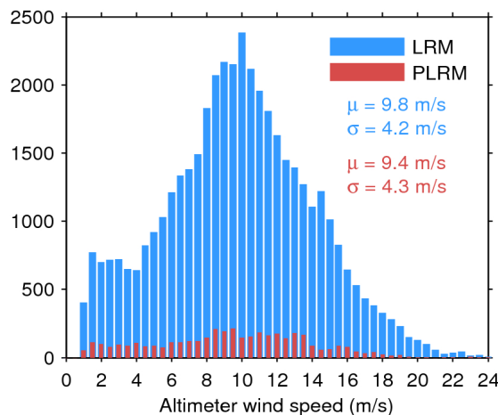
Figure 35. Histogram of science-valid wind over oceans and lakes for LRM (blue) and PLRM (red) for 29/01/2017. The mean ( \mu ) and standard deviation ( \sigma ) are also shown. Note that values larger than 24 m/s are excluded from the histogram for the sake of readability but not from the computation of \mu and \sigma .
