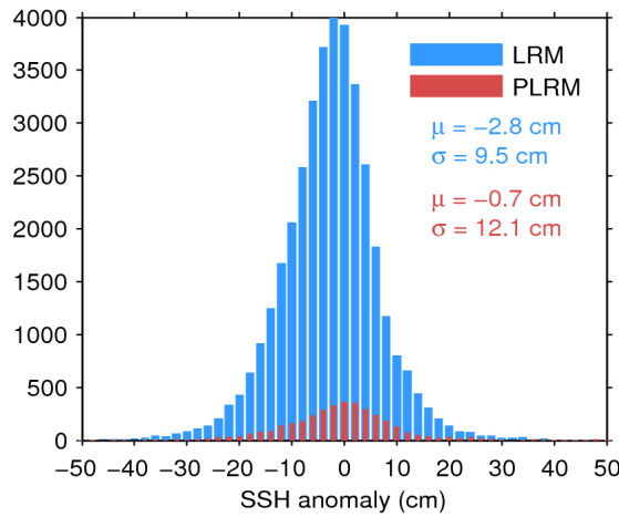
Figure 11. Histogram of science-valid SSH anomaly over oceans and lakes for LRM (blue) and PLRM (red) for 29/01/2017. The mean ( \mu ) and standard deviation ( \sigma ) are also shown. Note that values outside [-50 50] cm are excluded from the histogram for the sake of readability but not from the computation of \mu and \sigma .
