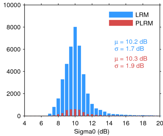
Figure 28. Histogram of science-valid sigma0 over oceans and lakes for LRM (blue) and PLRM (red) for 29/01/2017. The mean ( \mu ) and standard deviation ( \sigma ) are also shown. Note that values outside [4 20] dB are excluded from the histogram for the sake of readability but not from the computation of \mu and \sigma .
