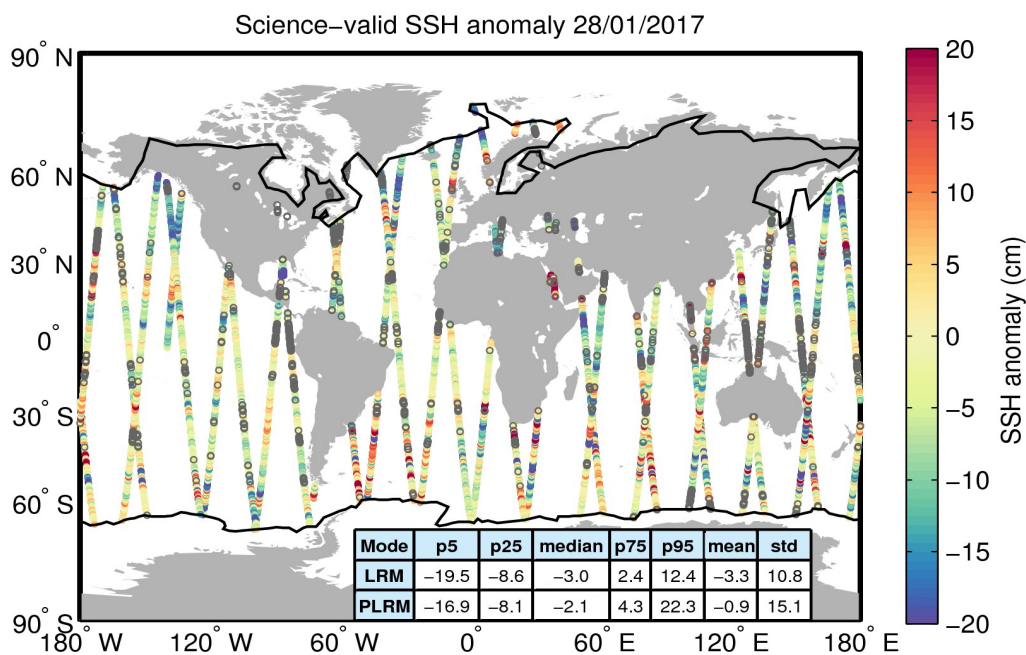
Figure 10. Geographical distribution of science-valid SSH anomaly data over oceans and lakes for 28/01/2017. The statistical values shown in the table refer to the SSH anomaly in cm and are calculated separately for LRM and PLRM regions. The black lines mark the outer limit of the Arctic and Antarctic polar polygons. Gray circles denote records that have been rejected based on the editing criteria described in Table 2.
