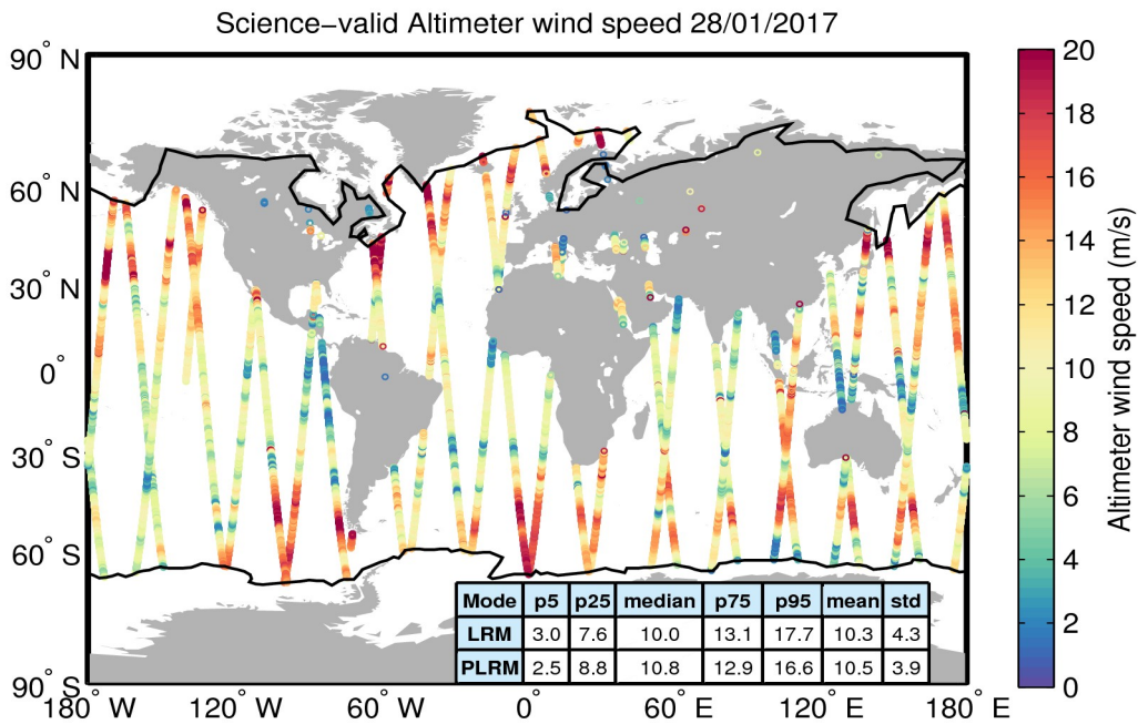
Figure 34. Geographical distribution of science-valid wind data over oceans and lakes for 28/01/2017. The statistical values shown in the table refer to the wind in m/s and are calculated separately for LRM and PLRM regions. The black lines mark the outer limit of the Arctic and Antarctic polar polygons. Gray circles denote records that have been rejected based on the editing criteria described in Table 5.
