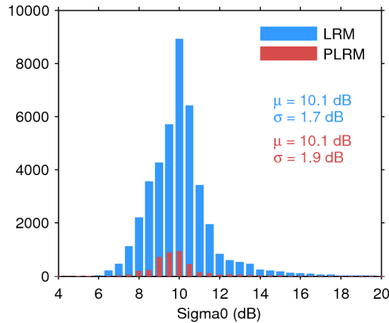
Figure 25. Histogram of flag-valid sigma0 over oceans and lakes for LRM (blue) and PLRM (red) for 28/01/2017. The mean ( \mu ) and standard deviation ( \sigma ) are also shown. Note that values outside [4 20] dB are excluded from the histogram for the sake of readability but not from the computation of \mu and \sigma .
