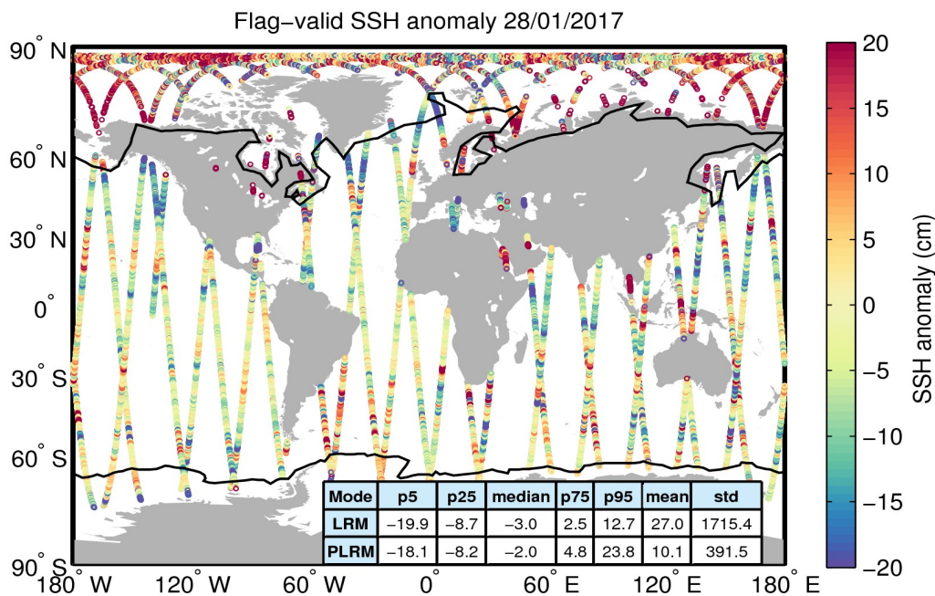
Figure 5. Geographical distribution of flag-valid 1-Hz SSH anomaly data over oceans and lakes for 28/01/2017. The statistical values shown in the table refer to the SSH anomaly in cm and are calculated separately for LRM and PLRM regions. Measurements taken over polar polygons have been excluded from the computation of the statistical values. The black lines mark the outer limit of the Arctic and Antarctic polar polygons.
