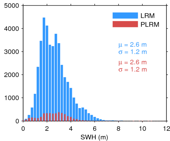
Figure 17. Histogram of flag-valid SWH over oceans and lakes for LRM (blue) and PLRM (red) for 28/01/2017. The mean ( \mu ) and standard deviation ( \sigma ) are also shown. Note that values larger than 12 m are excluded from the histogram for the sake of readability but not from the computation of \mu and \sigma .
