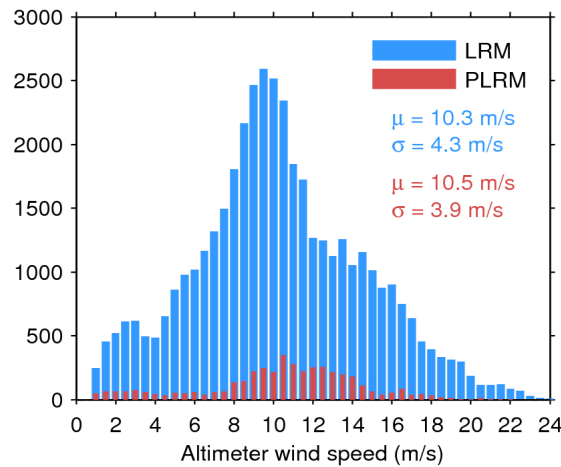
Figure 33. Histogram of flag-valid wind over oceans and lakes for LRM (blue) and PLRM (red) for 28/01/2017. The mean ( \mu ) and standard deviation ( \sigma ) are also shown. Note that values larger than 24 m/s are excluded from the histogram for the sake of readability but not from the computation of \mu and \sigma .
