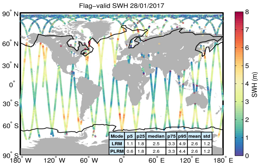
Figure 15. Geographical distribution of flag-valid SWH data over oceans and lakes for 28/01/2017. The statistical values shown in the table refer to the SWH in m and are calculated separately for LRM and PLRM regions. Measurements taken over polar polygons have been excluded from the computation of the statistical values. The black lines mark the outer limit of the Arctic and Antarctic polar polygons.
