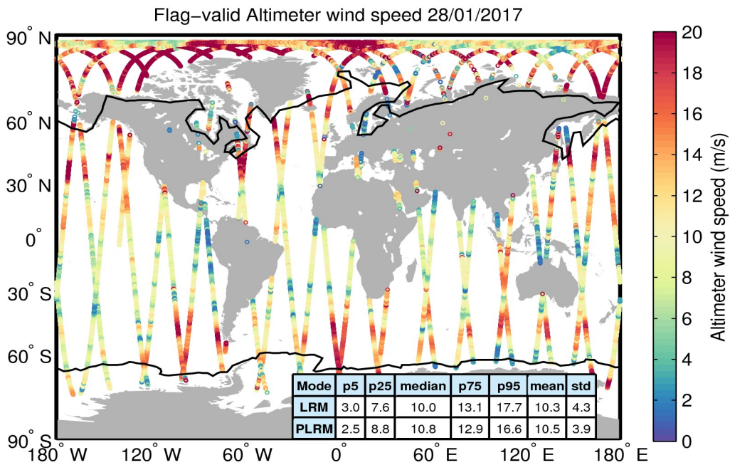
Figure 31. Geographical distribution of flag-valid wind data over oceans and lakes for 28/01/2017. The statistical values shown in the table refer to the wind in m/s and are calculated separately for LRM and PLRM regions. Measurements taken over polar polygons have been excluded from the computation of the statistical values. The black lines mark the outer limit of the Arctic and Antarctic polar polygons.
