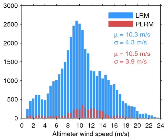
Figure 35. Histogram of science-valid wind over oceans and lakes for LRM (blue) and PLRM (red) for 28/01/2017. The mean ( \mu ) and standard deviation ( \sigma ) are also shown. Note that values larger than 24 m/s are excluded from the histogram for the sake of readability but not from the computation of \mu and \sigma .
