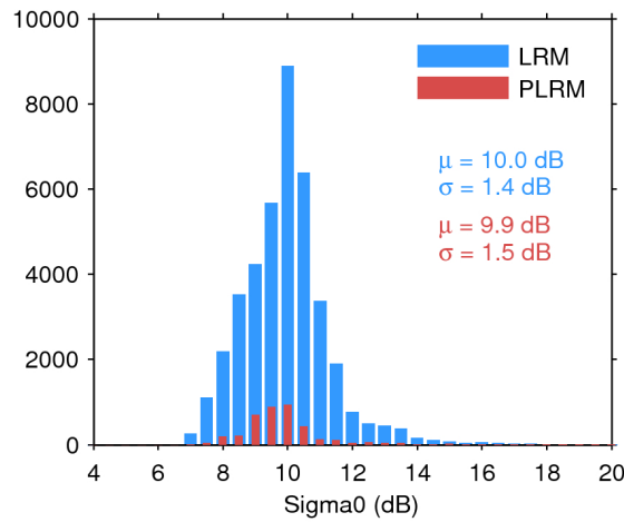
Figure 28. Histogram of science-valid sigma0 over oceans and lakes for LRM (blue) and PLRM (red) for 28/01/2017. The mean ( \mu ) and standard deviation ( \sigma ) are also shown. Note that values outside [4 20] dB are excluded from the histogram for the sake of readability but not from the computation of \mu and \sigma .
