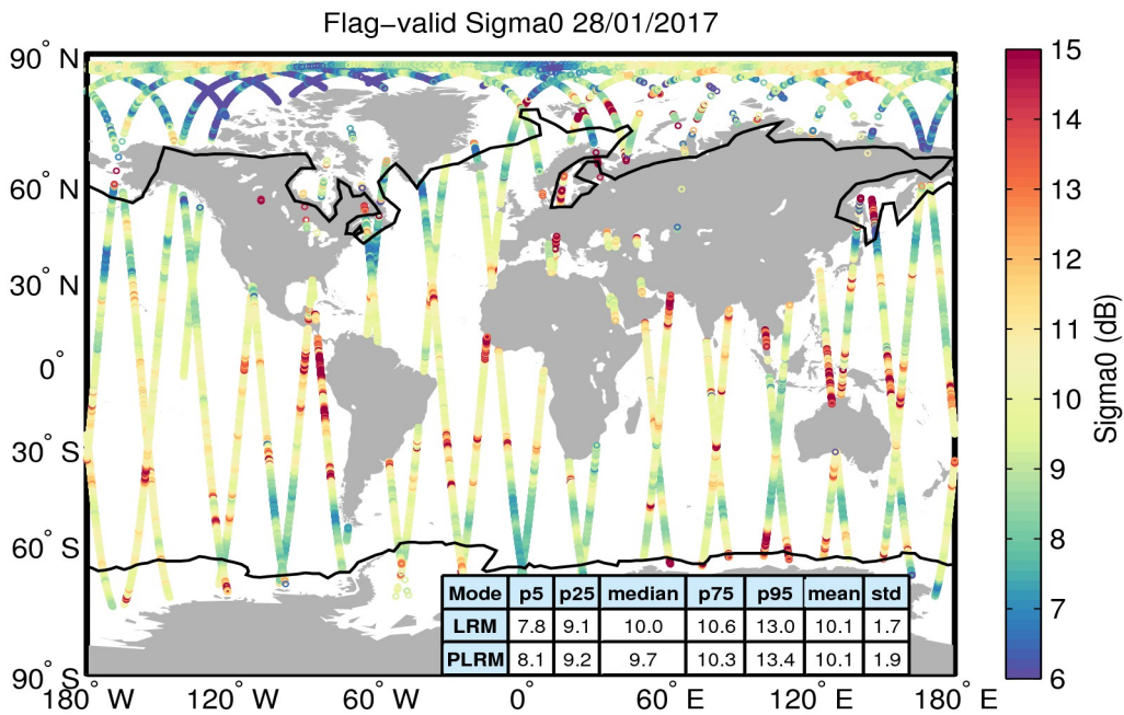
Figure 23. Geographical distribution of flag-valid sigma0 data over oceans and lakes for 28/01/2017. The statistical values shown in the table refer to the sigma0 in dB and are calculated separately for LRM and PLRM regions. Measurements taken over polar polygons have been excluded from the computation of the statistical values. The black lines mark the outer limit of the Arctic and Antarctic polar polygons.
