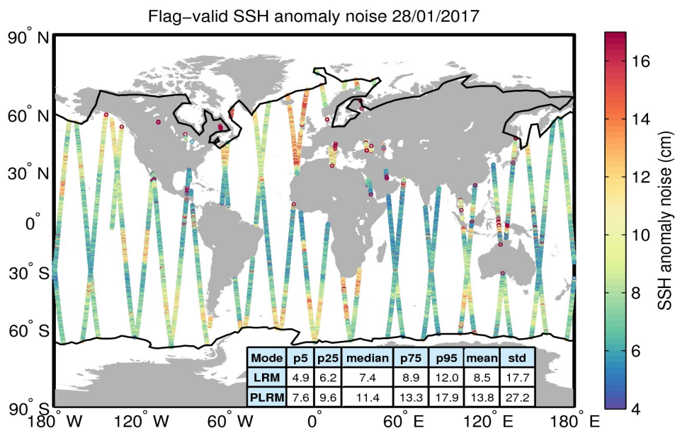
Figure 8. Geographical distribution of flag-valid 20-Hz SSH anomaly measurement noise over oceans and lakes for 28/01/2017. The statistical values shown in the table refer to the SSH anomaly noise and are calculated separately for LRM and PLRM regions. Measurements taken over polar polygons have been excluded from the computation of the statistical values. The black lines mark the outer limit of the Arctic and Antarctic polar polygons.
