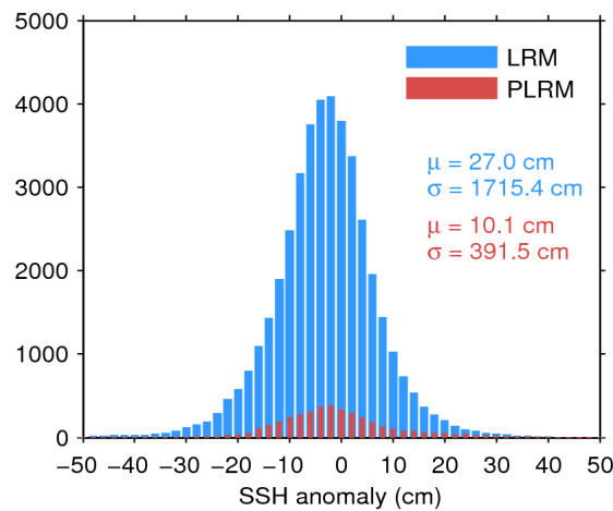
Figure 7. Histogram of flag-valid SSH anomaly over oceans and lakes for LRM (blue) and PLRM (red) for 28/01/2017. The mean ( \mu ) and standard deviation ( \sigma ) are also shown. Note that values outside [-50\ 50] cm are excluded from the histogram for the sake of readability but not from the computation of \mu and \sigma .
