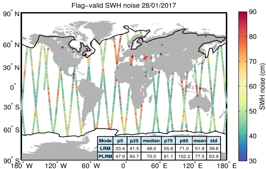
Figure 18. Geographical distribution of flag-valid 20-Hz SWH measurement noise over oceans and lakes for 28/01/2017. The statistical values shown in the table refer to the SWH noise and are calculated separately for LRM and PLRM regions. Measurements taken over polar polygons have been excluded from the computation of the statistical values. The black lines mark the outer limit of the Arctic and Antarctic polar polygons.
