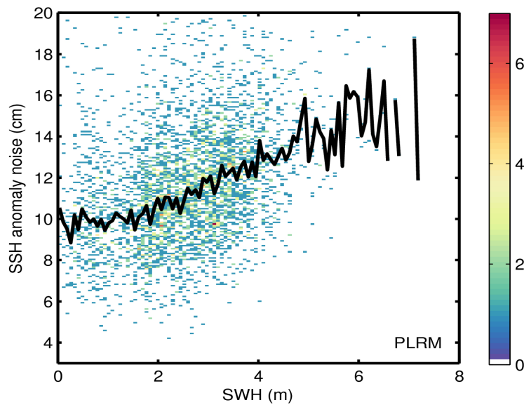
Figure 9. 2D histogram showing flag-valid SSH anomaly noise as a function of SWH for LRM (top) and PLRM (bottom) for 28/01/2017. The black line denotes the median SSH anomaly noise as a function of SWH.
