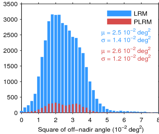
Figure 39. Histogram of flag-valid mispointing over oceans and lakes for LRM (blue) and PLRM (red) for 28/01/2017. Only positive values have been considered. The mean ( \mu ) and standard deviation ( \sigma ) are also shown. Note that values larger than 8 \cdot 10^{-2} \text{ deg}^2 are excluded from the histogram for the sake of readability but not from the computation of \mu and \sigma .
