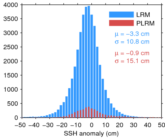
Figure 11. Histogram of science-valid SSH anomaly over oceans and lakes for LRM (blue) and PLRM (red) for 28/01/2017. The mean ( \mu ) and standard deviation ( \sigma ) are also shown. Note that values outside [-50 50] cm are excluded from the histogram for the sake of readability but not from the computation of \mu and \sigma .
