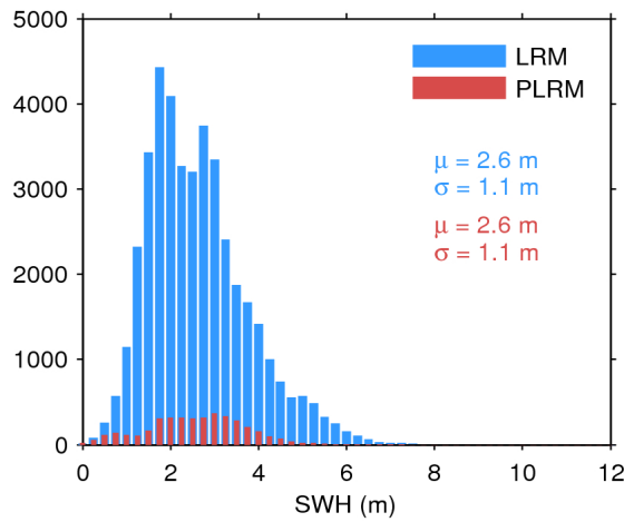
Figure 20. Histogram of science-valid SWH over oceans and lakes for LRM (blue) and PLRM (red) for 28/01/2017. The mean ( \mu ) and standard deviation ( \sigma ) are also shown. Note that values larger than 12 m are excluded from the histogram for the sake of readability but not from the computation of \mu and \sigma .
