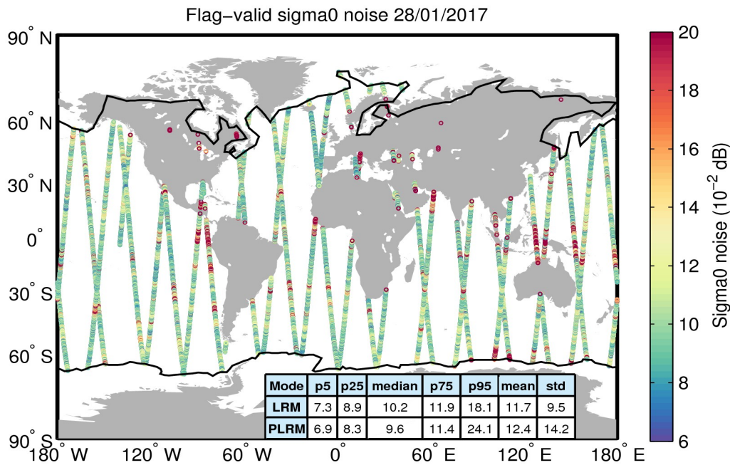
Figure 26. Geographical distribution of flag-valid 20-Hz sigma0 measurement noise over oceans and lakes for 28/01/2017. The statistical values shown in the table refer to the sigma0 noise and are calculated separately for LRM and PLRM regions. Measurements taken over polar polygons have been excluded from the computation of the statistical values. The black lines mark the outer limit of the Arctic and Antarctic polar polygons.
