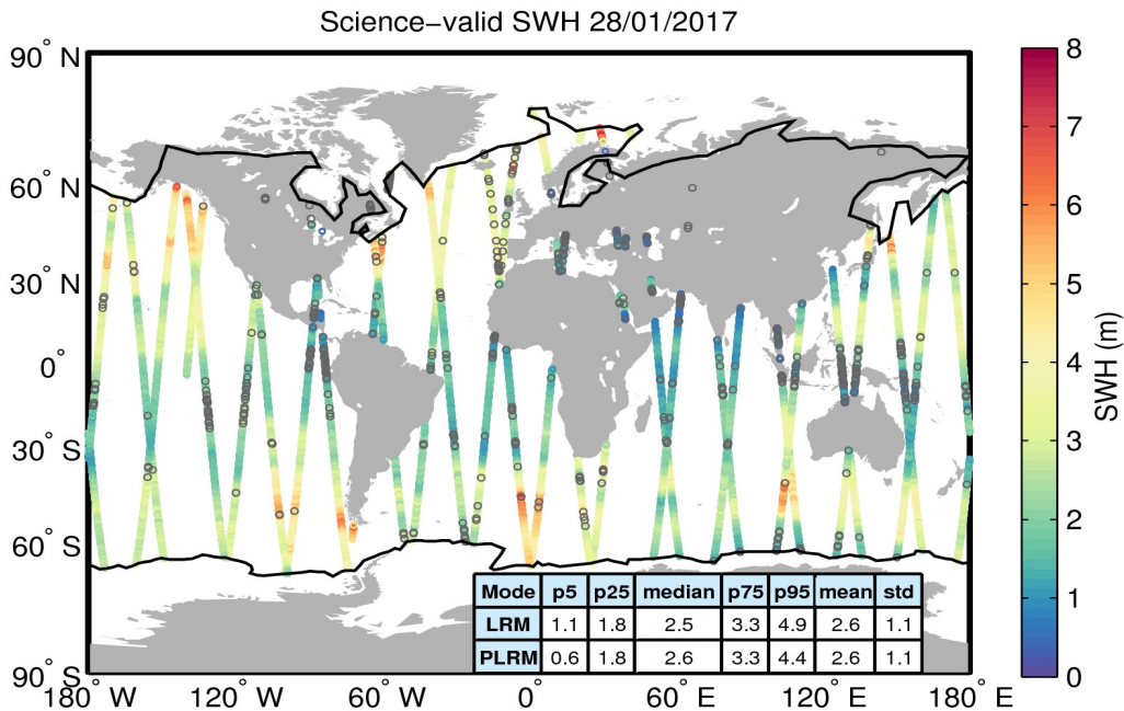
Figure 19. Geographical distribution of science-valid SWH data over oceans and lakes for 28/01/2017. The statistical values shown in the table refer to the SWH in m and are calculated separately for LRM and PLRM regions. The black lines mark the outer limit of the Arctic and Antarctic polar polygons. Gray circles denote records that have been rejected based on the editing criteria described in Table 3.
