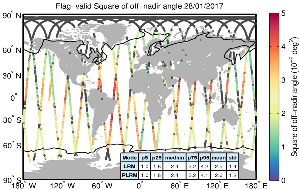
Figure 37. Geographical distribution of flag-valid mispointing data over oceans and lakes for 28/01/2017. The statistical values shown in the table refer to the mispointing in 10^{-2} deg 2 and are calculated separately for LRM and PLRM regions. Measurements taken over polar polygons have been excluded from the computation of the statistical values. The black lines mark the outer limit of the Arctic and Antarctic polar polygons. Gray circles denote negative values.
