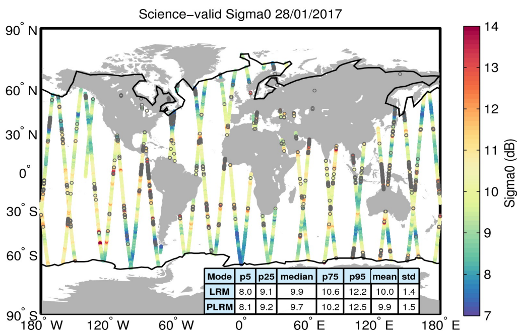
Figure 27. Geographical distribution of science-valid sigma0 data over oceans and lakes for 28/01/2017. The statistical values shown in the table refer to the sigma0 in dB and are calculated separately for LRM and PLRM regions. The black lines mark the outer limit of the Arctic and Antarctic polar polygons. Gray circles denote records that have been rejected based on the editing criteria described in Table 4.
