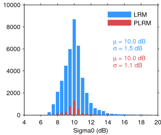
Figure 28. Histogram of science-valid sigma0 over oceans and lakes for LRM (blue) and PLRM (red) for 27/01/2017. The mean ( \mu ) and standard deviation ( \sigma ) are also shown. Note that values outside [4 20] dB are excluded from the histogram for the sake of readability but not from the computation of \mu and \sigma .
