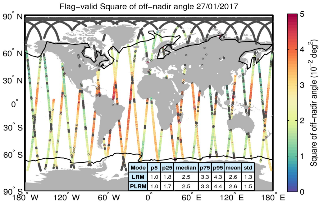
Figure 37. Geographical distribution of flag-valid mispointing data over oceans and lakes for 27/01/2017. The statistical values shown in the table refer to the mispointing in 10^{-2} deg 2 and are calculated separately for LRM and PLRM regions. Measurements taken over polar polygons have been excluded from the computation of the statistical values. The black lines mark the outer limit of the Arctic and Antarctic polar polygons. Gray circles denote negative values.
