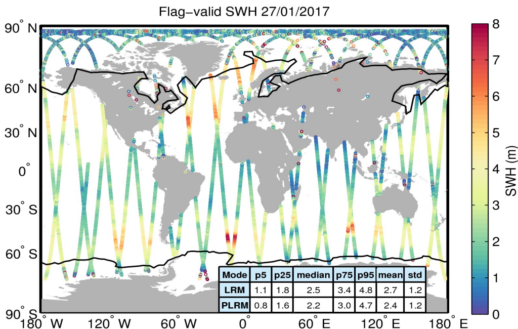
Figure 15. Geographical distribution of flag-valid SWH data over oceans and lakes for 27/01/2017. The statistical values shown in the table refer to the SWH in m and are calculated separately for LRM and PLRM regions. Measurements taken over polar polygons have been excluded from the computation of the statistical values. The black lines mark the outer limit of the Arctic and Antarctic polar polygons.
