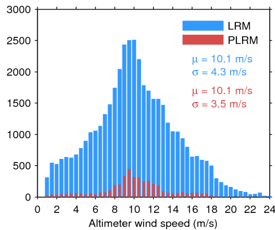
Figure 33. Histogram of flag-valid wind over oceans and lakes for LRM (blue) and PLRM (red) for 27/01/2017. The mean ( \mu ) and standard deviation ( \sigma ) are also shown. Note that values larger than 24 m/s are excluded from the histogram for the sake of readability but not from the computation of \mu and \sigma .
