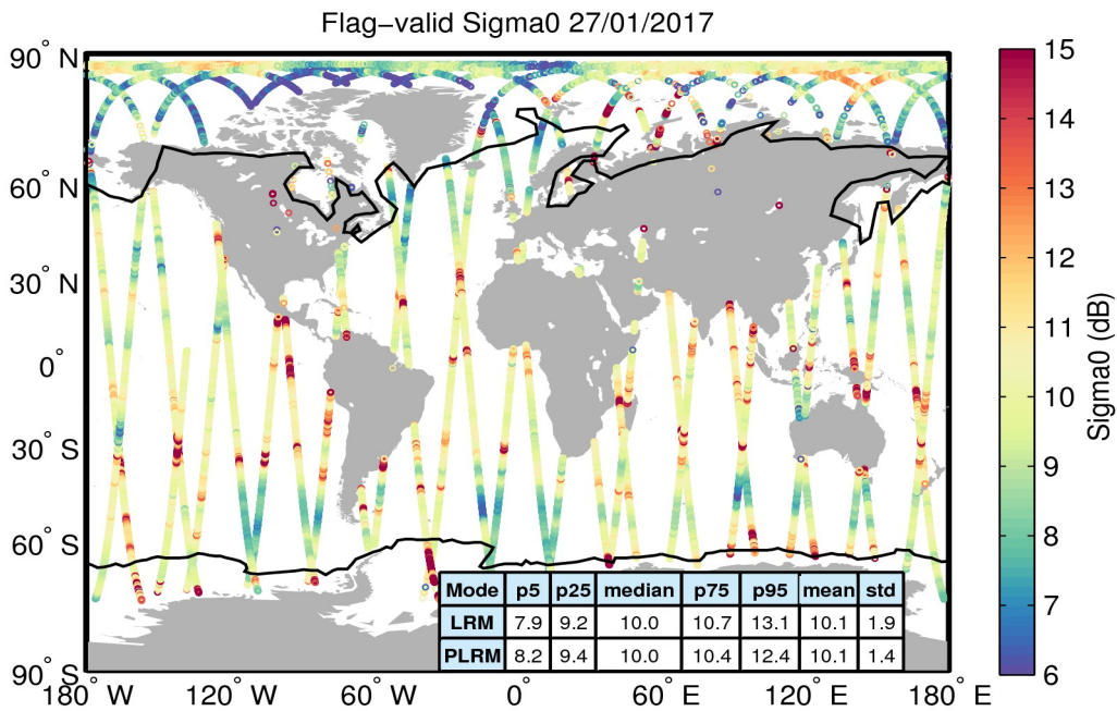
Figure 23. Geographical distribution of flag-valid sigma0 data over oceans and lakes for 27/01/2017. The statistical values shown in the table refer to the sigma0 in dB and are calculated separately for LRM and PLRM regions. Measurements taken over polar polygons have been excluded from the computation of the statistical values. The black lines mark the outer limit of the Arctic and Antarctic polar polygons.
