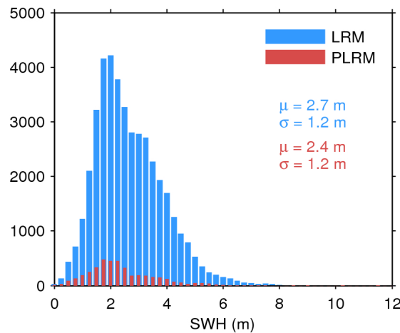
Figure 17. Histogram of flag-valid SWH over oceans and lakes for LRM (blue) and PLRM (red) for 27/01/2017. The mean ( \mu ) and standard deviation ( \sigma ) are also shown. Note that values larger than 12 m are excluded from the histogram for the sake of readability but not from the computation of \mu and \sigma .
