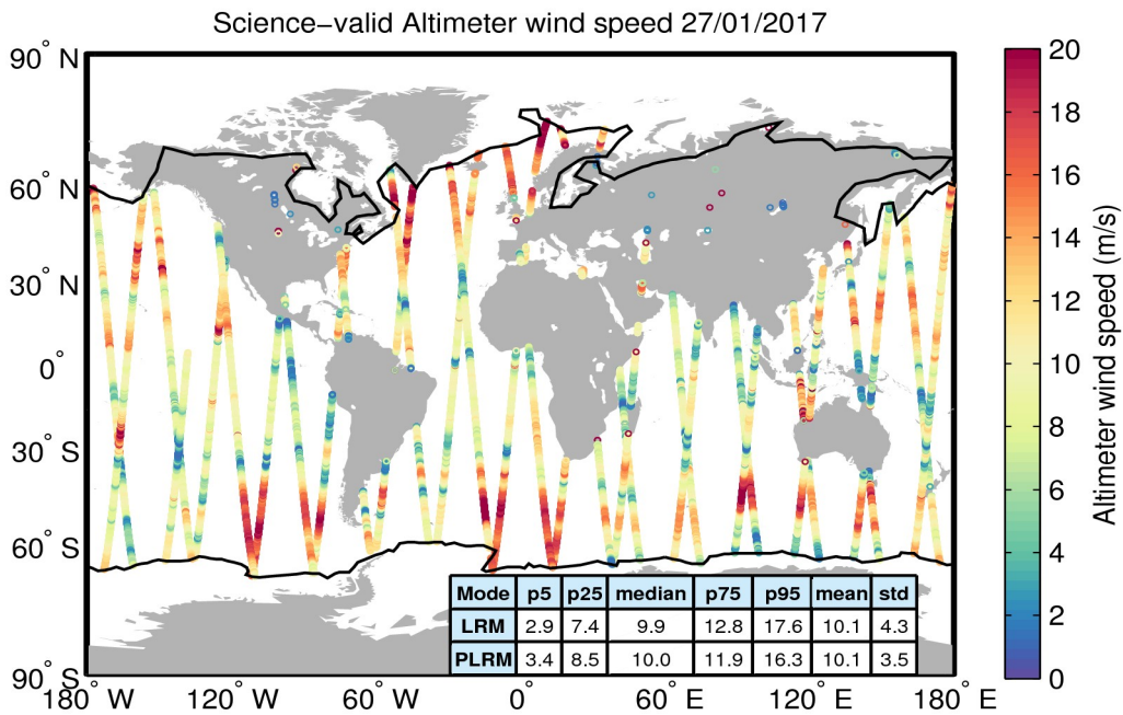
Figure 34. Geographical distribution of science-valid wind data over oceans and lakes for 27/01/2017. The statistical values shown in the table refer to the wind in m/s and are calculated separately for LRM and PLRM regions. The black lines mark the outer limit of the Arctic and Antarctic polar polygons. Gray circles denote records that have been rejected based on the editing criteria described in Table 5.
