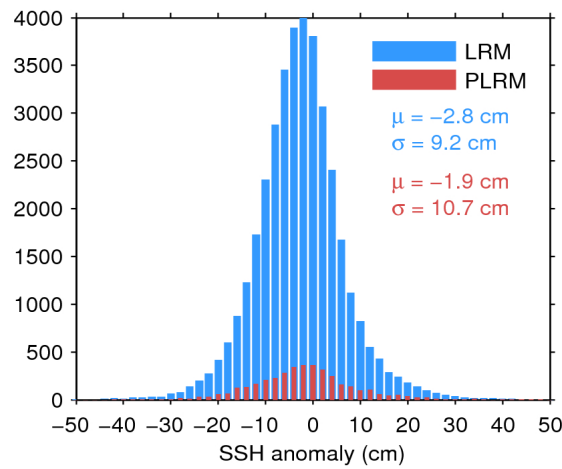
Figure 11. Histogram of science-valid SSH anomaly over oceans and lakes for LRM (blue) and PLRM (red) for 27/01/2017. The mean ( \mu ) and standard deviation ( \sigma ) are also shown. Note that values outside [-50 50] cm are excluded from the histogram for the sake of readability but not from the computation of \mu and \sigma .
