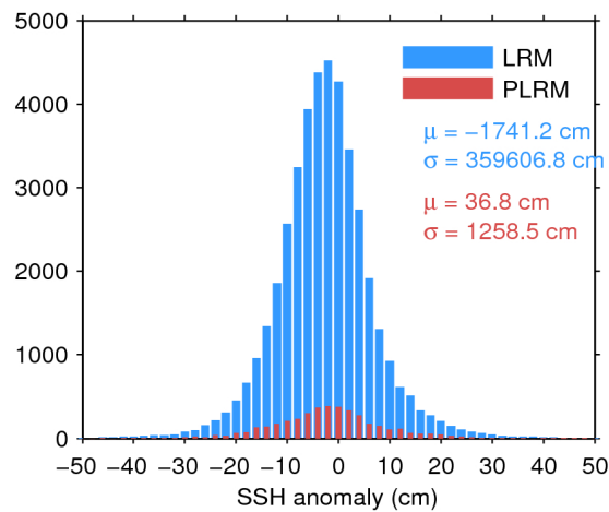
Figure 7. Histogram of flag-valid SSH anomaly over oceans and lakes for LRM (blue) and PLRM (red) for 27/01/2017. The mean ( \mu ) and standard deviation ( \sigma ) are also shown. Note that values outside [-50 \ 50] cm are excluded from the histogram for the sake of readability but not from the computation of \mu and \sigma .
