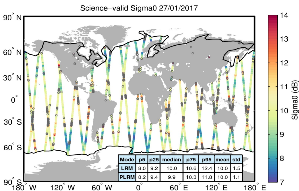
Figure 27. Geographical distribution of science-valid sigma0 data over oceans and lakes for 27/01/2017. The statistical values shown in the table refer to the sigma0 in dB and are calculated separately for LRM and PLRM regions. The black lines mark the outer limit of the Arctic and Antarctic polar polygons. Gray circles denote records that have been rejected based on the editing criteria described in Table 4.
