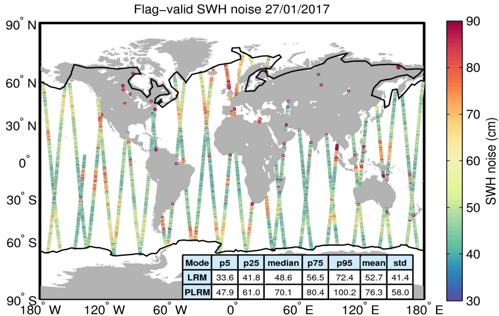
Figure 18. Geographical distribution of flag-valid 20-Hz SWH measurement noise over oceans and lakes for 27/01/2017. The statistical values shown in the table refer to the SWH noise and are calculated separately for LRM and PLRM regions. Measurements taken over polar polygons have been excluded from the computation of the statistical values. The black lines mark the outer limit of the Arctic and Antarctic polar polygons.
