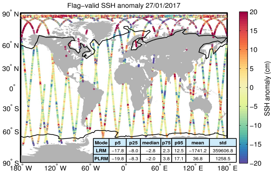
Figure 5. Geographical distribution of flag-valid 1-Hz SSH anomaly data over oceans and lakes for 27/01/2017. The statistical values shown in the table refer to the SSH anomaly in cm and are calculated separately for LRM and PLRM regions. Measurements taken over polar polygons have been excluded from the computation of the statistical values. The black lines mark the outer limit of the Arctic and Antarctic polar polygons.
