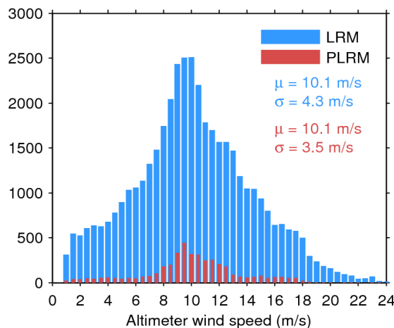
Figure 35. Histogram of science-valid wind over oceans and lakes for LRM (blue) and PLRM (red) for 27/01/2017. The mean ( \mu ) and standard deviation ( \sigma ) are also shown. Note that values larger than 24 m/s are excluded from the histogram for the sake of readability but not from the computation of \mu and \sigma .
