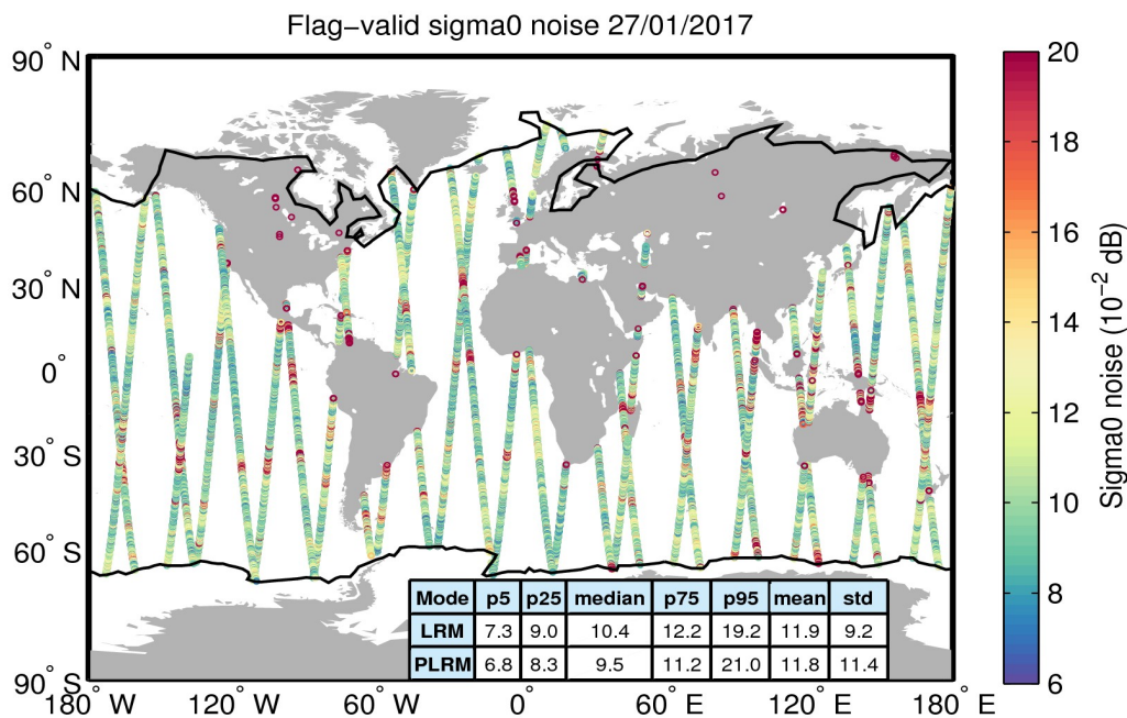
Figure 26. Geographical distribution of flag-valid 20-Hz sigma0 measurement noise over oceans and lakes for 27/01/2017. The statistical values shown in the table refer to the sigma0 noise and are calculated separately for LRM and PLRM regions. Measurements taken over polar polygons have been excluded from the computation of the statistical values. The black lines mark the outer limit of the Arctic and Antarctic polar polygons.
