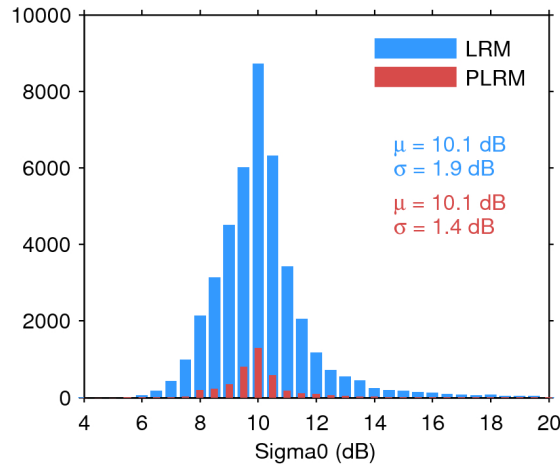
Figure 25. Histogram of flag-valid sigma0 over oceans and lakes for LRM (blue) and PLRM (red) for 27/01/2017. The mean ( \mu ) and standard deviation ( \sigma ) are also shown. Note that values outside [4 20] dB are excluded from the histogram for the sake of readability but not from the computation of \mu and \sigma .
