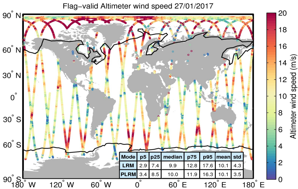
Figure 31. Geographical distribution of flag-valid wind data over oceans and lakes for 27/01/2017. The statistical values shown in the table refer to the wind in m/s and are calculated separately for LRM and PLRM regions. Measurements taken over polar polygons have been excluded from the computation of the statistical values. The black lines mark the outer limit of the Arctic and Antarctic polar polygons.
