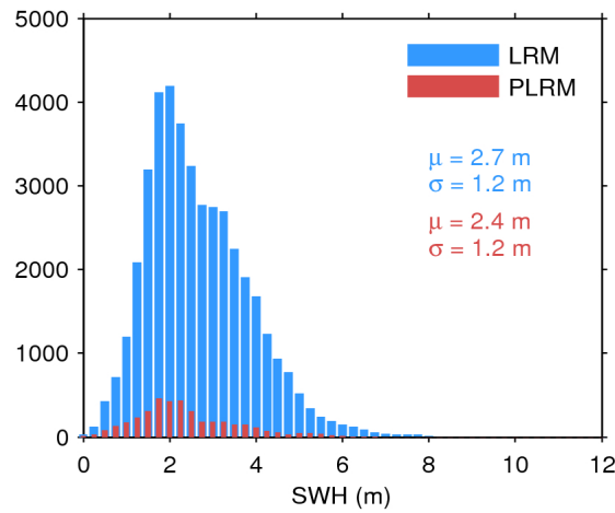
Figure 20. Histogram of science-valid SWH over oceans and lakes for LRM (blue) and PLRM (red) for 27/01/2017. The mean ( \mu ) and standard deviation ( \sigma ) are also shown. Note that values larger than 12 m are excluded from the histogram for the sake of readability but not from the computation of \mu and \sigma .
