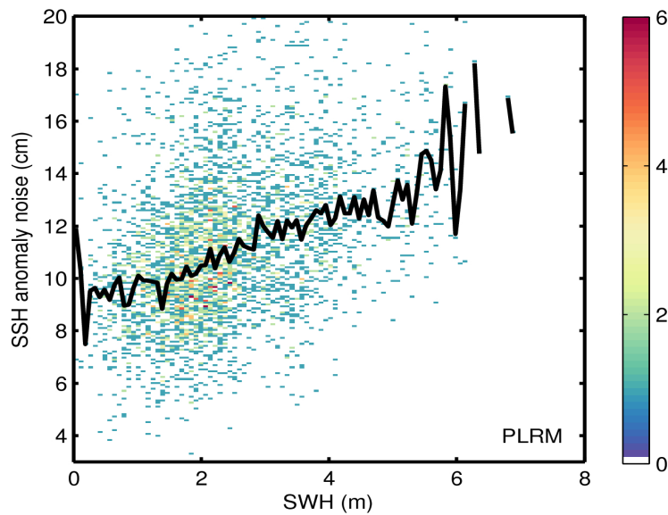
Figure 9. 2D histogram showing flag-valid SSH anomaly noise as a function of SWH for LRM (top) and PLRM (bottom) for 27/01/2017. The black line denotes the median SSH anomaly noise as a function of SWH.
