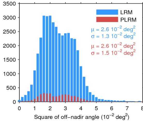
Figure 39. Histogram of flag-valid mispointing over oceans and lakes for LRM (blue) and PLRM (red) for 27/01/2017. Only positive values have been considered. The mean ( \mu ) and standard deviation ( \sigma ) are also shown. Note that values larger than 8 \cdot 10^{-2} \text{ deg}^2 are excluded from the histogram for the sake of readability but not from the computation of \mu and \sigma .
