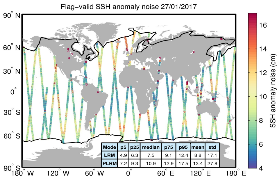
Figure 8. Geographical distribution of flag-valid 20-Hz SSH anomaly measurement noise over oceans and lakes for 27/01/2017. The statistical values shown in the table refer to the SSH anomaly noise and are calculated separately for LRM and PLRM regions. Measurements taken over polar polygons have been excluded from the computation of the statistical values. The black lines mark the outer limit of the Arctic and Antarctic polar polygons.
