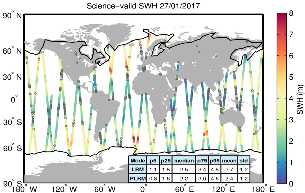
Figure 19. Geographical distribution of science-valid SWH data over oceans and lakes for 27/01/2017. The statistical values shown in the table refer to the SWH in m and are calculated separately for LRM and PLRM regions. The black lines mark the outer limit of the Arctic and Antarctic polar polygons. Gray circles denote records that have been rejected based on the editing criteria described in Table 3.
