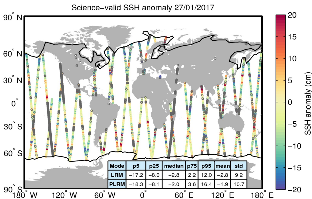
Figure 10. Geographical distribution of science-valid SSH anomaly data over oceans and lakes for 27/01/2017. The statistical values shown in the table refer to the SSH anomaly in cm and are calculated separately for LRM and PLRM regions. The black lines mark the outer limit of the Arctic and Antarctic polar polygons. Gray circles denote records that have been rejected based on the editing criteria described in Table 2.
