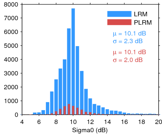
Figure 25. Histogram of flag-valid sigma0 over oceans and lakes for LRM (blue) and PLRM (red) for 24/01/2017. The mean ( \mu ) and standard deviation ( \sigma ) are also shown. Note that values outside [4 20] dB are excluded from the histogram for the sake of readability but not from the computation of \mu and \sigma .
