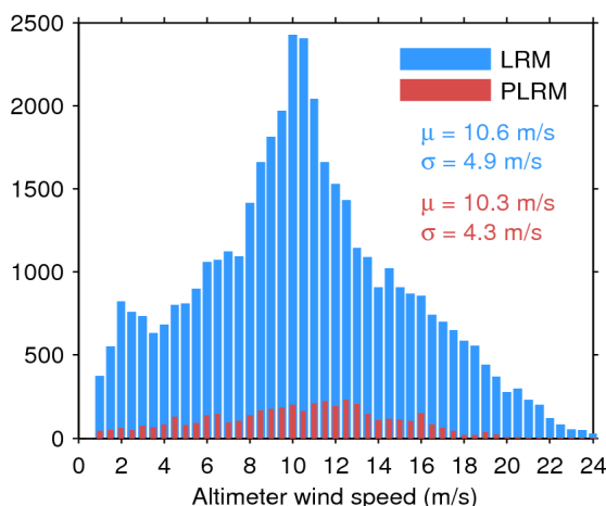
Figure 33. Histogram of flag-valid wind over oceans and lakes for LRM (blue) and PLRM (red) for 24/01/2017. The mean ( \mu ) and standard deviation ( \sigma ) are also shown. Note that values larger than 24 m/s are excluded from the histogram for the sake of readability but not from the computation of \mu and \sigma .
