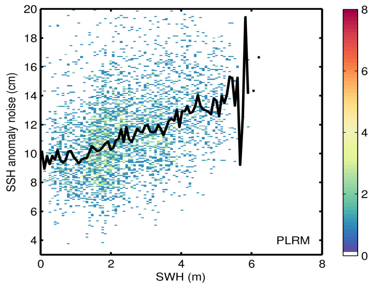
Figure 9. 2D histogram showing flag-valid SSH anomaly noise as a function of SWH for LRM (top) and PLRM (bottom) for 24/01/2017. The black line denotes the median SSH anomaly noise as a function of SWH.
