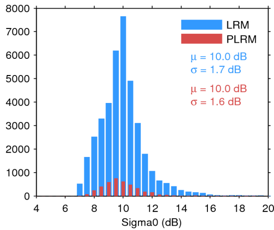
Figure 28. Histogram of science-valid sigma0 over oceans and lakes for LRM (blue) and PLRM (red) for 24/01/2017. The mean ( \mu ) and standard deviation ( \sigma ) are also shown. Note that values outside [4 20] dB are excluded from the histogram for the sake of readability but not from the computation of \mu and \sigma .
