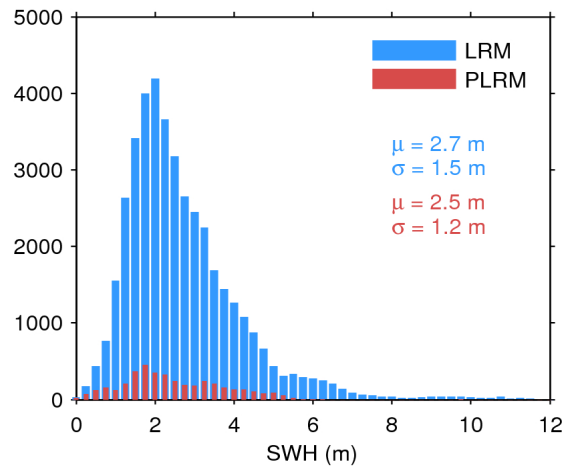
Figure 20. Histogram of science-valid SWH over oceans and lakes for LRM (blue) and PLRM (red) for 24/01/2017. The mean ( \mu ) and standard deviation ( \sigma ) are also shown. Note that values larger than 12 m are excluded from the histogram for the sake of readability but not from the computation of \mu and \sigma .
