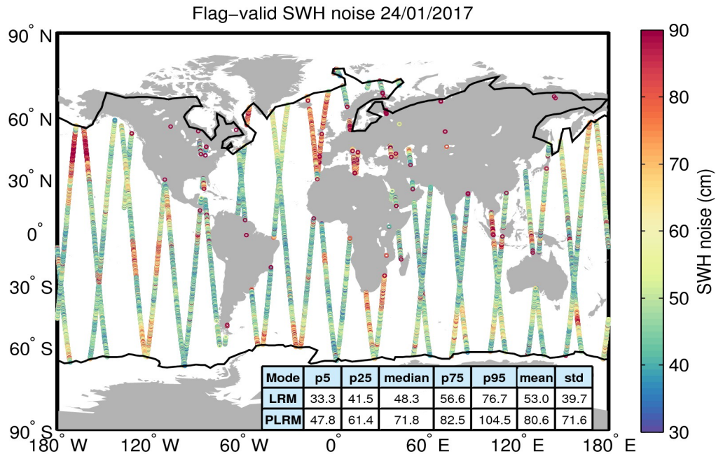
Figure 18. Geographical distribution of flag-valid 20-Hz SWH measurement noise over oceans and lakes for 24/01/2017. The statistical values shown in the table refer to the SWH noise and are calculated separately for LRM and PLRM regions. Measurements taken over polar polygons have been excluded from the computation of the statistical values. The black lines mark the outer limit of the Arctic and Antarctic polar polygons.
