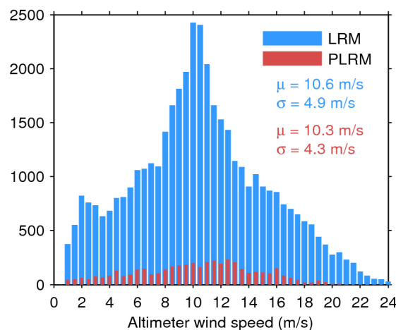
Figure 35. Histogram of science-valid wind over oceans and lakes for LRM (blue) and PLRM (red) for 24/01/2017. The mean ( \mu ) and standard deviation ( \sigma ) are also shown. Note that values larger than 24 m/s are excluded from the histogram for the sake of readability but not from the computation of \mu and \sigma .
