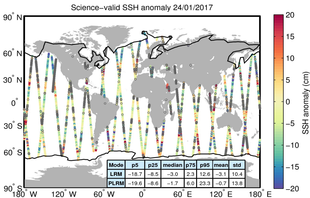
Figure 10. Geographical distribution of science-valid SSH anomaly data over oceans and lakes for 24/01/2017. The statistical values shown in the table refer to the SSH anomaly in cm and are calculated separately for LRM and PLRM regions. The black lines mark the outer limit of the Arctic and Antarctic polar polygons. Gray circles denote records that have been rejected based on the editing criteria described in Table 2.
