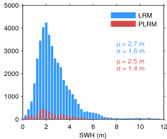
Figure 17. Histogram of flag-valid SWH over oceans and lakes for LRM (blue) and PLRM (red) for 24/01/2017. The mean ( \mu ) and standard deviation ( \sigma ) are also shown. Note that values larger than 12 m are excluded from the histogram for the sake of readability but not from the computation of \mu and \sigma .
