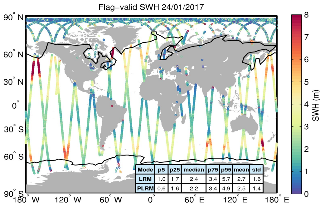
Figure 15. Geographical distribution of flag-valid SWH data over oceans and lakes for 24/01/2017. The statistical values shown in the table refer to the SWH in m and are calculated separately for LRM and PLRM regions. Measurements taken over polar polygons have been excluded from the computation of the statistical values. The black lines mark the outer limit of the Arctic and Antarctic polar polygons.
