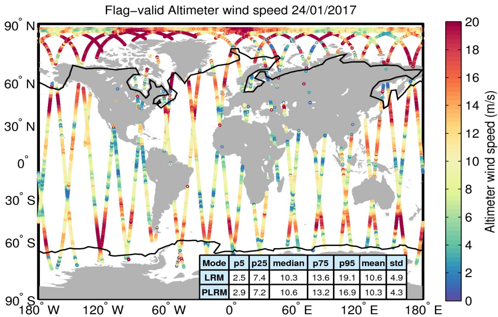
Figure 31. Geographical distribution of flag-valid wind data over oceans and lakes for 24/01/2017. The statistical values shown in the table refer to the wind in m/s and are calculated separately for LRM and PLRM regions. Measurements taken over polar polygons have been excluded from the computation of the statistical values. The black lines mark the outer limit of the Arctic and Antarctic polar polygons.
