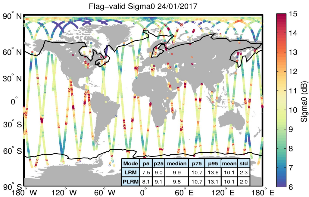
Figure 23. Geographical distribution of flag-valid sigma0 data over oceans and lakes for 24/01/2017. The statistical values shown in the table refer to the sigma0 in dB and are calculated separately for LRM and PLRM regions. Measurements taken over polar polygons have been excluded from the computation of the statistical values. The black lines mark the outer limit of the Arctic and Antarctic polar polygons.
