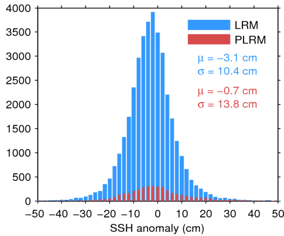
Figure 11. Histogram of science-valid SSH anomaly over oceans and lakes for LRM (blue) and PLRM (red) for 24/01/2017. The mean ( \mu ) and standard deviation ( \sigma ) are also shown. Note that values outside [-50 50] cm are excluded from the histogram for the sake of readability but not from the computation of \mu and \sigma .
