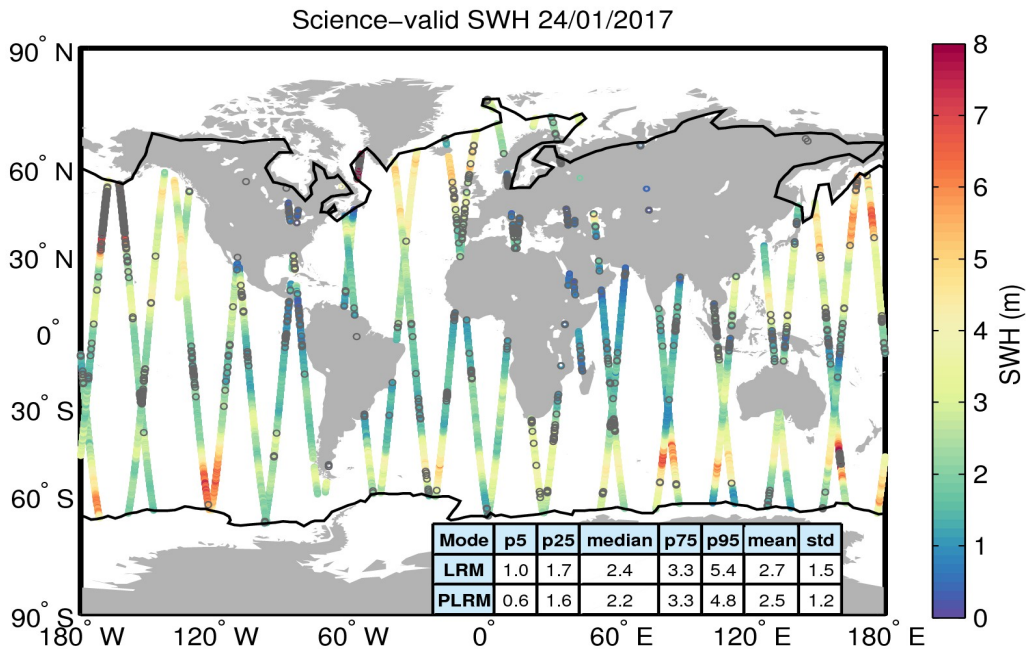
Figure 19. Geographical distribution of science-valid SWH data over oceans and lakes for 24/01/2017. The statistical values shown in the table refer to the SWH in m and are calculated separately for LRM and PLRM regions. The black lines mark the outer limit of the Arctic and Antarctic polar polygons. Gray circles denote records that have been rejected based on the editing criteria described in Table 3.
