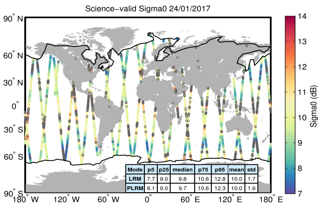
Figure 27. Geographical distribution of science-valid sigma0 data over oceans and lakes for 24/01/2017. The statistical values shown in the table refer to the sigma0 in dB and are calculated separately for LRM and PLRM regions. The black lines mark the outer limit of the Arctic and Antarctic polar polygons. Gray circles denote records that have been rejected based on the editing criteria described in Table 4.
