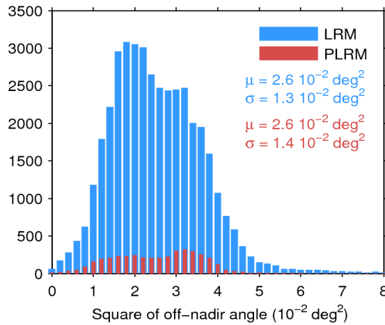
Figure 39. Histogram of flag-valid mispointing over oceans and lakes for LRM (blue) and PLRM (red) for 24/01/2017. Only positive values have been considered. The mean ( \mu ) and standard deviation ( \sigma ) are also shown. Note that values larger than 8 \cdot 10^{-2} \text{ deg}^2 are excluded from the histogram for the sake of readability but not from the computation of \mu and \sigma .
