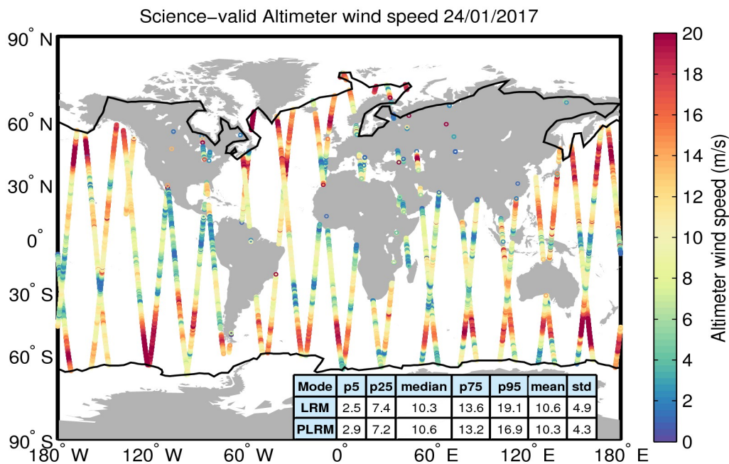
Figure 34. Geographical distribution of science-valid wind data over oceans and lakes for 24/01/2017. The statistical values shown in the table refer to the wind in m/s and are calculated separately for LRM and PLRM regions. The black lines mark the outer limit of the Arctic and Antarctic polar polygons. Gray circles denote records that have been rejected based on the editing criteria described in Table 5.
