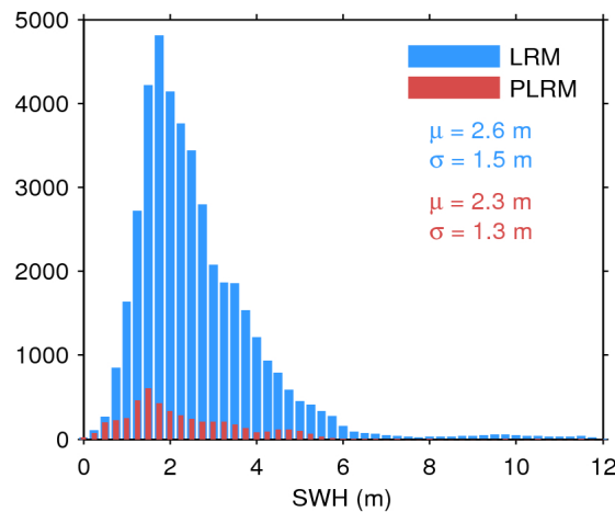
Figure 17. Histogram of flag-valid SWH over oceans and lakes for LRM (blue) and PLRM (red) for 23/01/2017. The mean ( \mu ) and standard deviation ( \sigma ) are also shown. Note that values larger than 12 m are excluded from the histogram for the sake of readability but not from the computation of \mu and \sigma .
