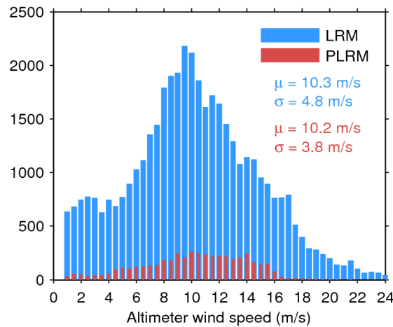
Figure 33. Histogram of flag-valid wind over oceans and lakes for LRM (blue) and PLRM (red) for 23/01/2017. The mean ( \mu ) and standard deviation ( \sigma ) are also shown. Note that values larger than 24 m/s are excluded from the histogram for the sake of readability but not from the computation of \mu and \sigma .
