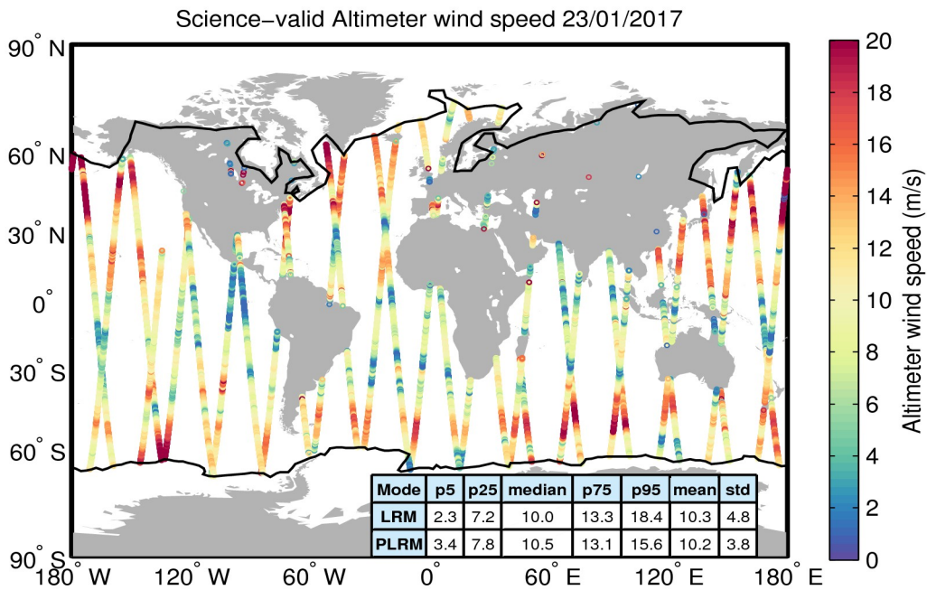
Figure 34. Geographical distribution of science-valid wind data over oceans and lakes for 23/01/2017. The statistical values shown in the table refer to the wind in m/s and are calculated separately for LRM and PLRM regions. The black lines mark the outer limit of the Arctic and Antarctic polar polygons. Gray circles denote records that have been rejected based on the editing criteria described in Table 5.
