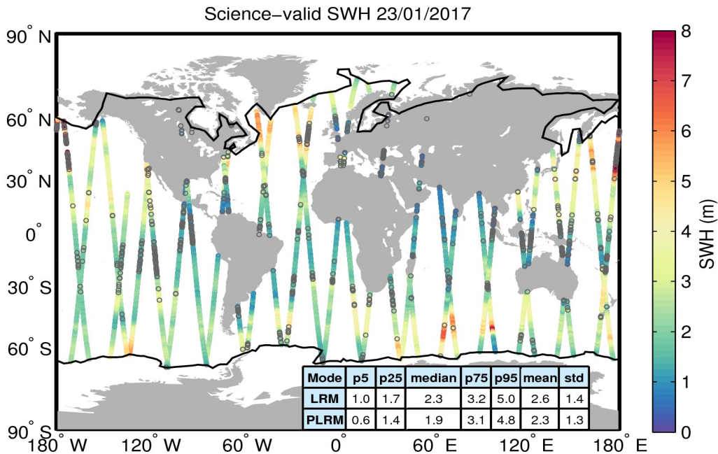
Figure 19. Geographical distribution of science-valid SWH data over oceans and lakes for 23/01/2017. The statistical values shown in the table refer to the SWH in m and are calculated separately for LRM and PLRM regions. The black lines mark the outer limit of the Arctic and Antarctic polar polygons. Gray circles denote records that have been rejected based on the editing criteria described in Table 3.
