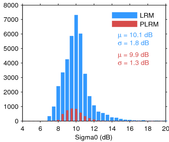
Figure 28. Histogram of science-valid sigma0 over oceans and lakes for LRM (blue) and PLRM (red) for 23/01/2017. The mean ( \mu ) and standard deviation ( \sigma ) are also shown. Note that values outside [4 20] dB are excluded from the histogram for the sake of readability but not from the computation of \mu and \sigma .
