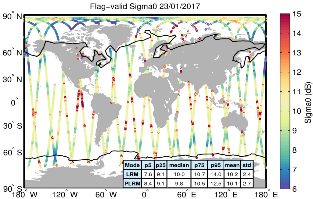
Figure 23. Geographical distribution of flag-valid sigma0 data over oceans and lakes for 23/01/2017. The statistical values shown in the table refer to the sigma0 in dB and are calculated separately for LRM and PLRM regions. Measurements taken over polar polygons have been excluded from the computation of the statistical values. The black lines mark the outer limit of the Arctic and Antarctic polar polygons.
