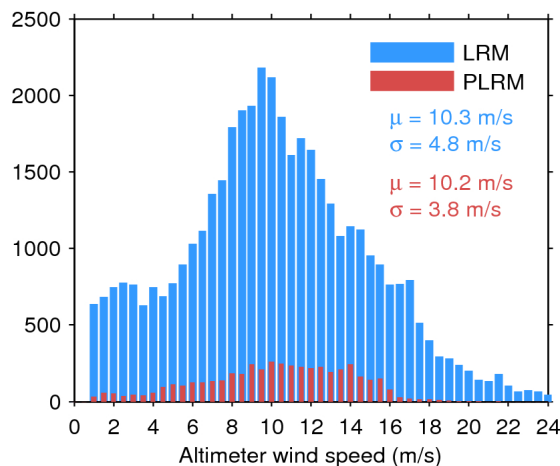
Figure 35. Histogram of science-valid wind over oceans and lakes for LRM (blue) and PLRM (red) for 23/01/2017. The mean ( \mu ) and standard deviation ( \sigma ) are also shown. Note that values larger than 24 m/s are excluded from the histogram for the sake of readability but not from the computation of \mu and \sigma .
