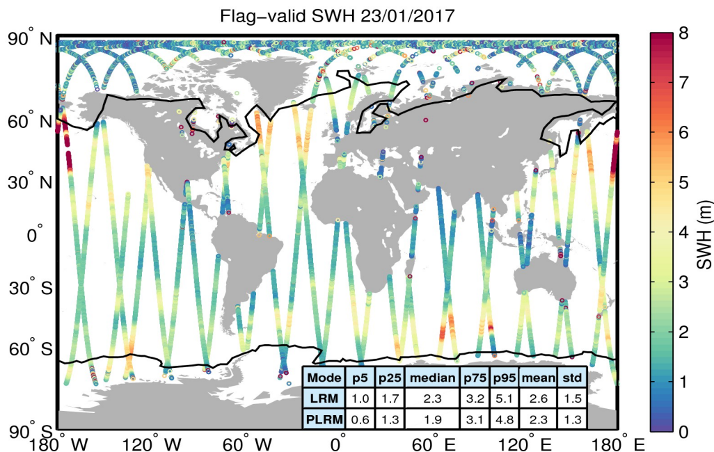
Figure 15. Geographical distribution of flag-valid SWH data over oceans and lakes for 23/01/2017. The statistical values shown in the table refer to the SWH in m and are calculated separately for LRM and PLRM regions. Measurements taken over polar polygons have been excluded from the computation of the statistical values. The black lines mark the outer limit of the Arctic and Antarctic polar polygons.
