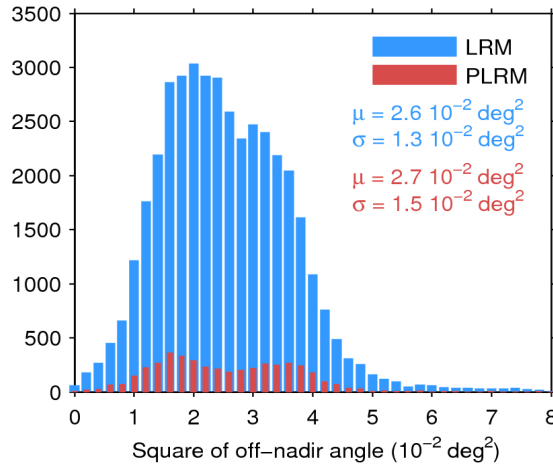
Figure 39. Histogram of flag-valid mispointing over oceans and lakes for LRM (blue) and PLRM (red) for 23/01/2017. Only positive values have been considered. The mean ( \mu ) and standard deviation ( \sigma ) are also shown. Note that values larger than 8 \cdot 10^{-2} \text{ deg}^2 are excluded from the histogram for the sake of readability but not from the computation of \mu and \sigma .
