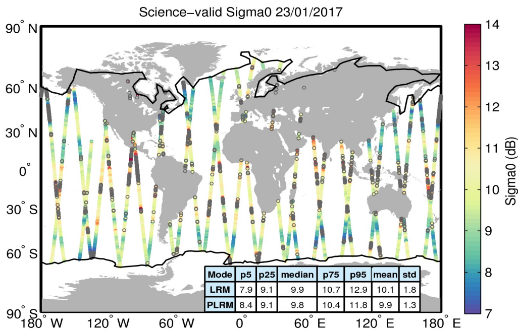
Figure 27. Geographical distribution of science-valid sigma0 data over oceans and lakes for 23/01/2017. The statistical values shown in the table refer to the sigma0 in dB and are calculated separately for LRM and PLRM regions. The black lines mark the outer limit of the Arctic and Antarctic polar polygons. Gray circles denote records that have been rejected based on the editing criteria described in Table 4.
