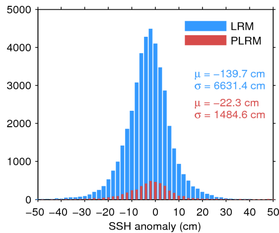
Figure 7. Histogram of flag-valid SSH anomaly over oceans and lakes for LRM (blue) and PLRM (red) for 23/01/2017. The mean ( \mu ) and standard deviation ( \sigma ) are also shown. Note that values outside [-50 50] cm are excluded from the histogram for the sake of readability but not from the computation of \mu and \sigma .
