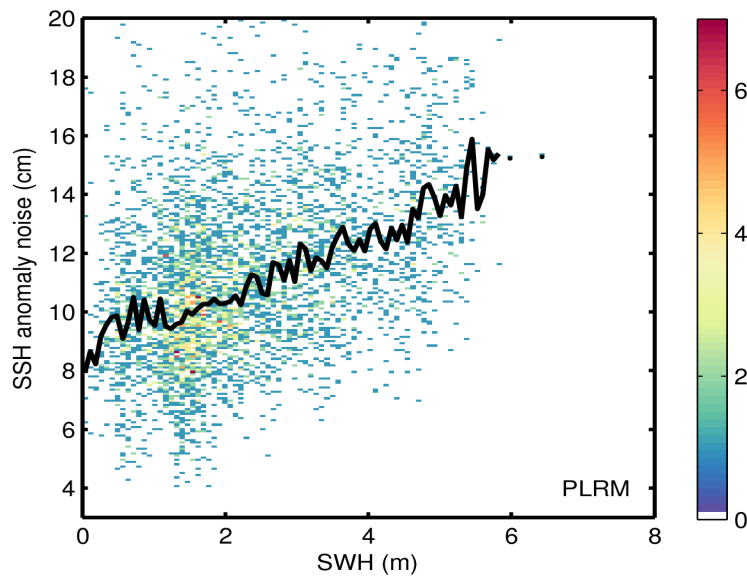
Figure 9. 2D histogram showing flag-valid SSH anomaly noise as a function of SWH for LRM (top) and PLRM (bottom) for 23/01/2017. The black line denotes the median SSH anomaly noise as a function of SWH.
