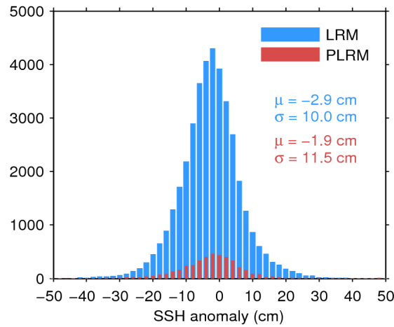
Figure 11. Histogram of science-valid SSH anomaly over oceans and lakes for LRM (blue) and PLRM (red) for 23/01/2017. The mean ( \mu ) and standard deviation ( \sigma ) are also shown. Note that values outside [-50 50] cm are excluded from the histogram for the sake of readability but not from the computation of \mu and \sigma .
