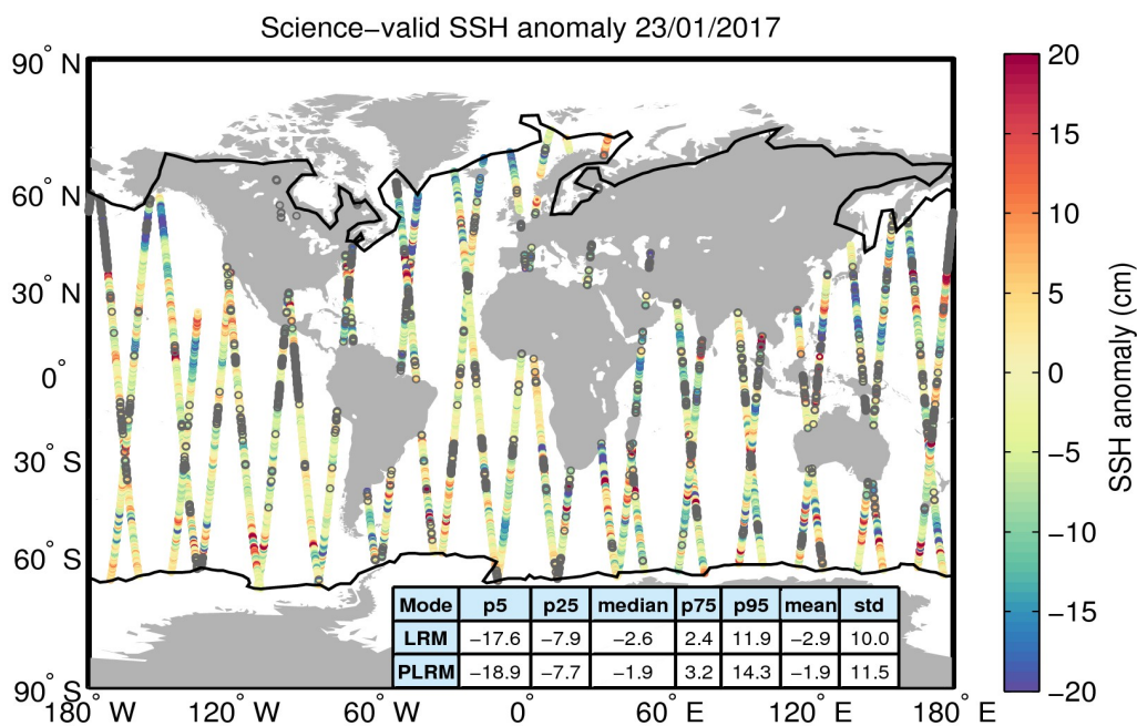
Figure 10. Geographical distribution of science-valid SSH anomaly data over oceans and lakes for 23/01/2017. The statistical values shown in the table refer to the SSH anomaly in cm and are calculated separately for LRM and PLRM regions. The black lines mark the outer limit of the Arctic and Antarctic polar polygons. Gray circles denote records that have been rejected based on the editing criteria described in Table 2.
