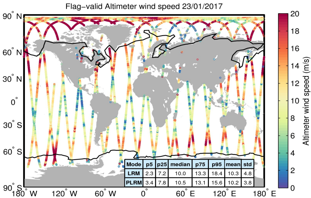
Figure 31. Geographical distribution of flag-valid wind data over oceans and lakes for 23/01/2017. The statistical values shown in the table refer to the wind in m/s and are calculated separately for LRM and PLRM regions. Measurements taken over polar polygons have been excluded from the computation of the statistical values. The black lines mark the outer limit of the Arctic and Antarctic polar polygons.
