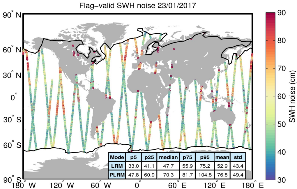
Figure 18. Geographical distribution of flag-valid 20-Hz SWH measurement noise over oceans and lakes for 23/01/2017. The statistical values shown in the table refer to the SWH noise and are calculated separately for LRM and PLRM regions. Measurements taken over polar polygons have been excluded from the computation of the statistical values. The black lines mark the outer limit of the Arctic and Antarctic polar polygons.
