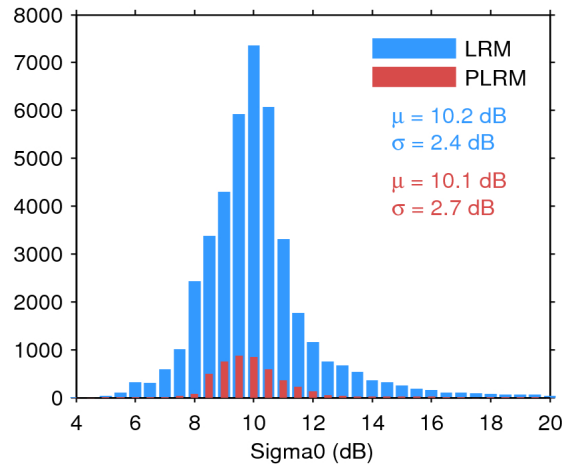
Figure 25. Histogram of flag-valid sigma0 over oceans and lakes for LRM (blue) and PLRM (red) for 23/01/2017. The mean ( \mu ) and standard deviation ( \sigma ) are also shown. Note that values outside [4 20] dB are excluded from the histogram for the sake of readability but not from the computation of \mu and \sigma .
