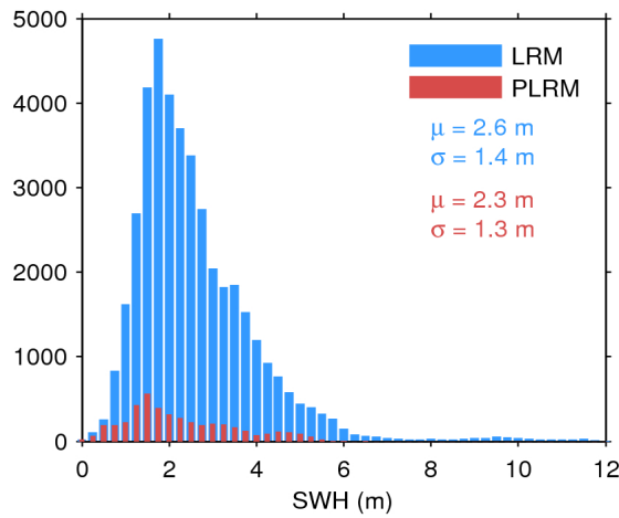
Figure 20. Histogram of science-valid SWH over oceans and lakes for LRM (blue) and PLRM (red) for 23/01/2017. The mean ( \mu ) and standard deviation ( \sigma ) are also shown. Note that values larger than 12 m are excluded from the histogram for the sake of readability but not from the computation of \mu and \sigma .
