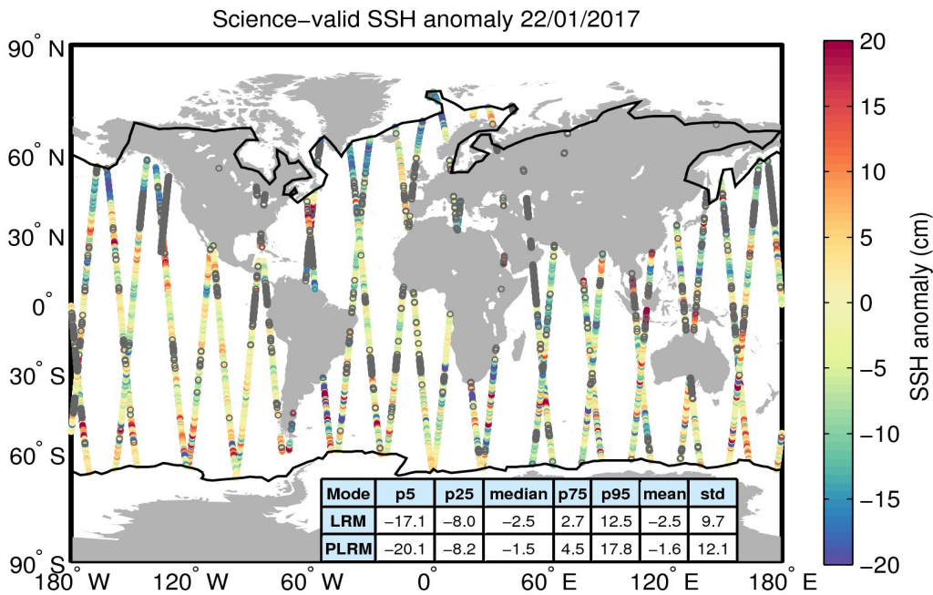
Figure 10. Geographical distribution of science-valid SSH anomaly data over oceans and lakes for 22/01/2017. The statistical values shown in the table refer to the SSH anomaly in cm and are calculated separately for LRM and PLRM regions. The black lines mark the outer limit of the Arctic and Antarctic polar polygons. Gray circles denote records that have been rejected based on the editing criteria described in Table 2.
