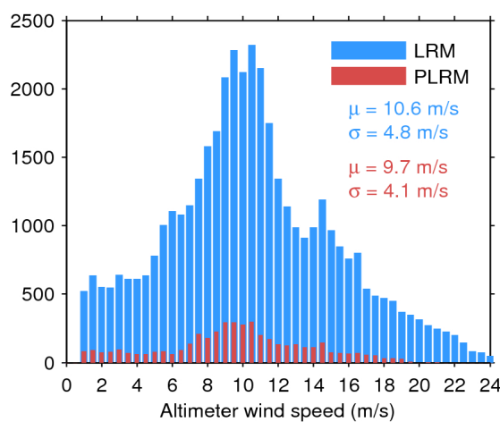
Figure 35. Histogram of science-valid wind over oceans and lakes for LRM (blue) and PLRM (red) for 22/01/2017. The mean ( \mu ) and standard deviation ( \sigma ) are also shown. Note that values larger than 24 m/s are excluded from the histogram for the sake of readability but not from the computation of \mu and \sigma .
