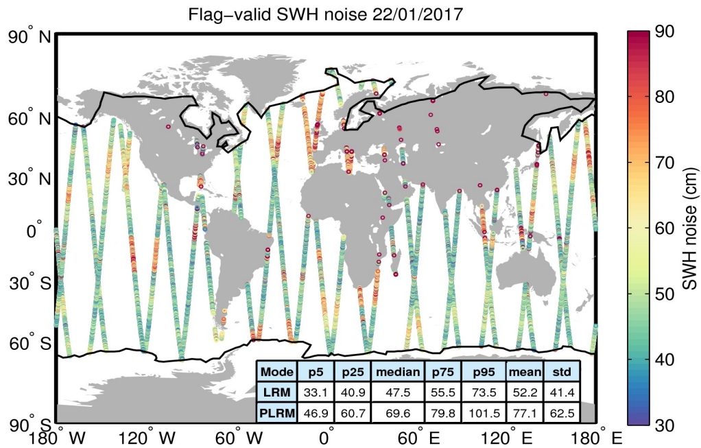
Figure 18. Geographical distribution of flag-valid 20-Hz SWH measurement noise over oceans and lakes for 22/01/2017. The statistical values shown in the table refer to the SWH noise and are calculated separately for LRM and PLRM regions. Measurements taken over polar polygons have been excluded from the computation of the statistical values. The black lines mark the outer limit of the Arctic and Antarctic polar polygons.
