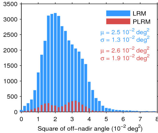
Figure 39. Histogram of flag-valid mispointing over oceans and lakes for LRM (blue) and PLRM (red) for 22/01/2017. Only positive values have been considered. The mean ( \mu ) and standard deviation ( \sigma ) are also shown. Note that values larger than 8 \cdot 10^{-2} \text{ deg}^2 are excluded from the histogram for the sake of readability but not from the computation of \mu and \sigma .
