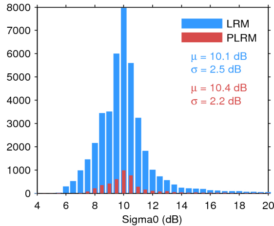
Figure 25. Histogram of flag-valid sigma0 over oceans and lakes for LRM (blue) and PLRM (red) for 22/01/2017. The mean ( \mu ) and standard deviation ( \sigma ) are also shown. Note that values outside [4 20] dB are excluded from the histogram for the sake of readability but not from the computation of \mu and \sigma .
