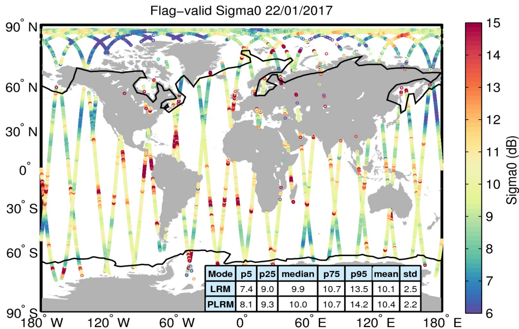
Figure 23. Geographical distribution of flag-valid sigma0 data over oceans and lakes for 22/01/2017. The statistical values shown in the table refer to the sigma0 in dB and are calculated separately for LRM and PLRM regions. Measurements taken over polar polygons have been excluded from the computation of the statistical values. The black lines mark the outer limit of the Arctic and Antarctic polar polygons.
