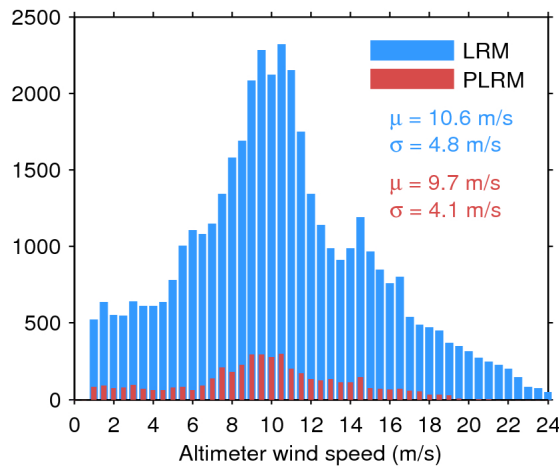
Figure 33. Histogram of flag-valid wind over oceans and lakes for LRM (blue) and PLRM (red) for 22/01/2017. The mean ( \mu ) and standard deviation ( \sigma ) are also shown. Note that values larger than 24 m/s are excluded from the histogram for the sake of readability but not from the computation of \mu and \sigma .
