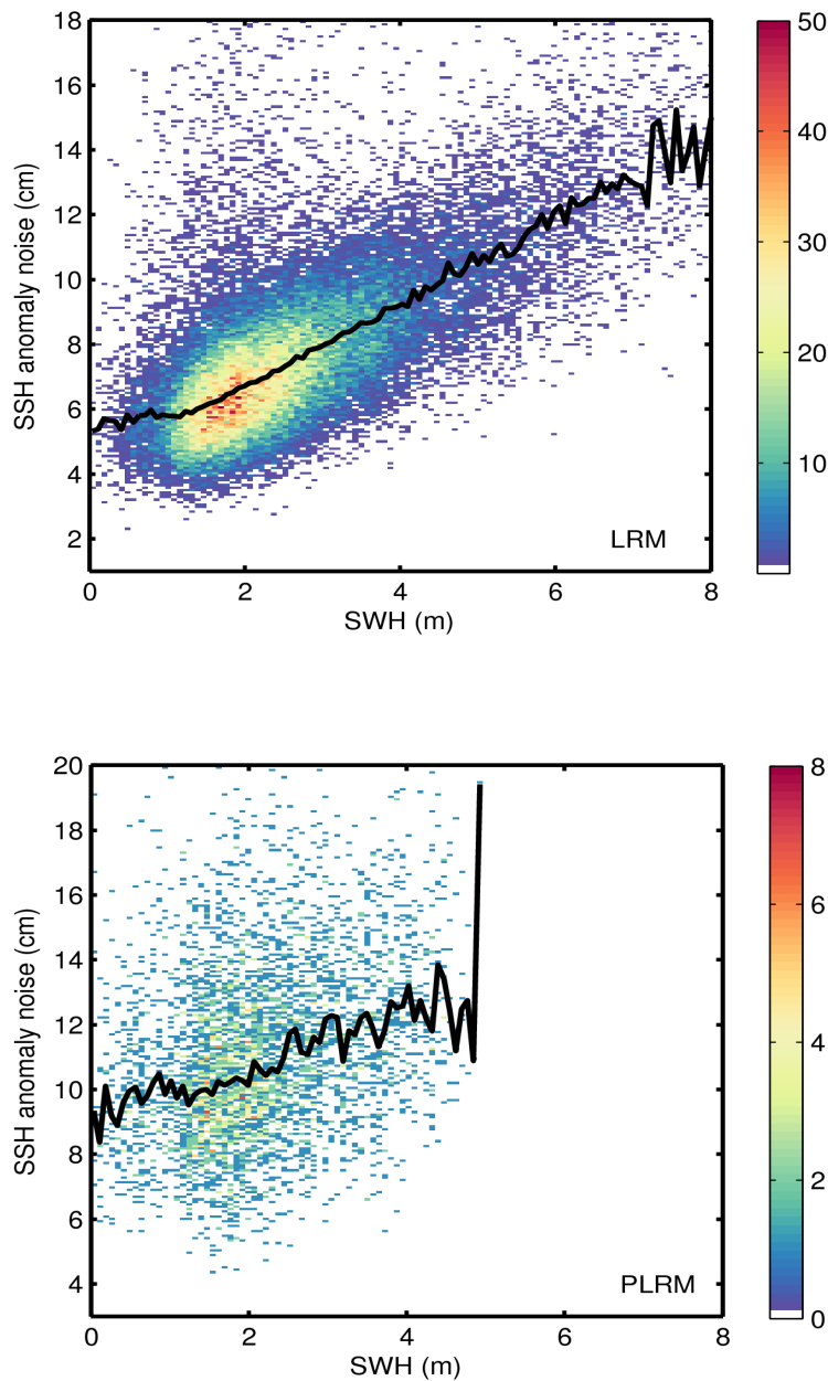
Figure 9. 2D histogram showing flag-valid SSH anomaly noise as a function of SWH for LRM (top) and PLRM (bottom) for 22/01/2017. The black line denotes the median SSH anomaly noise as a function of SWH.
