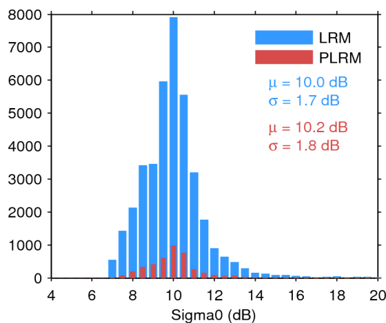
Figure 28. Histogram of science-valid sigma0 over oceans and lakes for LRM (blue) and PLRM (red) for 22/01/2017. The mean ( \mu ) and standard deviation ( \sigma ) are also shown. Note that values outside [4 20] dB are excluded from the histogram for the sake of readability but not from the computation of \mu and \sigma .
