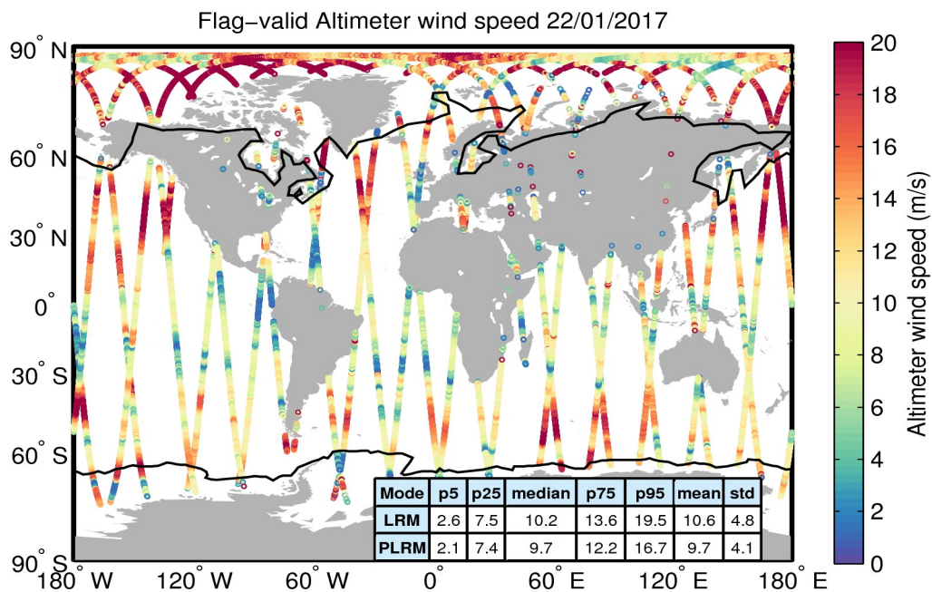
Figure 31. Geographical distribution of flag-valid wind data over oceans and lakes for 22/01/2017. The statistical values shown in the table refer to the wind in m/s and are calculated separately for LRM and PLRM regions. Measurements taken over polar polygons have been excluded from the computation of the statistical values. The black lines mark the outer limit of the Arctic and Antarctic polar polygons.
