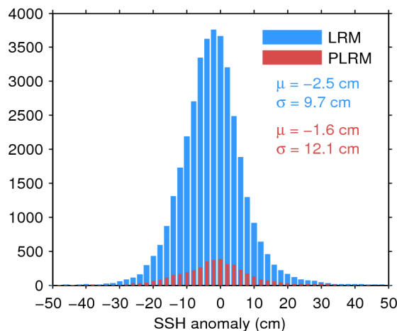
Figure 11. Histogram of science-valid SSH anomaly over oceans and lakes for LRM (blue) and PLRM (red) for 22/01/2017. The mean ( \mu ) and standard deviation ( \sigma ) are also shown. Note that values outside [-50 50] cm are excluded from the histogram for the sake of readability but not from the computation of \mu and \sigma .
