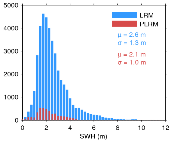
Figure 20. Histogram of science-valid SWH over oceans and lakes for LRM (blue) and PLRM (red) for 22/01/2017. The mean ( \mu ) and standard deviation ( \sigma ) are also shown. Note that values larger than 12 m are excluded from the histogram for the sake of readability but not from the computation of \mu and \sigma .
