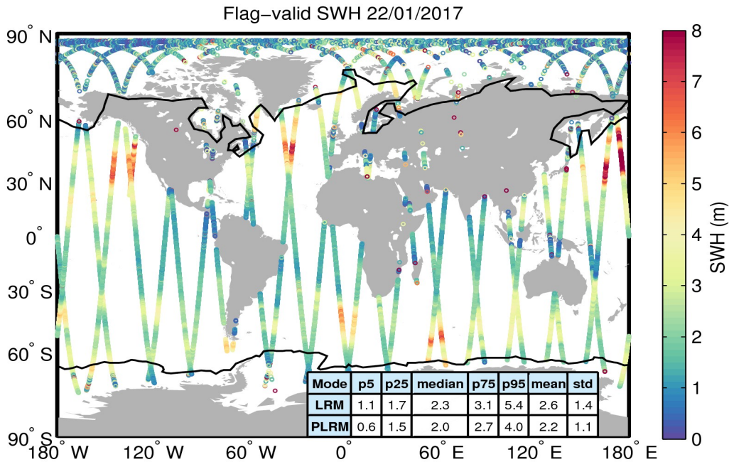
Figure 15. Geographical distribution of flag-valid SWH data over oceans and lakes for 22/01/2017. The statistical values shown in the table refer to the SWH in m and are calculated separately for LRM and PLRM regions. Measurements taken over polar polygons have been excluded from the computation of the statistical values. The black lines mark the outer limit of the Arctic and Antarctic polar polygons.
