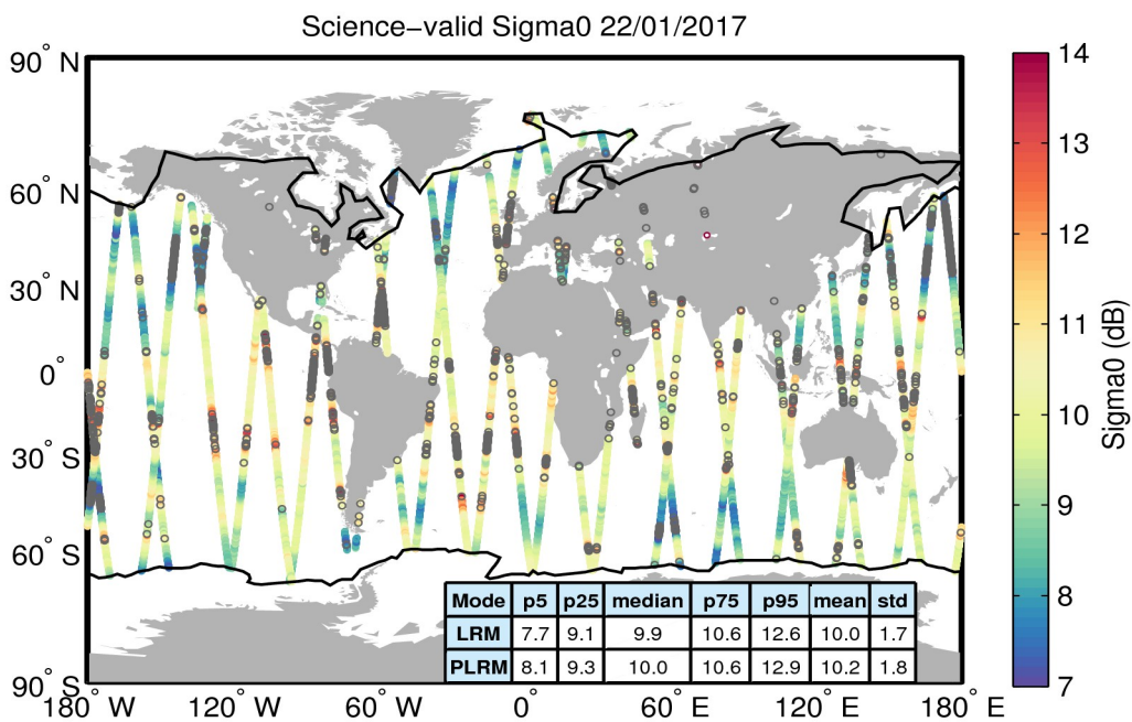
Figure 27. Geographical distribution of science-valid sigma0 data over oceans and lakes for 22/01/2017. The statistical values shown in the table refer to the sigma0 in dB and are calculated separately for LRM and PLRM regions. The black lines mark the outer limit of the Arctic and Antarctic polar polygons. Gray circles denote records that have been rejected based on the editing criteria described in Table 4.
