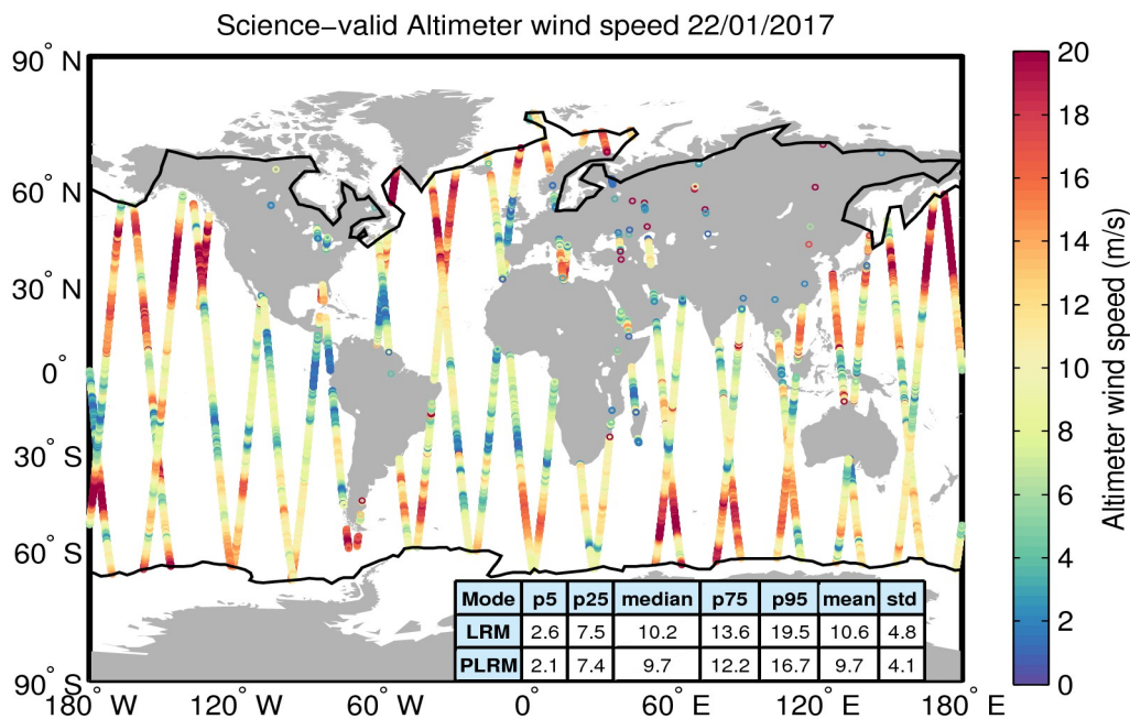
Figure 34. Geographical distribution of science-valid wind data over oceans and lakes for 22/01/2017. The statistical values shown in the table refer to the wind in m/s and are calculated separately for LRM and PLRM regions. The black lines mark the outer limit of the Arctic and Antarctic polar polygons. Gray circles denote records that have been rejected based on the editing criteria described in Table 5.
