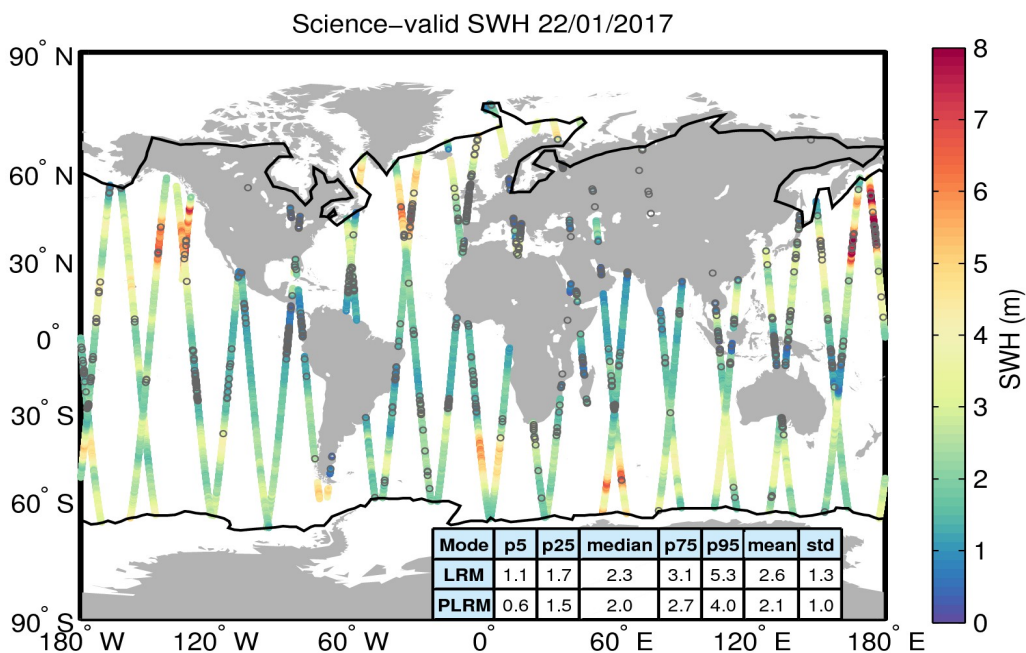
Figure 19. Geographical distribution of science-valid SWH data over oceans and lakes for 22/01/2017. The statistical values shown in the table refer to the SWH in m and are calculated separately for LRM and PLRM regions. The black lines mark the outer limit of the Arctic and Antarctic polar polygons. Gray circles denote records that have been rejected based on the editing criteria described in Table 3.
