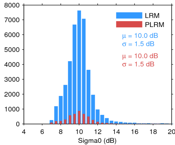
Figure 28. Histogram of science-valid sigma0 over oceans and lakes for LRM (blue) and PLRM (red) for 17/01/2017. The mean ( \mu ) and standard deviation ( \sigma ) are also shown. Note that values outside [4 20] dB are excluded from the histogram for the sake of readability but not from the computation of \mu and \sigma .
