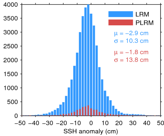
Figure 11. Histogram of science-valid SSH anomaly over oceans and lakes for LRM (blue) and PLRM (red) for 16/01/2017. The mean ( \mu ) and standard deviation ( \sigma ) are also shown. Note that values outside [-50 50] cm are excluded from the histogram for the sake of readability but not from the computation of \mu and \sigma .
