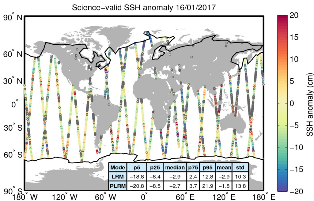
Figure 10. Geographical distribution of science-valid SSH anomaly data over oceans and lakes for 16/01/2017. The statistical values shown in the table refer to the SSH anomaly in cm and are calculated separately for LRM and PLRM regions. The black lines mark the outer limit of the Arctic and Antarctic polar polygons. Gray circles denote records that have been rejected based on the editing criteria described in Table 2.
