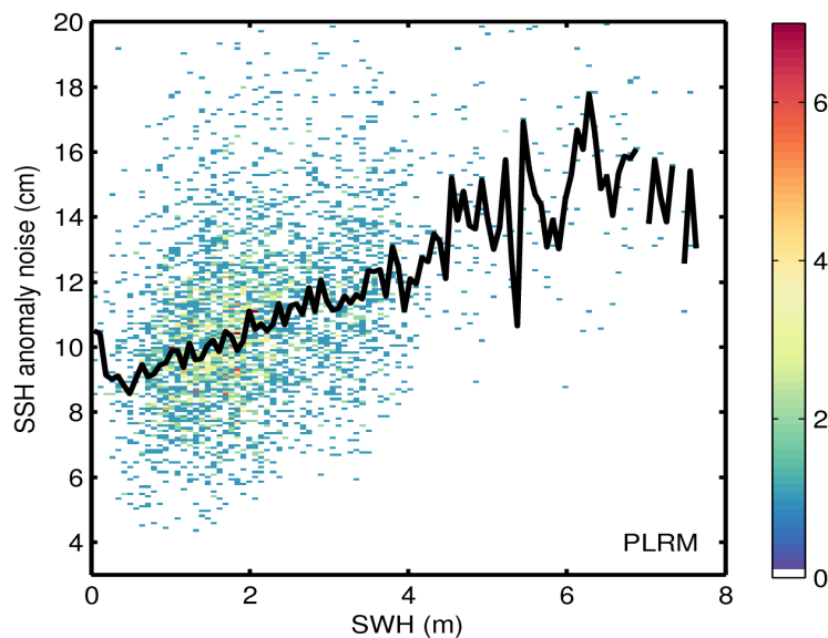
Figure 9. 2D histogram showing flag-valid SSH anomaly noise as a function of SWH for LRM (top) and PLRM (bottom) for 16/01/2017. The black line denotes the median SSH anomaly noise as a function of SWH.
