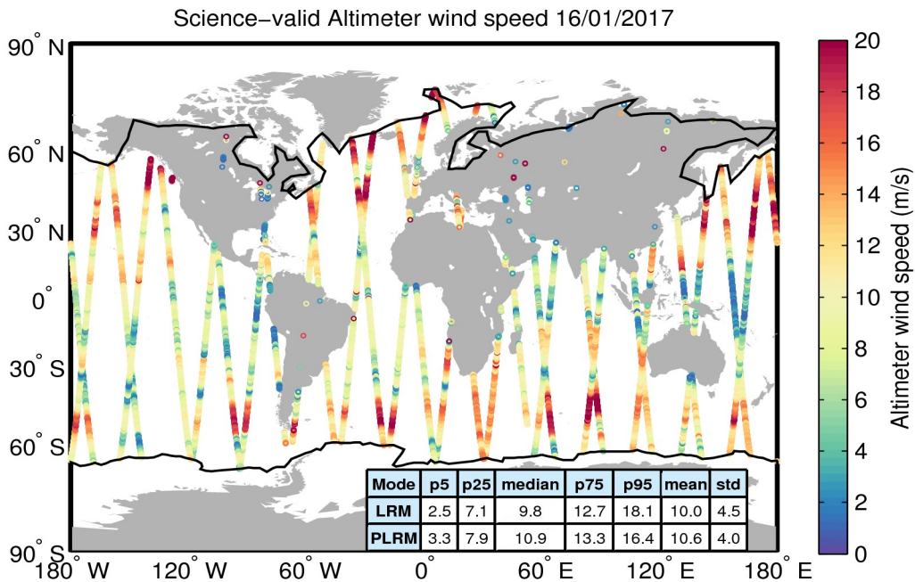
Figure 34. Geographical distribution of science-valid wind data over oceans and lakes for 16/01/2017. The statistical values shown in the table refer to the wind in m/s and are calculated separately for LRM and PLRM regions. The black lines mark the outer limit of the Arctic and Antarctic polar polygons. Gray circles denote records that have been rejected based on the editing criteria described in Table 5.
