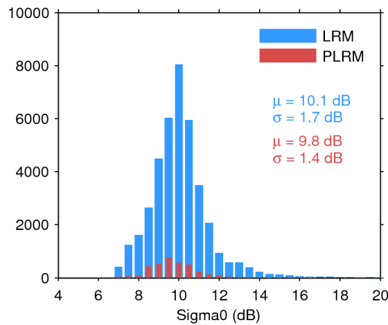
Figure 28. Histogram of science-valid sigma0 over oceans and lakes for LRM (blue) and PLRM (red) for 16/01/2017. The mean ( \mu ) and standard deviation ( \sigma ) are also shown. Note that values outside [4 20] dB are excluded from the histogram for the sake of readability but not from the computation of \mu and \sigma .
