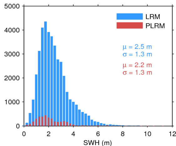
Figure 17. Histogram of flag-valid SWH over oceans and lakes for LRM (blue) and PLRM (red) for 16/01/2017. The mean ( \mu ) and standard deviation ( \sigma ) are also shown. Note that values larger than 12 m are excluded from the histogram for the sake of readability but not from the computation of \mu and \sigma .
