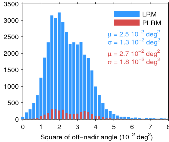
Figure 39. Histogram of flag-valid mispointing over oceans and lakes for LRM (blue) and PLRM (red) for 16/01/2017. Only positive values have been considered. The mean ( \mu ) and standard deviation ( \sigma ) are also shown. Note that values larger than 8 \cdot 10^{-2} \text{ deg}^2 are excluded from the histogram for the sake of readability but not from the computation of \mu and \sigma .
