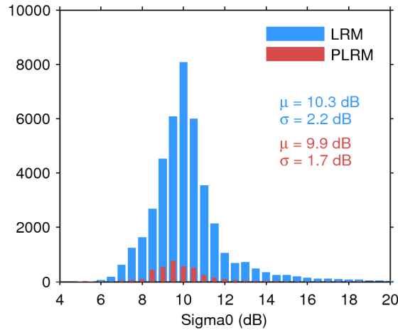
Figure 25. Histogram of flag-valid sigma0 over oceans and lakes for LRM (blue) and PLRM (red) for 16/01/2017. The mean ( \mu ) and standard deviation ( \sigma ) are also shown. Note that values outside [4 20] dB are excluded from the histogram for the sake of readability but not from the computation of \mu and \sigma .
