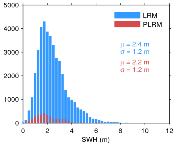
Figure 20. Histogram of science-valid SWH over oceans and lakes for LRM (blue) and PLRM (red) for 16/01/2017. The mean ( \mu ) and standard deviation ( \sigma ) are also shown. Note that values larger than 12 m are excluded from the histogram for the sake of readability but not from the computation of \mu and \sigma .
