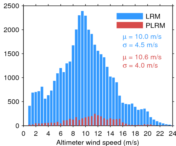
Figure 35. Histogram of science-valid wind over oceans and lakes for LRM (blue) and PLRM (red) for 16/01/2017. The mean ( \mu ) and standard deviation ( \sigma ) are also shown. Note that values larger than 24 m/s are excluded from the histogram for the sake of readability but not from the computation of \mu and \sigma .
