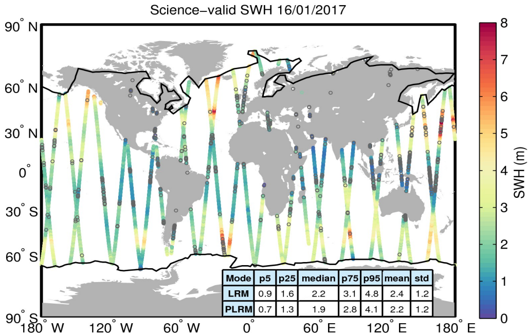
Figure 19. Geographical distribution of science-valid SWH data over oceans and lakes for 16/01/2017. The statistical values shown in the table refer to the SWH in m and are calculated separately for LRM and PLRM regions. The black lines mark the outer limit of the Arctic and Antarctic polar polygons. Gray circles denote records that have been rejected based on the editing criteria described in Table 3.
