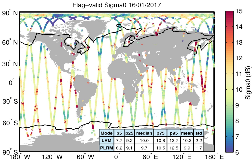
Figure 23. Geographical distribution of flag-valid sigma0 data over oceans and lakes for 16/01/2017. The statistical values shown in the table refer to the sigma0 in dB and are calculated separately for LRM and PLRM regions. Measurements taken over polar polygons have been excluded from the computation of the statistical values. The black lines mark the outer limit of the Arctic and Antarctic polar polygons.
