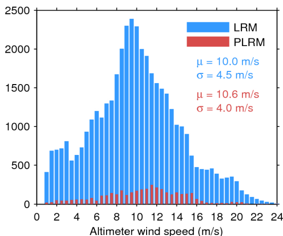
Figure 33. Histogram of flag-valid wind over oceans and lakes for LRM (blue) and PLRM (red) for 16/01/2017. The mean ( \mu ) and standard deviation ( \sigma ) are also shown. Note that values larger than 24 m/s are excluded from the histogram for the sake of readability but not from the computation of \mu and \sigma .
