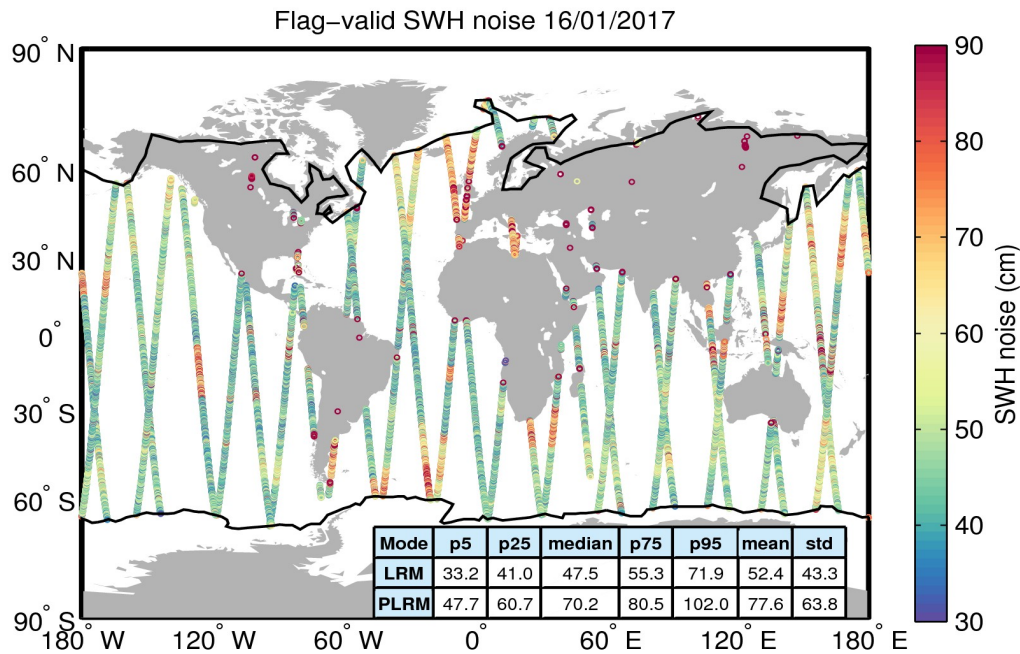
Figure 18. Geographical distribution of flag-valid 20-Hz SWH measurement noise over oceans and lakes for 16/01/2017. The statistical values shown in the table refer to the SWH noise and are calculated separately for LRM and PLRM regions. Measurements taken over polar polygons have been excluded from the computation of the statistical values. The black lines mark the outer limit of the Arctic and Antarctic polar polygons.
