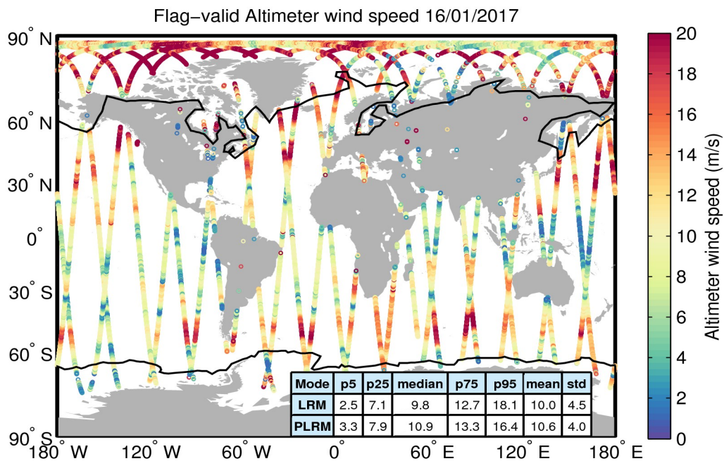
Figure 31. Geographical distribution of flag-valid wind data over oceans and lakes for 16/01/2017. The statistical values shown in the table refer to the wind in m/s and are calculated separately for LRM and PLRM regions. Measurements taken over polar polygons have been excluded from the computation of the statistical values. The black lines mark the outer limit of the Arctic and Antarctic polar polygons.
