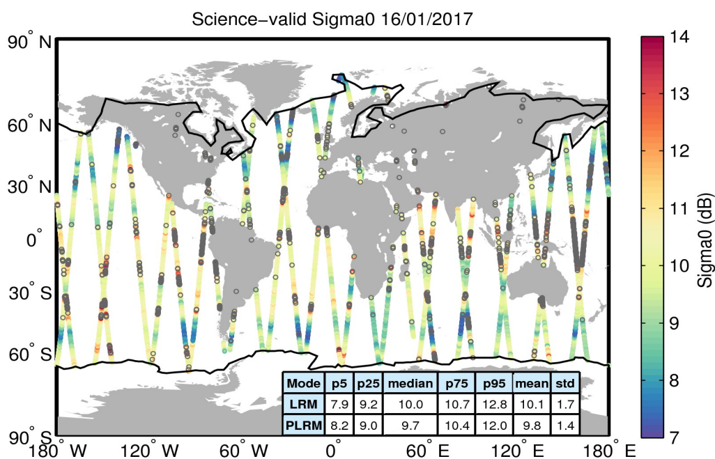
Figure 27. Geographical distribution of science-valid sigma0 data over oceans and lakes for 16/01/2017. The statistical values shown in the table refer to the sigma0 in dB and are calculated separately for LRM and PLRM regions. The black lines mark the outer limit of the Arctic and Antarctic polar polygons. Gray circles denote records that have been rejected based on the editing criteria described in Table 4.
