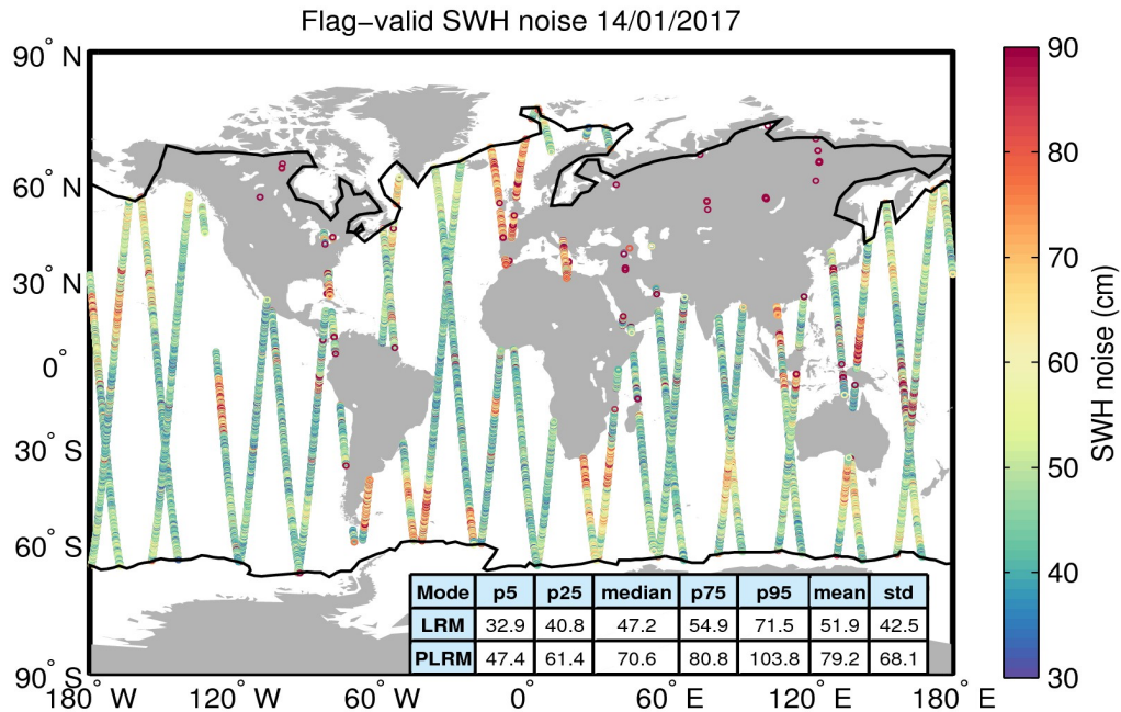
Figure 18. Geographical distribution of flag-valid 20-Hz SWH measurement noise over oceans and lakes for 14/01/2017. The statistical values shown in the table refer to the SWH noise and are calculated separately for LRM and PLRM regions. Measurements taken over polar polygons have been excluded from the computation of the statistical values. The black lines mark the outer limit of the Arctic and Antarctic polar polygons.
