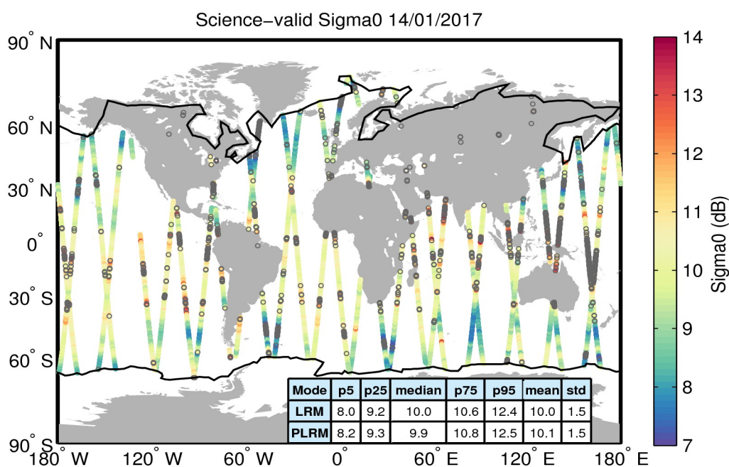
Figure 27. Geographical distribution of science-valid sigma0 data over oceans and lakes for 14/01/2017. The statistical values shown in the table refer to the sigma0 in dB and are calculated separately for LRM and PLRM regions. The black lines mark the outer limit of the Arctic and Antarctic polar polygons. Gray circles denote records that have been rejected based on the editing criteria described in Table 4.
