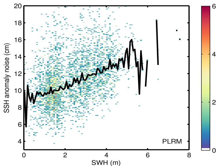
Figure 9. 2D histogram showing flag-valid SSH anomaly noise as a function of SWH for LRM (top) and PLRM (bottom) for 14/01/2017. The black line denotes the median SSH anomaly noise as a function of SWH.
