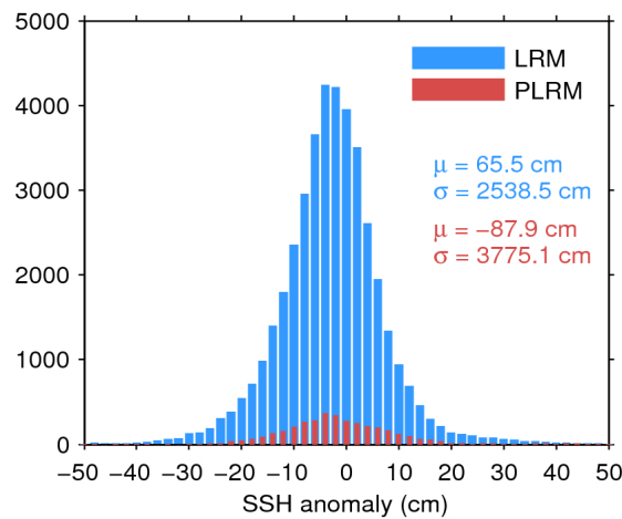
Figure 7. Histogram of flag-valid SSH anomaly over oceans and lakes for LRM (blue) and PLRM (red) for 14/01/2017. The mean ( \mu ) and standard deviation ( \sigma ) are also shown. Note that values outside [-50 50] cm are excluded from the histogram for the sake of readability but not from the computation of \mu and \sigma .
