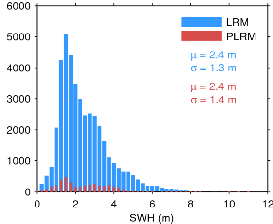
Figure 17. Histogram of flag-valid SWH over oceans and lakes for LRM (blue) and PLRM (red) for 14/01/2017. The mean ( \mu ) and standard deviation ( \sigma ) are also shown. Note that values larger than 12 m are excluded from the histogram for the sake of readability but not from the computation of \mu and \sigma .
