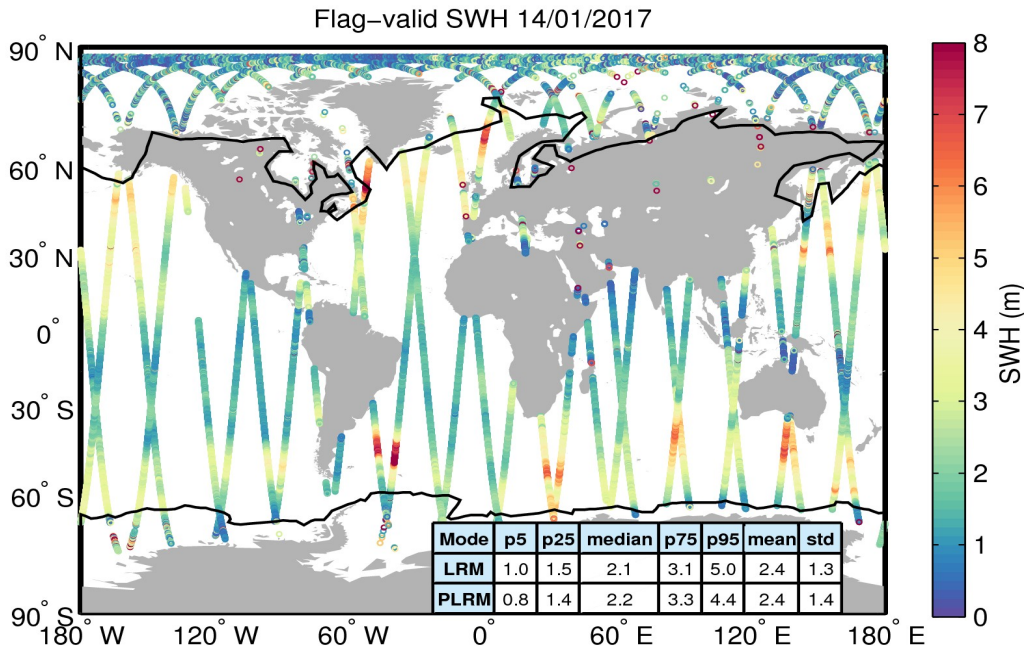
Figure 15. Geographical distribution of flag-valid SWH data over oceans and lakes for 14/01/2017. The statistical values shown in the table refer to the SWH in m and are calculated separately for LRM and PLRM regions. Measurements taken over polar polygons have been excluded from the computation of the statistical values. The black lines mark the outer limit of the Arctic and Antarctic polar polygons.
