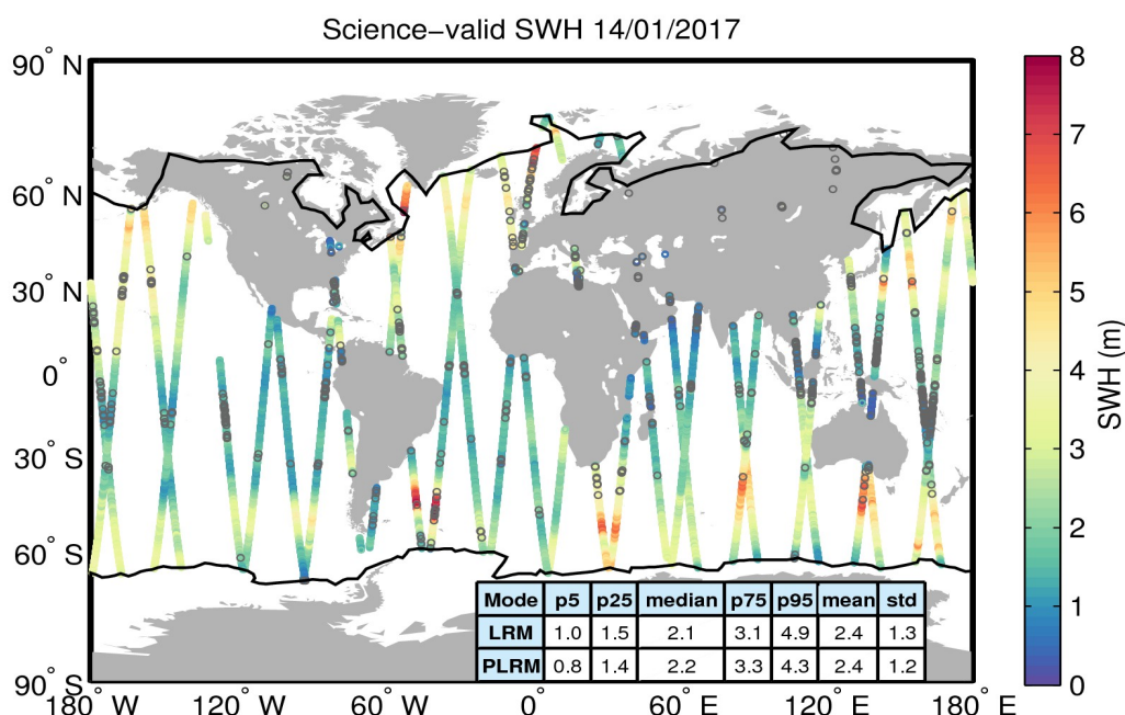
Figure 19. Geographical distribution of science-valid SWH data over oceans and lakes for 14/01/2017. The statistical values shown in the table refer to the SWH in m and are calculated separately for LRM and PLRM regions. The black lines mark the outer limit of the Arctic and Antarctic polar polygons. Gray circles denote records that have been rejected based on the editing criteria described in Table 3.
