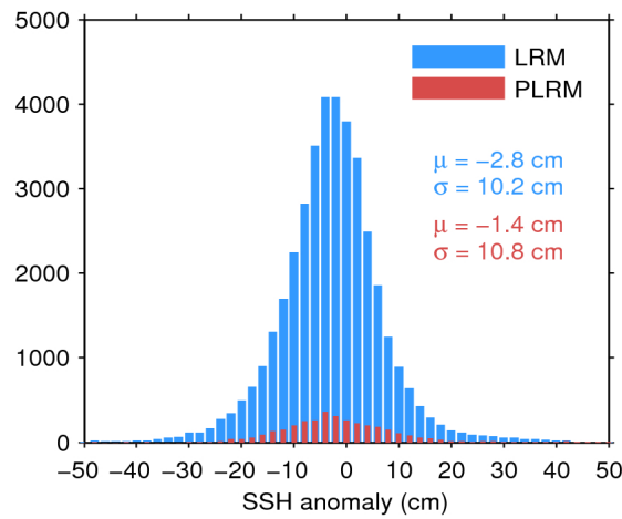
Figure 11. Histogram of science-valid SSH anomaly over oceans and lakes for LRM (blue) and PLRM (red) for 14/01/2017. The mean ( \mu ) and standard deviation ( \sigma ) are also shown. Note that values outside [-50\ 50] cm are excluded from the histogram for the sake of readability but not from the computation of \mu and \sigma .
