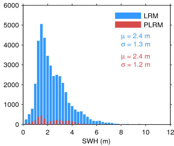
Figure 20. Histogram of science-valid SWH over oceans and lakes for LRM (blue) and PLRM (red) for 14/01/2017. The mean ( \mu ) and standard deviation ( \sigma ) are also shown. Note that values larger than 12 m are excluded from the histogram for the sake of readability but not from the computation of \mu and \sigma .
