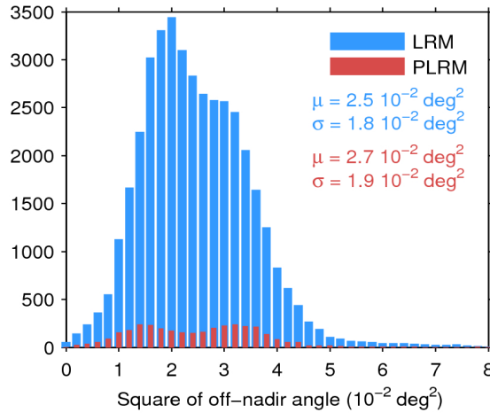
Figure 39. Histogram of flag-valid mispointing over oceans and lakes for LRM (blue) and PLRM (red) for 14/01/2017. Only positive values have been considered. The mean ( \mu ) and standard deviation ( \sigma ) are also shown. Note that values larger than 8 \cdot 10^{-2} \text{ deg}^2 are excluded from the histogram for the sake of readability but not from the computation of \mu and \sigma .
