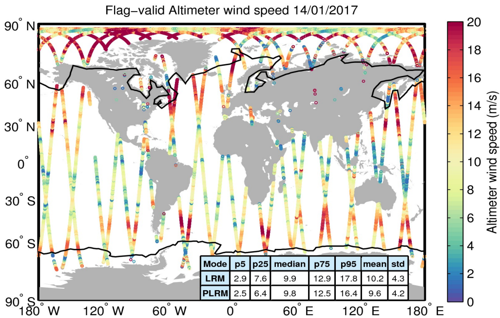
Figure 31. Geographical distribution of flag-valid wind data over oceans and lakes for 14/01/2017. The statistical values shown in the table refer to the wind in m/s and are calculated separately for LRM and PLRM regions. Measurements taken over polar polygons have been excluded from the computation of the statistical values. The black lines mark the outer limit of the Arctic and Antarctic polar polygons.
