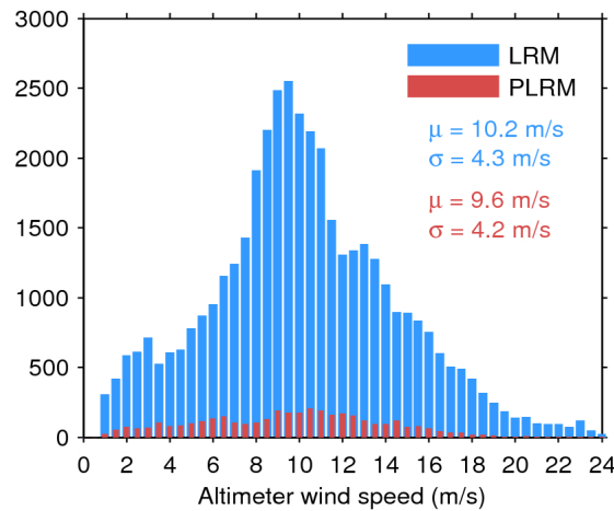
Figure 33. Histogram of flag-valid wind over oceans and lakes for LRM (blue) and PLRM (red) for 14/01/2017. The mean ( \mu ) and standard deviation ( \sigma ) are also shown. Note that values larger than 24 m/s are excluded from the histogram for the sake of readability but not from the computation of \mu and \sigma .
