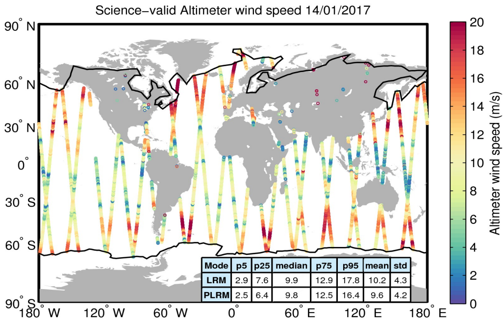
Figure 34. Geographical distribution of science-valid wind data over oceans and lakes for 14/01/2017. The statistical values shown in the table refer to the wind in m/s and are calculated separately for LRM and PLRM regions. The black lines mark the outer limit of the Arctic and Antarctic polar polygons. Gray circles denote records that have been rejected based on the editing criteria described in Table 5.
