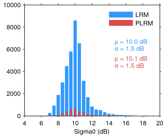
Figure 28. Histogram of science-valid sigma0 over oceans and lakes for LRM (blue) and PLRM (red) for 14/01/2017. The mean ( \mu ) and standard deviation ( \sigma ) are also shown. Note that values outside [4 20] dB are excluded from the histogram for the sake of readability but not from the computation of \mu and \sigma .
