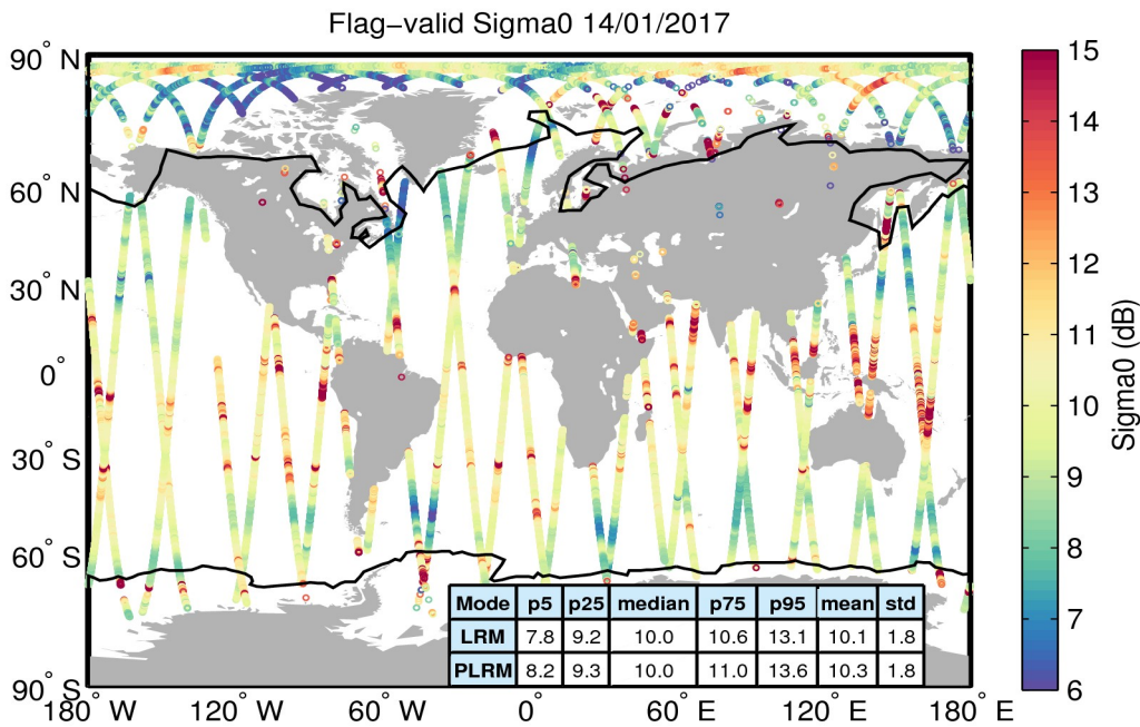
Figure 23. Geographical distribution of flag-valid sigma0 data over oceans and lakes for 14/01/2017. The statistical values shown in the table refer to the sigma0 in dB and are calculated separately for LRM and PLRM regions. Measurements taken over polar polygons have been excluded from the computation of the statistical values. The black lines mark the outer limit of the Arctic and Antarctic polar polygons.
