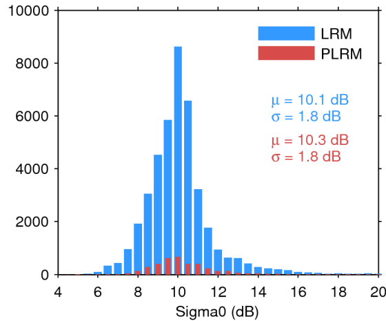
Figure 25. Histogram of flag-valid sigma0 over oceans and lakes for LRM (blue) and PLRM (red) for 14/01/2017. The mean ( \mu ) and standard deviation ( \sigma ) are also shown. Note that values outside [4 20] dB are excluded from the histogram for the sake of readability but not from the computation of \mu and \sigma .
