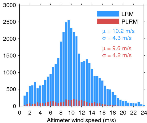
Figure 35. Histogram of science-valid wind over oceans and lakes for LRM (blue) and PLRM (red) for 14/01/2017. The mean ( \mu ) and standard deviation ( \sigma ) are also shown. Note that values larger than 24 m/s are excluded from the histogram for the sake of readability but not from the computation of \mu and \sigma .
