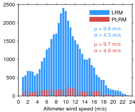
Figure 33. Histogram of flag-valid wind over oceans and lakes for LRM (blue) and PLRM (red) for 13/01/2017. The mean ( \mu ) and standard deviation ( \sigma ) are also shown. Note that values larger than 24 m/s are excluded from the histogram for the sake of readability but not from the computation of \mu and \sigma .
