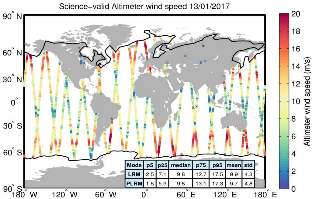
Figure 34. Geographical distribution of science-valid wind data over oceans and lakes for 13/01/2017. The statistical values shown in the table refer to the wind in m/s and are calculated separately for LRM and PLRM regions. The black lines mark the outer limit of the Arctic and Antarctic polar polygons. Gray circles denote records that have been rejected based on the editing criteria described in Table 5.
