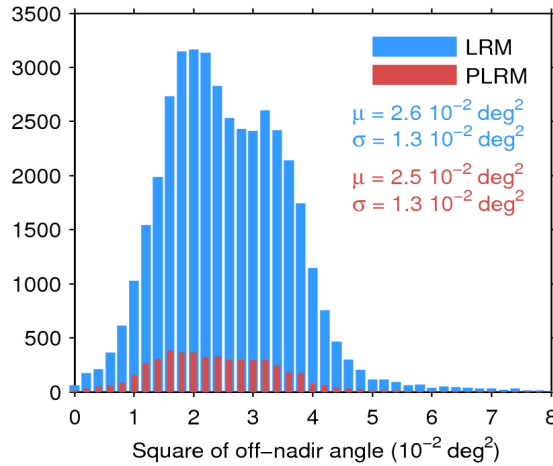
Figure 39. Histogram of flag-valid mispointing over oceans and lakes for LRM (blue) and PLRM (red) for 13/01/2017. Only positive values have been considered. The mean ( \mu ) and standard deviation ( \sigma ) are also shown. Note that values larger than 8 \cdot 10^{-2} \text{ deg}^2 are excluded from the histogram for the sake of readability but not from the computation of \mu and \sigma .
