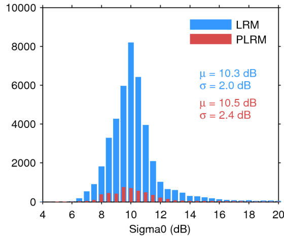
Figure 25. Histogram of flag-valid sigma0 over oceans and lakes for LRM (blue) and PLRM (red) for 13/01/2017. The mean ( \mu ) and standard deviation ( \sigma ) are also shown. Note that values outside [4 20] dB are excluded from the histogram for the sake of readability but not from the computation of \mu and \sigma .
