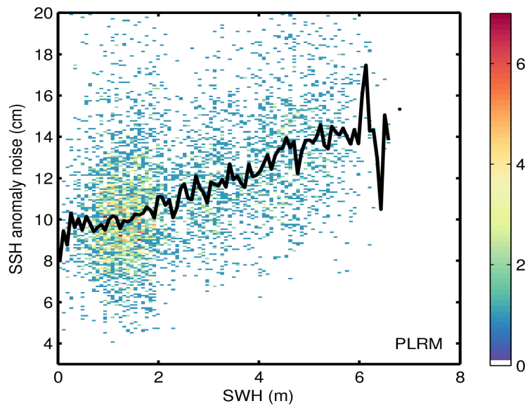
Figure 9. 2D histogram showing flag-valid SSH anomaly noise as a function of SWH for LRM (top) and PLRM (bottom) for 13/01/2017. The black line denotes the median SSH anomaly noise as a function of SWH.
