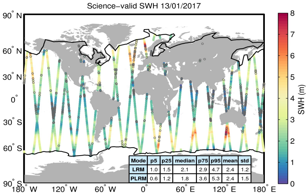
Figure 19. Geographical distribution of science-valid SWH data over oceans and lakes for 13/01/2017. The statistical values shown in the table refer to the SWH in m and are calculated separately for LRM and PLRM regions. The black lines mark the outer limit of the Arctic and Antarctic polar polygons. Gray circles denote records that have been rejected based on the editing criteria described in Table 3.
