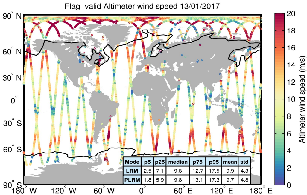
Figure 31. Geographical distribution of flag-valid wind data over oceans and lakes for 13/01/2017. The statistical values shown in the table refer to the wind in m/s and are calculated separately for LRM and PLRM regions. Measurements taken over polar polygons have been excluded from the computation of the statistical values. The black lines mark the outer limit of the Arctic and Antarctic polar polygons.
