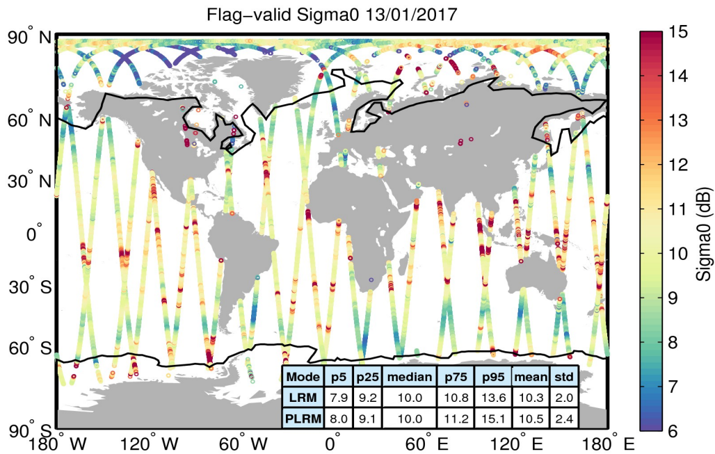
Figure 23. Geographical distribution of flag-valid sigma0 data over oceans and lakes for 13/01/2017. The statistical values shown in the table refer to the sigma0 in dB and are calculated separately for LRM and PLRM regions. Measurements taken over polar polygons have been excluded from the computation of the statistical values. The black lines mark the outer limit of the Arctic and Antarctic polar polygons.
