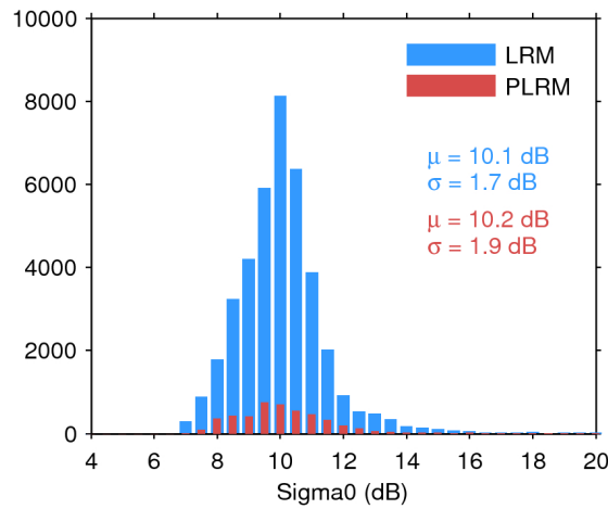
Figure 28. Histogram of science-valid sigma0 over oceans and lakes for LRM (blue) and PLRM (red) for 13/01/2017. The mean ( \mu ) and standard deviation ( \sigma ) are also shown. Note that values outside [4 20] dB are excluded from the histogram for the sake of readability but not from the computation of \mu and \sigma .
