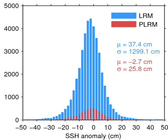
Figure 7. Histogram of flag-valid SSH anomaly over oceans and lakes for LRM (blue) and PLRM (red) for 13/01/2017. The mean ( \mu ) and standard deviation ( \sigma ) are also shown. Note that values outside [-50 50] cm are excluded from the histogram for the sake of readability but not from the computation of \mu and \sigma .
