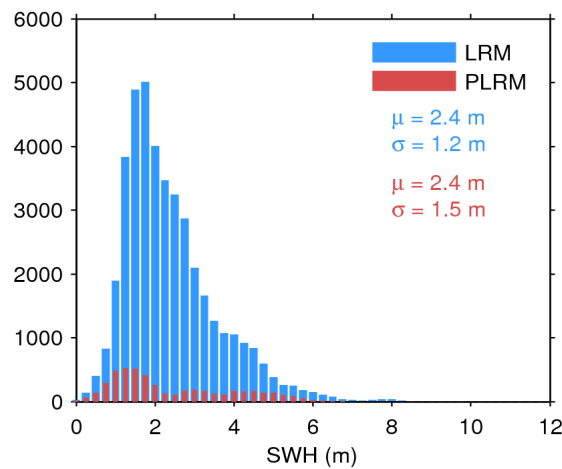
Figure 20. Histogram of science-valid SWH over oceans and lakes for LRM (blue) and PLRM (red) for 13/01/2017. The mean ( \mu ) and standard deviation ( \sigma ) are also shown. Note that values larger than 12 m are excluded from the histogram for the sake of readability but not from the computation of \mu and \sigma .
