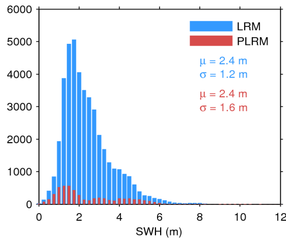
Figure 17. Histogram of flag-valid SWH over oceans and lakes for LRM (blue) and PLRM (red) for 13/01/2017. The mean ( \mu ) and standard deviation ( \sigma ) are also shown. Note that values larger than 12 m are excluded from the histogram for the sake of readability but not from the computation of \mu and \sigma .
