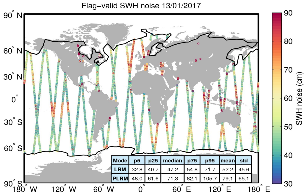
Figure 18. Geographical distribution of flag-valid 20-Hz SWH measurement noise over oceans and lakes for 13/01/2017. The statistical values shown in the table refer to the SWH noise and are calculated separately for LRM and PLRM regions. Measurements taken over polar polygons have been excluded from the computation of the statistical values. The black lines mark the outer limit of the Arctic and Antarctic polar polygons.
