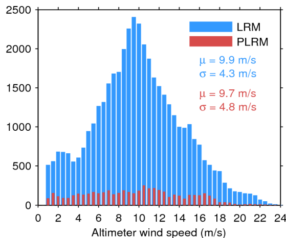
Figure 35. Histogram of science-valid wind over oceans and lakes for LRM (blue) and PLRM (red) for 13/01/2017. The mean ( \mu ) and standard deviation ( \sigma ) are also shown. Note that values larger than 24 m/s are excluded from the histogram for the sake of readability but not from the computation of \mu and \sigma .
