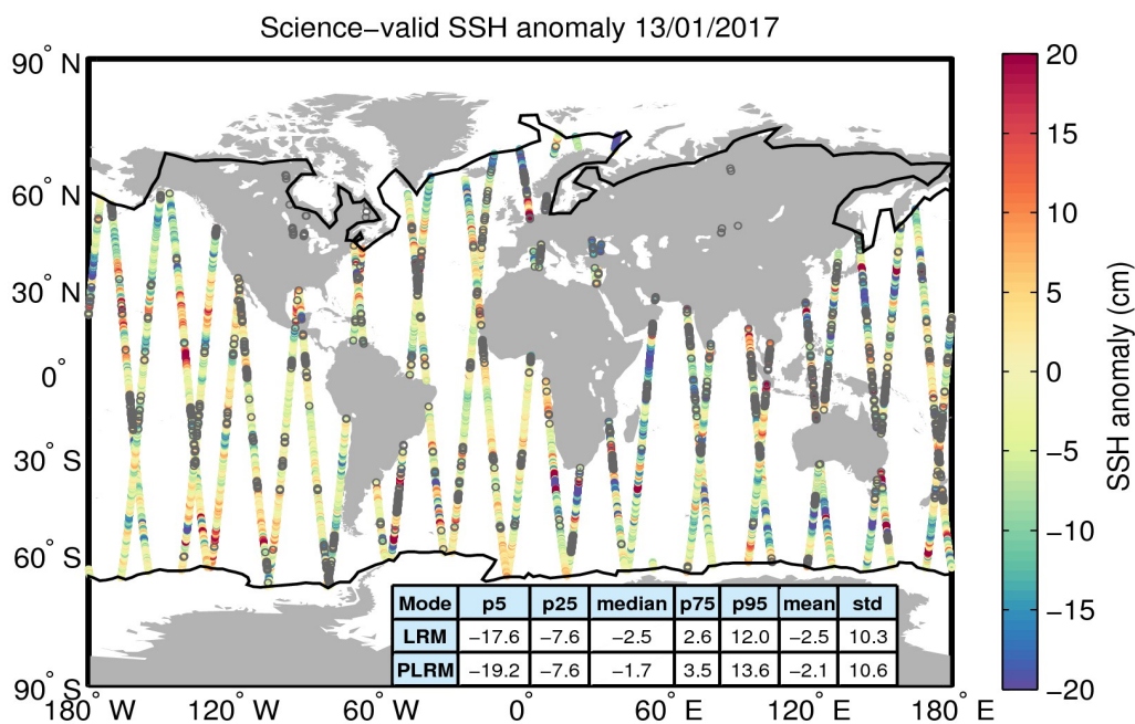
Figure 10. Geographical distribution of science-valid SSH anomaly data over oceans and lakes for 13/01/2017. The statistical values shown in the table refer to the SSH anomaly in cm and are calculated separately for LRM and PLRM regions. The black lines mark the outer limit of the Arctic and Antarctic polar polygons. Gray circles denote records that have been rejected based on the editing criteria described in Table 2.
