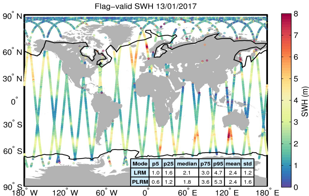
Figure 15. Geographical distribution of flag-valid SWH data over oceans and lakes for 13/01/2017. The statistical values shown in the table refer to the SWH in m and are calculated separately for LRM and PLRM regions. Measurements taken over polar polygons have been excluded from the computation of the statistical values. The black lines mark the outer limit of the Arctic and Antarctic polar polygons.
