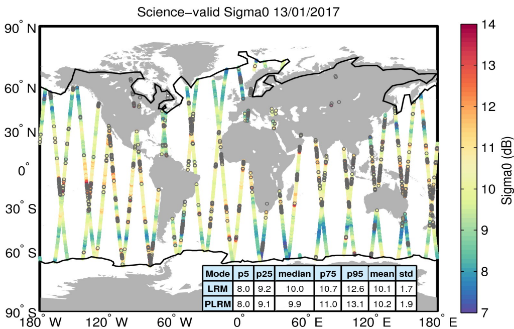
Figure 27. Geographical distribution of science-valid sigma0 data over oceans and lakes for 13/01/2017. The statistical values shown in the table refer to the sigma0 in dB and are calculated separately for LRM and PLRM regions. The black lines mark the outer limit of the Arctic and Antarctic polar polygons. Gray circles denote records that have been rejected based on the editing criteria described in Table 4.
