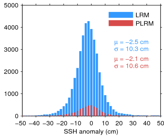
Figure 11. Histogram of science-valid SSH anomaly over oceans and lakes for LRM (blue) and PLRM (red) for 13/01/2017. The mean ( \mu ) and standard deviation ( \sigma ) are also shown. Note that values outside [-50 50] cm are excluded from the histogram for the sake of readability but not from the computation of \mu and \sigma .
