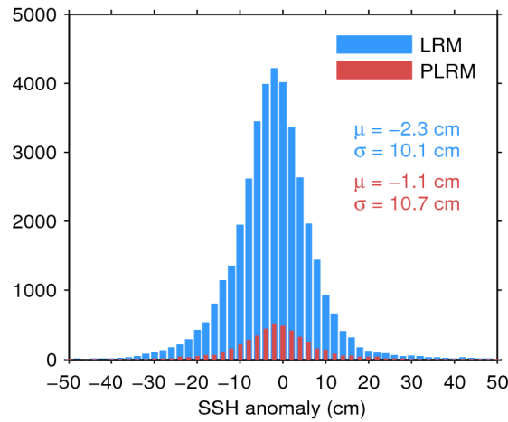
Figure 11. Histogram of science-valid SSH anomaly over oceans and lakes for LRM (blue) and PLRM (red) for 11/01/2017. The mean ( \mu ) and standard deviation ( \sigma ) are also shown. Note that values outside [-50\ 50] cm are excluded from the histogram for the sake of readability but not from the computation of \mu and \sigma .
