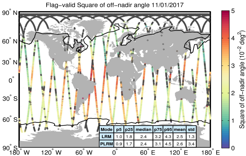
Figure 37. Geographical distribution of flag-valid mispointing data over oceans and lakes for 11/01/2017. The statistical values shown in the table refer to the mispointing in 10^{-2} deg 2 and are calculated separately for LRM and PLRM regions. Measurements taken over polar polygons have been excluded from the computation of the statistical values. The black lines mark the outer limit of the Arctic and Antarctic polar polygons. Gray circles denote negative values.
