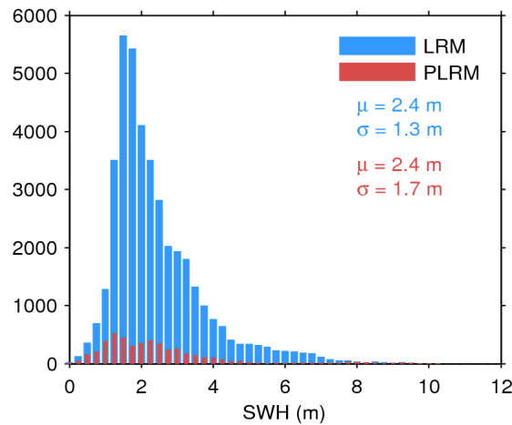
Figure 20. Histogram of science-valid SWH over oceans and lakes for LRM (blue) and PLRM (red) for 11/01/2017. The mean ( \mu ) and standard deviation ( \sigma ) are also shown. Note that values larger than 12 m are excluded from the histogram for the sake of readability but not from the computation of \mu and \sigma .
