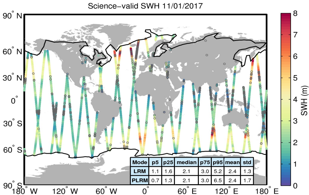
Figure 19. Geographical distribution of science-valid SWH data over oceans and lakes for 11/01/2017. The statistical values shown in the table refer to the SWH in m and are calculated separately for LRM and PLRM regions. The black lines mark the outer limit of the Arctic and Antarctic polar polygons. Gray circles denote records that have been rejected based on the editing criteria described in Table 3.
