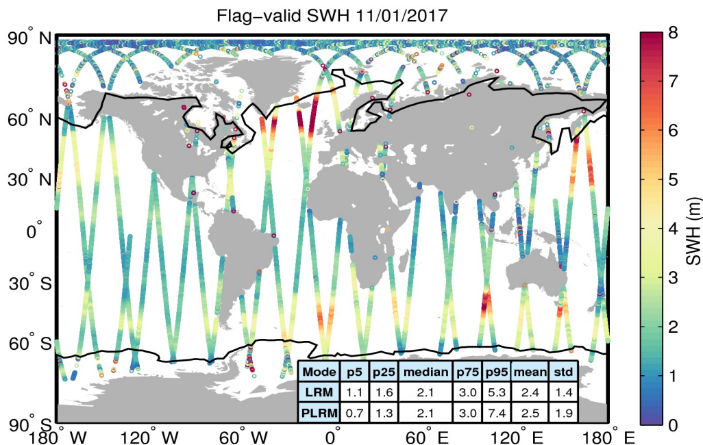
Figure 15. Geographical distribution of flag-valid SWH data over oceans and lakes for 11/01/2017. The statistical values shown in the table refer to the SWH in m and are calculated separately for LRM and PLRM regions. Measurements taken over polar polygons have been excluded from the computation of the statistical values. The black lines mark the outer limit of the Arctic and Antarctic polar polygons.
