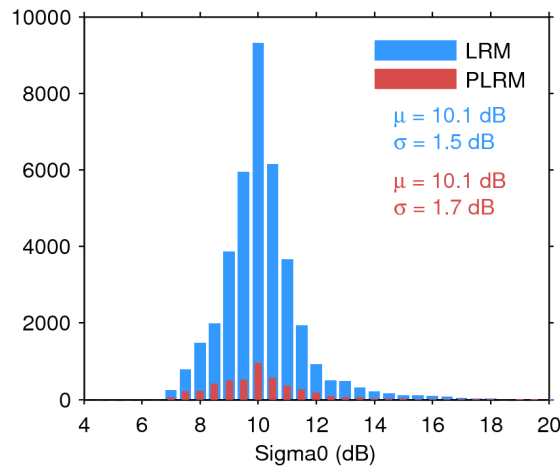
Figure 28. Histogram of science-valid sigma0 over oceans and lakes for LRM (blue) and PLRM (red) for 11/01/2017. The mean ( \mu ) and standard deviation ( \sigma ) are also shown. Note that values outside [4 20] dB are excluded from the histogram for the sake of readability but not from the computation of \mu and \sigma .
