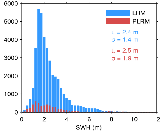
Figure 17. Histogram of flag-valid SWH over oceans and lakes for LRM (blue) and PLRM (red) for 11/01/2017. The mean ( \mu ) and standard deviation ( \sigma ) are also shown. Note that values larger than 12 m are excluded from the histogram for the sake of readability but not from the computation of \mu and \sigma .
