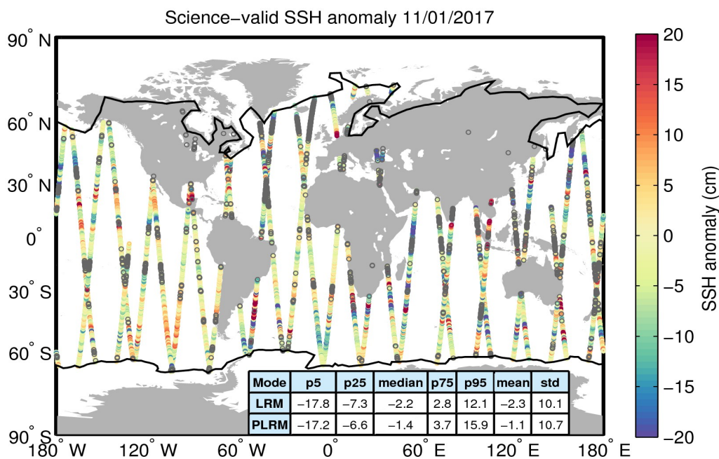
Figure 10. Geographical distribution of science-valid SSH anomaly data over oceans and lakes for 11/01/2017. The statistical values shown in the table refer to the SSH anomaly in cm and are calculated separately for LRM and PLRM regions. The black lines mark the outer limit of the Arctic and Antarctic polar polygons. Gray circles denote records that have been rejected based on the editing criteria described in Table 2.
