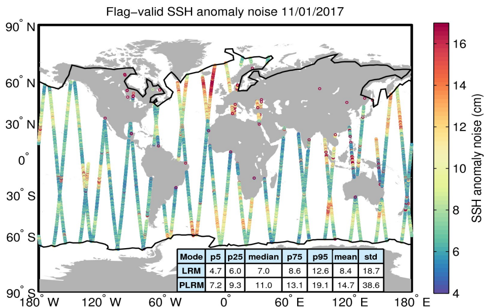
Figure 8. Geographical distribution of flag-valid 20-Hz SSH anomaly measurement noise over oceans and lakes for 11/01/2017. The statistical values shown in the table refer to the SSH anomaly noise and are calculated separately for LRM and PLRM regions. Measurements taken over polar polygons have been excluded from the computation of the statistical values. The black lines mark the outer limit of the Arctic and Antarctic polar polygons.
