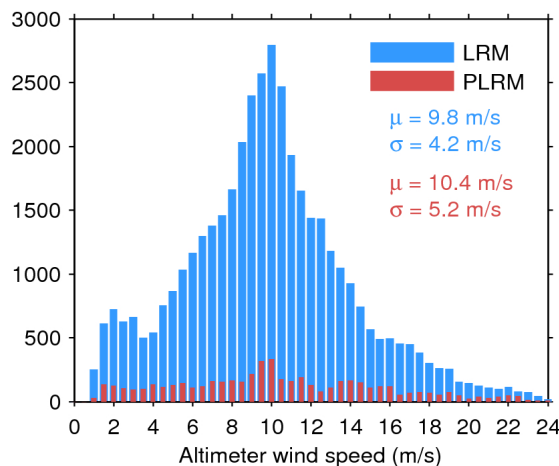
Figure 35. Histogram of science-valid wind over oceans and lakes for LRM (blue) and PLRM (red) for 11/01/2017. The mean ( \mu ) and standard deviation ( \sigma ) are also shown. Note that values larger than 24 m/s are excluded from the histogram for the sake of readability but not from the computation of \mu and \sigma .
