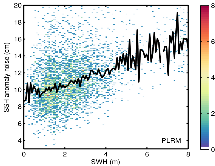
Figure 9. 2D histogram showing flag-valid SSH anomaly noise as a function of SWH for LRM (top) and PLRM (bottom) for 11/01/2017. The black line denotes the median SSH anomaly noise as a function of SWH.
