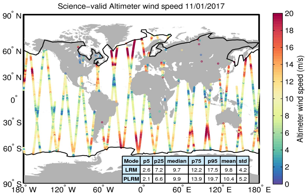
Figure 34. Geographical distribution of science-valid wind data over oceans and lakes for 11/01/2017. The statistical values shown in the table refer to the wind in m/s and are calculated separately for LRM and PLRM regions. The black lines mark the outer limit of the Arctic and Antarctic polar polygons. Gray circles denote records that have been rejected based on the editing criteria described in Table 5.
