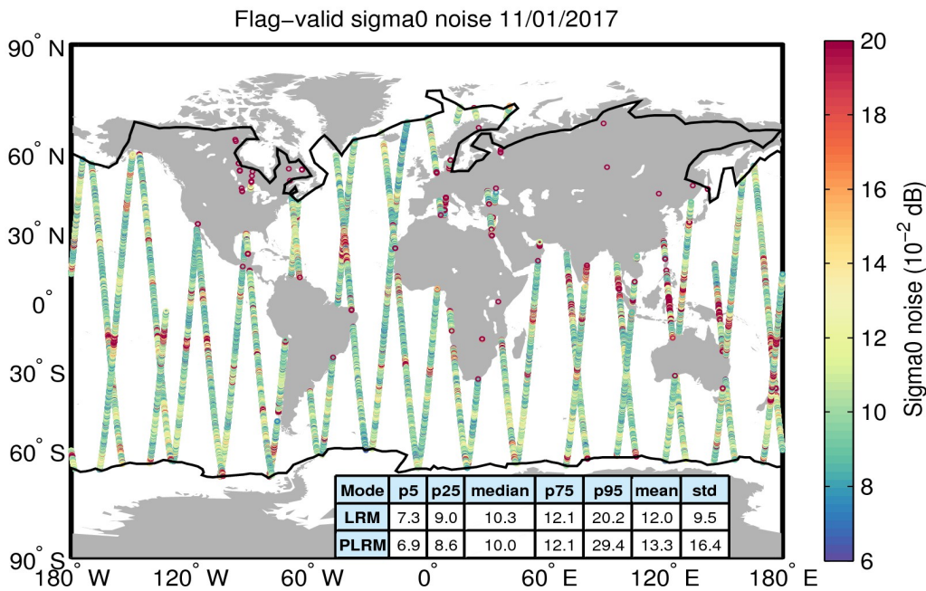
Figure 26. Geographical distribution of flag-valid 20-Hz sigma0 measurement noise over oceans and lakes for 11/01/2017. The statistical values shown in the table refer to the sigma0 noise and are calculated separately for LRM and PLRM regions. Measurements taken over polar polygons have been excluded from the computation of the statistical values. The black lines mark the outer limit of the Arctic and Antarctic polar polygons.
