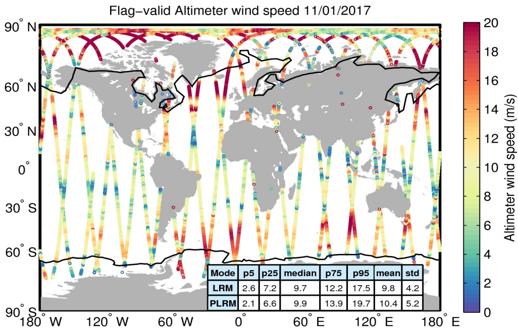
Figure 31. Geographical distribution of flag-valid wind data over oceans and lakes for 11/01/2017. The statistical values shown in the table refer to the wind in m/s and are calculated separately for LRM and PLRM regions. Measurements taken over polar polygons have been excluded from the computation of the statistical values. The black lines mark the outer limit of the Arctic and Antarctic polar polygons.
