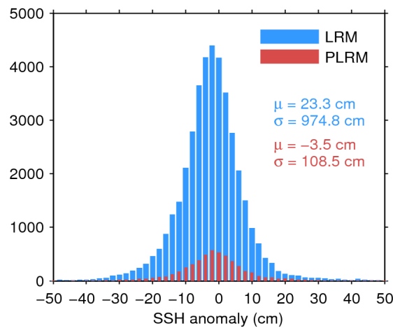
Figure 7. Histogram of flag-valid SSH anomaly over oceans and lakes for LRM (blue) and PLRM (red) for 11/01/2017. The mean ( \mu ) and standard deviation ( \sigma ) are also shown. Note that values outside [-50 50] cm are excluded from the histogram for the sake of readability but not from the computation of \mu and \sigma .
