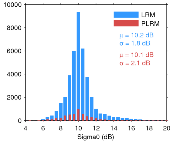
Figure 25. Histogram of flag-valid sigma0 over oceans and lakes for LRM (blue) and PLRM (red) for 11/01/2017. The mean ( \mu ) and standard deviation ( \sigma ) are also shown. Note that values outside [4 20] dB are excluded from the histogram for the sake of readability but not from the computation of \mu and \sigma .
