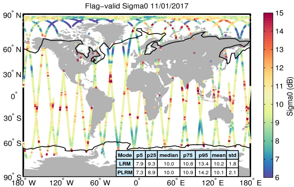
Figure 23. Geographical distribution of flag-valid sigma0 data over oceans and lakes for 11/01/2017. The statistical values shown in the table refer to the sigma0 in dB and are calculated separately for LRM and PLRM regions. Measurements taken over polar polygons have been excluded from the computation of the statistical values. The black lines mark the outer limit of the Arctic and Antarctic polar polygons.
