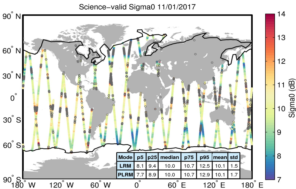
Figure 27. Geographical distribution of science-valid sigma0 data over oceans and lakes for 11/01/2017. The statistical values shown in the table refer to the sigma0 in dB and are calculated separately for LRM and PLRM regions. The black lines mark the outer limit of the Arctic and Antarctic polar polygons. Gray circles denote records that have been rejected based on the editing criteria described in Table 4.
