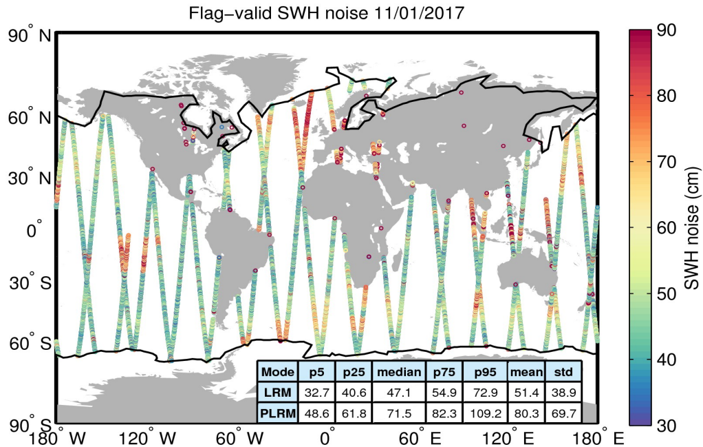
Figure 18. Geographical distribution of flag-valid 20-Hz SWH measurement noise over oceans and lakes for 11/01/2017. The statistical values shown in the table refer to the SWH noise and are calculated separately for LRM and PLRM regions. Measurements taken over polar polygons have been excluded from the computation of the statistical values. The black lines mark the outer limit of the Arctic and Antarctic polar polygons.
