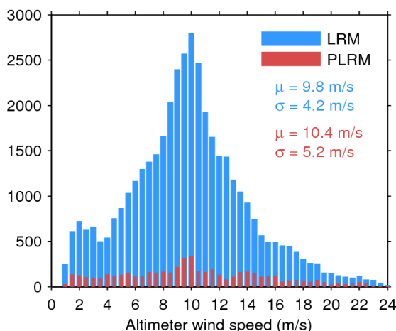
Figure 33. Histogram of flag-valid wind over oceans and lakes for LRM (blue) and PLRM (red) for 11/01/2017. The mean ( \mu ) and standard deviation ( \sigma ) are also shown. Note that values larger than 24 m/s are excluded from the histogram for the sake of readability but not from the computation of \mu and \sigma .
