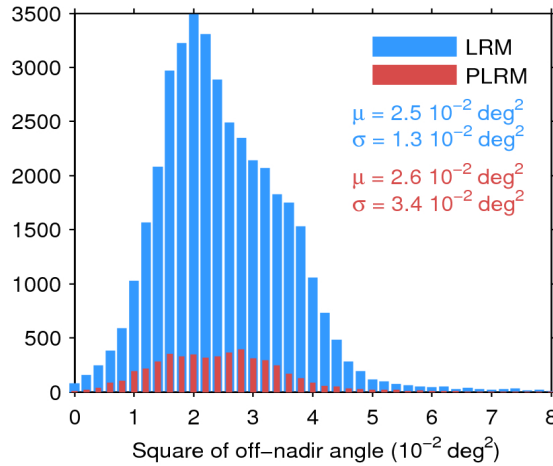
Figure 39. Histogram of flag-valid mispointing over oceans and lakes for LRM (blue) and PLRM (red) for 11/01/2017. Only positive values have been considered. The mean ( \mu ) and standard deviation ( \sigma ) are also shown. Note that values larger than 8 \cdot 10^{-2} \text{ deg}^2 are excluded from the histogram for the sake of readability but not from the computation of \mu and \sigma .
