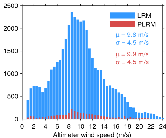
Figure 35. Histogram of science-valid wind over oceans and lakes for LRM (blue) and PLRM (red) for 08/01/2017. The mean ( \mu ) and standard deviation ( \sigma ) are also shown. Note that values larger than 24 m/s are excluded from the histogram for the sake of readability but not from the computation of \mu and \sigma .
