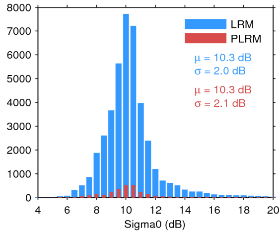
Figure 25. Histogram of flag-valid sigma0 over oceans and lakes for LRM (blue) and PLRM (red) for 08/01/2017. The mean ( \mu ) and standard deviation ( \sigma ) are also shown. Note that values outside [4 20] dB are excluded from the histogram for the sake of readability but not from the computation of \mu and \sigma .
