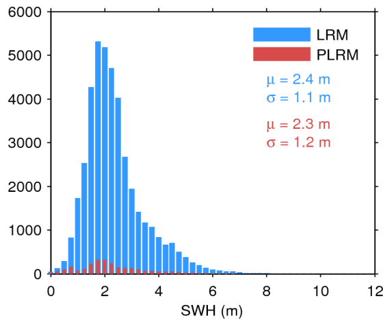
Figure 20. Histogram of science-valid SWH over oceans and lakes for LRM (blue) and PLRM (red) for 08/01/2017. The mean ( \mu ) and standard deviation ( \sigma ) are also shown. Note that values larger than 12 m are excluded from the histogram for the sake of readability but not from the computation of \mu and \sigma .
