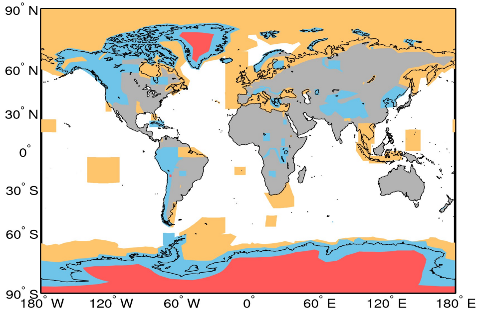
Figure A1. Extent of the regions defining the geographical mode mask for 08/01/2017. The regions where SAR, and SARIn are operated are denoted by the orange and blue polygons, respectively. LRM is operated over areas of the continental ice sheets (red polygons) and over oceans and land not covered by other modes.
