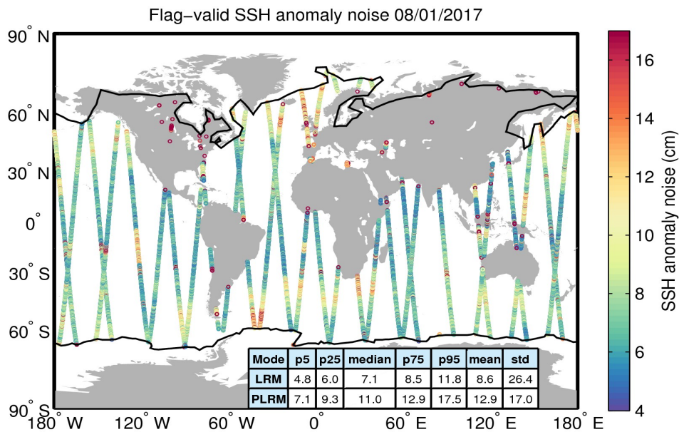
Figure 8. Geographical distribution of flag-valid 20-Hz SSH anomaly measurement noise over oceans and lakes for 08/01/2017. The statistical values shown in the table refer to the SSH anomaly noise and are calculated separately for LRM and PLRM regions. Measurements taken over polar polygons have been excluded from the computation of the statistical values. The black lines mark the outer limit of the Arctic and Antarctic polar polygons.
