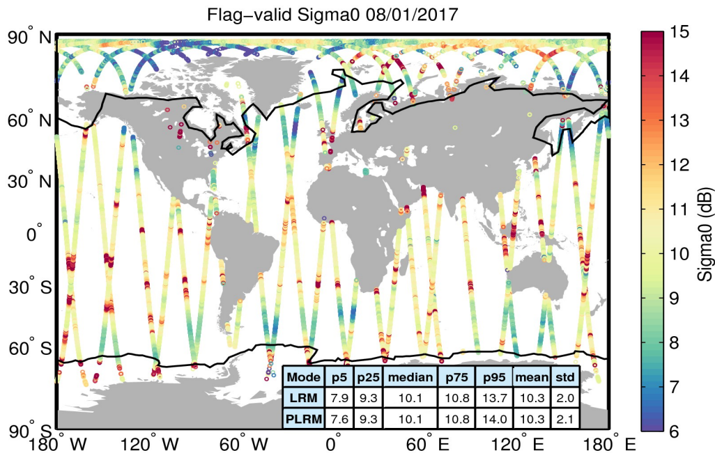
Figure 23. Geographical distribution of flag-valid sigma0 data over oceans and lakes for 08/01/2017. The statistical values shown in the table refer to the sigma0 in dB and are calculated separately for LRM and PLRM regions. Measurements taken over polar polygons have been excluded from the computation of the statistical values. The black lines mark the outer limit of the Arctic and Antarctic polar polygons.
