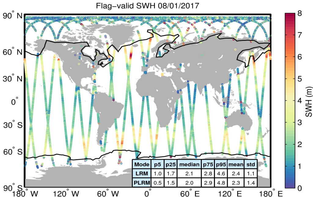
Figure 15. Geographical distribution of flag-valid SWH data over oceans and lakes for 08/01/2017. The statistical values shown in the table refer to the SWH in m and are calculated separately for LRM and PLRM regions. Measurements taken over polar polygons have been excluded from the computation of the statistical values. The black lines mark the outer limit of the Arctic and Antarctic polar polygons.
