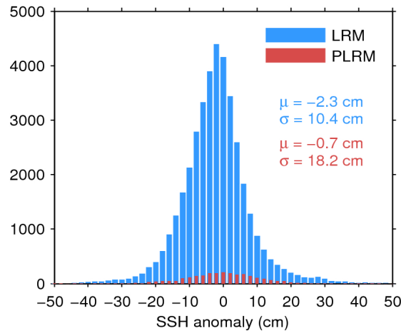
Figure 11. Histogram of science-valid SSH anomaly over oceans and lakes for LRM (blue) and PLRM (red) for 08/01/2017. The mean ( \mu ) and standard deviation ( \sigma ) are also shown. Note that values outside [-50\ 50] cm are excluded from the histogram for the sake of readability but not from the computation of \mu and \sigma .
