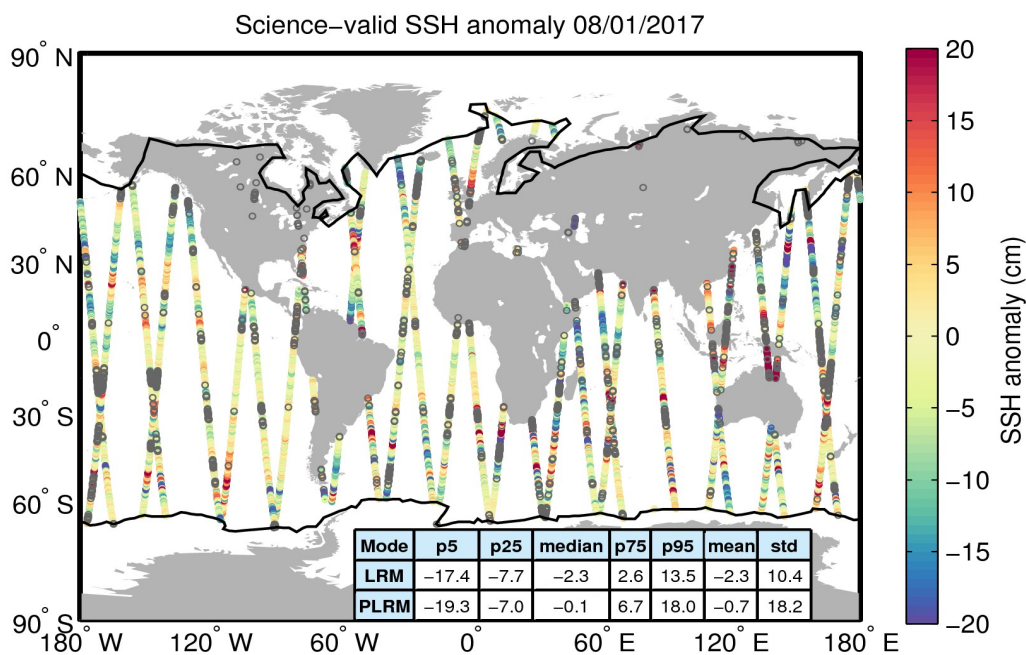
Figure 10. Geographical distribution of science-valid SSH anomaly data over oceans and lakes for 08/01/2017. The statistical values shown in the table refer to the SSH anomaly in cm and are calculated separately for LRM and PLRM regions. The black lines mark the outer limit of the Arctic and Antarctic polar polygons. Gray circles denote records that have been rejected based on the editing criteria described in Table 2.
