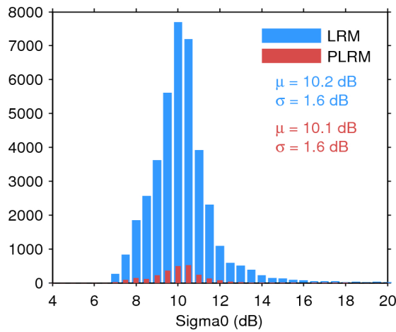
Figure 28. Histogram of science-valid sigma0 over oceans and lakes for LRM (blue) and PLRM (red) for 08/01/2017. The mean ( \mu ) and standard deviation ( \sigma ) are also shown. Note that values outside [4 20] dB are excluded from the histogram for the sake of readability but not from the computation of \mu and \sigma .
