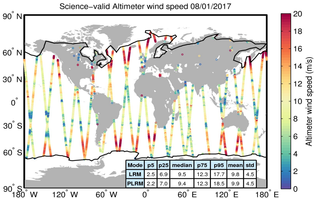
Figure 34. Geographical distribution of science-valid wind data over oceans and lakes for 08/01/2017. The statistical values shown in the table refer to the wind in m/s and are calculated separately for LRM and PLRM regions. The black lines mark the outer limit of the Arctic and Antarctic polar polygons. Gray circles denote records that have been rejected based on the editing criteria described in Table 5.
