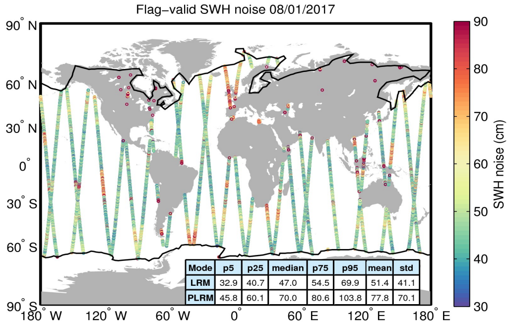
Figure 18. Geographical distribution of flag-valid 20-Hz SWH measurement noise over oceans and lakes for 08/01/2017. The statistical values shown in the table refer to the SWH noise and are calculated separately for LRM and PLRM regions. Measurements taken over polar polygons have been excluded from the computation of the statistical values. The black lines mark the outer limit of the Arctic and Antarctic polar polygons.
