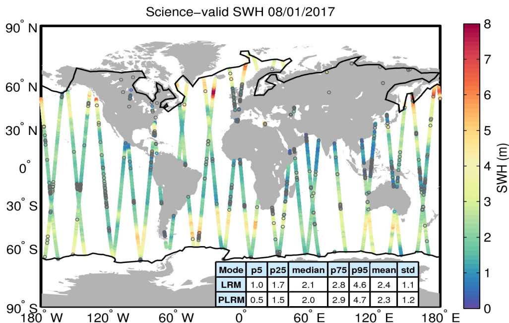
Figure 19. Geographical distribution of science-valid SWH data over oceans and lakes for 08/01/2017. The statistical values shown in the table refer to the SWH in m and are calculated separately for LRM and PLRM regions. The black lines mark the outer limit of the Arctic and Antarctic polar polygons. Gray circles denote records that have been rejected based on the editing criteria described in Table 3.
