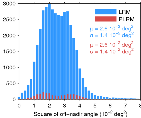
Figure 39. Histogram of flag-valid mispointing over oceans and lakes for LRM (blue) and PLRM (red) for 08/01/2017. Only positive values have been considered. The mean ( \mu ) and standard deviation ( \sigma ) are also shown. Note that values larger than 8 \cdot 10^{-2} \text{ deg}^2 are excluded from the histogram for the sake of readability but not from the computation of \mu and \sigma .
