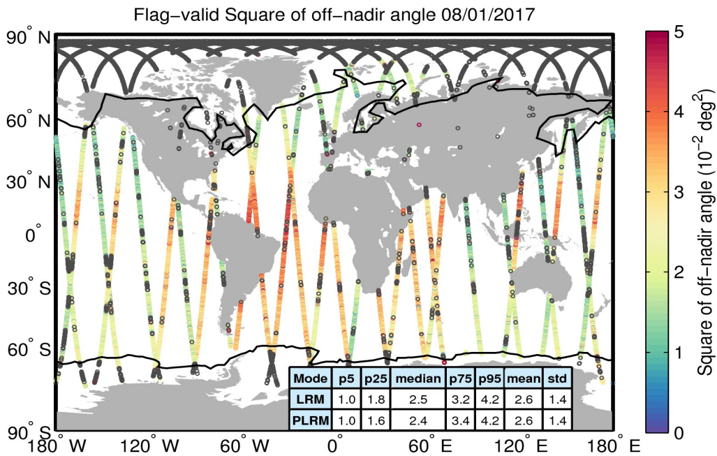
Figure 37. Geographical distribution of flag-valid mispointing data over oceans and lakes for 08/01/2017. The statistical values shown in the table refer to the mispointing in 10^{-2} deg 2 and are calculated separately for LRM and PLRM regions. Measurements taken over polar polygons have been excluded from the computation of the statistical values. The black lines mark the outer limit of the Arctic and Antarctic polar polygons. Gray circles denote negative values.
