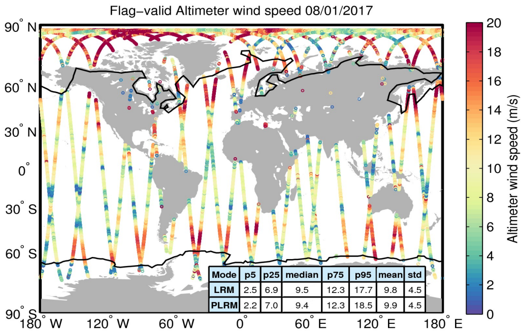
Figure 31. Geographical distribution of flag-valid wind data over oceans and lakes for 08/01/2017. The statistical values shown in the table refer to the wind in m/s and are calculated separately for LRM and PLRM regions. Measurements taken over polar polygons have been excluded from the computation of the statistical values. The black lines mark the outer limit of the Arctic and Antarctic polar polygons.
