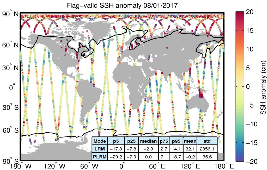
Figure 5. Geographical distribution of flag-valid 1-Hz SSH anomaly data over oceans and lakes for 08/01/2017. The statistical values shown in the table refer to the SSH anomaly in cm and are calculated separately for LRM and PLRM regions. Measurements taken over polar polygons have been excluded from the computation of the statistical values. The black lines mark the outer limit of the Arctic and Antarctic polar polygons.
