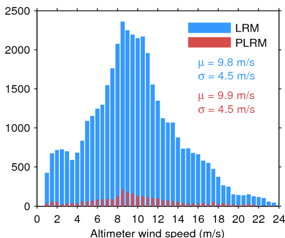
Figure 33. Histogram of flag-valid wind over oceans and lakes for LRM (blue) and PLRM (red) for 08/01/2017. The mean ( \mu ) and standard deviation ( \sigma ) are also shown. Note that values larger than 24 m/s are excluded from the histogram for the sake of readability but not from the computation of \mu and \sigma .
