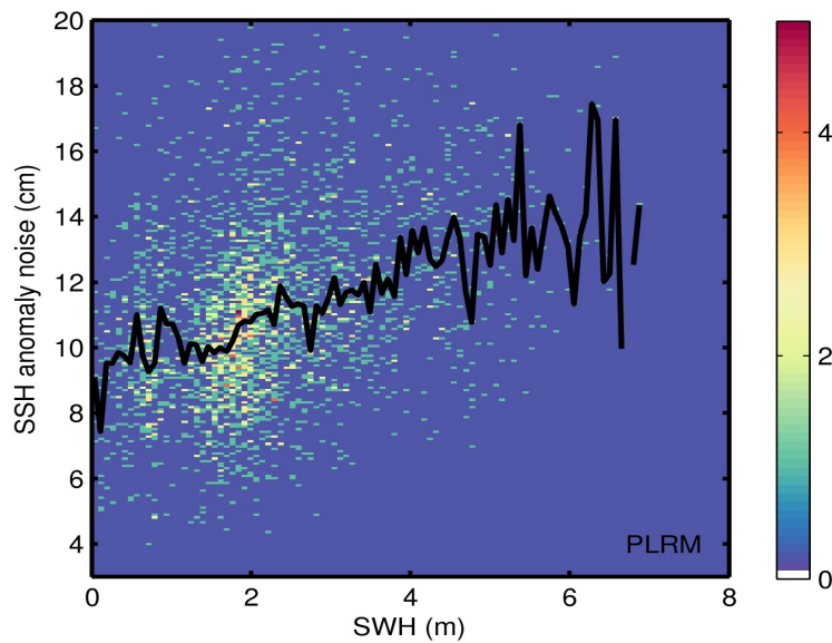
Figure 9. 2D histogram showing flag-valid SSH anomaly noise as a function of SWH for LRM (top) and PLRM (bottom) for 08/01/2017. The black line denotes the median SSH anomaly noise as a function of SWH.
