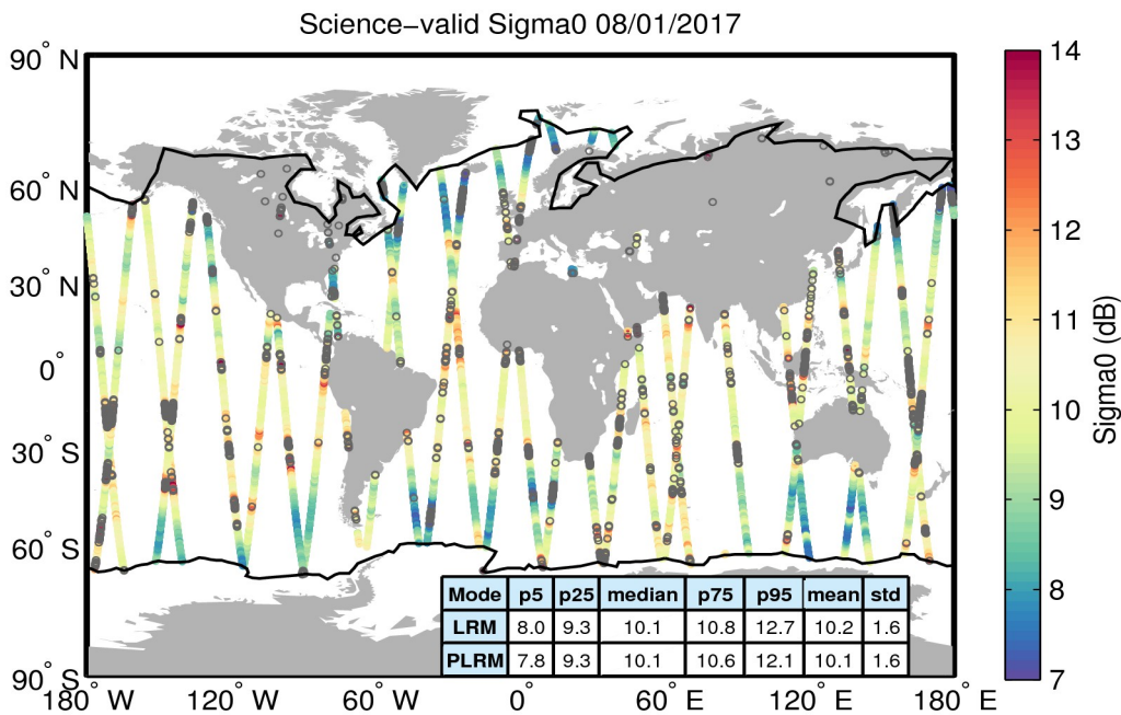
Figure 27. Geographical distribution of science-valid sigma0 data over oceans and lakes for 08/01/2017. The statistical values shown in the table refer to the sigma0 in dB and are calculated separately for LRM and PLRM regions. The black lines mark the outer limit of the Arctic and Antarctic polar polygons. Gray circles denote records that have been rejected based on the editing criteria described in Table 4.
