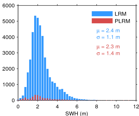
Figure 17. Histogram of flag-valid SWH over oceans and lakes for LRM (blue) and PLRM (red) for 08/01/2017. The mean ( \mu ) and standard deviation ( \sigma ) are also shown. Note that values larger than 12 m are excluded from the histogram for the sake of readability but not from the computation of \mu and \sigma .
