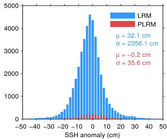
Figure 7. Histogram of flag-valid SSH anomaly over oceans and lakes for LRM (blue) and PLRM (red) for 08/01/2017. The mean ( \mu ) and standard deviation ( \sigma ) are also shown. Note that values outside [-50\ 50] cm are excluded from the histogram for the sake of readability but not from the computation of \mu and \sigma .
