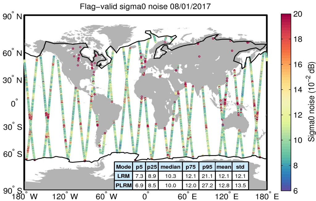
Figure 26. Geographical distribution of flag-valid 20-Hz sigma0 measurement noise over oceans and lakes for 08/01/2017. The statistical values shown in the table refer to the sigma0 noise and are calculated separately for LRM and PLRM regions. Measurements taken over polar polygons have been excluded from the computation of the statistical values. The black lines mark the outer limit of the Arctic and Antarctic polar polygons.
