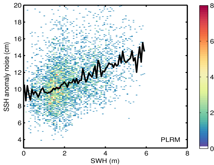
Figure 9. 2D histogram showing flag-valid SSH anomaly noise as a function of SWH for LRM (top) and PLRM (bottom) for 05/01/2017. The black line denotes the median SSH anomaly noise as a function of SWH.
