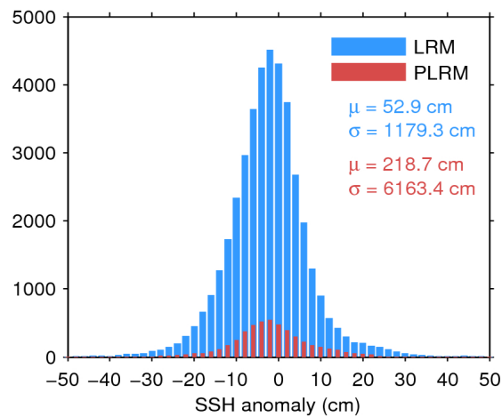
Figure 7. Histogram of flag-valid SSH anomaly over oceans and lakes for LRM (blue) and PLRM (red) for 05/01/2017. The mean ( \mu ) and standard deviation ( \sigma ) are also shown. Note that values outside [-50 50] cm are excluded from the histogram for the sake of readability but not from the computation of \mu and \sigma .
