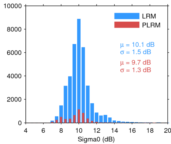
Figure 28. Histogram of science-valid sigma0 over oceans and lakes for LRM (blue) and PLRM (red) for 05/01/2017. The mean ( \mu ) and standard deviation ( \sigma ) are also shown. Note that values outside [4 20] dB are excluded from the histogram for the sake of readability but not from the computation of \mu and \sigma .
