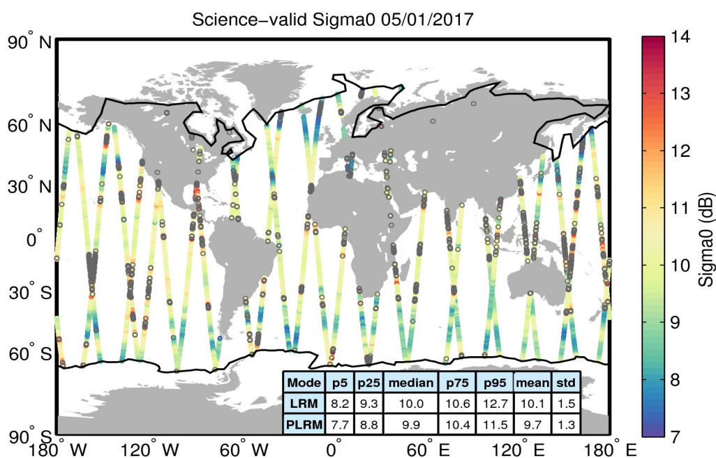
Figure 27. Geographical distribution of science-valid sigma0 data over oceans and lakes for 05/01/2017. The statistical values shown in the table refer to the sigma0 in dB and are calculated separately for LRM and PLRM regions. The black lines mark the outer limit of the Arctic and Antarctic polar polygons. Gray circles denote records that have been rejected based on the editing criteria described in Table 4.
