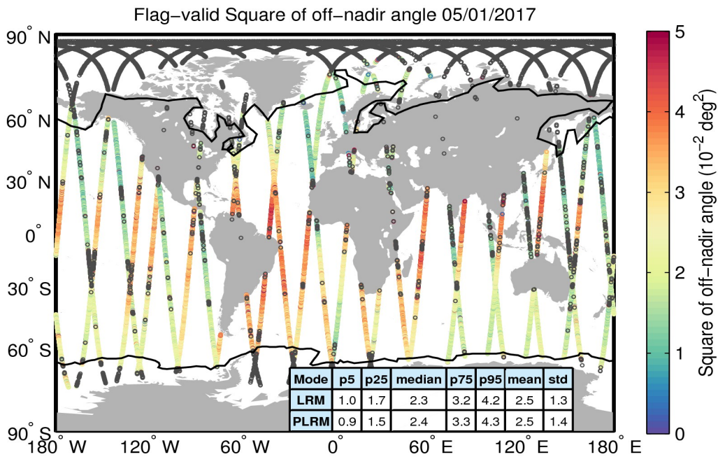
Figure 37. Geographical distribution of flag-valid mispointing data over oceans and lakes for 05/01/2017. The statistical values shown in the table refer to the mispointing in 10^{-2} deg 2 and are calculated separately for LRM and PLRM regions. Measurements taken over polar polygons have been excluded from the computation of the statistical values. The black lines mark the outer limit of the Arctic and Antarctic polar polygons. Gray circles denote negative values.
