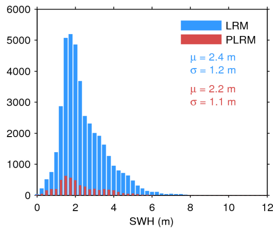
Figure 20. Histogram of science-valid SWH over oceans and lakes for LRM (blue) and PLRM (red) for 05/01/2017. The mean ( \mu ) and standard deviation ( \sigma ) are also shown. Note that values larger than 12 m are excluded from the histogram for the sake of readability but not from the computation of \mu and \sigma .
