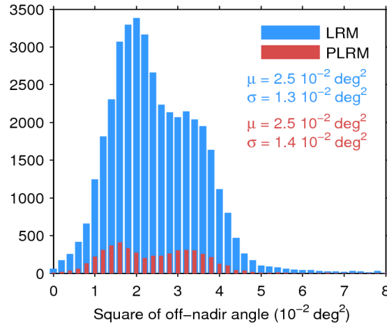
Figure 39. Histogram of flag-valid mispointing over oceans and lakes for LRM (blue) and PLRM (red) for 05/01/2017. Only positive values have been considered. The mean ( \mu ) and standard deviation ( \sigma ) are also shown. Note that values larger than 8 \cdot 10^{-2} \text{ deg}^2 are excluded from the histogram for the sake of readability but not from the computation of \mu and \sigma .
