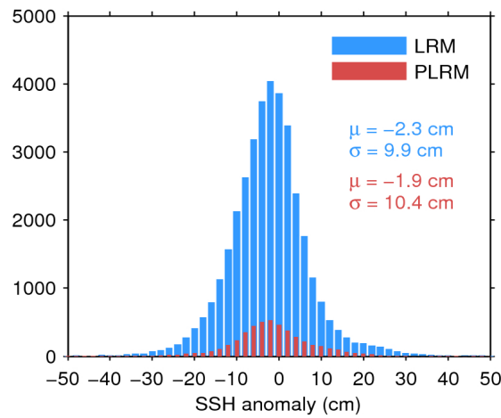
Figure 11. Histogram of science-valid SSH anomaly over oceans and lakes for LRM (blue) and PLRM (red) for 05/01/2017. The mean ( \mu ) and standard deviation ( \sigma ) are also shown. Note that values outside [-50\ 50] cm are excluded from the histogram for the sake of readability but not from the computation of \mu and \sigma .
