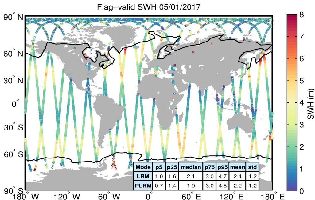
Figure 15. Geographical distribution of flag-valid SWH data over oceans and lakes for 05/01/2017. The statistical values shown in the table refer to the SWH in m and are calculated separately for LRM and PLRM regions. Measurements taken over polar polygons have been excluded from the computation of the statistical values. The black lines mark the outer limit of the Arctic and Antarctic polar polygons.
