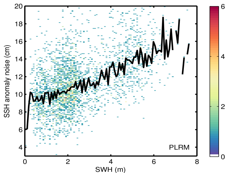
Figure 9. 2D histogram showing flag-valid SSH anomaly noise as a function of SWH for LRM (top) and PLRM (bottom) for 04/01/2017. The black line denotes the median SSH anomaly noise as a function of SWH.
