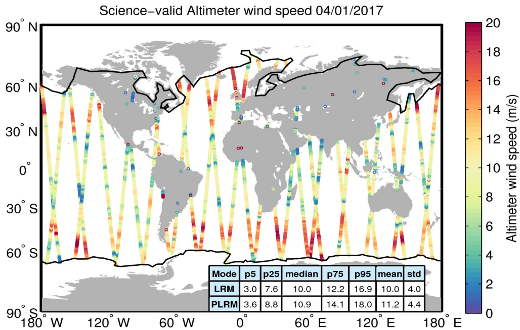
Figure 34. Geographical distribution of science-valid wind data over oceans and lakes for 04/01/2017. The statistical values shown in the table refer to the wind in m/s and are calculated separately for LRM and PLRM regions. The black lines mark the outer limit of the Arctic and Antarctic polar polygons. Gray circles denote records that have been rejected based on the editing criteria described in Table 5.
