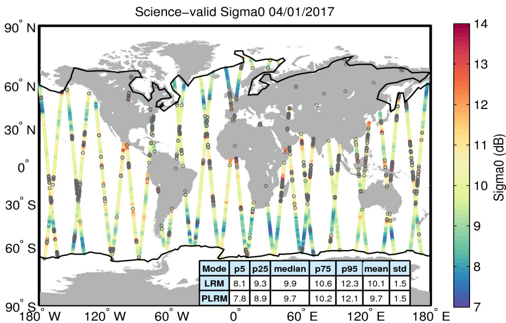
Figure 27. Geographical distribution of science-valid sigma0 data over oceans and lakes for 04/01/2017. The statistical values shown in the table refer to the sigma0 in dB and are calculated separately for LRM and PLRM regions. The black lines mark the outer limit of the Arctic and Antarctic polar polygons. Gray circles denote records that have been rejected based on the editing criteria described in Table 4.
