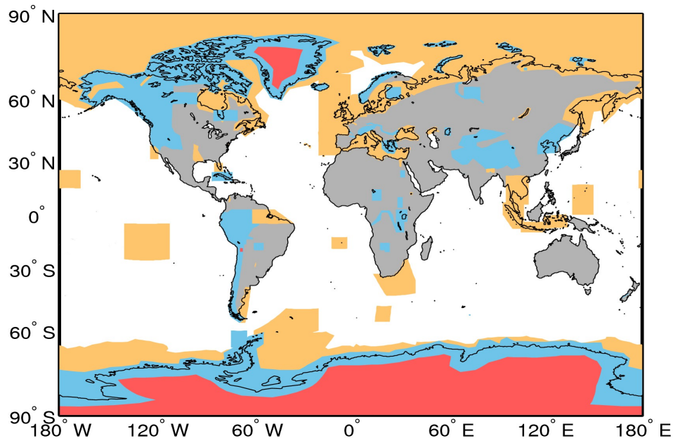
Figure A1. Extent of the regions defining the geographical mode mask for 04/01/2017. The regions where SAR, and SARIn are operated are denoted by the orange and blue polygons, respectively. LRM is operated over areas of the continental ice sheets (red polygons) and over oceans and land not covered by other modes.
