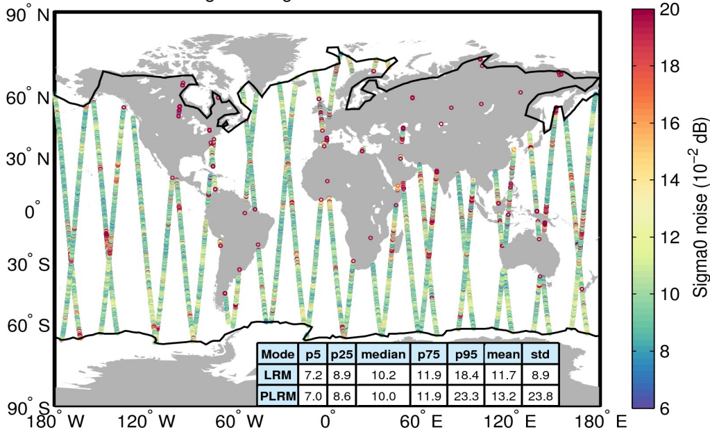
Flag-valid sigma0 noise 04/01/2017
