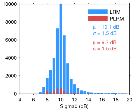
Figure 28. Histogram of science-valid sigma0 over oceans and lakes for LRM (blue) and PLRM (red) for 04/01/2017. The mean ( \mu ) and standard deviation ( \sigma ) are also shown. Note that values outside [4 20] dB are excluded from the histogram for the sake of readability but not from the computation of \mu and \sigma .
