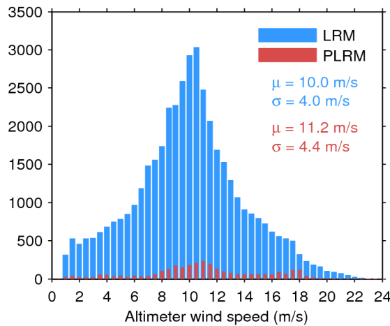
Figure 33. Histogram of flag-valid wind over oceans and lakes for LRM (blue) and PLRM (red) for 04/01/2017. The mean ( \mu ) and standard deviation ( \sigma ) are also shown. Note that values larger than 24 m/s are excluded from the histogram for the sake of readability but not from the computation of \mu and \sigma .
