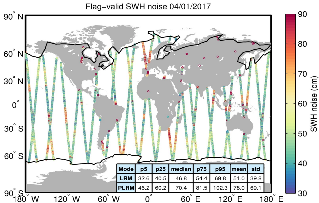
Figure 18. Geographical distribution of flag-valid 20-Hz SWH measurement noise over oceans and lakes for 04/01/2017. The statistical values shown in the table refer to the SWH noise and are calculated separately for LRM and PLRM regions. Measurements taken over polar polygons have been excluded from the computation of the statistical values. The black lines mark the outer limit of the Arctic and Antarctic polar polygons.
