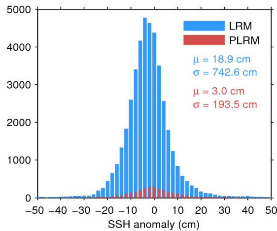
Figure 7. Histogram of flag-valid SSH anomaly over oceans and lakes for LRM (blue) and PLRM (red) for 04/01/2017. The mean ( \mu ) and standard deviation ( \sigma ) are also shown. Note that values outside [-50 50] cm are excluded from the histogram for the sake of readability but not from the computation of \mu and \sigma .
