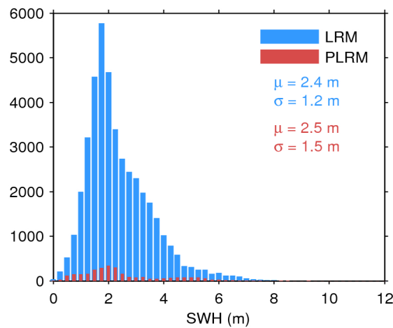
Figure 20. Histogram of science-valid SWH over oceans and lakes for LRM (blue) and PLRM (red) for 04/01/2017. The mean ( \mu ) and standard deviation ( \sigma ) are also shown. Note that values larger than 12 m are excluded from the histogram for the sake of readability but not from the computation of \mu and \sigma .
