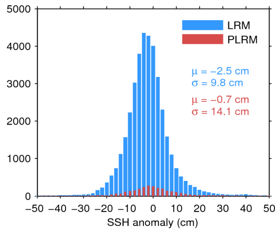
Figure 11. Histogram of science-valid SSH anomaly over oceans and lakes for LRM (blue) and PLRM (red) for 04/01/2017. The mean ( \mu ) and standard deviation ( \sigma ) are also shown. Note that values outside [-50\ 50] cm are excluded from the histogram for the sake of readability but not from the computation of \mu and \sigma .
