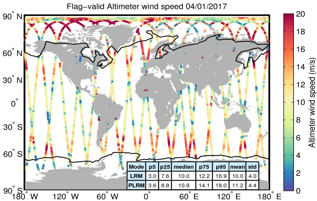
Figure 31. Geographical distribution of flag-valid wind data over oceans and lakes for 04/01/2017. The statistical values shown in the table refer to the wind in m/s and are calculated separately for LRM and PLRM regions. Measurements taken over polar polygons have been excluded from the computation of the statistical values. The black lines mark the outer limit of the Arctic and Antarctic polar polygons.
