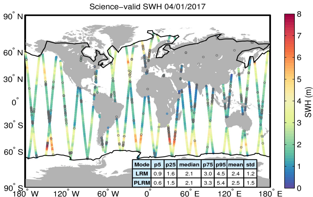
Figure 19. Geographical distribution of science-valid SWH data over oceans and lakes for 04/01/2017. The statistical values shown in the table refer to the SWH in m and are calculated separately for LRM and PLRM regions. The black lines mark the outer limit of the Arctic and Antarctic polar polygons. Gray circles denote records that have been rejected based on the editing criteria described in Table 3.
