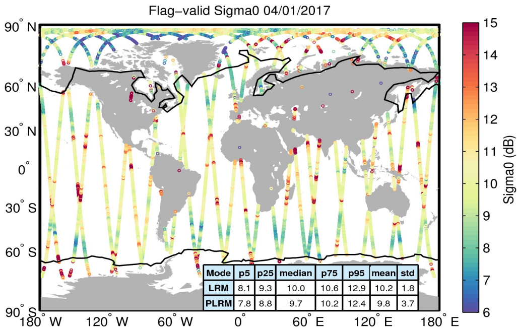
Figure 23. Geographical distribution of flag-valid sigma0 data over oceans and lakes for 04/01/2017. The statistical values shown in the table refer to the sigma0 in dB and are calculated separately for LRM and PLRM regions. Measurements taken over polar polygons have been excluded from the computation of the statistical values. The black lines mark the outer limit of the Arctic and Antarctic polar polygons.
