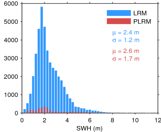
Figure 17. Histogram of flag-valid SWH over oceans and lakes for LRM (blue) and PLRM (red) for 04/01/2017. The mean ( \mu ) and standard deviation ( \sigma ) are also shown. Note that values larger than 12 m are excluded from the histogram for the sake of readability but not from the computation of \mu and \sigma .
