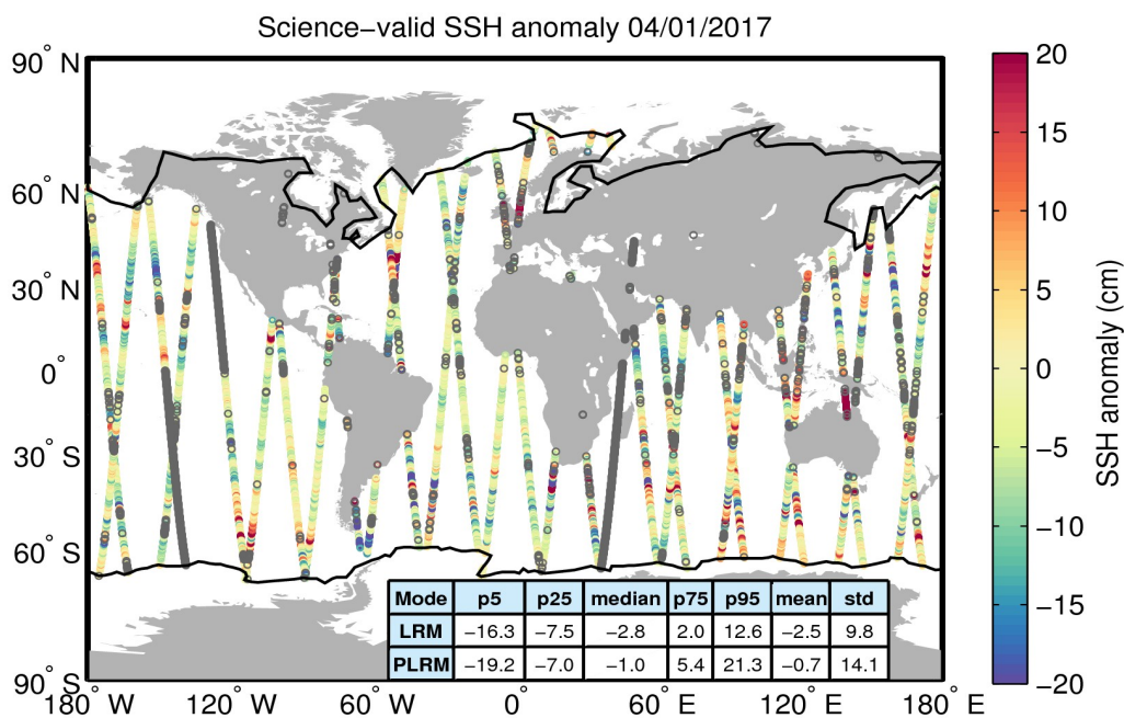
Figure 10. Geographical distribution of science-valid SSH anomaly data over oceans and lakes for 04/01/2017. The statistical values shown in the table refer to the SSH anomaly in cm and are calculated separately for LRM and PLRM regions. The black lines mark the outer limit of the Arctic and Antarctic polar polygons. Gray circles denote records that have been rejected based on the editing criteria described in Table 2.
