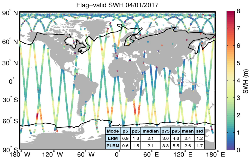
Figure 15. Geographical distribution of flag-valid SWH data over oceans and lakes for 04/01/2017. The statistical values shown in the table refer to the SWH in m and are calculated separately for LRM and PLRM regions. Measurements taken over polar polygons have been excluded from the computation of the statistical values. The black lines mark the outer limit of the Arctic and Antarctic polar polygons.
