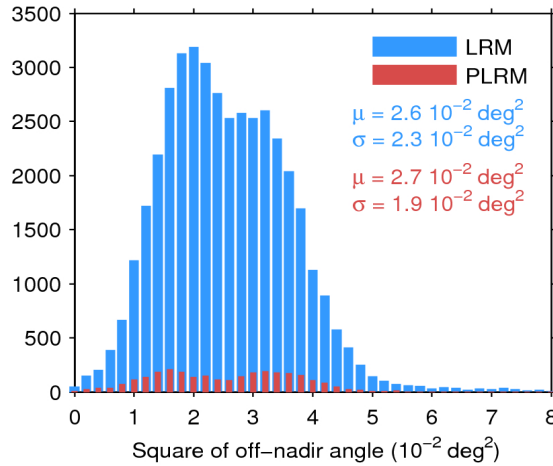
Figure 39. Histogram of flag-valid mispointing over oceans and lakes for LRM (blue) and PLRM (red) for 04/01/2017. Only positive values have been considered. The mean ( \mu ) and standard deviation ( \sigma ) are also shown. Note that values larger than 8 \cdot 10^{-2} \text{ deg}^2 are excluded from the histogram for the sake of readability but not from the computation of \mu and \sigma .
