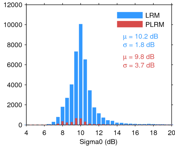
Figure 25. Histogram of flag-valid sigma0 over oceans and lakes for LRM (blue) and PLRM (red) for 04/01/2017. The mean ( \mu ) and standard deviation ( \sigma ) are also shown. Note that values outside [4 20] dB are excluded from the histogram for the sake of readability but not from the computation of \mu and \sigma .
