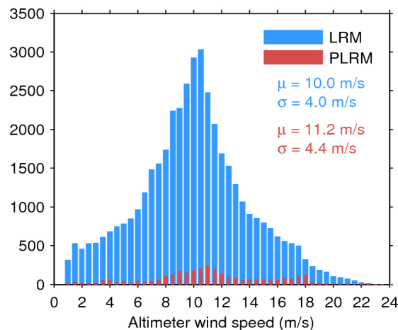
Figure 35. Histogram of science-valid wind over oceans and lakes for LRM (blue) and PLRM (red) for 04/01/2017. The mean ( \mu ) and standard deviation ( \sigma ) are also shown. Note that values larger than 24 m/s are excluded from the histogram for the sake of readability but not from the computation of \mu and \sigma .
