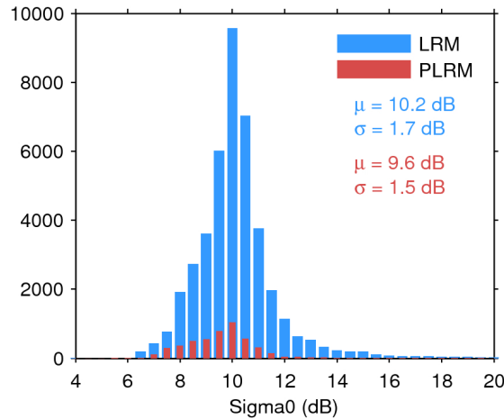
Figure 25. Histogram of flag-valid sigma0 over oceans and lakes for LRM (blue) and PLRM (red) for 03/01/2017. The mean ( \mu ) and standard deviation ( \sigma ) are also shown. Note that values outside [4 20] dB are excluded from the histogram for the sake of readability but not from the computation of \mu and \sigma .
