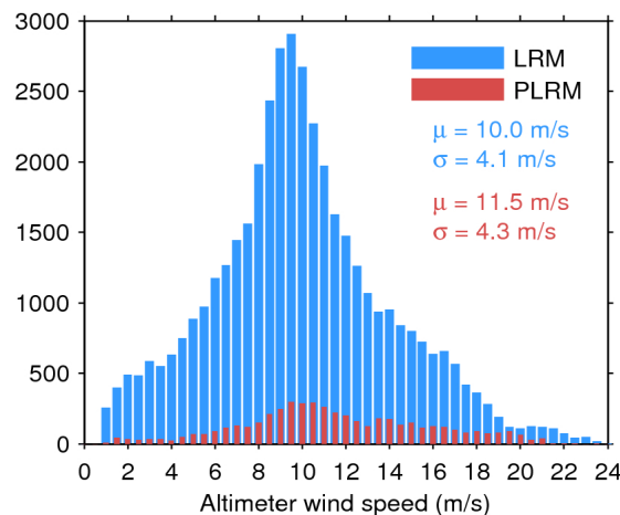
Figure 35. Histogram of science-valid wind over oceans and lakes for LRM (blue) and PLRM (red) for 03/01/2017. The mean ( \mu ) and standard deviation ( \sigma ) are also shown. Note that values larger than 24 m/s are excluded from the histogram for the sake of readability but not from the computation of \mu and \sigma .
