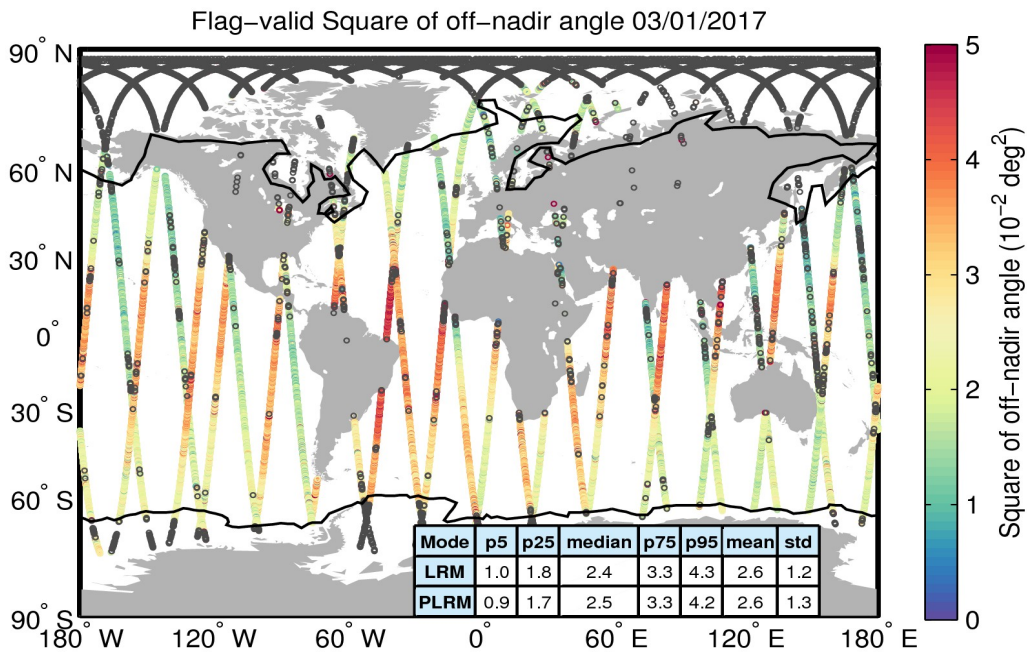
Figure 37. Geographical distribution of flag-valid mispointing data over oceans and lakes for 03/01/2017. The statistical values shown in the table refer to the mispointing in 10^{-2} deg 2 and are calculated separately for LRM and PLRM regions. Measurements taken over polar polygons have been excluded from the computation of the statistical values. The black lines mark the outer limit of the Arctic and Antarctic polar polygons. Gray circles denote negative values.
