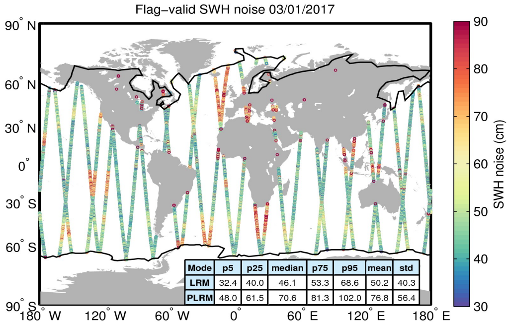
Figure 18. Geographical distribution of flag-valid 20-Hz SWH measurement noise over oceans and lakes for 03/01/2017. The statistical values shown in the table refer to the SWH noise and are calculated separately for LRM and PLRM regions. Measurements taken over polar polygons have been excluded from the computation of the statistical values. The black lines mark the outer limit of the Arctic and Antarctic polar polygons.
