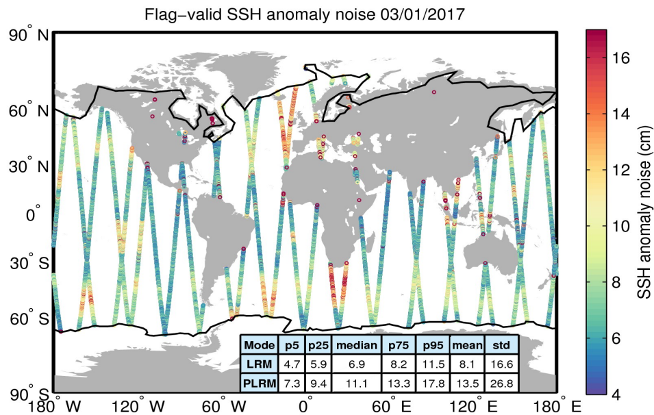
Figure 8. Geographical distribution of flag-valid 20-Hz SSH anomaly measurement noise over oceans and lakes for 03/01/2017. The statistical values shown in the table refer to the SSH anomaly noise and are calculated separately for LRM and PLRM regions. Measurements taken over polar polygons have been excluded from the computation of the statistical values. The black lines mark the outer limit of the Arctic and Antarctic polar polygons.
