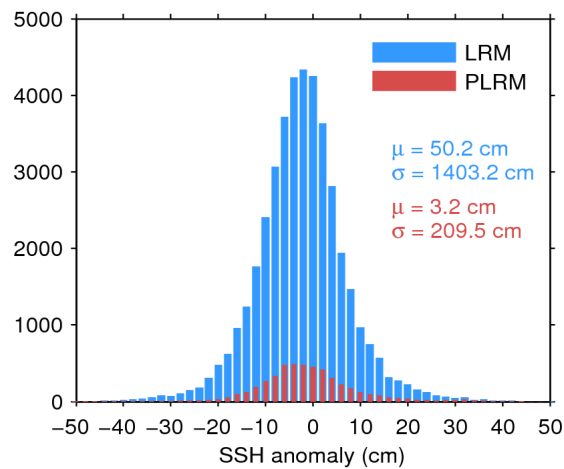
Figure 7. Histogram of flag-valid SSH anomaly over oceans and lakes for LRM (blue) and PLRM (red) for 03/01/2017. The mean ( \mu ) and standard deviation ( \sigma ) are also shown. Note that values outside [-50\ 50] cm are excluded from the histogram for the sake of readability but not from the computation of \mu and \sigma .
