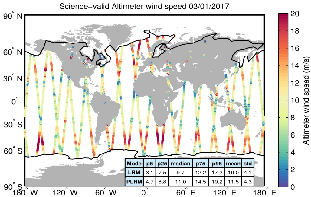
Figure 34. Geographical distribution of science-valid wind data over oceans and lakes for 03/01/2017. The statistical values shown in the table refer to the wind in m/s and are calculated separately for LRM and PLRM regions. The black lines mark the outer limit of the Arctic and Antarctic polar polygons. Gray circles denote records that have been rejected based on the editing criteria described in Table 5.
