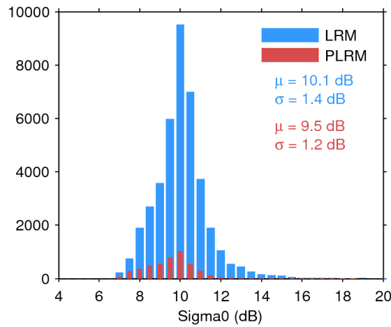
Figure 28. Histogram of science-valid sigma0 over oceans and lakes for LRM (blue) and PLRM (red) for 03/01/2017. The mean ( \mu ) and standard deviation ( \sigma ) are also shown. Note that values outside [4 20] dB are excluded from the histogram for the sake of readability but not from the computation of \mu and \sigma .
