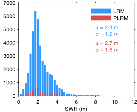
Figure 17. Histogram of flag-valid SWH over oceans and lakes for LRM (blue) and PLRM (red) for 03/01/2017. The mean ( \mu ) and standard deviation ( \sigma ) are also shown. Note that values larger than 12 m are excluded from the histogram for the sake of readability but not from the computation of \mu and \sigma .
