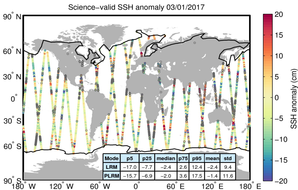
Figure 10. Geographical distribution of science-valid SSH anomaly data over oceans and lakes for 03/01/2017. The statistical values shown in the table refer to the SSH anomaly in cm and are calculated separately for LRM and PLRM regions. The black lines mark the outer limit of the Arctic and Antarctic polar polygons. Gray circles denote records that have been rejected based on the editing criteria described in Table 2.
