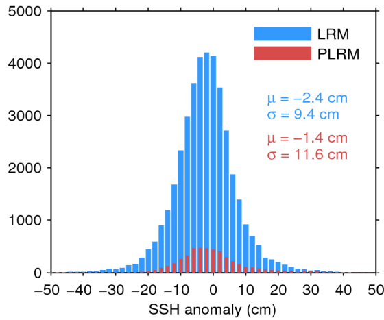
Figure 11. Histogram of science-valid SSH anomaly over oceans and lakes for LRM (blue) and PLRM (red) for 03/01/2017. The mean ( \mu ) and standard deviation ( \sigma ) are also shown. Note that values outside [-50\ 50] cm are excluded from the histogram for the sake of readability but not from the computation of \mu and \sigma .
