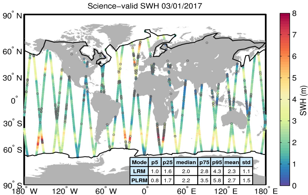
Figure 19. Geographical distribution of science-valid SWH data over oceans and lakes for 03/01/2017. The statistical values shown in the table refer to the SWH in m and are calculated separately for LRM and PLRM regions. The black lines mark the outer limit of the Arctic and Antarctic polar polygons. Gray circles denote records that have been rejected based on the editing criteria described in Table 3.
