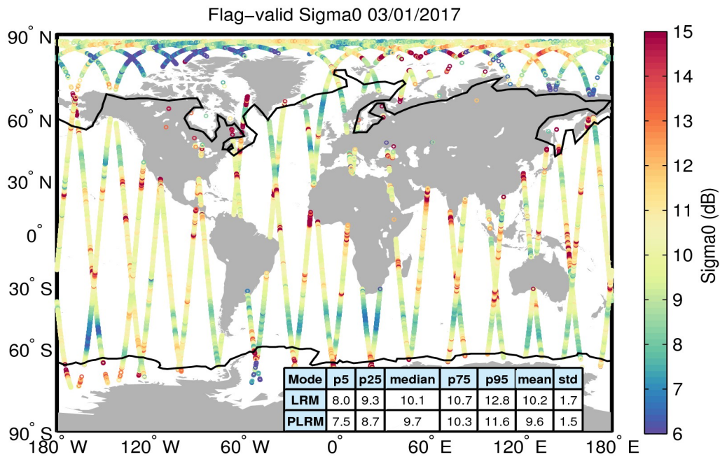
Figure 23. Geographical distribution of flag-valid sigma0 data over oceans and lakes for 03/01/2017. The statistical values shown in the table refer to the sigma0 in dB and are calculated separately for LRM and PLRM regions. Measurements taken over polar polygons have been excluded from the computation of the statistical values. The black lines mark the outer limit of the Arctic and Antarctic polar polygons.
