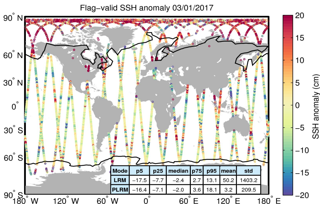
Figure 5. Geographical distribution of flag-valid 1-Hz SSH anomaly data over oceans and lakes for 03/01/2017. The statistical values shown in the table refer to the SSH anomaly in cm and are calculated separately for LRM and PLRM regions. Measurements taken over polar polygons have been excluded from the computation of the statistical values. The black lines mark the outer limit of the Arctic and Antarctic polar polygons.
