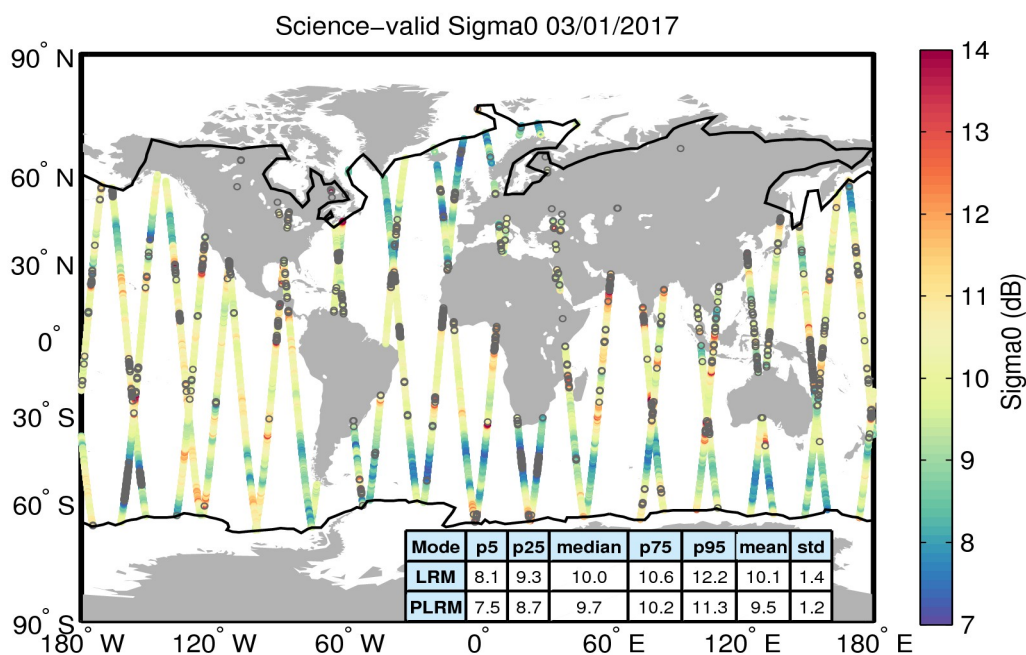
Figure 27. Geographical distribution of science-valid sigma0 data over oceans and lakes for 03/01/2017. The statistical values shown in the table refer to the sigma0 in dB and are calculated separately for LRM and PLRM regions. The black lines mark the outer limit of the Arctic and Antarctic polar polygons. Gray circles denote records that have been rejected based on the editing criteria described in Table 4.
