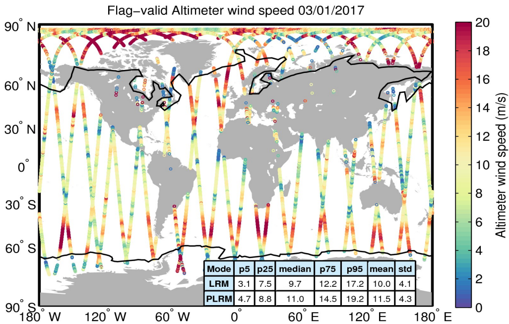
Figure 31. Geographical distribution of flag-valid wind data over oceans and lakes for 03/01/2017. The statistical values shown in the table refer to the wind in m/s and are calculated separately for LRM and PLRM regions. Measurements taken over polar polygons have been excluded from the computation of the statistical values. The black lines mark the outer limit of the Arctic and Antarctic polar polygons.
