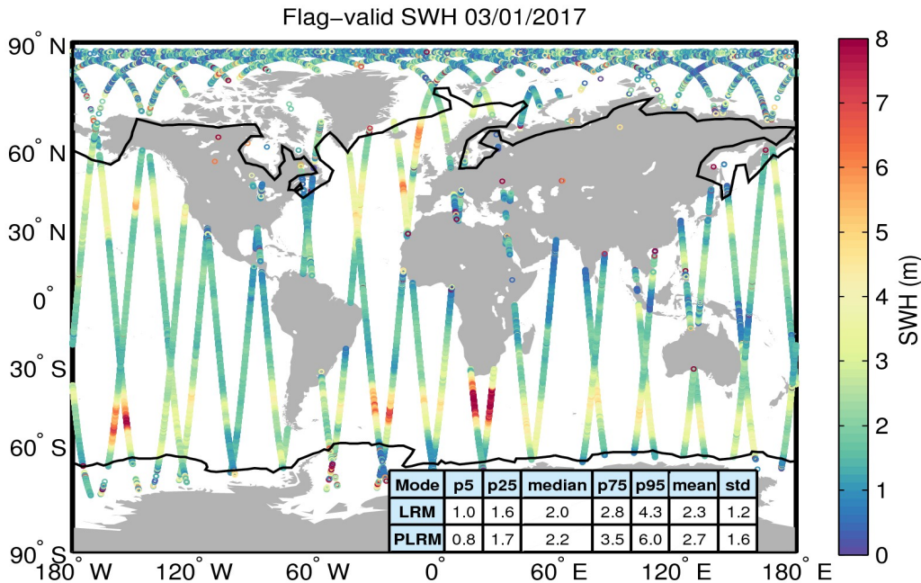
Figure 15. Geographical distribution of flag-valid SWH data over oceans and lakes for 03/01/2017. The statistical values shown in the table refer to the SWH in m and are calculated separately for LRM and PLRM regions. Measurements taken over polar polygons have been excluded from the computation of the statistical values. The black lines mark the outer limit of the Arctic and Antarctic polar polygons.
