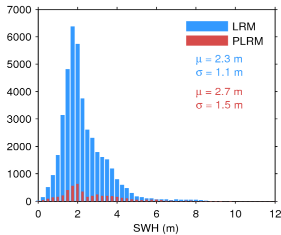
Figure 20. Histogram of science-valid SWH over oceans and lakes for LRM (blue) and PLRM (red) for 03/01/2017. The mean ( \mu ) and standard deviation ( \sigma ) are also shown. Note that values larger than 12 m are excluded from the histogram for the sake of readability but not from the computation of \mu and \sigma .
