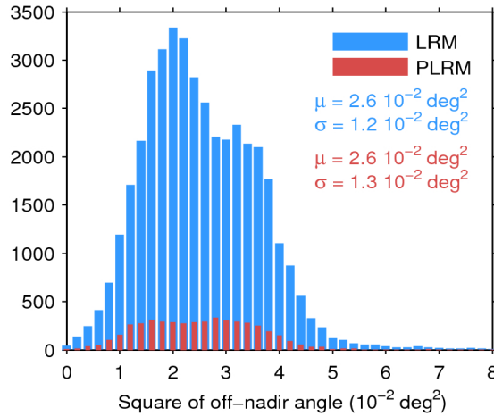
Figure 39. Histogram of flag-valid mispointing over oceans and lakes for LRM (blue) and PLRM (red) for 03/01/2017. Only positive values have been considered. The mean ( \mu ) and standard deviation ( \sigma ) are also shown. Note that values larger than 8 \cdot 10^{-2} \text{ deg}^2 are excluded from the histogram for the sake of readability but not from the computation of \mu and \sigma .
