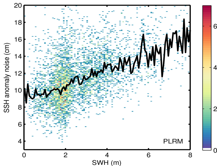
Figure 9. 2D histogram showing flag-valid SSH anomaly noise as a function of SWH for LRM (top) and PLRM (bottom) for 03/01/2017. The black line denotes the median SSH anomaly noise as a function of SWH.
