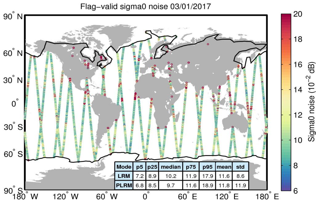
Figure 26. Geographical distribution of flag-valid 20-Hz sigma0 measurement noise over oceans and lakes for 03/01/2017. The statistical values shown in the table refer to the sigma0 noise and are calculated separately for LRM and PLRM regions. Measurements taken over polar polygons have been excluded from the computation of the statistical values. The black lines mark the outer limit of the Arctic and Antarctic polar polygons.
