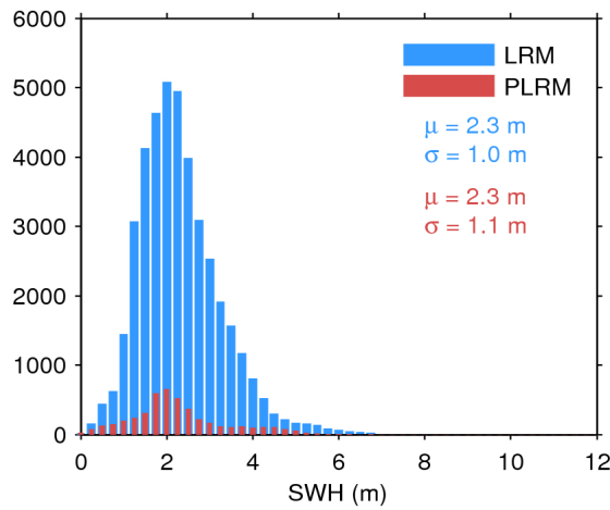
Figure 20. Histogram of science-valid SWH over oceans and lakes for LRM (blue) and PLRM (red) for 01/01/2017. The mean ( \mu ) and standard deviation ( \sigma ) are also shown. Note that values larger than 12 m are excluded from the histogram for the sake of readability but not from the computation of \mu and \sigma .
