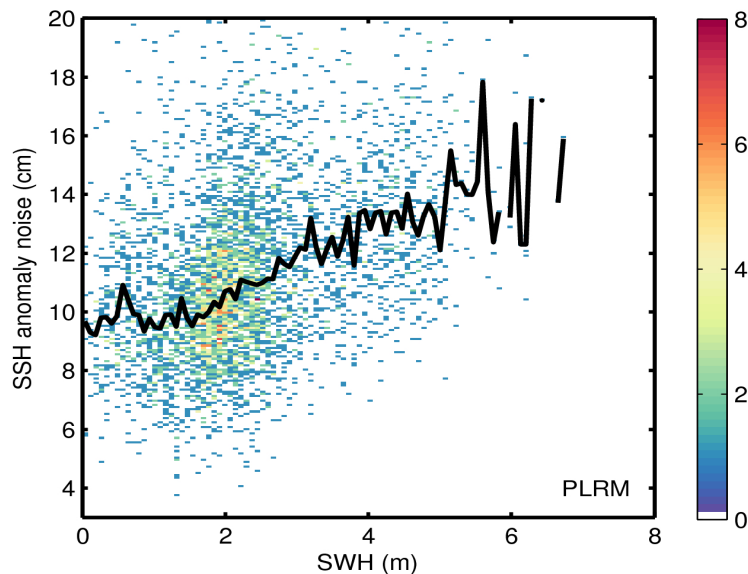
Figure 9. 2D histogram showing flag-valid SSH anomaly noise as a function of SWH for LRM (top) and PLRM (bottom) for 01/01/2017. The black line denotes the median SSH anomaly noise as a function of SWH.
