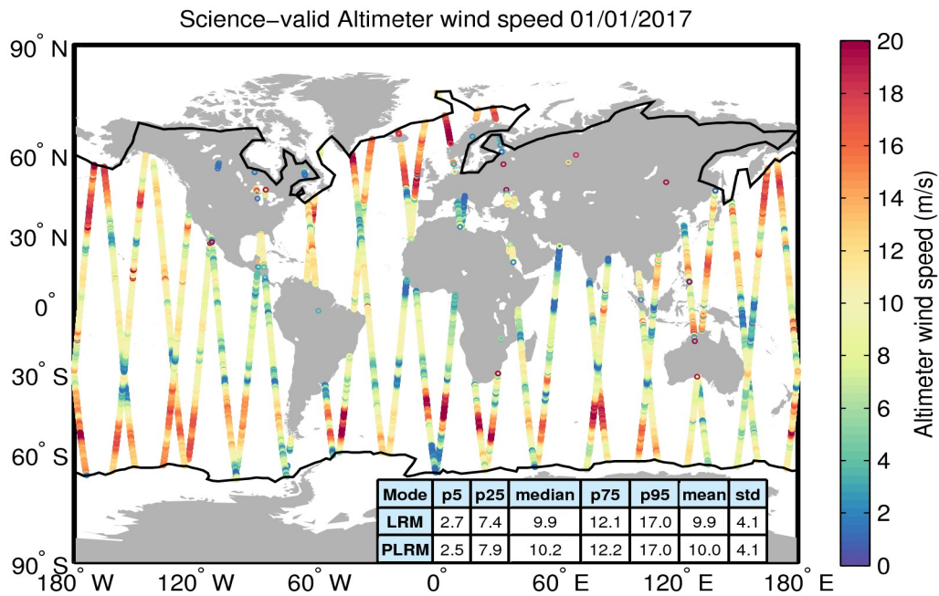
Figure 34. Geographical distribution of science-valid wind data over oceans and lakes for 01/01/2017. The statistical values shown in the table refer to the wind in m/s and are calculated separately for LRM and PLRM regions. The black lines mark the outer limit of the Arctic and Antarctic polar polygons. Gray circles denote records that have been rejected based on the editing criteria described in Table 5.
