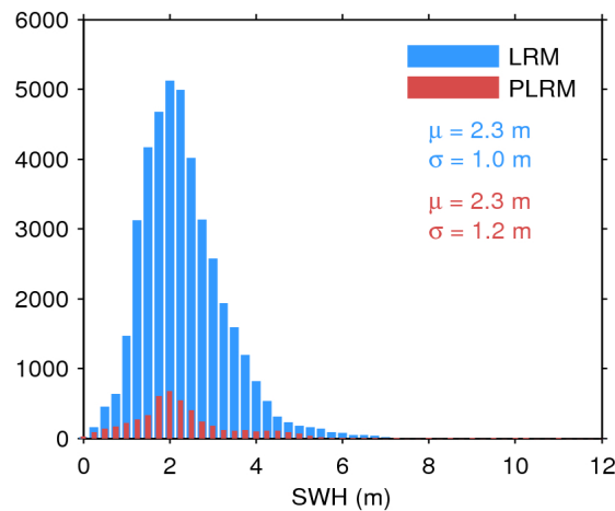
Figure 17. Histogram of flag-valid SWH over oceans and lakes for LRM (blue) and PLRM (red) for 01/01/2017. The mean ( \mu ) and standard deviation ( \sigma ) are also shown. Note that values larger than 12 m are excluded from the histogram for the sake of readability but not from the computation of \mu and \sigma .
