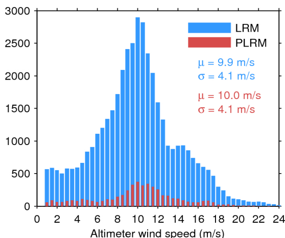
Figure 33. Histogram of flag-valid wind over oceans and lakes for LRM (blue) and PLRM (red) for 01/01/2017. The mean ( \mu ) and standard deviation ( \sigma ) are also shown. Note that values larger than 24 m/s are excluded from the histogram for the sake of readability but not from the computation of \mu and \sigma .
