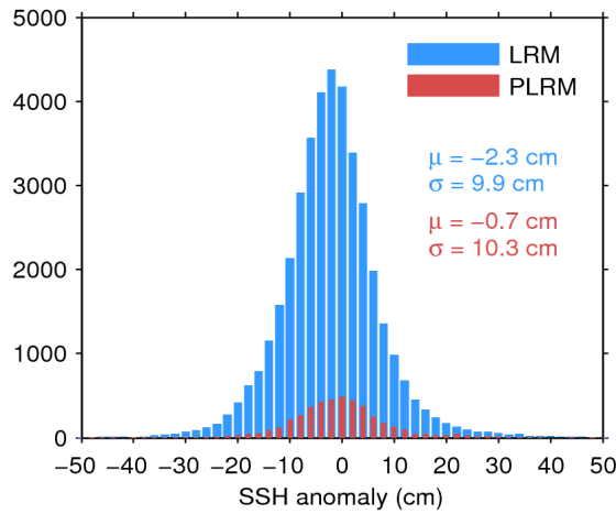
Figure 11. Histogram of science-valid SSH anomaly over oceans and lakes for LRM (blue) and PLRM (red) for 01/01/2017. The mean ( \mu ) and standard deviation ( \sigma ) are also shown. Note that values outside [-50\ 50] cm are excluded from the histogram for the sake of readability but not from the computation of \mu and \sigma .
