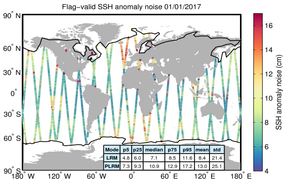
Figure 8. Geographical distribution of flag-valid 20-Hz SSH anomaly measurement noise over oceans and lakes for 01/01/2017. The statistical values shown in the table refer to the SSH anomaly noise and are calculated separately for LRM and PLRM regions. Measurements taken over polar polygons have been excluded from the computation of the statistical values. The black lines mark the outer limit of the Arctic and Antarctic polar polygons.
