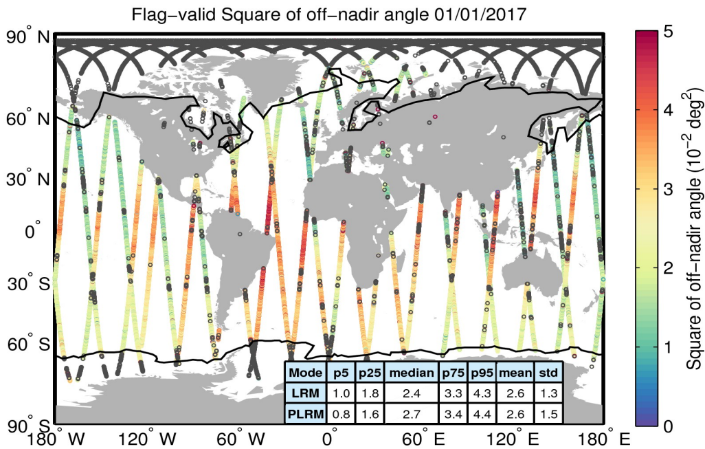
Figure 37. Geographical distribution of flag-valid mispointing data over oceans and lakes for 01/01/2017. The statistical values shown in the table refer to the mispointing in 10^{-2} deg 2 and are calculated separately for LRM and PLRM regions. Measurements taken over polar polygons have been excluded from the computation of the statistical values. The black lines mark the outer limit of the Arctic and Antarctic polar polygons. Gray circles denote negative values.
