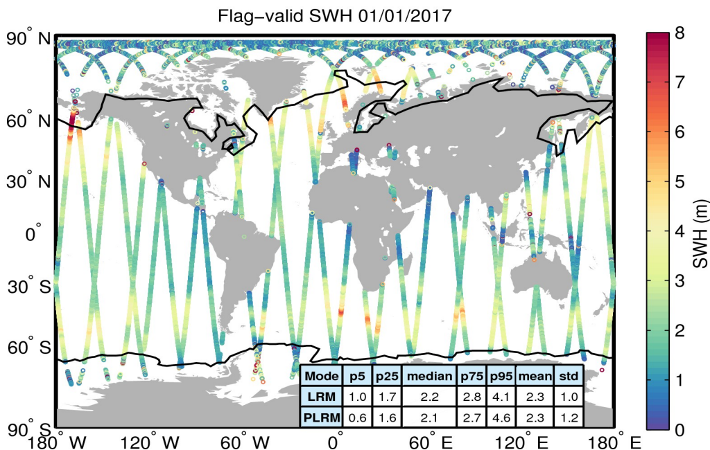
Figure 15. Geographical distribution of flag-valid SWH data over oceans and lakes for 01/01/2017. The statistical values shown in the table refer to the SWH in m and are calculated separately for LRM and PLRM regions. Measurements taken over polar polygons have been excluded from the computation of the statistical values. The black lines mark the outer limit of the Arctic and Antarctic polar polygons.
