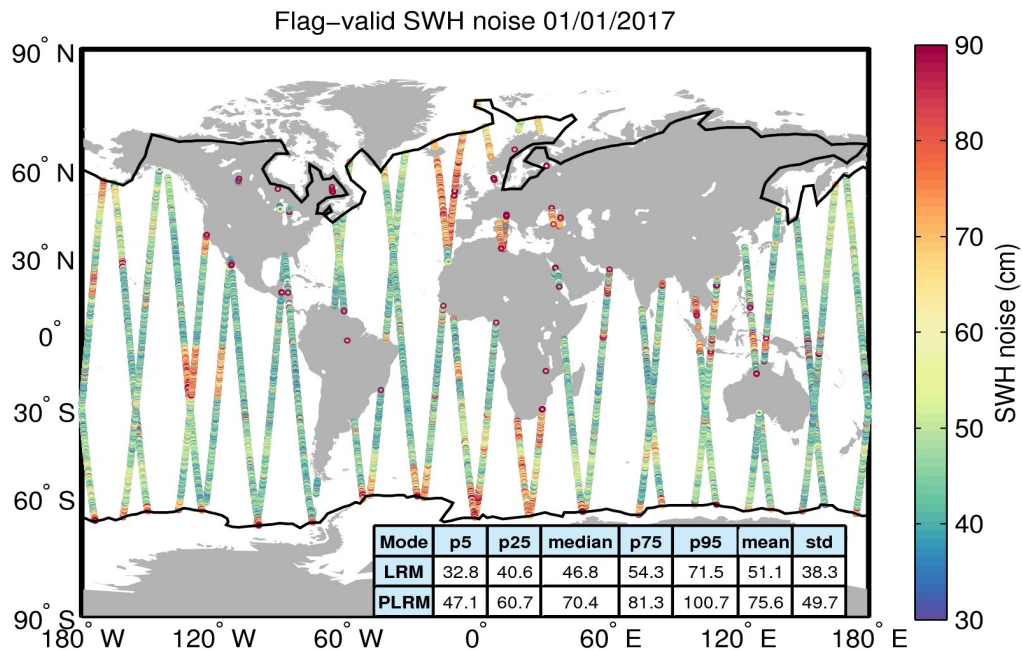
Figure 18. Geographical distribution of flag-valid 20-Hz SWH measurement noise over oceans and lakes for 01/01/2017. The statistical values shown in the table refer to the SWH noise and are calculated separately for LRM and PLRM regions. Measurements taken over polar polygons have been excluded from the computation of the statistical values. The black lines mark the outer limit of the Arctic and Antarctic polar polygons.
