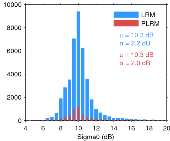
Figure 25. Histogram of flag-valid sigma0 over oceans and lakes for LRM (blue) and PLRM (red) for 01/01/2017. The mean ( \mu ) and standard deviation ( \sigma ) are also shown. Note that values outside [4 20] dB are excluded from the histogram for the sake of readability but not from the computation of \mu and \sigma .
