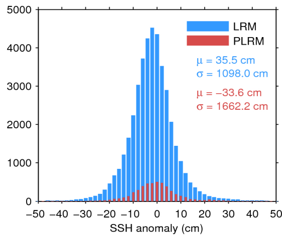
Figure 7. Histogram of flag-valid SSH anomaly over oceans and lakes for LRM (blue) and PLRM (red) for 01/01/2017. The mean ( \mu ) and standard deviation ( \sigma ) are also shown. Note that values outside [-50\ 50] cm are excluded from the histogram for the sake of readability but not from the computation of \mu and \sigma .
