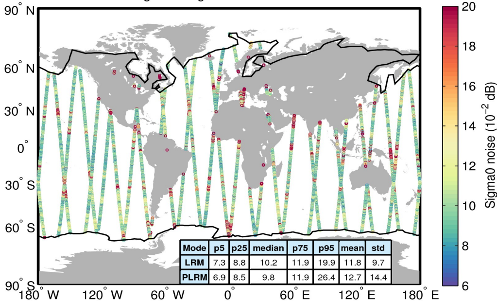
Flag-valid sigma0 noise 01/01/2017
