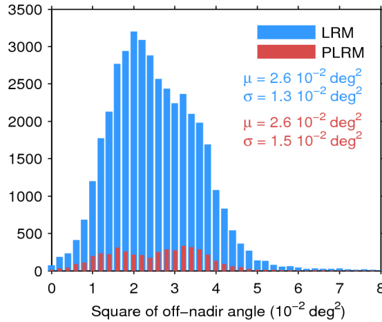
Figure 39. Histogram of flag-valid mispointing over oceans and lakes for LRM (blue) and PLRM (red) for 01/01/2017. Only positive values have been considered. The mean ( \mu ) and standard deviation ( \sigma ) are also shown. Note that values larger than 8 \cdot 10^{-2} \text{ deg}^2 are excluded from the histogram for the sake of readability but not from the computation of \mu and \sigma .
