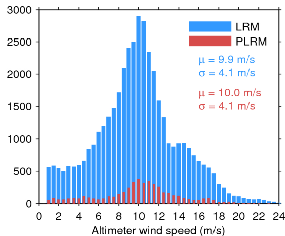
Figure 35. Histogram of science-valid wind over oceans and lakes for LRM (blue) and PLRM (red) for 01/01/2017. The mean ( \mu ) and standard deviation ( \sigma ) are also shown. Note that values larger than 24 m/s are excluded from the histogram for the sake of readability but not from the computation of \mu and \sigma .
