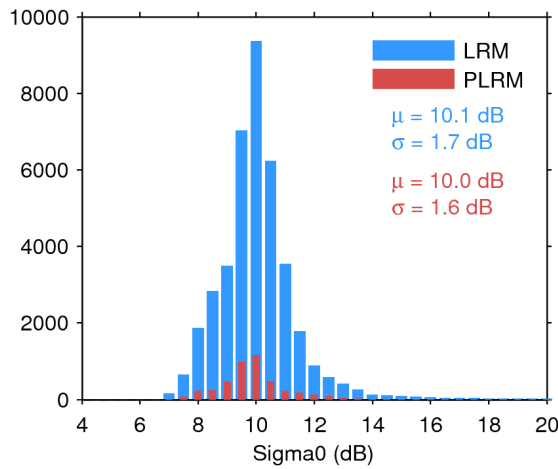
Figure 28. Histogram of science-valid sigma0 over oceans and lakes for LRM (blue) and PLRM (red) for 01/01/2017. The mean ( \mu ) and standard deviation ( \sigma ) are also shown. Note that values outside [4 20] dB are excluded from the histogram for the sake of readability but not from the computation of \mu and \sigma .
