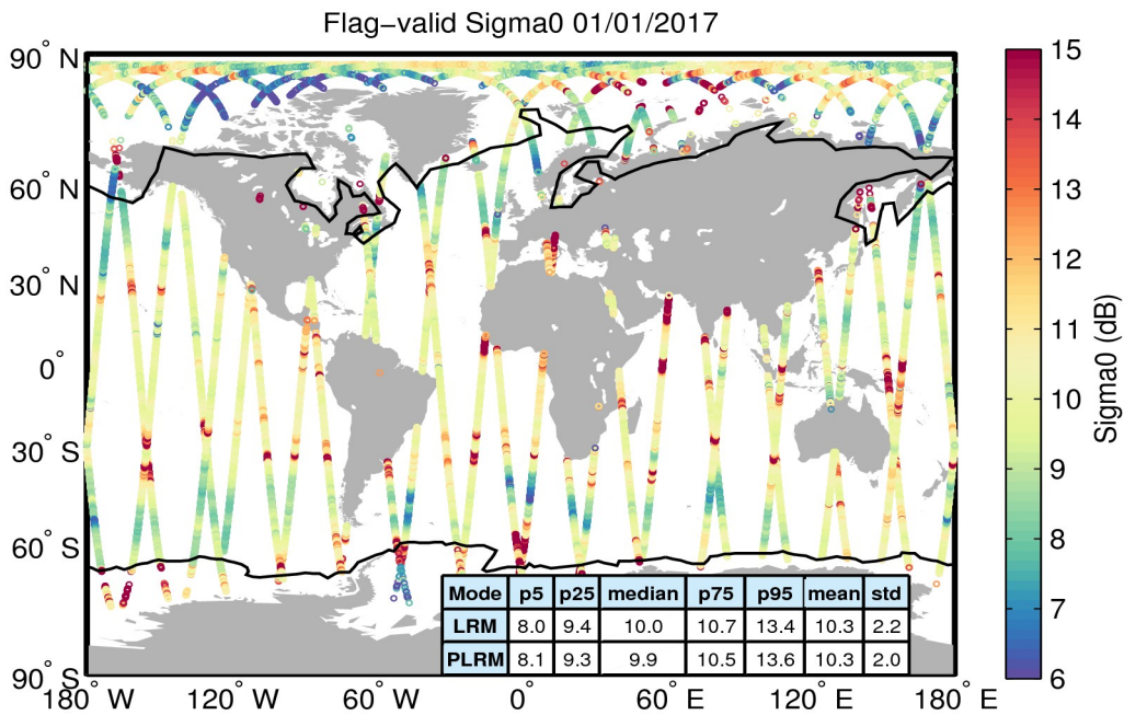
Figure 23. Geographical distribution of flag-valid sigma0 data over oceans and lakes for 01/01/2017. The statistical values shown in the table refer to the sigma0 in dB and are calculated separately for LRM and PLRM regions. Measurements taken over polar polygons have been excluded from the computation of the statistical values. The black lines mark the outer limit of the Arctic and Antarctic polar polygons.
