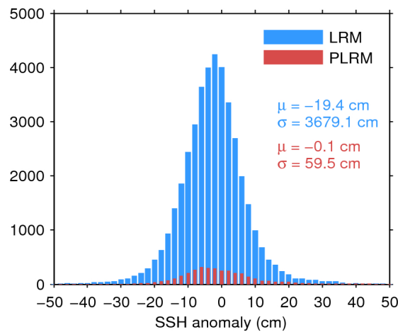
Figure 7. Histogram of flag-valid SSH anomaly over oceans and lakes for LRM (blue) and PLRM (red) for 29/12/2016. The mean ( \mu ) and standard deviation ( \sigma ) are also shown. Note that values outside [-50 \ 50] cm are excluded from the histogram for the sake of readability but not from the computation of \mu and \sigma .
