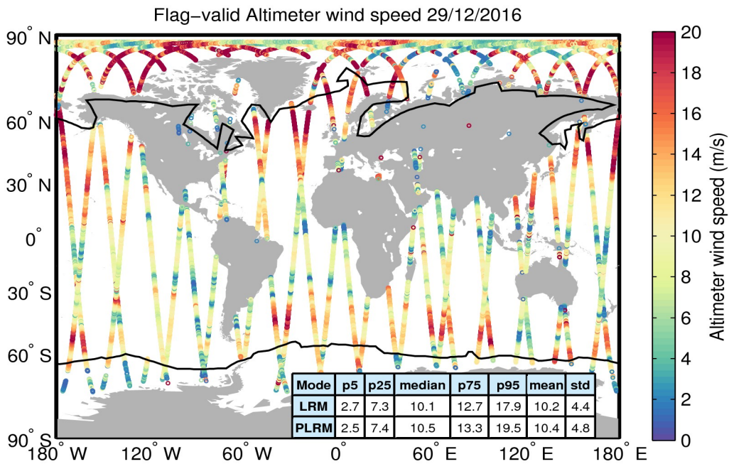
Figure 31. Geographical distribution of flag-valid wind data over oceans and lakes for 29/12/2016. The statistical values shown in the table refer to the wind in m/s and are calculated separately for LRM and PLRM regions. Measurements taken over polar polygons have been excluded from the computation of the statistical values. The black lines mark the outer limit of the Arctic and Antarctic polar polygons.
