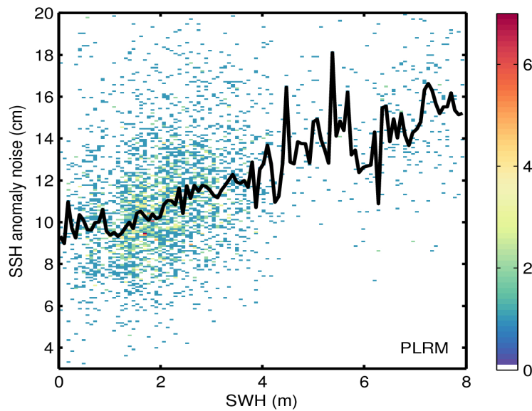
Figure 9. 2D histogram showing flag-valid SSH anomaly noise as a function of SWH for LRM (top) and PLRM (bottom) for 29/12/2016. The black line denotes the median SSH anomaly noise as a function of SWH.
