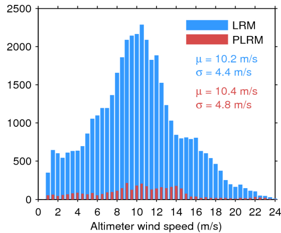
Figure 33. Histogram of flag-valid wind over oceans and lakes for LRM (blue) and PLRM (red) for 29/12/2016. The mean ( \mu ) and standard deviation ( \sigma ) are also shown. Note that values larger than 24 m/s are excluded from the histogram for the sake of readability but not from the computation of \mu and \sigma .
