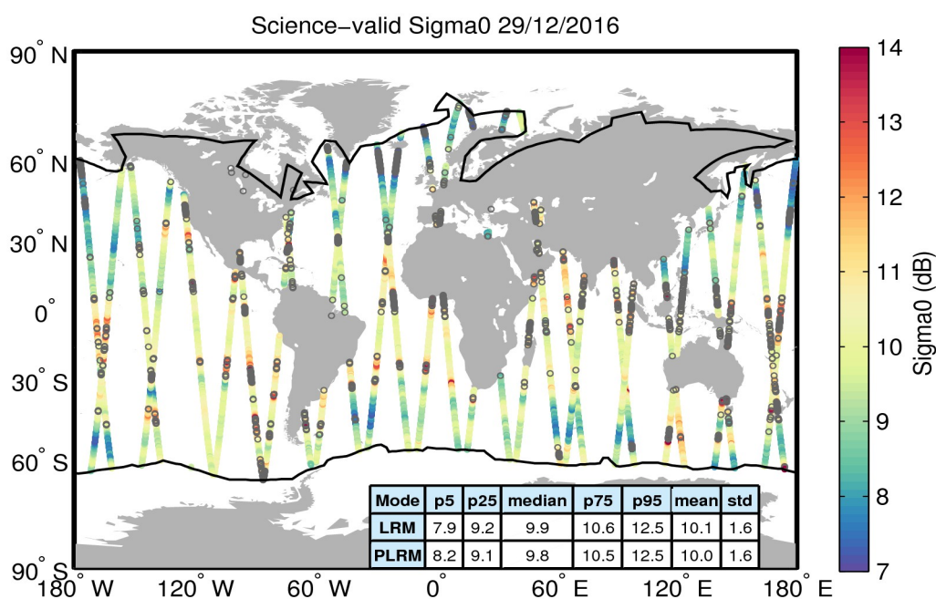
Figure 27. Geographical distribution of science-valid sigma0 data over oceans and lakes for 29/12/2016. The statistical values shown in the table refer to the sigma0 in dB and are calculated separately for LRM and PLRM regions. The black lines mark the outer limit of the Arctic and Antarctic polar polygons. Gray circles denote records that have been rejected based on the editing criteria described in Table 4.
