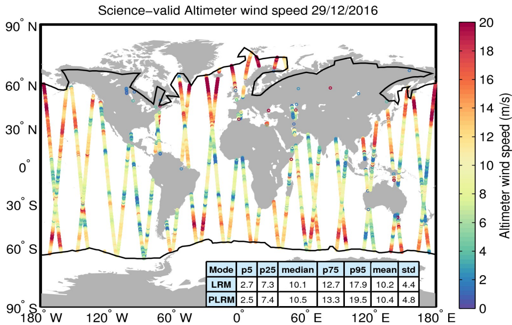
Figure 34. Geographical distribution of science-valid wind data over oceans and lakes for 29/12/2016. The statistical values shown in the table refer to the wind in m/s and are calculated separately for LRM and PLRM regions. The black lines mark the outer limit of the Arctic and Antarctic polar polygons. Gray circles denote records that have been rejected based on the editing criteria described in Table 5.
