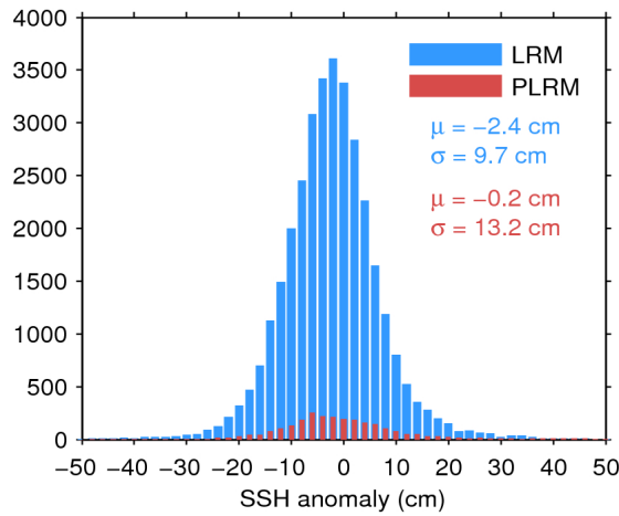
Figure 11. Histogram of science-valid SSH anomaly over oceans and lakes for LRM (blue) and PLRM (red) for 29/12/2016. The mean ( \mu ) and standard deviation ( \sigma ) are also shown. Note that values outside [-50 50] cm are excluded from the histogram for the sake of readability but not from the computation of \mu and \sigma .
