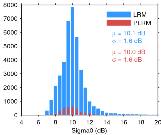
Figure 28. Histogram of science-valid sigma0 over oceans and lakes for LRM (blue) and PLRM (red) for 29/12/2016. The mean ( \mu ) and standard deviation ( \sigma ) are also shown. Note that values outside [4 20] dB are excluded from the histogram for the sake of readability but not from the computation of \mu and \sigma .
