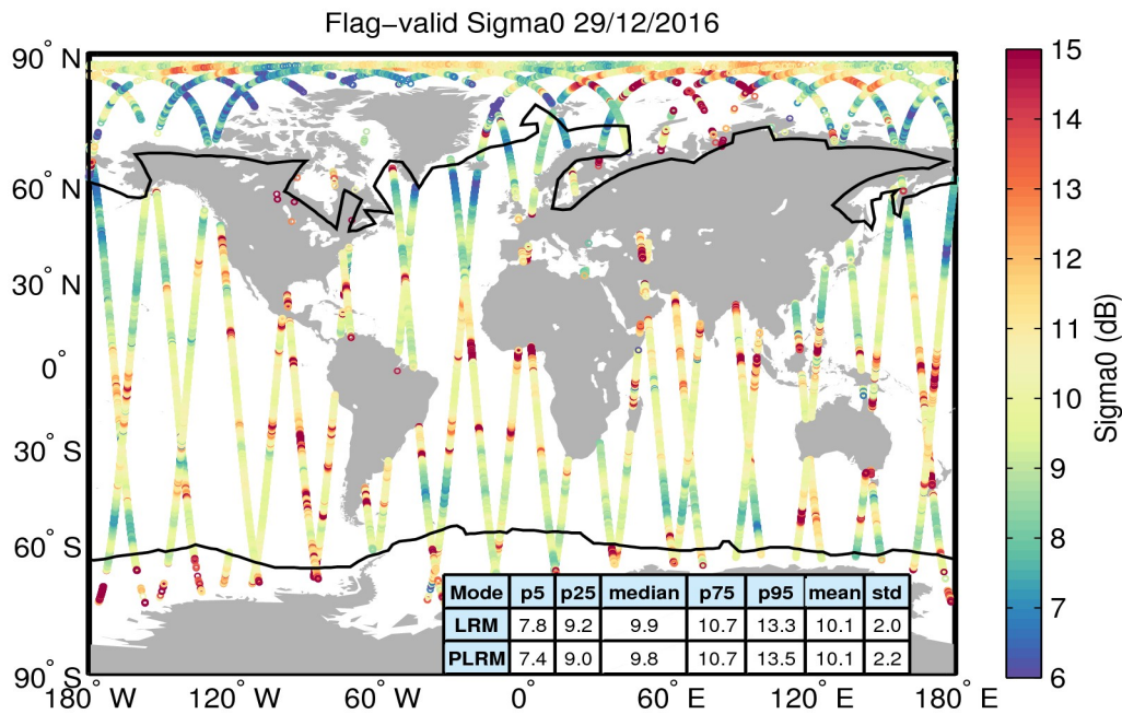
Figure 23. Geographical distribution of flag-valid sigma0 data over oceans and lakes for 29/12/2016. The statistical values shown in the table refer to the sigma0 in dB and are calculated separately for LRM and PLRM regions. Measurements taken over polar polygons have been excluded from the computation of the statistical values. The black lines mark the outer limit of the Arctic and Antarctic polar polygons.
