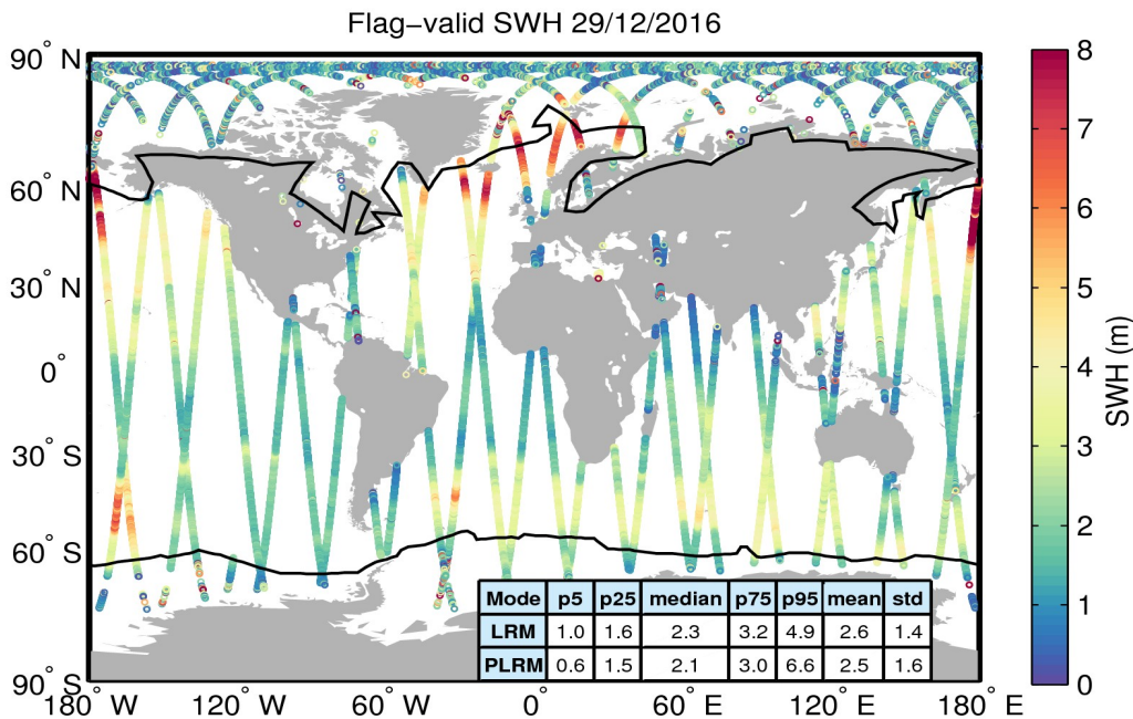
Figure 15. Geographical distribution of flag-valid SWH data over oceans and lakes for 29/12/2016. The statistical values shown in the table refer to the SWH in m and are calculated separately for LRM and PLRM regions. Measurements taken over polar polygons have been excluded from the computation of the statistical values. The black lines mark the outer limit of the Arctic and Antarctic polar polygons.
