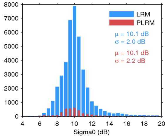
Figure 25. Histogram of flag-valid sigma0 over oceans and lakes for LRM (blue) and PLRM (red) for 29/12/2016. The mean ( \mu ) and standard deviation ( \sigma ) are also shown. Note that values outside [4 20] dB are excluded from the histogram for the sake of readability but not from the computation of \mu and \sigma .
