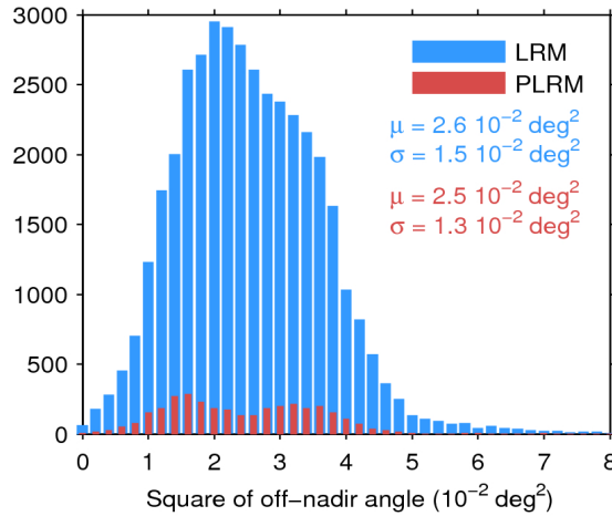
Figure 39. Histogram of flag-valid mispointing over oceans and lakes for LRM (blue) and PLRM (red) for 29/12/2016. Only positive values have been considered. The mean ( \mu ) and standard deviation ( \sigma ) are also shown. Note that values larger than 8 \cdot 10^{-2} \text{ deg}^2 are excluded from the histogram for the sake of readability but not from the computation of \mu and \sigma .
