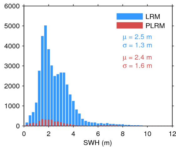
Figure 20. Histogram of science-valid SWH over oceans and lakes for LRM (blue) and PLRM (red) for 29/12/2016. The mean ( \mu ) and standard deviation ( \sigma ) are also shown. Note that values larger than 12 m are excluded from the histogram for the sake of readability but not from the computation of \mu and \sigma .
