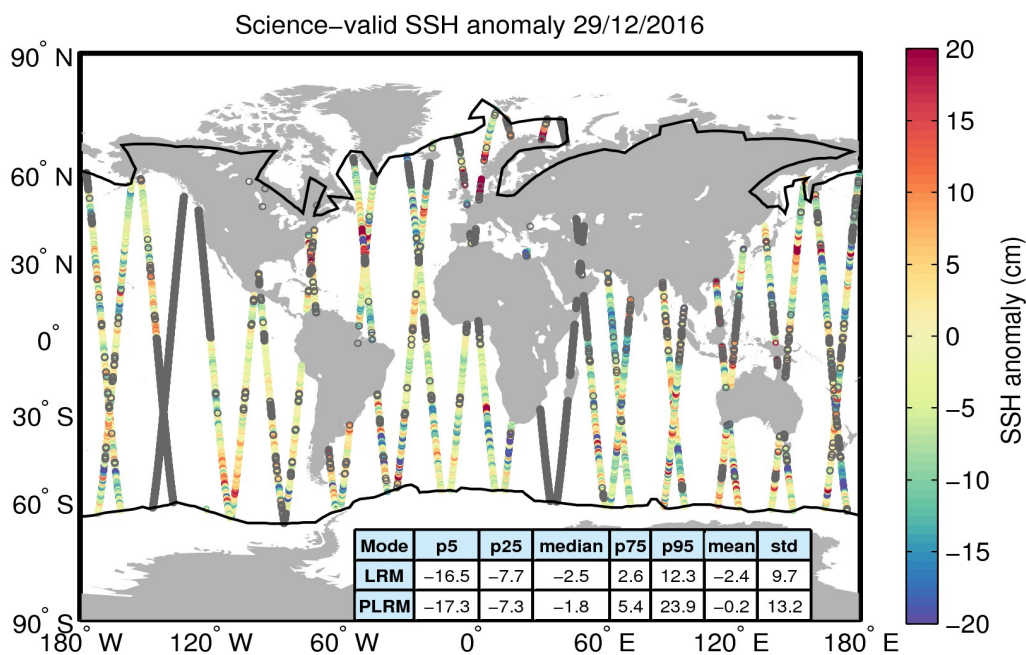
Figure 10. Geographical distribution of science-valid SSH anomaly data over oceans and lakes for 29/12/2016. The statistical values shown in the table refer to the SSH anomaly in cm and are calculated separately for LRM and PLRM regions. The black lines mark the outer limit of the Arctic and Antarctic polar polygons. Gray circles denote records that have been rejected based on the editing criteria described in Table 2.
