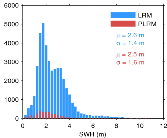
Figure 17. Histogram of flag-valid SWH over oceans and lakes for LRM (blue) and PLRM (red) for 29/12/2016. The mean ( \mu ) and standard deviation ( \sigma ) are also shown. Note that values larger than 12 m are excluded from the histogram for the sake of readability but not from the computation of \mu and \sigma .
