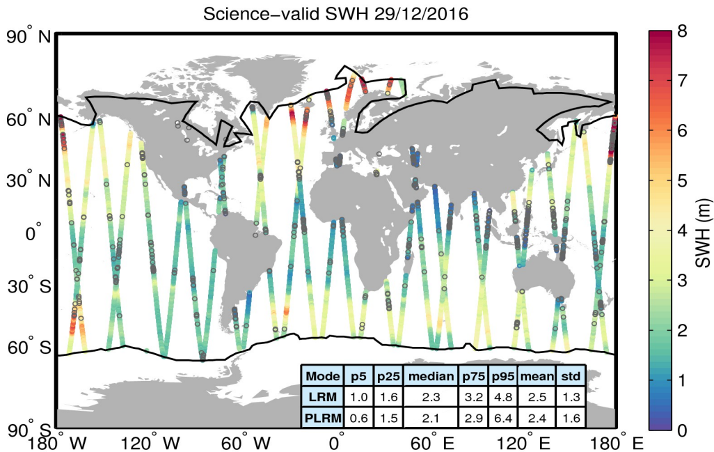
Figure 19. Geographical distribution of science-valid SWH data over oceans and lakes for 29/12/2016. The statistical values shown in the table refer to the SWH in m and are calculated separately for LRM and PLRM regions. The black lines mark the outer limit of the Arctic and Antarctic polar polygons. Gray circles denote records that have been rejected based on the editing criteria described in Table 3.
