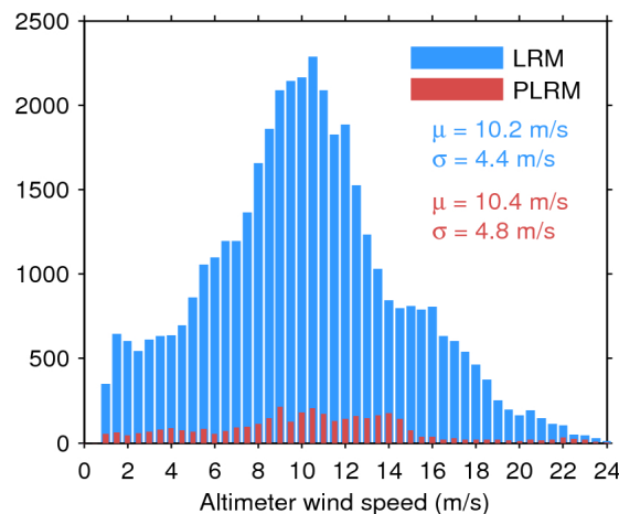
Figure 35. Histogram of science-valid wind over oceans and lakes for LRM (blue) and PLRM (red) for 29/12/2016. The mean ( \mu ) and standard deviation ( \sigma ) are also shown. Note that values larger than 24 m/s are excluded from the histogram for the sake of readability but not from the computation of \mu and \sigma .
