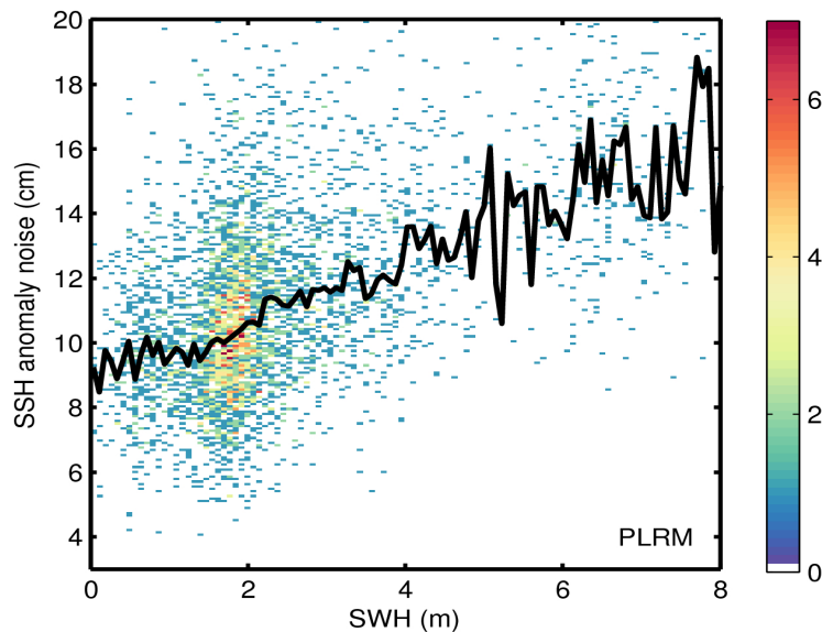
Figure 9. 2D histogram showing flag-valid SSH anomaly noise as a function of SWH for LRM (top) and PLRM (bottom) for 28/12/2016. The black line denotes the median SSH anomaly noise as a function of SWH.
