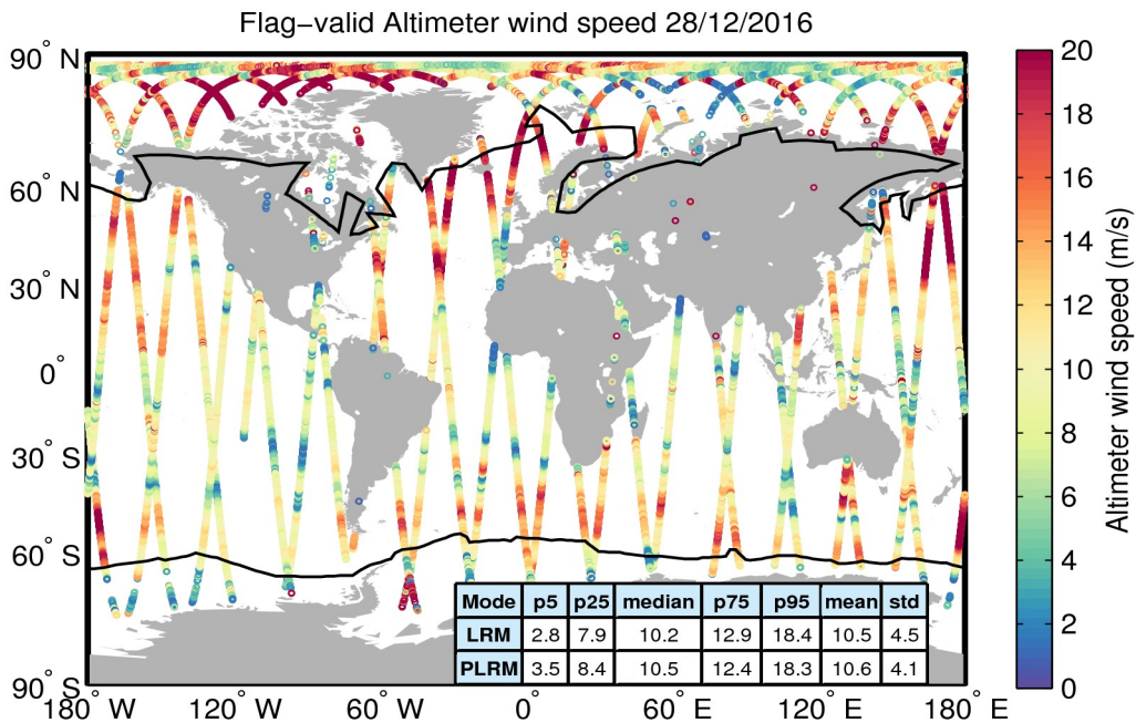
Figure 31. Geographical distribution of flag-valid wind data over oceans and lakes for 28/12/2016. The statistical values shown in the table refer to the wind in m/s and are calculated separately for LRM and PLRM regions. Measurements taken over polar polygons have been excluded from the computation of the statistical values. The black lines mark the outer limit of the Arctic and Antarctic polar polygons.
