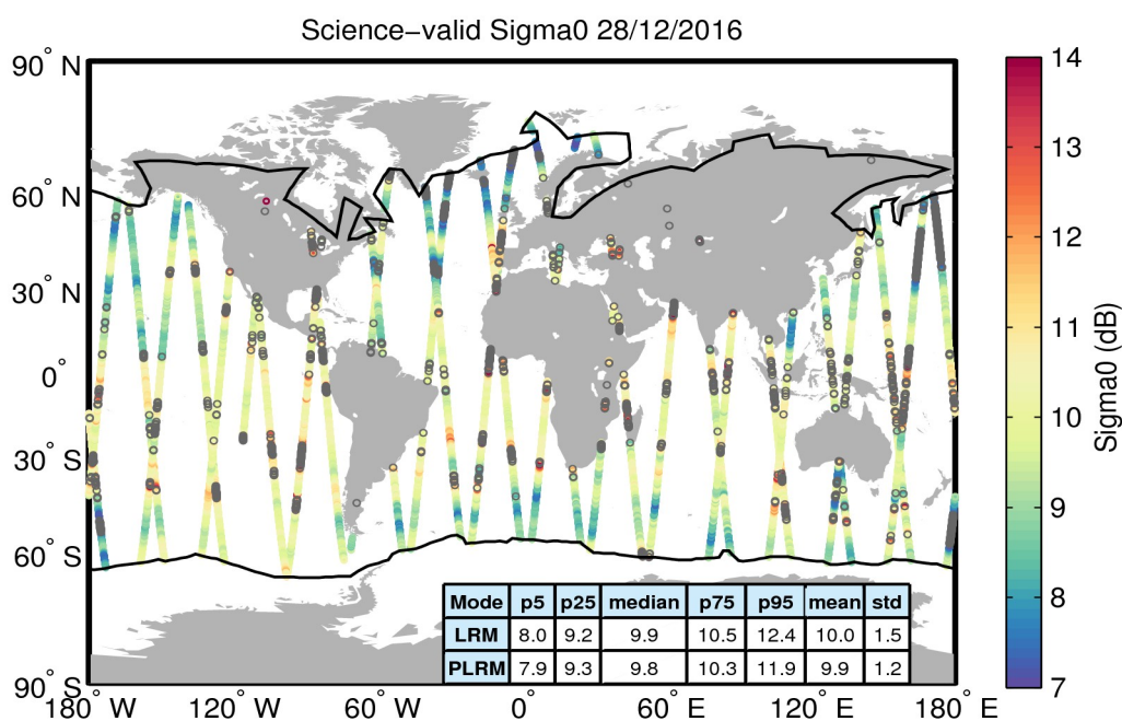
Figure 27. Geographical distribution of science-valid sigma0 data over oceans and lakes for 28/12/2016. The statistical values shown in the table refer to the sigma0 in dB and are calculated separately for LRM and PLRM regions. The black lines mark the outer limit of the Arctic and Antarctic polar polygons. Gray circles denote records that have been rejected based on the editing criteria described in Table 4.
