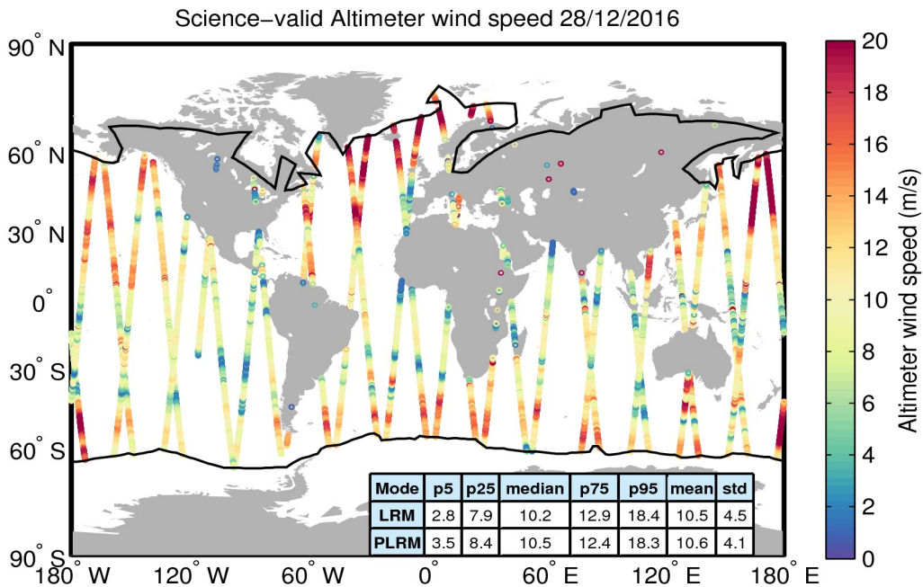
Figure 34. Geographical distribution of science-valid wind data over oceans and lakes for 28/12/2016. The statistical values shown in the table refer to the wind in m/s and are calculated separately for LRM and PLRM regions. The black lines mark the outer limit of the Arctic and Antarctic polar polygons. Gray circles denote records that have been rejected based on the editing criteria described in Table 5.
