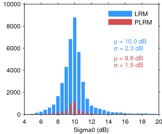
Figure 25. Histogram of flag-valid sigma0 over oceans and lakes for LRM (blue) and PLRM (red) for 28/12/2016. The mean ( \mu ) and standard deviation ( \sigma ) are also shown. Note that values outside [4 20] dB are excluded from the histogram for the sake of readability but not from the computation of \mu and \sigma .
