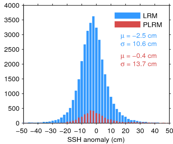
Figure 11. Histogram of science-valid SSH anomaly over oceans and lakes for LRM (blue) and PLRM (red) for 28/12/2016. The mean ( \mu ) and standard deviation ( \sigma ) are also shown. Note that values outside [-50\ 50] cm are excluded from the histogram for the sake of readability but not from the computation of \mu and \sigma .
