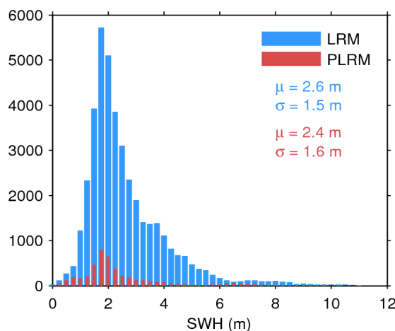
Figure 17. Histogram of flag-valid SWH over oceans and lakes for LRM (blue) and PLRM (red) for 28/12/2016. The mean ( \mu ) and standard deviation ( \sigma ) are also shown. Note that values larger than 12 m are excluded from the histogram for the sake of readability but not from the computation of \mu and \sigma .
