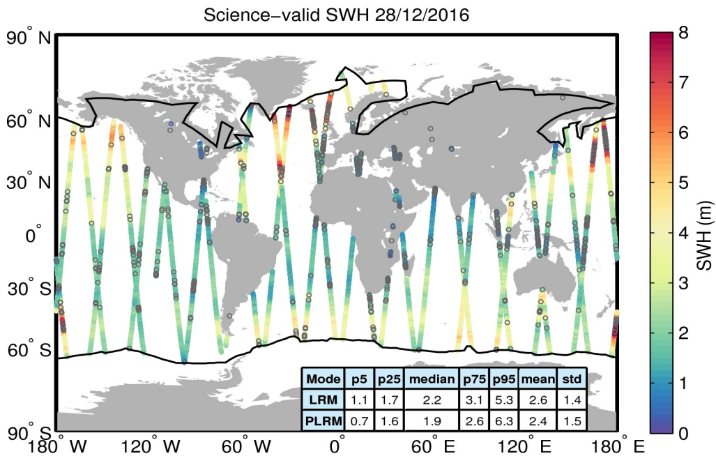
Figure 19. Geographical distribution of science-valid SWH data over oceans and lakes for 28/12/2016. The statistical values shown in the table refer to the SWH in m and are calculated separately for LRM and PLRM regions. The black lines mark the outer limit of the Arctic and Antarctic polar polygons. Gray circles denote records that have been rejected based on the editing criteria described in Table 3.
