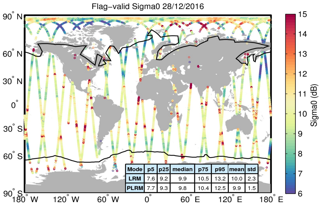
Figure 23. Geographical distribution of flag-valid sigma0 data over oceans and lakes for 28/12/2016. The statistical values shown in the table refer to the sigma0 in dB and are calculated separately for LRM and PLRM regions. Measurements taken over polar polygons have been excluded from the computation of the statistical values. The black lines mark the outer limit of the Arctic and Antarctic polar polygons.
