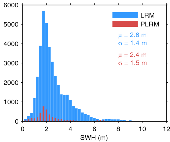
Figure 20. Histogram of science-valid SWH over oceans and lakes for LRM (blue) and PLRM (red) for 28/12/2016. The mean ( \mu ) and standard deviation ( \sigma ) are also shown. Note that values larger than 12 m are excluded from the histogram for the sake of readability but not from the computation of \mu and \sigma .
