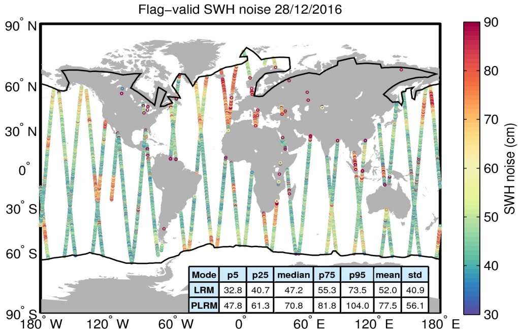
Figure 18. Geographical distribution of flag-valid 20-Hz SWH measurement noise over oceans and lakes for 28/12/2016. The statistical values shown in the table refer to the SWH noise and are calculated separately for LRM and PLRM regions. Measurements taken over polar polygons have been excluded from the computation of the statistical values. The black lines mark the outer limit of the Arctic and Antarctic polar polygons.
