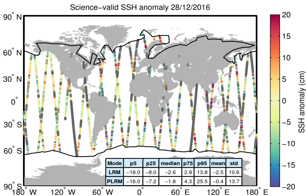
Figure 10. Geographical distribution of science-valid SSH anomaly data over oceans and lakes for 28/12/2016. The statistical values shown in the table refer to the SSH anomaly in cm and are calculated separately for LRM and PLRM regions. The black lines mark the outer limit of the Arctic and Antarctic polar polygons. Gray circles denote records that have been rejected based on the editing criteria described in Table 2.
