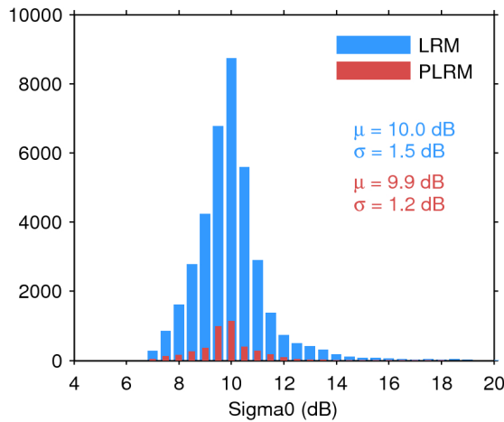
Figure 28. Histogram of science-valid sigma0 over oceans and lakes for LRM (blue) and PLRM (red) for 28/12/2016. The mean ( \mu ) and standard deviation ( \sigma ) are also shown. Note that values outside [4 20] dB are excluded from the histogram for the sake of readability but not from the computation of \mu and \sigma .
