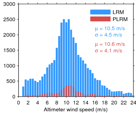
Figure 33. Histogram of flag-valid wind over oceans and lakes for LRM (blue) and PLRM (red) for 28/12/2016. The mean ( \mu ) and standard deviation ( \sigma ) are also shown. Note that values larger than 24 m/s are excluded from the histogram for the sake of readability but not from the computation of \mu and \sigma .
