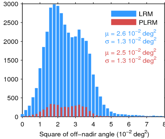
Figure 39. Histogram of flag-valid mispointing over oceans and lakes for LRM (blue) and PLRM (red) for 28/12/2016. Only positive values have been considered. The mean ( \mu ) and standard deviation ( \sigma ) are also shown. Note that values larger than 8 \cdot 10^{-2} \text{ deg}^2 are excluded from the histogram for the sake of readability but not from the computation of \mu and \sigma .
