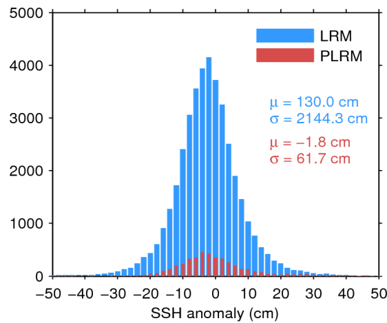
Figure 7. Histogram of flag-valid SSH anomaly over oceans and lakes for LRM (blue) and PLRM (red) for 28/12/2016. The mean ( \mu ) and standard deviation ( \sigma ) are also shown. Note that values outside [-50\ 50] cm are excluded from the histogram for the sake of readability but not from the computation of \mu and \sigma .
