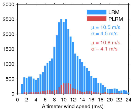
Figure 35. Histogram of science-valid wind over oceans and lakes for LRM (blue) and PLRM (red) for 28/12/2016. The mean ( \mu ) and standard deviation ( \sigma ) are also shown. Note that values larger than 24 m/s are excluded from the histogram for the sake of readability but not from the computation of \mu and \sigma .
