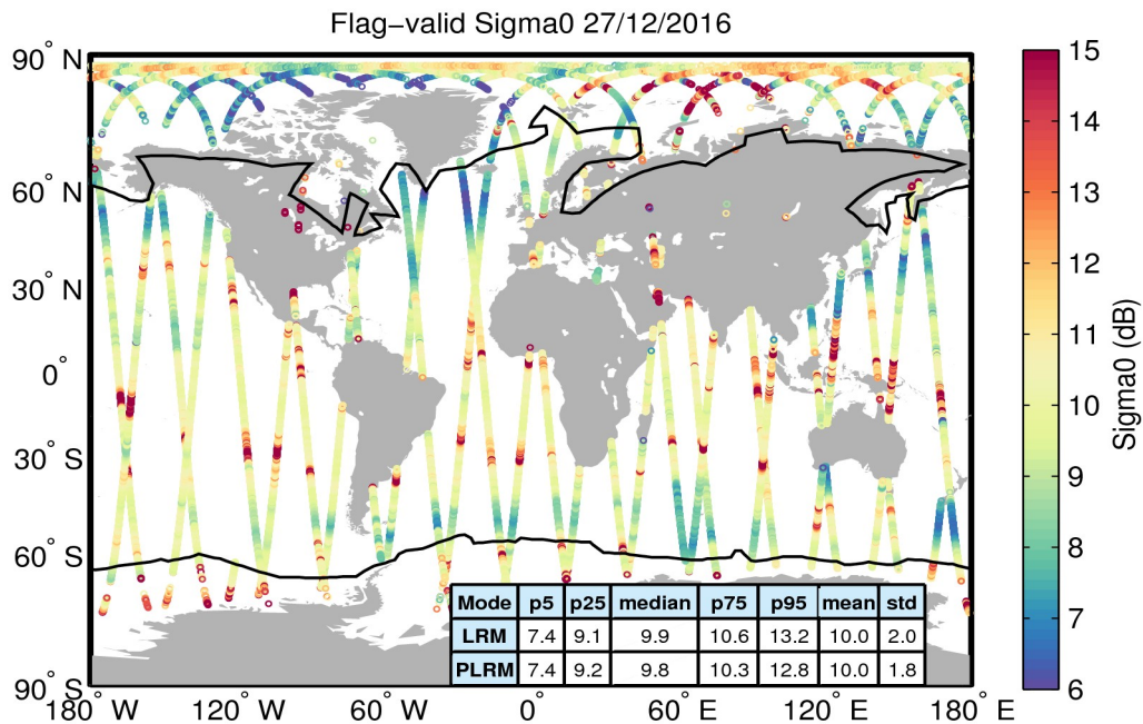
Figure 23. Geographical distribution of flag-valid sigma0 data over oceans and lakes for 27/12/2016. The statistical values shown in the table refer to the sigma0 in dB and are calculated separately for LRM and PLRM regions. Measurements taken over polar polygons have been excluded from the computation of the statistical values. The black lines mark the outer limit of the Arctic and Antarctic polar polygons.
