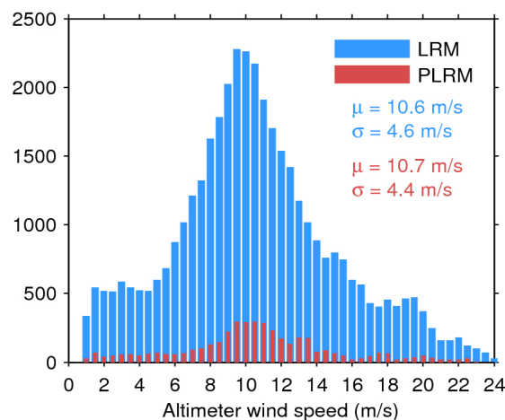
Figure 35. Histogram of science-valid wind over oceans and lakes for LRM (blue) and PLRM (red) for 27/12/2016. The mean ( \mu ) and standard deviation ( \sigma ) are also shown. Note that values larger than 24 m/s are excluded from the histogram for the sake of readability but not from the computation of \mu and \sigma .
