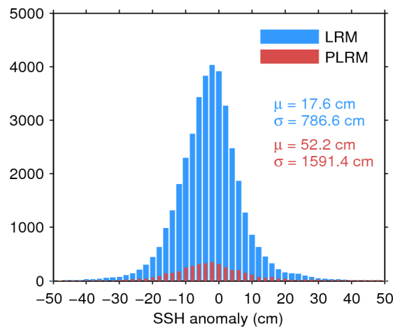
Figure 7. Histogram of flag-valid SSH anomaly over oceans and lakes for LRM (blue) and PLRM (red) for 27/12/2016. The mean ( \mu ) and standard deviation ( \sigma ) are also shown. Note that values outside [-50\ 50] cm are excluded from the histogram for the sake of readability but not from the computation of \mu and \sigma .
