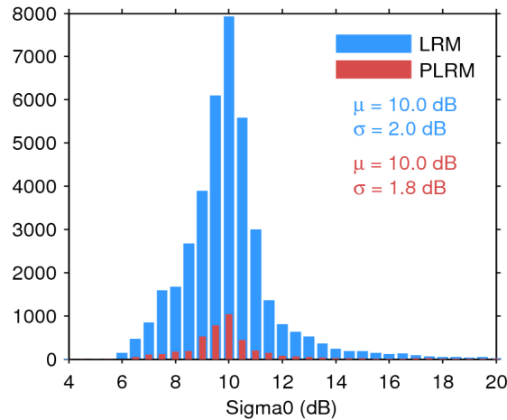
Figure 25. Histogram of flag-valid sigma0 over oceans and lakes for LRM (blue) and PLRM (red) for 27/12/2016. The mean ( \mu ) and standard deviation ( \sigma ) are also shown. Note that values outside [4 20] dB are excluded from the histogram for the sake of readability but not from the computation of \mu and \sigma .
