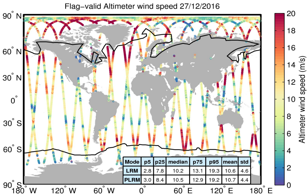
Figure 31. Geographical distribution of flag-valid wind data over oceans and lakes for 27/12/2016. The statistical values shown in the table refer to the wind in m/s and are calculated separately for LRM and PLRM regions. Measurements taken over polar polygons have been excluded from the computation of the statistical values. The black lines mark the outer limit of the Arctic and Antarctic polar polygons.
