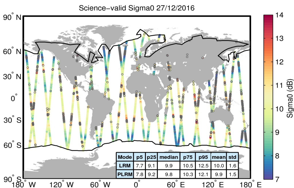
Figure 27. Geographical distribution of science-valid sigma0 data over oceans and lakes for 27/12/2016. The statistical values shown in the table refer to the sigma0 in dB and are calculated separately for LRM and PLRM regions. The black lines mark the outer limit of the Arctic and Antarctic polar polygons. Gray circles denote records that have been rejected based on the editing criteria described in Table 4.
