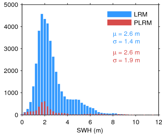
Figure 17. Histogram of flag-valid SWH over oceans and lakes for LRM (blue) and PLRM (red) for 27/12/2016. The mean ( \mu ) and standard deviation ( \sigma ) are also shown. Note that values larger than 12 m are excluded from the histogram for the sake of readability but not from the computation of \mu and \sigma .
