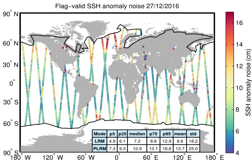
Figure 8. Geographical distribution of flag-valid 20-Hz SSH anomaly measurement noise over oceans and lakes for 27/12/2016. The statistical values shown in the table refer to the SSH anomaly noise and are calculated separately for LRM and PLRM regions. Measurements taken over polar polygons have been excluded from the computation of the statistical values. The black lines mark the outer limit of the Arctic and Antarctic polar polygons.
