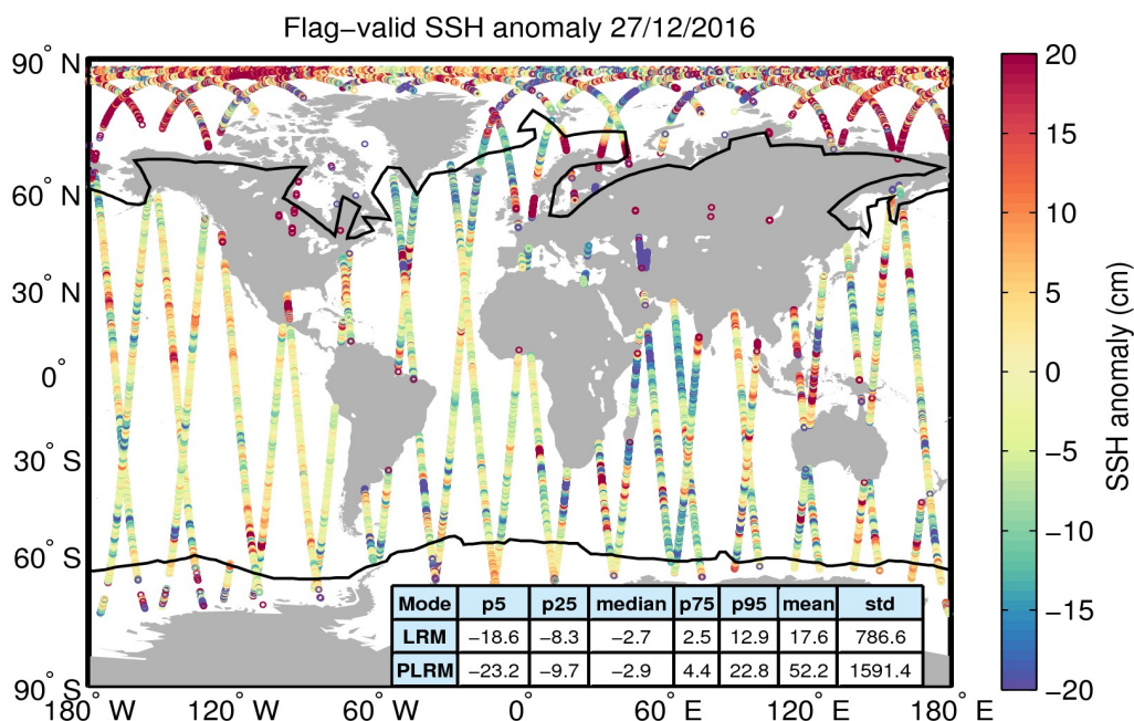
Figure 5. Geographical distribution of flag-valid 1-Hz SSH anomaly data over oceans and lakes for 27/12/2016. The statistical values shown in the table refer to the SSH anomaly in cm and are calculated separately for LRM and PLRM regions. Measurements taken over polar polygons have been excluded from the computation of the statistical values. The black lines mark the outer limit of the Arctic and Antarctic polar polygons.
