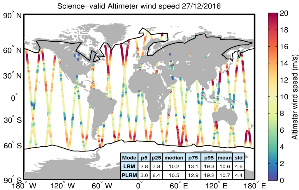
Figure 34. Geographical distribution of science-valid wind data over oceans and lakes for 27/12/2016. The statistical values shown in the table refer to the wind in m/s and are calculated separately for LRM and PLRM regions. The black lines mark the outer limit of the Arctic and Antarctic polar polygons. Gray circles denote records that have been rejected based on the editing criteria described in Table 5.
