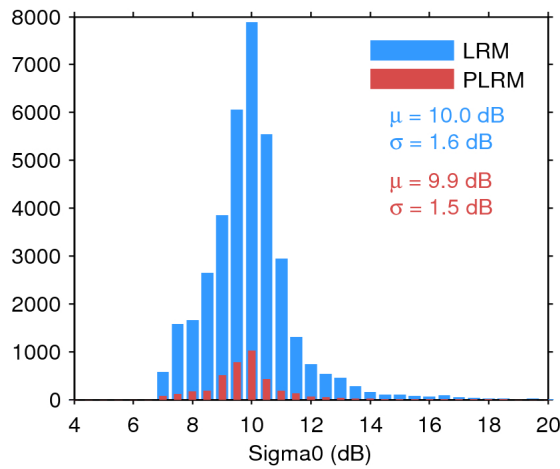
Figure 28. Histogram of science-valid sigma0 over oceans and lakes for LRM (blue) and PLRM (red) for 27/12/2016. The mean ( \mu ) and standard deviation ( \sigma ) are also shown. Note that values outside [4 20] dB are excluded from the histogram for the sake of readability but not from the computation of \mu and \sigma .
