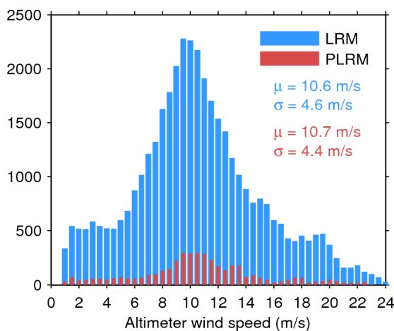
Figure 33. Histogram of flag-valid wind over oceans and lakes for LRM (blue) and PLRM (red) for 27/12/2016. The mean ( \mu ) and standard deviation ( \sigma ) are also shown. Note that values larger than 24 m/s are excluded from the histogram for the sake of readability but not from the computation of \mu and \sigma .
