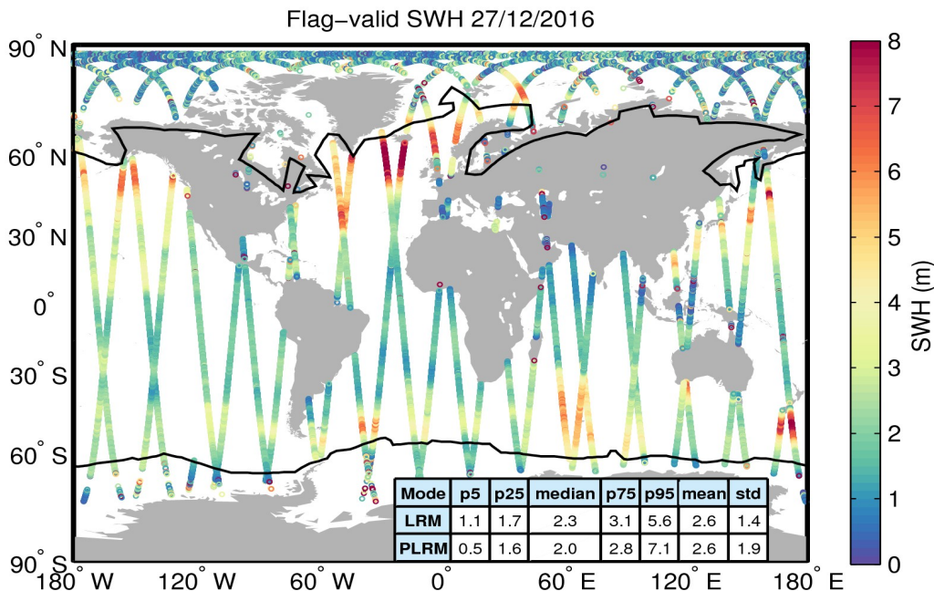
Figure 15. Geographical distribution of flag-valid SWH data over oceans and lakes for 27/12/2016. The statistical values shown in the table refer to the SWH in m and are calculated separately for LRM and PLRM regions. Measurements taken over polar polygons have been excluded from the computation of the statistical values. The black lines mark the outer limit of the Arctic and Antarctic polar polygons.
