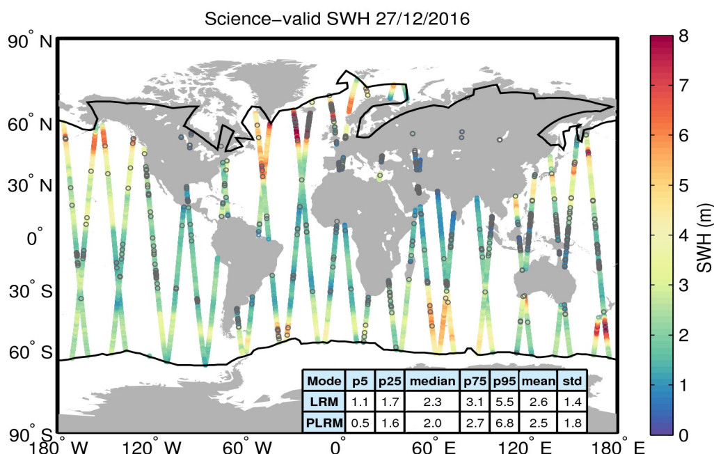
Figure 19. Geographical distribution of science-valid SWH data over oceans and lakes for 27/12/2016. The statistical values shown in the table refer to the SWH in m and are calculated separately for LRM and PLRM regions. The black lines mark the outer limit of the Arctic and Antarctic polar polygons. Gray circles denote records that have been rejected based on the editing criteria described in Table 3.
