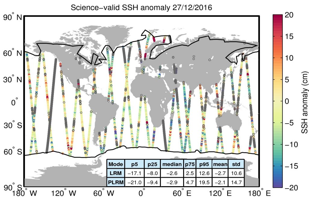
Figure 10. Geographical distribution of science-valid SSH anomaly data over oceans and lakes for 27/12/2016. The statistical values shown in the table refer to the SSH anomaly in cm and are calculated separately for LRM and PLRM regions. The black lines mark the outer limit of the Arctic and Antarctic polar polygons. Gray circles denote records that have been rejected based on the editing criteria described in Table 2.
