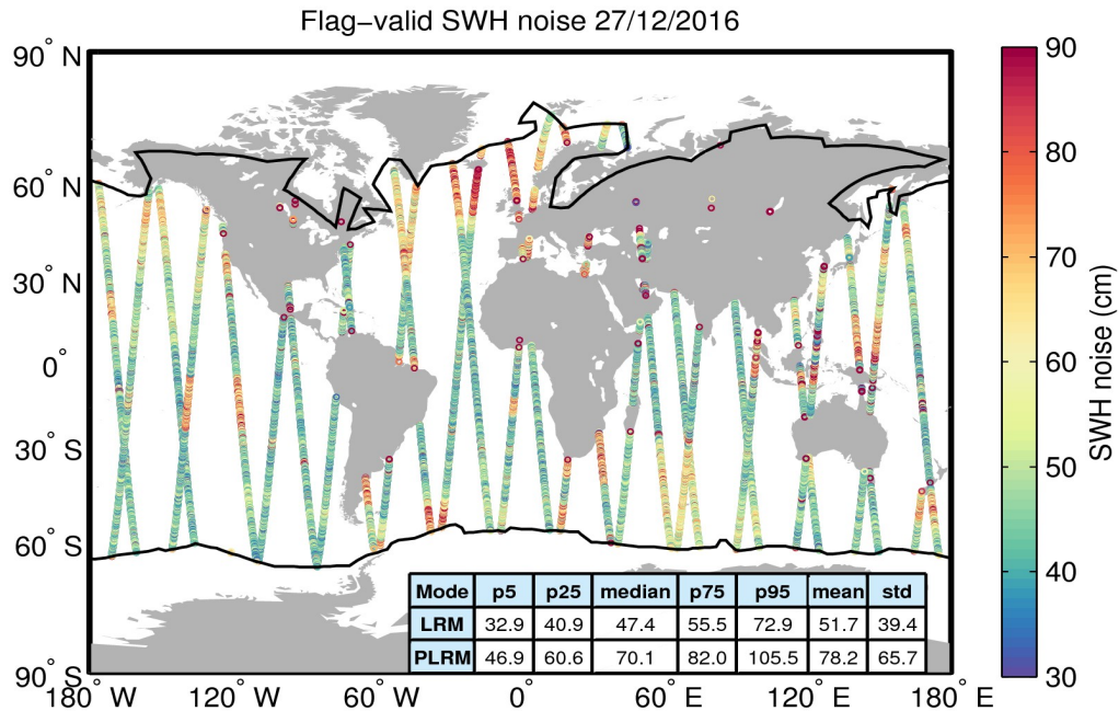
Figure 18. Geographical distribution of flag-valid 20-Hz SWH measurement noise over oceans and lakes for 27/12/2016. The statistical values shown in the table refer to the SWH noise and are calculated separately for LRM and PLRM regions. Measurements taken over polar polygons have been excluded from the computation of the statistical values. The black lines mark the outer limit of the Arctic and Antarctic polar polygons.
