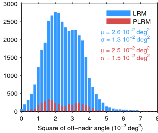
Figure 39. Histogram of flag-valid mispointing over oceans and lakes for LRM (blue) and PLRM (red) for 27/12/2016. Only positive values have been considered. The mean ( \mu ) and standard deviation ( \sigma ) are also shown. Note that values larger than 8 \cdot 10^{-2} \text{ deg}^2 are excluded from the histogram for the sake of readability but not from the computation of \mu and \sigma .
