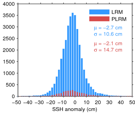
Figure 11. Histogram of science-valid SSH anomaly over oceans and lakes for LRM (blue) and PLRM (red) for 27/12/2016. The mean ( \mu ) and standard deviation ( \sigma ) are also shown. Note that values outside [-50 50] cm are excluded from the histogram for the sake of readability but not from the computation of \mu and \sigma .
