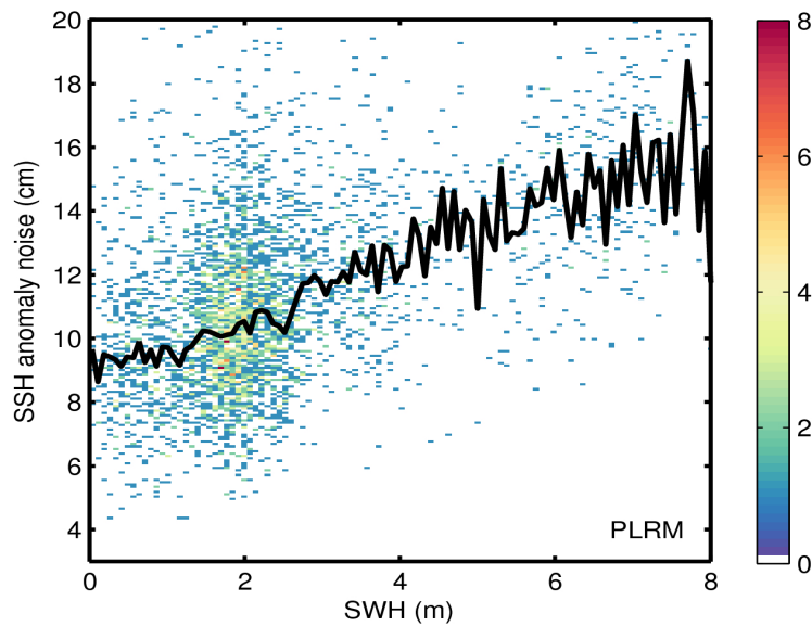
Figure 9. 2D histogram showing flag-valid SSH anomaly noise as a function of SWH for LRM (top) and PLRM (bottom) for 27/12/2016. The black line denotes the median SSH anomaly noise as a function of SWH.
