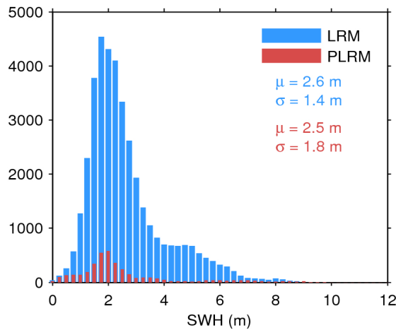
Figure 20. Histogram of science-valid SWH over oceans and lakes for LRM (blue) and PLRM (red) for 27/12/2016. The mean ( \mu ) and standard deviation ( \sigma ) are also shown. Note that values larger than 12 m are excluded from the histogram for the sake of readability but not from the computation of \mu and \sigma .
