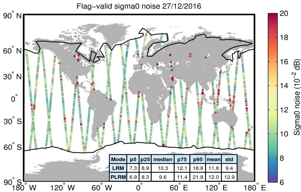
Figure 26. Geographical distribution of flag-valid 20-Hz sigma0 measurement noise over oceans and lakes for 27/12/2016. The statistical values shown in the table refer to the sigma0 noise and are calculated separately for LRM and PLRM regions. Measurements taken over polar polygons have been excluded from the computation of the statistical values. The black lines mark the outer limit of the Arctic and Antarctic polar polygons.
