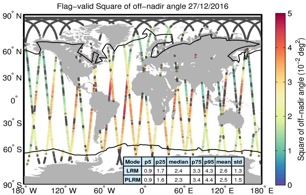
Figure 37. Geographical distribution of flag-valid mispointing data over oceans and lakes for 27/12/2016. The statistical values shown in the table refer to the mispointing in 10^{-2} deg 2 and are calculated separately for LRM and PLRM regions. Measurements taken over polar polygons have been excluded from the computation of the statistical values. The black lines mark the outer limit of the Arctic and Antarctic polar polygons. Gray circles denote negative values.
