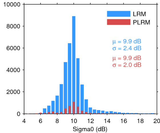
Figure 25. Histogram of flag-valid sigma0 over oceans and lakes for LRM (blue) and PLRM (red) for 26/12/2016. The mean ( \mu ) and standard deviation ( \sigma ) are also shown. Note that values outside [4 20] dB are excluded from the histogram for the sake of readability but not from the computation of \mu and \sigma .
