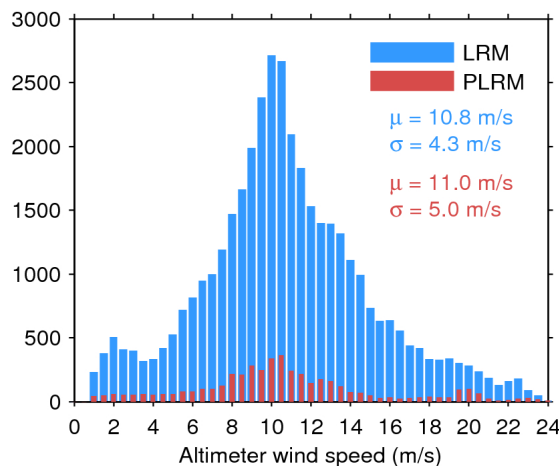
Figure 35. Histogram of science-valid wind over oceans and lakes for LRM (blue) and PLRM (red) for 26/12/2016. The mean ( \mu ) and standard deviation ( \sigma ) are also shown. Note that values larger than 24 m/s are excluded from the histogram for the sake of readability but not from the computation of \mu and \sigma .
