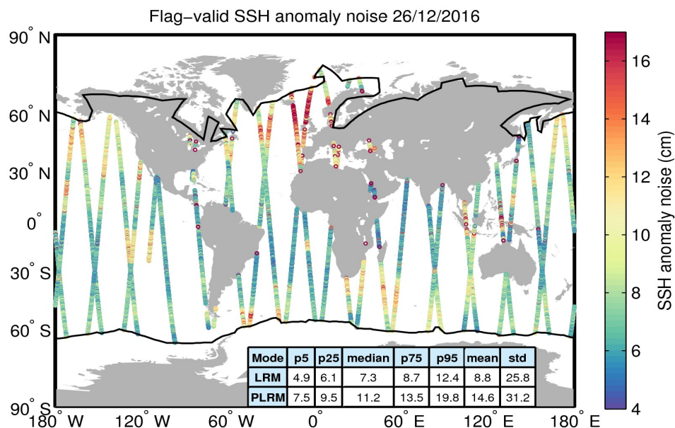
Figure 8. Geographical distribution of flag-valid 20-Hz SSH anomaly measurement noise over oceans and lakes for 26/12/2016. The statistical values shown in the table refer to the SSH anomaly noise and are calculated separately for LRM and PLRM regions. Measurements taken over polar polygons have been excluded from the computation of the statistical values. The black lines mark the outer limit of the Arctic and Antarctic polar polygons.
