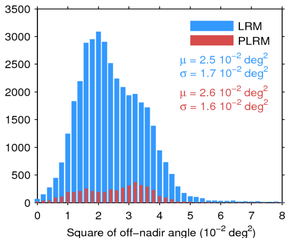
Figure 39. Histogram of flag-valid mispointing over oceans and lakes for LRM (blue) and PLRM (red) for 26/12/2016. Only positive values have been considered. The mean ( \mu ) and standard deviation ( \sigma ) are also shown. Note that values larger than 8 \cdot 10^{-2} \text{ deg}^2 are excluded from the histogram for the sake of readability but not from the computation of \mu and \sigma .
