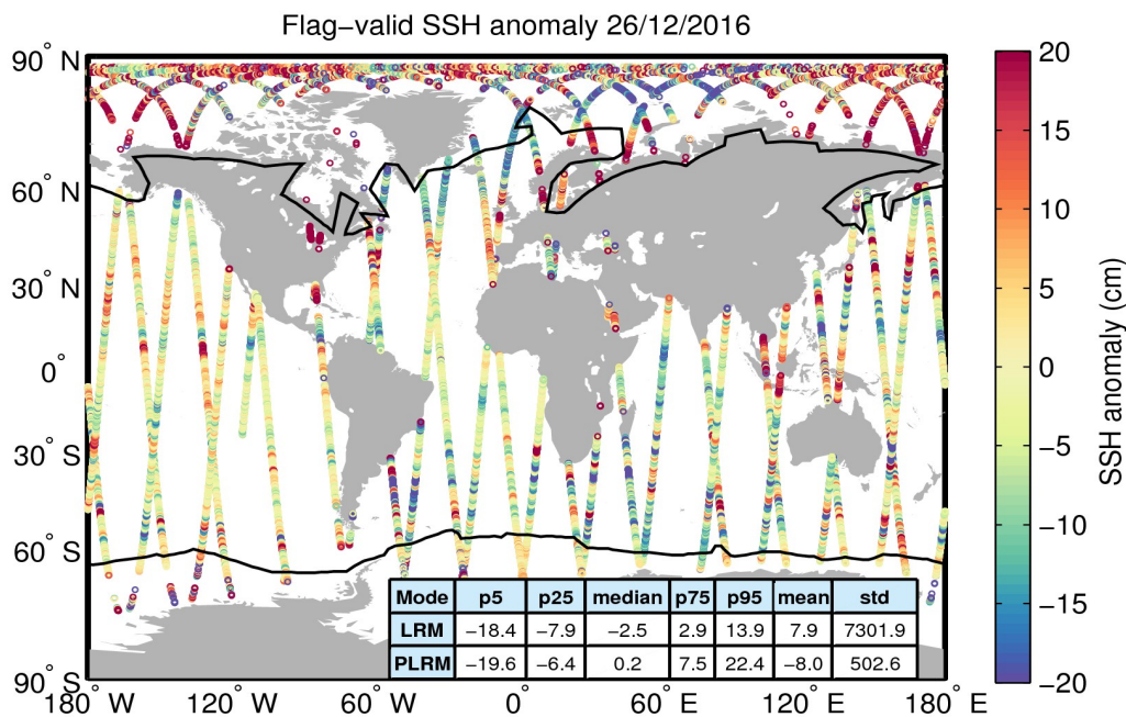
Figure 5. Geographical distribution of flag-valid 1-Hz SSH anomaly data over oceans and lakes for 26/12/2016. The statistical values shown in the table refer to the SSH anomaly in cm and are calculated separately for LRM and PLRM regions. Measurements taken over polar polygons have been excluded from the computation of the statistical values. The black lines mark the outer limit of the Arctic and Antarctic polar polygons.
