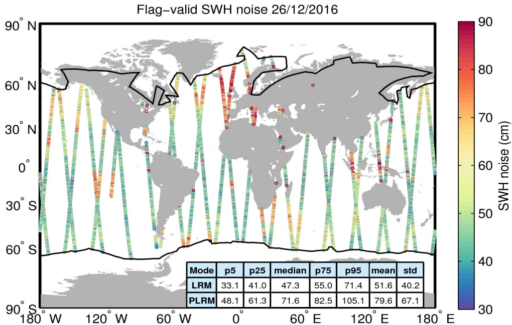
Figure 18. Geographical distribution of flag-valid 20-Hz SWH measurement noise over oceans and lakes for 26/12/2016. The statistical values shown in the table refer to the SWH noise and are calculated separately for LRM and PLRM regions. Measurements taken over polar polygons have been excluded from the computation of the statistical values. The black lines mark the outer limit of the Arctic and Antarctic polar polygons.
