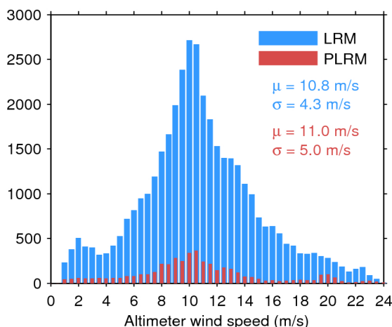
Figure 33. Histogram of flag-valid wind over oceans and lakes for LRM (blue) and PLRM (red) for 26/12/2016. The mean ( \mu ) and standard deviation ( \sigma ) are also shown. Note that values larger than 24 m/s are excluded from the histogram for the sake of readability but not from the computation of \mu and \sigma .
