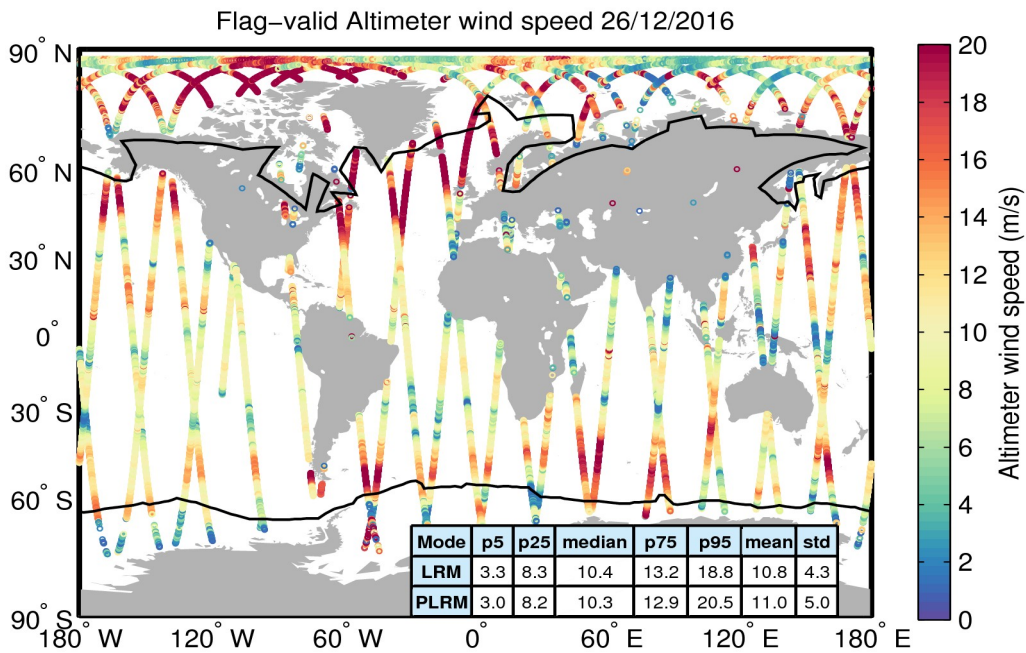
Figure 31. Geographical distribution of flag-valid wind data over oceans and lakes for 26/12/2016. The statistical values shown in the table refer to the wind in m/s and are calculated separately for LRM and PLRM regions. Measurements taken over polar polygons have been excluded from the computation of the statistical values. The black lines mark the outer limit of the Arctic and Antarctic polar polygons.
