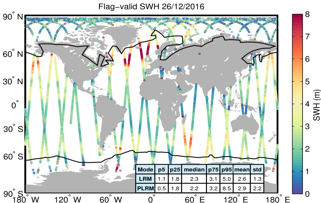
Figure 15. Geographical distribution of flag-valid SWH data over oceans and lakes for 26/12/2016. The statistical values shown in the table refer to the SWH in m and are calculated separately for LRM and PLRM regions. Measurements taken over polar polygons have been excluded from the computation of the statistical values. The black lines mark the outer limit of the Arctic and Antarctic polar polygons.
