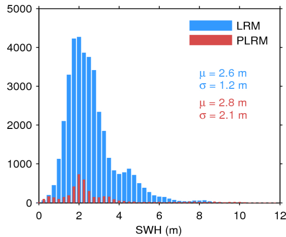
Figure 20. Histogram of science-valid SWH over oceans and lakes for LRM (blue) and PLRM (red) for 26/12/2016. The mean ( \mu ) and standard deviation ( \sigma ) are also shown. Note that values larger than 12 m are excluded from the histogram for the sake of readability but not from the computation of \mu and \sigma .
