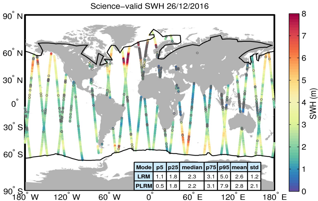
Figure 19. Geographical distribution of science-valid SWH data over oceans and lakes for 26/12/2016. The statistical values shown in the table refer to the SWH in m and are calculated separately for LRM and PLRM regions. The black lines mark the outer limit of the Arctic and Antarctic polar polygons. Gray circles denote records that have been rejected based on the editing criteria described in Table 3.
