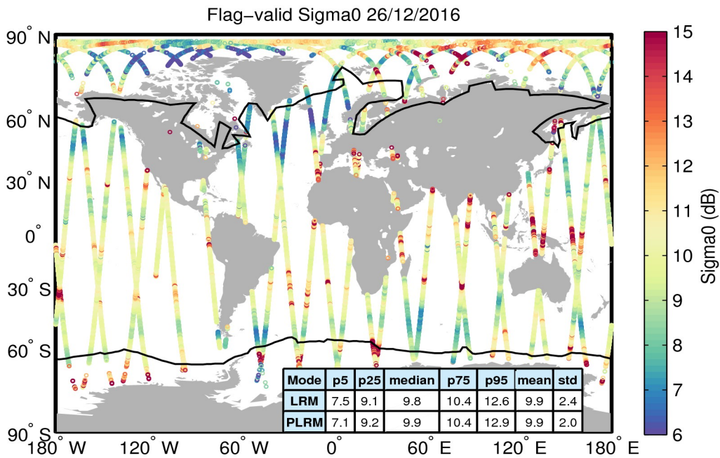
Figure 23. Geographical distribution of flag-valid sigma0 data over oceans and lakes for 26/12/2016. The statistical values shown in the table refer to the sigma0 in dB and are calculated separately for LRM and PLRM regions. Measurements taken over polar polygons have been excluded from the computation of the statistical values. The black lines mark the outer limit of the Arctic and Antarctic polar polygons.
