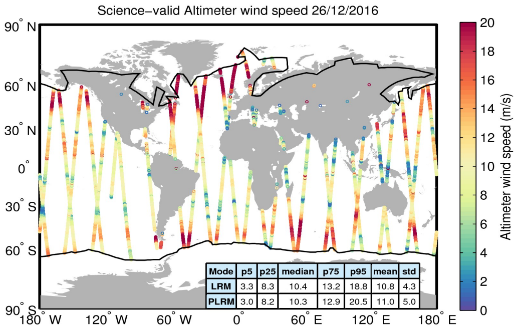
Figure 34. Geographical distribution of science-valid wind data over oceans and lakes for 26/12/2016. The statistical values shown in the table refer to the wind in m/s and are calculated separately for LRM and PLRM regions. The black lines mark the outer limit of the Arctic and Antarctic polar polygons. Gray circles denote records that have been rejected based on the editing criteria described in Table 5.
