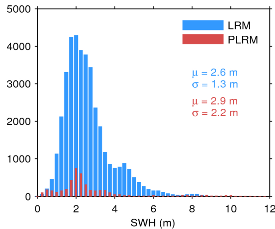
Figure 17. Histogram of flag-valid SWH over oceans and lakes for LRM (blue) and PLRM (red) for 26/12/2016. The mean ( \mu ) and standard deviation ( \sigma ) are also shown. Note that values larger than 12 m are excluded from the histogram for the sake of readability but not from the computation of \mu and \sigma .
