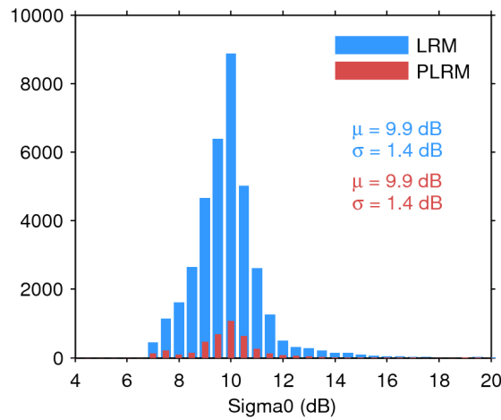
Figure 28. Histogram of science-valid sigma0 over oceans and lakes for LRM (blue) and PLRM (red) for 26/12/2016. The mean ( \mu ) and standard deviation ( \sigma ) are also shown. Note that values outside [4 20] dB are excluded from the histogram for the sake of readability but not from the computation of \mu and \sigma .
