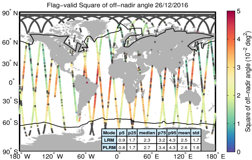
Figure 37. Geographical distribution of flag-valid mispointing data over oceans and lakes for 26/12/2016. The statistical values shown in the table refer to the mispointing in 10^{-2} deg 2 and are calculated separately for LRM and PLRM regions. Measurements taken over polar polygons have been excluded from the computation of the statistical values. The black lines mark the outer limit of the Arctic and Antarctic polar polygons. Gray circles denote negative values.
