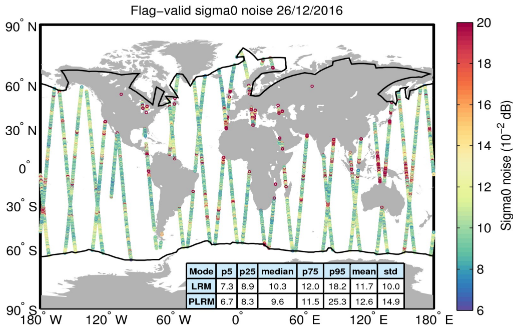
Figure 26. Geographical distribution of flag-valid 20-Hz sigma0 measurement noise over oceans and lakes for 26/12/2016. The statistical values shown in the table refer to the sigma0 noise and are calculated separately for LRM and PLRM regions. Measurements taken over polar polygons have been excluded from the computation of the statistical values. The black lines mark the outer limit of the Arctic and Antarctic polar polygons.
