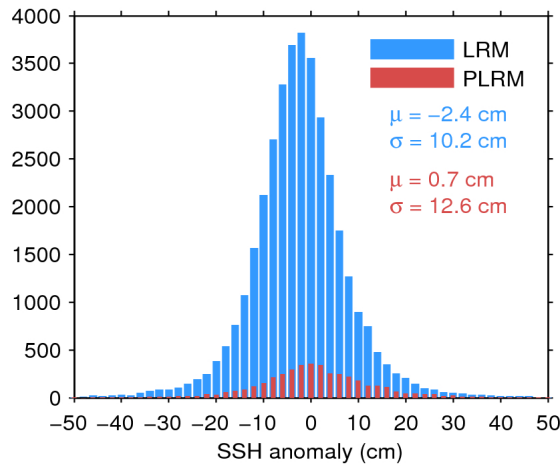
Figure 11. Histogram of science-valid SSH anomaly over oceans and lakes for LRM (blue) and PLRM (red) for 26/12/2016. The mean ( \mu ) and standard deviation ( \sigma ) are also shown. Note that values outside [-50 50] cm are excluded from the histogram for the sake of readability but not from the computation of \mu and \sigma .
