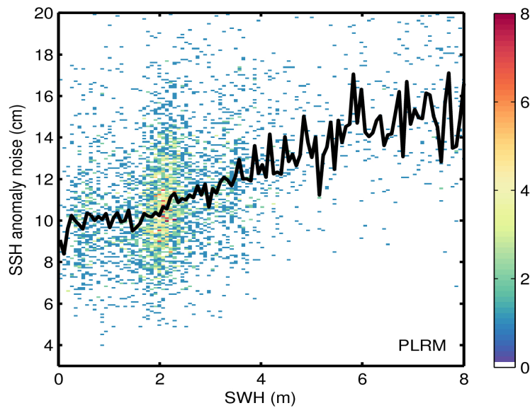
Figure 9. 2D histogram showing flag-valid SSH anomaly noise as a function of SWH for LRM (top) and PLRM (bottom) for 26/12/2016. The black line denotes the median SSH anomaly noise as a function of SWH.
