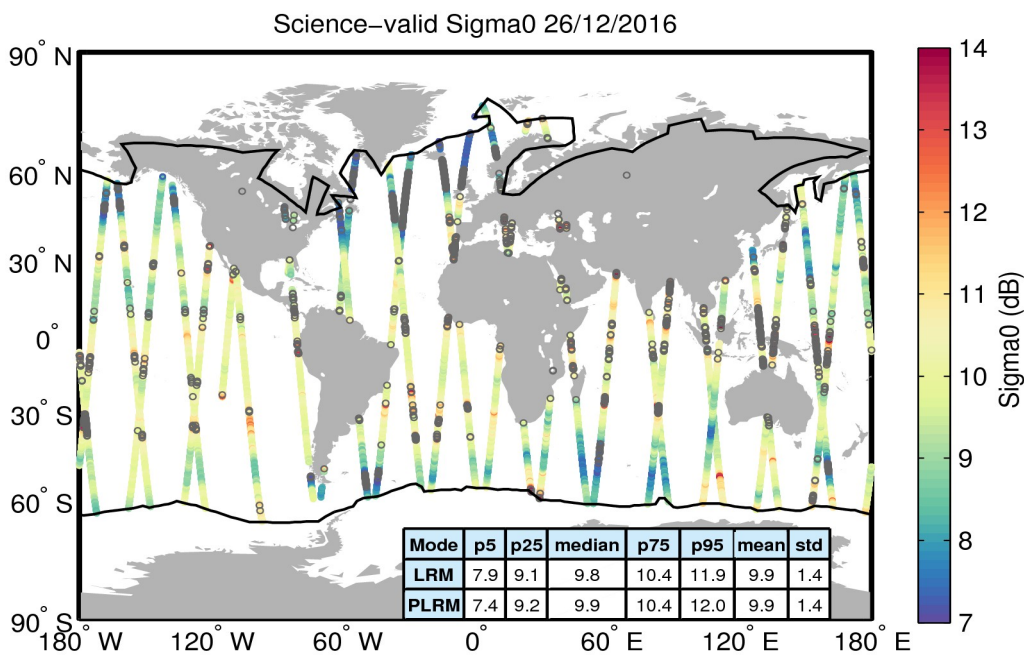
Figure 27. Geographical distribution of science-valid sigma0 data over oceans and lakes for 26/12/2016. The statistical values shown in the table refer to the sigma0 in dB and are calculated separately for LRM and PLRM regions. The black lines mark the outer limit of the Arctic and Antarctic polar polygons. Gray circles denote records that have been rejected based on the editing criteria described in Table 4.
