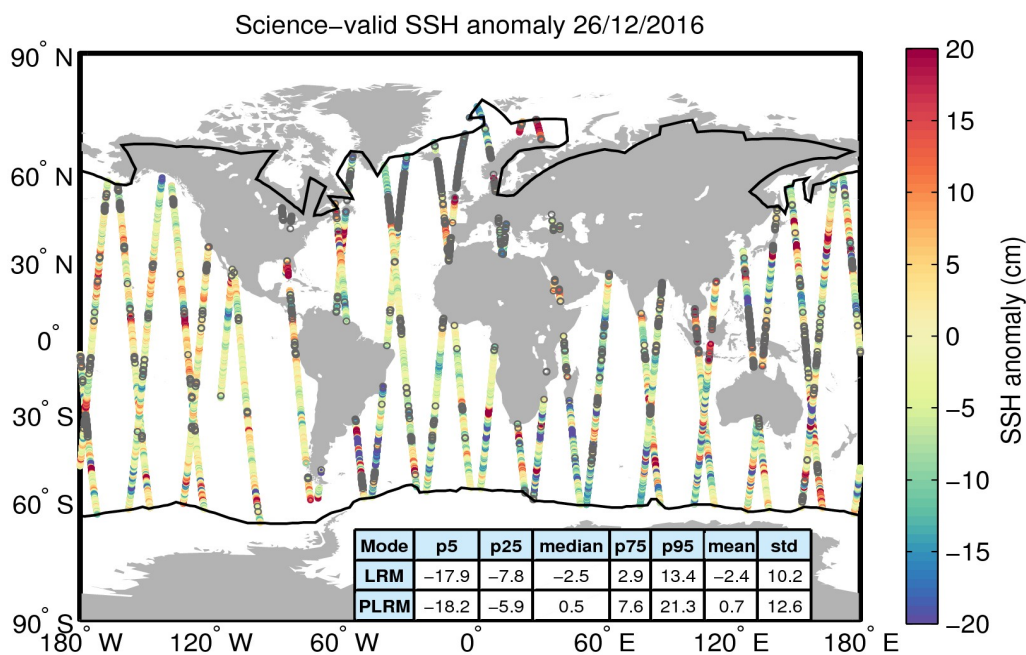
Figure 10. Geographical distribution of science-valid SSH anomaly data over oceans and lakes for 26/12/2016. The statistical values shown in the table refer to the SSH anomaly in cm and are calculated separately for LRM and PLRM regions. The black lines mark the outer limit of the Arctic and Antarctic polar polygons. Gray circles denote records that have been rejected based on the editing criteria described in Table 2.
