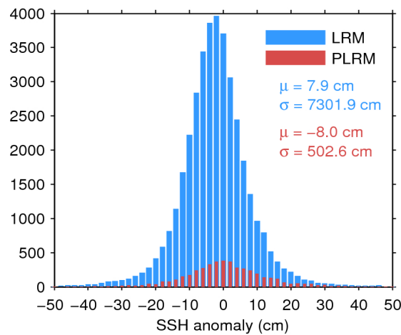
Figure 7. Histogram of flag-valid SSH anomaly over oceans and lakes for LRM (blue) and PLRM (red) for 26/12/2016. The mean ( \mu ) and standard deviation ( \sigma ) are also shown. Note that values outside [-50 \ 50] cm are excluded from the histogram for the sake of readability but not from the computation of \mu and \sigma .
