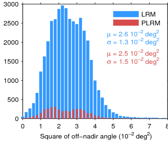
Figure 39. Histogram of flag-valid mispointing over oceans and lakes for LRM (blue) and PLRM (red) for 25/12/2016. Only positive values have been considered. The mean ( \mu ) and standard deviation ( \sigma ) are also shown. Note that values larger than 8 \cdot 10^{-2} \text{ deg}^2 are excluded from the histogram for the sake of readability but not from the computation of \mu and \sigma .
