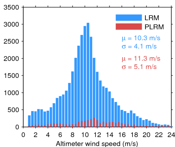
Figure 35. Histogram of science-valid wind over oceans and lakes for LRM (blue) and PLRM (red) for 25/12/2016. The mean ( \mu ) and standard deviation ( \sigma ) are also shown. Note that values larger than 24 m/s are excluded from the histogram for the sake of readability but not from the computation of \mu and \sigma .
