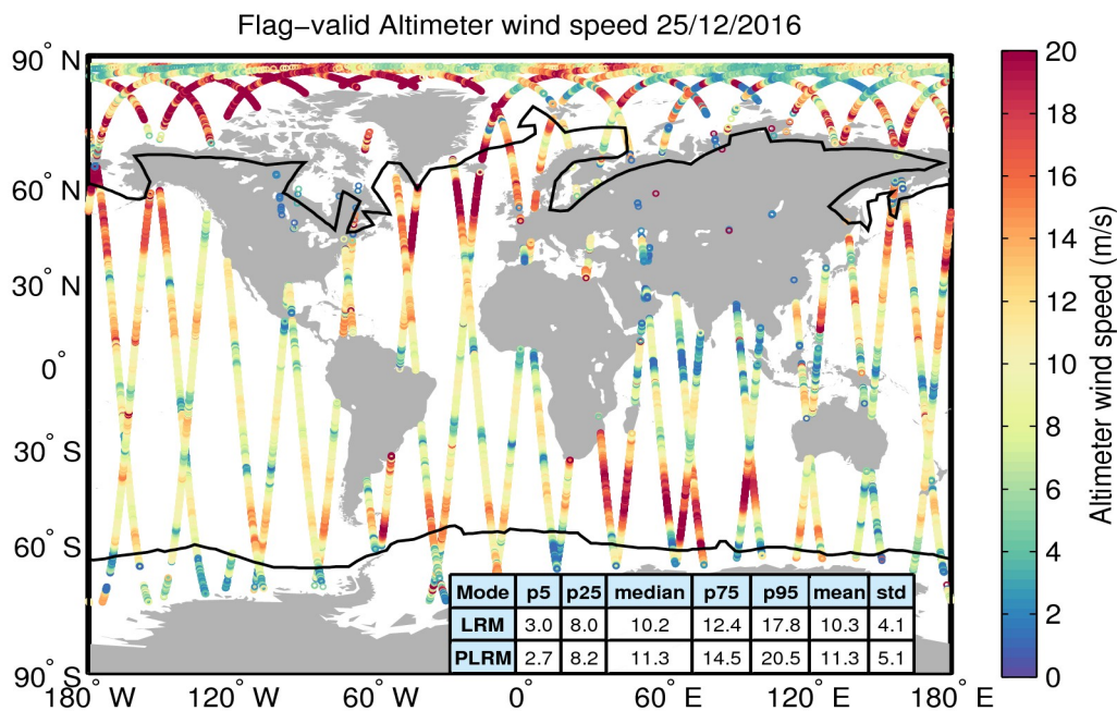
Figure 31. Geographical distribution of flag-valid wind data over oceans and lakes for 25/12/2016. The statistical values shown in the table refer to the wind in m/s and are calculated separately for LRM and PLRM regions. Measurements taken over polar polygons have been excluded from the computation of the statistical values. The black lines mark the outer limit of the Arctic and Antarctic polar polygons.
