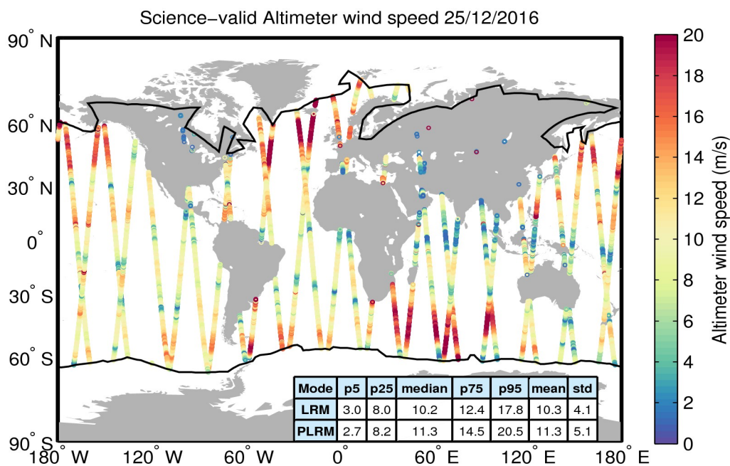
Figure 34. Geographical distribution of science-valid wind data over oceans and lakes for 25/12/2016. The statistical values shown in the table refer to the wind in m/s and are calculated separately for LRM and PLRM regions. The black lines mark the outer limit of the Arctic and Antarctic polar polygons. Gray circles denote records that have been rejected based on the editing criteria described in Table 5.
