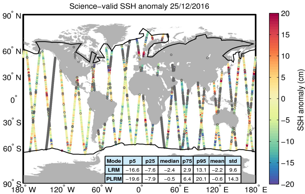
Figure 10. Geographical distribution of science-valid SSH anomaly data over oceans and lakes for 25/12/2016. The statistical values shown in the table refer to the SSH anomaly in cm and are calculated separately for LRM and PLRM regions. The black lines mark the outer limit of the Arctic and Antarctic polar polygons. Gray circles denote records that have been rejected based on the editing criteria described in Table 2.
