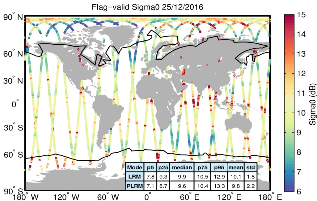
Figure 23. Geographical distribution of flag-valid sigma0 data over oceans and lakes for 25/12/2016. The statistical values shown in the table refer to the sigma0 in dB and are calculated separately for LRM and PLRM regions. Measurements taken over polar polygons have been excluded from the computation of the statistical values. The black lines mark the outer limit of the Arctic and Antarctic polar polygons.
