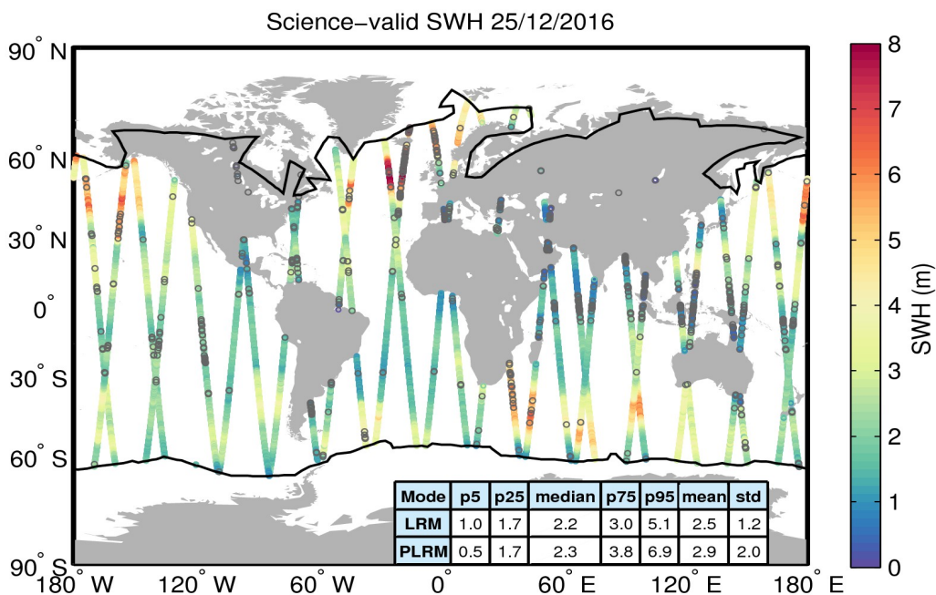
Figure 19. Geographical distribution of science-valid SWH data over oceans and lakes for 25/12/2016. The statistical values shown in the table refer to the SWH in m and are calculated separately for LRM and PLRM regions. The black lines mark the outer limit of the Arctic and Antarctic polar polygons. Gray circles denote records that have been rejected based on the editing criteria described in Table 3.
