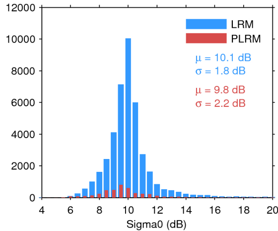
Figure 25. Histogram of flag-valid sigma0 over oceans and lakes for LRM (blue) and PLRM (red) for 25/12/2016. The mean ( \mu ) and standard deviation ( \sigma ) are also shown. Note that values outside [4 20] dB are excluded from the histogram for the sake of readability but not from the computation of \mu and \sigma .
