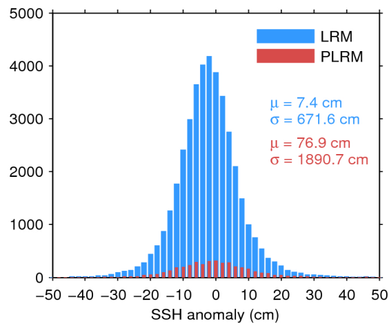
Figure 7. Histogram of flag-valid SSH anomaly over oceans and lakes for LRM (blue) and PLRM (red) for 25/12/2016. The mean ( \mu ) and standard deviation ( \sigma ) are also shown. Note that values outside [-50\ 50] cm are excluded from the histogram for the sake of readability but not from the computation of \mu and \sigma .
