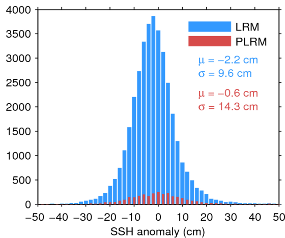
Figure 11. Histogram of science-valid SSH anomaly over oceans and lakes for LRM (blue) and PLRM (red) for 25/12/2016. The mean ( \mu ) and standard deviation ( \sigma ) are also shown. Note that values outside [-50 50] cm are excluded from the histogram for the sake of readability but not from the computation of \mu and \sigma .
