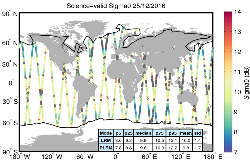
Figure 27. Geographical distribution of science-valid sigma0 data over oceans and lakes for 25/12/2016. The statistical values shown in the table refer to the sigma0 in dB and are calculated separately for LRM and PLRM regions. The black lines mark the outer limit of the Arctic and Antarctic polar polygons. Gray circles denote records that have been rejected based on the editing criteria described in Table 4.
