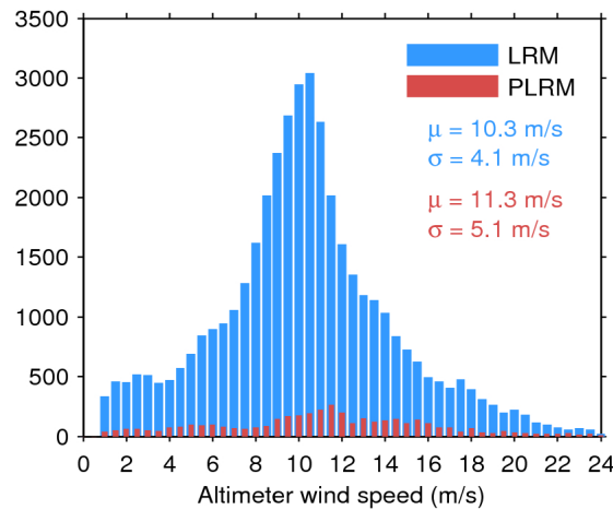
Figure 33. Histogram of flag-valid wind over oceans and lakes for LRM (blue) and PLRM (red) for 25/12/2016. The mean ( \mu ) and standard deviation ( \sigma ) are also shown. Note that values larger than 24 m/s are excluded from the histogram for the sake of readability but not from the computation of \mu and \sigma .
