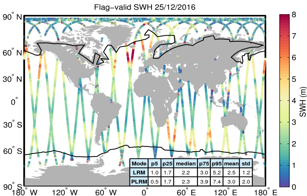
Figure 15. Geographical distribution of flag-valid SWH data over oceans and lakes for 25/12/2016. The statistical values shown in the table refer to the SWH in m and are calculated separately for LRM and PLRM regions. Measurements taken over polar polygons have been excluded from the computation of the statistical values. The black lines mark the outer limit of the Arctic and Antarctic polar polygons.
