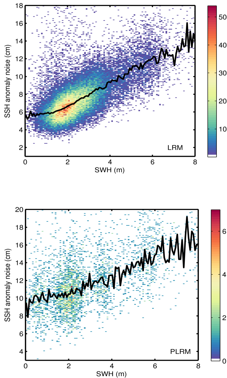
Figure 9. 2D histogram showing flag-valid SSH anomaly noise as a function of SWH for LRM (top) and PLRM (bottom) for 25/12/2016. The black line denotes the median SSH anomaly noise as a function of SWH.
