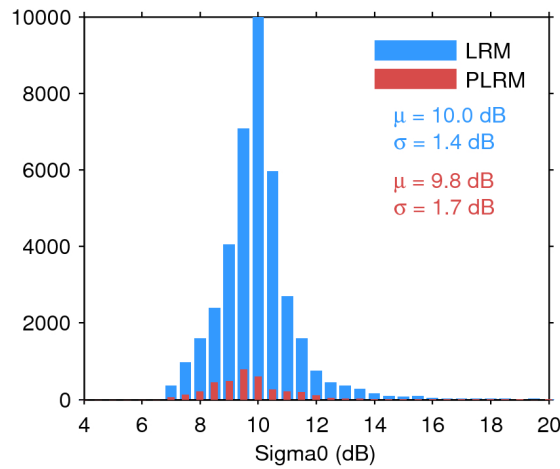
Figure 28. Histogram of science-valid sigma0 over oceans and lakes for LRM (blue) and PLRM (red) for 25/12/2016. The mean ( \mu ) and standard deviation ( \sigma ) are also shown. Note that values outside [4 20] dB are excluded from the histogram for the sake of readability but not from the computation of \mu and \sigma .
