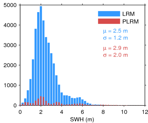
Figure 20. Histogram of science-valid SWH over oceans and lakes for LRM (blue) and PLRM (red) for 25/12/2016. The mean ( \mu ) and standard deviation ( \sigma ) are also shown. Note that values larger than 12 m are excluded from the histogram for the sake of readability but not from the computation of \mu and \sigma .
