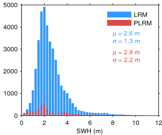
Figure 20. Histogram of science-valid SWH over oceans and lakes for LRM (blue) and PLRM (red) for 24/12/2016. The mean ( \mu ) and standard deviation ( \sigma ) are also shown. Note that values larger than 12 m are excluded from the histogram for the sake of readability but not from the computation of \mu and \sigma .
