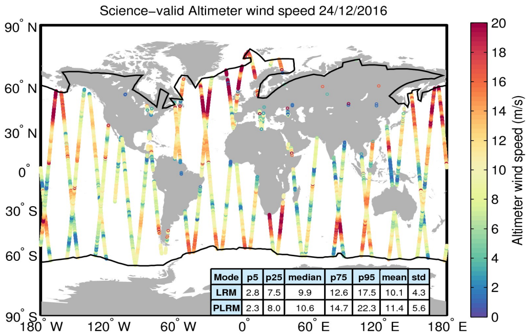
Figure 34. Geographical distribution of science-valid wind data over oceans and lakes for 24/12/2016. The statistical values shown in the table refer to the wind in m/s and are calculated separately for LRM and PLRM regions. The black lines mark the outer limit of the Arctic and Antarctic polar polygons. Gray circles denote records that have been rejected based on the editing criteria described in Table 5.
