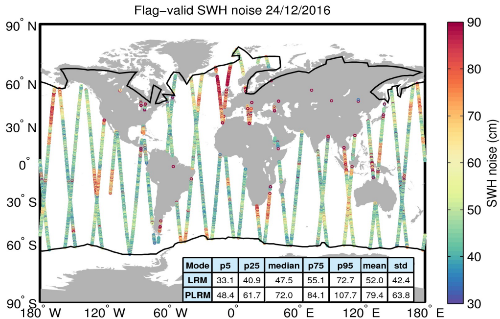
Figure 18. Geographical distribution of flag-valid 20-Hz SWH measurement noise over oceans and lakes for 24/12/2016. The statistical values shown in the table refer to the SWH noise and are calculated separately for LRM and PLRM regions. Measurements taken over polar polygons have been excluded from the computation of the statistical values. The black lines mark the outer limit of the Arctic and Antarctic polar polygons.
