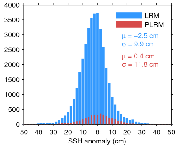
Figure 11. Histogram of science-valid SSH anomaly over oceans and lakes for LRM (blue) and PLRM (red) for 24/12/2016. The mean ( \mu ) and standard deviation ( \sigma ) are also shown. Note that values outside [-50\ 50] cm are excluded from the histogram for the sake of readability but not from the computation of \mu and \sigma .
