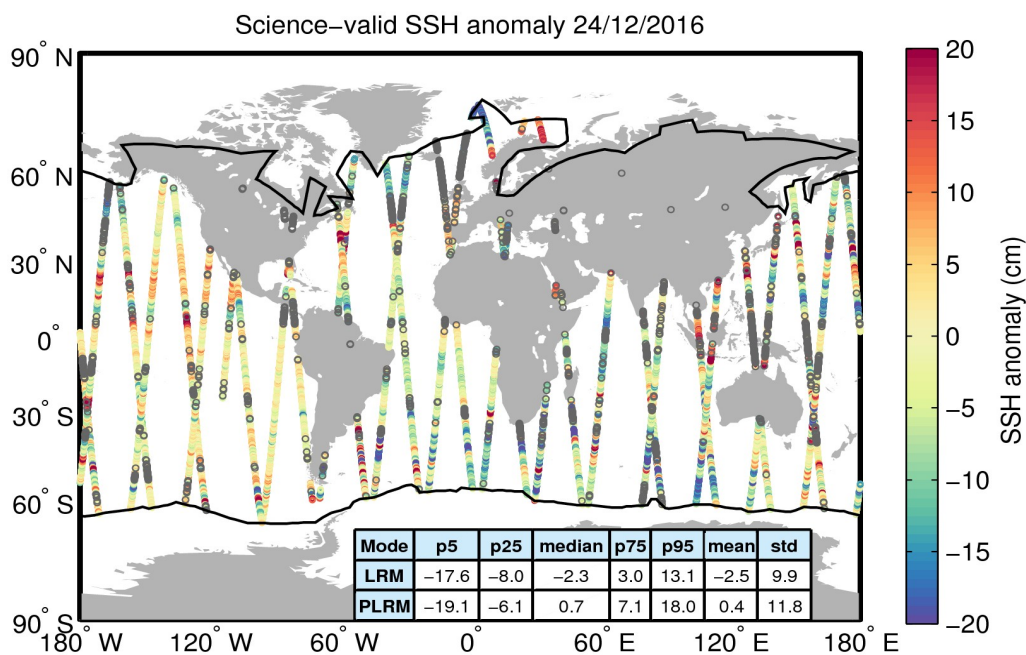
Figure 10. Geographical distribution of science-valid SSH anomaly data over oceans and lakes for 24/12/2016. The statistical values shown in the table refer to the SSH anomaly in cm and are calculated separately for LRM and PLRM regions. The black lines mark the outer limit of the Arctic and Antarctic polar polygons. Gray circles denote records that have been rejected based on the editing criteria described in Table 2.
