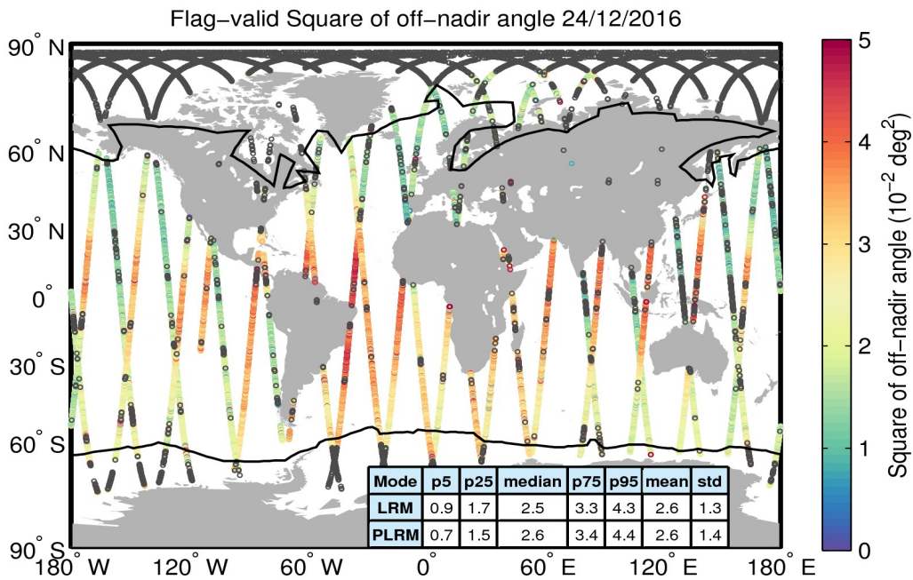
Figure 37. Geographical distribution of flag-valid mispointing data over oceans and lakes for 24/12/2016. The statistical values shown in the table refer to the mispointing in 10^{-2} deg 2 and are calculated separately for LRM and PLRM regions. Measurements taken over polar polygons have been excluded from the computation of the statistical values. The black lines mark the outer limit of the Arctic and Antarctic polar polygons. Gray circles denote negative values.
