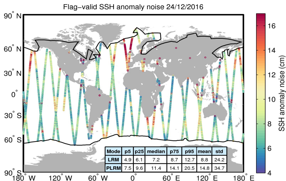
Figure 8. Geographical distribution of flag-valid 20-Hz SSH anomaly measurement noise over oceans and lakes for 24/12/2016. The statistical values shown in the table refer to the SSH anomaly noise and are calculated separately for LRM and PLRM regions. Measurements taken over polar polygons have been excluded from the computation of the statistical values. The black lines mark the outer limit of the Arctic and Antarctic polar polygons.
