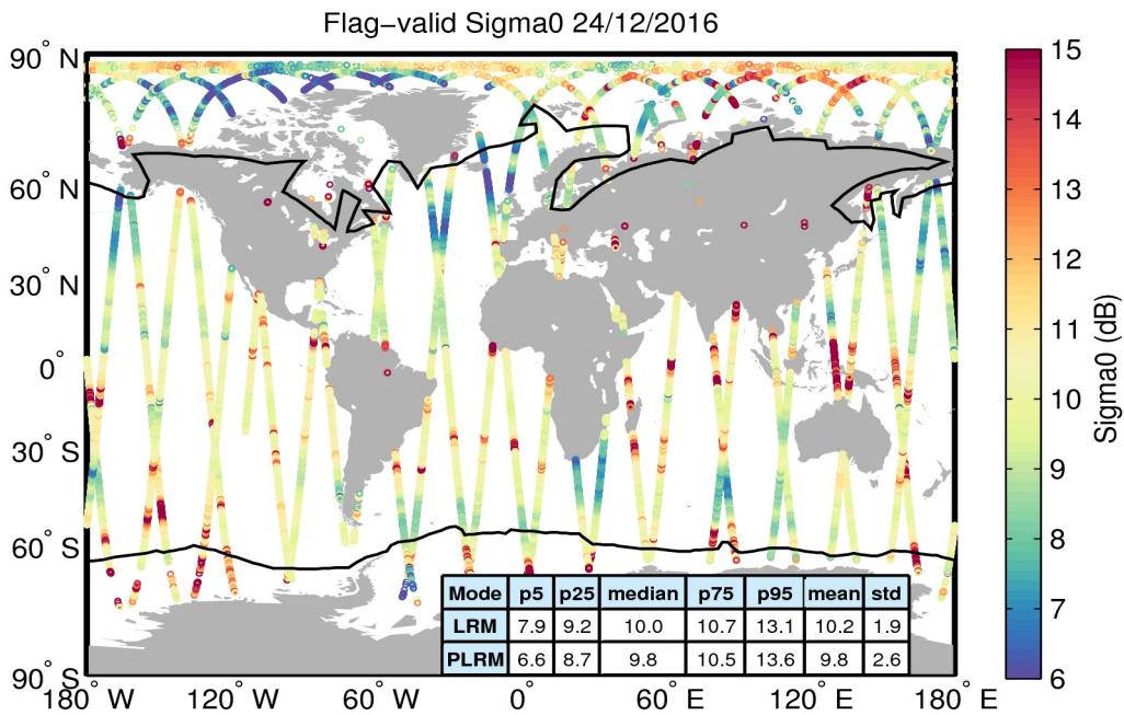
Figure 23. Geographical distribution of flag-valid sigma0 data over oceans and lakes for 24/12/2016. The statistical values shown in the table refer to the sigma0 in dB and are calculated separately for LRM and PLRM regions. Measurements taken over polar polygons have been excluded from the computation of the statistical values. The black lines mark the outer limit of the Arctic and Antarctic polar polygons.
