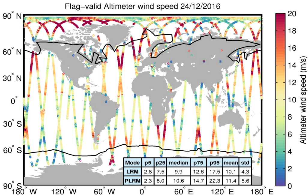
Figure 31. Geographical distribution of flag-valid wind data over oceans and lakes for 24/12/2016. The statistical values shown in the table refer to the wind in m/s and are calculated separately for LRM and PLRM regions. Measurements taken over polar polygons have been excluded from the computation of the statistical values. The black lines mark the outer limit of the Arctic and Antarctic polar polygons.
