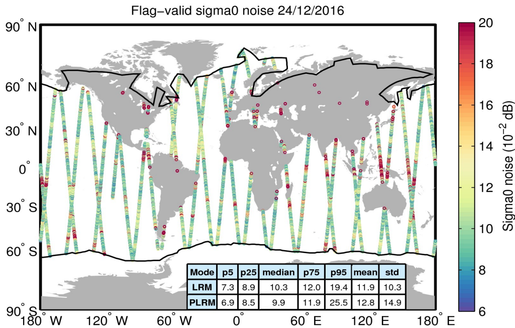
Figure 26. Geographical distribution of flag-valid 20-Hz sigma0 measurement noise over oceans and lakes for 24/12/2016. The statistical values shown in the table refer to the sigma0 noise and are calculated separately for LRM and PLRM regions. Measurements taken over polar polygons have been excluded from the computation of the statistical values. The black lines mark the outer limit of the Arctic and Antarctic polar polygons.
