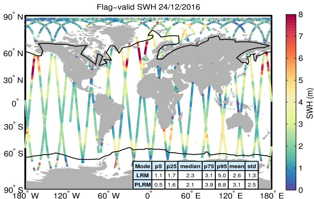
Figure 15. Geographical distribution of flag-valid SWH data over oceans and lakes for 24/12/2016. The statistical values shown in the table refer to the SWH in m and are calculated separately for LRM and PLRM regions. Measurements taken over polar polygons have been excluded from the computation of the statistical values. The black lines mark the outer limit of the Arctic and Antarctic polar polygons.
