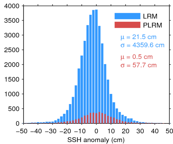
Figure 7. Histogram of flag-valid SSH anomaly over oceans and lakes for LRM (blue) and PLRM (red) for 24/12/2016. The mean ( \mu ) and standard deviation ( \sigma ) are also shown. Note that values outside [-50 50] cm are excluded from the histogram for the sake of readability but not from the computation of \mu and \sigma .
