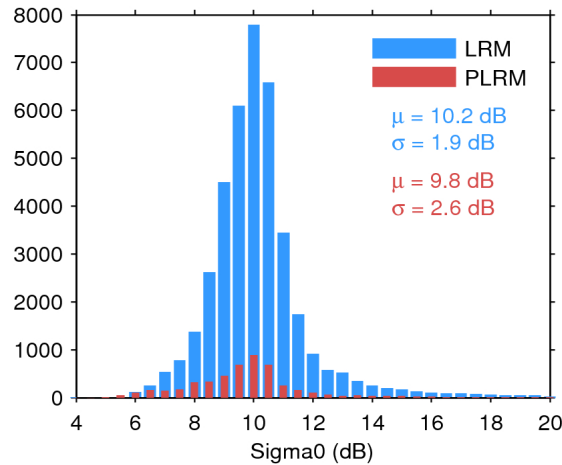
Figure 25. Histogram of flag-valid sigma0 over oceans and lakes for LRM (blue) and PLRM (red) for 24/12/2016. The mean ( \mu ) and standard deviation ( \sigma ) are also shown. Note that values outside [4 20] dB are excluded from the histogram for the sake of readability but not from the computation of \mu and \sigma .
