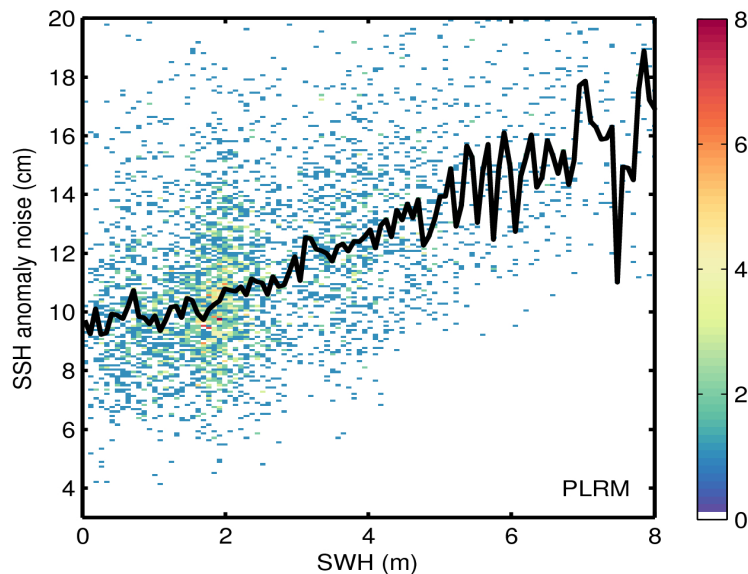
Figure 9. 2D histogram showing flag-valid SSH anomaly noise as a function of SWH for LRM (top) and PLRM (bottom) for 24/12/2016. The black line denotes the median SSH anomaly noise as a function of SWH.
