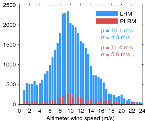
Figure 35. Histogram of science-valid wind over oceans and lakes for LRM (blue) and PLRM (red) for 24/12/2016. The mean ( \mu ) and standard deviation ( \sigma ) are also shown. Note that values larger than 24 m/s are excluded from the histogram for the sake of readability but not from the computation of \mu and \sigma .
