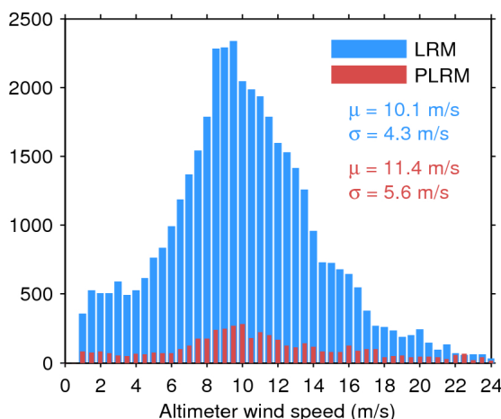
Figure 33. Histogram of flag-valid wind over oceans and lakes for LRM (blue) and PLRM (red) for 24/12/2016. The mean ( \mu ) and standard deviation ( \sigma ) are also shown. Note that values larger than 24 m/s are excluded from the histogram for the sake of readability but not from the computation of \mu and \sigma .
