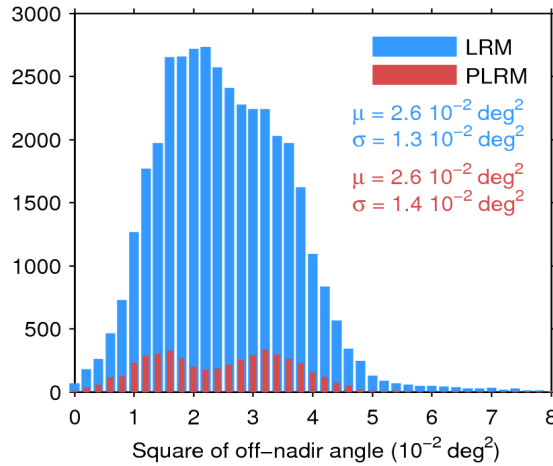
Figure 39. Histogram of flag-valid mispointing over oceans and lakes for LRM (blue) and PLRM (red) for 24/12/2016. Only positive values have been considered. The mean ( \mu ) and standard deviation ( \sigma ) are also shown. Note that values larger than 8 \cdot 10^{-2} \text{ deg}^2 are excluded from the histogram for the sake of readability but not from the computation of \mu and \sigma .
