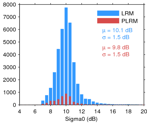
Figure 28. Histogram of science-valid sigma0 over oceans and lakes for LRM (blue) and PLRM (red) for 24/12/2016. The mean ( \mu ) and standard deviation ( \sigma ) are also shown. Note that values outside [4 20] dB are excluded from the histogram for the sake of readability but not from the computation of \mu and \sigma .
