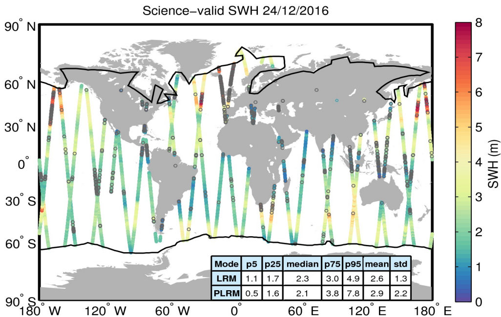
Figure 19. Geographical distribution of science-valid SWH data over oceans and lakes for 24/12/2016. The statistical values shown in the table refer to the SWH in m and are calculated separately for LRM and PLRM regions. The black lines mark the outer limit of the Arctic and Antarctic polar polygons. Gray circles denote records that have been rejected based on the editing criteria described in Table 3.
