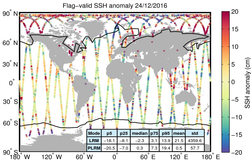
Figure 5. Geographical distribution of flag-valid 1-Hz SSH anomaly data over oceans and lakes for 24/12/2016. The statistical values shown in the table refer to the SSH anomaly in cm and are calculated separately for LRM and PLRM regions. Measurements taken over polar polygons have been excluded from the computation of the statistical values. The black lines mark the outer limit of the Arctic and Antarctic polar polygons.
