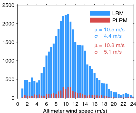
Figure 33. Histogram of flag-valid wind over oceans and lakes for LRM (blue) and PLRM (red) for 23/12/2016. The mean ( \mu ) and standard deviation ( \sigma ) are also shown. Note that values larger than 24 m/s are excluded from the histogram for the sake of readability but not from the computation of \mu and \sigma .
