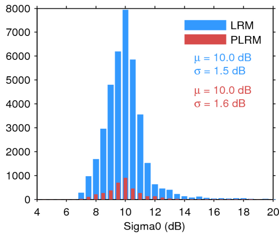
Figure 28. Histogram of science-valid sigma0 over oceans and lakes for LRM (blue) and PLRM (red) for 23/12/2016. The mean ( \mu ) and standard deviation ( \sigma ) are also shown. Note that values outside [4 20] dB are excluded from the histogram for the sake of readability but not from the computation of \mu and \sigma .
