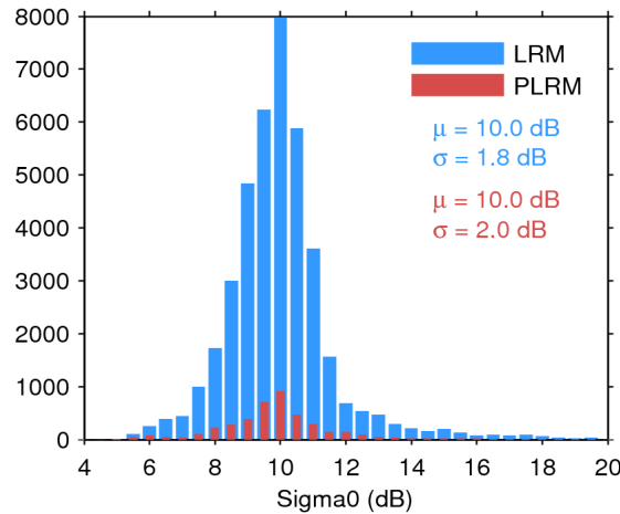
Figure 25. Histogram of flag-valid sigma0 over oceans and lakes for LRM (blue) and PLRM (red) for 23/12/2016. The mean ( \mu ) and standard deviation ( \sigma ) are also shown. Note that values outside [4 20] dB are excluded from the histogram for the sake of readability but not from the computation of \mu and \sigma .
