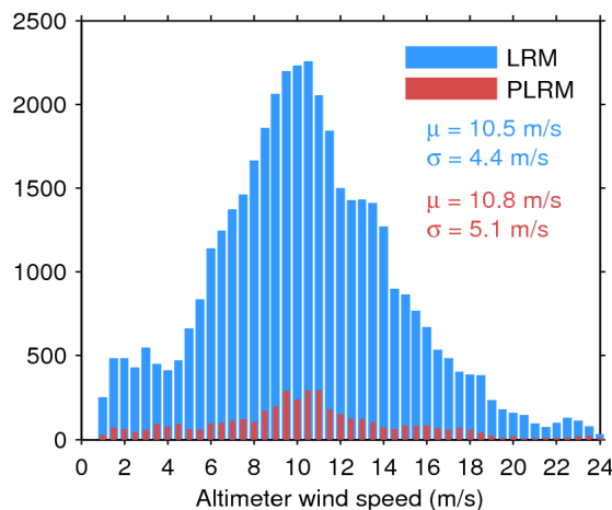
Figure 35. Histogram of science-valid wind over oceans and lakes for LRM (blue) and PLRM (red) for 23/12/2016. The mean ( \mu ) and standard deviation ( \sigma ) are also shown. Note that values larger than 24 m/s are excluded from the histogram for the sake of readability but not from the computation of \mu and \sigma .
