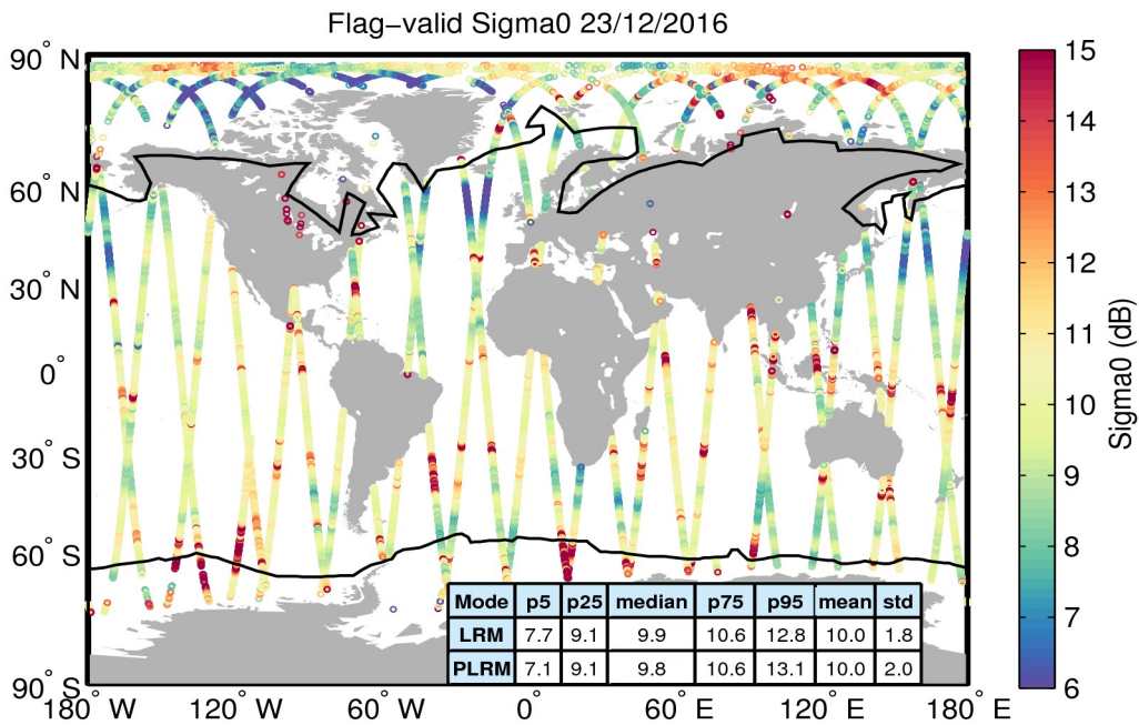
Figure 23. Geographical distribution of flag-valid sigma0 data over oceans and lakes for 23/12/2016. The statistical values shown in the table refer to the sigma0 in dB and are calculated separately for LRM and PLRM regions. Measurements taken over polar polygons have been excluded from the computation of the statistical values. The black lines mark the outer limit of the Arctic and Antarctic polar polygons.
