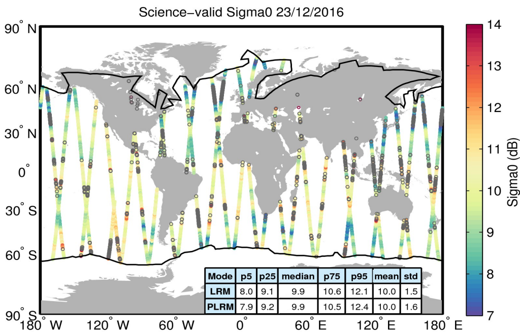
Figure 27. Geographical distribution of science-valid sigma0 data over oceans and lakes for 23/12/2016. The statistical values shown in the table refer to the sigma0 in dB and are calculated separately for LRM and PLRM regions. The black lines mark the outer limit of the Arctic and Antarctic polar polygons. Gray circles denote records that have been rejected based on the editing criteria described in Table 4.
