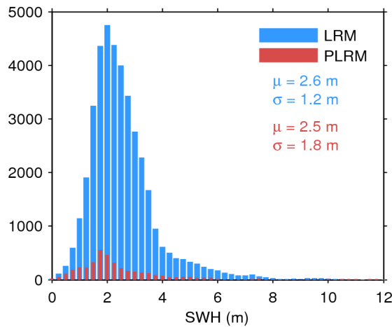
Figure 20. Histogram of science-valid SWH over oceans and lakes for LRM (blue) and PLRM (red) for 23/12/2016. The mean ( \mu ) and standard deviation ( \sigma ) are also shown. Note that values larger than 12 m are excluded from the histogram for the sake of readability but not from the computation of \mu and \sigma .
