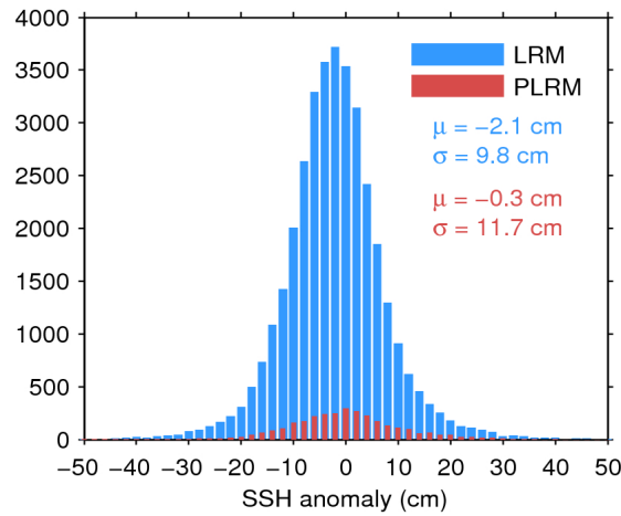
Figure 11. Histogram of science-valid SSH anomaly over oceans and lakes for LRM (blue) and PLRM (red) for 23/12/2016. The mean ( \mu ) and standard deviation ( \sigma ) are also shown. Note that values outside [-50\ 50] cm are excluded from the histogram for the sake of readability but not from the computation of \mu and \sigma .
