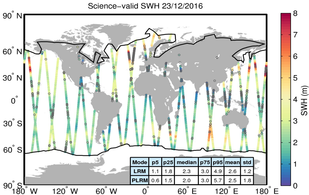
Figure 19. Geographical distribution of science-valid SWH data over oceans and lakes for 23/12/2016. The statistical values shown in the table refer to the SWH in m and are calculated separately for LRM and PLRM regions. The black lines mark the outer limit of the Arctic and Antarctic polar polygons. Gray circles denote records that have been rejected based on the editing criteria described in Table 3.
