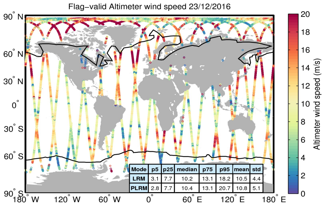
Figure 31. Geographical distribution of flag-valid wind data over oceans and lakes for 23/12/2016. The statistical values shown in the table refer to the wind in m/s and are calculated separately for LRM and PLRM regions. Measurements taken over polar polygons have been excluded from the computation of the statistical values. The black lines mark the outer limit of the Arctic and Antarctic polar polygons.
