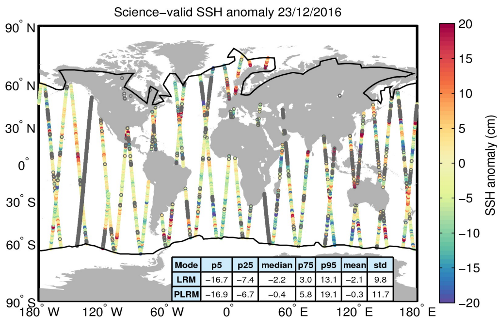
Figure 10. Geographical distribution of science-valid SSH anomaly data over oceans and lakes for 23/12/2016. The statistical values shown in the table refer to the SSH anomaly in cm and are calculated separately for LRM and PLRM regions. The black lines mark the outer limit of the Arctic and Antarctic polar polygons. Gray circles denote records that have been rejected based on the editing criteria described in Table 2.
