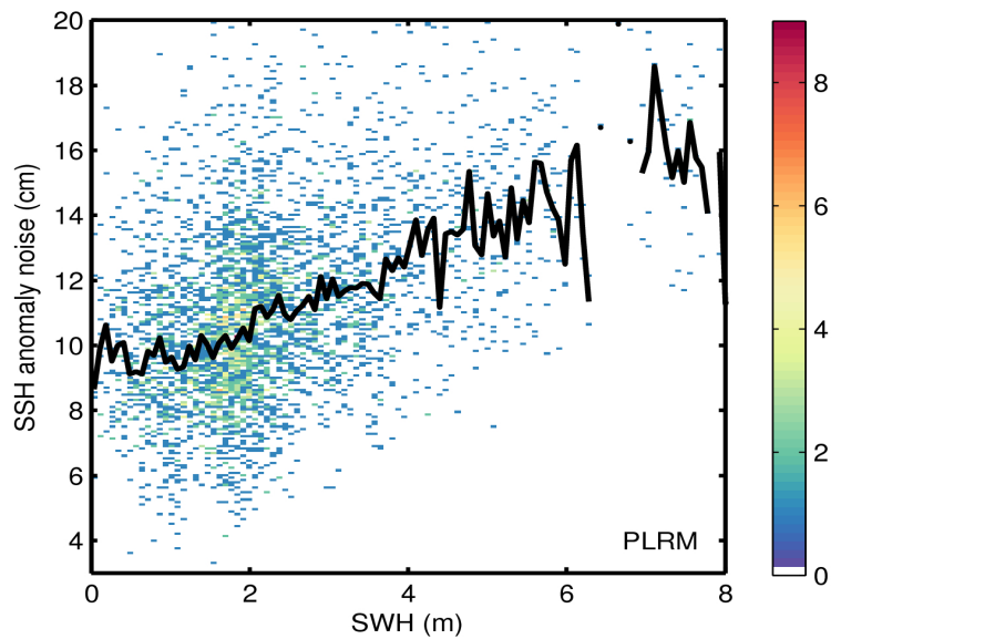
Figure 9. 2D histogram showing flag-valid SSH anomaly noise as a function of SWH for LRM (top) and PLRM (bottom) for 23/12/2016. The black line denotes the median SSH anomaly noise as a function of SWH.
