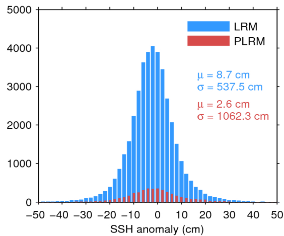
Figure 7. Histogram of flag-valid SSH anomaly over oceans and lakes for LRM (blue) and PLRM (red) for 23/12/2016. The mean ( \mu ) and standard deviation ( \sigma ) are also shown. Note that values outside [-50\ 50] cm are excluded from the histogram for the sake of readability but not from the computation of \mu and \sigma .
