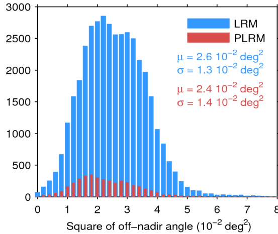
Figure 39. Histogram of flag-valid mispointing over oceans and lakes for LRM (blue) and PLRM (red) for 23/12/2016. Only positive values have been considered. The mean ( \mu ) and standard deviation ( \sigma ) are also shown. Note that values larger than 8 \cdot 10^{-2} \text{ deg}^2 are excluded from the histogram for the sake of readability but not from the computation of \mu and \sigma .
