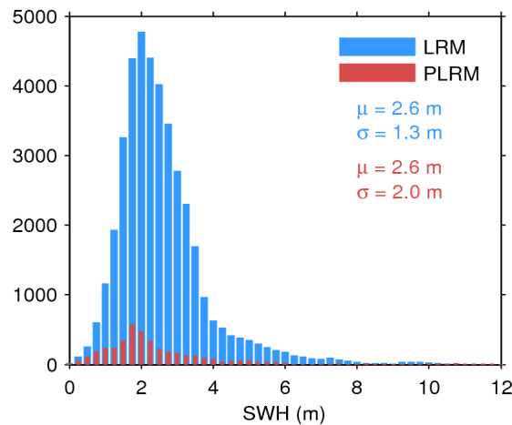
Figure 17. Histogram of flag-valid SWH over oceans and lakes for LRM (blue) and PLRM (red) for 23/12/2016. The mean ( \mu ) and standard deviation ( \sigma ) are also shown. Note that values larger than 12 m are excluded from the histogram for the sake of readability but not from the computation of \mu and \sigma .
