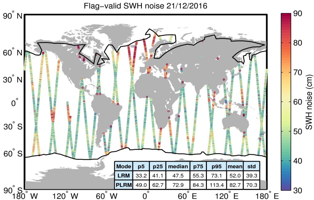
Figure 18. Geographical distribution of flag-valid 20-Hz SWH measurement noise over oceans and lakes for 21/12/2016. The statistical values shown in the table refer to the SWH noise and are calculated separately for LRM and PLRM regions. Measurements taken over polar polygons have been excluded from the computation of the statistical values. The black lines mark the outer limit of the Arctic and Antarctic polar polygons.
