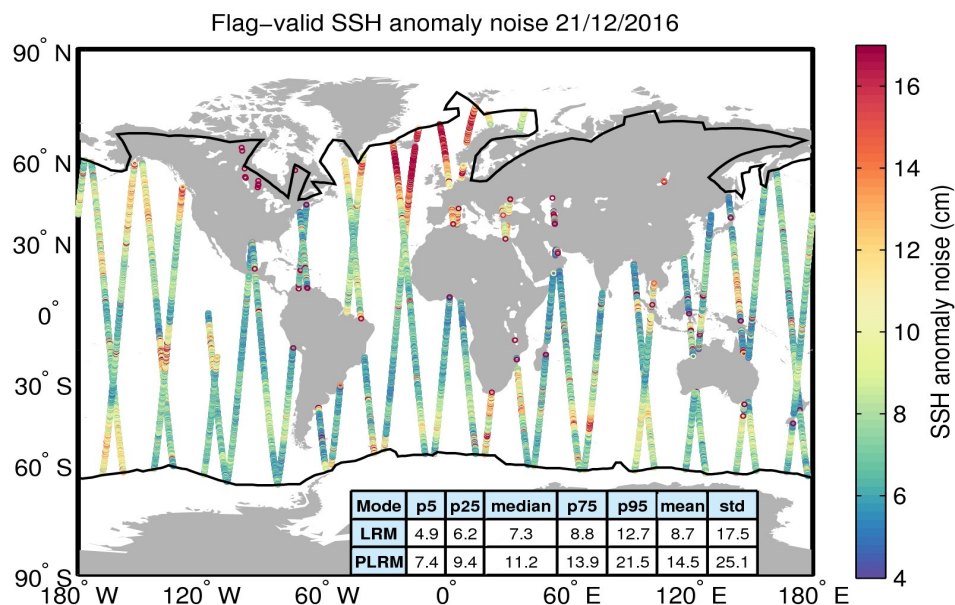
Figure 8. Geographical distribution of flag-valid 20-Hz SSH anomaly measurement noise over oceans and lakes for 21/12/2016. The statistical values shown in the table refer to the SSH anomaly noise and are calculated separately for LRM and PLRM regions. Measurements taken over polar polygons have been excluded from the computation of the statistical values. The black lines mark the outer limit of the Arctic and Antarctic polar polygons.
