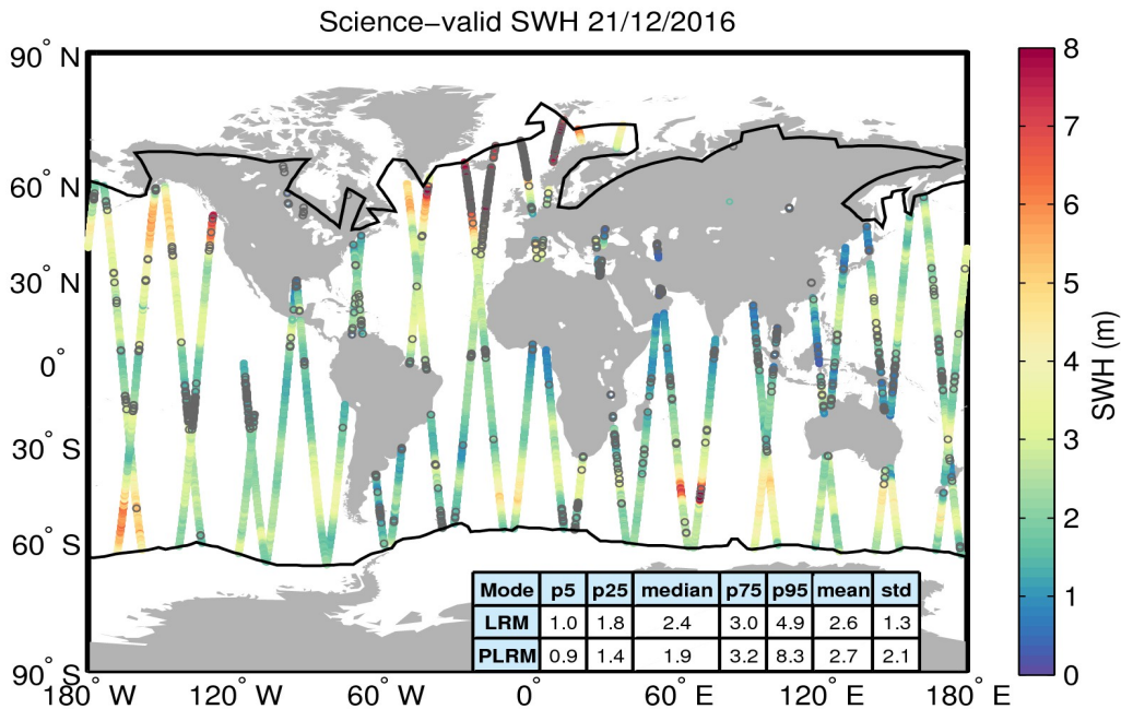
Figure 19. Geographical distribution of science-valid SWH data over oceans and lakes for 21/12/2016. The statistical values shown in the table refer to the SWH in m and are calculated separately for LRM and PLRM regions. The black lines mark the outer limit of the Arctic and Antarctic polar polygons. Gray circles denote records that have been rejected based on the editing criteria described in Table 3.
