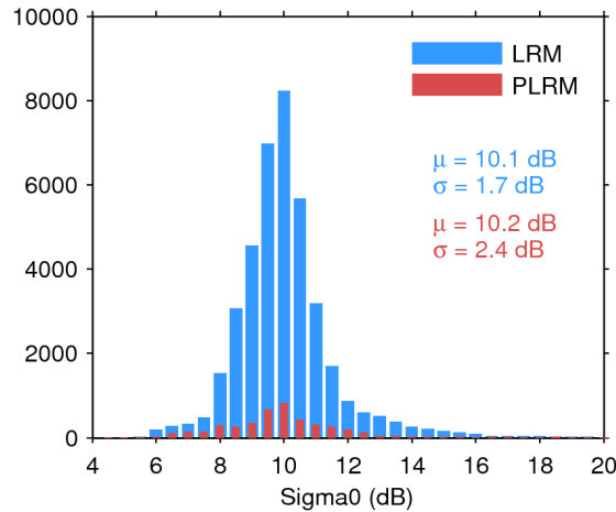
Figure 25. Histogram of flag-valid sigma0 over oceans and lakes for LRM (blue) and PLRM (red) for 21/12/2016. The mean ( \mu ) and standard deviation ( \sigma ) are also shown. Note that values outside [4 20] dB are excluded from the histogram for the sake of readability but not from the computation of \mu and \sigma .
