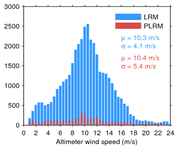
Figure 33. Histogram of flag-valid wind over oceans and lakes for LRM (blue) and PLRM (red) for 21/12/2016. The mean ( \mu ) and standard deviation ( \sigma ) are also shown. Note that values larger than 24 m/s are excluded from the histogram for the sake of readability but not from the computation of \mu and \sigma .
