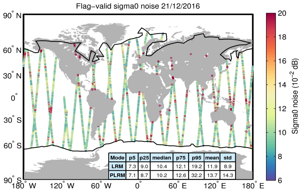
Figure 26. Geographical distribution of flag-valid 20-Hz sigma0 measurement noise over oceans and lakes for 21/12/2016. The statistical values shown in the table refer to the sigma0 noise and are calculated separately for LRM and PLRM regions. Measurements taken over polar polygons have been excluded from the computation of the statistical values. The black lines mark the outer limit of the Arctic and Antarctic polar polygons.
