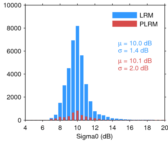
Figure 28. Histogram of science-valid sigma0 over oceans and lakes for LRM (blue) and PLRM (red) for 21/12/2016. The mean ( \mu ) and standard deviation ( \sigma ) are also shown. Note that values outside [4 20] dB are excluded from the histogram for the sake of readability but not from the computation of \mu and \sigma .
