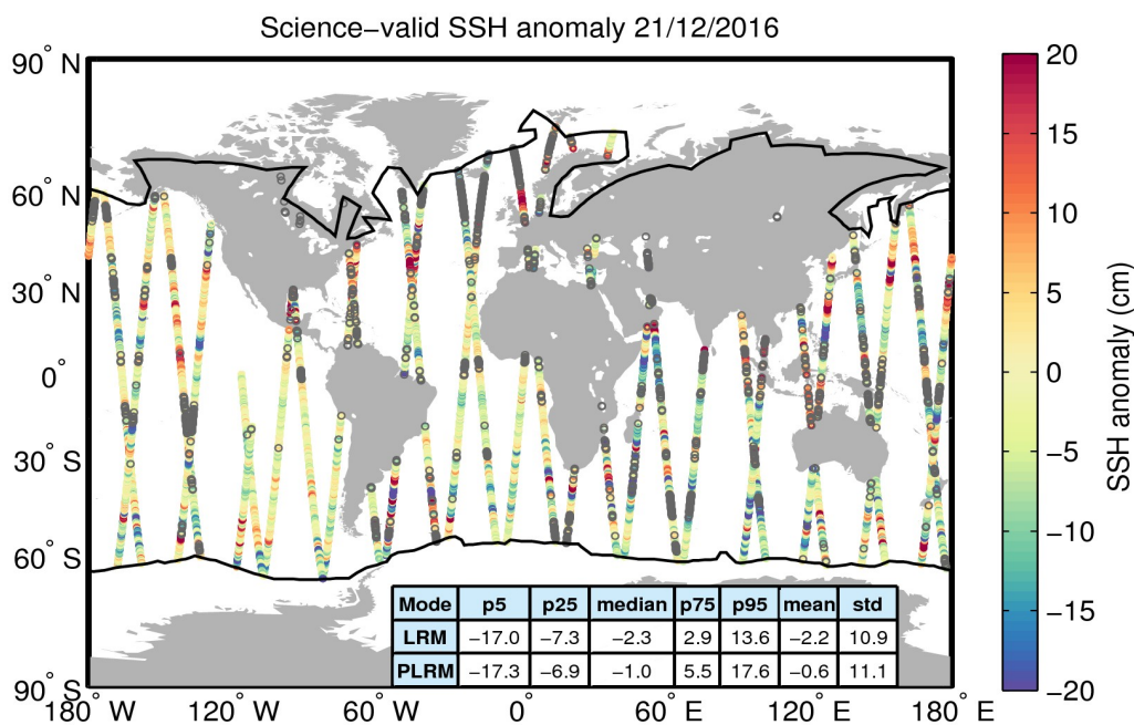
Figure 10. Geographical distribution of science-valid SSH anomaly data over oceans and lakes for 21/12/2016. The statistical values shown in the table refer to the SSH anomaly in cm and are calculated separately for LRM and PLRM regions. The black lines mark the outer limit of the Arctic and Antarctic polar polygons. Gray circles denote records that have been rejected based on the editing criteria described in Table 2.
