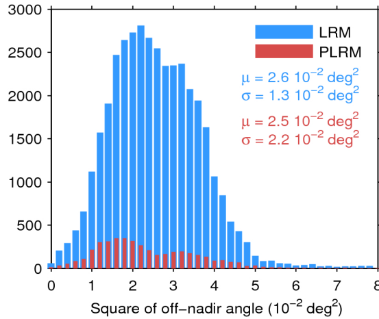
Figure 39. Histogram of flag-valid mispointing over oceans and lakes for LRM (blue) and PLRM (red) for 21/12/2016. Only positive values have been considered. The mean ( \mu ) and standard deviation ( \sigma ) are also shown. Note that values larger than 8 \cdot 10^{-2} \text{ deg}^2 are excluded from the histogram for the sake of readability but not from the computation of \mu and \sigma .
