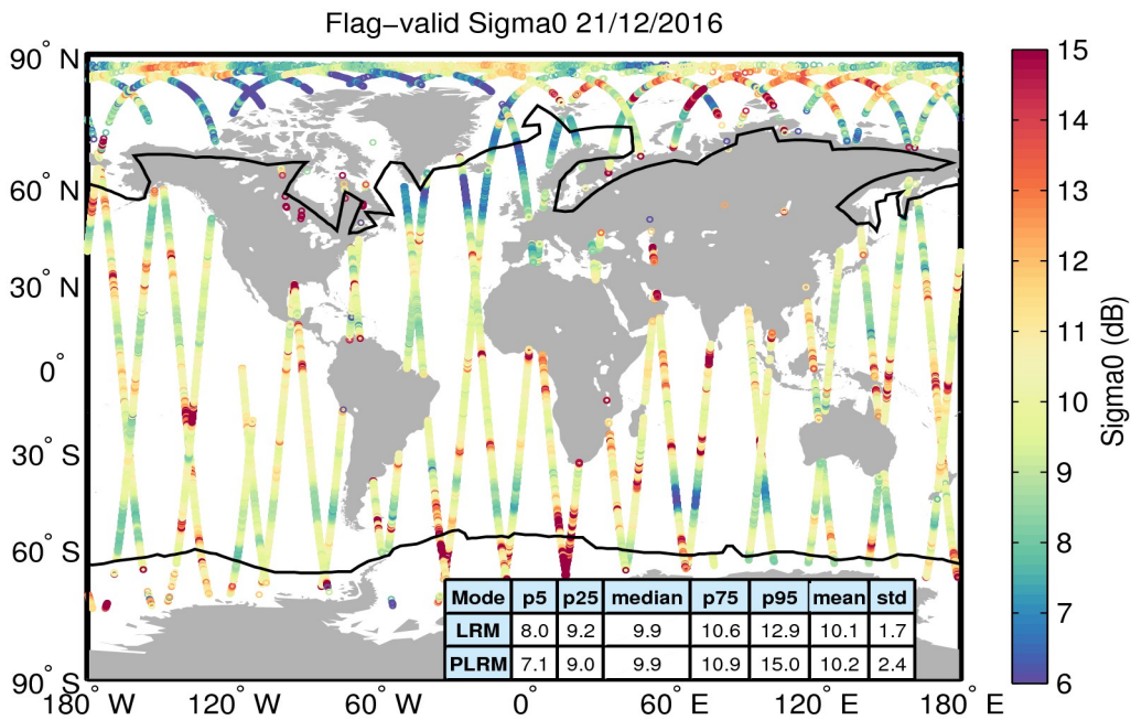
Figure 23. Geographical distribution of flag-valid sigma0 data over oceans and lakes for 21/12/2016. The statistical values shown in the table refer to the sigma0 in dB and are calculated separately for LRM and PLRM regions. Measurements taken over polar polygons have been excluded from the computation of the statistical values. The black lines mark the outer limit of the Arctic and Antarctic polar polygons.
