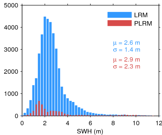
Figure 17. Histogram of flag-valid SWH over oceans and lakes for LRM (blue) and PLRM (red) for 21/12/2016. The mean ( \mu ) and standard deviation ( \sigma ) are also shown. Note that values larger than 12 m are excluded from the histogram for the sake of readability but not from the computation of \mu and \sigma .
