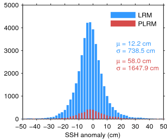
Figure 7. Histogram of flag-valid SSH anomaly over oceans and lakes for LRM (blue) and PLRM (red) for 21/12/2016. The mean ( \mu ) and standard deviation ( \sigma ) are also shown. Note that values outside [-50\ 50] cm are excluded from the histogram for the sake of readability but not from the computation of \mu and \sigma .
