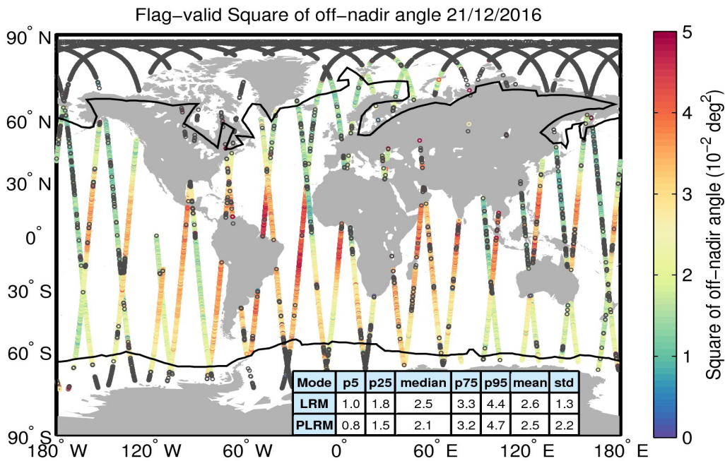
Figure 37. Geographical distribution of flag-valid mispointing data over oceans and lakes for 21/12/2016. The statistical values shown in the table refer to the mispointing in 10^{-2} deg 2 and are calculated separately for LRM and PLRM regions. Measurements taken over polar polygons have been excluded from the computation of the statistical values. The black lines mark the outer limit of the Arctic and Antarctic polar polygons. Gray circles denote negative values.
