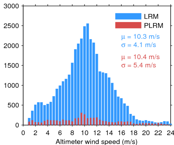
Figure 35. Histogram of science-valid wind over oceans and lakes for LRM (blue) and PLRM (red) for 21/12/2016. The mean ( \mu ) and standard deviation ( \sigma ) are also shown. Note that values larger than 24 m/s are excluded from the histogram for the sake of readability but not from the computation of \mu and \sigma .
