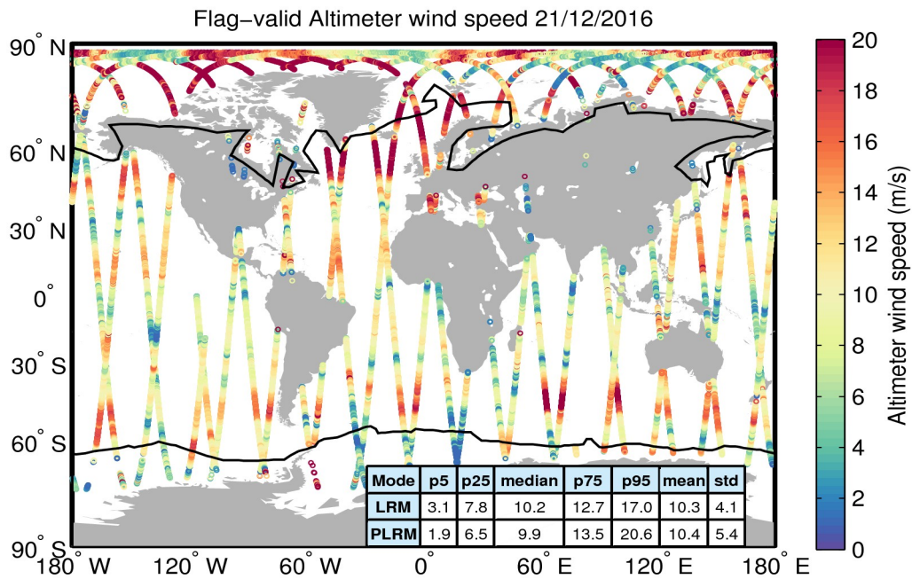
Figure 31. Geographical distribution of flag-valid wind data over oceans and lakes for 21/12/2016. The statistical values shown in the table refer to the wind in m/s and are calculated separately for LRM and PLRM regions. Measurements taken over polar polygons have been excluded from the computation of the statistical values. The black lines mark the outer limit of the Arctic and Antarctic polar polygons.
