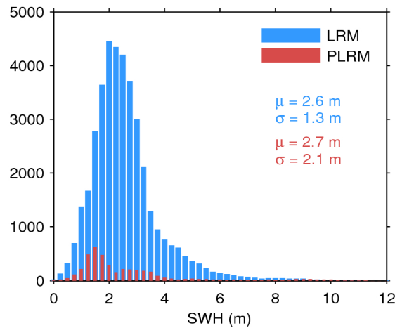
Figure 20. Histogram of science-valid SWH over oceans and lakes for LRM (blue) and PLRM (red) for 21/12/2016. The mean ( \mu ) and standard deviation ( \sigma ) are also shown. Note that values larger than 12 m are excluded from the histogram for the sake of readability but not from the computation of \mu and \sigma .
