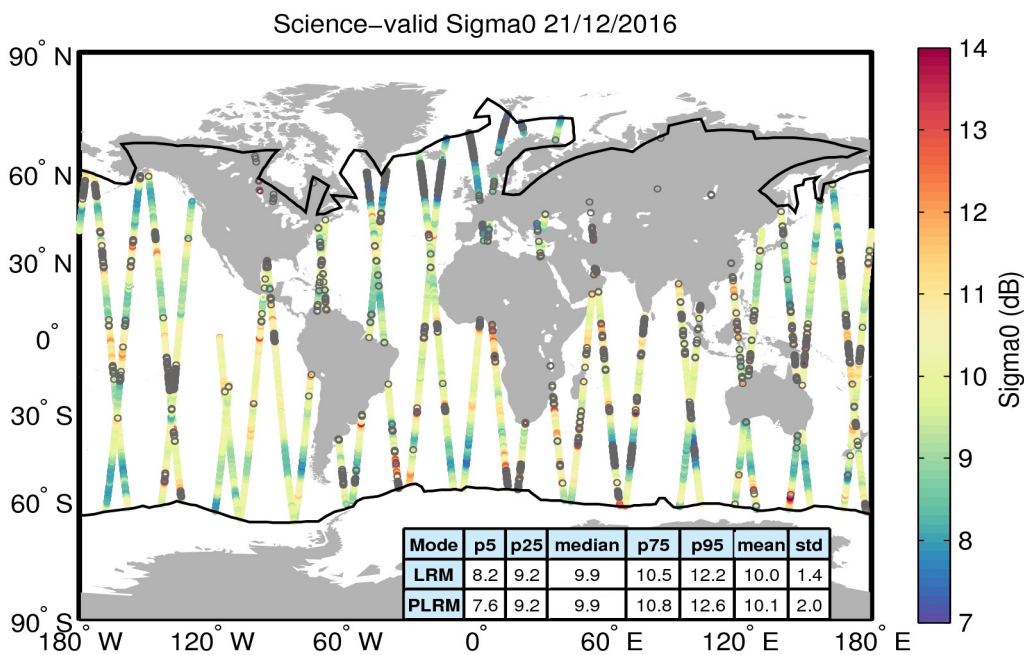
Figure 27. Geographical distribution of science-valid sigma0 data over oceans and lakes for 21/12/2016. The statistical values shown in the table refer to the sigma0 in dB and are calculated separately for LRM and PLRM regions. The black lines mark the outer limit of the Arctic and Antarctic polar polygons. Gray circles denote records that have been rejected based on the editing criteria described in Table 4.
