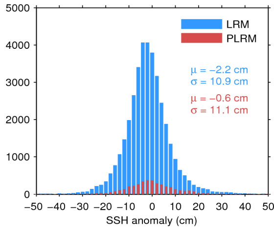
Figure 11. Histogram of science-valid SSH anomaly over oceans and lakes for LRM (blue) and PLRM (red) for 21/12/2016. The mean ( \mu ) and standard deviation ( \sigma ) are also shown. Note that values outside [-50\ 50] cm are excluded from the histogram for the sake of readability but not from the computation of \mu and \sigma .
