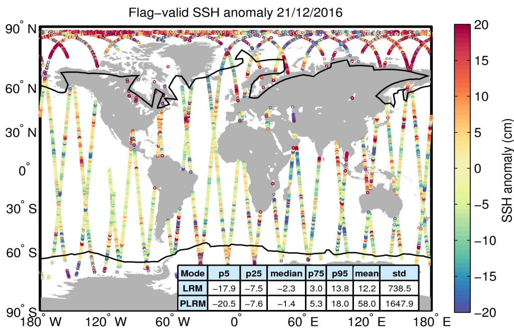
Figure 5. Geographical distribution of flag-valid 1-Hz SSH anomaly data over oceans and lakes for 21/12/2016. The statistical values shown in the table refer to the SSH anomaly in cm and are calculated separately for LRM and PLRM regions. Measurements taken over polar polygons have been excluded from the computation of the statistical values. The black lines mark the outer limit of the Arctic and Antarctic polar polygons.
