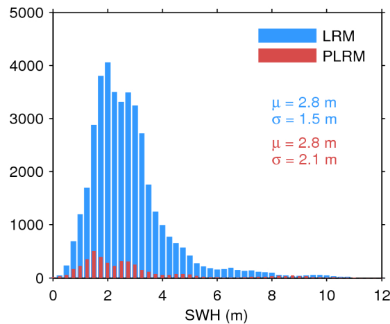
Figure 17. Histogram of flag-valid SWH over oceans and lakes for LRM (blue) and PLRM (red) for 20/12/2016. The mean ( \mu ) and standard deviation ( \sigma ) are also shown. Note that values larger than 12 m are excluded from the histogram for the sake of readability but not from the computation of \mu and \sigma .
