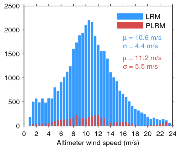
Figure 33. Histogram of flag-valid wind over oceans and lakes for LRM (blue) and PLRM (red) for 20/12/2016. The mean ( \mu ) and standard deviation ( \sigma ) are also shown. Note that values larger than 24 m/s are excluded from the histogram for the sake of readability but not from the computation of \mu and \sigma .
