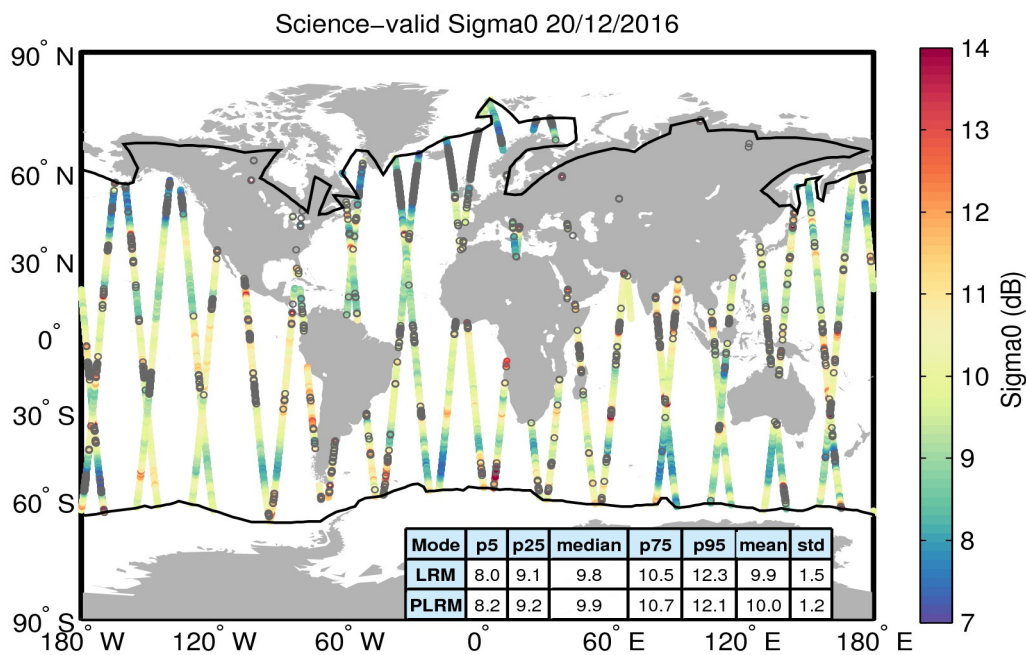
Figure 27. Geographical distribution of science-valid sigma0 data over oceans and lakes for 20/12/2016. The statistical values shown in the table refer to the sigma0 in dB and are calculated separately for LRM and PLRM regions. The black lines mark the outer limit of the Arctic and Antarctic polar polygons. Gray circles denote records that have been rejected based on the editing criteria described in Table 4.
