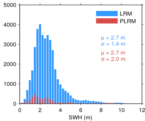
Figure 20. Histogram of science-valid SWH over oceans and lakes for LRM (blue) and PLRM (red) for 20/12/2016. The mean ( \mu ) and standard deviation ( \sigma ) are also shown. Note that values larger than 12 m are excluded from the histogram for the sake of readability but not from the computation of \mu and \sigma .
