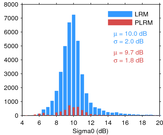
Figure 25. Histogram of flag-valid sigma0 over oceans and lakes for LRM (blue) and PLRM (red) for 20/12/2016. The mean ( \mu ) and standard deviation ( \sigma ) are also shown. Note that values outside [4 20] dB are excluded from the histogram for the sake of readability but not from the computation of \mu and \sigma .
