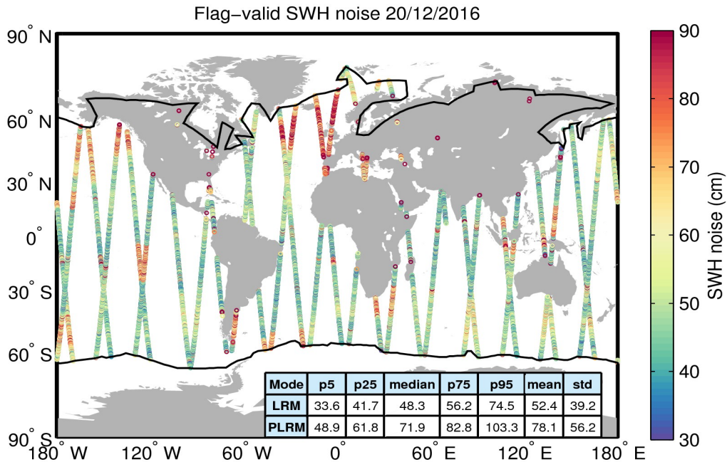
Figure 18. Geographical distribution of flag-valid 20-Hz SWH measurement noise over oceans and lakes for 20/12/2016. The statistical values shown in the table refer to the SWH noise and are calculated separately for LRM and PLRM regions. Measurements taken over polar polygons have been excluded from the computation of the statistical values. The black lines mark the outer limit of the Arctic and Antarctic polar polygons.
