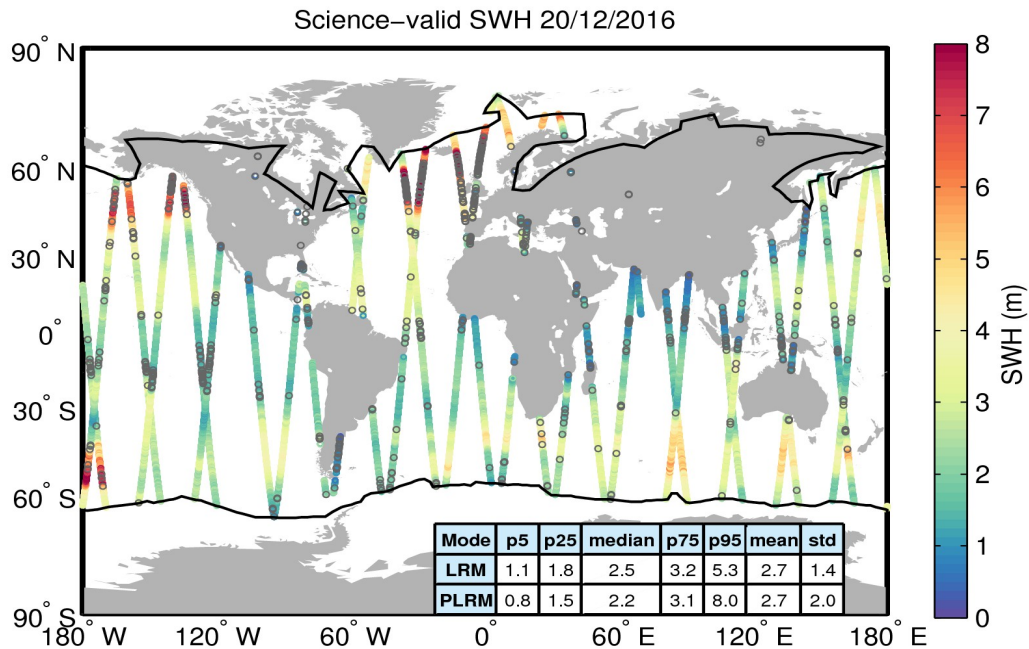
Figure 19. Geographical distribution of science-valid SWH data over oceans and lakes for 20/12/2016. The statistical values shown in the table refer to the SWH in m and are calculated separately for LRM and PLRM regions. The black lines mark the outer limit of the Arctic and Antarctic polar polygons. Gray circles denote records that have been rejected based on the editing criteria described in Table 3.
