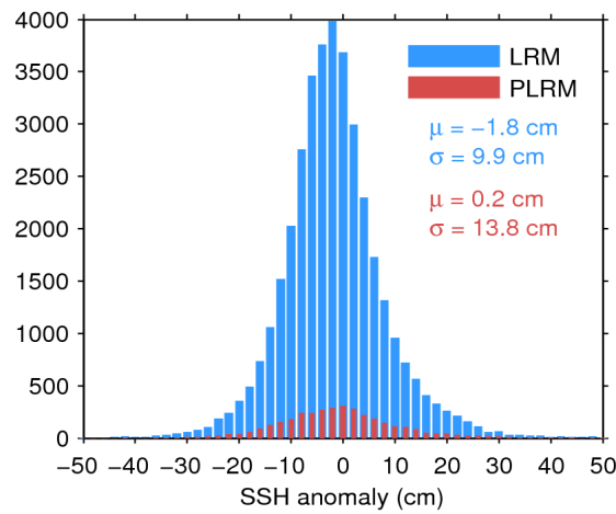
Figure 11. Histogram of science-valid SSH anomaly over oceans and lakes for LRM (blue) and PLRM (red) for 20/12/2016. The mean ( \mu ) and standard deviation ( \sigma ) are also shown. Note that values outside [-50\ 50] cm are excluded from the histogram for the sake of readability but not from the computation of \mu and \sigma .
