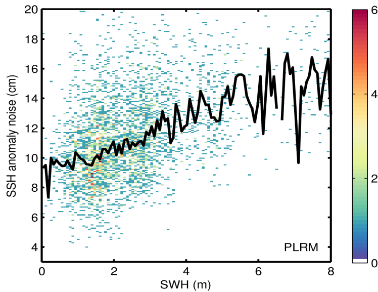
Figure 9. 2D histogram showing flag-valid SSH anomaly noise as a function of SWH for LRM (top) and PLRM (bottom) for 20/12/2016. The black line denotes the median SSH anomaly noise as a function of SWH.
