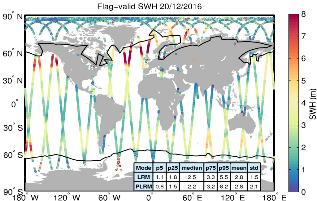
Figure 15. Geographical distribution of flag-valid SWH data over oceans and lakes for 20/12/2016. The statistical values shown in the table refer to the SWH in m and are calculated separately for LRM and PLRM regions. Measurements taken over polar polygons have been excluded from the computation of the statistical values. The black lines mark the outer limit of the Arctic and Antarctic polar polygons.
