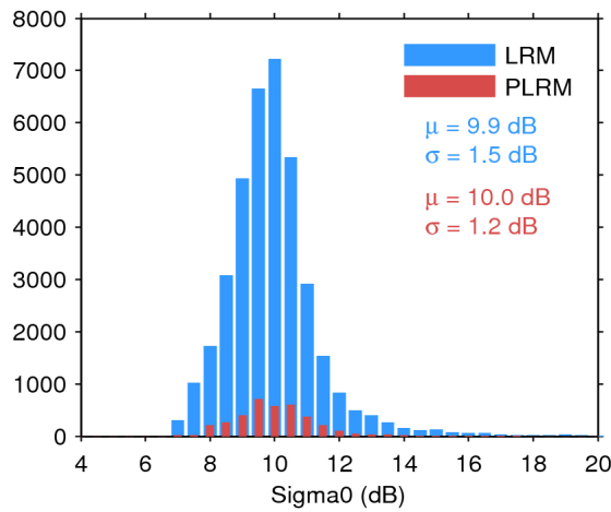
Figure 28. Histogram of science-valid sigma0 over oceans and lakes for LRM (blue) and PLRM (red) for 20/12/2016. The mean ( \mu ) and standard deviation ( \sigma ) are also shown. Note that values outside [4 20] dB are excluded from the histogram for the sake of readability but not from the computation of \mu and \sigma .
