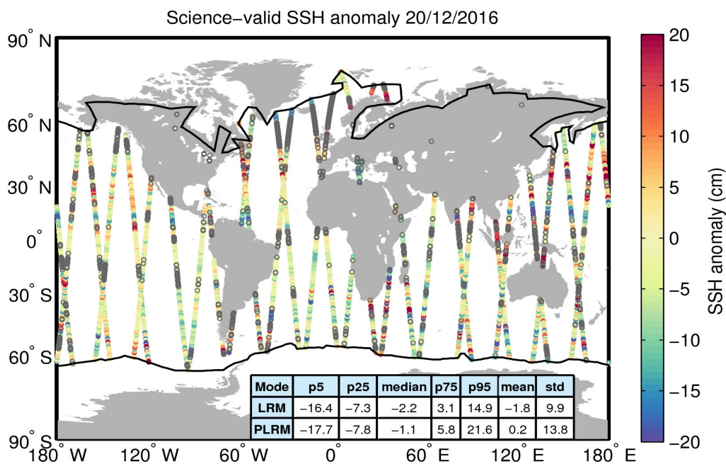
Figure 10. Geographical distribution of science-valid SSH anomaly data over oceans and lakes for 20/12/2016. The statistical values shown in the table refer to the SSH anomaly in cm and are calculated separately for LRM and PLRM regions. The black lines mark the outer limit of the Arctic and Antarctic polar polygons. Gray circles denote records that have been rejected based on the editing criteria described in Table 2.
