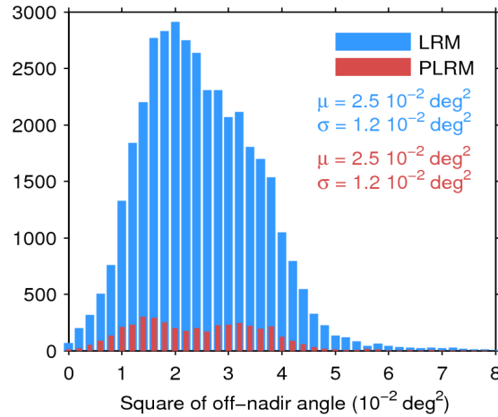
Figure 39. Histogram of flag-valid mispointing over oceans and lakes for LRM (blue) and PLRM (red) for 20/12/2016. Only positive values have been considered. The mean ( \mu ) and standard deviation ( \sigma ) are also shown. Note that values larger than 8 \cdot 10^{-2} \text{ deg}^2 are excluded from the histogram for the sake of readability but not from the computation of \mu and \sigma .
