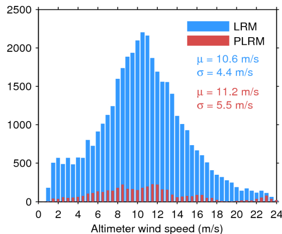
Figure 35. Histogram of science-valid wind over oceans and lakes for LRM (blue) and PLRM (red) for 20/12/2016. The mean ( \mu ) and standard deviation ( \sigma ) are also shown. Note that values larger than 24 m/s are excluded from the histogram for the sake of readability but not from the computation of \mu and \sigma .
