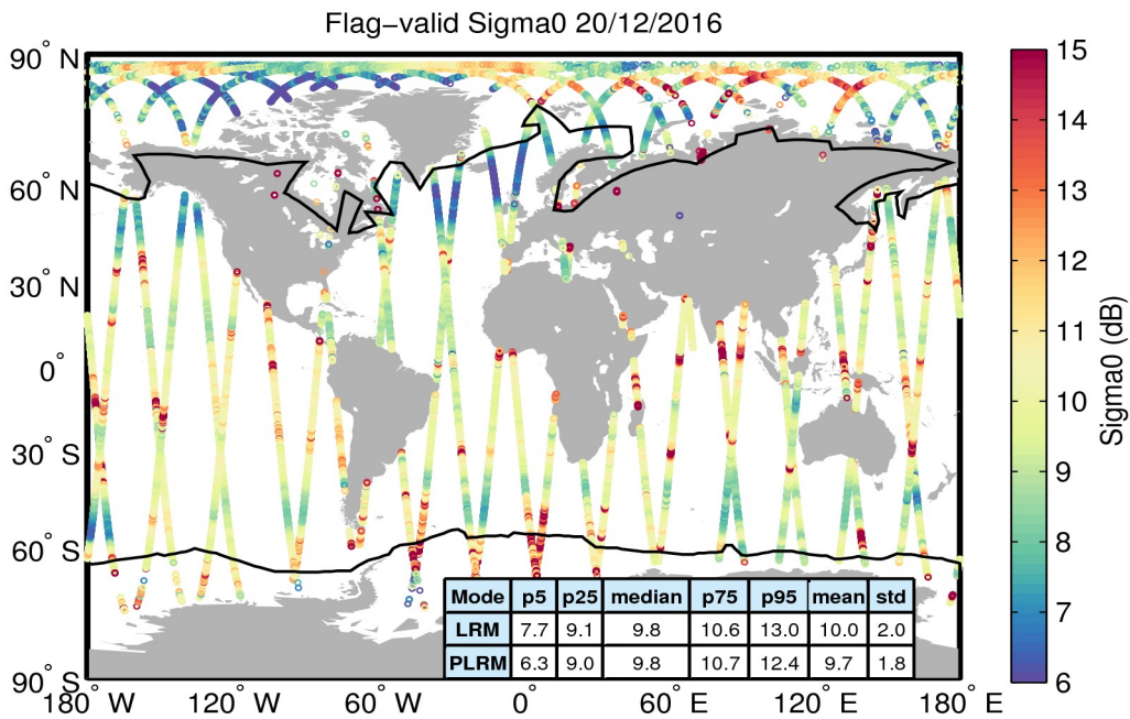
Figure 23. Geographical distribution of flag-valid sigma0 data over oceans and lakes for 20/12/2016. The statistical values shown in the table refer to the sigma0 in dB and are calculated separately for LRM and PLRM regions. Measurements taken over polar polygons have been excluded from the computation of the statistical values. The black lines mark the outer limit of the Arctic and Antarctic polar polygons.
