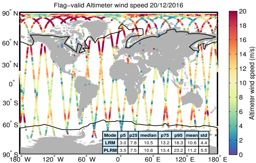
Figure 31. Geographical distribution of flag-valid wind data over oceans and lakes for 20/12/2016. The statistical values shown in the table refer to the wind in m/s and are calculated separately for LRM and PLRM regions. Measurements taken over polar polygons have been excluded from the computation of the statistical values. The black lines mark the outer limit of the Arctic and Antarctic polar polygons.
