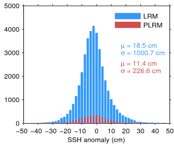
Figure 7. Histogram of flag-valid SSH anomaly over oceans and lakes for LRM (blue) and PLRM (red) for 20/12/2016. The mean ( \mu ) and standard deviation ( \sigma ) are also shown. Note that values outside [-50\ 50] cm are excluded from the histogram for the sake of readability but not from the computation of \mu and \sigma .
