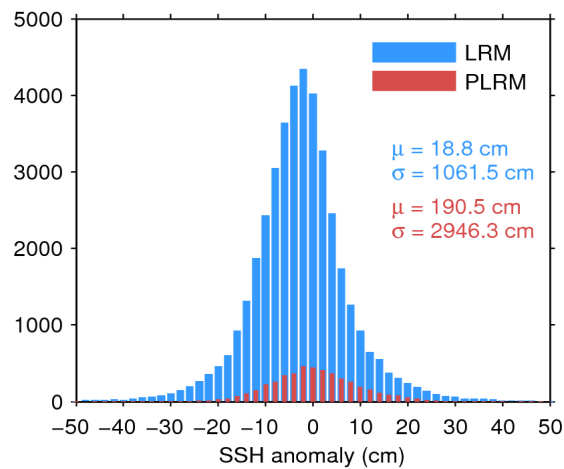
Figure 7. Histogram of flag-valid SSH anomaly over oceans and lakes for LRM (blue) and PLRM (red) for 19/12/2016. The mean ( \mu ) and standard deviation ( \sigma ) are also shown. Note that values outside [-50\ 50] cm are excluded from the histogram for the sake of readability but not from the computation of \mu and \sigma .
