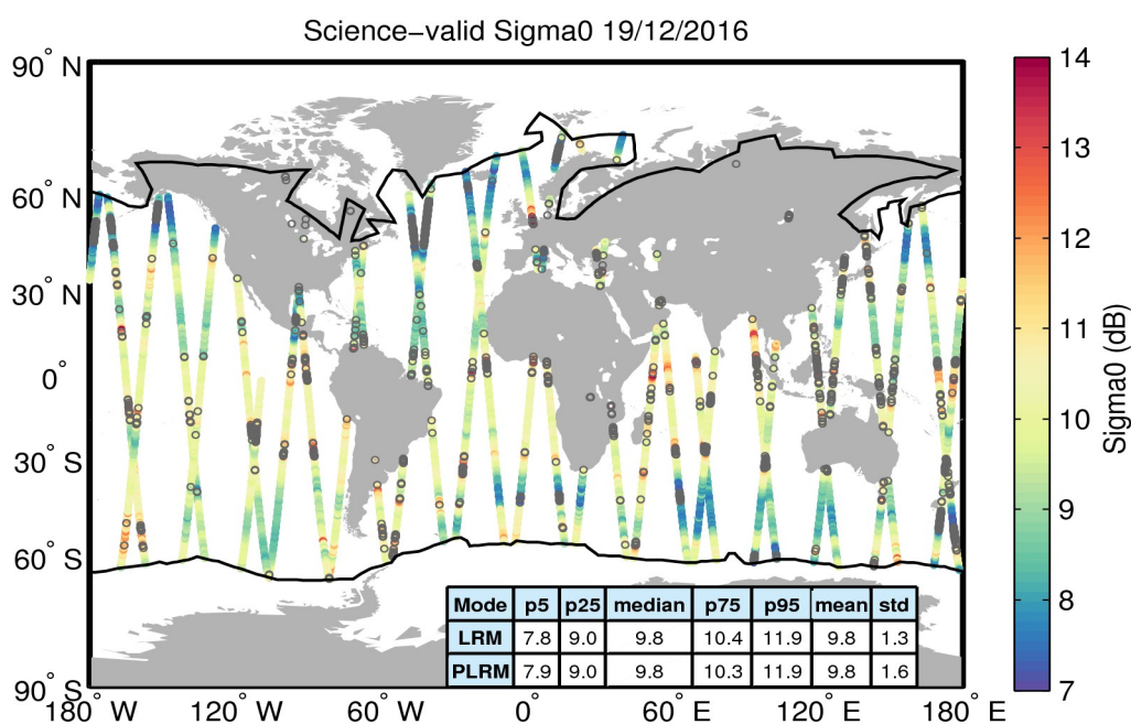
Figure 27. Geographical distribution of science-valid sigma0 data over oceans and lakes for 19/12/2016. The statistical values shown in the table refer to the sigma0 in dB and are calculated separately for LRM and PLRM regions. The black lines mark the outer limit of the Arctic and Antarctic polar polygons. Gray circles denote records that have been rejected based on the editing criteria described in Table 4.
