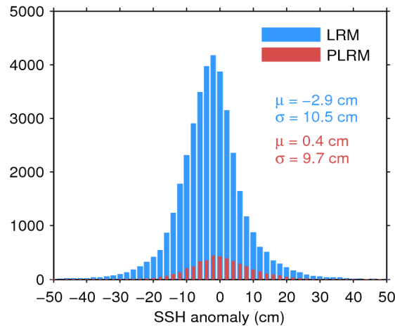
Figure 11. Histogram of science-valid SSH anomaly over oceans and lakes for LRM (blue) and PLRM (red) for 19/12/2016. The mean ( \mu ) and standard deviation ( \sigma ) are also shown. Note that values outside [-50\ 50] cm are excluded from the histogram for the sake of readability but not from the computation of \mu and \sigma .
