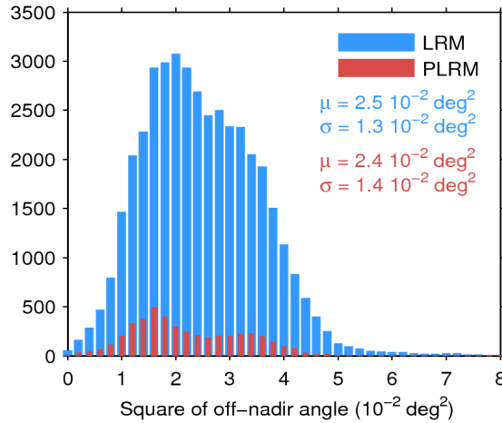
Figure 39. Histogram of flag-valid mispointing over oceans and lakes for LRM (blue) and PLRM (red) for 19/12/2016. Only positive values have been considered. The mean ( \mu ) and standard deviation ( \sigma ) are also shown. Note that values larger than 8 \cdot 10^{-2} \text{ deg}^2 are excluded from the histogram for the sake of readability but not from the computation of \mu and \sigma .
