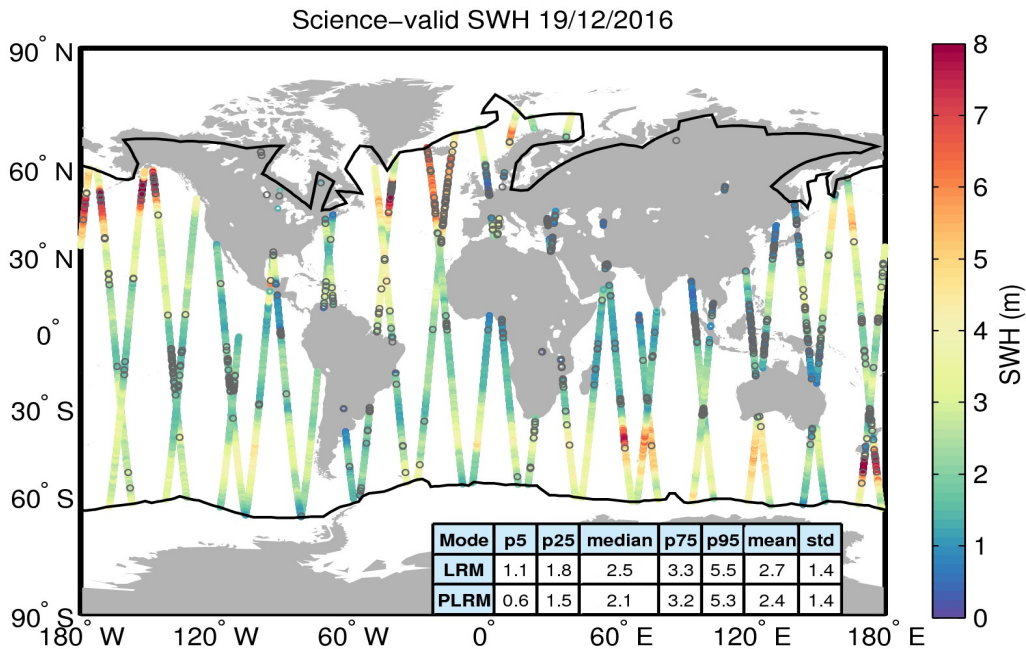
Figure 19. Geographical distribution of science-valid SWH data over oceans and lakes for 19/12/2016. The statistical values shown in the table refer to the SWH in m and are calculated separately for LRM and PLRM regions. The black lines mark the outer limit of the Arctic and Antarctic polar polygons. Gray circles denote records that have been rejected based on the editing criteria described in Table 3.
