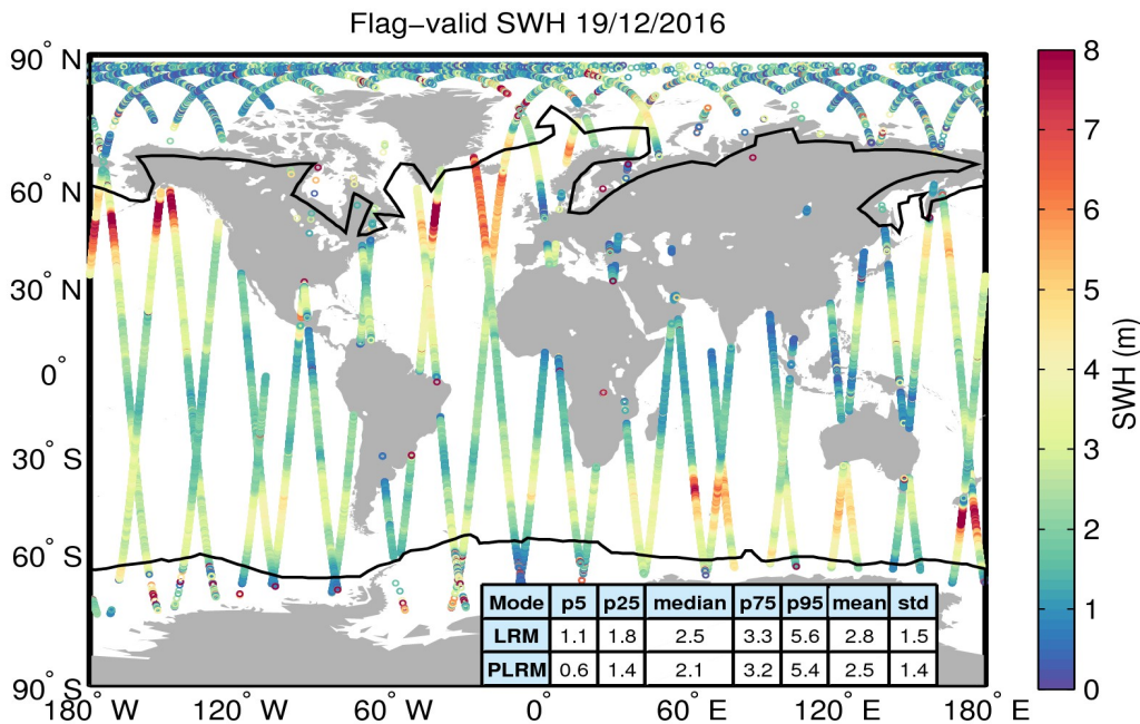
Figure 15. Geographical distribution of flag-valid SWH data over oceans and lakes for 19/12/2016. The statistical values shown in the table refer to the SWH in m and are calculated separately for LRM and PLRM regions. Measurements taken over polar polygons have been excluded from the computation of the statistical values. The black lines mark the outer limit of the Arctic and Antarctic polar polygons.
