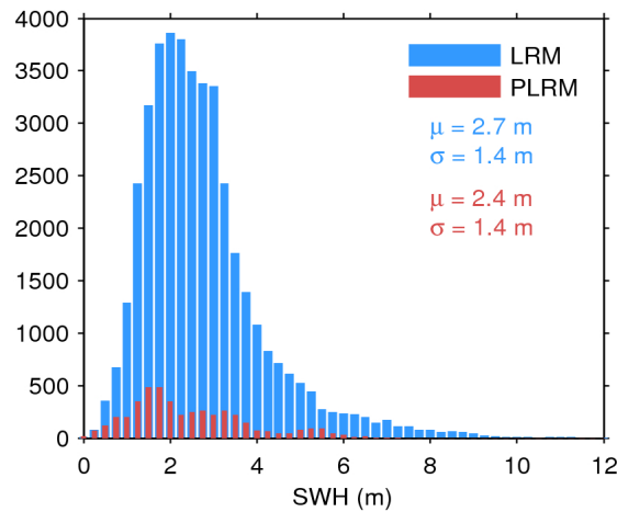
Figure 20. Histogram of science-valid SWH over oceans and lakes for LRM (blue) and PLRM (red) for 19/12/2016. The mean ( \mu ) and standard deviation ( \sigma ) are also shown. Note that values larger than 12 m are excluded from the histogram for the sake of readability but not from the computation of \mu and \sigma .
