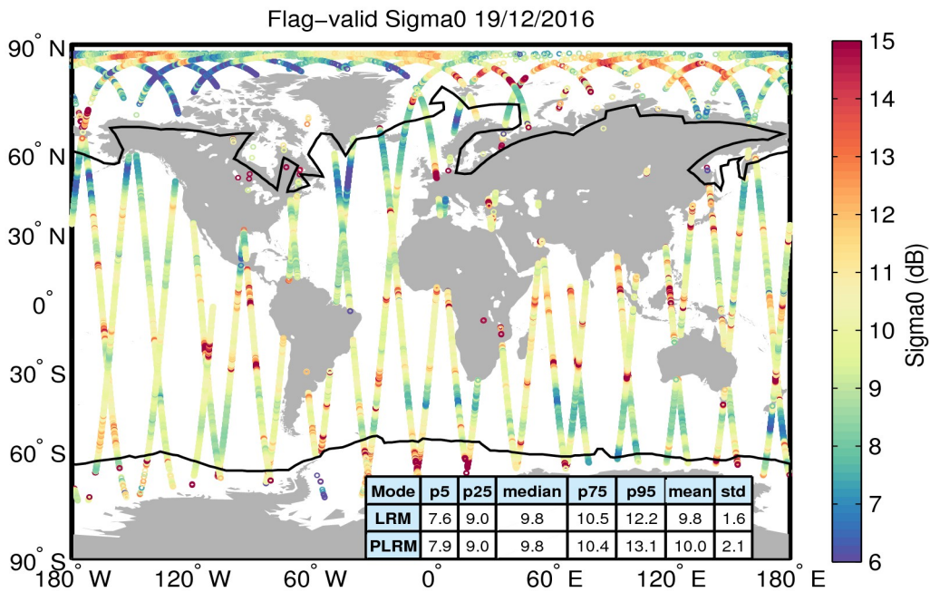
Figure 23. Geographical distribution of flag-valid sigma0 data over oceans and lakes for 19/12/2016. The statistical values shown in the table refer to the sigma0 in dB and are calculated separately for LRM and PLRM regions. Measurements taken over polar polygons have been excluded from the computation of the statistical values. The black lines mark the outer limit of the Arctic and Antarctic polar polygons.
