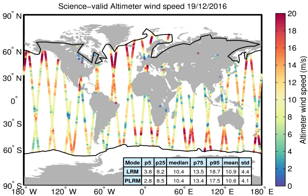
Figure 34. Geographical distribution of science-valid wind data over oceans and lakes for 19/12/2016. The statistical values shown in the table refer to the wind in m/s and are calculated separately for LRM and PLRM regions. The black lines mark the outer limit of the Arctic and Antarctic polar polygons. Gray circles denote records that have been rejected based on the editing criteria described in Table 5.
