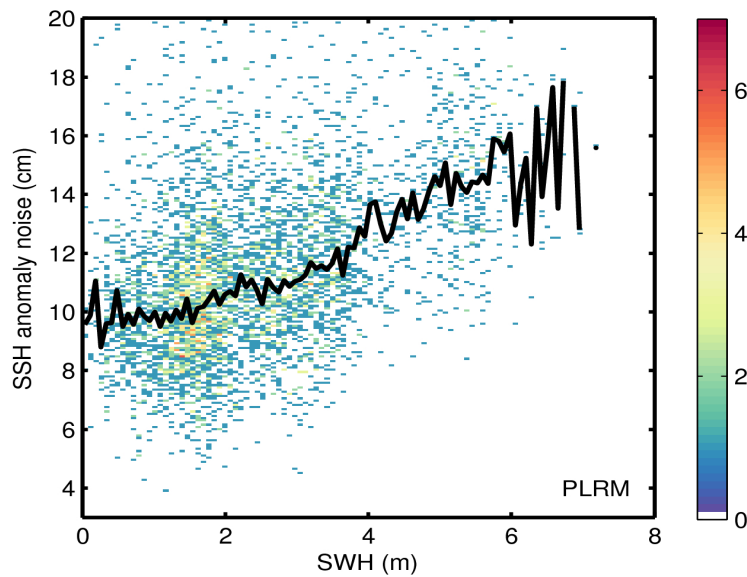
Figure 9. 2D histogram showing flag-valid SSH anomaly noise as a function of SWH for LRM (top) and PLRM (bottom) for 19/12/2016. The black line denotes the median SSH anomaly noise as a function of SWH.
