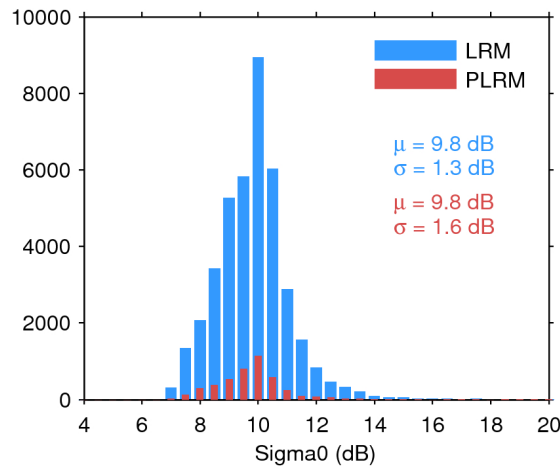
Figure 28. Histogram of science-valid sigma0 over oceans and lakes for LRM (blue) and PLRM (red) for 19/12/2016. The mean ( \mu ) and standard deviation ( \sigma ) are also shown. Note that values outside [4 20] dB are excluded from the histogram for the sake of readability but not from the computation of \mu and \sigma .
