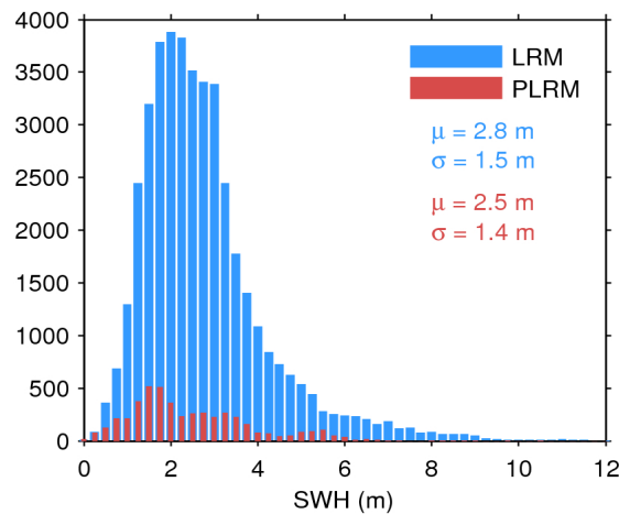
Figure 17. Histogram of flag-valid SWH over oceans and lakes for LRM (blue) and PLRM (red) for 19/12/2016. The mean ( \mu ) and standard deviation ( \sigma ) are also shown. Note that values larger than 12 m are excluded from the histogram for the sake of readability but not from the computation of \mu and \sigma .
