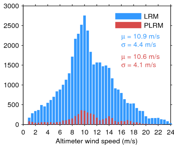
Figure 35. Histogram of science-valid wind over oceans and lakes for LRM (blue) and PLRM (red) for 19/12/2016. The mean ( \mu ) and standard deviation ( \sigma ) are also shown. Note that values larger than 24 m/s are excluded from the histogram for the sake of readability but not from the computation of \mu and \sigma .
