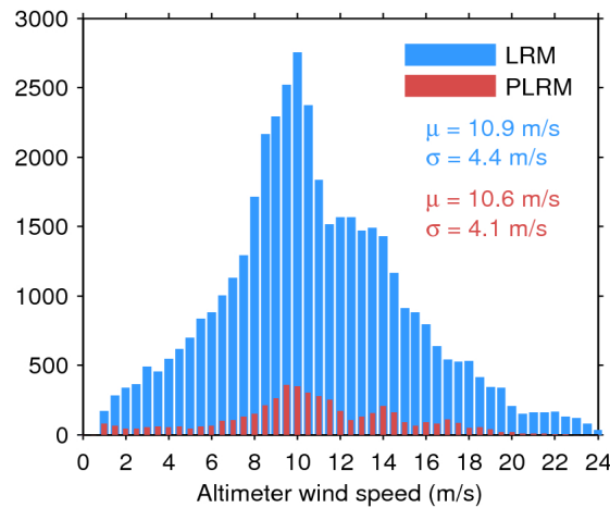
Figure 33. Histogram of flag-valid wind over oceans and lakes for LRM (blue) and PLRM (red) for 19/12/2016. The mean ( \mu ) and standard deviation ( \sigma ) are also shown. Note that values larger than 24 m/s are excluded from the histogram for the sake of readability but not from the computation of \mu and \sigma .
