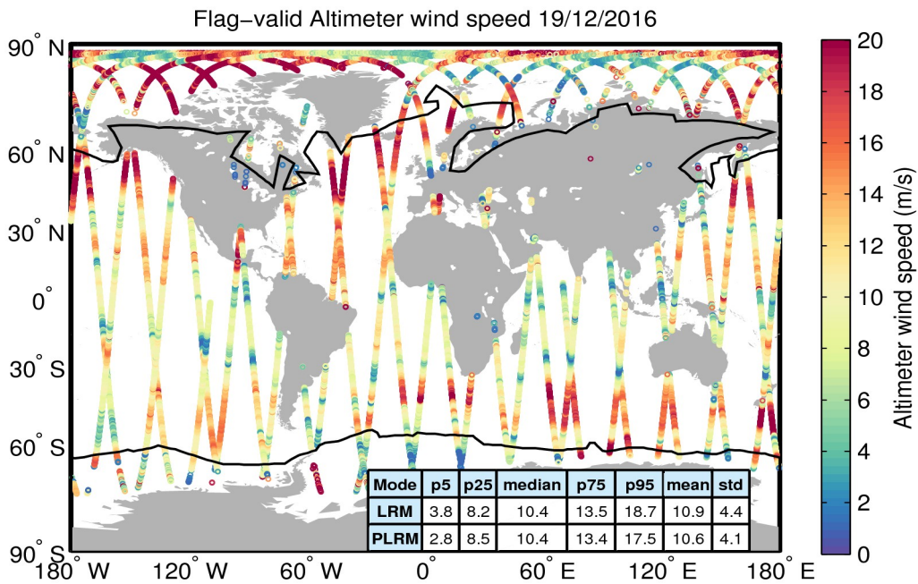
Figure 31. Geographical distribution of flag-valid wind data over oceans and lakes for 19/12/2016. The statistical values shown in the table refer to the wind in m/s and are calculated separately for LRM and PLRM regions. Measurements taken over polar polygons have been excluded from the computation of the statistical values. The black lines mark the outer limit of the Arctic and Antarctic polar polygons.
