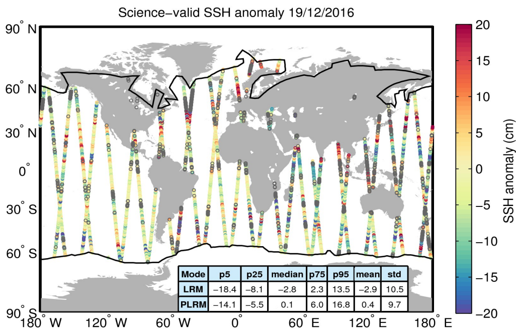
Figure 10. Geographical distribution of science-valid SSH anomaly data over oceans and lakes for 19/12/2016. The statistical values shown in the table refer to the SSH anomaly in cm and are calculated separately for LRM and PLRM regions. The black lines mark the outer limit of the Arctic and Antarctic polar polygons. Gray circles denote records that have been rejected based on the editing criteria described in Table 2.
