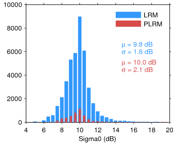
Figure 25. Histogram of flag-valid sigma0 over oceans and lakes for LRM (blue) and PLRM (red) for 19/12/2016. The mean ( \mu ) and standard deviation ( \sigma ) are also shown. Note that values outside [4 20] dB are excluded from the histogram for the sake of readability but not from the computation of \mu and \sigma .
