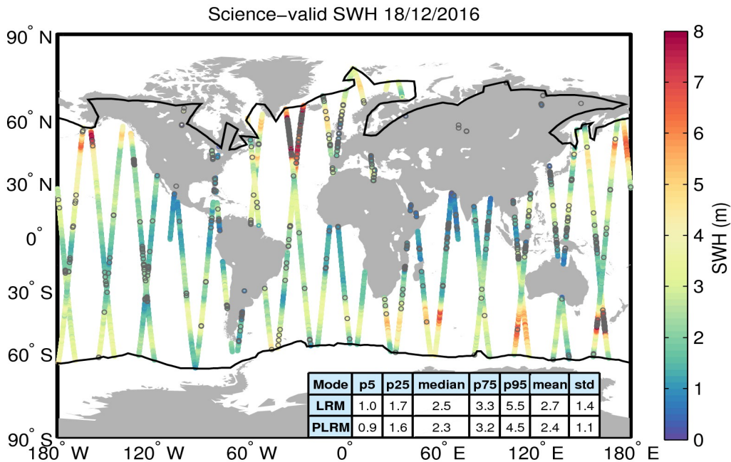
Figure 19. Geographical distribution of science-valid SWH data over oceans and lakes for 18/12/2016. The statistical values shown in the table refer to the SWH in m and are calculated separately for LRM and PLRM regions. The black lines mark the outer limit of the Arctic and Antarctic polar polygons. Gray circles denote records that have been rejected based on the editing criteria described in Table 3.
