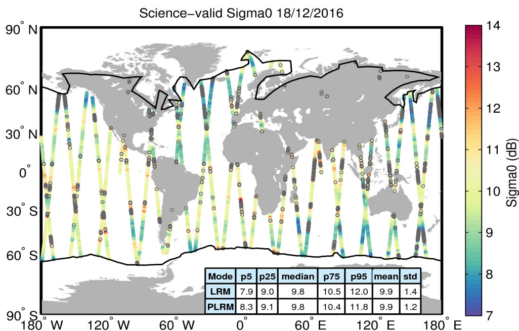
Figure 27. Geographical distribution of science-valid sigma0 data over oceans and lakes for 18/12/2016. The statistical values shown in the table refer to the sigma0 in dB and are calculated separately for LRM and PLRM regions. The black lines mark the outer limit of the Arctic and Antarctic polar polygons. Gray circles denote records that have been rejected based on the editing criteria described in Table 4.
