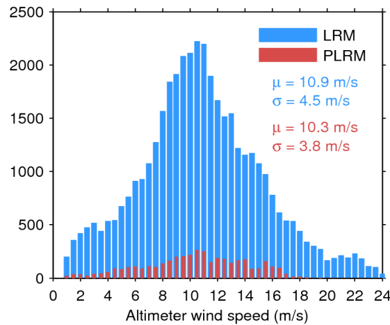
Figure 33. Histogram of flag-valid wind over oceans and lakes for LRM (blue) and PLRM (red) for 18/12/2016. The mean ( \mu ) and standard deviation ( \sigma ) are also shown. Note that values larger than 24 m/s are excluded from the histogram for the sake of readability but not from the computation of \mu and \sigma .
