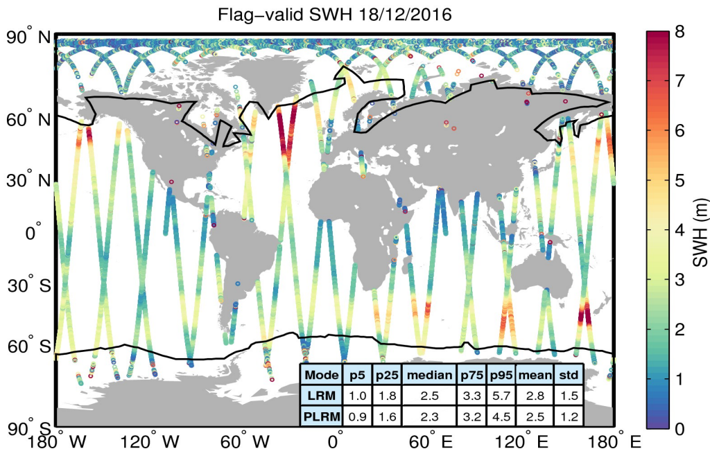
Figure 15. Geographical distribution of flag-valid SWH data over oceans and lakes for 18/12/2016. The statistical values shown in the table refer to the SWH in m and are calculated separately for LRM and PLRM regions. Measurements taken over polar polygons have been excluded from the computation of the statistical values. The black lines mark the outer limit of the Arctic and Antarctic polar polygons.
