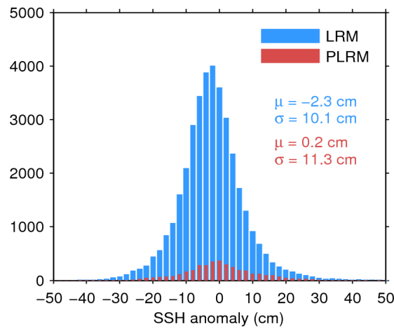
Figure 11. Histogram of science-valid SSH anomaly over oceans and lakes for LRM (blue) and PLRM (red) for 18/12/2016. The mean ( \mu ) and standard deviation ( \sigma ) are also shown. Note that values outside [-50 50] cm are excluded from the histogram for the sake of readability but not from the computation of \mu and \sigma .
