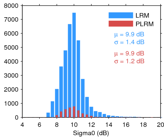
Figure 28. Histogram of science-valid sigma0 over oceans and lakes for LRM (blue) and PLRM (red) for 18/12/2016. The mean ( \mu ) and standard deviation ( \sigma ) are also shown. Note that values outside [4 20] dB are excluded from the histogram for the sake of readability but not from the computation of \mu and \sigma .
