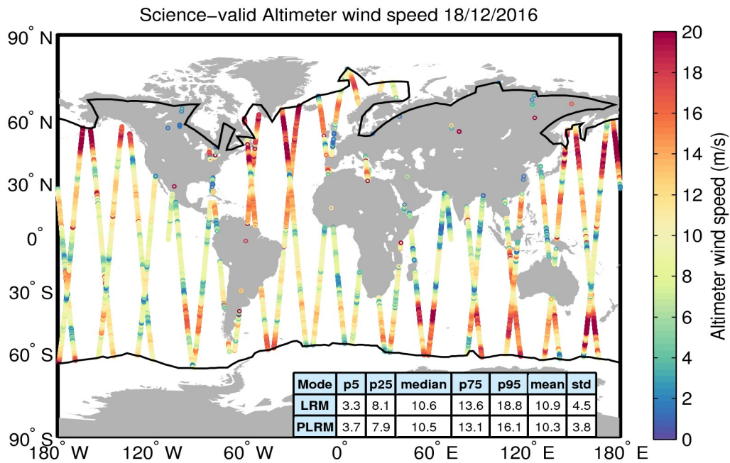
Figure 34. Geographical distribution of science-valid wind data over oceans and lakes for 18/12/2016. The statistical values shown in the table refer to the wind in m/s and are calculated separately for LRM and PLRM regions. The black lines mark the outer limit of the Arctic and Antarctic polar polygons. Gray circles denote records that have been rejected based on the editing criteria described in Table 5.
