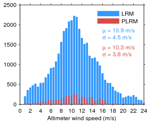
Figure 35. Histogram of science-valid wind over oceans and lakes for LRM (blue) and PLRM (red) for 18/12/2016. The mean ( \mu ) and standard deviation ( \sigma ) are also shown. Note that values larger than 24 m/s are excluded from the histogram for the sake of readability but not from the computation of \mu and \sigma .
