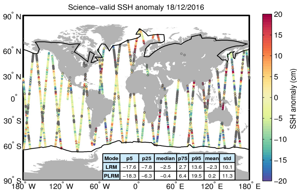
Figure 10. Geographical distribution of science-valid SSH anomaly data over oceans and lakes for 18/12/2016. The statistical values shown in the table refer to the SSH anomaly in cm and are calculated separately for LRM and PLRM regions. The black lines mark the outer limit of the Arctic and Antarctic polar polygons. Gray circles denote records that have been rejected based on the editing criteria described in Table 2.
