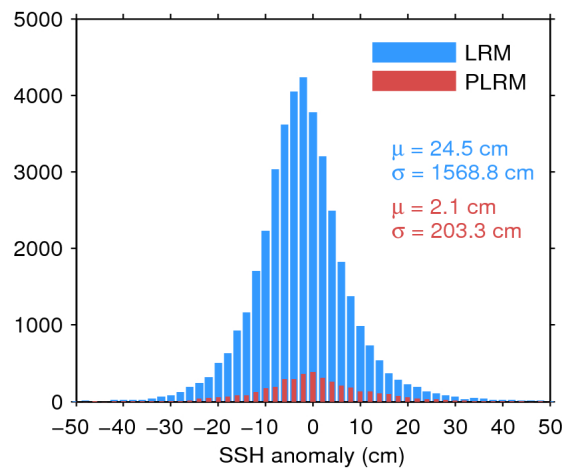
Figure 7. Histogram of flag-valid SSH anomaly over oceans and lakes for LRM (blue) and PLRM (red) for 18/12/2016. The mean ( \mu ) and standard deviation ( \sigma ) are also shown. Note that values outside [-50\ 50] cm are excluded from the histogram for the sake of readability but not from the computation of \mu and \sigma .
