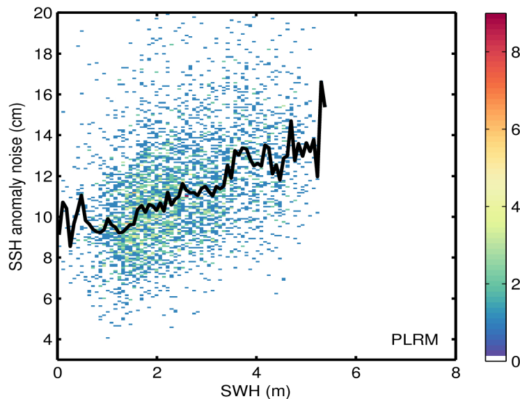
Figure 9. 2D histogram showing flag-valid SSH anomaly noise as a function of SWH for LRM (top) and PLRM (bottom) for 18/12/2016. The black line denotes the median SSH anomaly noise as a function of SWH.
