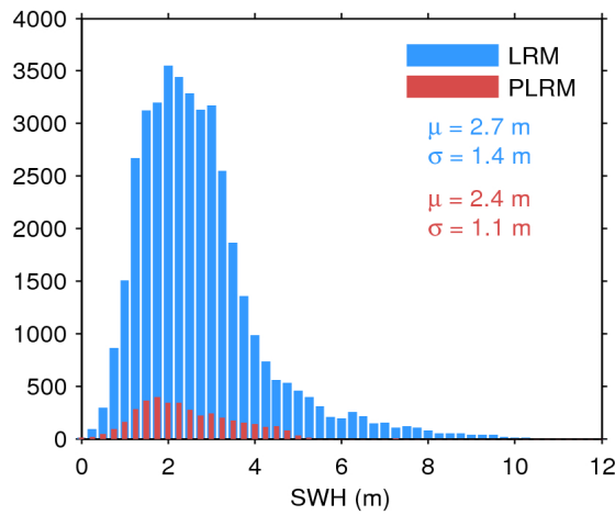
Figure 20. Histogram of science-valid SWH over oceans and lakes for LRM (blue) and PLRM (red) for 18/12/2016. The mean ( \mu ) and standard deviation ( \sigma ) are also shown. Note that values larger than 12 m are excluded from the histogram for the sake of readability but not from the computation of \mu and \sigma .
