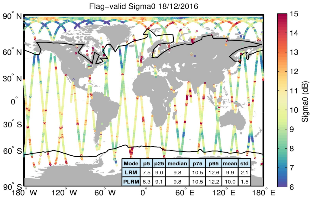
Figure 23. Geographical distribution of flag-valid sigma0 data over oceans and lakes for 18/12/2016. The statistical values shown in the table refer to the sigma0 in dB and are calculated separately for LRM and PLRM regions. Measurements taken over polar polygons have been excluded from the computation of the statistical values. The black lines mark the outer limit of the Arctic and Antarctic polar polygons.
