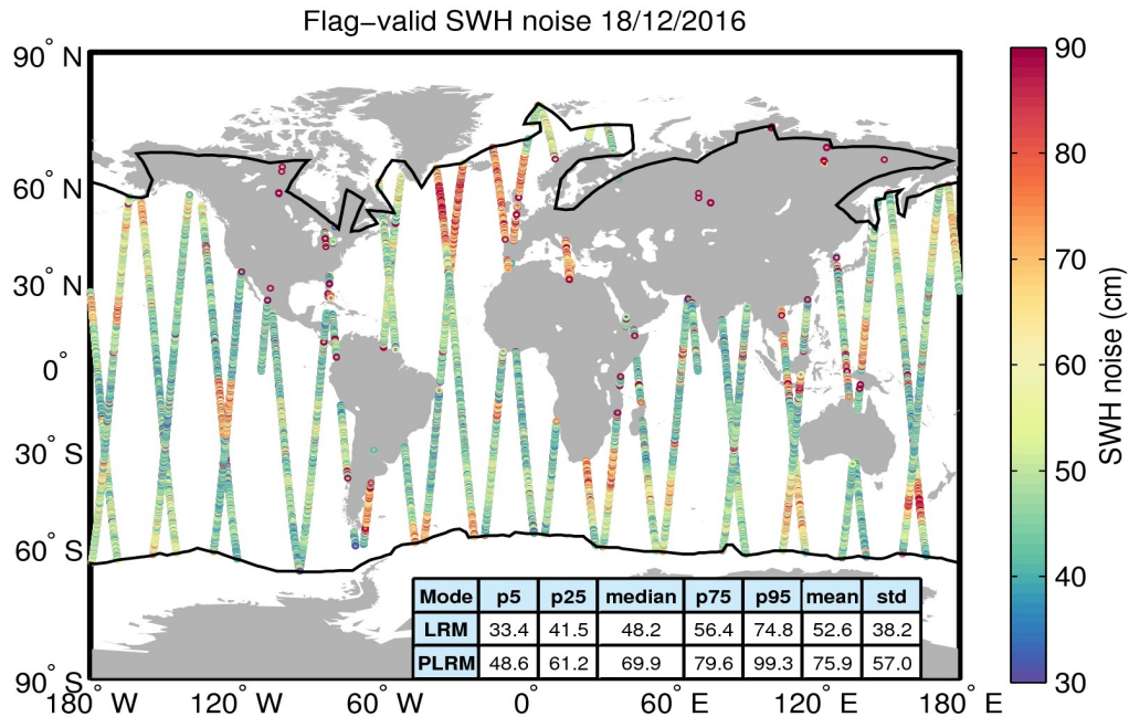
Figure 18. Geographical distribution of flag-valid 20-Hz SWH measurement noise over oceans and lakes for 18/12/2016. The statistical values shown in the table refer to the SWH noise and are calculated separately for LRM and PLRM regions. Measurements taken over polar polygons have been excluded from the computation of the statistical values. The black lines mark the outer limit of the Arctic and Antarctic polar polygons.
