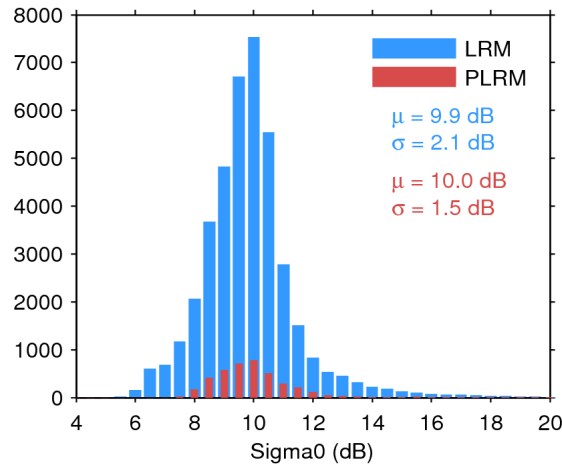
Figure 25. Histogram of flag-valid sigma0 over oceans and lakes for LRM (blue) and PLRM (red) for 18/12/2016. The mean ( \mu ) and standard deviation ( \sigma ) are also shown. Note that values outside [4 20] dB are excluded from the histogram for the sake of readability but not from the computation of \mu and \sigma .
