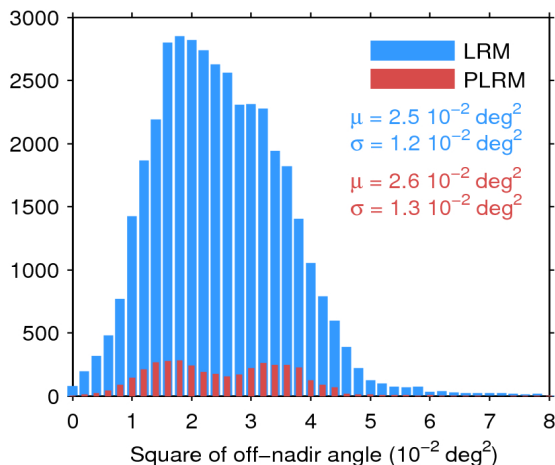
Figure 39. Histogram of flag-valid mispointing over oceans and lakes for LRM (blue) and PLRM (red) for 18/12/2016. Only positive values have been considered. The mean ( \mu ) and standard deviation ( \sigma ) are also shown. Note that values larger than 8 \cdot 10^{-2} \text{ deg}^2 are excluded from the histogram for the sake of readability but not from the computation of \mu and \sigma .
