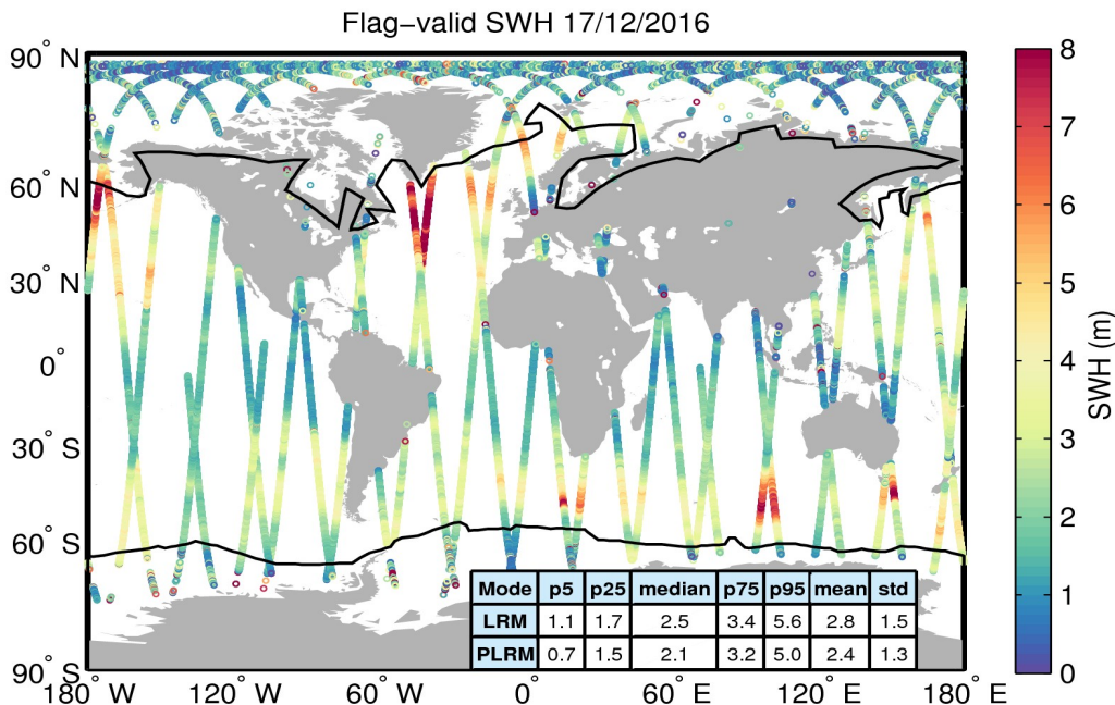
Figure 15. Geographical distribution of flag-valid SWH data over oceans and lakes for 17/12/2016. The statistical values shown in the table refer to the SWH in m and are calculated separately for LRM and PLRM regions. Measurements taken over polar polygons have been excluded from the computation of the statistical values. The black lines mark the outer limit of the Arctic and Antarctic polar polygons.
