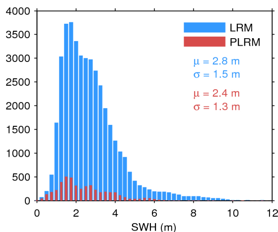
Figure 17. Histogram of flag-valid SWH over oceans and lakes for LRM (blue) and PLRM (red) for 17/12/2016. The mean ( \mu ) and standard deviation ( \sigma ) are also shown. Note that values larger than 12 m are excluded from the histogram for the sake of readability but not from the computation of \mu and \sigma .
