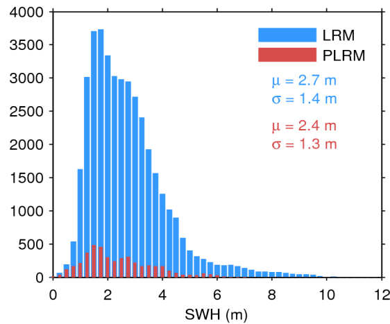
Figure 20. Histogram of science-valid SWH over oceans and lakes for LRM (blue) and PLRM (red) for 17/12/2016. The mean ( \mu ) and standard deviation ( \sigma ) are also shown. Note that values larger than 12 m are excluded from the histogram for the sake of readability but not from the computation of \mu and \sigma .
