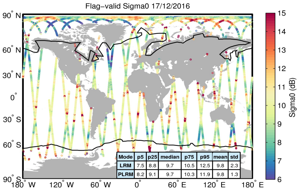
Figure 23. Geographical distribution of flag-valid sigma0 data over oceans and lakes for 17/12/2016. The statistical values shown in the table refer to the sigma0 in dB and are calculated separately for LRM and PLRM regions. Measurements taken over polar polygons have been excluded from the computation of the statistical values. The black lines mark the outer limit of the Arctic and Antarctic polar polygons.
