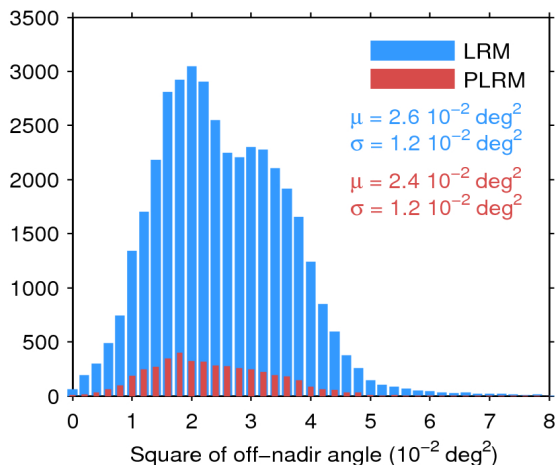
Figure 39. Histogram of flag-valid mispointing over oceans and lakes for LRM (blue) and PLRM (red) for 17/12/2016. Only positive values have been considered. The mean ( \mu ) and standard deviation ( \sigma ) are also shown. Note that values larger than 8 \cdot 10^{-2} \text{ deg}^2 are excluded from the histogram for the sake of readability but not from the computation of \mu and \sigma .
