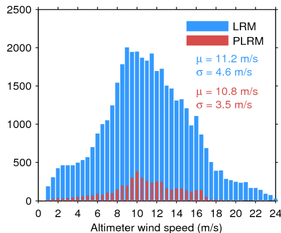
Figure 35. Histogram of science-valid wind over oceans and lakes for LRM (blue) and PLRM (red) for 17/12/2016. The mean ( \mu ) and standard deviation ( \sigma ) are also shown. Note that values larger than 24 m/s are excluded from the histogram for the sake of readability but not from the computation of \mu and \sigma .
