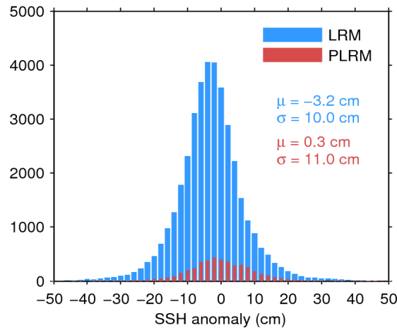
Figure 11. Histogram of science-valid SSH anomaly over oceans and lakes for LRM (blue) and PLRM (red) for 17/12/2016. The mean ( \mu ) and standard deviation ( \sigma ) are also shown. Note that values outside [-50\ 50] cm are excluded from the histogram for the sake of readability but not from the computation of \mu and \sigma .
