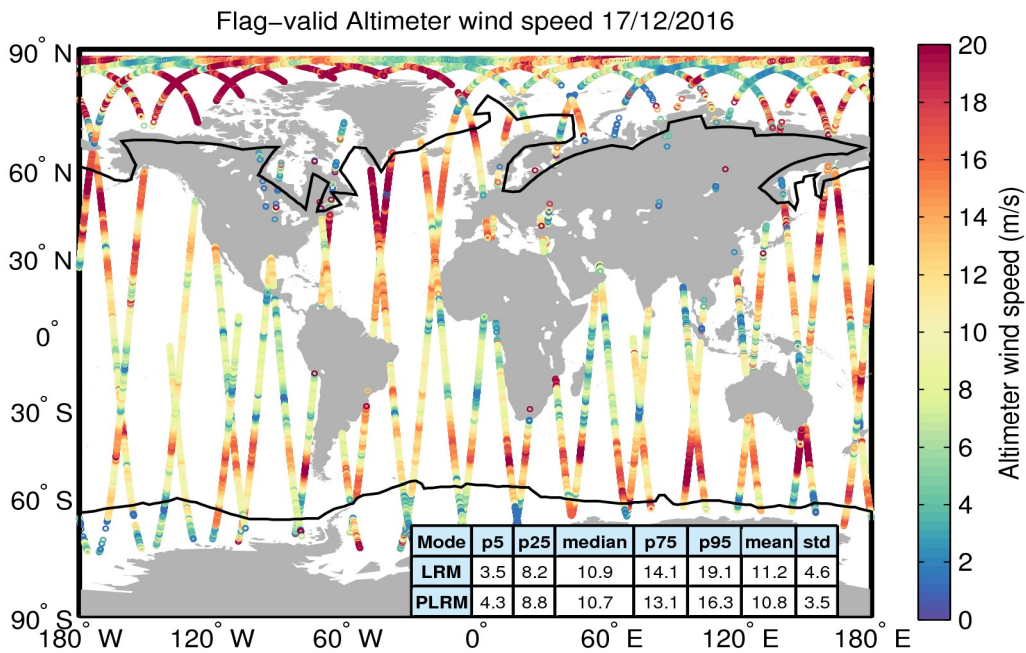
Figure 31. Geographical distribution of flag-valid wind data over oceans and lakes for 17/12/2016. The statistical values shown in the table refer to the wind in m/s and are calculated separately for LRM and PLRM regions. Measurements taken over polar polygons have been excluded from the computation of the statistical values. The black lines mark the outer limit of the Arctic and Antarctic polar polygons.
