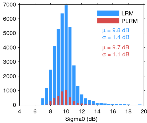
Figure 28. Histogram of science-valid sigma0 over oceans and lakes for LRM (blue) and PLRM (red) for 17/12/2016. The mean ( \mu ) and standard deviation ( \sigma ) are also shown. Note that values outside [4 20] dB are excluded from the histogram for the sake of readability but not from the computation of \mu and \sigma .
