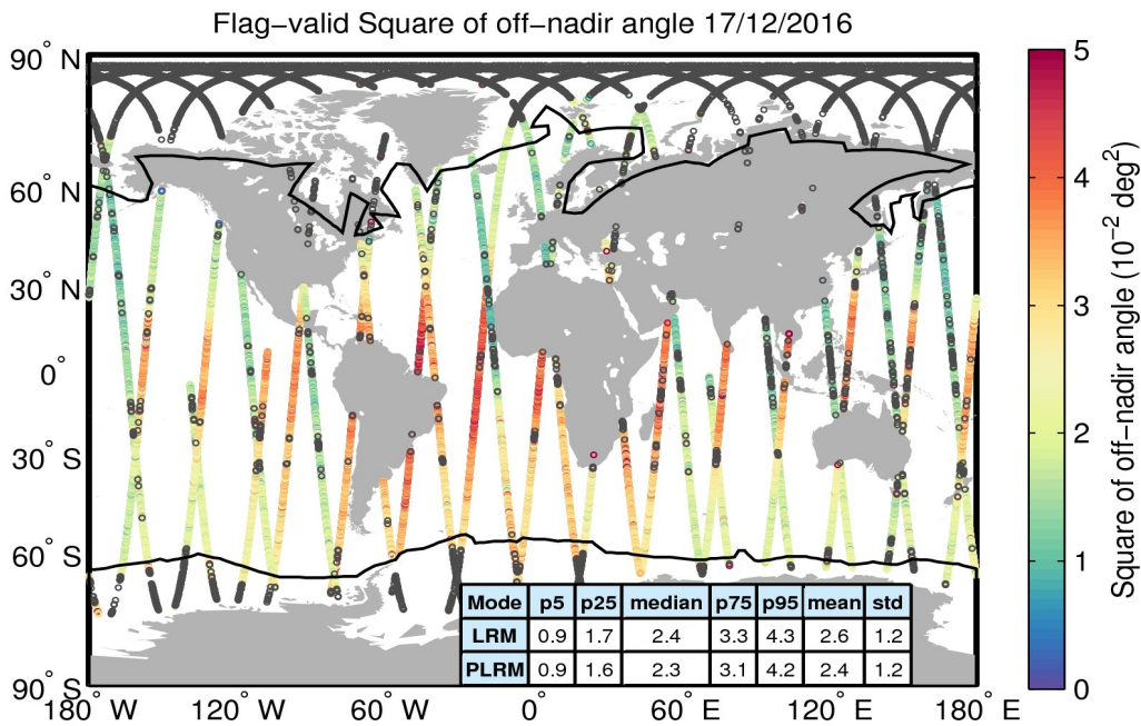
Figure 37. Geographical distribution of flag-valid mispointing data over oceans and lakes for 17/12/2016. The statistical values shown in the table refer to the mispointing in 10^{-2} \text{ deg}^2 and are calculated separately for LRM and PLRM regions. Measurements taken over polar polygons have been excluded from the computation of the statistical values. The black lines mark the outer limit of the Arctic and Antarctic polar polygons. Gray circles denote negative values.
