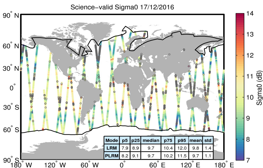
Figure 27. Geographical distribution of science-valid sigma0 data over oceans and lakes for 17/12/2016. The statistical values shown in the table refer to the sigma0 in dB and are calculated separately for LRM and PLRM regions. The black lines mark the outer limit of the Arctic and Antarctic polar polygons. Gray circles denote records that have been rejected based on the editing criteria described in Table 4.
