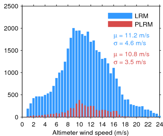
Figure 33. Histogram of flag-valid wind over oceans and lakes for LRM (blue) and PLRM (red) for 17/12/2016. The mean ( \mu ) and standard deviation ( \sigma ) are also shown. Note that values larger than 24 m/s are excluded from the histogram for the sake of readability but not from the computation of \mu and \sigma .
