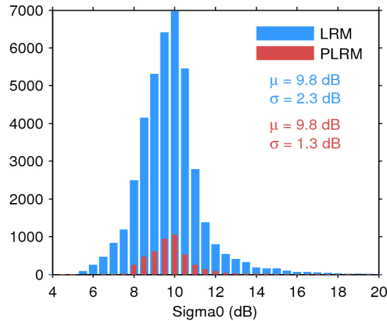
Figure 25. Histogram of flag-valid sigma0 over oceans and lakes for LRM (blue) and PLRM (red) for 17/12/2016. The mean ( \mu ) and standard deviation ( \sigma ) are also shown. Note that values outside [4 20] dB are excluded from the histogram for the sake of readability but not from the computation of \mu and \sigma .
