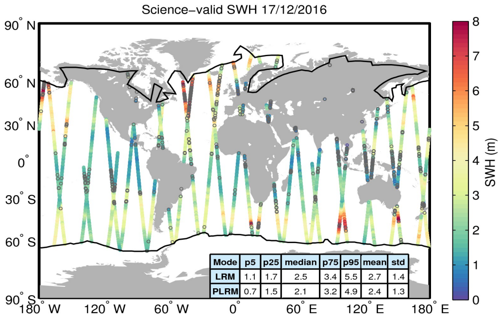
Figure 19. Geographical distribution of science-valid SWH data over oceans and lakes for 17/12/2016. The statistical values shown in the table refer to the SWH in m and are calculated separately for LRM and PLRM regions. The black lines mark the outer limit of the Arctic and Antarctic polar polygons. Gray circles denote records that have been rejected based on the editing criteria described in Table 3.
