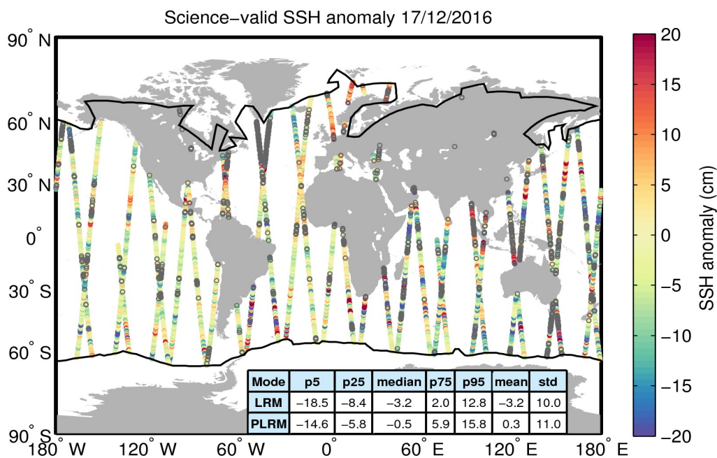
Figure 10. Geographical distribution of science-valid SSH anomaly data over oceans and lakes for 17/12/2016. The statistical values shown in the table refer to the SSH anomaly in cm and are calculated separately for LRM and PLRM regions. The black lines mark the outer limit of the Arctic and Antarctic polar polygons. Gray circles denote records that have been rejected based on the editing criteria described in Table 2.
