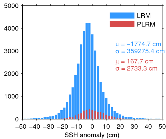
Figure 7. Histogram of flag-valid SSH anomaly over oceans and lakes for LRM (blue) and PLRM (red) for 17/12/2016. The mean ( \mu ) and standard deviation ( \sigma ) are also shown. Note that values outside [-50\ 50] cm are excluded from the histogram for the sake of readability but not from the computation of \mu and \sigma .
