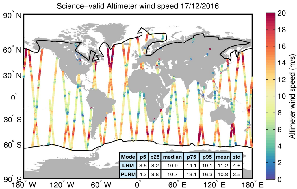
Figure 34. Geographical distribution of science-valid wind data over oceans and lakes for 17/12/2016. The statistical values shown in the table refer to the wind in m/s and are calculated separately for LRM and PLRM regions. The black lines mark the outer limit of the Arctic and Antarctic polar polygons. Gray circles denote records that have been rejected based on the editing criteria described in Table 5.
