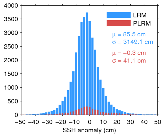
Figure 7. Histogram of flag-valid SSH anomaly over oceans and lakes for LRM (blue) and PLRM (red) for 16/12/2016. The mean ( \mu ) and standard deviation ( \sigma ) are also shown. Note that values outside [-50 \ 50] cm are excluded from the histogram for the sake of readability but not from the computation of \mu and \sigma .
