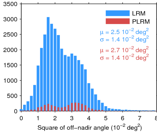
Figure 39. Histogram of flag-valid mispointing over oceans and lakes for LRM (blue) and PLRM (red) for 16/12/2016. Only positive values have been considered. The mean ( \mu ) and standard deviation ( \sigma ) are also shown. Note that values larger than 8 \cdot 10^{-2} \text{ deg}^2 are excluded from the histogram for the sake of readability but not from the computation of \mu and \sigma .
