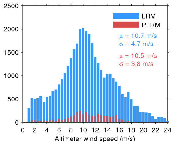
Figure 35. Histogram of science-valid wind over oceans and lakes for LRM (blue) and PLRM (red) for 16/12/2016. The mean ( \mu ) and standard deviation ( \sigma ) are also shown. Note that values larger than 24 m/s are excluded from the histogram for the sake of readability but not from the computation of \mu and \sigma .
