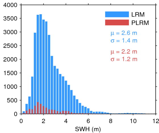
Figure 20. Histogram of science-valid SWH over oceans and lakes for LRM (blue) and PLRM (red) for 16/12/2016. The mean ( \mu ) and standard deviation ( \sigma ) are also shown. Note that values larger than 12 m are excluded from the histogram for the sake of readability but not from the computation of \mu and \sigma .
