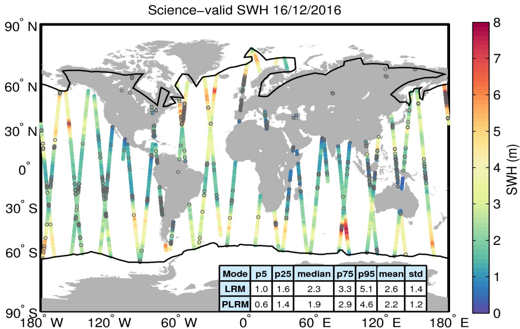
Figure 19. Geographical distribution of science-valid SWH data over oceans and lakes for 16/12/2016. The statistical values shown in the table refer to the SWH in m and are calculated separately for LRM and PLRM regions. The black lines mark the outer limit of the Arctic and Antarctic polar polygons. Gray circles denote records that have been rejected based on the editing criteria described in Table 3.
