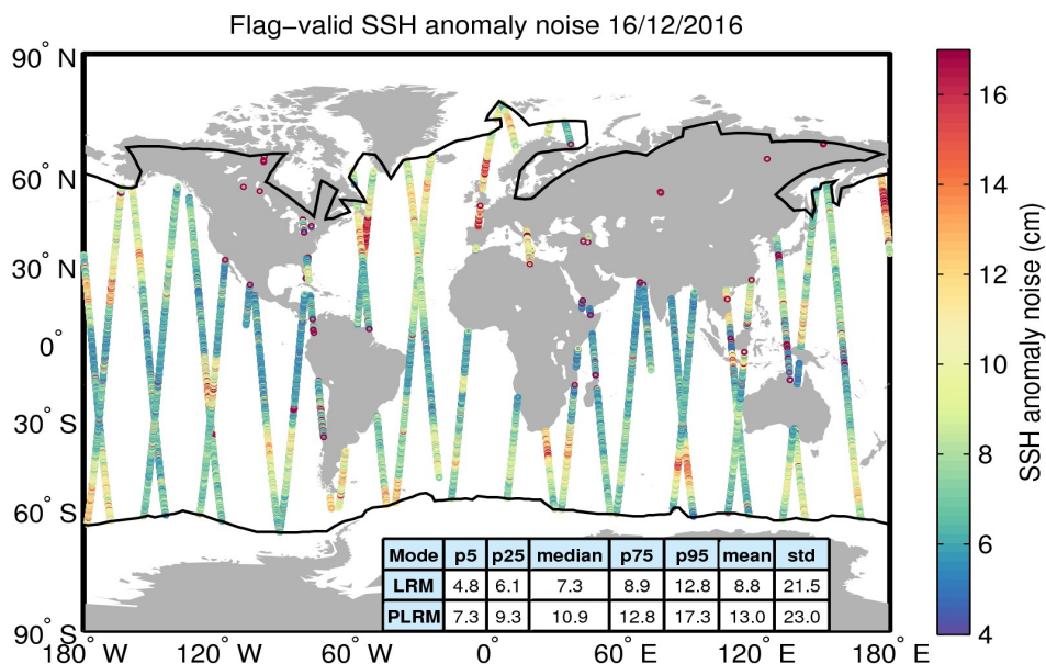
Figure 8. Geographical distribution of flag-valid 20-Hz SSH anomaly measurement noise over oceans and lakes for 16/12/2016. The statistical values shown in the table refer to the SSH anomaly noise and are calculated separately for LRM and PLRM regions. Measurements taken over polar polygons have been excluded from the computation of the statistical values. The black lines mark the outer limit of the Arctic and Antarctic polar polygons.
