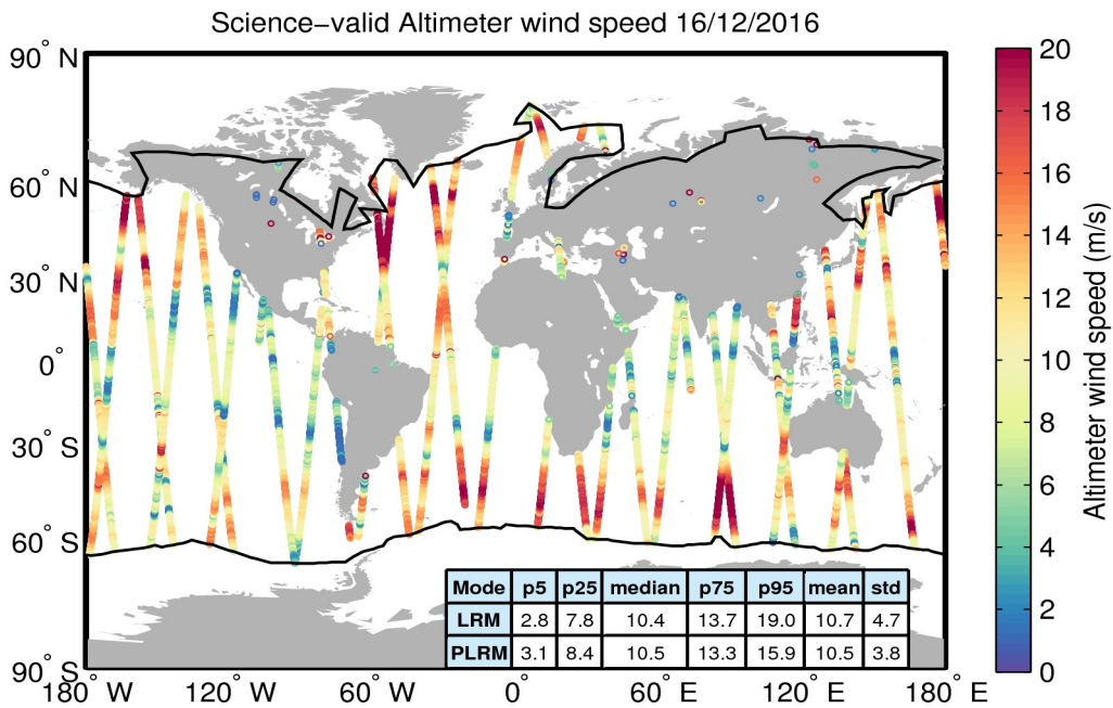
Figure 34. Geographical distribution of science-valid wind data over oceans and lakes for 16/12/2016. The statistical values shown in the table refer to the wind in m/s and are calculated separately for LRM and PLRM regions. The black lines mark the outer limit of the Arctic and Antarctic polar polygons. Gray circles denote records that have been rejected based on the editing criteria described in Table 5.
