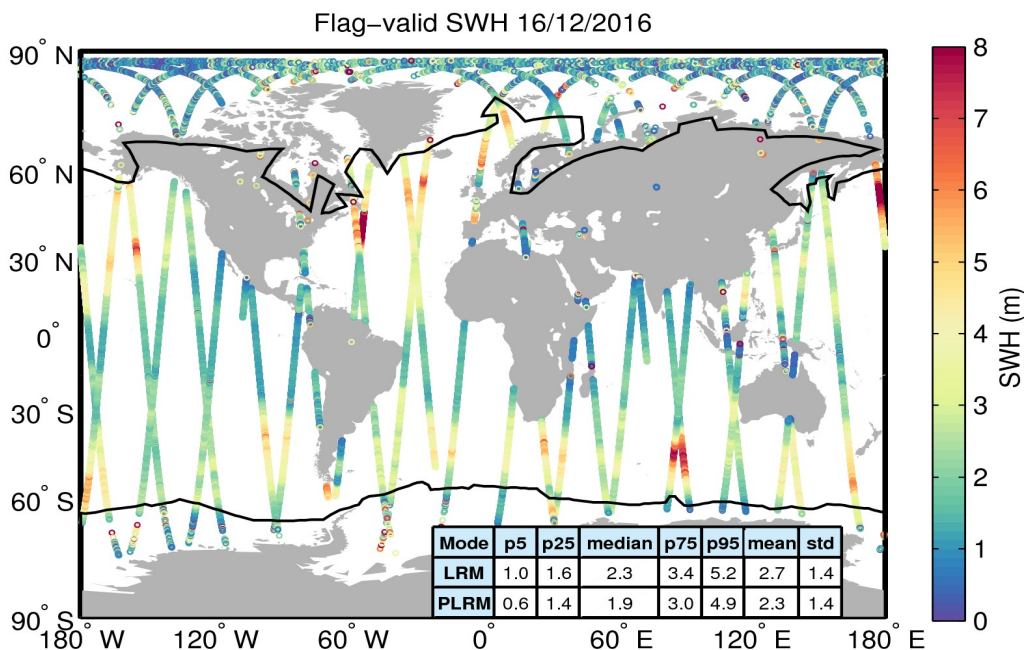
Figure 15. Geographical distribution of flag-valid SWH data over oceans and lakes for 16/12/2016. The statistical values shown in the table refer to the SWH in m and are calculated separately for LRM and PLRM regions. Measurements taken over polar polygons have been excluded from the computation of the statistical values. The black lines mark the outer limit of the Arctic and Antarctic polar polygons.
