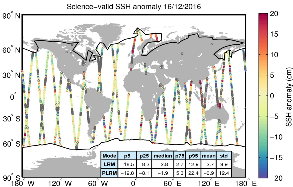
Figure 10. Geographical distribution of science-valid SSH anomaly data over oceans and lakes for 16/12/2016. The statistical values shown in the table refer to the SSH anomaly in cm and are calculated separately for LRM and PLRM regions. The black lines mark the outer limit of the Arctic and Antarctic polar polygons. Gray circles denote records that have been rejected based on the editing criteria described in Table 2.
