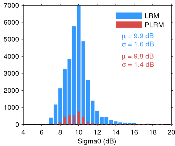
Figure 28. Histogram of science-valid sigma0 over oceans and lakes for LRM (blue) and PLRM (red) for 16/12/2016. The mean ( \mu ) and standard deviation ( \sigma ) are also shown. Note that values outside [4 20] dB are excluded from the histogram for the sake of readability but not from the computation of \mu and \sigma .
