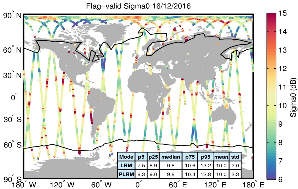
Figure 23. Geographical distribution of flag-valid sigma0 data over oceans and lakes for 16/12/2016. The statistical values shown in the table refer to the sigma0 in dB and are calculated separately for LRM and PLRM regions. Measurements taken over polar polygons have been excluded from the computation of the statistical values. The black lines mark the outer limit of the Arctic and Antarctic polar polygons.
