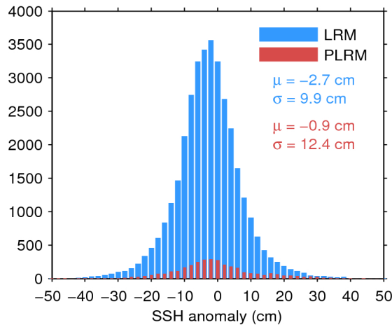
Figure 11. Histogram of science-valid SSH anomaly over oceans and lakes for LRM (blue) and PLRM (red) for 16/12/2016. The mean ( \mu ) and standard deviation ( \sigma ) are also shown. Note that values outside [-50 50] cm are excluded from the histogram for the sake of readability but not from the computation of \mu and \sigma .
