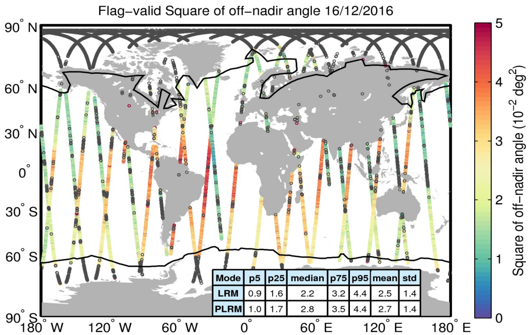
Figure 37. Geographical distribution of flag-valid mispointing data over oceans and lakes for 16/12/2016. The statistical values shown in the table refer to the mispointing in 10^{-2} \text{ deg}^2 and are calculated separately for LRM and PLRM regions. Measurements taken over polar polygons have been excluded from the computation of the statistical values. The black lines mark the outer limit of the Arctic and Antarctic polar polygons. Gray circles denote negative values.
