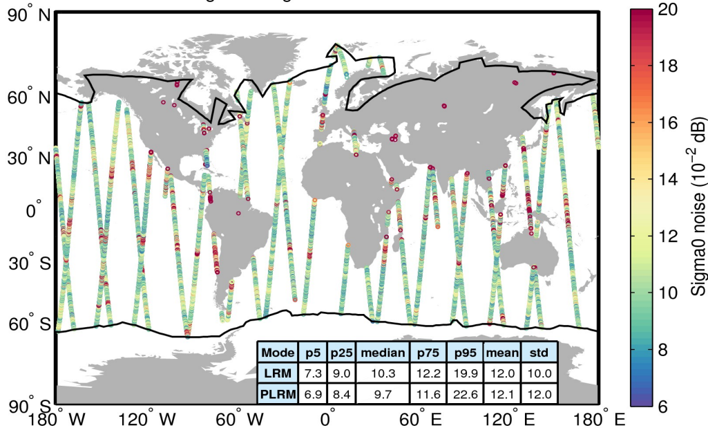
Flag-valid sigma0 noise 16/12/2016
