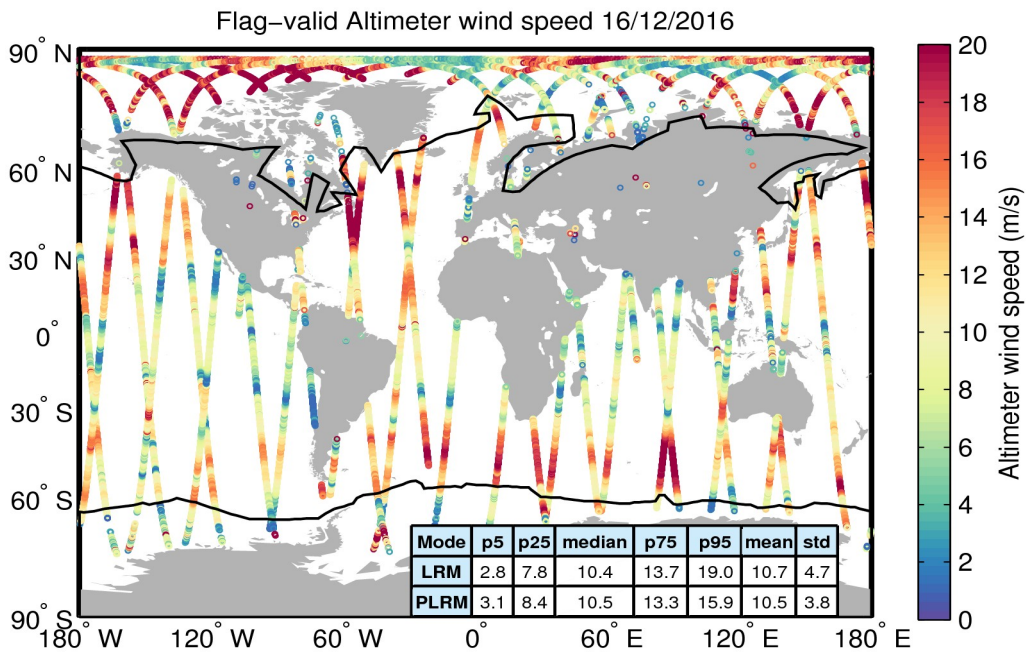
Figure 31. Geographical distribution of flag-valid wind data over oceans and lakes for 16/12/2016. The statistical values shown in the table refer to the wind in m/s and are calculated separately for LRM and PLRM regions. Measurements taken over polar polygons have been excluded from the computation of the statistical values. The black lines mark the outer limit of the Arctic and Antarctic polar polygons.
