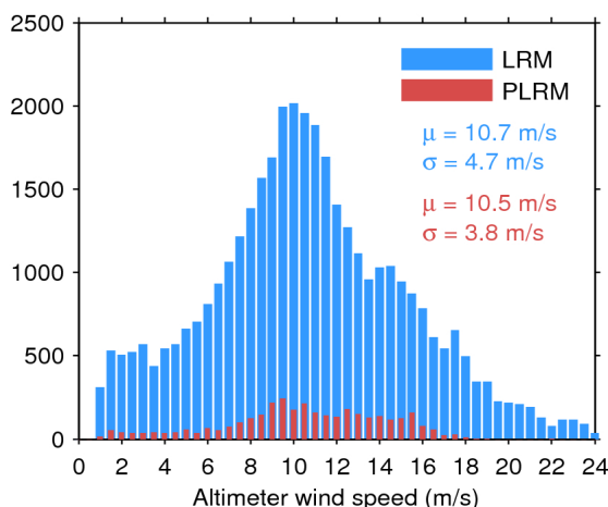
Figure 33. Histogram of flag-valid wind over oceans and lakes for LRM (blue) and PLRM (red) for 16/12/2016. The mean ( \mu ) and standard deviation ( \sigma ) are also shown. Note that values larger than 24 m/s are excluded from the histogram for the sake of readability but not from the computation of \mu and \sigma .
