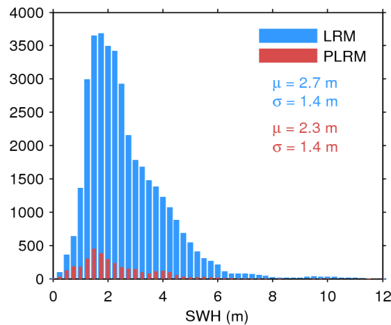
Figure 17. Histogram of flag-valid SWH over oceans and lakes for LRM (blue) and PLRM (red) for 16/12/2016. The mean ( \mu ) and standard deviation ( \sigma ) are also shown. Note that values larger than 12 m are excluded from the histogram for the sake of readability but not from the computation of \mu and \sigma .
