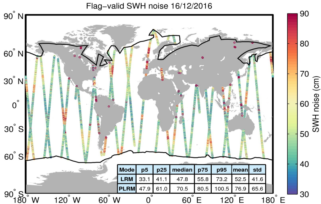
Figure 18. Geographical distribution of flag-valid 20-Hz SWH measurement noise over oceans and lakes for 16/12/2016. The statistical values shown in the table refer to the SWH noise and are calculated separately for LRM and PLRM regions. Measurements taken over polar polygons have been excluded from the computation of the statistical values. The black lines mark the outer limit of the Arctic and Antarctic polar polygons.
