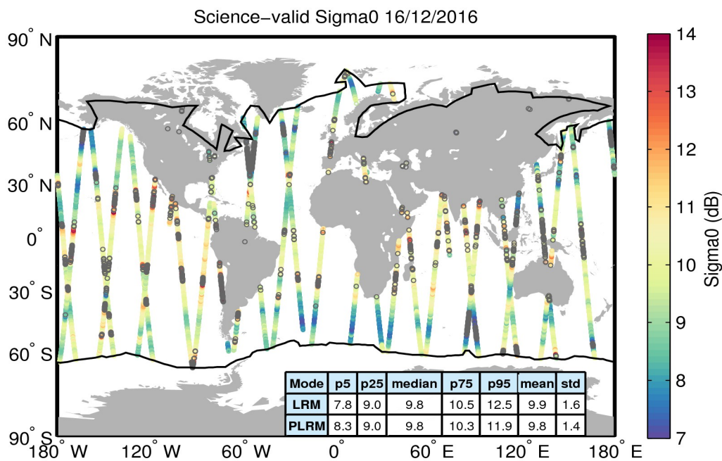
Figure 27. Geographical distribution of science-valid sigma0 data over oceans and lakes for 16/12/2016. The statistical values shown in the table refer to the sigma0 in dB and are calculated separately for LRM and PLRM regions. The black lines mark the outer limit of the Arctic and Antarctic polar polygons. Gray circles denote records that have been rejected based on the editing criteria described in Table 4.
