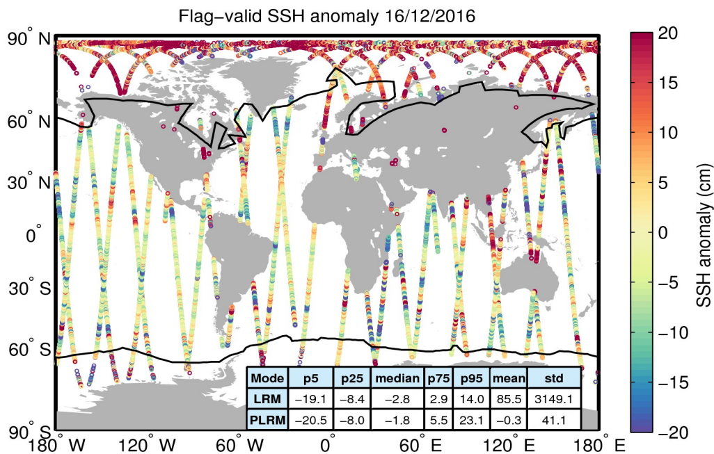
Figure 5. Geographical distribution of flag-valid 1-Hz SSH anomaly data over oceans and lakes for 16/12/2016. The statistical values shown in the table refer to the SSH anomaly in cm and are calculated separately for LRM and PLRM regions. Measurements taken over polar polygons have been excluded from the computation of the statistical values. The black lines mark the outer limit of the Arctic and Antarctic polar polygons.
