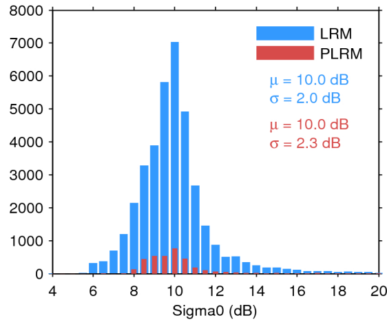
Figure 25. Histogram of flag-valid sigma0 over oceans and lakes for LRM (blue) and PLRM (red) for 16/12/2016. The mean ( \mu ) and standard deviation ( \sigma ) are also shown. Note that values outside [4 20] dB are excluded from the histogram for the sake of readability but not from the computation of \mu and \sigma .
