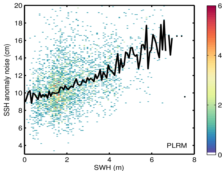
Figure 9. 2D histogram showing flag-valid SSH anomaly noise as a function of SWH for LRM (top) and PLRM (bottom) for 16/12/2016. The black line denotes the median SSH anomaly noise as a function of SWH.
