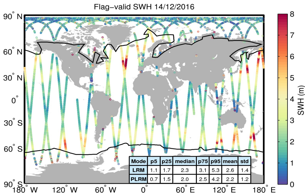
Figure 15. Geographical distribution of flag-valid SWH data over oceans and lakes for 14/12/2016. The statistical values shown in the table refer to the SWH in m and are calculated separately for LRM and PLRM regions. Measurements taken over polar polygons have been excluded from the computation of the statistical values. The black lines mark the outer limit of the Arctic and Antarctic polar polygons.
