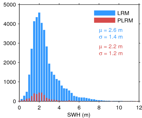
Figure 17. Histogram of flag-valid SWH over oceans and lakes for LRM (blue) and PLRM (red) for 14/12/2016. The mean ( \mu ) and standard deviation ( \sigma ) are also shown. Note that values larger than 12 m are excluded from the histogram for the sake of readability but not from the computation of \mu and \sigma .
