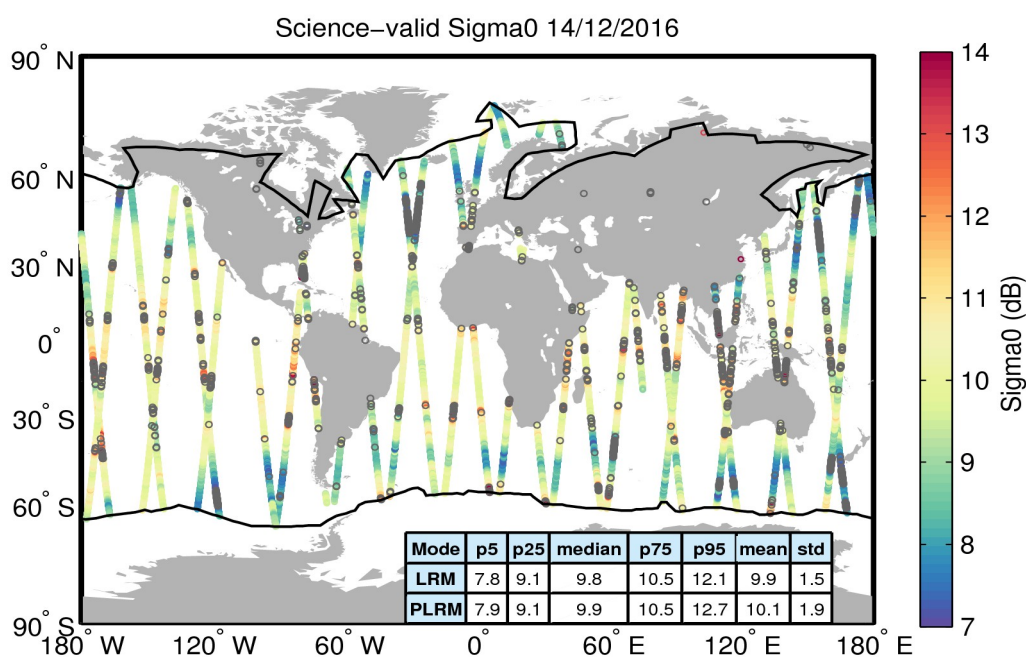
Figure 27. Geographical distribution of science-valid sigma0 data over oceans and lakes for 14/12/2016. The statistical values shown in the table refer to the sigma0 in dB and are calculated separately for LRM and PLRM regions. The black lines mark the outer limit of the Arctic and Antarctic polar polygons. Gray circles denote records that have been rejected based on the editing criteria described in Table 4.
