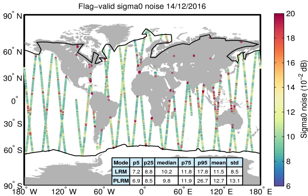
Figure 26. Geographical distribution of flag-valid 20-Hz sigma0 measurement noise over oceans and lakes for 14/12/2016. The statistical values shown in the table refer to the sigma0 noise and are calculated separately for LRM and PLRM regions. Measurements taken over polar polygons have been excluded from the computation of the statistical values. The black lines mark the outer limit of the Arctic and Antarctic polar polygons.
