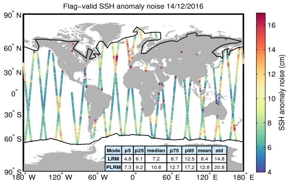
Figure 8. Geographical distribution of flag-valid 20-Hz SSH anomaly measurement noise over oceans and lakes for 14/12/2016. The statistical values shown in the table refer to the SSH anomaly noise and are calculated separately for LRM and PLRM regions. Measurements taken over polar polygons have been excluded from the computation of the statistical values. The black lines mark the outer limit of the Arctic and Antarctic polar polygons.
