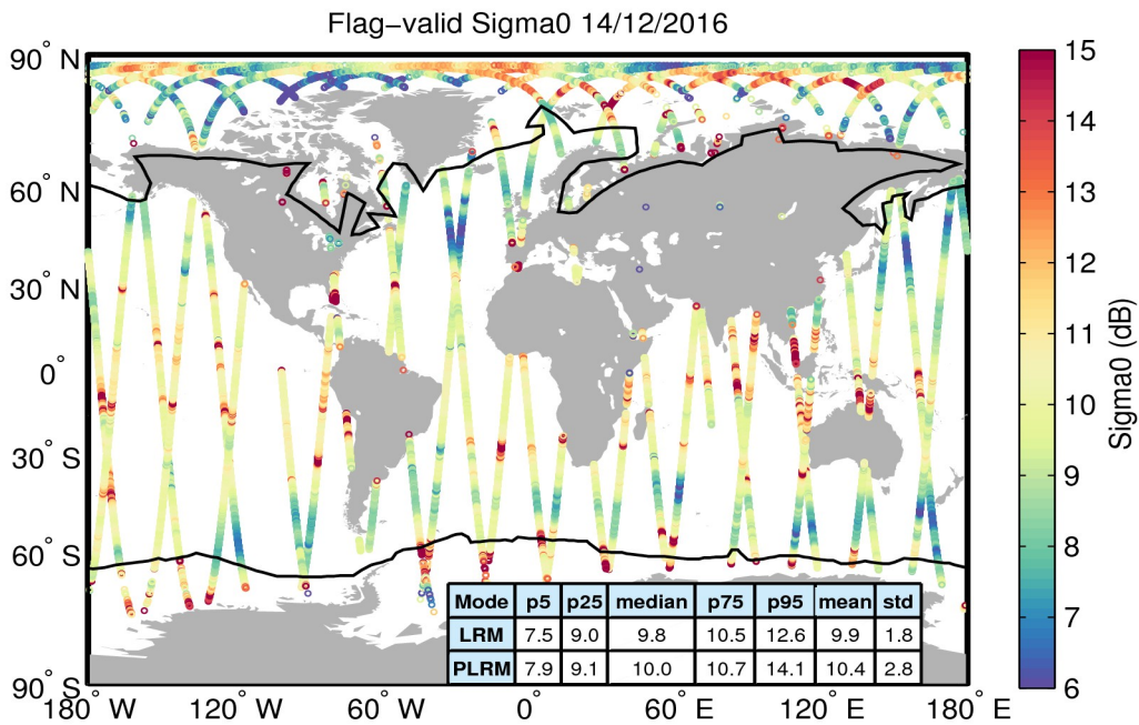
Figure 23. Geographical distribution of flag-valid sigma0 data over oceans and lakes for 14/12/2016. The statistical values shown in the table refer to the sigma0 in dB and are calculated separately for LRM and PLRM regions. Measurements taken over polar polygons have been excluded from the computation of the statistical values. The black lines mark the outer limit of the Arctic and Antarctic polar polygons.
