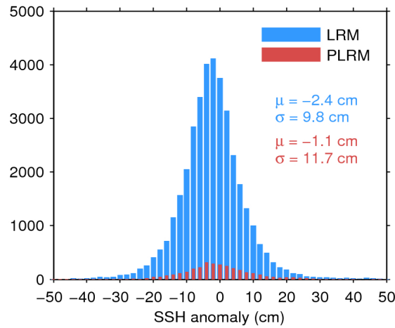
Figure 11. Histogram of science-valid SSH anomaly over oceans and lakes for LRM (blue) and PLRM (red) for 14/12/2016. The mean ( \mu ) and standard deviation ( \sigma ) are also shown. Note that values outside [-50\ 50] cm are excluded from the histogram for the sake of readability but not from the computation of \mu and \sigma .
