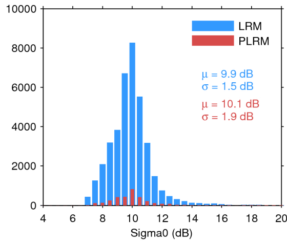
Figure 28. Histogram of science-valid sigma0 over oceans and lakes for LRM (blue) and PLRM (red) for 14/12/2016. The mean ( \mu ) and standard deviation ( \sigma ) are also shown. Note that values outside [4 20] dB are excluded from the histogram for the sake of readability but not from the computation of \mu and \sigma .
