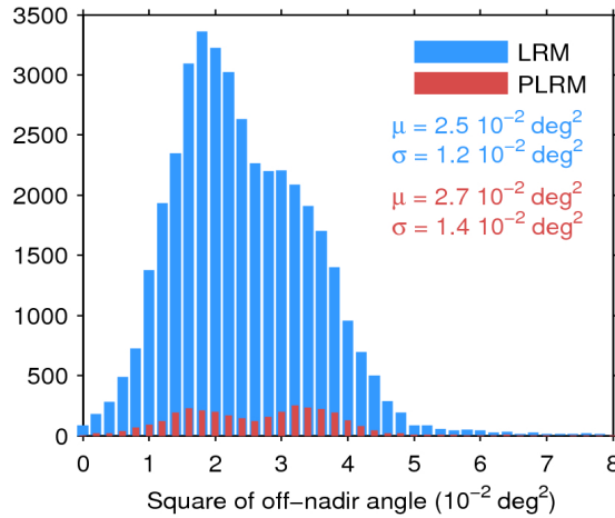
Figure 39. Histogram of flag-valid mispointing over oceans and lakes for LRM (blue) and PLRM (red) for 14/12/2016. Only positive values have been considered. The mean ( \mu ) and standard deviation ( \sigma ) are also shown. Note that values larger than 8 \cdot 10^{-2} \text{ deg}^2 are excluded from the histogram for the sake of readability but not from the computation of \mu and \sigma .
