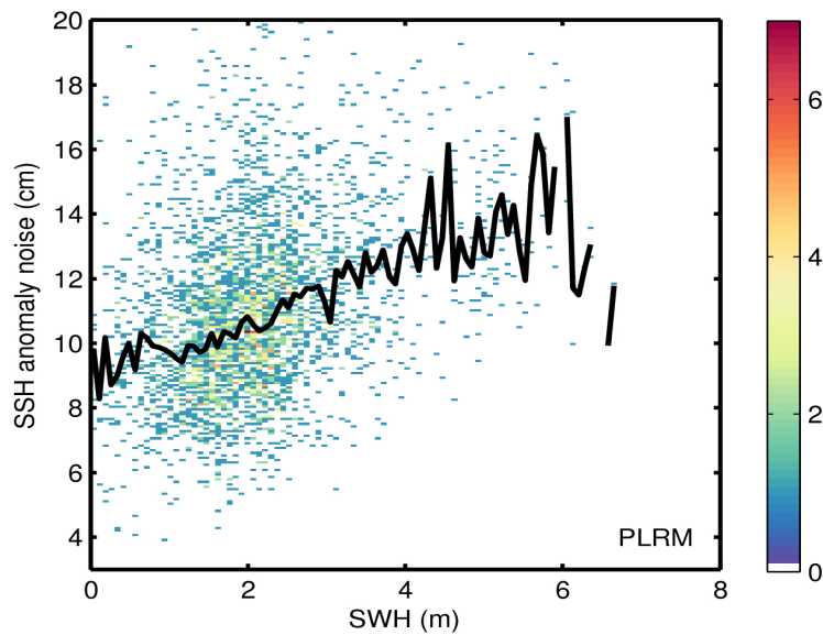
Figure 9. 2D histogram showing flag-valid SSH anomaly noise as a function of SWH for LRM (top) and PLRM (bottom) for 14/12/2016. The black line denotes the median SSH anomaly noise as a function of SWH.
