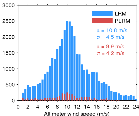
Figure 33. Histogram of flag-valid wind over oceans and lakes for LRM (blue) and PLRM (red) for 14/12/2016. The mean ( \mu ) and standard deviation ( \sigma ) are also shown. Note that values larger than 24 m/s are excluded from the histogram for the sake of readability but not from the computation of \mu and \sigma .
