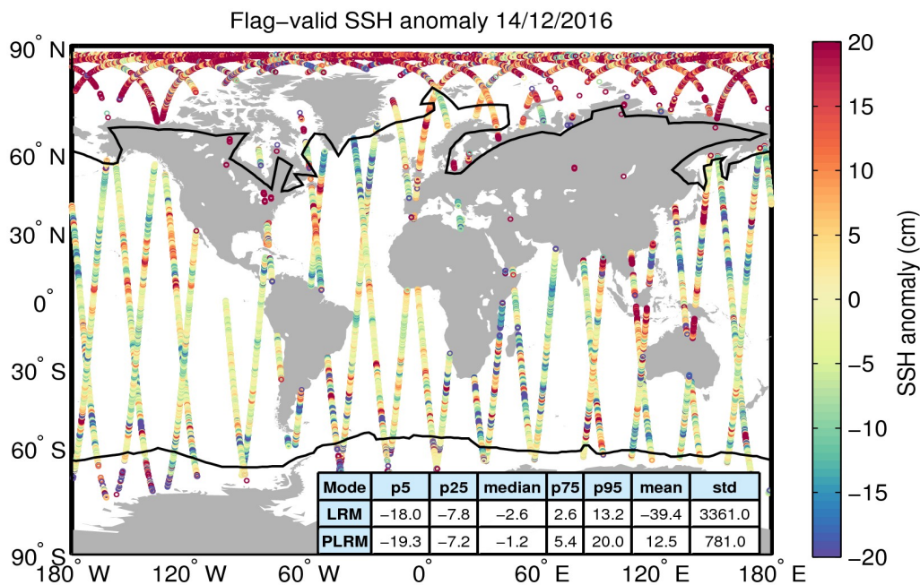
Figure 5. Geographical distribution of flag-valid 1-Hz SSH anomaly data over oceans and lakes for 14/12/2016. The statistical values shown in the table refer to the SSH anomaly in cm and are calculated separately for LRM and PLRM regions. Measurements taken over polar polygons have been excluded from the computation of the statistical values. The black lines mark the outer limit of the Arctic and Antarctic polar polygons.
