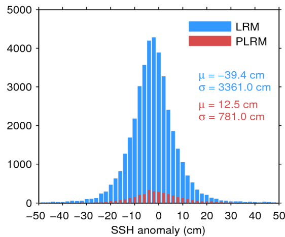
Figure 7. Histogram of flag-valid SSH anomaly over oceans and lakes for LRM (blue) and PLRM (red) for 14/12/2016. The mean ( \mu ) and standard deviation ( \sigma ) are also shown. Note that values outside [-50 50] cm are excluded from the histogram for the sake of readability but not from the computation of \mu and \sigma .
