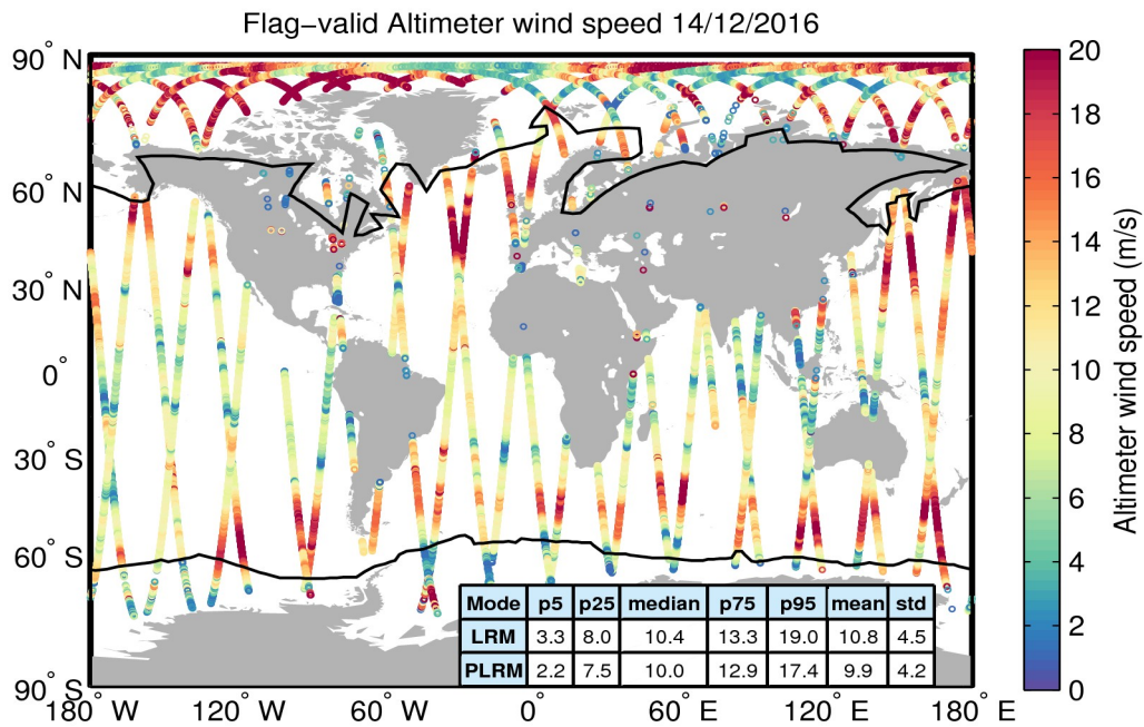
Figure 31. Geographical distribution of flag-valid wind data over oceans and lakes for 14/12/2016. The statistical values shown in the table refer to the wind in m/s and are calculated separately for LRM and PLRM regions. Measurements taken over polar polygons have been excluded from the computation of the statistical values. The black lines mark the outer limit of the Arctic and Antarctic polar polygons.
