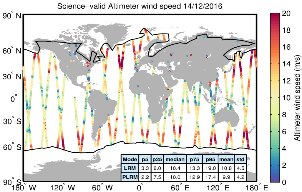
Figure 34. Geographical distribution of science-valid wind data over oceans and lakes for 14/12/2016. The statistical values shown in the table refer to the wind in m/s and are calculated separately for LRM and PLRM regions. The black lines mark the outer limit of the Arctic and Antarctic polar polygons. Gray circles denote records that have been rejected based on the editing criteria described in Table 5.
