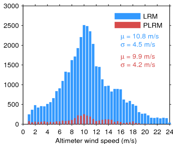
Figure 35. Histogram of science-valid wind over oceans and lakes for LRM (blue) and PLRM (red) for 14/12/2016. The mean ( \mu ) and standard deviation ( \sigma ) are also shown. Note that values larger than 24 m/s are excluded from the histogram for the sake of readability but not from the computation of \mu and \sigma .
