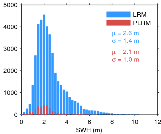
Figure 20. Histogram of science-valid SWH over oceans and lakes for LRM (blue) and PLRM (red) for 14/12/2016. The mean ( \mu ) and standard deviation ( \sigma ) are also shown. Note that values larger than 12 m are excluded from the histogram for the sake of readability but not from the computation of \mu and \sigma .
