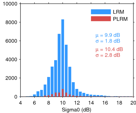
Figure 25. Histogram of flag-valid sigma0 over oceans and lakes for LRM (blue) and PLRM (red) for 14/12/2016. The mean ( \mu ) and standard deviation ( \sigma ) are also shown. Note that values outside [4 20] dB are excluded from the histogram for the sake of readability but not from the computation of \mu and \sigma .
