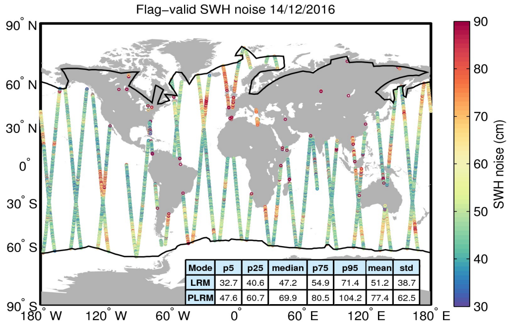
Figure 18. Geographical distribution of flag-valid 20-Hz SWH measurement noise over oceans and lakes for 14/12/2016. The statistical values shown in the table refer to the SWH noise and are calculated separately for LRM and PLRM regions. Measurements taken over polar polygons have been excluded from the computation of the statistical values. The black lines mark the outer limit of the Arctic and Antarctic polar polygons.
