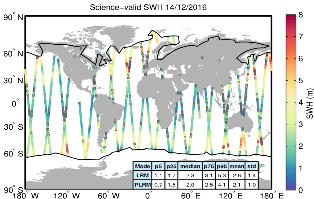
Figure 19. Geographical distribution of science-valid SWH data over oceans and lakes for 14/12/2016. The statistical values shown in the table refer to the SWH in m and are calculated separately for LRM and PLRM regions. The black lines mark the outer limit of the Arctic and Antarctic polar polygons. Gray circles denote records that have been rejected based on the editing criteria described in Table 3.
