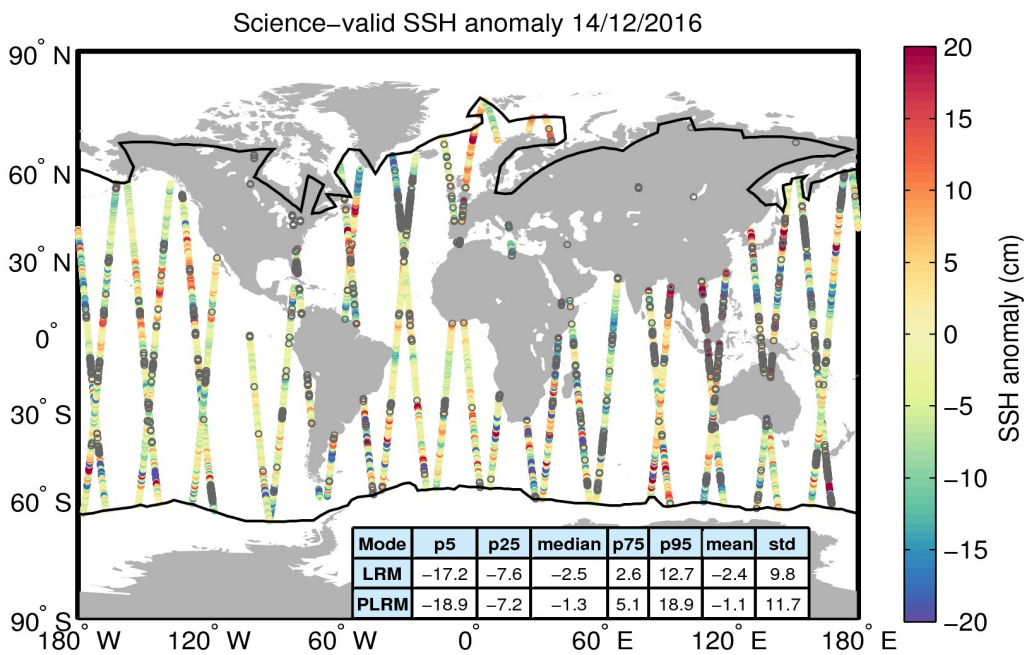
Figure 10. Geographical distribution of science-valid SSH anomaly data over oceans and lakes for 14/12/2016. The statistical values shown in the table refer to the SSH anomaly in cm and are calculated separately for LRM and PLRM regions. The black lines mark the outer limit of the Arctic and Antarctic polar polygons. Gray circles denote records that have been rejected based on the editing criteria described in Table 2.
