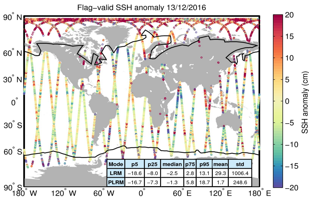
Figure 5. Geographical distribution of flag-valid 1-Hz SSH anomaly data over oceans and lakes for 13/12/2016. The statistical values shown in the table refer to the SSH anomaly in cm and are calculated separately for LRM and PLRM regions. Measurements taken over polar polygons have been excluded from the computation of the statistical values. The black lines mark the outer limit of the Arctic and Antarctic polar polygons.
