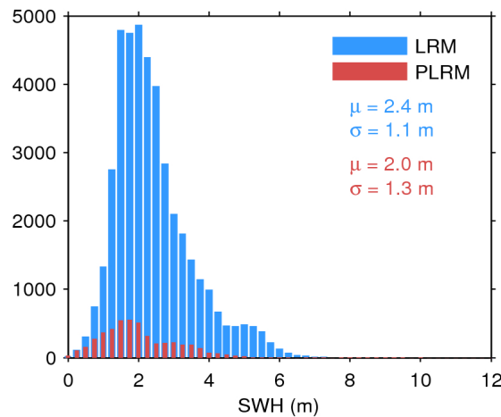
Figure 17. Histogram of flag-valid SWH over oceans and lakes for LRM (blue) and PLRM (red) for 13/12/2016. The mean ( \mu ) and standard deviation ( \sigma ) are also shown. Note that values larger than 12 m are excluded from the histogram for the sake of readability but not from the computation of \mu and \sigma .
