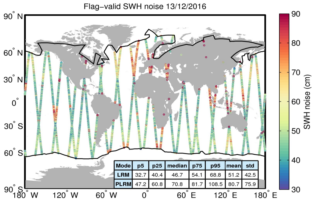
Figure 18. Geographical distribution of flag-valid 20-Hz SWH measurement noise over oceans and lakes for 13/12/2016. The statistical values shown in the table refer to the SWH noise and are calculated separately for LRM and PLRM regions. Measurements taken over polar polygons have been excluded from the computation of the statistical values. The black lines mark the outer limit of the Arctic and Antarctic polar polygons.
