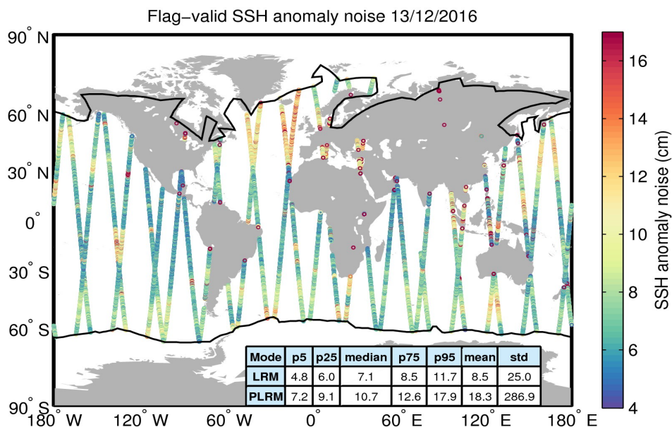
Figure 8. Geographical distribution of flag-valid 20-Hz SSH anomaly measurement noise over oceans and lakes for 13/12/2016. The statistical values shown in the table refer to the SSH anomaly noise and are calculated separately for LRM and PLRM regions. Measurements taken over polar polygons have been excluded from the computation of the statistical values. The black lines mark the outer limit of the Arctic and Antarctic polar polygons.
