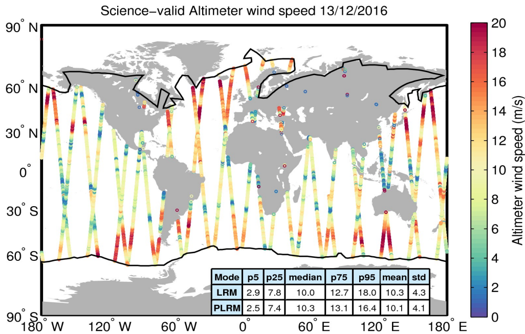
Figure 34. Geographical distribution of science-valid wind data over oceans and lakes for 13/12/2016. The statistical values shown in the table refer to the wind in m/s and are calculated separately for LRM and PLRM regions. The black lines mark the outer limit of the Arctic and Antarctic polar polygons. Gray circles denote records that have been rejected based on the editing criteria described in Table 5.
