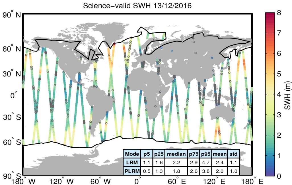
Figure 19. Geographical distribution of science-valid SWH data over oceans and lakes for 13/12/2016. The statistical values shown in the table refer to the SWH in m and are calculated separately for LRM and PLRM regions. The black lines mark the outer limit of the Arctic and Antarctic polar polygons. Gray circles denote records that have been rejected based on the editing criteria described in Table 3.
