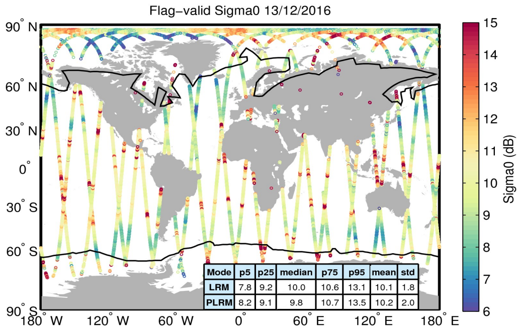
Figure 23. Geographical distribution of flag-valid sigma0 data over oceans and lakes for 13/12/2016. The statistical values shown in the table refer to the sigma0 in dB and are calculated separately for LRM and PLRM regions. Measurements taken over polar polygons have been excluded from the computation of the statistical values. The black lines mark the outer limit of the Arctic and Antarctic polar polygons.
