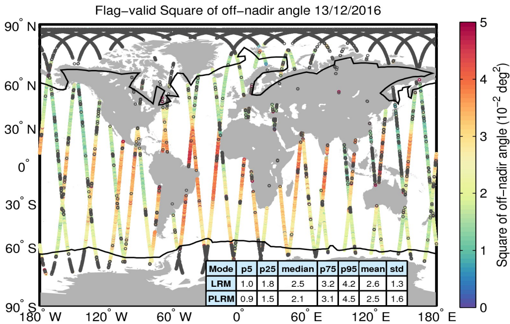
Figure 37. Geographical distribution of flag-valid mispointing data over oceans and lakes for 13/12/2016. The statistical values shown in the table refer to the mispointing in 10^{-2} \text{deg}^2 and are calculated separately for LRM and PLRM regions. Measurements taken over polar polygons have been excluded from the computation of the statistical values. The black lines mark the outer limit of the Arctic and Antarctic polar polygons. Gray circles denote negative values.
