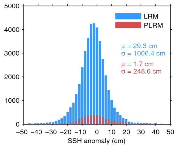
Figure 7. Histogram of flag-valid SSH anomaly over oceans and lakes for LRM (blue) and PLRM (red) for 13/12/2016. The mean ( \mu ) and standard deviation ( \sigma ) are also shown. Note that values outside [-50\ 50] cm are excluded from the histogram for the sake of readability but not from the computation of \mu and \sigma .
