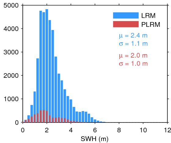
Figure 20. Histogram of science-valid SWH over oceans and lakes for LRM (blue) and PLRM (red) for 13/12/2016. The mean ( \mu ) and standard deviation ( \sigma ) are also shown. Note that values larger than 12 m are excluded from the histogram for the sake of readability but not from the computation of \mu and \sigma .
