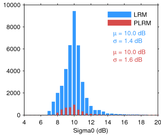
Figure 28. Histogram of science-valid sigma0 over oceans and lakes for LRM (blue) and PLRM (red) for 13/12/2016. The mean ( \mu ) and standard deviation ( \sigma ) are also shown. Note that values outside [4 20] dB are excluded from the histogram for the sake of readability but not from the computation of \mu and \sigma .
