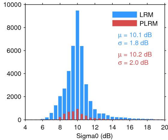
Figure 25. Histogram of flag-valid sigma0 over oceans and lakes for LRM (blue) and PLRM (red) for 13/12/2016. The mean ( \mu ) and standard deviation ( \sigma ) are also shown. Note that values outside [4 20] dB are excluded from the histogram for the sake of readability but not from the computation of \mu and \sigma .
