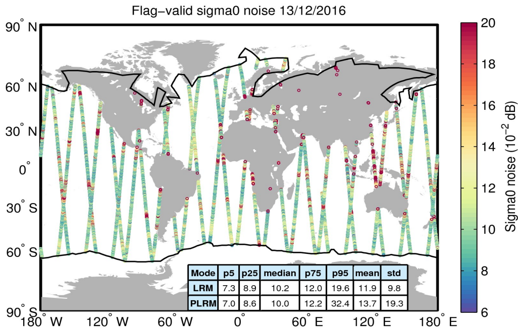
Figure 26. Geographical distribution of flag-valid 20-Hz sigma0 measurement noise over oceans and lakes for 13/12/2016. The statistical values shown in the table refer to the sigma0 noise and are calculated separately for LRM and PLRM regions. Measurements taken over polar polygons have been excluded from the computation of the statistical values. The black lines mark the outer limit of the Arctic and Antarctic polar polygons.
