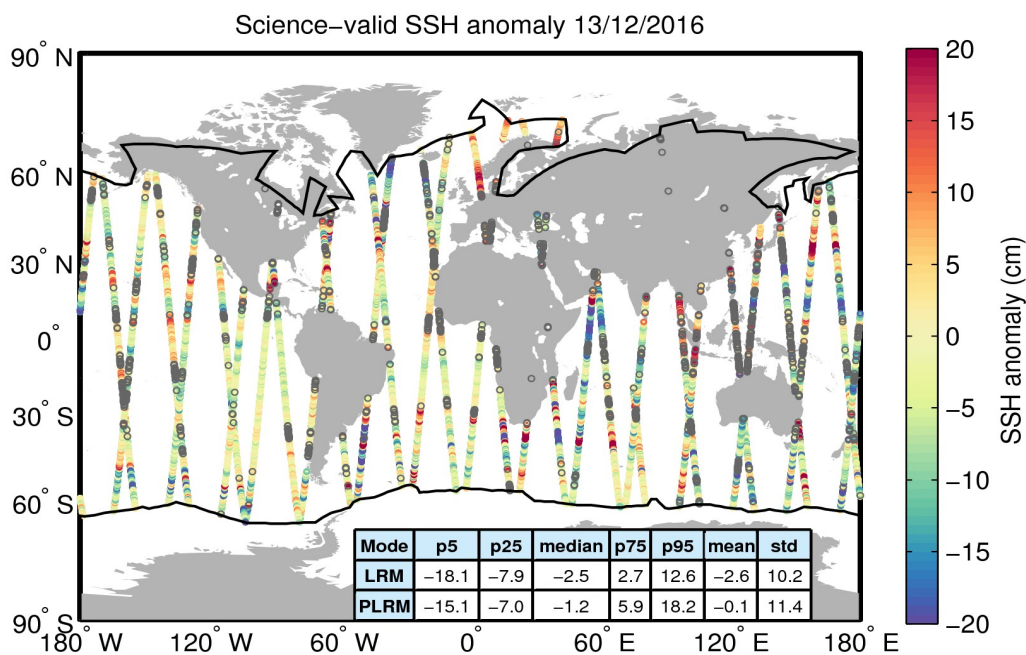
Figure 10. Geographical distribution of science-valid SSH anomaly data over oceans and lakes for 13/12/2016. The statistical values shown in the table refer to the SSH anomaly in cm and are calculated separately for LRM and PLRM regions. The black lines mark the outer limit of the Arctic and Antarctic polar polygons. Gray circles denote records that have been rejected based on the editing criteria described in Table 2.
