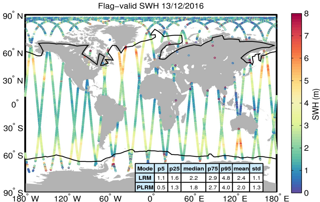
Figure 15. Geographical distribution of flag-valid SWH data over oceans and lakes for 13/12/2016. The statistical values shown in the table refer to the SWH in m and are calculated separately for LRM and PLRM regions. Measurements taken over polar polygons have been excluded from the computation of the statistical values. The black lines mark the outer limit of the Arctic and Antarctic polar polygons.
