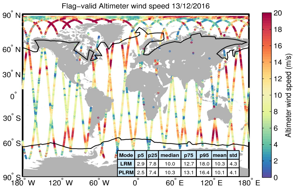
Figure 31. Geographical distribution of flag-valid wind data over oceans and lakes for 13/12/2016. The statistical values shown in the table refer to the wind in m/s and are calculated separately for LRM and PLRM regions. Measurements taken over polar polygons have been excluded from the computation of the statistical values. The black lines mark the outer limit of the Arctic and Antarctic polar polygons.
