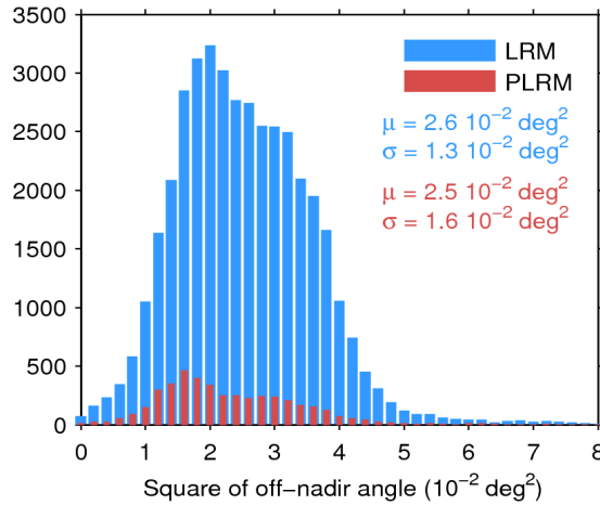
Figure 39. Histogram of flag-valid mispointing over oceans and lakes for LRM (blue) and PLRM (red) for 13/12/2016. Only positive values have been considered. The mean ( \mu ) and standard deviation ( \sigma ) are also shown. Note that values larger than 8 \cdot 10^{-2} \text{ deg}^2 are excluded from the histogram for the sake of readability but not from the computation of \mu and \sigma .
