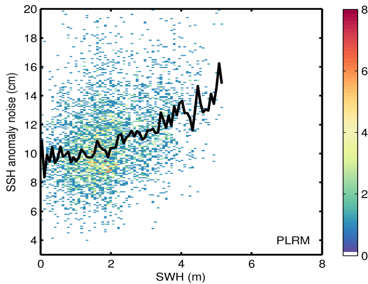
Figure 9. 2D histogram showing flag-valid SSH anomaly noise as a function of SWH for LRM (top) and PLRM (bottom) for 13/12/2016. The black line denotes the median SSH anomaly noise as a function of SWH.
