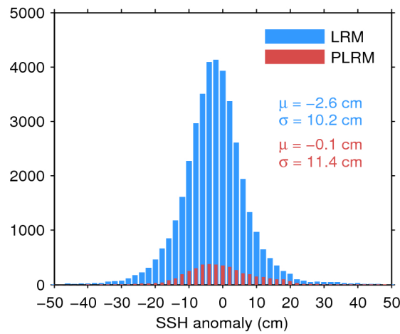
Figure 11. Histogram of science-valid SSH anomaly over oceans and lakes for LRM (blue) and PLRM (red) for 13/12/2016. The mean ( \mu ) and standard deviation ( \sigma ) are also shown. Note that values outside [-50\ 50] cm are excluded from the histogram for the sake of readability but not from the computation of \mu and \sigma .
