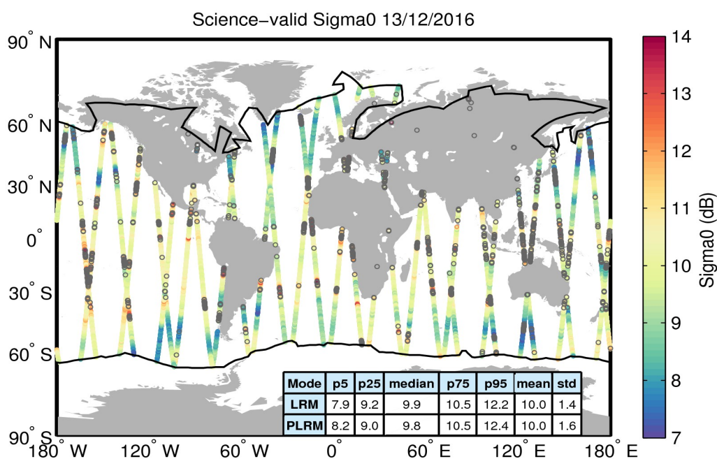
Figure 27. Geographical distribution of science-valid sigma0 data over oceans and lakes for 13/12/2016. The statistical values shown in the table refer to the sigma0 in dB and are calculated separately for LRM and PLRM regions. The black lines mark the outer limit of the Arctic and Antarctic polar polygons. Gray circles denote records that have been rejected based on the editing criteria described in Table 4.
