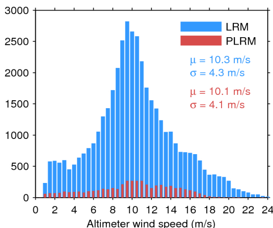
Figure 33. Histogram of flag-valid wind over oceans and lakes for LRM (blue) and PLRM (red) for 13/12/2016. The mean ( \mu ) and standard deviation ( \sigma ) are also shown. Note that values larger than 24 m/s are excluded from the histogram for the sake of readability but not from the computation of \mu and \sigma .
