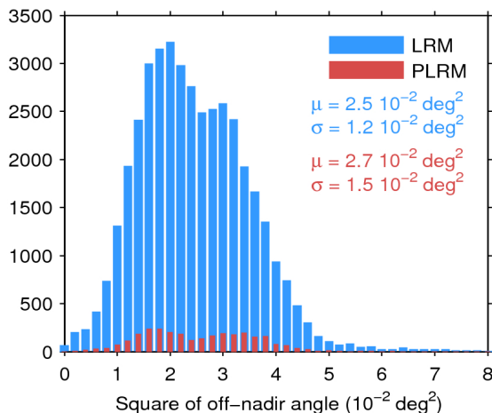
Figure 39. Histogram of flag-valid mispointing over oceans and lakes for LRM (blue) and PLRM (red) for 12/12/2016. Only positive values have been considered. The mean ( \mu ) and standard deviation ( \sigma ) are also shown. Note that values larger than 8 \cdot 10^{-2} \text{ deg}^2 are excluded from the histogram for the sake of readability but not from the computation of \mu and \sigma .
