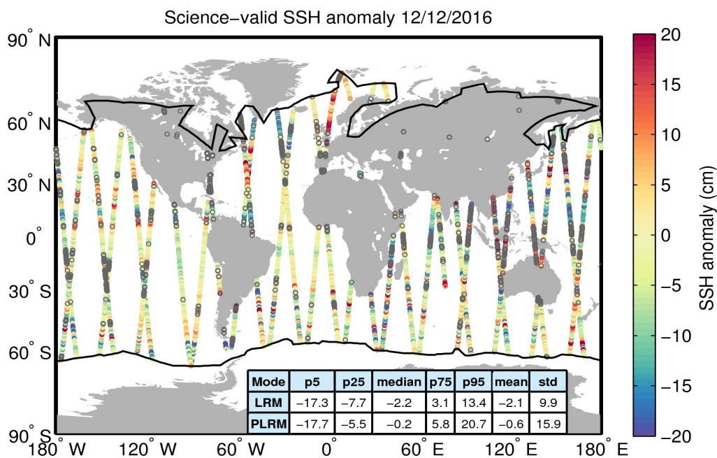
Figure 10. Geographical distribution of science-valid SSH anomaly data over oceans and lakes for 12/12/2016. The statistical values shown in the table refer to the SSH anomaly in cm and are calculated separately for LRM and PLRM regions. The black lines mark the outer limit of the Arctic and Antarctic polar polygons. Gray circles denote records that have been rejected based on the editing criteria described in Table 2.
