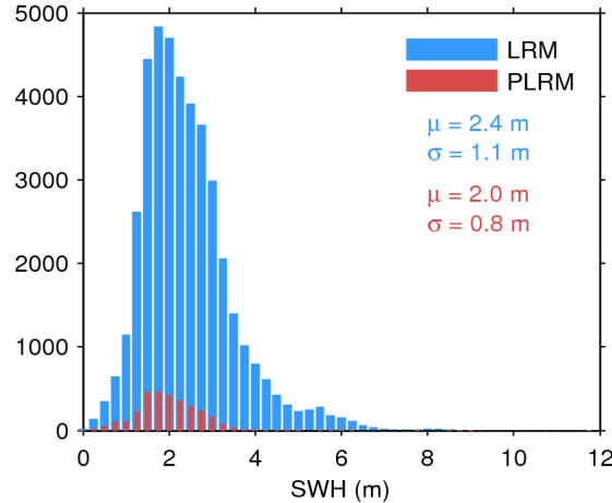
Figure 17. Histogram of flag-valid SWH over oceans and lakes for LRM (blue) and PLRM (red) for 12/12/2016. The mean ( \mu ) and standard deviation ( \sigma ) are also shown. Note that values larger than 12 m are excluded from the histogram for the sake of readability but not from the computation of \mu and \sigma .
