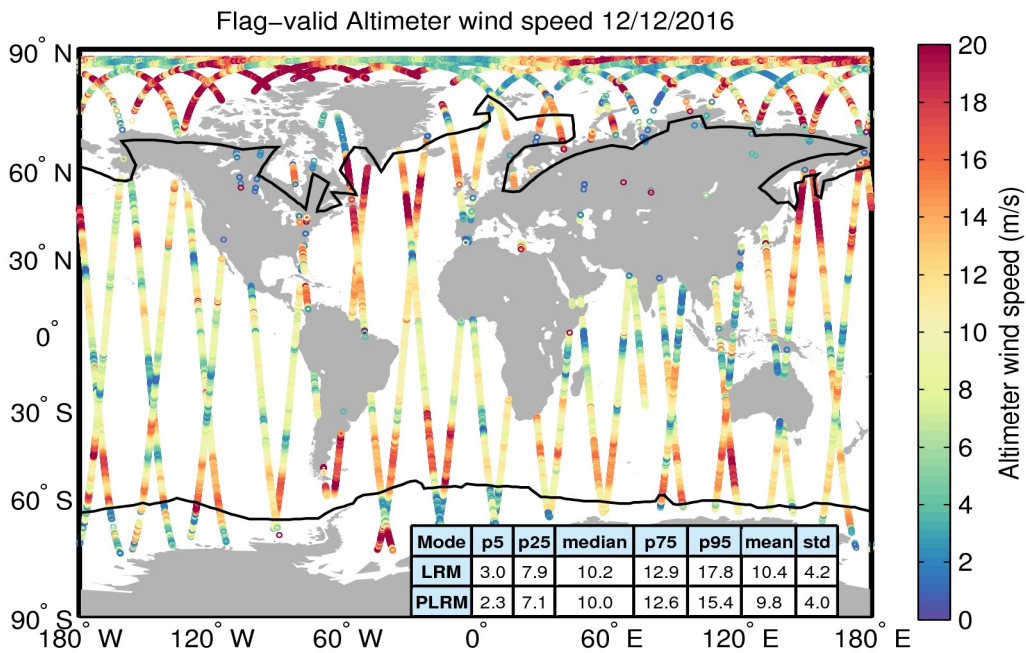
Figure 31. Geographical distribution of flag-valid wind data over oceans and lakes for 12/12/2016. The statistical values shown in the table refer to the wind in m/s and are calculated separately for LRM and PLRM regions. Measurements taken over polar polygons have been excluded from the computation of the statistical values. The black lines mark the outer limit of the Arctic and Antarctic polar polygons.
