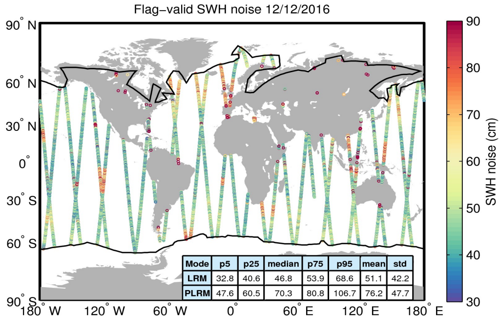
Figure 18. Geographical distribution of flag-valid 20-Hz SWH measurement noise over oceans and lakes for 12/12/2016. The statistical values shown in the table refer to the SWH noise and are calculated separately for LRM and PLRM regions. Measurements taken over polar polygons have been excluded from the computation of the statistical values. The black lines mark the outer limit of the Arctic and Antarctic polar polygons.
