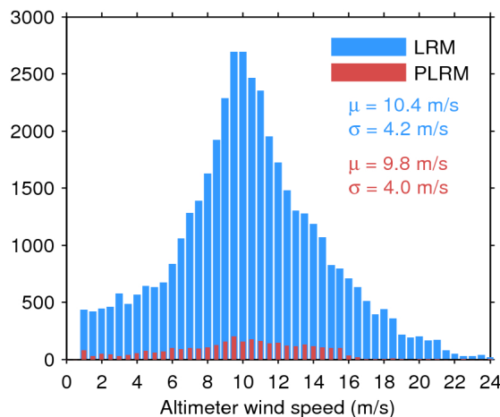
Figure 35. Histogram of science-valid wind over oceans and lakes for LRM (blue) and PLRM (red) for 12/12/2016. The mean ( \mu ) and standard deviation ( \sigma ) are also shown. Note that values larger than 24 m/s are excluded from the histogram for the sake of readability but not from the computation of \mu and \sigma .
