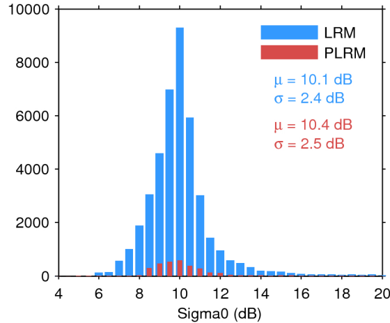
Figure 25. Histogram of flag-valid sigma0 over oceans and lakes for LRM (blue) and PLRM (red) for 12/12/2016. The mean ( \mu ) and standard deviation ( \sigma ) are also shown. Note that values outside [4 20] dB are excluded from the histogram for the sake of readability but not from the computation of \mu and \sigma .
