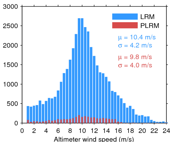
Figure 33. Histogram of flag-valid wind over oceans and lakes for LRM (blue) and PLRM (red) for 12/12/2016. The mean ( \mu ) and standard deviation ( \sigma ) are also shown. Note that values larger than 24 m/s are excluded from the histogram for the sake of readability but not from the computation of \mu and \sigma .
