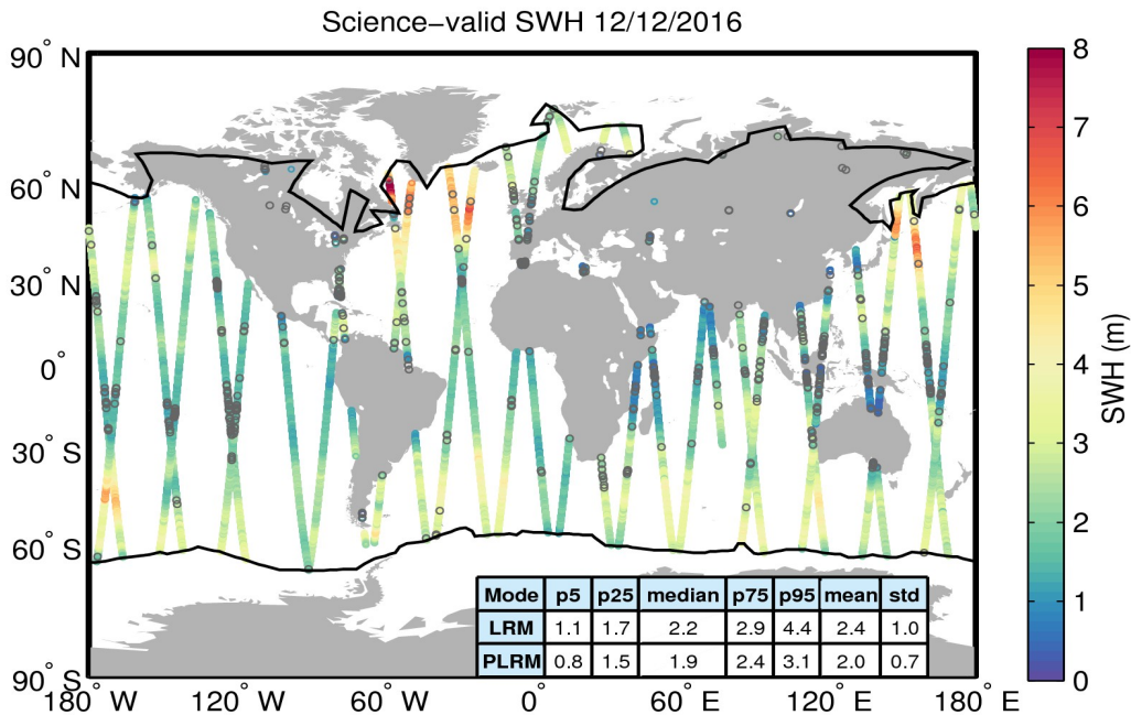
Figure 19. Geographical distribution of science-valid SWH data over oceans and lakes for 12/12/2016. The statistical values shown in the table refer to the SWH in m and are calculated separately for LRM and PLRM regions. The black lines mark the outer limit of the Arctic and Antarctic polar polygons. Gray circles denote records that have been rejected based on the editing criteria described in Table 3.
