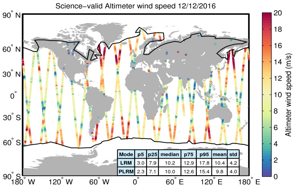
Figure 34. Geographical distribution of science-valid wind data over oceans and lakes for 12/12/2016. The statistical values shown in the table refer to the wind in m/s and are calculated separately for LRM and PLRM regions. The black lines mark the outer limit of the Arctic and Antarctic polar polygons. Gray circles denote records that have been rejected based on the editing criteria described in Table 5.
