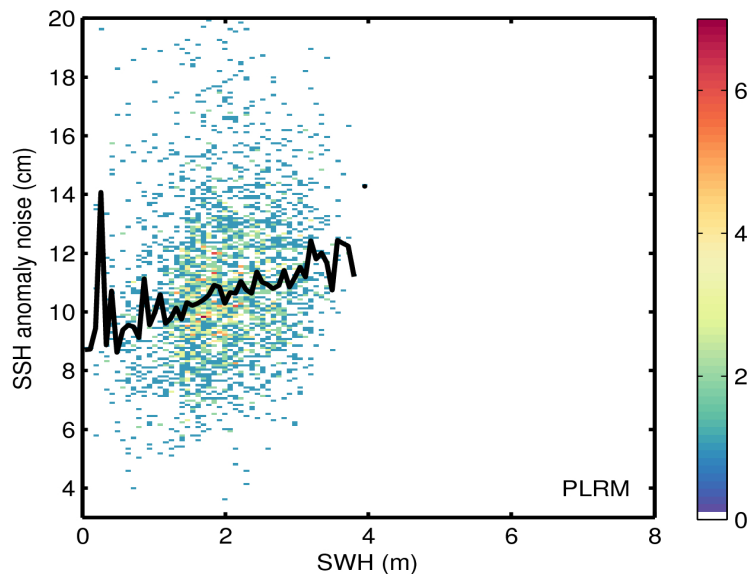
Figure 9. 2D histogram showing flag-valid SSH anomaly noise as a function of SWH for LRM (top) and PLRM (bottom) for 12/12/2016. The black line denotes the median SSH anomaly noise as a function of SWH.
