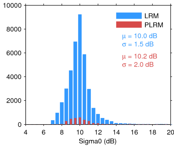
Figure 28. Histogram of science-valid sigma0 over oceans and lakes for LRM (blue) and PLRM (red) for 12/12/2016. The mean ( \mu ) and standard deviation ( \sigma ) are also shown. Note that values outside [4 20] dB are excluded from the histogram for the sake of readability but not from the computation of \mu and \sigma .
