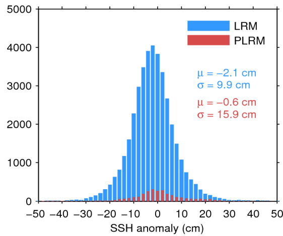
Figure 11. Histogram of science-valid SSH anomaly over oceans and lakes for LRM (blue) and PLRM (red) for 12/12/2016. The mean ( \mu ) and standard deviation ( \sigma ) are also shown. Note that values outside [-50 50] cm are excluded from the histogram for the sake of readability but not from the computation of \mu and \sigma .
