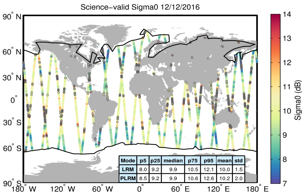
Figure 27. Geographical distribution of science-valid sigma0 data over oceans and lakes for 12/12/2016. The statistical values shown in the table refer to the sigma0 in dB and are calculated separately for LRM and PLRM regions. The black lines mark the outer limit of the Arctic and Antarctic polar polygons. Gray circles denote records that have been rejected based on the editing criteria described in Table 4.
