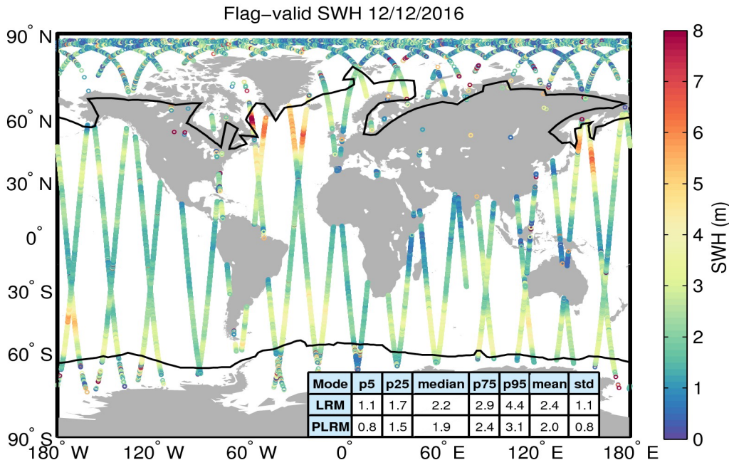
Figure 15. Geographical distribution of flag-valid SWH data over oceans and lakes for 12/12/2016. The statistical values shown in the table refer to the SWH in m and are calculated separately for LRM and PLRM regions. Measurements taken over polar polygons have been excluded from the computation of the statistical values. The black lines mark the outer limit of the Arctic and Antarctic polar polygons.
