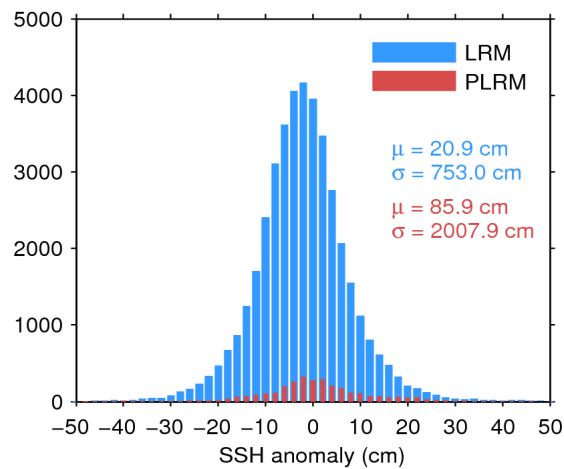
Figure 7. Histogram of flag-valid SSH anomaly over oceans and lakes for LRM (blue) and PLRM (red) for 12/12/2016. The mean ( \mu ) and standard deviation ( \sigma ) are also shown. Note that values outside [-50 50] cm are excluded from the histogram for the sake of readability but not from the computation of \mu and \sigma .
