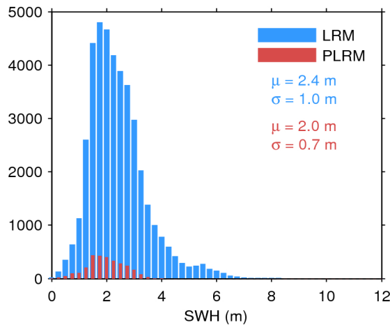
Figure 20. Histogram of science-valid SWH over oceans and lakes for LRM (blue) and PLRM (red) for 12/12/2016. The mean ( \mu ) and standard deviation ( \sigma ) are also shown. Note that values larger than 12 m are excluded from the histogram for the sake of readability but not from the computation of \mu and \sigma .
