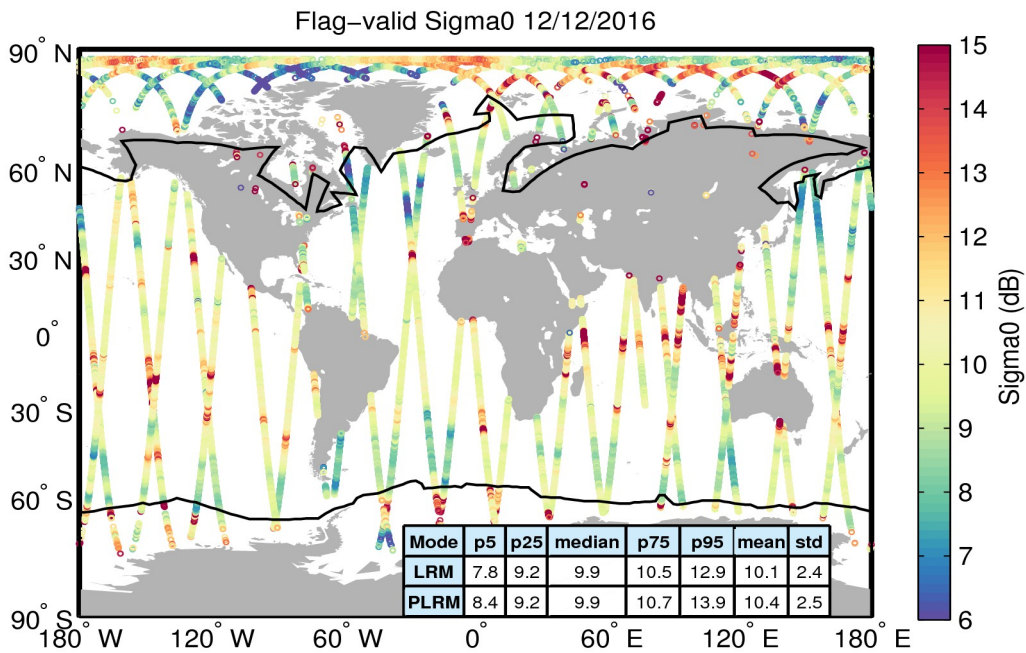
Figure 23. Geographical distribution of flag-valid sigma0 data over oceans and lakes for 12/12/2016. The statistical values shown in the table refer to the sigma0 in dB and are calculated separately for LRM and PLRM regions. Measurements taken over polar polygons have been excluded from the computation of the statistical values. The black lines mark the outer limit of the Arctic and Antarctic polar polygons.
