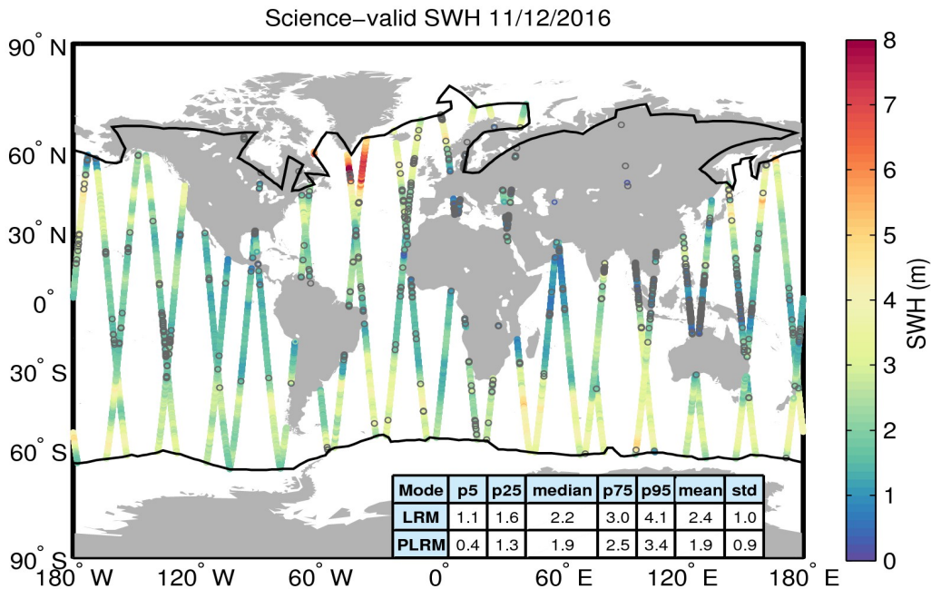
Figure 19. Geographical distribution of science-valid SWH data over oceans and lakes for 11/12/2016. The statistical values shown in the table refer to the SWH in m and are calculated separately for LRM and PLRM regions. The black lines mark the outer limit of the Arctic and Antarctic polar polygons. Gray circles denote records that have been rejected based on the editing criteria described in Table 3.
