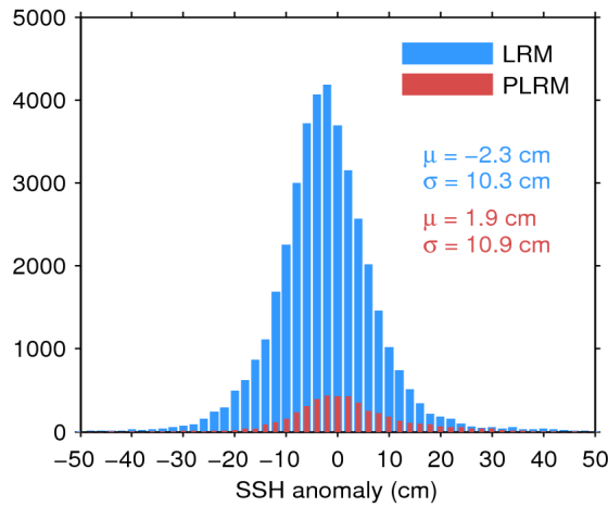
Figure 11. Histogram of science-valid SSH anomaly over oceans and lakes for LRM (blue) and PLRM (red) for 11/12/2016. The mean ( \mu ) and standard deviation ( \sigma ) are also shown. Note that values outside [-50\ 50] cm are excluded from the histogram for the sake of readability but not from the computation of \mu and \sigma .
