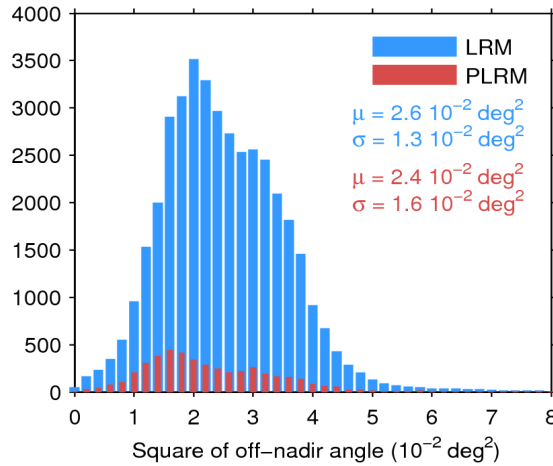
Figure 39. Histogram of flag-valid mispointing over oceans and lakes for LRM (blue) and PLRM (red) for 11/12/2016. Only positive values have been considered. The mean ( \mu ) and standard deviation ( \sigma ) are also shown. Note that values larger than 8 \cdot 10^{-2} \text{ deg}^2 are excluded from the histogram for the sake of readability but not from the computation of \mu and \sigma .
