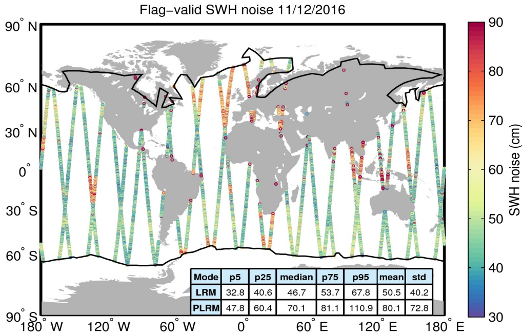
Figure 18. Geographical distribution of flag-valid 20-Hz SWH measurement noise over oceans and lakes for 11/12/2016. The statistical values shown in the table refer to the SWH noise and are calculated separately for LRM and PLRM regions. Measurements taken over polar polygons have been excluded from the computation of the statistical values. The black lines mark the outer limit of the Arctic and Antarctic polar polygons.
