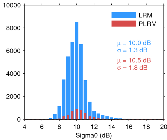
Figure 28. Histogram of science-valid sigma0 over oceans and lakes for LRM (blue) and PLRM (red) for 11/12/2016. The mean ( \mu ) and standard deviation ( \sigma ) are also shown. Note that values outside [4 20] dB are excluded from the histogram for the sake of readability but not from the computation of \mu and \sigma .
