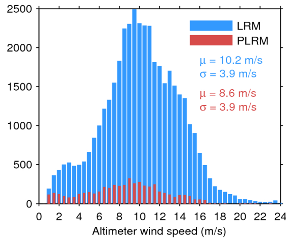
Figure 33. Histogram of flag-valid wind over oceans and lakes for LRM (blue) and PLRM (red) for 11/12/2016. The mean ( \mu ) and standard deviation ( \sigma ) are also shown. Note that values larger than 24 m/s are excluded from the histogram for the sake of readability but not from the computation of \mu and \sigma .
