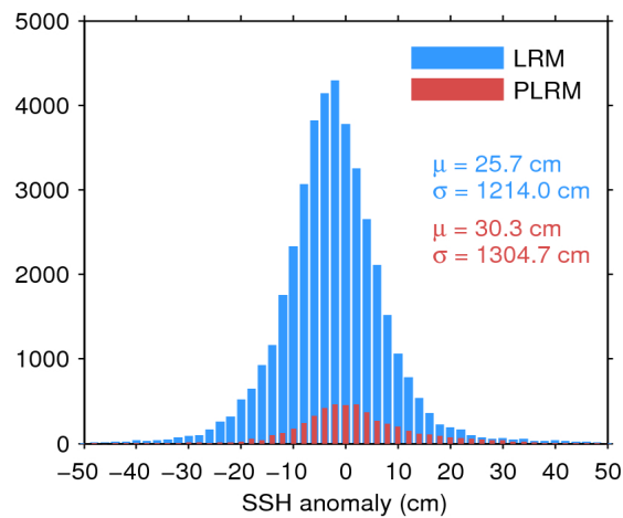
Figure 7. Histogram of flag-valid SSH anomaly over oceans and lakes for LRM (blue) and PLRM (red) for 11/12/2016. The mean ( \mu ) and standard deviation ( \sigma ) are also shown. Note that values outside [-50\ 50] cm are excluded from the histogram for the sake of readability but not from the computation of \mu and \sigma .
