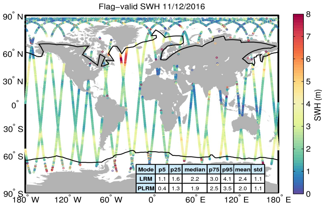
Figure 15. Geographical distribution of flag-valid SWH data over oceans and lakes for 11/12/2016. The statistical values shown in the table refer to the SWH in m and are calculated separately for LRM and PLRM regions. Measurements taken over polar polygons have been excluded from the computation of the statistical values. The black lines mark the outer limit of the Arctic and Antarctic polar polygons.
