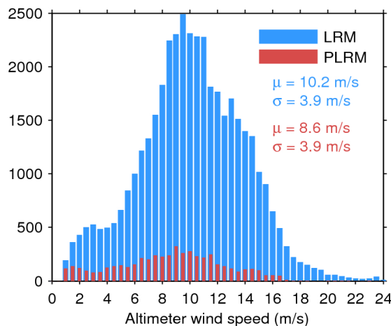
Figure 35. Histogram of science-valid wind over oceans and lakes for LRM (blue) and PLRM (red) for 11/12/2016. The mean ( \mu ) and standard deviation ( \sigma ) are also shown. Note that values larger than 24 m/s are excluded from the histogram for the sake of readability but not from the computation of \mu and \sigma .
