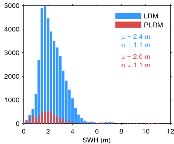
Figure 17. Histogram of flag-valid SWH over oceans and lakes for LRM (blue) and PLRM (red) for 11/12/2016. The mean ( \mu ) and standard deviation ( \sigma ) are also shown. Note that values larger than 12 m are excluded from the histogram for the sake of readability but not from the computation of \mu and \sigma .
