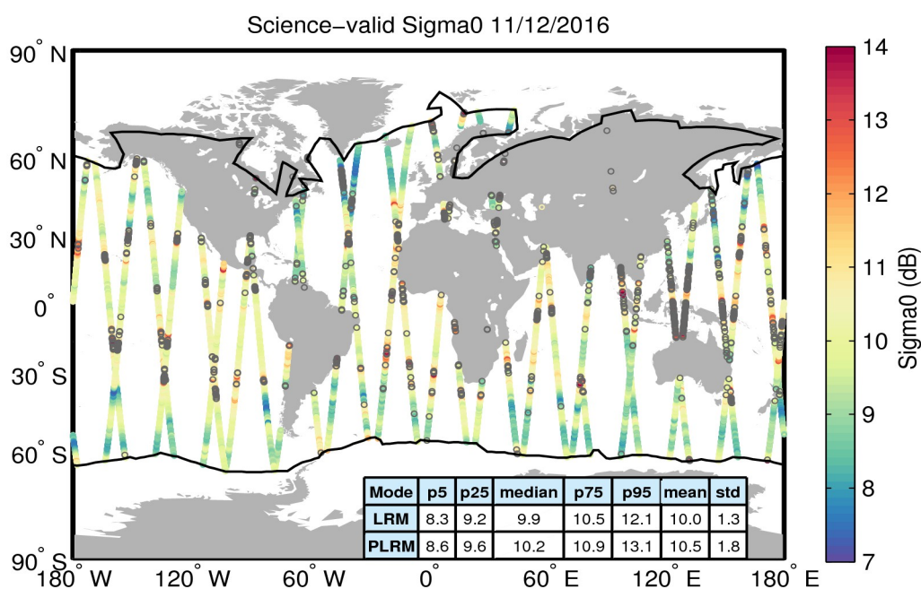
Figure 27. Geographical distribution of science-valid sigma0 data over oceans and lakes for 11/12/2016. The statistical values shown in the table refer to the sigma0 in dB and are calculated separately for LRM and PLRM regions. The black lines mark the outer limit of the Arctic and Antarctic polar polygons. Gray circles denote records that have been rejected based on the editing criteria described in Table 4.
