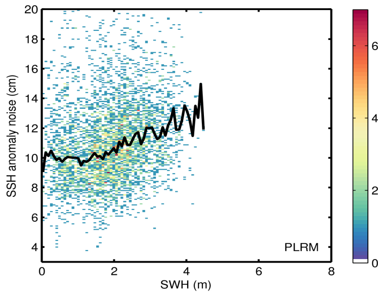
Figure 9. 2D histogram showing flag-valid SSH anomaly noise as a function of SWH for LRM (top) and PLRM (bottom) for 11/12/2016. The black line denotes the median SSH anomaly noise as a function of SWH.
