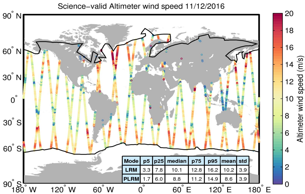
Figure 34. Geographical distribution of science-valid wind data over oceans and lakes for 11/12/2016. The statistical values shown in the table refer to the wind in m/s and are calculated separately for LRM and PLRM regions. The black lines mark the outer limit of the Arctic and Antarctic polar polygons. Gray circles denote records that have been rejected based on the editing criteria described in Table 5.
