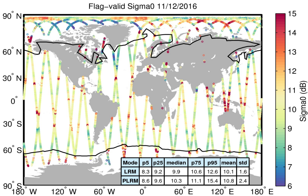
Figure 23. Geographical distribution of flag-valid sigma0 data over oceans and lakes for 11/12/2016. The statistical values shown in the table refer to the sigma0 in dB and are calculated separately for LRM and PLRM regions. Measurements taken over polar polygons have been excluded from the computation of the statistical values. The black lines mark the outer limit of the Arctic and Antarctic polar polygons.
