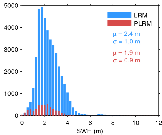
Figure 20. Histogram of science-valid SWH over oceans and lakes for LRM (blue) and PLRM (red) for 11/12/2016. The mean ( \mu ) and standard deviation ( \sigma ) are also shown. Note that values larger than 12 m are excluded from the histogram for the sake of readability but not from the computation of \mu and \sigma .
