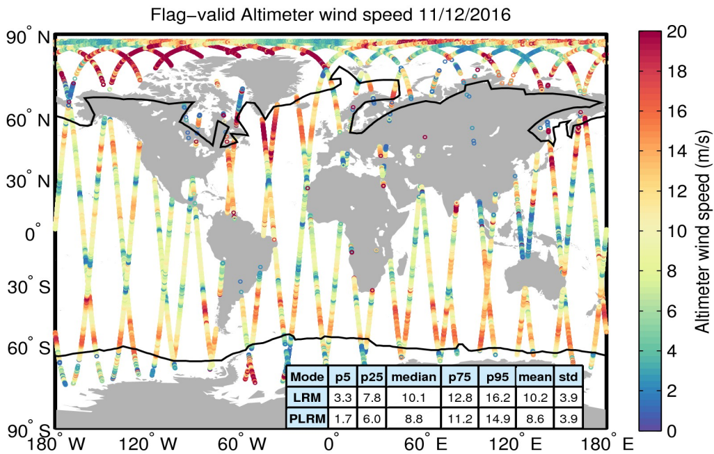
Figure 31. Geographical distribution of flag-valid wind data over oceans and lakes for 11/12/2016. The statistical values shown in the table refer to the wind in m/s and are calculated separately for LRM and PLRM regions. Measurements taken over polar polygons have been excluded from the computation of the statistical values. The black lines mark the outer limit of the Arctic and Antarctic polar polygons.
