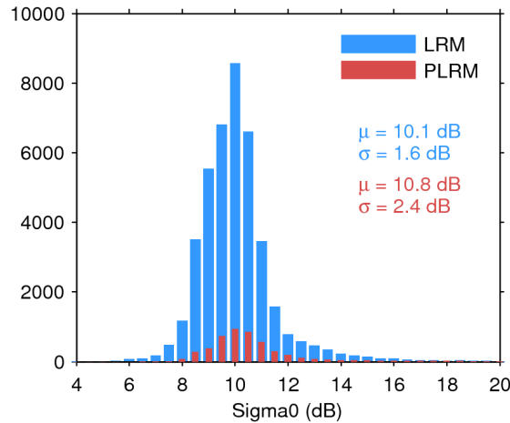
Figure 25. Histogram of flag-valid sigma0 over oceans and lakes for LRM (blue) and PLRM (red) for 11/12/2016. The mean ( \mu ) and standard deviation ( \sigma ) are also shown. Note that values outside [4 20] dB are excluded from the histogram for the sake of readability but not from the computation of \mu and \sigma .
