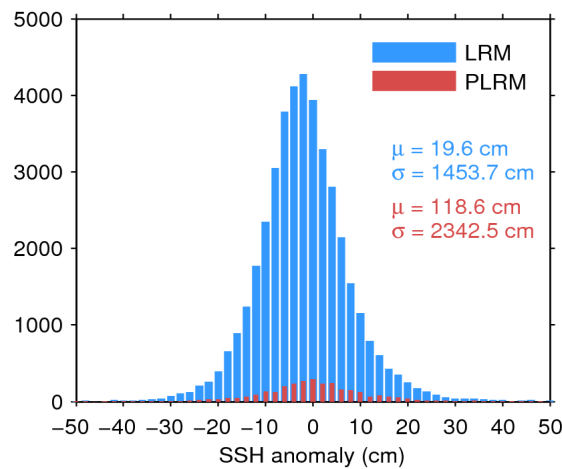
Figure 7. Histogram of flag-valid SSH anomaly over oceans and lakes for LRM (blue) and PLRM (red) for 10/12/2016. The mean ( \mu ) and standard deviation ( \sigma ) are also shown. Note that values outside [-50\ 50] cm are excluded from the histogram for the sake of readability but not from the computation of \mu and \sigma .
