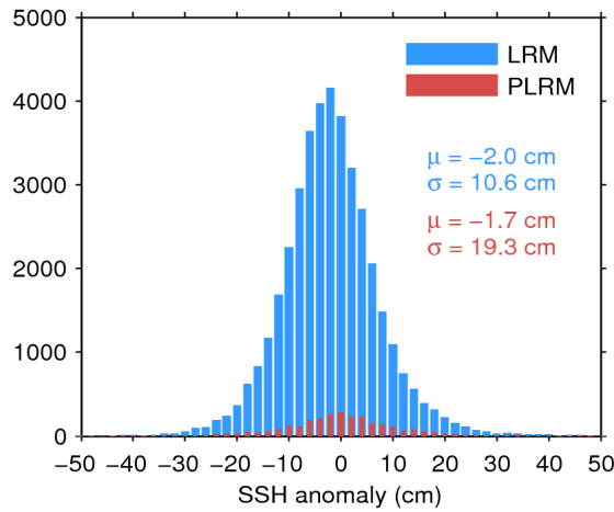
Figure 11. Histogram of science-valid SSH anomaly over oceans and lakes for LRM (blue) and PLRM (red) for 10/12/2016. The mean ( \mu ) and standard deviation ( \sigma ) are also shown. Note that values outside [-50 50] cm are excluded from the histogram for the sake of readability but not from the computation of \mu and \sigma .
