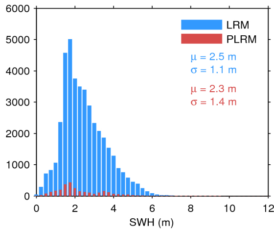
Figure 20. Histogram of science-valid SWH over oceans and lakes for LRM (blue) and PLRM (red) for 10/12/2016. The mean ( \mu ) and standard deviation ( \sigma ) are also shown. Note that values larger than 12 m are excluded from the histogram for the sake of readability but not from the computation of \mu and \sigma .
