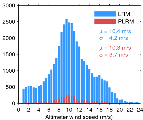
Figure 33. Histogram of flag-valid wind over oceans and lakes for LRM (blue) and PLRM (red) for 10/12/2016. The mean ( \mu ) and standard deviation ( \sigma ) are also shown. Note that values larger than 24 m/s are excluded from the histogram for the sake of readability but not from the computation of \mu and \sigma .
