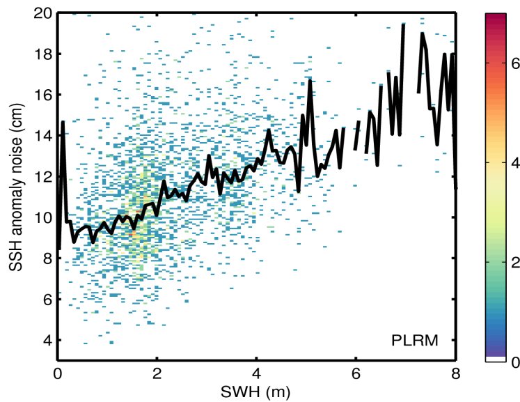
Figure 9. 2D histogram showing flag-valid SSH anomaly noise as a function of SWH for LRM (top) and PLRM (bottom) for 10/12/2016. The black line denotes the median SSH anomaly noise as a function of SWH.
