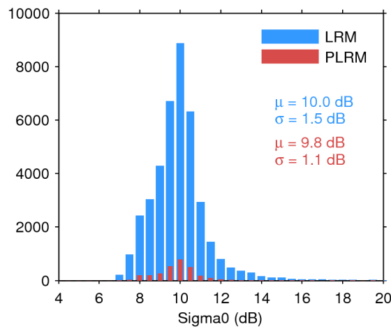
Figure 28. Histogram of science-valid sigma0 over oceans and lakes for LRM (blue) and PLRM (red) for 10/12/2016. The mean ( \mu ) and standard deviation ( \sigma ) are also shown. Note that values outside [4 20] dB are excluded from the histogram for the sake of readability but not from the computation of \mu and \sigma .
