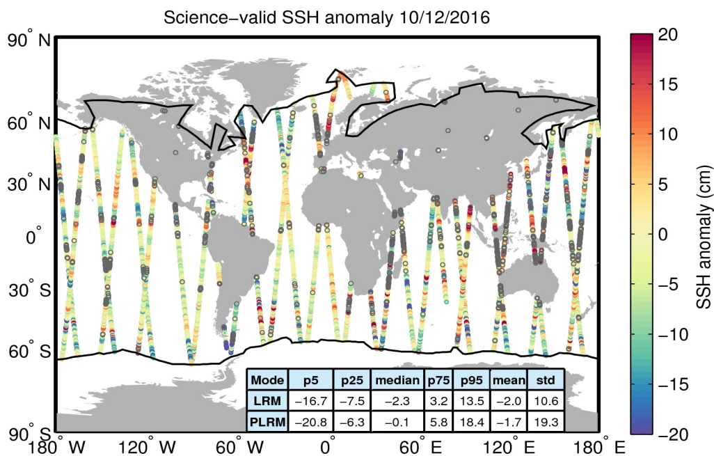
Figure 10. Geographical distribution of science-valid SSH anomaly data over oceans and lakes for 10/12/2016. The statistical values shown in the table refer to the SSH anomaly in cm and are calculated separately for LRM and PLRM regions. The black lines mark the outer limit of the Arctic and Antarctic polar polygons. Gray circles denote records that have been rejected based on the editing criteria described in Table 2.
