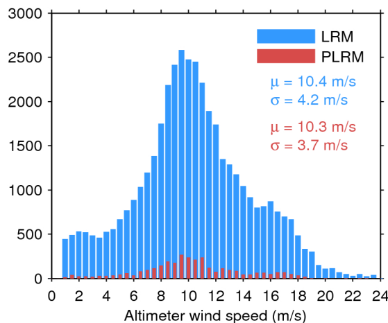
Figure 35. Histogram of science-valid wind over oceans and lakes for LRM (blue) and PLRM (red) for 10/12/2016. The mean ( \mu ) and standard deviation ( \sigma ) are also shown. Note that values larger than 24 m/s are excluded from the histogram for the sake of readability but not from the computation of \mu and \sigma .
