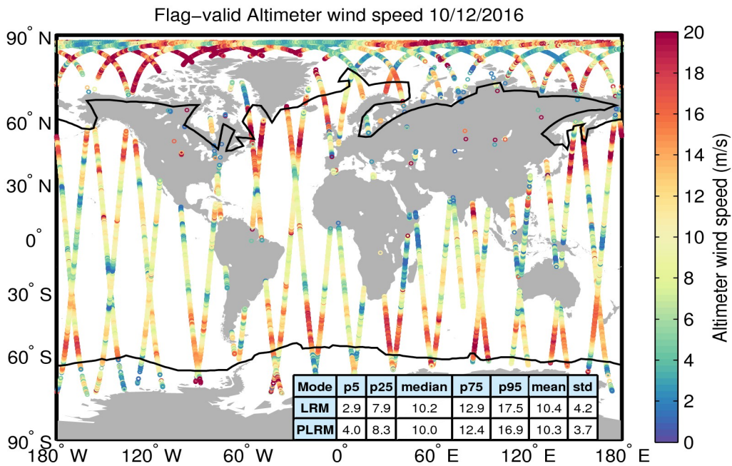
Figure 31. Geographical distribution of flag-valid wind data over oceans and lakes for 10/12/2016. The statistical values shown in the table refer to the wind in m/s and are calculated separately for LRM and PLRM regions. Measurements taken over polar polygons have been excluded from the computation of the statistical values. The black lines mark the outer limit of the Arctic and Antarctic polar polygons.
