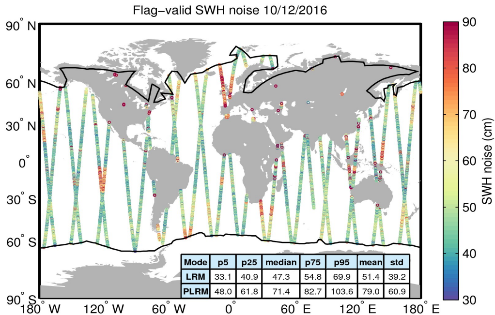
Figure 18. Geographical distribution of flag-valid 20-Hz SWH measurement noise over oceans and lakes for 10/12/2016. The statistical values shown in the table refer to the SWH noise and are calculated separately for LRM and PLRM regions. Measurements taken over polar polygons have been excluded from the computation of the statistical values. The black lines mark the outer limit of the Arctic and Antarctic polar polygons.
