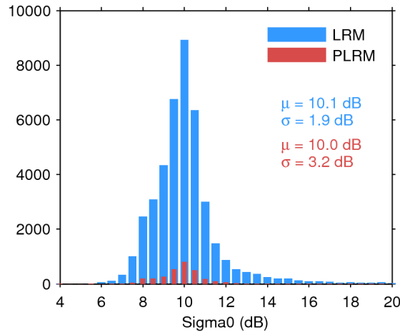
Figure 25. Histogram of flag-valid sigma0 over oceans and lakes for LRM (blue) and PLRM (red) for 10/12/2016. The mean ( \mu ) and standard deviation ( \sigma ) are also shown. Note that values outside [4 20] dB are excluded from the histogram for the sake of readability but not from the computation of \mu and \sigma .
