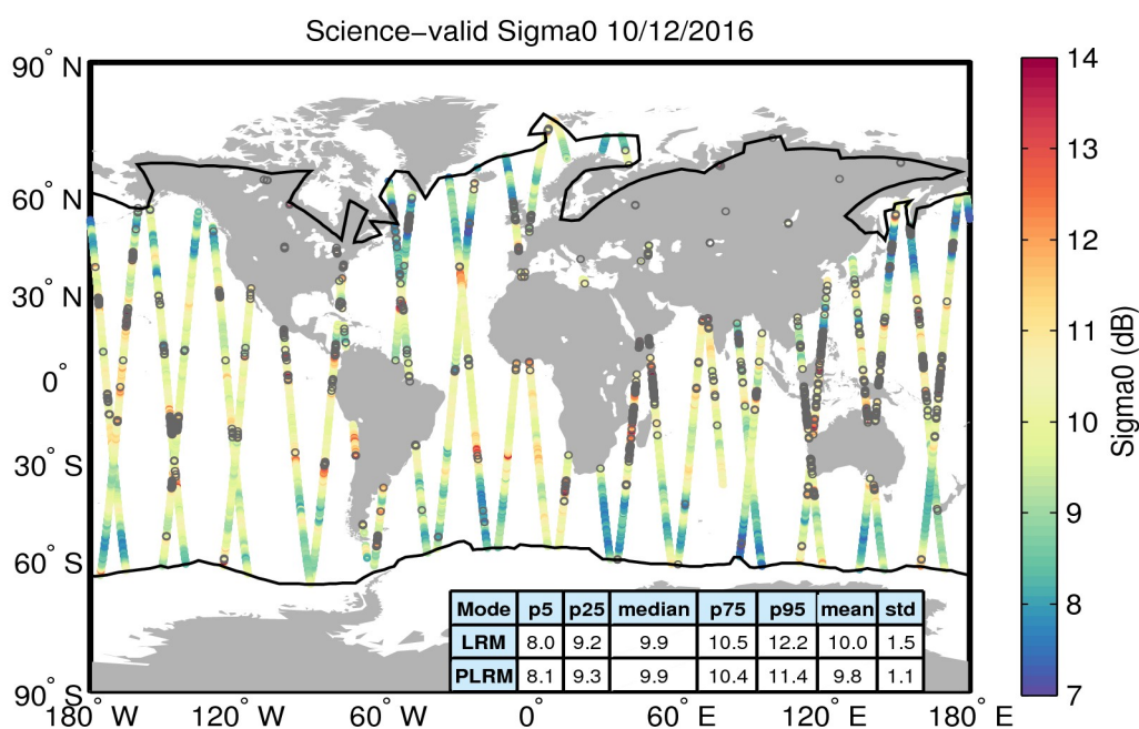
Figure 27. Geographical distribution of science-valid sigma0 data over oceans and lakes for 10/12/2016. The statistical values shown in the table refer to the sigma0 in dB and are calculated separately for LRM and PLRM regions. The black lines mark the outer limit of the Arctic and Antarctic polar polygons. Gray circles denote records that have been rejected based on the editing criteria described in Table 4.
