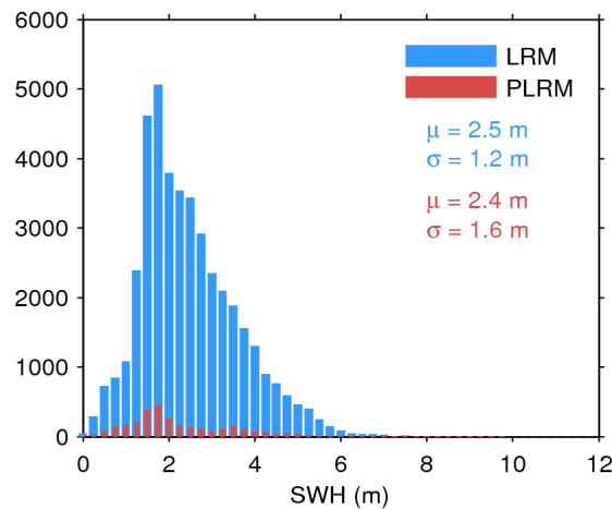
Figure 17. Histogram of flag-valid SWH over oceans and lakes for LRM (blue) and PLRM (red) for 10/12/2016. The mean ( \mu ) and standard deviation ( \sigma ) are also shown. Note that values larger than 12 m are excluded from the histogram for the sake of readability but not from the computation of \mu and \sigma .
