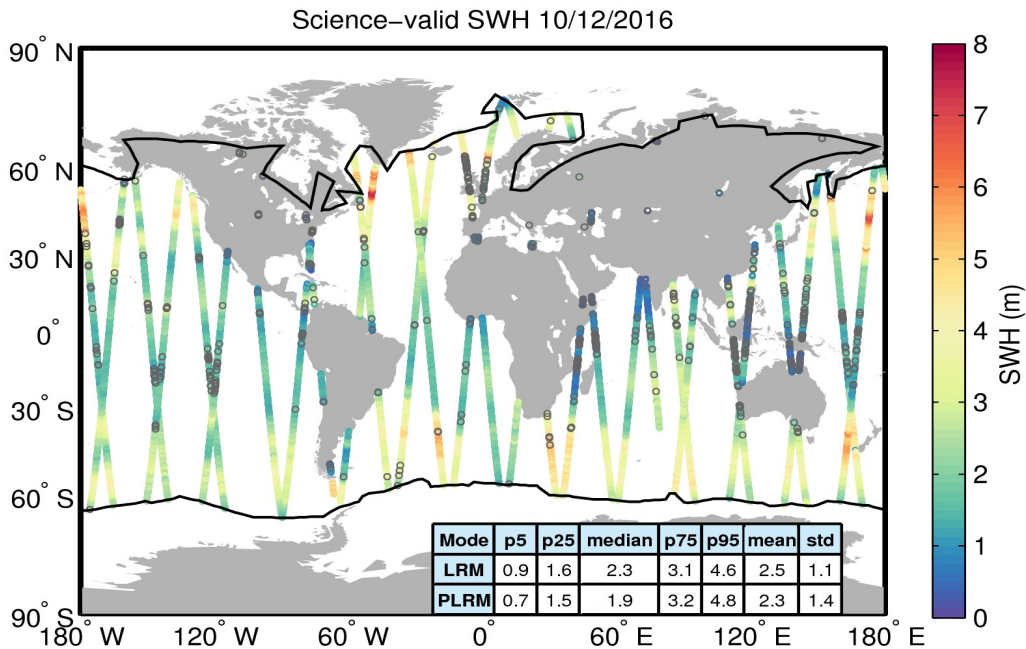
Figure 19. Geographical distribution of science-valid SWH data over oceans and lakes for 10/12/2016. The statistical values shown in the table refer to the SWH in m and are calculated separately for LRM and PLRM regions. The black lines mark the outer limit of the Arctic and Antarctic polar polygons. Gray circles denote records that have been rejected based on the editing criteria described in Table 3.
