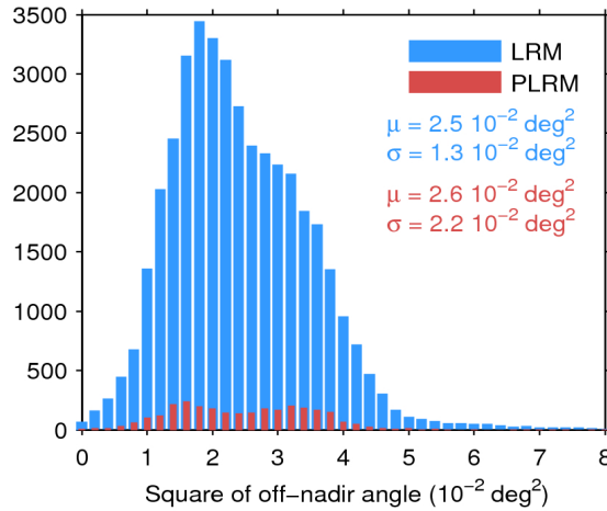
Figure 39. Histogram of flag-valid mispointing over oceans and lakes for LRM (blue) and PLRM (red) for 10/12/2016. Only positive values have been considered. The mean ( \mu ) and standard deviation ( \sigma ) are also shown. Note that values larger than 8 \cdot 10^{-2} \text{ deg}^2 are excluded from the histogram for the sake of readability but not from the computation of \mu and \sigma .
