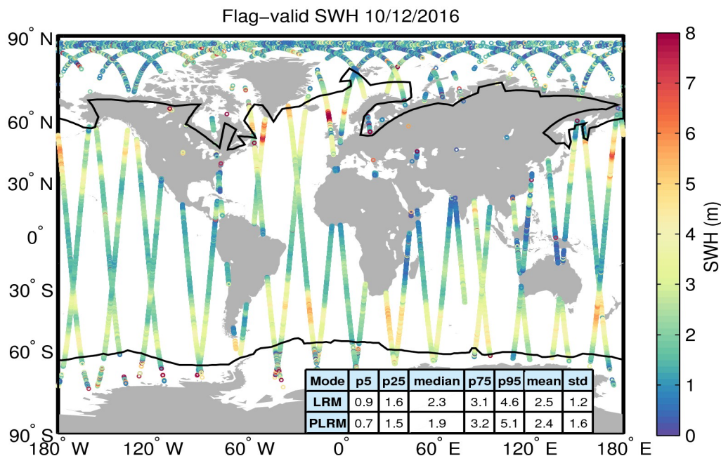
Figure 15. Geographical distribution of flag-valid SWH data over oceans and lakes for 10/12/2016. The statistical values shown in the table refer to the SWH in m and are calculated separately for LRM and PLRM regions. Measurements taken over polar polygons have been excluded from the computation of the statistical values. The black lines mark the outer limit of the Arctic and Antarctic polar polygons.
