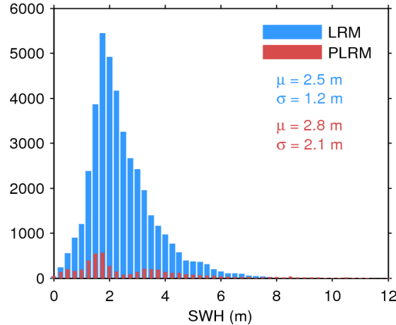
Figure 17. Histogram of flag-valid SWH over oceans and lakes for LRM (blue) and PLRM (red) for 09/12/2016. The mean ( \mu ) and standard deviation ( \sigma ) are also shown. Note that values larger than 12 m are excluded from the histogram for the sake of readability but not from the computation of \mu and \sigma .
