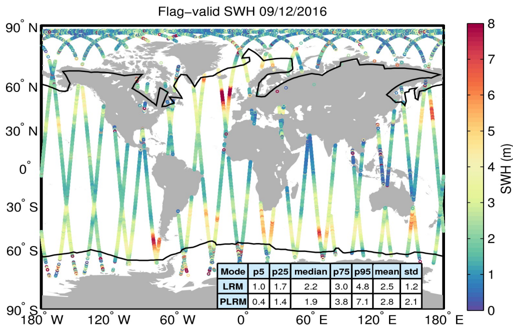
Figure 15. Geographical distribution of flag-valid SWH data over oceans and lakes for 09/12/2016. The statistical values shown in the table refer to the SWH in m and are calculated separately for LRM and PLRM regions. Measurements taken over polar polygons have been excluded from the computation of the statistical values. The black lines mark the outer limit of the Arctic and Antarctic polar polygons.
