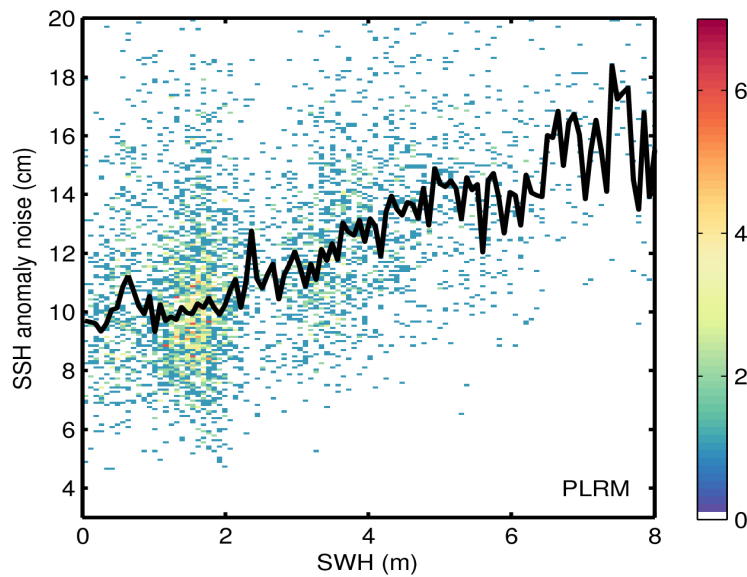
Figure 9. 2D histogram showing flag-valid SSH anomaly noise as a function of SWH for LRM (top) and PLRM (bottom) for 09/12/2016. The black line denotes the median SSH anomaly noise as a function of SWH.
