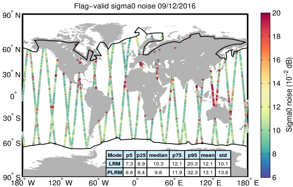
Figure 26. Geographical distribution of flag-valid 20-Hz sigma0 measurement noise over oceans and lakes for 09/12/2016. The statistical values shown in the table refer to the sigma0 noise and are calculated separately for LRM and PLRM regions. Measurements taken over polar polygons have been excluded from the computation of the statistical values. The black lines mark the outer limit of the Arctic and Antarctic polar polygons.
