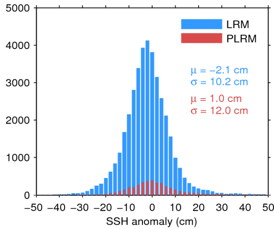
Figure 11. Histogram of science-valid SSH anomaly over oceans and lakes for LRM (blue) and PLRM (red) for 09/12/2016. The mean ( \mu ) and standard deviation ( \sigma ) are also shown. Note that values outside [-50 50] cm are excluded from the histogram for the sake of readability but not from the computation of \mu and \sigma .
