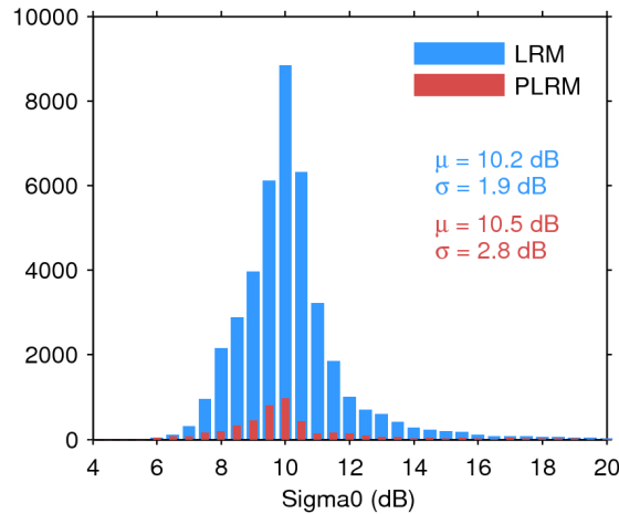
Figure 25. Histogram of flag-valid sigma0 over oceans and lakes for LRM (blue) and PLRM (red) for 09/12/2016. The mean ( \mu ) and standard deviation ( \sigma ) are also shown. Note that values outside [4 20] dB are excluded from the histogram for the sake of readability but not from the computation of \mu and \sigma .
