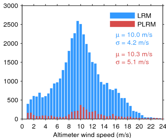
Figure 35. Histogram of science-valid wind over oceans and lakes for LRM (blue) and PLRM (red) for 09/12/2016. The mean ( \mu ) and standard deviation ( \sigma ) are also shown. Note that values larger than 24 m/s are excluded from the histogram for the sake of readability but not from the computation of \mu and \sigma .
