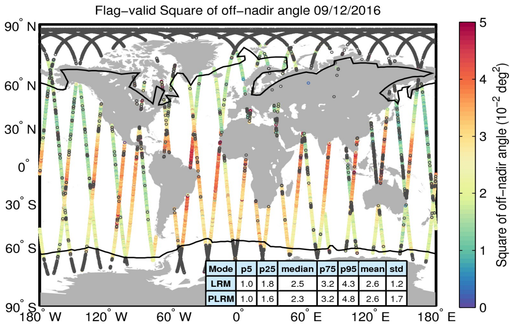
Figure 37. Geographical distribution of flag-valid mispointing data over oceans and lakes for 09/12/2016. The statistical values shown in the table refer to the mispointing in 10^{-2} deg 2 and are calculated separately for LRM and PLRM regions. Measurements taken over polar polygons have been excluded from the computation of the statistical values. The black lines mark the outer limit of the Arctic and Antarctic polar polygons. Gray circles denote negative values.
