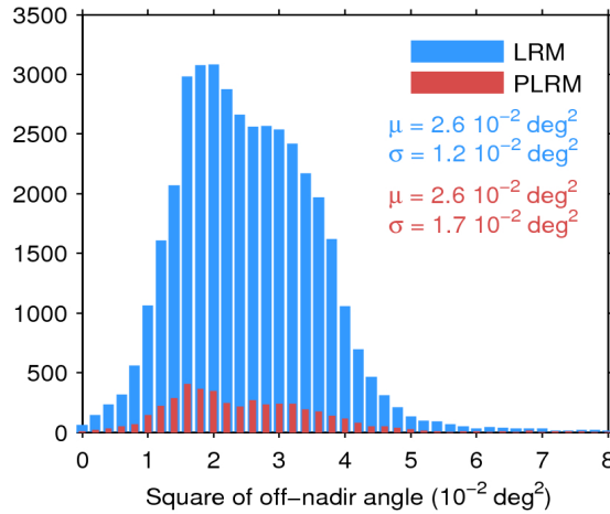
Figure 39. Histogram of flag-valid mispointing over oceans and lakes for LRM (blue) and PLRM (red) for 09/12/2016. Only positive values have been considered. The mean ( \mu ) and standard deviation ( \sigma ) are also shown. Note that values larger than 8 \cdot 10^{-2} \text{ deg}^2 are excluded from the histogram for the sake of readability but not from the computation of \mu and \sigma .
