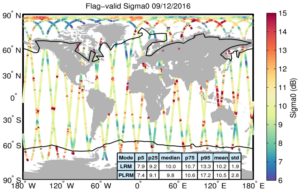
Figure 23. Geographical distribution of flag-valid sigma0 data over oceans and lakes for 09/12/2016. The statistical values shown in the table refer to the sigma0 in dB and are calculated separately for LRM and PLRM regions. Measurements taken over polar polygons have been excluded from the computation of the statistical values. The black lines mark the outer limit of the Arctic and Antarctic polar polygons.
