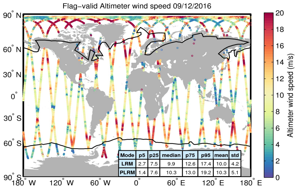
Figure 31. Geographical distribution of flag-valid wind data over oceans and lakes for 09/12/2016. The statistical values shown in the table refer to the wind in m/s and are calculated separately for LRM and PLRM regions. Measurements taken over polar polygons have been excluded from the computation of the statistical values. The black lines mark the outer limit of the Arctic and Antarctic polar polygons.
