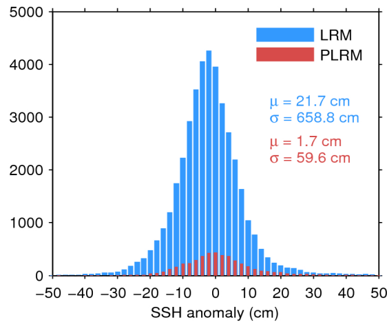
Figure 7. Histogram of flag-valid SSH anomaly over oceans and lakes for LRM (blue) and PLRM (red) for 09/12/2016. The mean ( \mu ) and standard deviation ( \sigma ) are also shown. Note that values outside [-50 50] cm are excluded from the histogram for the sake of readability but not from the computation of \mu and \sigma .
