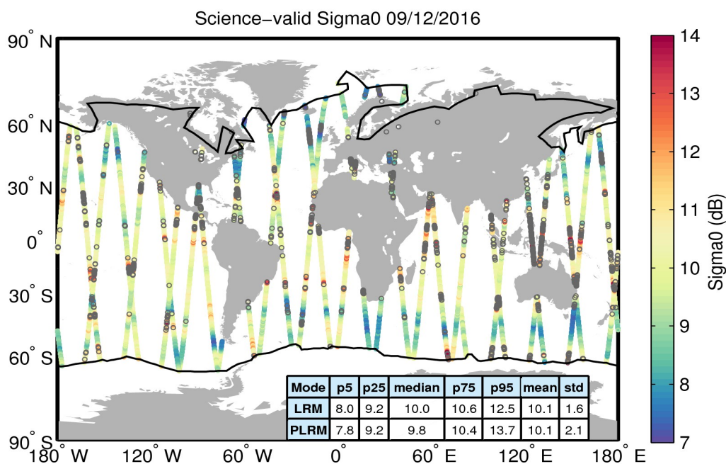
Figure 27. Geographical distribution of science-valid sigma0 data over oceans and lakes for 09/12/2016. The statistical values shown in the table refer to the sigma0 in dB and are calculated separately for LRM and PLRM regions. The black lines mark the outer limit of the Arctic and Antarctic polar polygons. Gray circles denote records that have been rejected based on the editing criteria described in Table 4.
