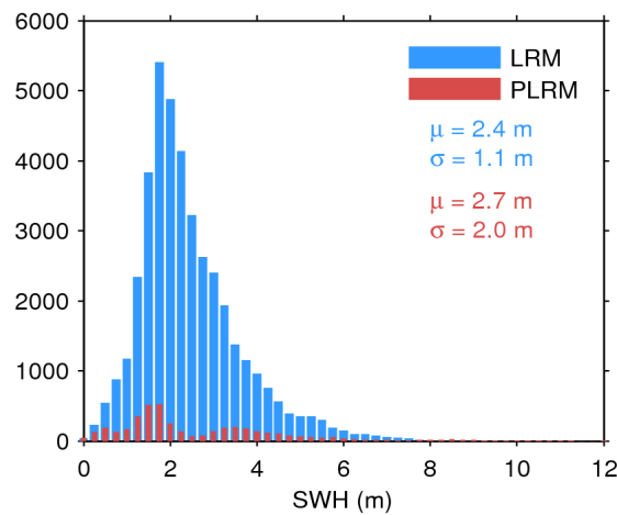
Figure 20. Histogram of science-valid SWH over oceans and lakes for LRM (blue) and PLRM (red) for 09/12/2016. The mean ( \mu ) and standard deviation ( \sigma ) are also shown. Note that values larger than 12 m are excluded from the histogram for the sake of readability but not from the computation of \mu and \sigma .
