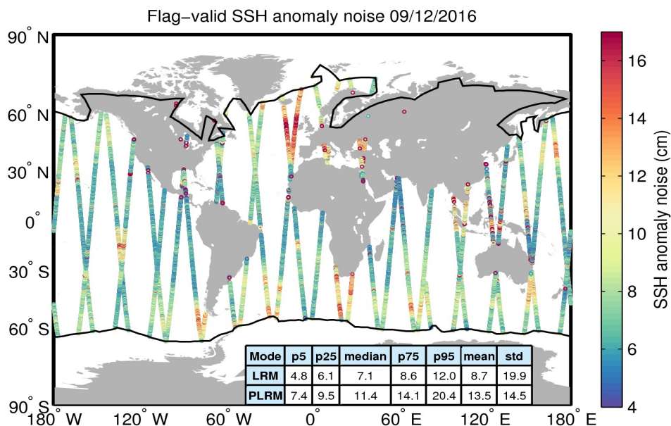
Figure 8. Geographical distribution of flag-valid 20-Hz SSH anomaly measurement noise over oceans and lakes for 09/12/2016. The statistical values shown in the table refer to the SSH anomaly noise and are calculated separately for LRM and PLRM regions. Measurements taken over polar polygons have been excluded from the computation of the statistical values. The black lines mark the outer limit of the Arctic and Antarctic polar polygons.
