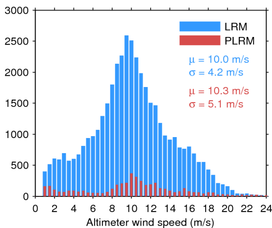
Figure 33. Histogram of flag-valid wind over oceans and lakes for LRM (blue) and PLRM (red) for 09/12/2016. The mean ( \mu ) and standard deviation ( \sigma ) are also shown. Note that values larger than 24 m/s are excluded from the histogram for the sake of readability but not from the computation of \mu and \sigma .
