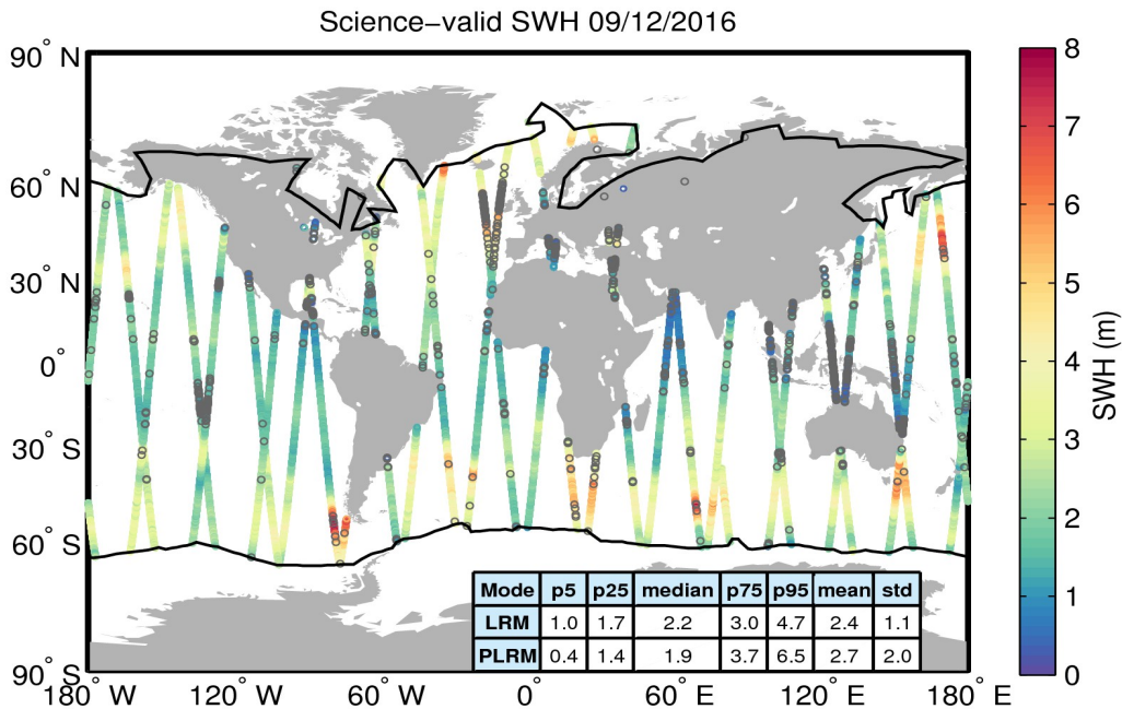
Figure 19. Geographical distribution of science-valid SWH data over oceans and lakes for 09/12/2016. The statistical values shown in the table refer to the SWH in m and are calculated separately for LRM and PLRM regions. The black lines mark the outer limit of the Arctic and Antarctic polar polygons. Gray circles denote records that have been rejected based on the editing criteria described in Table 3.
