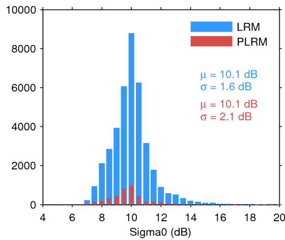
Figure 28. Histogram of science-valid sigma0 over oceans and lakes for LRM (blue) and PLRM (red) for 09/12/2016. The mean ( \mu ) and standard deviation ( \sigma ) are also shown. Note that values outside [4 20] dB are excluded from the histogram for the sake of readability but not from the computation of \mu and \sigma .
