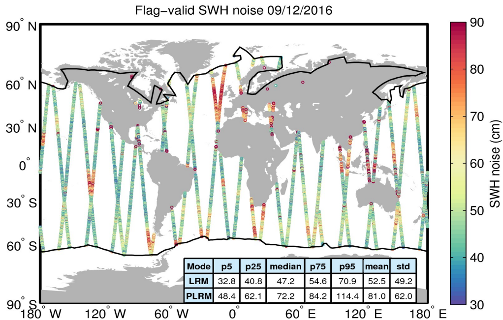
Figure 18. Geographical distribution of flag-valid 20-Hz SWH measurement noise over oceans and lakes for 09/12/2016. The statistical values shown in the table refer to the SWH noise and are calculated separately for LRM and PLRM regions. Measurements taken over polar polygons have been excluded from the computation of the statistical values. The black lines mark the outer limit of the Arctic and Antarctic polar polygons.
