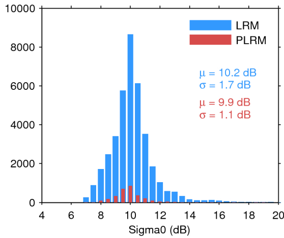
Figure 28. Histogram of science-valid sigma0 over oceans and lakes for LRM (blue) and PLRM (red) for 08/12/2016. The mean ( \mu ) and standard deviation ( \sigma ) are also shown. Note that values outside [4 20] dB are excluded from the histogram for the sake of readability but not from the computation of \mu and \sigma .
