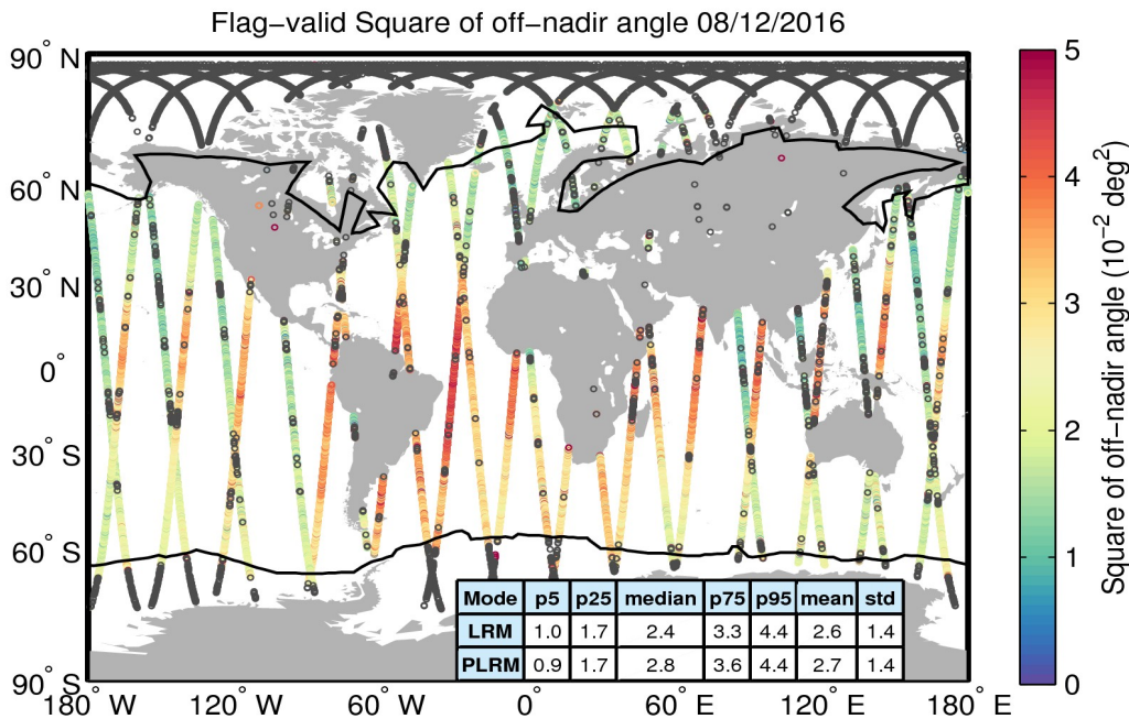
Figure 37. Geographical distribution of flag-valid mispointing data over oceans and lakes for 08/12/2016. The statistical values shown in the table refer to the mispointing in 10^{-2} deg 2 and are calculated separately for LRM and PLRM regions. Measurements taken over polar polygons have been excluded from the computation of the statistical values. The black lines mark the outer limit of the Arctic and Antarctic polar polygons. Gray circles denote negative values.
