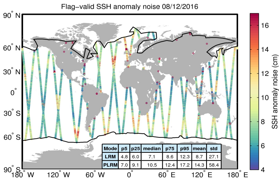
Figure 8. Geographical distribution of flag-valid 20-Hz SSH anomaly measurement noise over oceans and lakes for 08/12/2016. The statistical values shown in the table refer to the SSH anomaly noise and are calculated separately for LRM and PLRM regions. Measurements taken over polar polygons have been excluded from the computation of the statistical values. The black lines mark the outer limit of the Arctic and Antarctic polar polygons.
