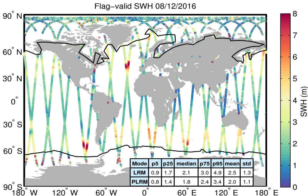
Figure 15. Geographical distribution of flag-valid SWH data over oceans and lakes for 08/12/2016. The statistical values shown in the table refer to the SWH in m and are calculated separately for LRM and PLRM regions. Measurements taken over polar polygons have been excluded from the computation of the statistical values. The black lines mark the outer limit of the Arctic and Antarctic polar polygons.
