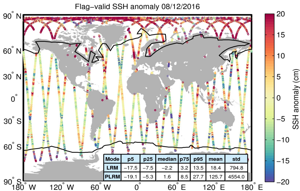
Figure 5. Geographical distribution of flag-valid 1-Hz SSH anomaly data over oceans and lakes for 08/12/2016. The statistical values shown in the table refer to the SSH anomaly in cm and are calculated separately for LRM and PLRM regions. Measurements taken over polar polygons have been excluded from the computation of the statistical values. The black lines mark the outer limit of the Arctic and Antarctic polar polygons.
