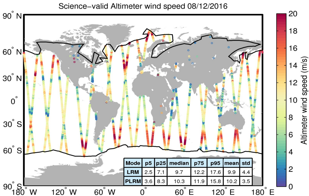
Figure 34. Geographical distribution of science-valid wind data over oceans and lakes for 08/12/2016. The statistical values shown in the table refer to the wind in m/s and are calculated separately for LRM and PLRM regions. The black lines mark the outer limit of the Arctic and Antarctic polar polygons. Gray circles denote records that have been rejected based on the editing criteria described in Table 5.
