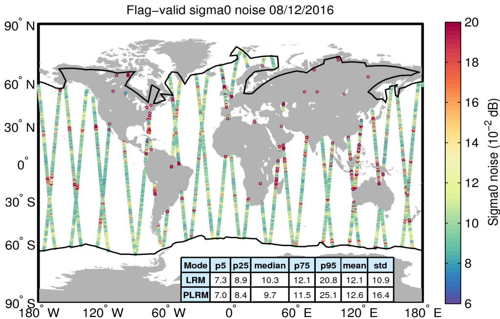
Figure 26. Geographical distribution of flag-valid 20-Hz sigma0 measurement noise over oceans and lakes for 08/12/2016. The statistical values shown in the table refer to the sigma0 noise and are calculated separately for LRM and PLRM regions. Measurements taken over polar polygons have been excluded from the computation of the statistical values. The black lines mark the outer limit of the Arctic and Antarctic polar polygons.
