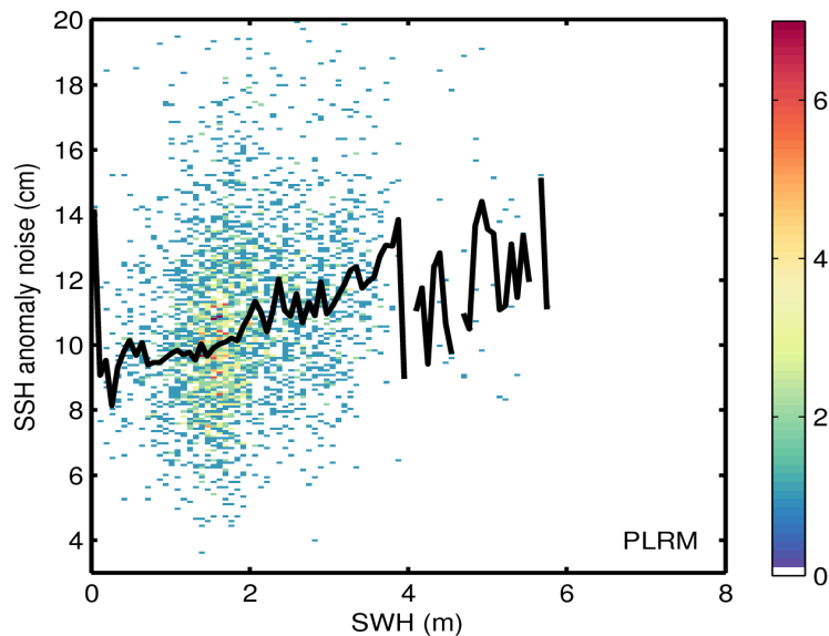
Figure 9. 2D histogram showing flag-valid SSH anomaly noise as a function of SWH for LRM (top) and PLRM (bottom) for 08/12/2016. The black line denotes the median SSH anomaly noise as a function of SWH.
