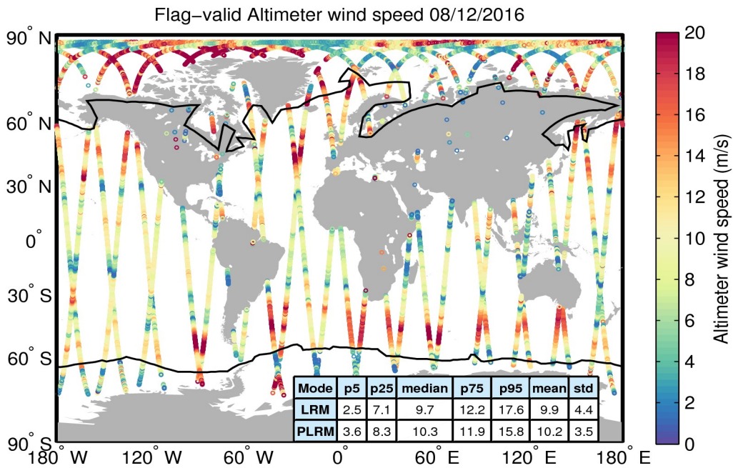
Figure 31. Geographical distribution of flag-valid wind data over oceans and lakes for 08/12/2016. The statistical values shown in the table refer to the wind in m/s and are calculated separately for LRM and PLRM regions. Measurements taken over polar polygons have been excluded from the computation of the statistical values. The black lines mark the outer limit of the Arctic and Antarctic polar polygons.
