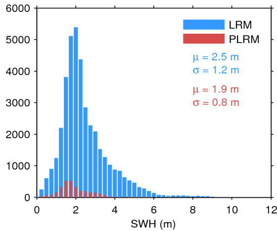
Figure 20. Histogram of science-valid SWH over oceans and lakes for LRM (blue) and PLRM (red) for 08/12/2016. The mean ( \mu ) and standard deviation ( \sigma ) are also shown. Note that values larger than 12 m are excluded from the histogram for the sake of readability but not from the computation of \mu and \sigma .
