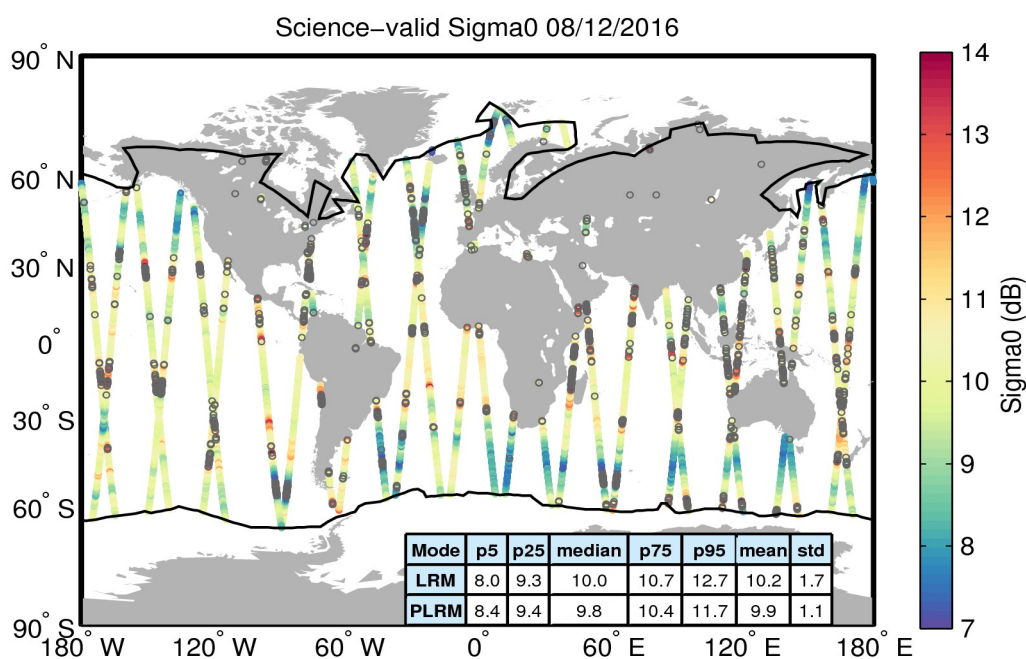
Figure 27. Geographical distribution of science-valid sigma0 data over oceans and lakes for 08/12/2016. The statistical values shown in the table refer to the sigma0 in dB and are calculated separately for LRM and PLRM regions. The black lines mark the outer limit of the Arctic and Antarctic polar polygons. Gray circles denote records that have been rejected based on the editing criteria described in Table 4.
