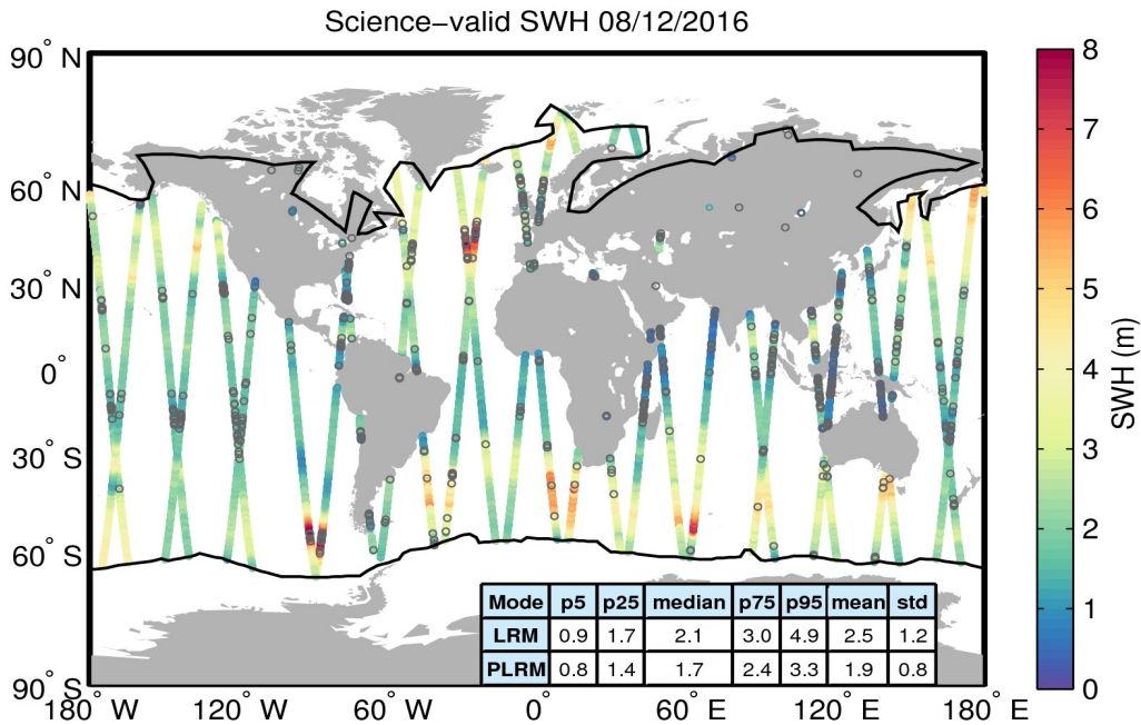
Figure 19. Geographical distribution of science-valid SWH data over oceans and lakes for 08/12/2016. The statistical values shown in the table refer to the SWH in m and are calculated separately for LRM and PLRM regions. The black lines mark the outer limit of the Arctic and Antarctic polar polygons. Gray circles denote records that have been rejected based on the editing criteria described in Table 3.
