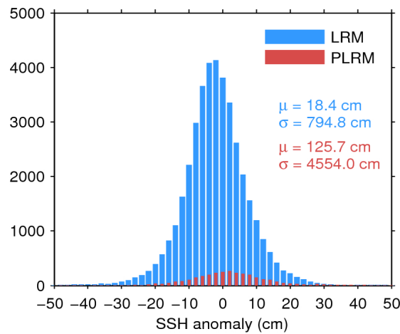
Figure 7. Histogram of flag-valid SSH anomaly over oceans and lakes for LRM (blue) and PLRM (red) for 08/12/2016. The mean ( \mu ) and standard deviation ( \sigma ) are also shown. Note that values outside [-50\ 50] cm are excluded from the histogram for the sake of readability but not from the computation of \mu and \sigma .
