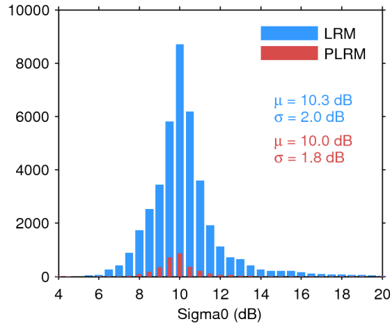
Figure 25. Histogram of flag-valid sigma0 over oceans and lakes for LRM (blue) and PLRM (red) for 08/12/2016. The mean ( \mu ) and standard deviation ( \sigma ) are also shown. Note that values outside [4 20] dB are excluded from the histogram for the sake of readability but not from the computation of \mu and \sigma .
