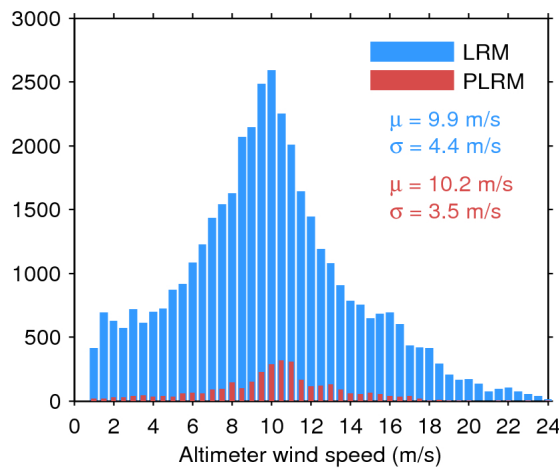
Figure 33. Histogram of flag-valid wind over oceans and lakes for LRM (blue) and PLRM (red) for 08/12/2016. The mean ( \mu ) and standard deviation ( \sigma ) are also shown. Note that values larger than 24 m/s are excluded from the histogram for the sake of readability but not from the computation of \mu and \sigma .
