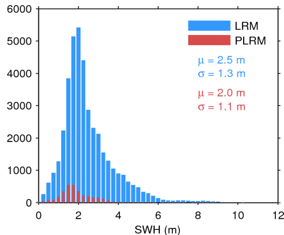
Figure 17. Histogram of flag-valid SWH over oceans and lakes for LRM (blue) and PLRM (red) for 08/12/2016. The mean ( \mu ) and standard deviation ( \sigma ) are also shown. Note that values larger than 12 m are excluded from the histogram for the sake of readability but not from the computation of \mu and \sigma .
