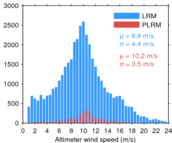
Figure 35. Histogram of science-valid wind over oceans and lakes for LRM (blue) and PLRM (red) for 08/12/2016. The mean ( \mu ) and standard deviation ( \sigma ) are also shown. Note that values larger than 24 m/s are excluded from the histogram for the sake of readability but not from the computation of \mu and \sigma .
