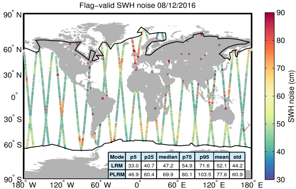
Figure 18. Geographical distribution of flag-valid 20-Hz SWH measurement noise over oceans and lakes for 08/12/2016. The statistical values shown in the table refer to the SWH noise and are calculated separately for LRM and PLRM regions. Measurements taken over polar polygons have been excluded from the computation of the statistical values. The black lines mark the outer limit of the Arctic and Antarctic polar polygons.
