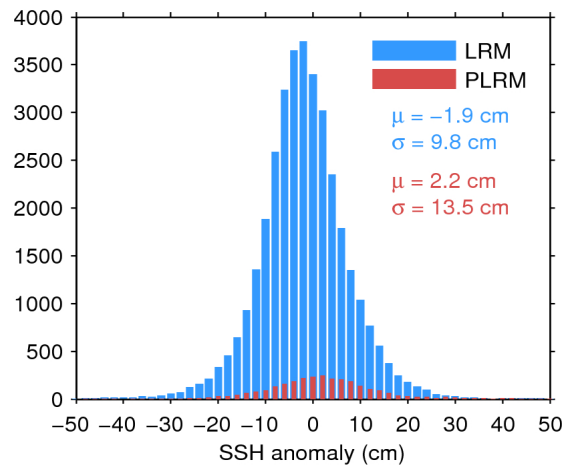
Figure 11. Histogram of science-valid SSH anomaly over oceans and lakes for LRM (blue) and PLRM (red) for 08/12/2016. The mean ( \mu ) and standard deviation ( \sigma ) are also shown. Note that values outside [-50\ 50] cm are excluded from the histogram for the sake of readability but not from the computation of \mu and \sigma .
