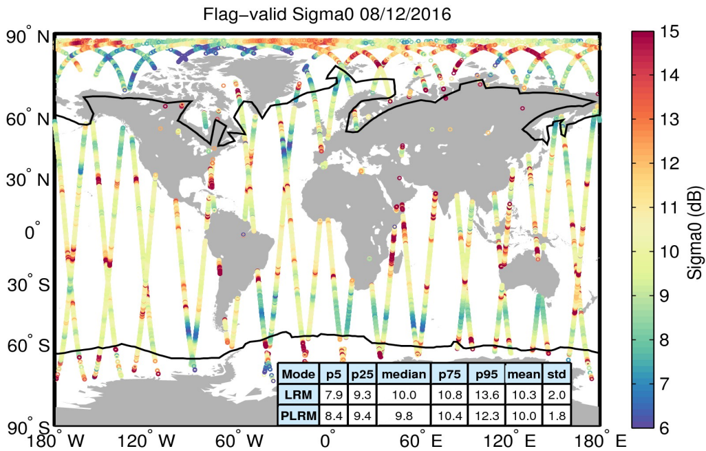
Figure 23. Geographical distribution of flag-valid sigma0 data over oceans and lakes for 08/12/2016. The statistical values shown in the table refer to the sigma0 in dB and are calculated separately for LRM and PLRM regions. Measurements taken over polar polygons have been excluded from the computation of the statistical values. The black lines mark the outer limit of the Arctic and Antarctic polar polygons.
