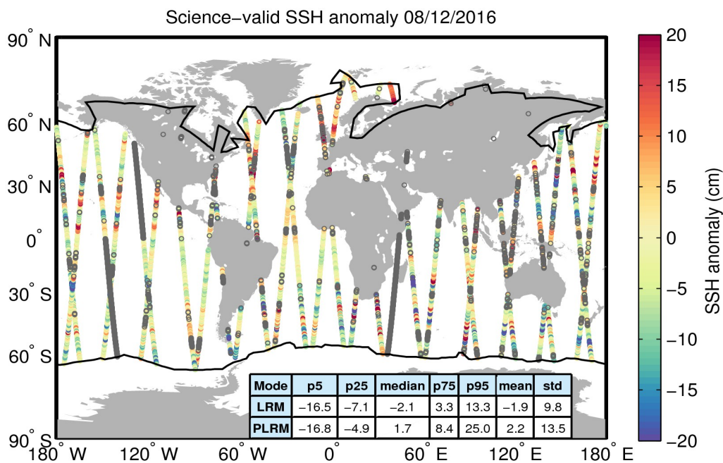
Figure 10. Geographical distribution of science-valid SSH anomaly data over oceans and lakes for 08/12/2016. The statistical values shown in the table refer to the SSH anomaly in cm and are calculated separately for LRM and PLRM regions. The black lines mark the outer limit of the Arctic and Antarctic polar polygons. Gray circles denote records that have been rejected based on the editing criteria described in Table 2.
