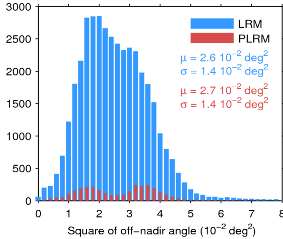
Figure 39. Histogram of flag-valid mispointing over oceans and lakes for LRM (blue) and PLRM (red) for 08/12/2016. Only positive values have been considered. The mean ( \mu ) and standard deviation ( \sigma ) are also shown. Note that values larger than 8 \cdot 10^{-2} \text{ deg}^2 are excluded from the histogram for the sake of readability but not from the computation of \mu and \sigma .
