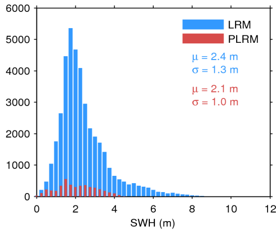
Figure 20. Histogram of science-valid SWH over oceans and lakes for LRM (blue) and PLRM (red) for 07/12/2016. The mean ( \mu ) and standard deviation ( \sigma ) are also shown. Note that values larger than 12 m are excluded from the histogram for the sake of readability but not from the computation of \mu and \sigma .
