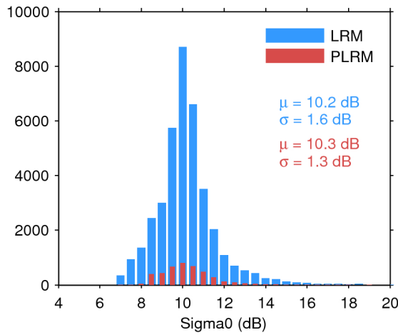
Figure 28. Histogram of science-valid sigma0 over oceans and lakes for LRM (blue) and PLRM (red) for 07/12/2016. The mean ( \mu ) and standard deviation ( \sigma ) are also shown. Note that values outside [4 20] dB are excluded from the histogram for the sake of readability but not from the computation of \mu and \sigma .
