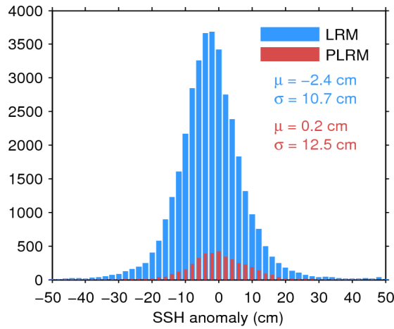
Figure 11. Histogram of science-valid SSH anomaly over oceans and lakes for LRM (blue) and PLRM (red) for 07/12/2016. The mean ( \mu ) and standard deviation ( \sigma ) are also shown. Note that values outside [-50\ 50] cm are excluded from the histogram for the sake of readability but not from the computation of \mu and \sigma .
