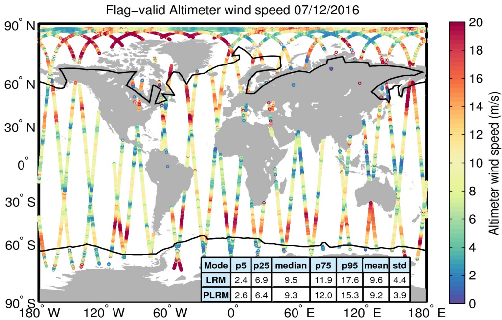
Figure 31. Geographical distribution of flag-valid wind data over oceans and lakes for 07/12/2016. The statistical values shown in the table refer to the wind in m/s and are calculated separately for LRM and PLRM regions. Measurements taken over polar polygons have been excluded from the computation of the statistical values. The black lines mark the outer limit of the Arctic and Antarctic polar polygons.
