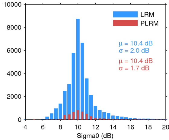
Figure 25. Histogram of flag-valid sigma0 over oceans and lakes for LRM (blue) and PLRM (red) for 07/12/2016. The mean ( \mu ) and standard deviation ( \sigma ) are also shown. Note that values outside [4 20] dB are excluded from the histogram for the sake of readability but not from the computation of \mu and \sigma .
