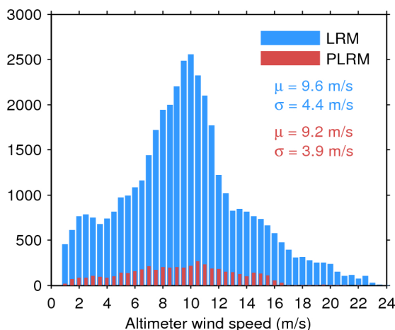
Figure 33. Histogram of flag-valid wind over oceans and lakes for LRM (blue) and PLRM (red) for 07/12/2016. The mean ( \mu ) and standard deviation ( \sigma ) are also shown. Note that values larger than 24 m/s are excluded from the histogram for the sake of readability but not from the computation of \mu and \sigma .
