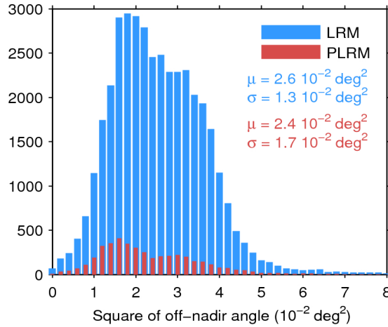
Figure 39. Histogram of flag-valid mispointing over oceans and lakes for LRM (blue) and PLRM (red) for 07/12/2016. Only positive values have been considered. The mean ( \mu ) and standard deviation ( \sigma ) are also shown. Note that values larger than 8 \cdot 10^{-2} \text{ deg}^2 are excluded from the histogram for the sake of readability but not from the computation of \mu and \sigma .
