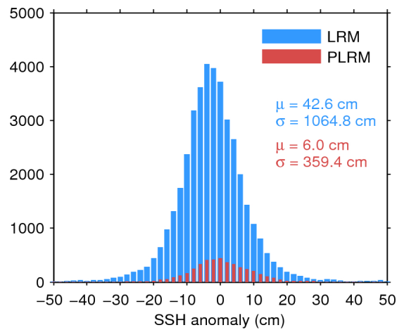
Figure 7. Histogram of flag-valid SSH anomaly over oceans and lakes for LRM (blue) and PLRM (red) for 07/12/2016. The mean ( \mu ) and standard deviation ( \sigma ) are also shown. Note that values outside [-50\ 50] cm are excluded from the histogram for the sake of readability but not from the computation of \mu and \sigma .
