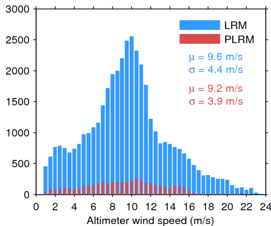
Figure 35. Histogram of science-valid wind over oceans and lakes for LRM (blue) and PLRM (red) for 07/12/2016. The mean ( \mu ) and standard deviation ( \sigma ) are also shown. Note that values larger than 24 m/s are excluded from the histogram for the sake of readability but not from the computation of \mu and \sigma .
