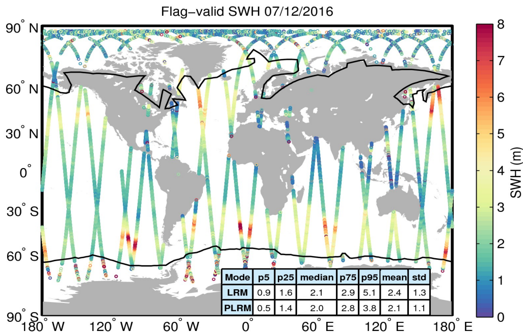
Figure 15. Geographical distribution of flag-valid SWH data over oceans and lakes for 07/12/2016. The statistical values shown in the table refer to the SWH in m and are calculated separately for LRM and PLRM regions. Measurements taken over polar polygons have been excluded from the computation of the statistical values. The black lines mark the outer limit of the Arctic and Antarctic polar polygons.
