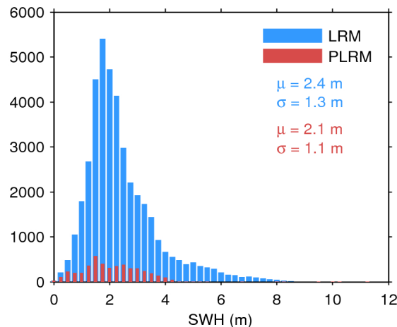
Figure 17. Histogram of flag-valid SWH over oceans and lakes for LRM (blue) and PLRM (red) for 07/12/2016. The mean ( \mu ) and standard deviation ( \sigma ) are also shown. Note that values larger than 12 m are excluded from the histogram for the sake of readability but not from the computation of \mu and \sigma .
