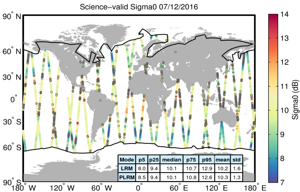
Figure 27. Geographical distribution of science-valid sigma0 data over oceans and lakes for 07/12/2016. The statistical values shown in the table refer to the sigma0 in dB and are calculated separately for LRM and PLRM regions. The black lines mark the outer limit of the Arctic and Antarctic polar polygons. Gray circles denote records that have been rejected based on the editing criteria described in Table 4.
