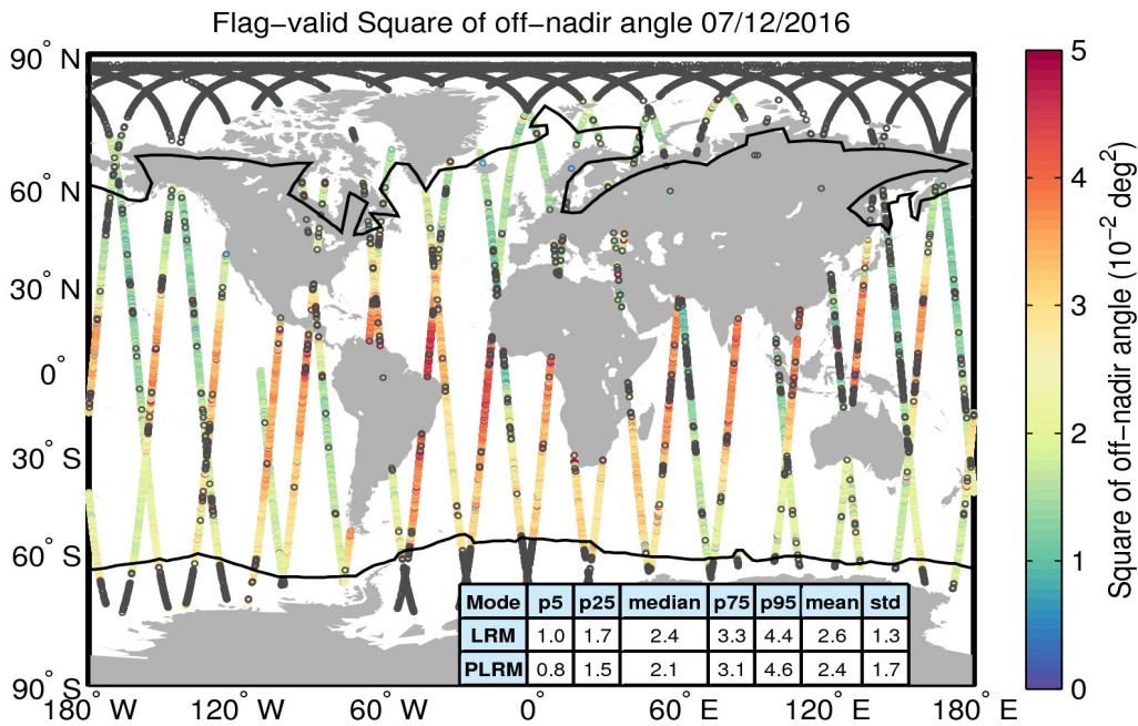
Figure 37. Geographical distribution of flag-valid mispointing data over oceans and lakes for 07/12/2016. The statistical values shown in the table refer to the mispointing in 10^{-2} \text{deg}^2 and are calculated separately for LRM and PLRM regions. Measurements taken over polar polygons have been excluded from the computation of the statistical values. The black lines mark the outer limit of the Arctic and Antarctic polar polygons. Gray circles denote negative values.
