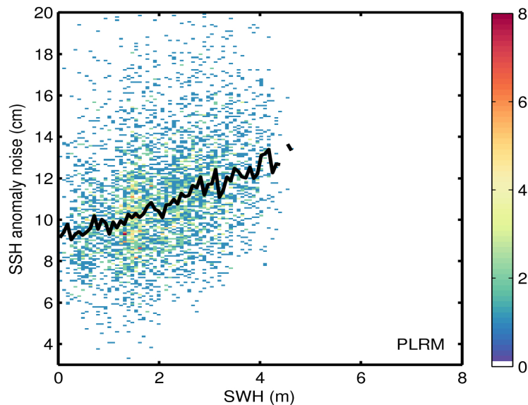
Figure 9. 2D histogram showing flag-valid SSH anomaly noise as a function of SWH for LRM (top) and PLRM (bottom) for 07/12/2016. The black line denotes the median SSH anomaly noise as a function of SWH.
