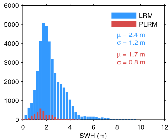
Figure 20. Histogram of science-valid SWH over oceans and lakes for LRM (blue) and PLRM (red) for 06/12/2016. The mean ( \mu ) and standard deviation ( \sigma ) are also shown. Note that values larger than 12 m are excluded from the histogram for the sake of readability but not from the computation of \mu and \sigma .
