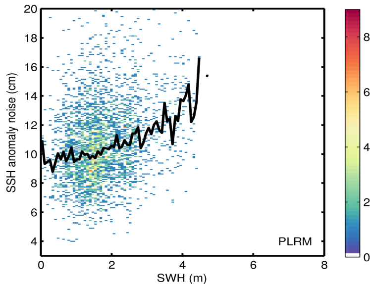
Figure 9. 2D histogram showing flag-valid SSH anomaly noise as a function of SWH for LRM (top) and PLRM (bottom) for 06/12/2016. The black line denotes the median SSH anomaly noise as a function of SWH.
