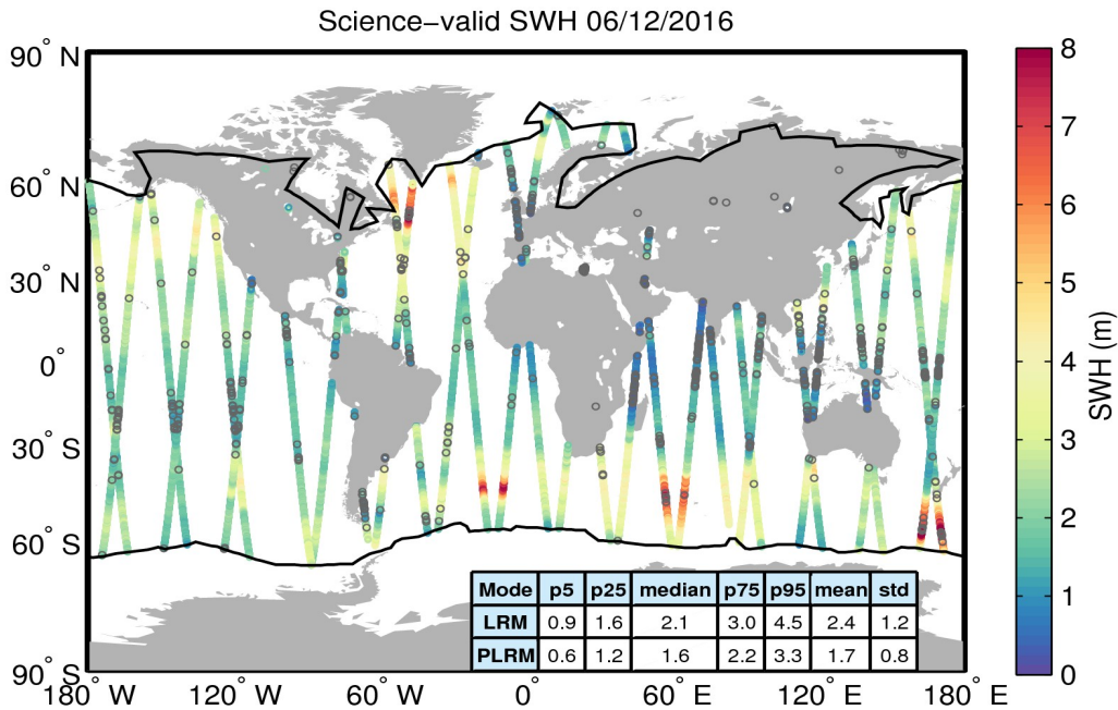
Figure 19. Geographical distribution of science-valid SWH data over oceans and lakes for 06/12/2016. The statistical values shown in the table refer to the SWH in m and are calculated separately for LRM and PLRM regions. The black lines mark the outer limit of the Arctic and Antarctic polar polygons. Gray circles denote records that have been rejected based on the editing criteria described in Table 3.
