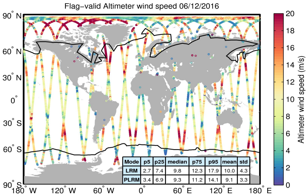
Figure 31. Geographical distribution of flag-valid wind data over oceans and lakes for 06/12/2016. The statistical values shown in the table refer to the wind in m/s and are calculated separately for LRM and PLRM regions. Measurements taken over polar polygons have been excluded from the computation of the statistical values. The black lines mark the outer limit of the Arctic and Antarctic polar polygons.
