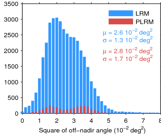
Figure 39. Histogram of flag-valid mispointing over oceans and lakes for LRM (blue) and PLRM (red) for 06/12/2016. Only positive values have been considered. The mean ( \mu ) and standard deviation ( \sigma ) are also shown. Note that values larger than 8 \cdot 10^{-2} \text{ deg}^2 are excluded from the histogram for the sake of readability but not from the computation of \mu and \sigma .
