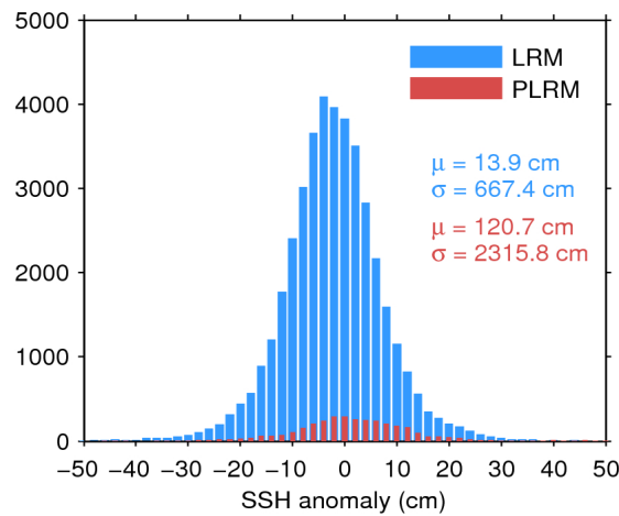
Figure 7. Histogram of flag-valid SSH anomaly over oceans and lakes for LRM (blue) and PLRM (red) for 06/12/2016. The mean ( \mu ) and standard deviation ( \sigma ) are also shown. Note that values outside [-50\ 50] cm are excluded from the histogram for the sake of readability but not from the computation of \mu and \sigma .
