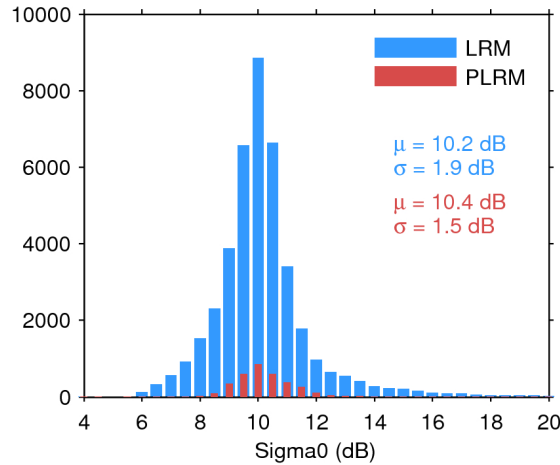
Figure 25. Histogram of flag-valid sigma0 over oceans and lakes for LRM (blue) and PLRM (red) for 06/12/2016. The mean ( \mu ) and standard deviation ( \sigma ) are also shown. Note that values outside [4 20] dB are excluded from the histogram for the sake of readability but not from the computation of \mu and \sigma .
