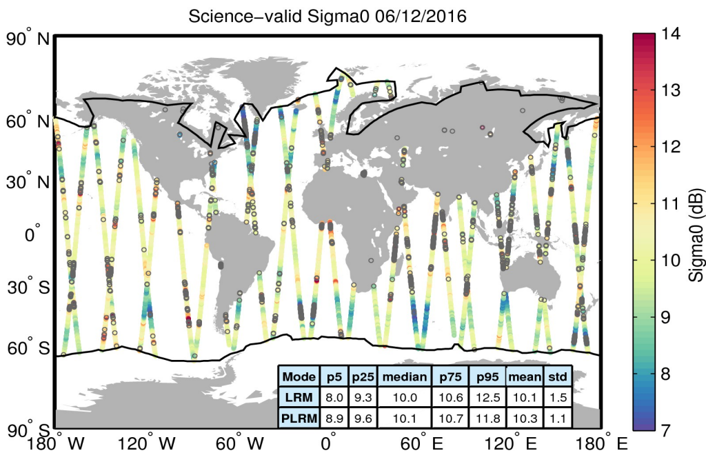
Figure 27. Geographical distribution of science-valid sigma0 data over oceans and lakes for 06/12/2016. The statistical values shown in the table refer to the sigma0 in dB and are calculated separately for LRM and PLRM regions. The black lines mark the outer limit of the Arctic and Antarctic polar polygons. Gray circles denote records that have been rejected based on the editing criteria described in Table 4.
