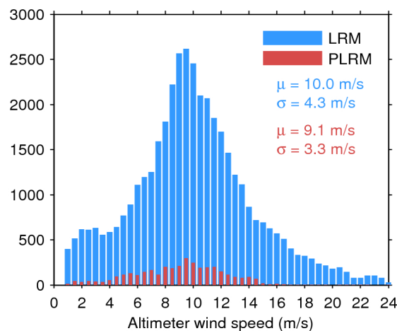
Figure 35. Histogram of science-valid wind over oceans and lakes for LRM (blue) and PLRM (red) for 06/12/2016. The mean ( \mu ) and standard deviation ( \sigma ) are also shown. Note that values larger than 24 m/s are excluded from the histogram for the sake of readability but not from the computation of \mu and \sigma .
