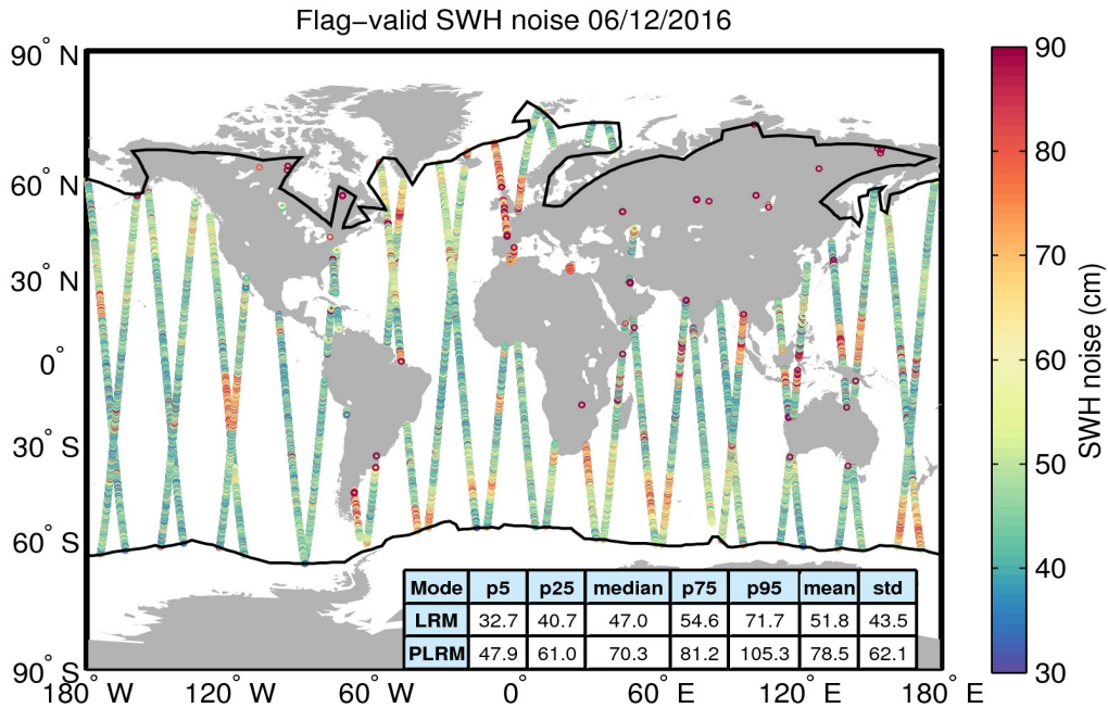
Figure 18. Geographical distribution of flag-valid 20-Hz SWH measurement noise over oceans and lakes for 06/12/2016. The statistical values shown in the table refer to the SWH noise and are calculated separately for LRM and PLRM regions. Measurements taken over polar polygons have been excluded from the computation of the statistical values. The black lines mark the outer limit of the Arctic and Antarctic polar polygons.
