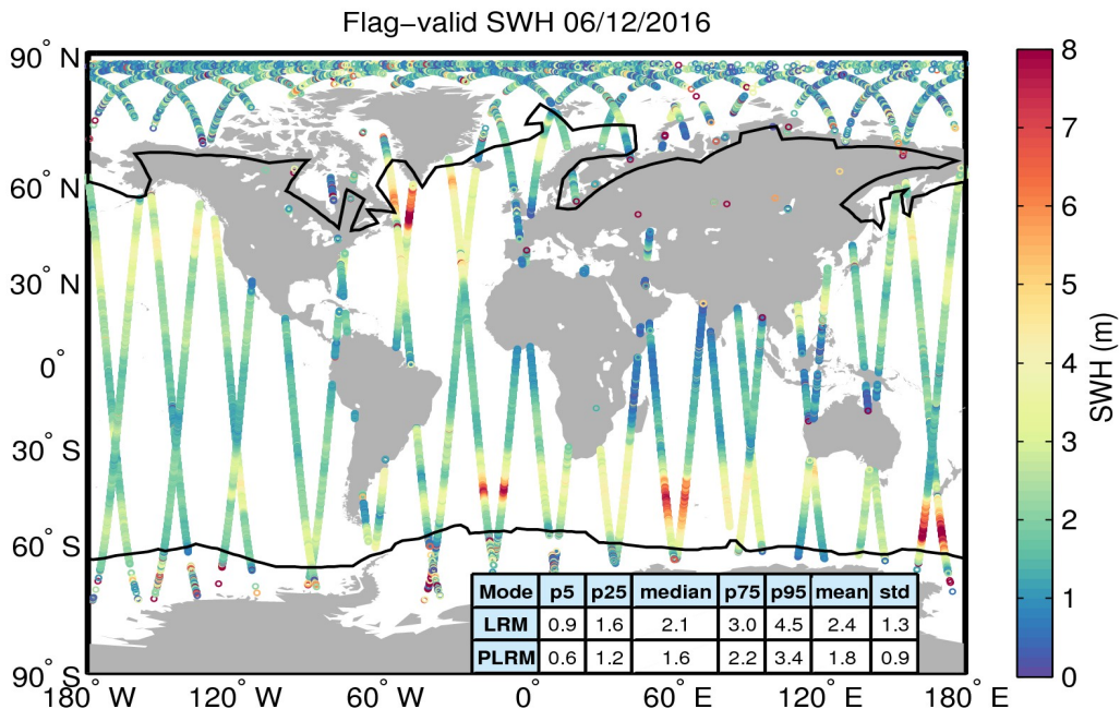
Figure 15. Geographical distribution of flag-valid SWH data over oceans and lakes for 06/12/2016. The statistical values shown in the table refer to the SWH in m and are calculated separately for LRM and PLRM regions. Measurements taken over polar polygons have been excluded from the computation of the statistical values. The black lines mark the outer limit of the Arctic and Antarctic polar polygons.
