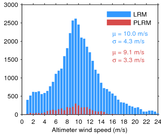
Figure 33. Histogram of flag-valid wind over oceans and lakes for LRM (blue) and PLRM (red) for 06/12/2016. The mean ( \mu ) and standard deviation ( \sigma ) are also shown. Note that values larger than 24 m/s are excluded from the histogram for the sake of readability but not from the computation of \mu and \sigma .
