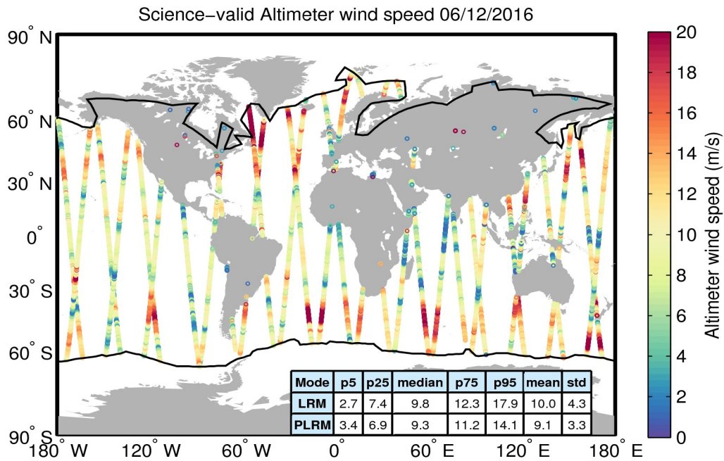
Figure 34. Geographical distribution of science-valid wind data over oceans and lakes for 06/12/2016. The statistical values shown in the table refer to the wind in m/s and are calculated separately for LRM and PLRM regions. The black lines mark the outer limit of the Arctic and Antarctic polar polygons. Gray circles denote records that have been rejected based on the editing criteria described in Table 5.
