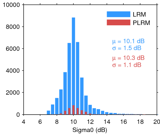
Figure 28. Histogram of science-valid sigma0 over oceans and lakes for LRM (blue) and PLRM (red) for 06/12/2016. The mean ( \mu ) and standard deviation ( \sigma ) are also shown. Note that values outside [4 20] dB are excluded from the histogram for the sake of readability but not from the computation of \mu and \sigma .
