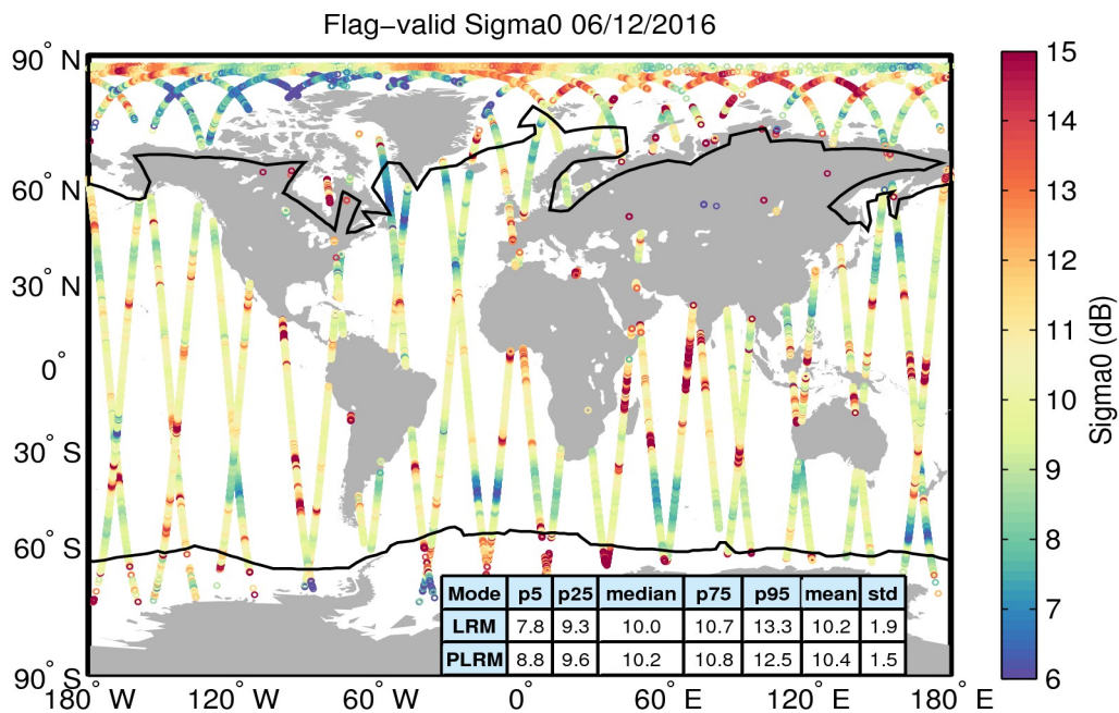
Figure 23. Geographical distribution of flag-valid sigma0 data over oceans and lakes for 06/12/2016. The statistical values shown in the table refer to the sigma0 in dB and are calculated separately for LRM and PLRM regions. Measurements taken over polar polygons have been excluded from the computation of the statistical values. The black lines mark the outer limit of the Arctic and Antarctic polar polygons.
