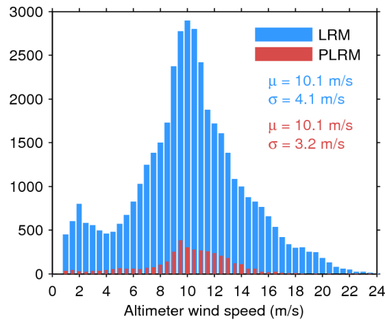
Figure 33. Histogram of flag-valid wind over oceans and lakes for LRM (blue) and PLRM (red) for 04/12/2016. The mean ( \mu ) and standard deviation ( \sigma ) are also shown. Note that values larger than 24 m/s are excluded from the histogram for the sake of readability but not from the computation of \mu and \sigma .
