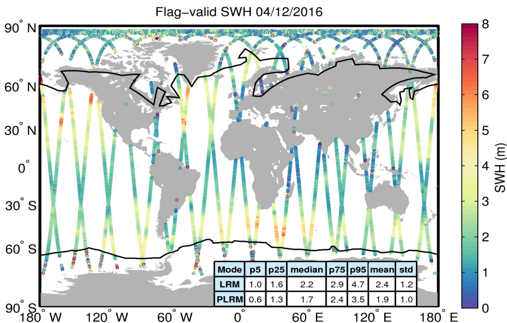
Figure 15. Geographical distribution of flag-valid SWH data over oceans and lakes for 04/12/2016. The statistical values shown in the table refer to the SWH in m and are calculated separately for LRM and PLRM regions. Measurements taken over polar polygons have been excluded from the computation of the statistical values. The black lines mark the outer limit of the Arctic and Antarctic polar polygons.
