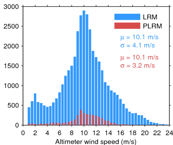
Figure 35. Histogram of science-valid wind over oceans and lakes for LRM (blue) and PLRM (red) for 04/12/2016. The mean ( \mu ) and standard deviation ( \sigma ) are also shown. Note that values larger than 24 m/s are excluded from the histogram for the sake of readability but not from the computation of \mu and \sigma .
