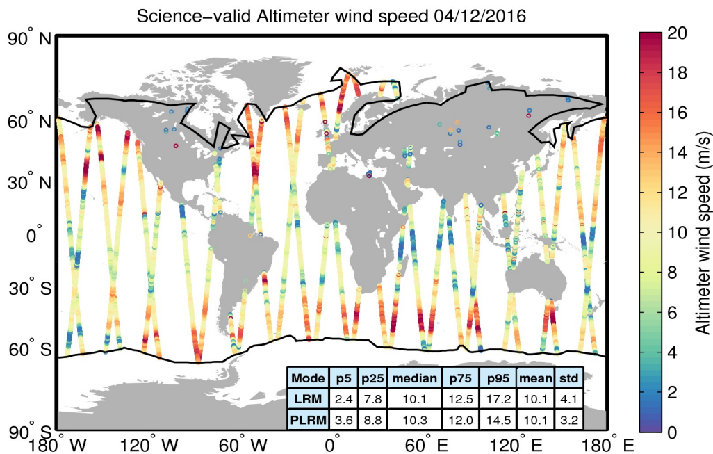
Figure 34. Geographical distribution of science-valid wind data over oceans and lakes for 04/12/2016. The statistical values shown in the table refer to the wind in m/s and are calculated separately for LRM and PLRM regions. The black lines mark the outer limit of the Arctic and Antarctic polar polygons. Gray circles denote records that have been rejected based on the editing criteria described in Table 5.
