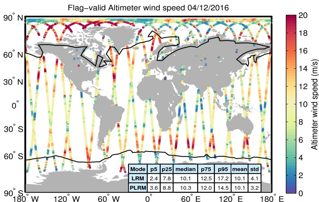
Figure 31. Geographical distribution of flag-valid wind data over oceans and lakes for 04/12/2016. The statistical values shown in the table refer to the wind in m/s and are calculated separately for LRM and PLRM regions. Measurements taken over polar polygons have been excluded from the computation of the statistical values. The black lines mark the outer limit of the Arctic and Antarctic polar polygons.
