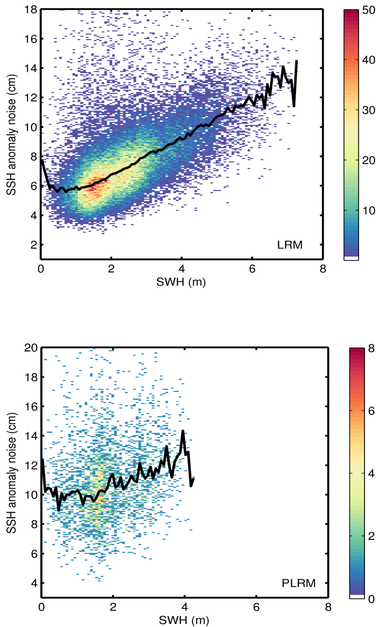
Figure 9. 2D histogram showing flag-valid SSH anomaly noise as a function of SWH for LRM (top) and PLRM (bottom) for 04/12/2016. The black line denotes the median SSH anomaly noise as a function of SWH.
