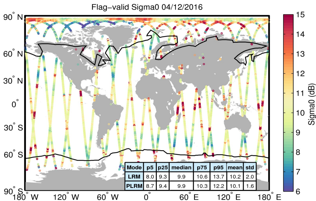
Figure 23. Geographical distribution of flag-valid sigma0 data over oceans and lakes for 04/12/2016. The statistical values shown in the table refer to the sigma0 in dB and are calculated separately for LRM and PLRM regions. Measurements taken over polar polygons have been excluded from the computation of the statistical values. The black lines mark the outer limit of the Arctic and Antarctic polar polygons.
