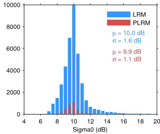
Figure 28. Histogram of science-valid sigma0 over oceans and lakes for LRM (blue) and PLRM (red) for 04/12/2016. The mean ( \mu ) and standard deviation ( \sigma ) are also shown. Note that values outside [4 20] dB are excluded from the histogram for the sake of readability but not from the computation of \mu and \sigma .
