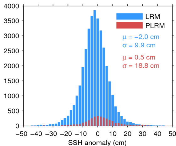
Figure 11. Histogram of science-valid SSH anomaly over oceans and lakes for LRM (blue) and PLRM (red) for 04/12/2016. The mean ( \mu ) and standard deviation ( \sigma ) are also shown. Note that values outside [-50 50] cm are excluded from the histogram for the sake of readability but not from the computation of \mu and \sigma .
