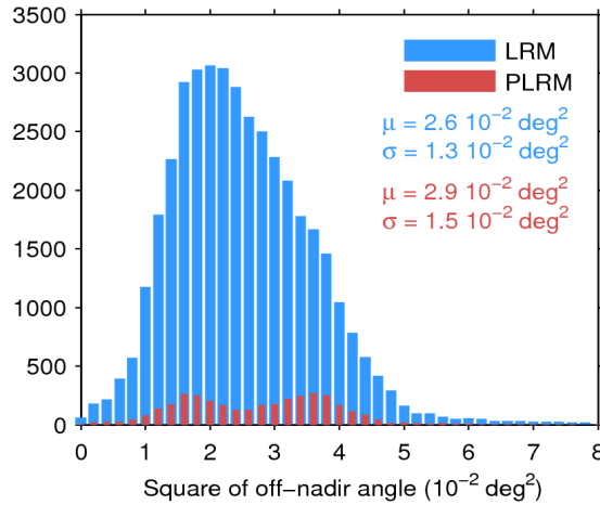
Figure 39. Histogram of flag-valid mispointing over oceans and lakes for LRM (blue) and PLRM (red) for 04/12/2016. Only positive values have been considered. The mean ( \mu ) and standard deviation ( \sigma ) are also shown. Note that values larger than 8 \cdot 10^{-2} \text{ deg}^2 are excluded from the histogram for the sake of readability but not from the computation of \mu and \sigma .
