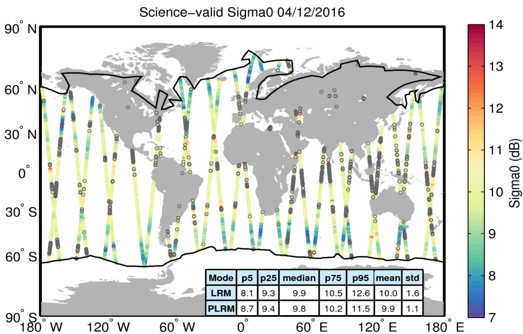
Figure 27. Geographical distribution of science-valid sigma0 data over oceans and lakes for 04/12/2016. The statistical values shown in the table refer to the sigma0 in dB and are calculated separately for LRM and PLRM regions. The black lines mark the outer limit of the Arctic and Antarctic polar polygons. Gray circles denote records that have been rejected based on the editing criteria described in Table 4.
