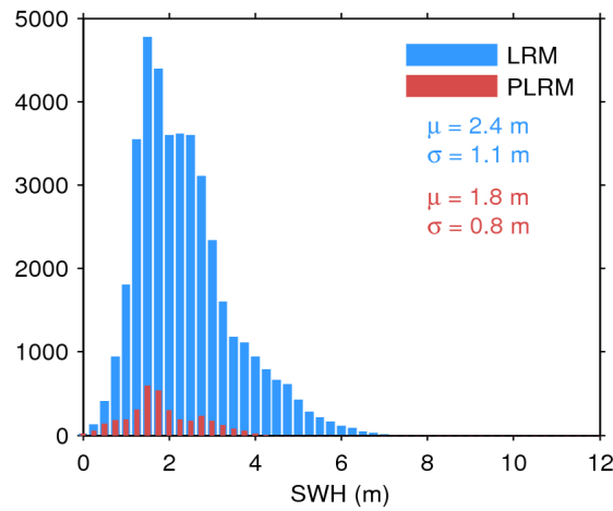
Figure 20. Histogram of science-valid SWH over oceans and lakes for LRM (blue) and PLRM (red) for 04/12/2016. The mean ( \mu ) and standard deviation ( \sigma ) are also shown. Note that values larger than 12 m are excluded from the histogram for the sake of readability but not from the computation of \mu and \sigma .
