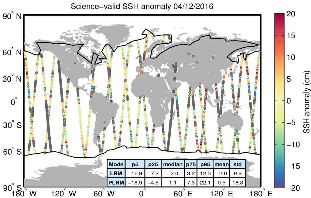
Figure 10. Geographical distribution of science-valid SSH anomaly data over oceans and lakes for 04/12/2016. The statistical values shown in the table refer to the SSH anomaly in cm and are calculated separately for LRM and PLRM regions. The black lines mark the outer limit of the Arctic and Antarctic polar polygons. Gray circles denote records that have been rejected based on the editing criteria described in Table 2.
