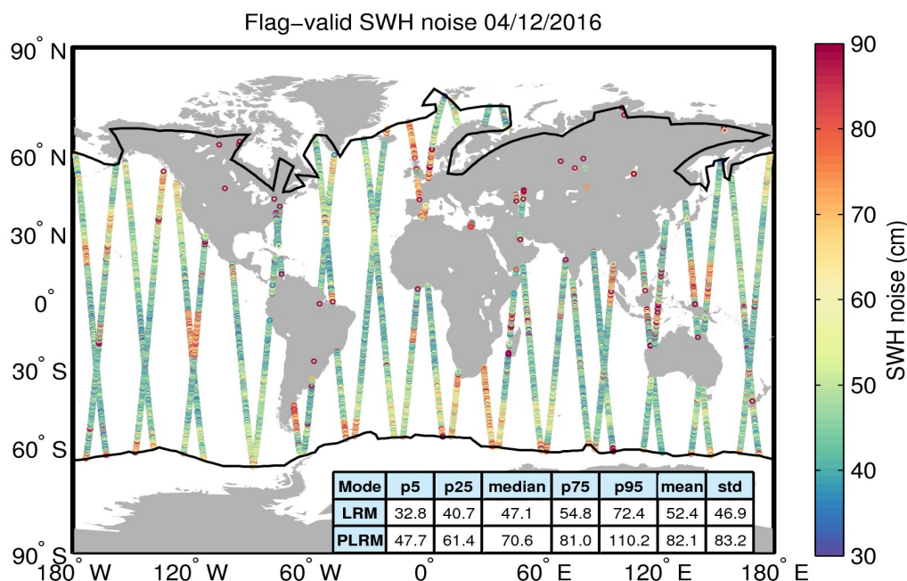
Figure 18. Geographical distribution of flag-valid 20-Hz SWH measurement noise over oceans and lakes for 04/12/2016. The statistical values shown in the table refer to the SWH noise and are calculated separately for LRM and PLRM regions. Measurements taken over polar polygons have been excluded from the computation of the statistical values. The black lines mark the outer limit of the Arctic and Antarctic polar polygons.
