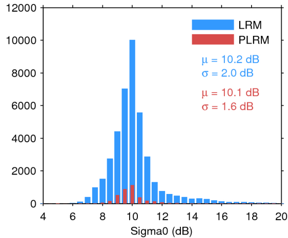
Figure 25. Histogram of flag-valid sigma0 over oceans and lakes for LRM (blue) and PLRM (red) for 04/12/2016. The mean ( \mu ) and standard deviation ( \sigma ) are also shown. Note that values outside [4 20] dB are excluded from the histogram for the sake of readability but not from the computation of \mu and \sigma .
