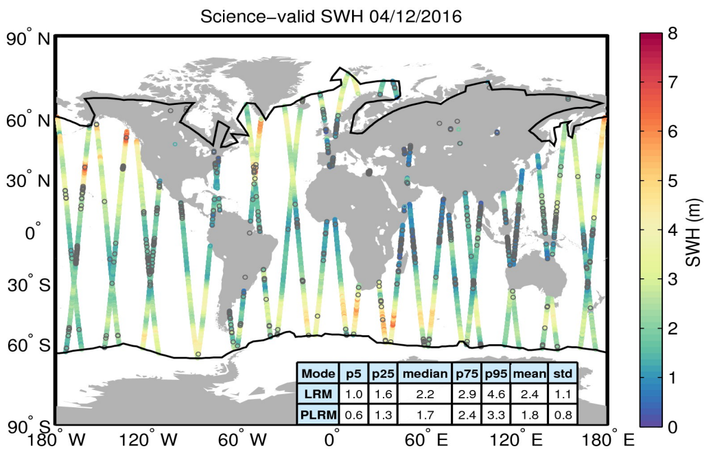
Figure 19. Geographical distribution of science-valid SWH data over oceans and lakes for 04/12/2016. The statistical values shown in the table refer to the SWH in m and are calculated separately for LRM and PLRM regions. The black lines mark the outer limit of the Arctic and Antarctic polar polygons. Gray circles denote records that have been rejected based on the editing criteria described in Table 3.
