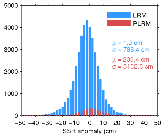
Figure 7. Histogram of flag-valid SSH anomaly over oceans and lakes for LRM (blue) and PLRM (red) for 04/12/2016. The mean ( \mu ) and standard deviation ( \sigma ) are also shown. Note that values outside [-50\ 50] cm are excluded from the histogram for the sake of readability but not from the computation of \mu and \sigma .
