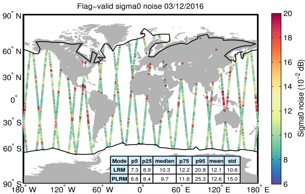
Figure 26. Geographical distribution of flag-valid 20-Hz sigma0 measurement noise over oceans and lakes for 03/12/2016. The statistical values shown in the table refer to the sigma0 noise and are calculated separately for LRM and PLRM regions. Measurements taken over polar polygons have been excluded from the computation of the statistical values. The black lines mark the outer limit of the Arctic and Antarctic polar polygons.
