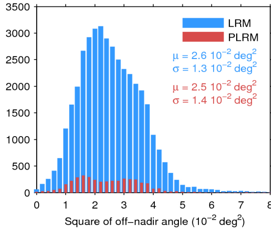
Figure 39. Histogram of flag-valid mispointing over oceans and lakes for LRM (blue) and PLRM (red) for 03/12/2016. Only positive values have been considered. The mean ( \mu ) and standard deviation ( \sigma ) are also shown. Note that values larger than 8 \cdot 10^{-2} \text{ deg}^2 are excluded from the histogram for the sake of readability but not from the computation of \mu and \sigma .
