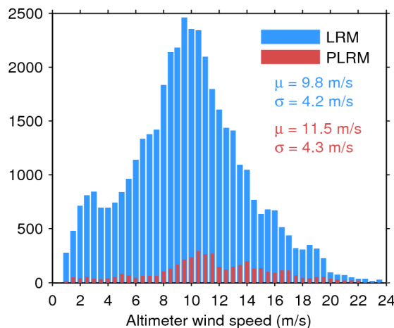
Figure 35. Histogram of science-valid wind over oceans and lakes for LRM (blue) and PLRM (red) for 03/12/2016. The mean ( \mu ) and standard deviation ( \sigma ) are also shown. Note that values larger than 24 m/s are excluded from the histogram for the sake of readability but not from the computation of \mu and \sigma .
