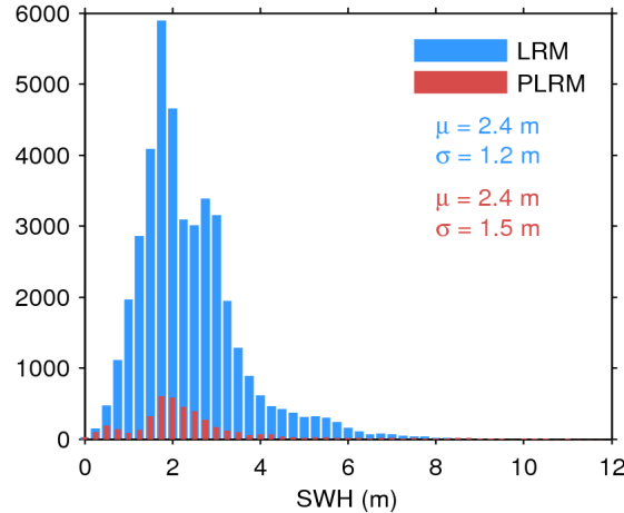
Figure 17. Histogram of flag-valid SWH over oceans and lakes for LRM (blue) and PLRM (red) for 03/12/2016. The mean ( \mu ) and standard deviation ( \sigma ) are also shown. Note that values larger than 12 m are excluded from the histogram for the sake of readability but not from the computation of \mu and \sigma .
