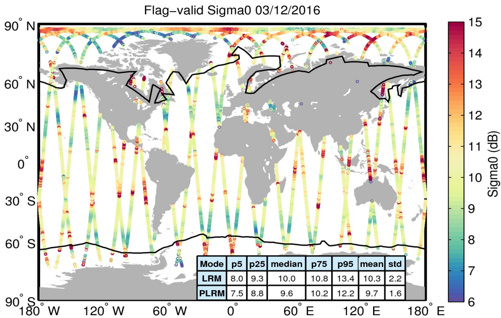
Figure 23. Geographical distribution of flag-valid sigma0 data over oceans and lakes for 03/12/2016. The statistical values shown in the table refer to the sigma0 in dB and are calculated separately for LRM and PLRM regions. Measurements taken over polar polygons have been excluded from the computation of the statistical values. The black lines mark the outer limit of the Arctic and Antarctic polar polygons.
