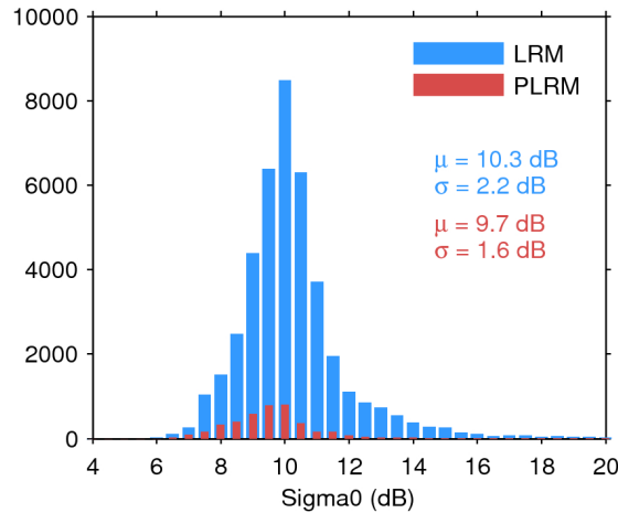
Figure 25. Histogram of flag-valid sigma0 over oceans and lakes for LRM (blue) and PLRM (red) for 03/12/2016. The mean ( \mu ) and standard deviation ( \sigma ) are also shown. Note that values outside [4 20] dB are excluded from the histogram for the sake of readability but not from the computation of \mu and \sigma .
