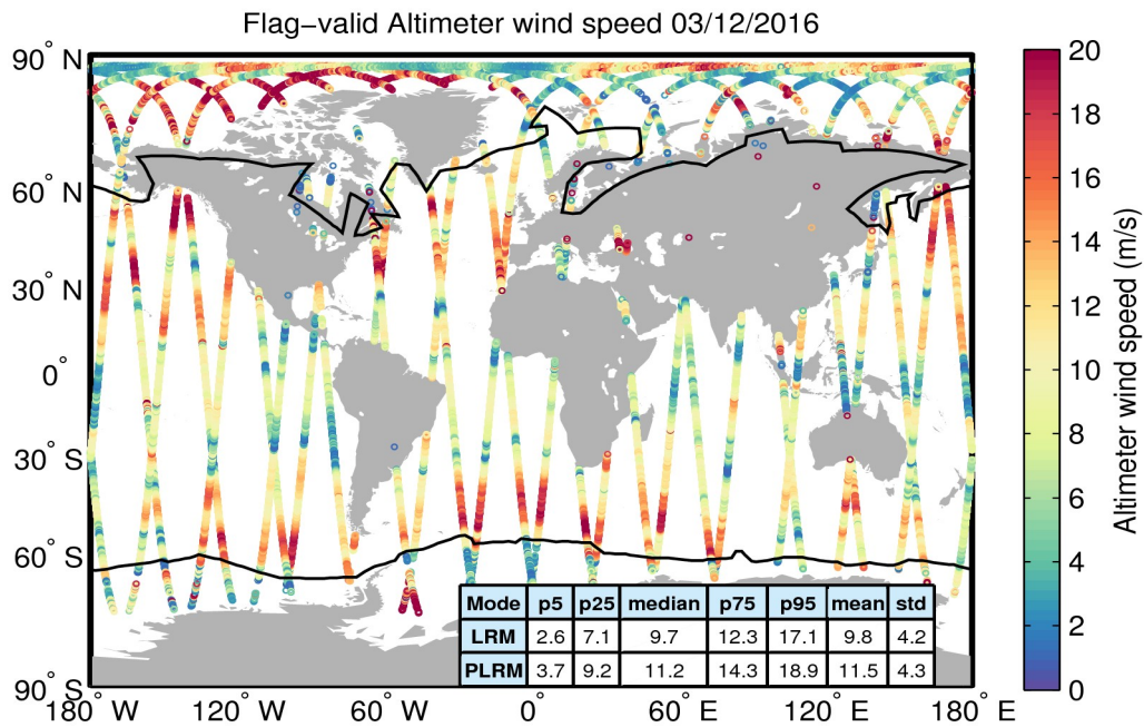
Figure 31. Geographical distribution of flag-valid wind data over oceans and lakes for 03/12/2016. The statistical values shown in the table refer to the wind in m/s and are calculated separately for LRM and PLRM regions. Measurements taken over polar polygons have been excluded from the computation of the statistical values. The black lines mark the outer limit of the Arctic and Antarctic polar polygons.
