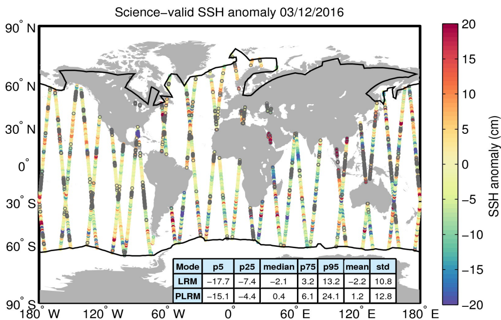
Figure 10. Geographical distribution of science-valid SSH anomaly data over oceans and lakes for 03/12/2016. The statistical values shown in the table refer to the SSH anomaly in cm and are calculated separately for LRM and PLRM regions. The black lines mark the outer limit of the Arctic and Antarctic polar polygons. Gray circles denote records that have been rejected based on the editing criteria described in Table 2.
