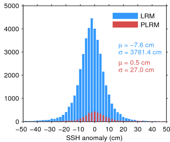
Figure 7. Histogram of flag-valid SSH anomaly over oceans and lakes for LRM (blue) and PLRM (red) for 03/12/2016. The mean ( \mu ) and standard deviation ( \sigma ) are also shown. Note that values outside [-50\ 50] cm are excluded from the histogram for the sake of readability but not from the computation of \mu and \sigma .
