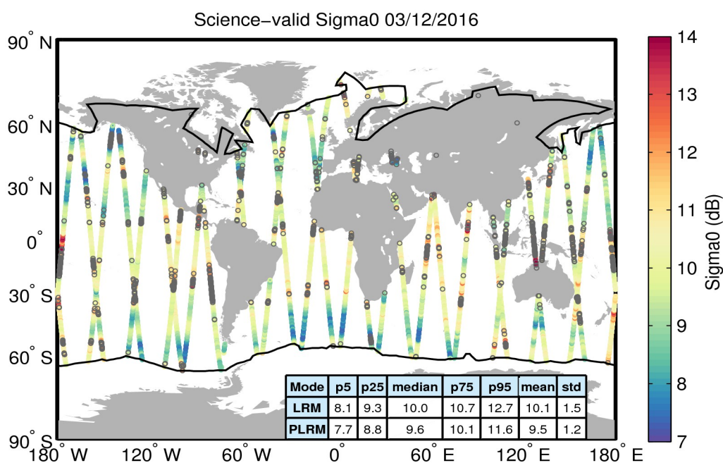
Figure 27. Geographical distribution of science-valid sigma0 data over oceans and lakes for 03/12/2016. The statistical values shown in the table refer to the sigma0 in dB and are calculated separately for LRM and PLRM regions. The black lines mark the outer limit of the Arctic and Antarctic polar polygons. Gray circles denote records that have been rejected based on the editing criteria described in Table 4.
