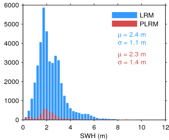
Figure 20. Histogram of science-valid SWH over oceans and lakes for LRM (blue) and PLRM (red) for 03/12/2016. The mean ( \mu ) and standard deviation ( \sigma ) are also shown. Note that values larger than 12 m are excluded from the histogram for the sake of readability but not from the computation of \mu and \sigma .
