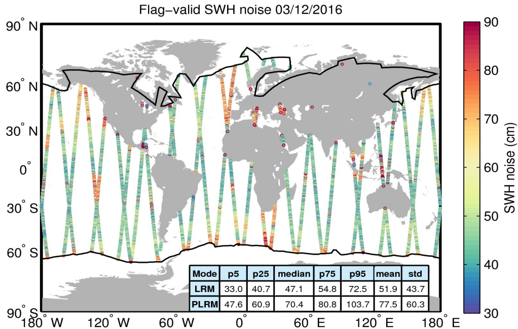
Figure 18. Geographical distribution of flag-valid 20-Hz SWH measurement noise over oceans and lakes for 03/12/2016. The statistical values shown in the table refer to the SWH noise and are calculated separately for LRM and PLRM regions. Measurements taken over polar polygons have been excluded from the computation of the statistical values. The black lines mark the outer limit of the Arctic and Antarctic polar polygons.
