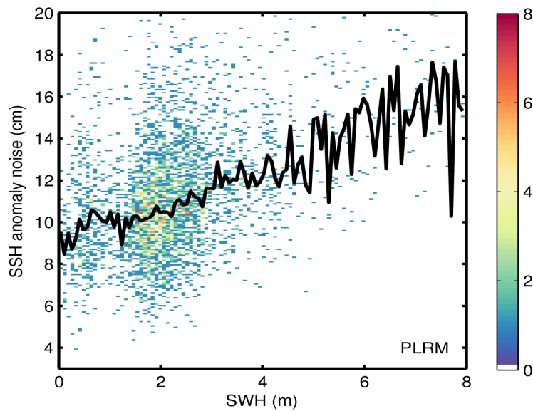
Figure 9. 2D histogram showing flag-valid SSH anomaly noise as a function of SWH for LRM (top) and PLRM (bottom) for 03/12/2016. The black line denotes the median SSH anomaly noise as a function of SWH.
