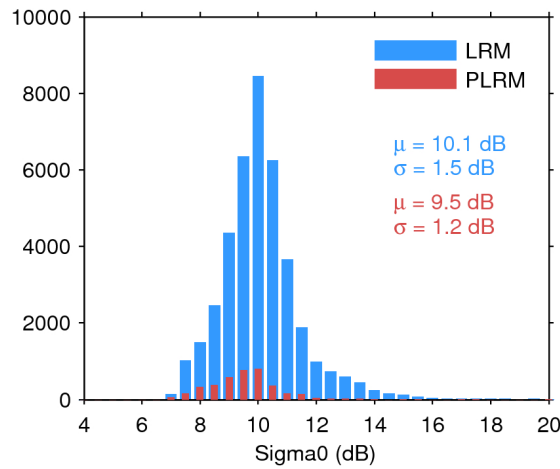
Figure 28. Histogram of science-valid sigma0 over oceans and lakes for LRM (blue) and PLRM (red) for 03/12/2016. The mean ( \mu ) and standard deviation ( \sigma ) are also shown. Note that values outside [4 20] dB are excluded from the histogram for the sake of readability but not from the computation of \mu and \sigma .
