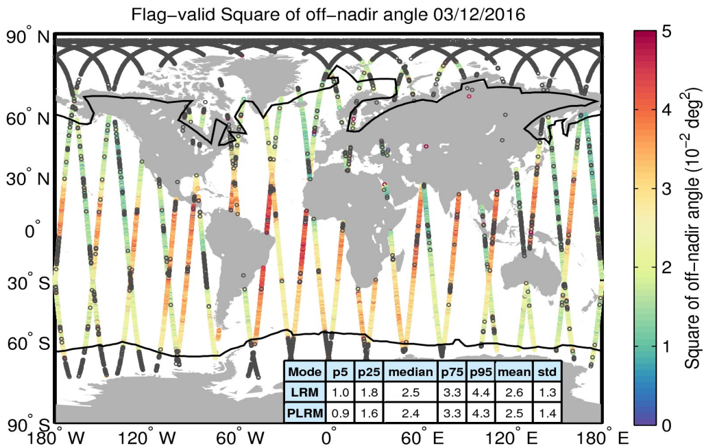
Figure 37. Geographical distribution of flag-valid mispointing data over oceans and lakes for 03/12/2016. The statistical values shown in the table refer to the mispointing in 10^{-2} deg 2 and are calculated separately for LRM and PLRM regions. Measurements taken over polar polygons have been excluded from the computation of the statistical values. The black lines mark the outer limit of the Arctic and Antarctic polar polygons. Gray circles denote negative values.
