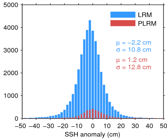
Figure 11. Histogram of science-valid SSH anomaly over oceans and lakes for LRM (blue) and PLRM (red) for 03/12/2016. The mean ( \mu ) and standard deviation ( \sigma ) are also shown. Note that values outside [-50\ 50] cm are excluded from the histogram for the sake of readability but not from the computation of \mu and \sigma .
