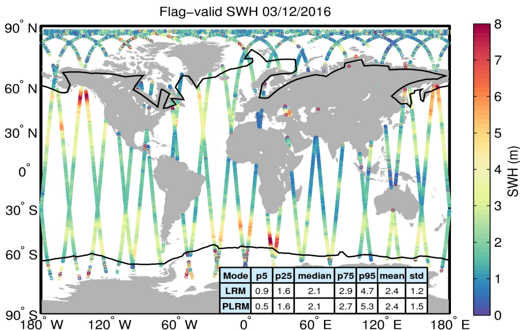
Figure 15. Geographical distribution of flag-valid SWH data over oceans and lakes for 03/12/2016. The statistical values shown in the table refer to the SWH in m and are calculated separately for LRM and PLRM regions. Measurements taken over polar polygons have been excluded from the computation of the statistical values. The black lines mark the outer limit of the Arctic and Antarctic polar polygons.
