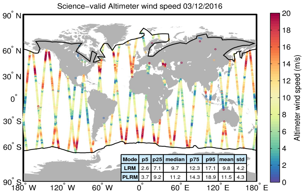
Figure 34. Geographical distribution of science-valid wind data over oceans and lakes for 03/12/2016. The statistical values shown in the table refer to the wind in m/s and are calculated separately for LRM and PLRM regions. The black lines mark the outer limit of the Arctic and Antarctic polar polygons. Gray circles denote records that have been rejected based on the editing criteria described in Table 5.
