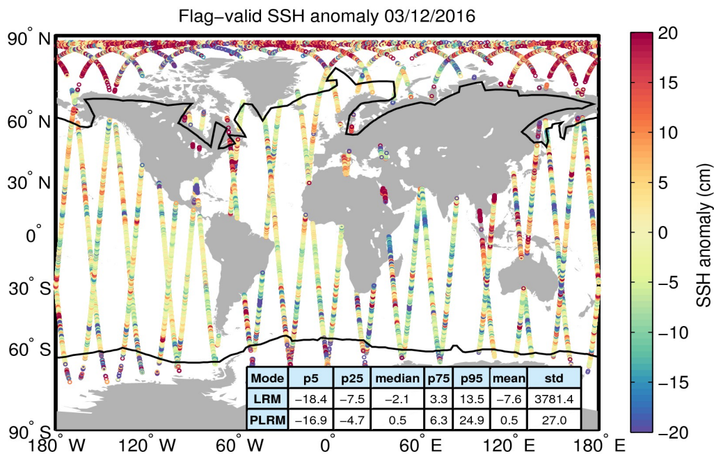
Figure 5. Geographical distribution of flag-valid 1-Hz SSH anomaly data over oceans and lakes for 03/12/2016. The statistical values shown in the table refer to the SSH anomaly in cm and are calculated separately for LRM and PLRM regions. Measurements taken over polar polygons have been excluded from the computation of the statistical values. The black lines mark the outer limit of the Arctic and Antarctic polar polygons.
