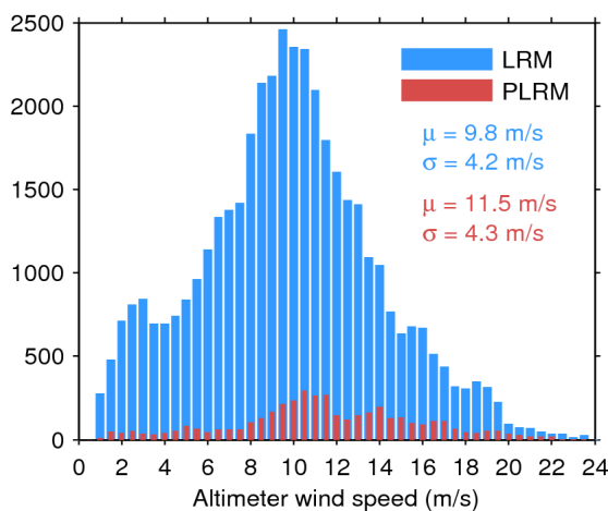
Figure 33. Histogram of flag-valid wind over oceans and lakes for LRM (blue) and PLRM (red) for 03/12/2016. The mean ( \mu ) and standard deviation ( \sigma ) are also shown. Note that values larger than 24 m/s are excluded from the histogram for the sake of readability but not from the computation of \mu and \sigma .
