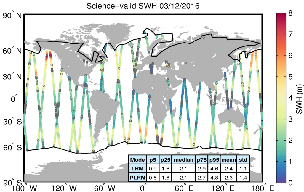
Figure 19. Geographical distribution of science-valid SWH data over oceans and lakes for 03/12/2016. The statistical values shown in the table refer to the SWH in m and are calculated separately for LRM and PLRM regions. The black lines mark the outer limit of the Arctic and Antarctic polar polygons. Gray circles denote records that have been rejected based on the editing criteria described in Table 3.
