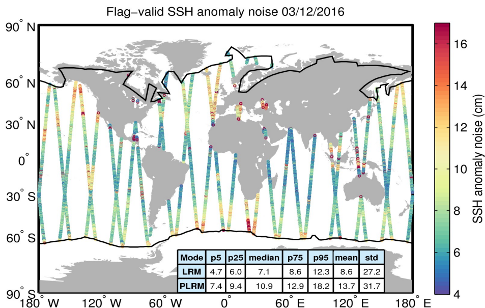
Figure 8. Geographical distribution of flag-valid 20-Hz SSH anomaly measurement noise over oceans and lakes for 03/12/2016. The statistical values shown in the table refer to the SSH anomaly noise and are calculated separately for LRM and PLRM regions. Measurements taken over polar polygons have been excluded from the computation of the statistical values. The black lines mark the outer limit of the Arctic and Antarctic polar polygons.
