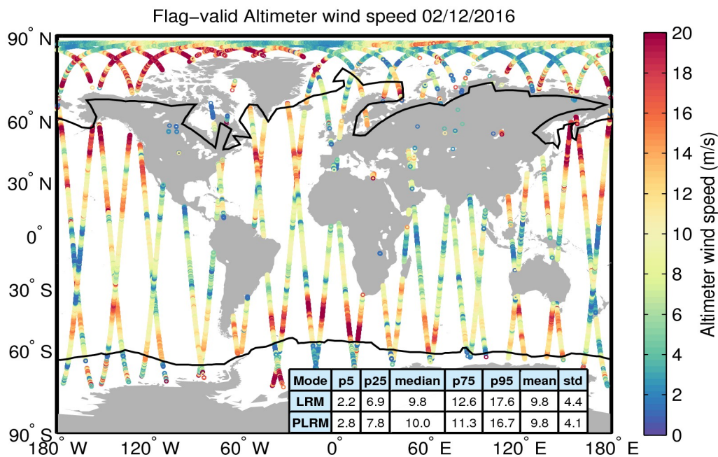
Figure 31. Geographical distribution of flag-valid wind data over oceans and lakes for 02/12/2016. The statistical values shown in the table refer to the wind in m/s and are calculated separately for LRM and PLRM regions. Measurements taken over polar polygons have been excluded from the computation of the statistical values. The black lines mark the outer limit of the Arctic and Antarctic polar polygons.
