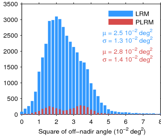
Figure 39. Histogram of flag-valid mispointing over oceans and lakes for LRM (blue) and PLRM (red) for 02/12/2016. Only positive values have been considered. The mean ( \mu ) and standard deviation ( \sigma ) are also shown. Note that values larger than 8 \cdot 10^{-2} \text{ deg}^2 are excluded from the histogram for the sake of readability but not from the computation of \mu and \sigma .
