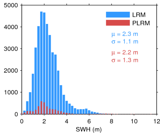
Figure 17. Histogram of flag-valid SWH over oceans and lakes for LRM (blue) and PLRM (red) for 02/12/2016. The mean ( \mu ) and standard deviation ( \sigma ) are also shown. Note that values larger than 12 m are excluded from the histogram for the sake of readability but not from the computation of \mu and \sigma .
