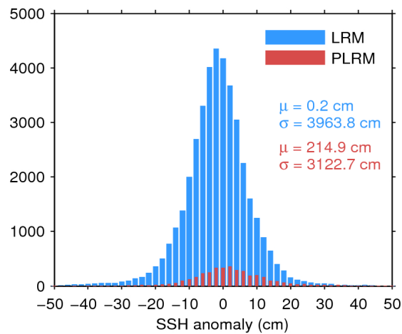
Figure 7. Histogram of flag-valid SSH anomaly over oceans and lakes for LRM (blue) and PLRM (red) for 02/12/2016. The mean ( \mu ) and standard deviation ( \sigma ) are also shown. Note that values outside [-50\ 50] cm are excluded from the histogram for the sake of readability but not from the computation of \mu and \sigma .
