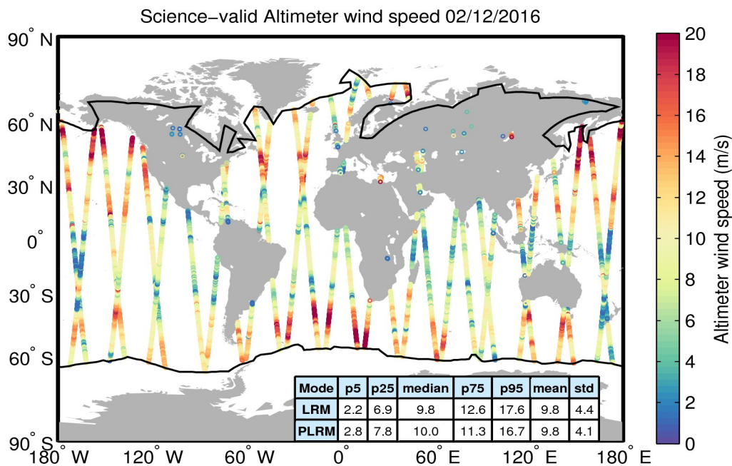
Figure 34. Geographical distribution of science-valid wind data over oceans and lakes for 02/12/2016. The statistical values shown in the table refer to the wind in m/s and are calculated separately for LRM and PLRM regions. The black lines mark the outer limit of the Arctic and Antarctic polar polygons. Gray circles denote records that have been rejected based on the editing criteria described in Table 5.
