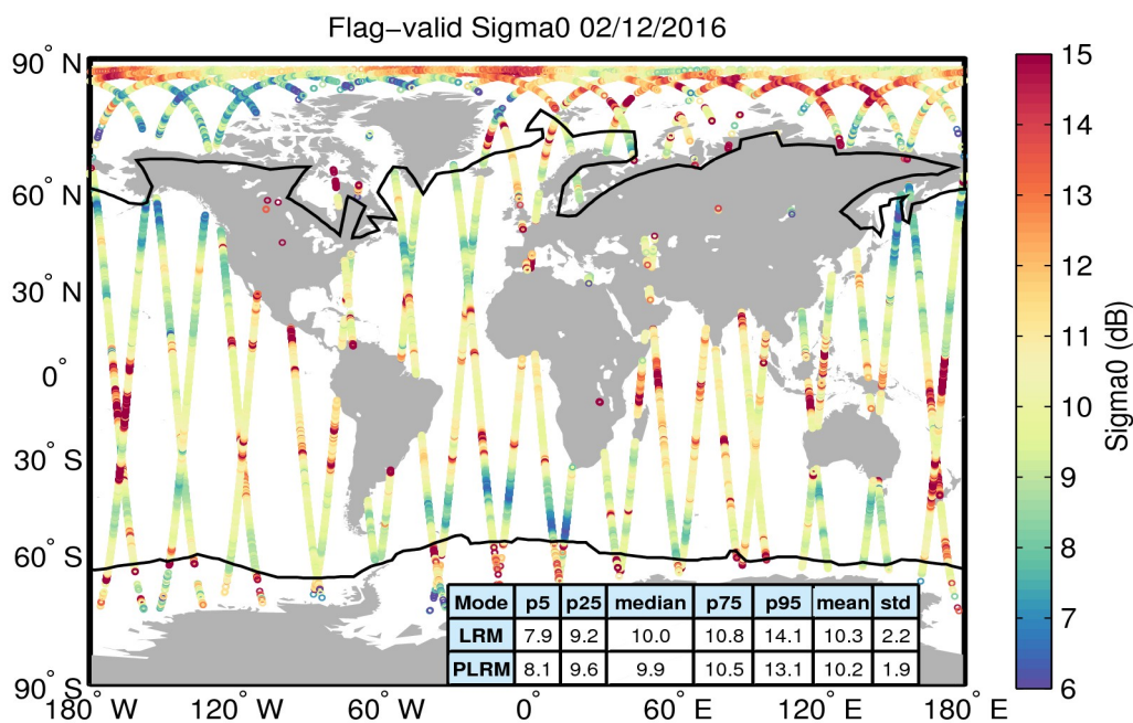
Figure 23. Geographical distribution of flag-valid sigma0 data over oceans and lakes for 02/12/2016. The statistical values shown in the table refer to the sigma0 in dB and are calculated separately for LRM and PLRM regions. Measurements taken over polar polygons have been excluded from the computation of the statistical values. The black lines mark the outer limit of the Arctic and Antarctic polar polygons.
