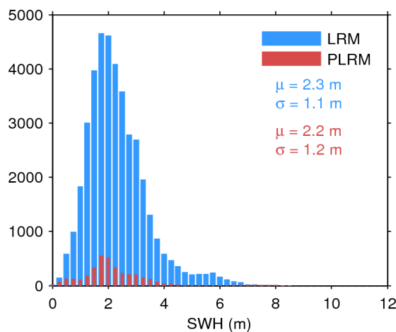
Figure 20. Histogram of science-valid SWH over oceans and lakes for LRM (blue) and PLRM (red) for 02/12/2016. The mean ( \mu ) and standard deviation ( \sigma ) are also shown. Note that values larger than 12 m are excluded from the histogram for the sake of readability but not from the computation of \mu and \sigma .
