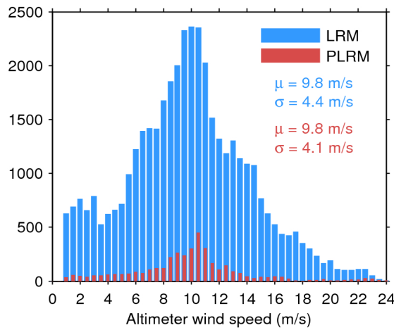
Figure 33. Histogram of flag-valid wind over oceans and lakes for LRM (blue) and PLRM (red) for 02/12/2016. The mean ( \mu ) and standard deviation ( \sigma ) are also shown. Note that values larger than 24 m/s are excluded from the histogram for the sake of readability but not from the computation of \mu and \sigma .
