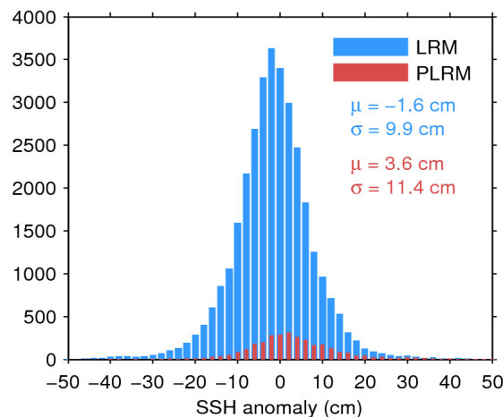
Figure 11. Histogram of science-valid SSH anomaly over oceans and lakes for LRM (blue) and PLRM (red) for 02/12/2016. The mean ( \mu ) and standard deviation ( \sigma ) are also shown. Note that values outside [-50 50] cm are excluded from the histogram for the sake of readability but not from the computation of \mu and \sigma .
