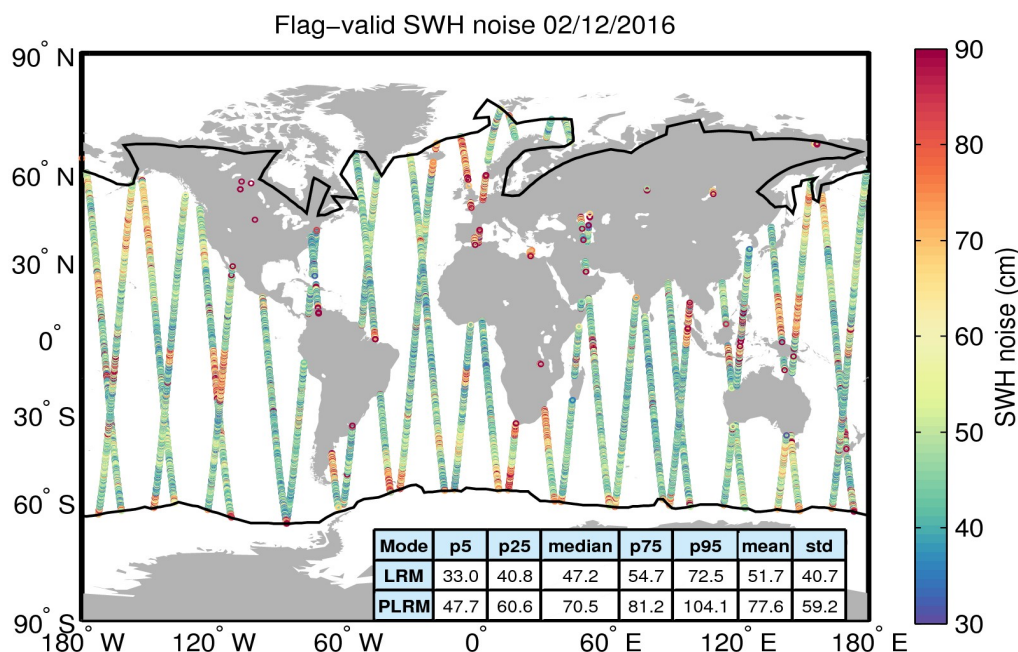
Figure 18. Geographical distribution of flag-valid 20-Hz SWH measurement noise over oceans and lakes for 02/12/2016. The statistical values shown in the table refer to the SWH noise and are calculated separately for LRM and PLRM regions. Measurements taken over polar polygons have been excluded from the computation of the statistical values. The black lines mark the outer limit of the Arctic and Antarctic polar polygons.
