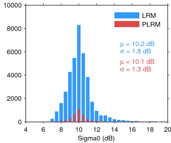
Figure 28. Histogram of science-valid sigma0 over oceans and lakes for LRM (blue) and PLRM (red) for 02/12/2016. The mean ( \mu ) and standard deviation ( \sigma ) are also shown. Note that values outside [4 20] dB are excluded from the histogram for the sake of readability but not from the computation of \mu and \sigma .
