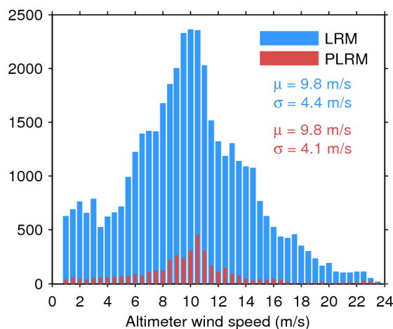
Figure 35. Histogram of science-valid wind over oceans and lakes for LRM (blue) and PLRM (red) for 02/12/2016. The mean ( \mu ) and standard deviation ( \sigma ) are also shown. Note that values larger than 24 m/s are excluded from the histogram for the sake of readability but not from the computation of \mu and \sigma .
