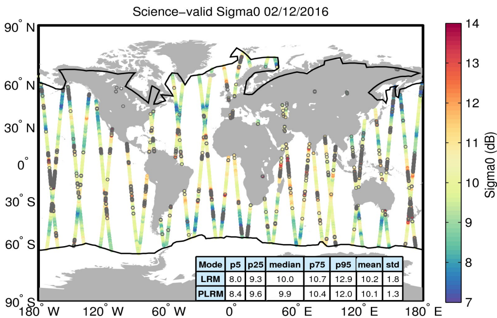
Figure 27. Geographical distribution of science-valid sigma0 data over oceans and lakes for 02/12/2016. The statistical values shown in the table refer to the sigma0 in dB and are calculated separately for LRM and PLRM regions. The black lines mark the outer limit of the Arctic and Antarctic polar polygons. Gray circles denote records that have been rejected based on the editing criteria described in Table 4.
