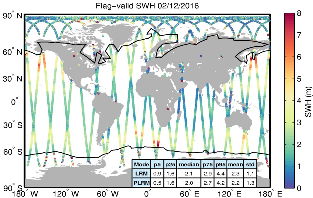
Figure 15. Geographical distribution of flag-valid SWH data over oceans and lakes for 02/12/2016. The statistical values shown in the table refer to the SWH in m and are calculated separately for LRM and PLRM regions. Measurements taken over polar polygons have been excluded from the computation of the statistical values. The black lines mark the outer limit of the Arctic and Antarctic polar polygons.
