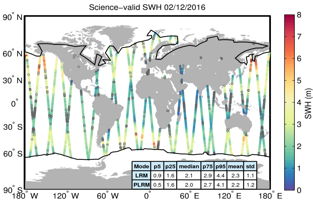
Figure 19. Geographical distribution of science-valid SWH data over oceans and lakes for 02/12/2016. The statistical values shown in the table refer to the SWH in m and are calculated separately for LRM and PLRM regions. The black lines mark the outer limit of the Arctic and Antarctic polar polygons. Gray circles denote records that have been rejected based on the editing criteria described in Table 3.
