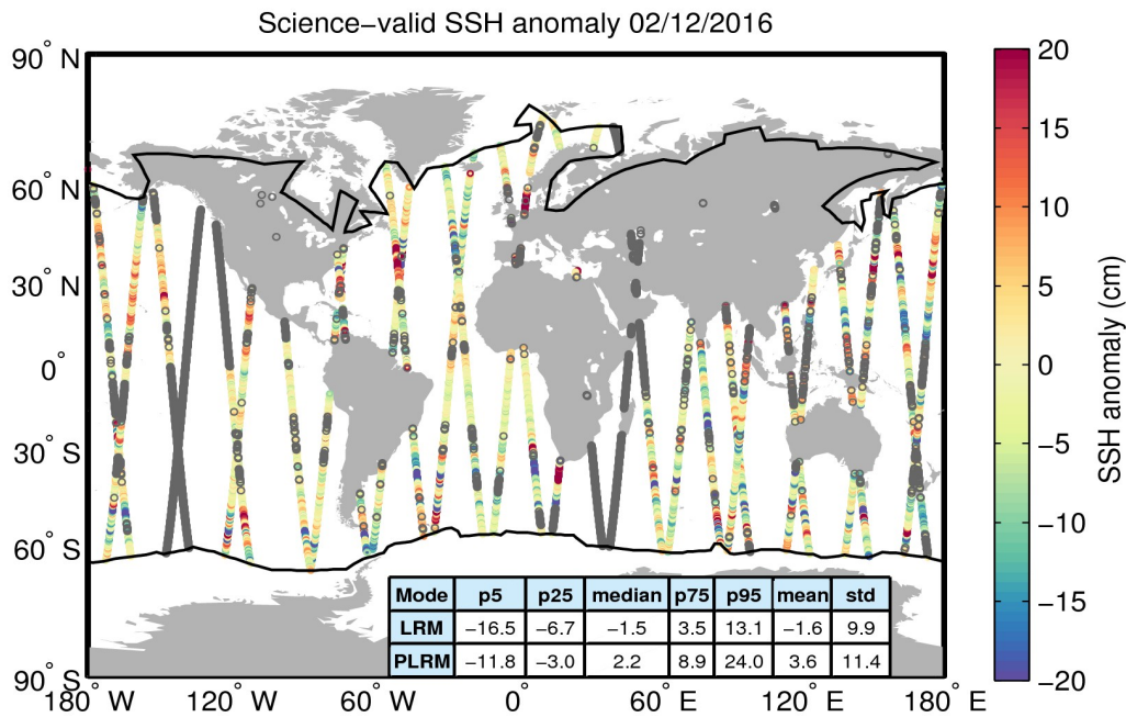
Figure 10. Geographical distribution of science-valid SSH anomaly data over oceans and lakes for 02/12/2016. The statistical values shown in the table refer to the SSH anomaly in cm and are calculated separately for LRM and PLRM regions. The black lines mark the outer limit of the Arctic and Antarctic polar polygons. Gray circles denote records that have been rejected based on the editing criteria described in Table 2.
