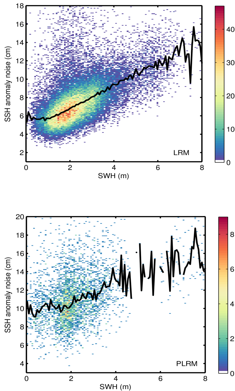
Figure 9. 2D histogram showing flag-valid SSH anomaly noise as a function of SWH for LRM (top) and PLRM (bottom) for 02/12/2016. The black line denotes the median SSH anomaly noise as a function of SWH.
