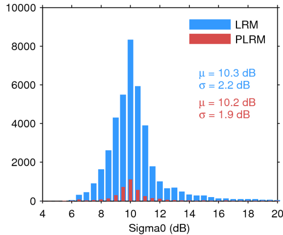
Figure 25. Histogram of flag-valid sigma0 over oceans and lakes for LRM (blue) and PLRM (red) for 02/12/2016. The mean ( \mu ) and standard deviation ( \sigma ) are also shown. Note that values outside [4 20] dB are excluded from the histogram for the sake of readability but not from the computation of \mu and \sigma .
